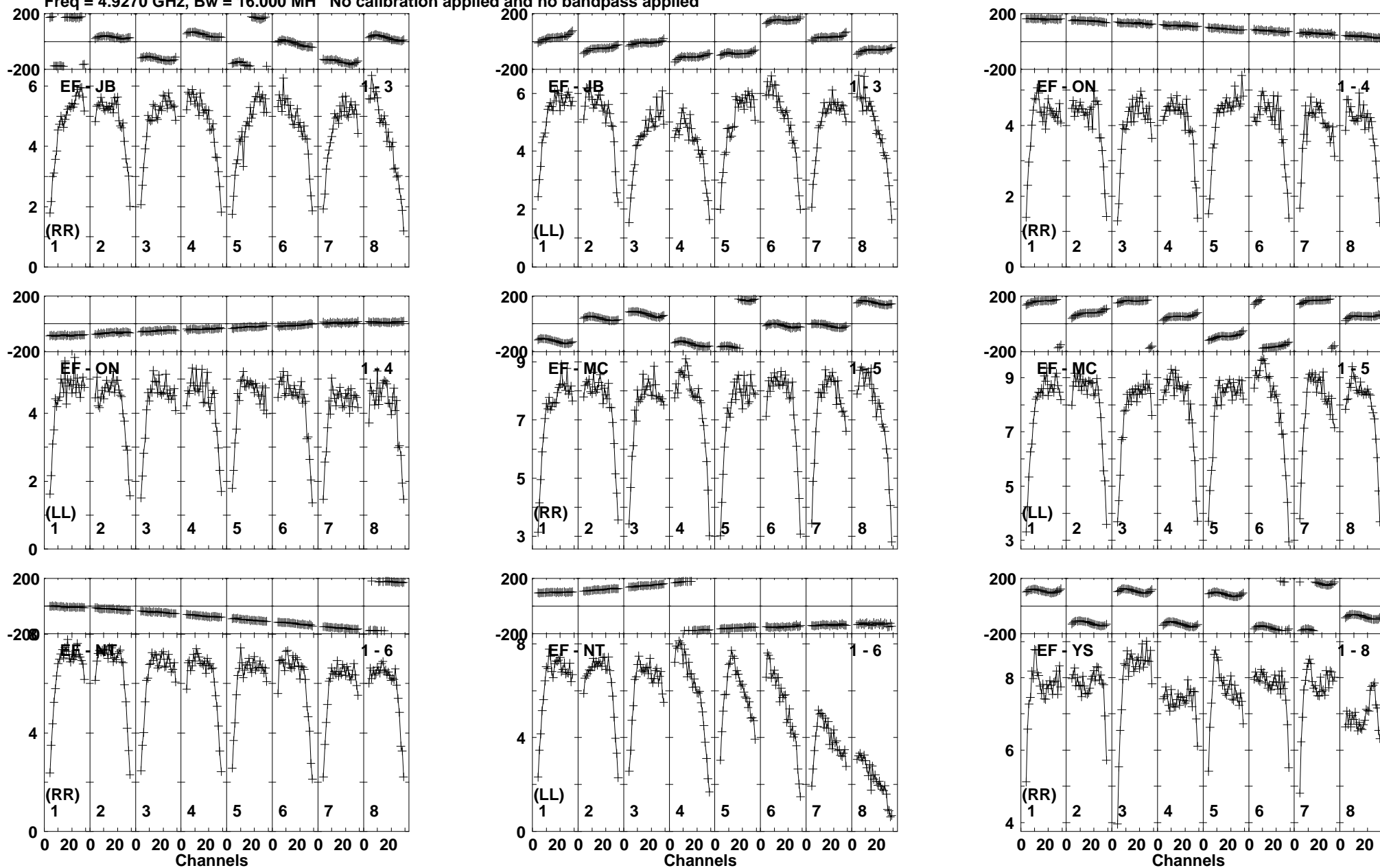
Lower frame: Milli Ampl Jy Top frame: Phas deg Vector averaged cross-power spectrum Baseline: EF (01) - JB (03) Timerange: 00/16:29:20 to 00/16:30:39
