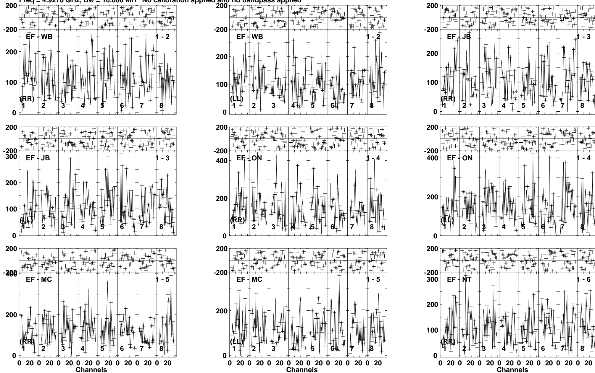
Lower frame: Micro Ampl Jy Top frame: Phas deg Vector averaged cross-power spectrum Baseline: EF (01) - WB (02) Timerange: 00/11:13:03 to 00/11:16:42
