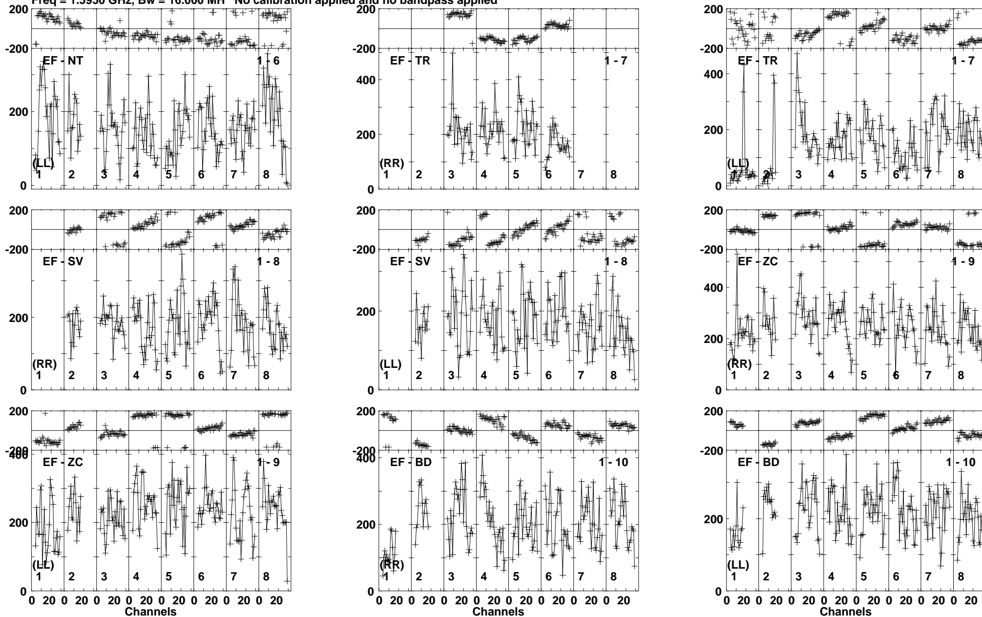
Lower frame: Micro Ampl Jy Top frame: Phas deg Vector averaged cross-power spectrum Baseline: EF (01) - NT (06) Timerange: 00/23:14:59 to 00/23:18:29
