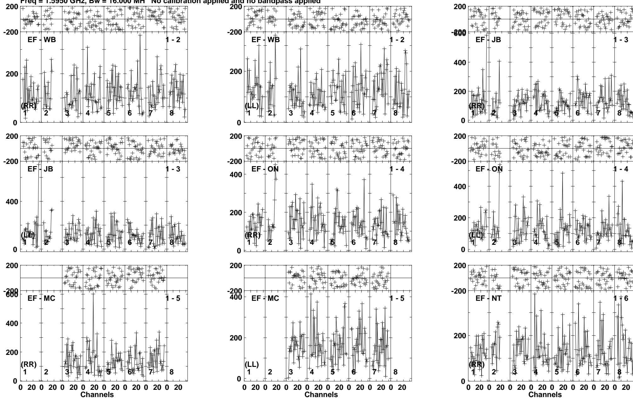
Lower frame: Micro Ampl Jy Top frame: Phas deg Vector averaged cross-power spectrum Baseline: EF (01) - WB (02) Timerange: 01/06:24:36 to 01/06:28:04
