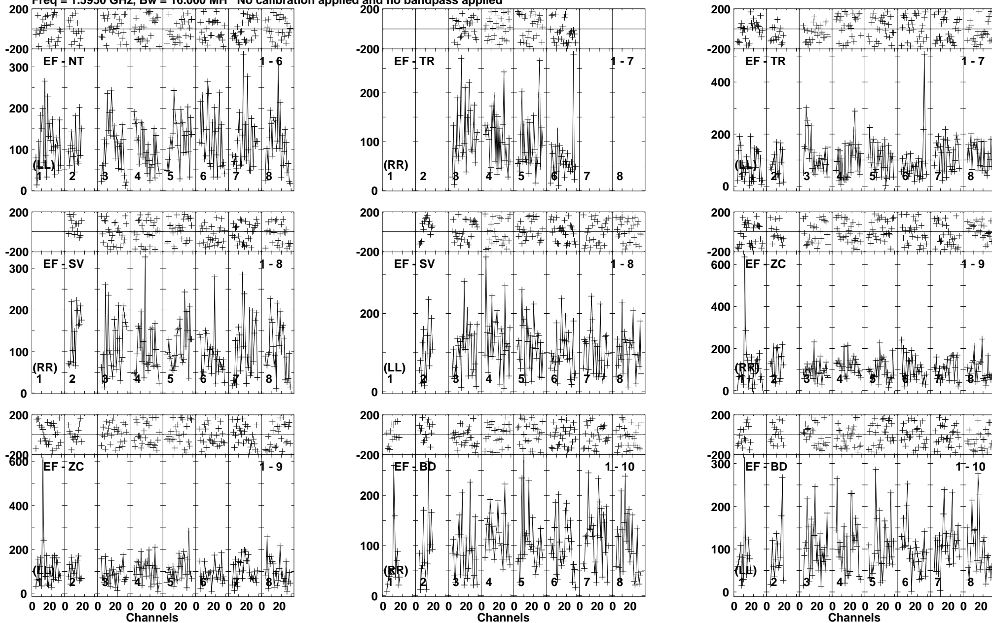
Lower frame: Micro Ampl Jy Top frame: Phas deg Vector averaged cross-power spectrum Baseline: EF (01) - NT (06) Timerange: 01/00:02:11 to 01/00:05:49
