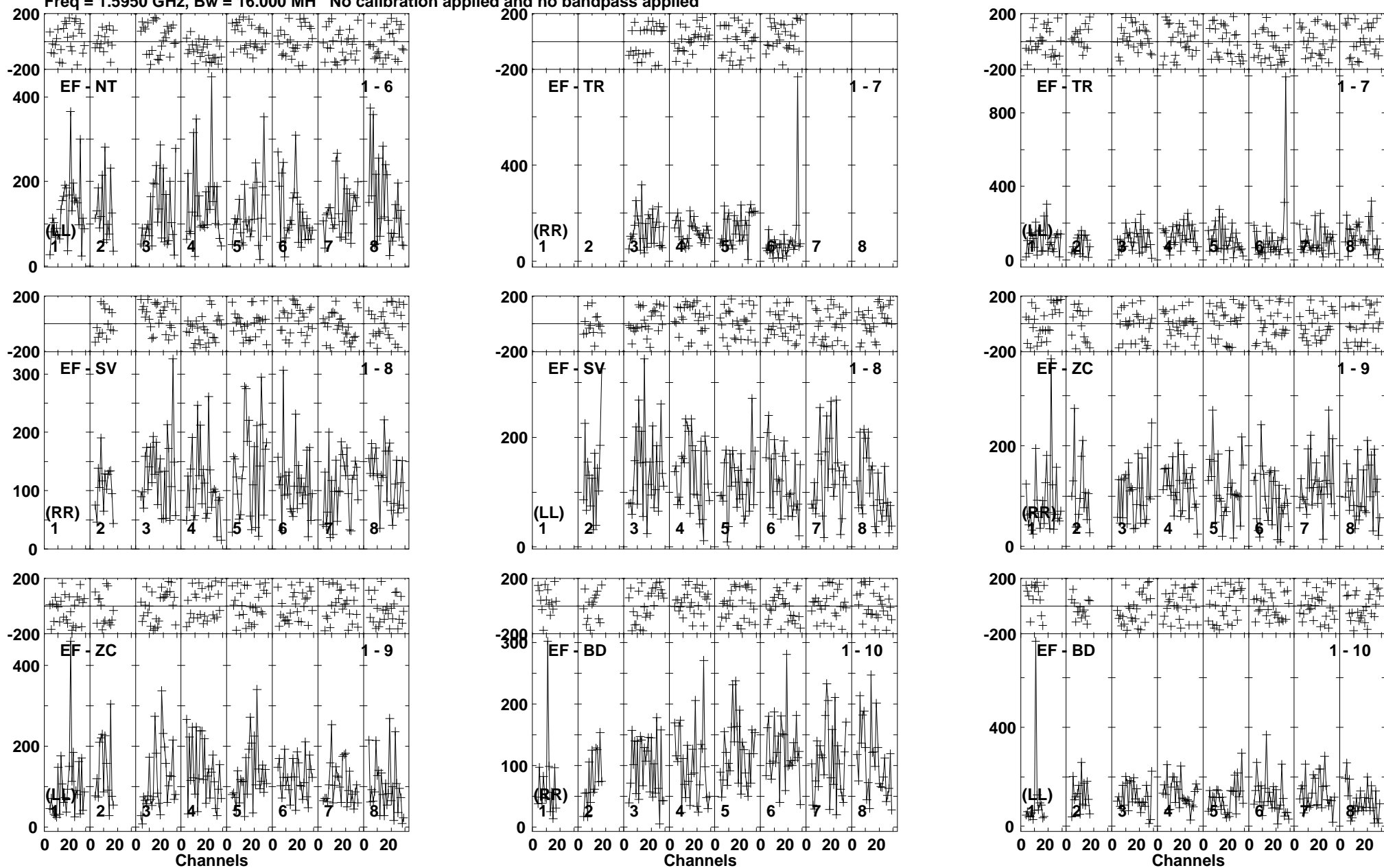
Lower frame: Micro Ampl Jy Top frame: Phas deg Vector averaged cross-power spectrum Baseline: EF (01) - NT (06) Timerange: 01/08:41:10 to 01/08:44:38
