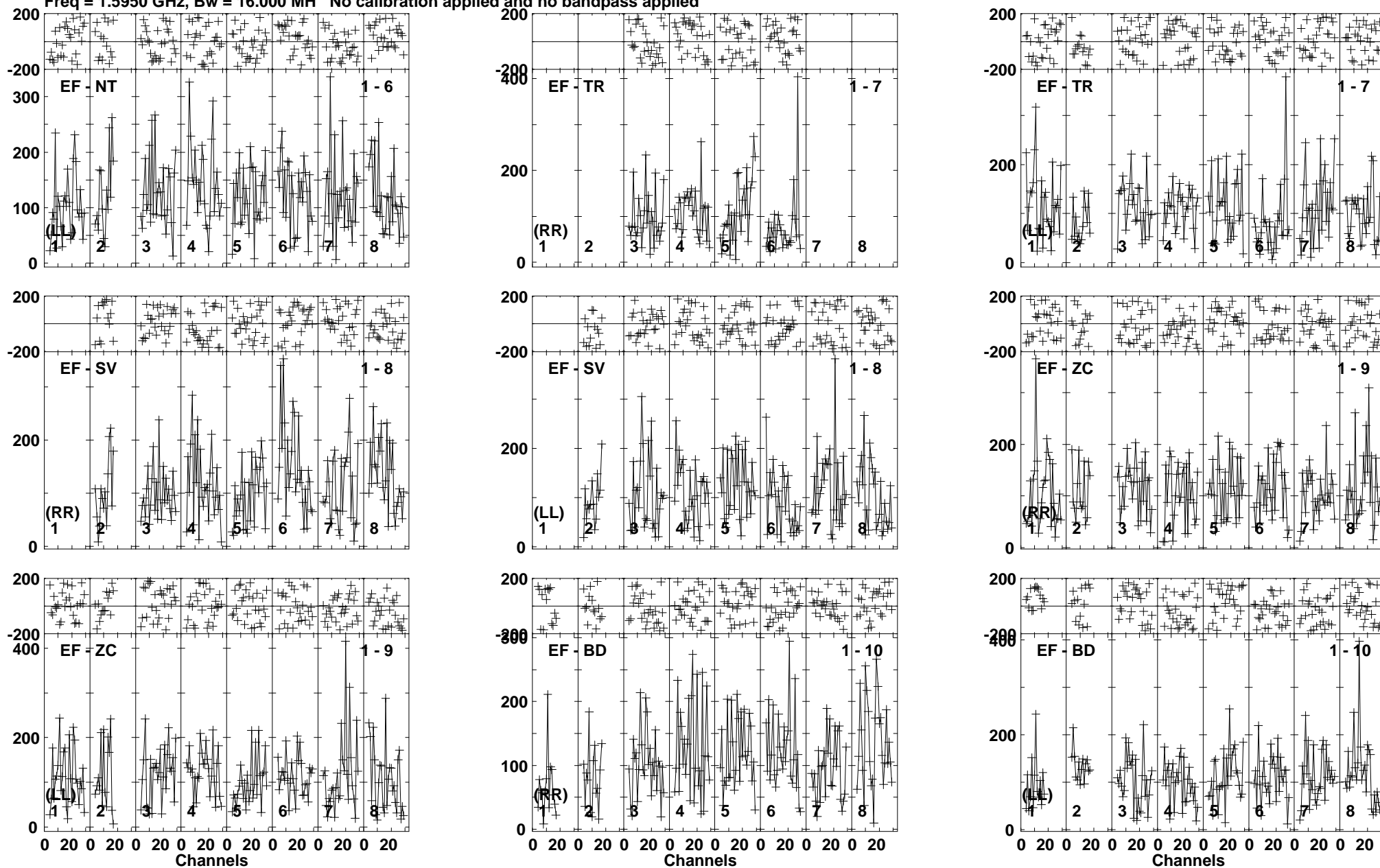
Lower frame: Micro Ampl Jy Top frame: Phas deg Vector averaged cross-power spectrum Baseline: EF (01) - NT (06) Timerange: 01/00:28:06 to 01/00:31:38
