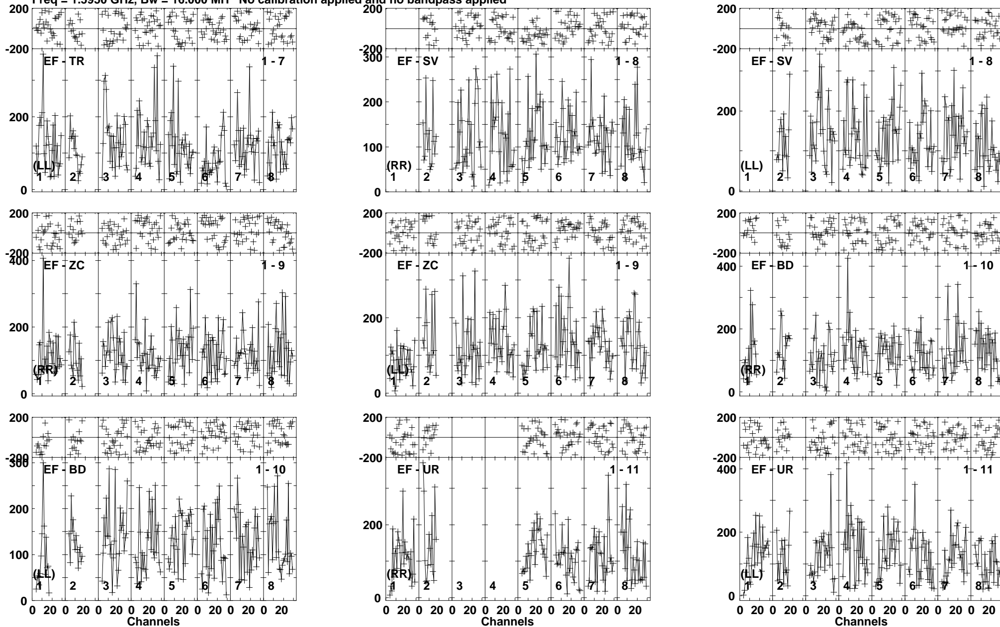
Lower frame: Micro Ampl Jy Top frame: Phas deg Vector averaged cross-power spectrum Baseline: EF (01) - TR (07) Timerange: 01/07:06:23 to 01/07:09:51
