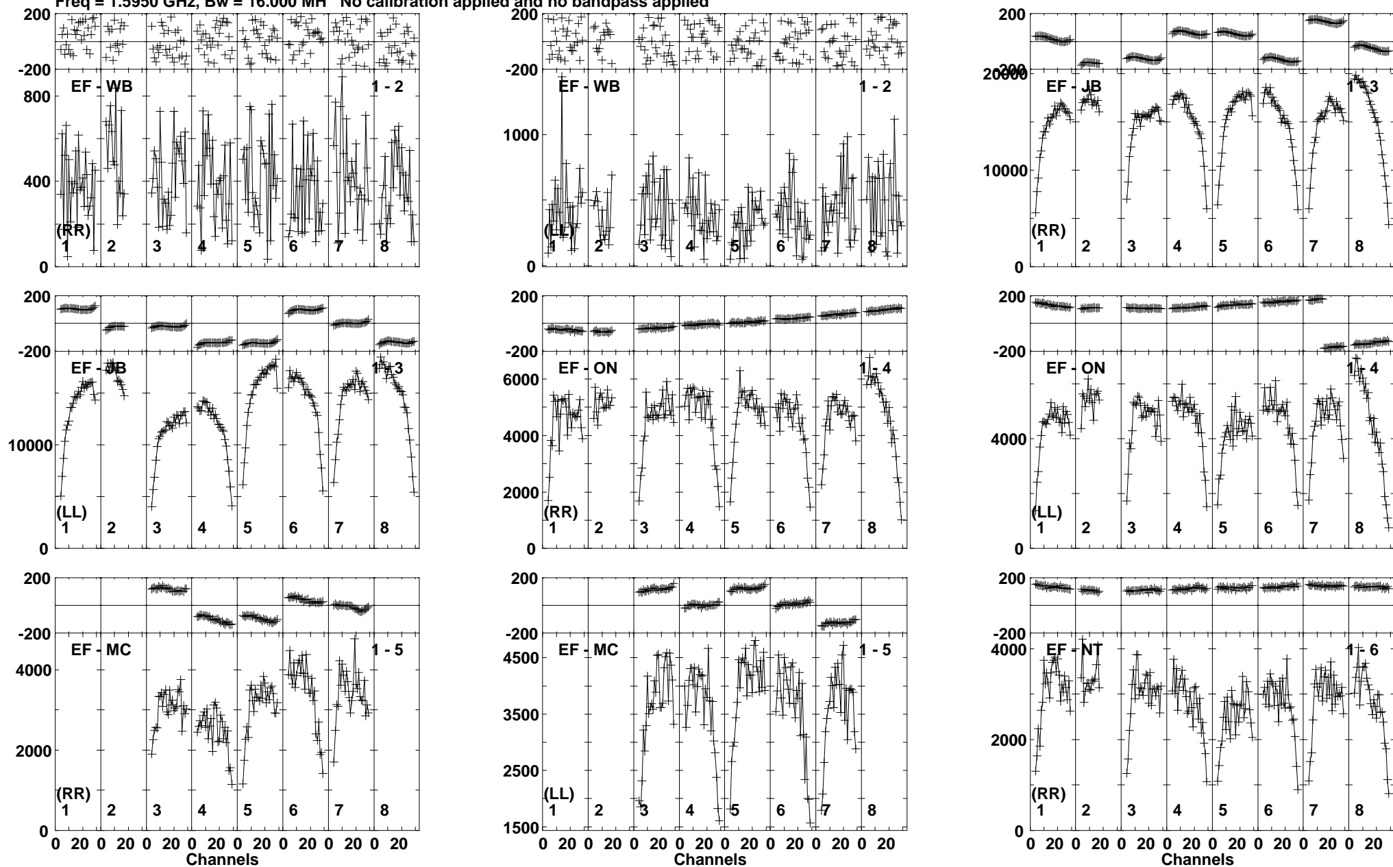
Lower frame: Micro Ampl Jy Top frame: Phas deg Vector averaged cross-power spectrum Baseline: EF (01) - WB (02) Timerange: 01/05:52:00 to 01/05:53:04
