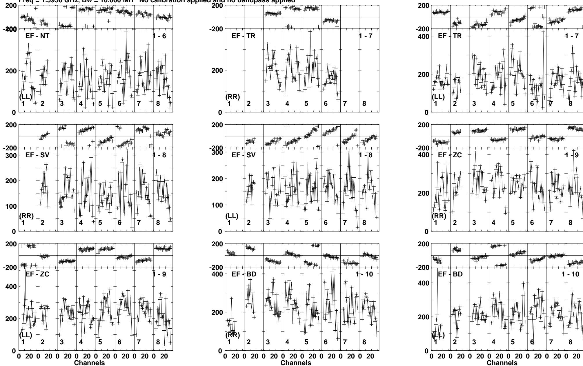
Lower frame: Micro Ampl Jy Top frame: Phas deg Vector averaged cross-power spectrum Baseline: EF (01) - NT (06) Timerange: 00:22:25:51 to 00:22:29:29
