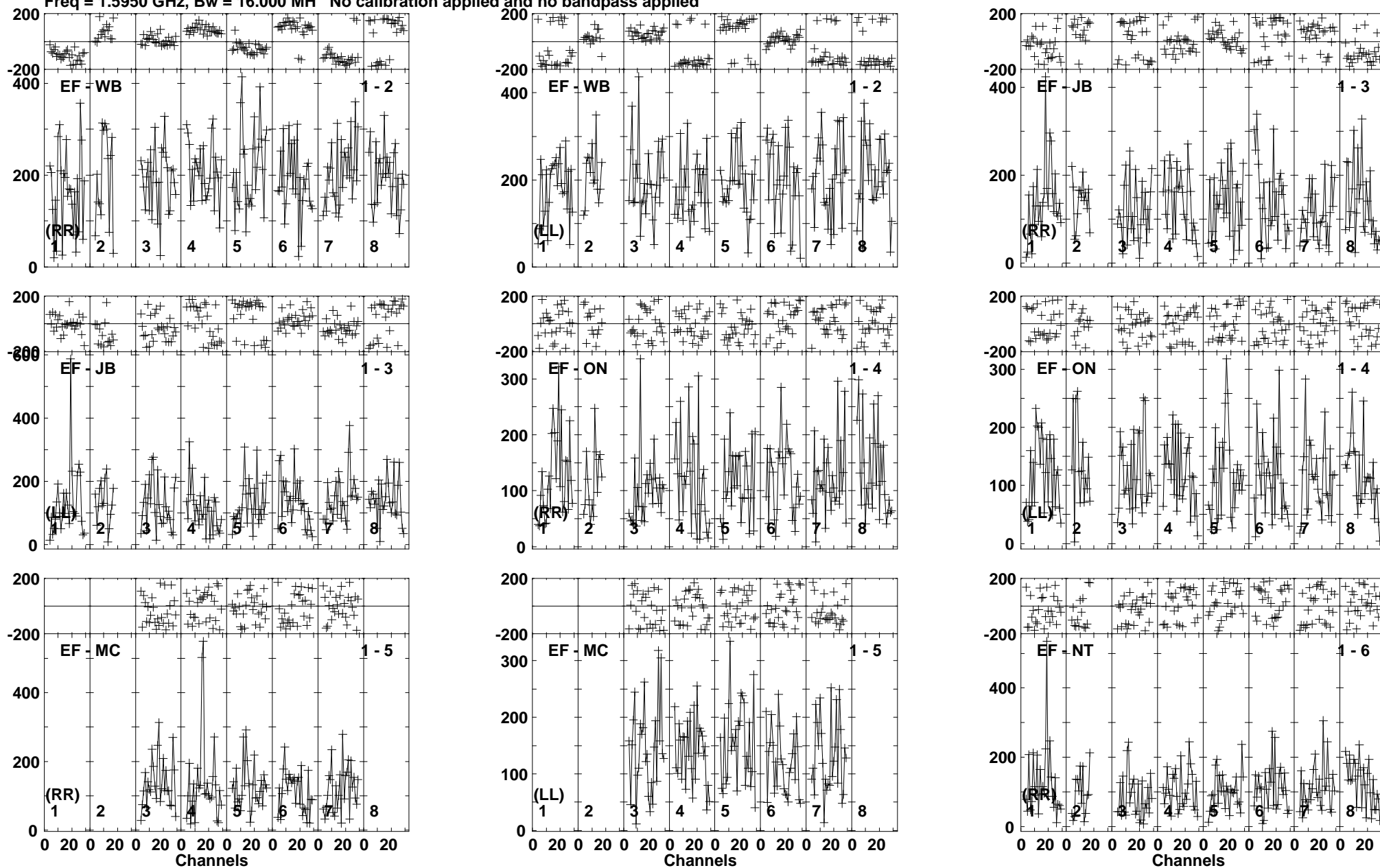
Lower frame: Micro Ampl Jy Top frame: Phas deg Vector averaged cross-power spectrum Baseline: EF (01) - WB (02) Timerange: 01/02:30:21 to 01/02:33:59
