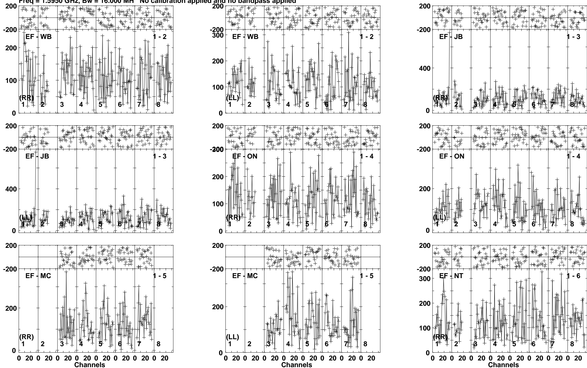
Lower frame: Micro Ampl Jy Top frame: Phas deg Vector averaged cross-power spectrum Baseline: EF (01) - WB (02) Timerange: 01/06:40:28 to 01/06:44:04
