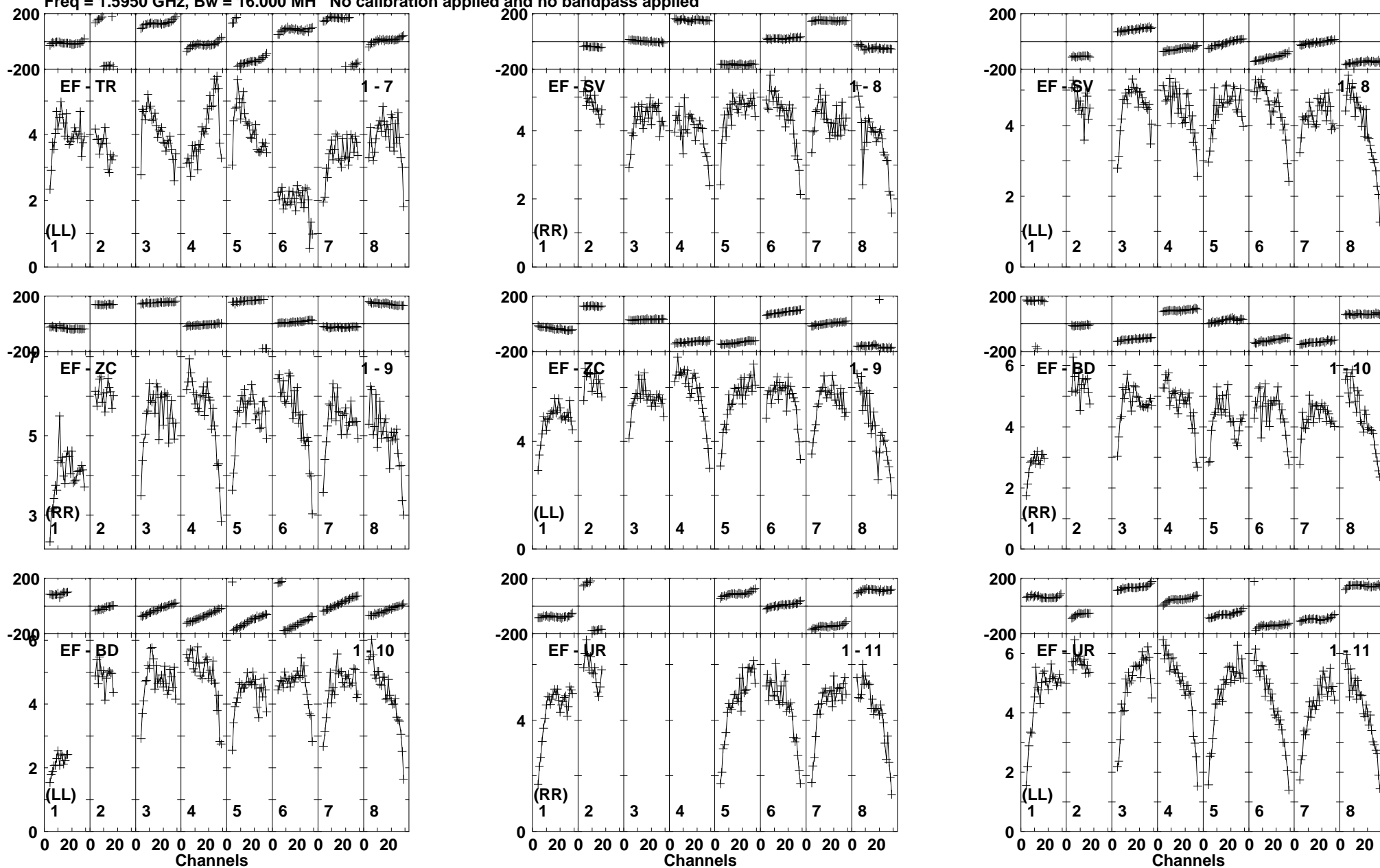
Lower frame: Milli Amply Jy Top frame: Phas deg Vector averaged cross-power spectrum Baseline: EF (01) - TR (07) Timerange: 01/06:59:35 to 01/07:00:39
