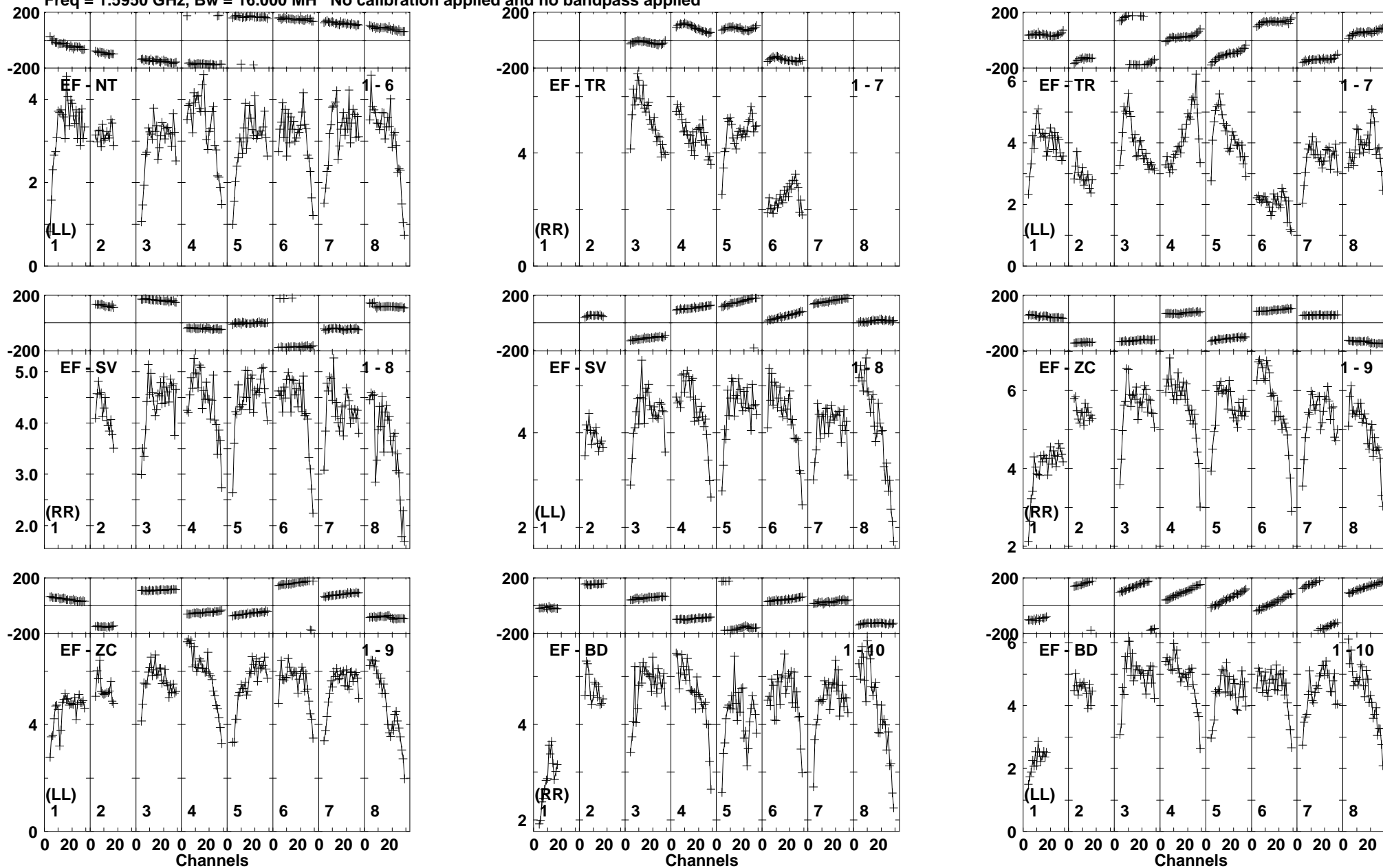
Lower frame: Milli Ampl Jy Top frame: Phas deg Vector averaged cross-power spectrum Baseline: EF (01) - NT (06) Timerange: 01/06:54:41 to 01/06:55:45
