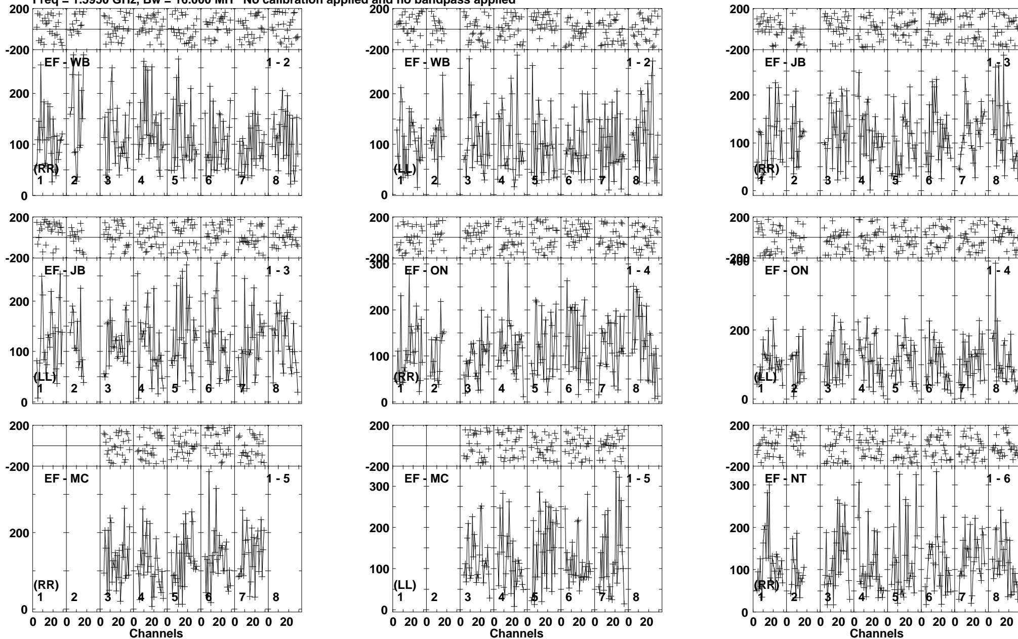
Lower frame: Micro Ampl Jy Top frame: Phas deg Vector averaged cross-power spectrum Baseline: EF (01) - WB (02) Timerange: 01/00:12:41 to 01/00:16:19
