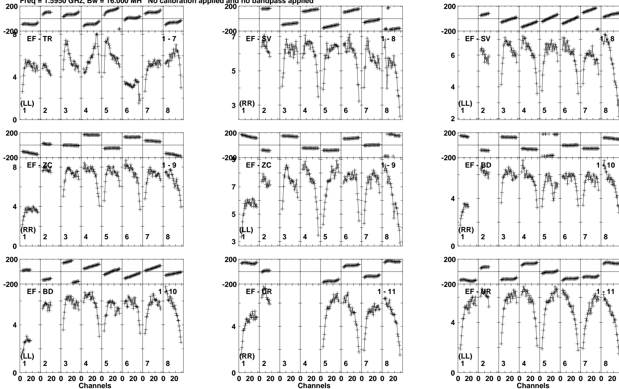
Lower frame: Milli Ampl Jy Top frame: Phas deg Vector averaged cross-power spectrum Baseline: EF (01) - TR (07) Timerange: 01/02:39:11 to 01/02:40:33
