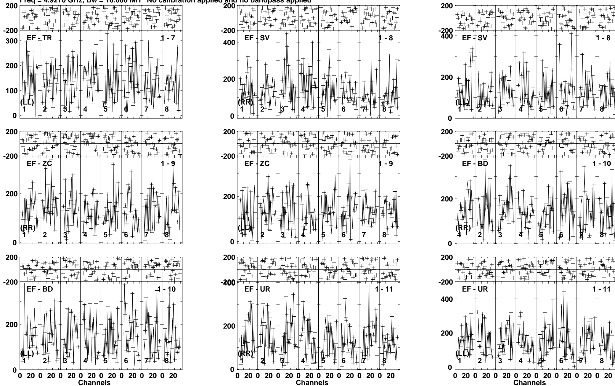
Lower frame: Micro Ampl Jy Top frame: Phas deg Vector averaged cross-power spectrum Baseline: EF (01) - TR (07) Timerange: 01/04:13:00 to 01/04:16:40
