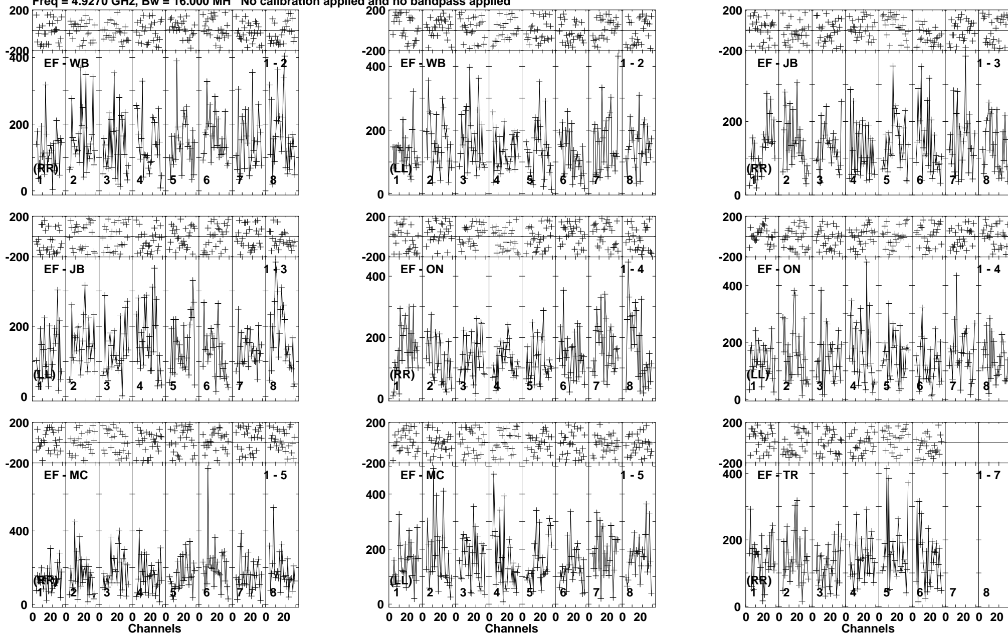
Lower frame: Micro Ampl Jy Top frame: Phas deg Vector averaged cross-power spectrum Baseline: EF (01) - WB (02) Timerange: 01/02:11:35 to 01/02:15:15
