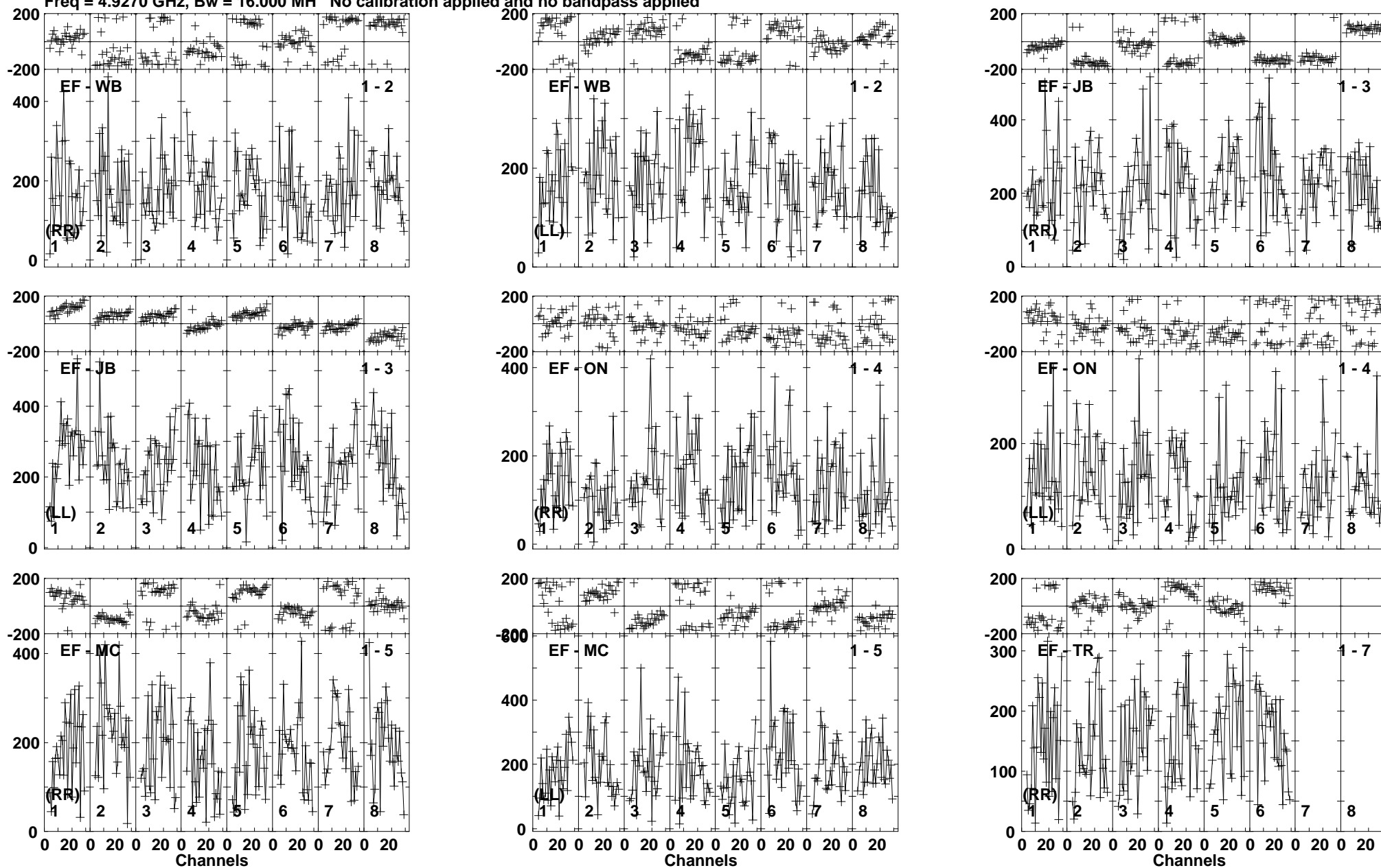
Lower frame: Micro Ampl Jy Top frame: Phas deg Vector averaged cross-power spectrum Baseline: EF (01) - WB (02) Timerange: 00/21:44:50 to 00/21:48:30
