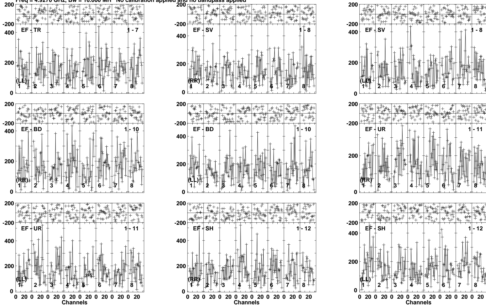
Lower frame: Micro Ampl Jy Top frame: Phas deg Vector averaged cross-power spectrum Baseline: EF (01) - TR (07) Timerange: 01/02:16:55 to 01/02:20:25
