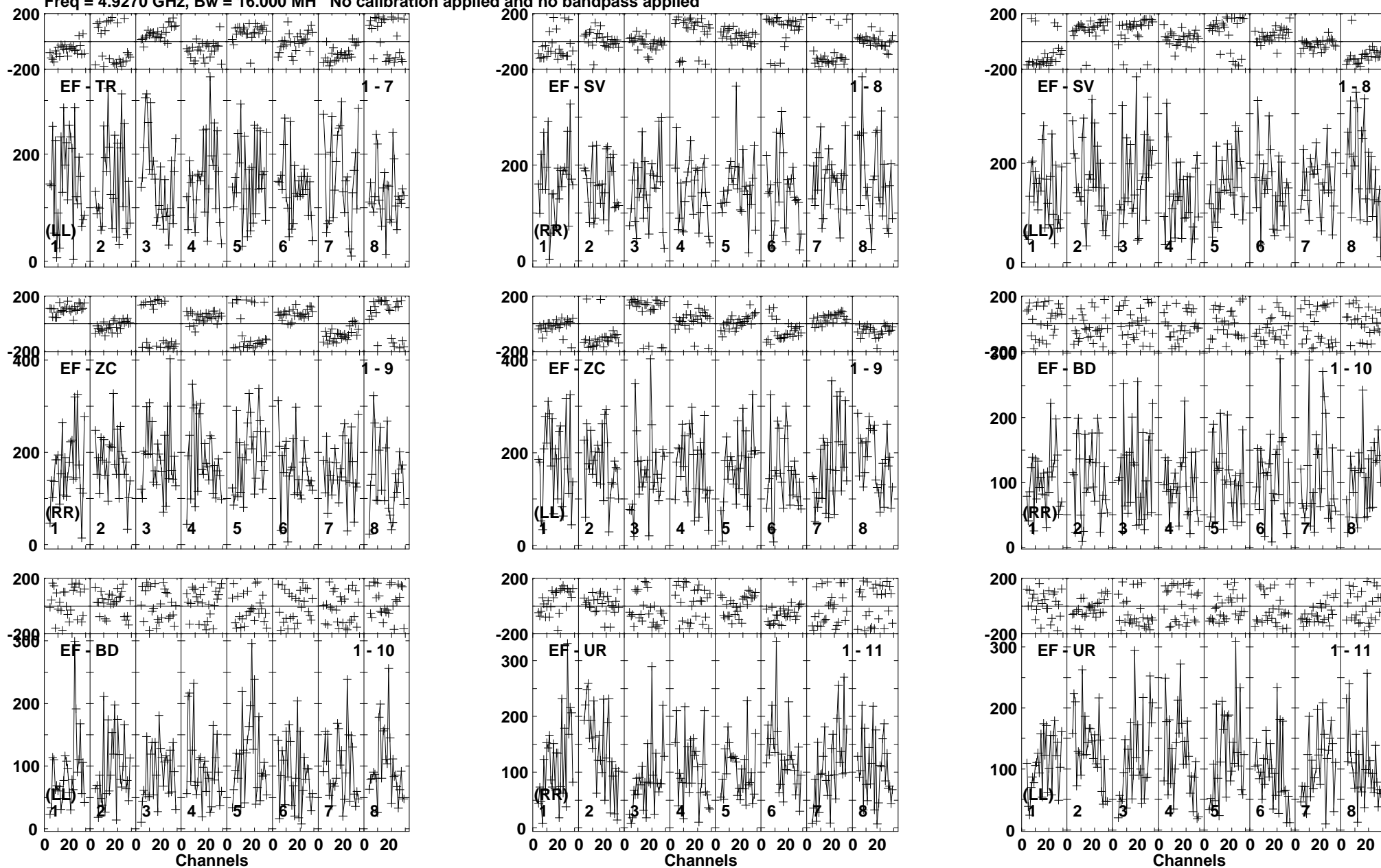
Lower frame: Micro Ampl Jy Top frame: Phas deg Vector averaged cross-power spectrum Baseline: EF (01) - TR (07) Timerange: 00:22:06:51 to 00:22:10:29
