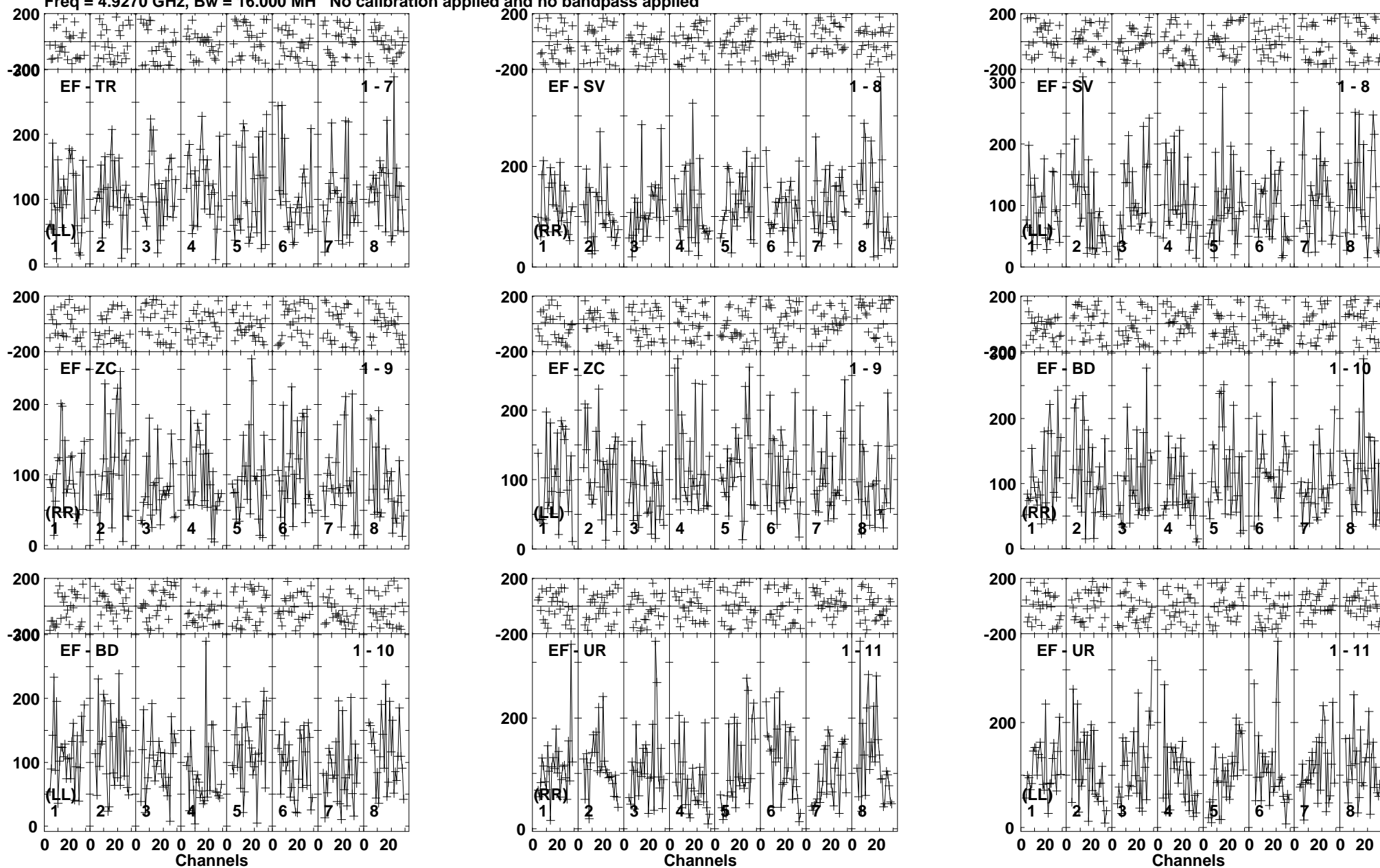
Lower frame: Micro Ampl Jy Top frame: Phas deg Vector averaged cross-power spectrum Baseline: EF (01) - TR (07) Timerange: 01/00:45:40 to 01/00:49:20
