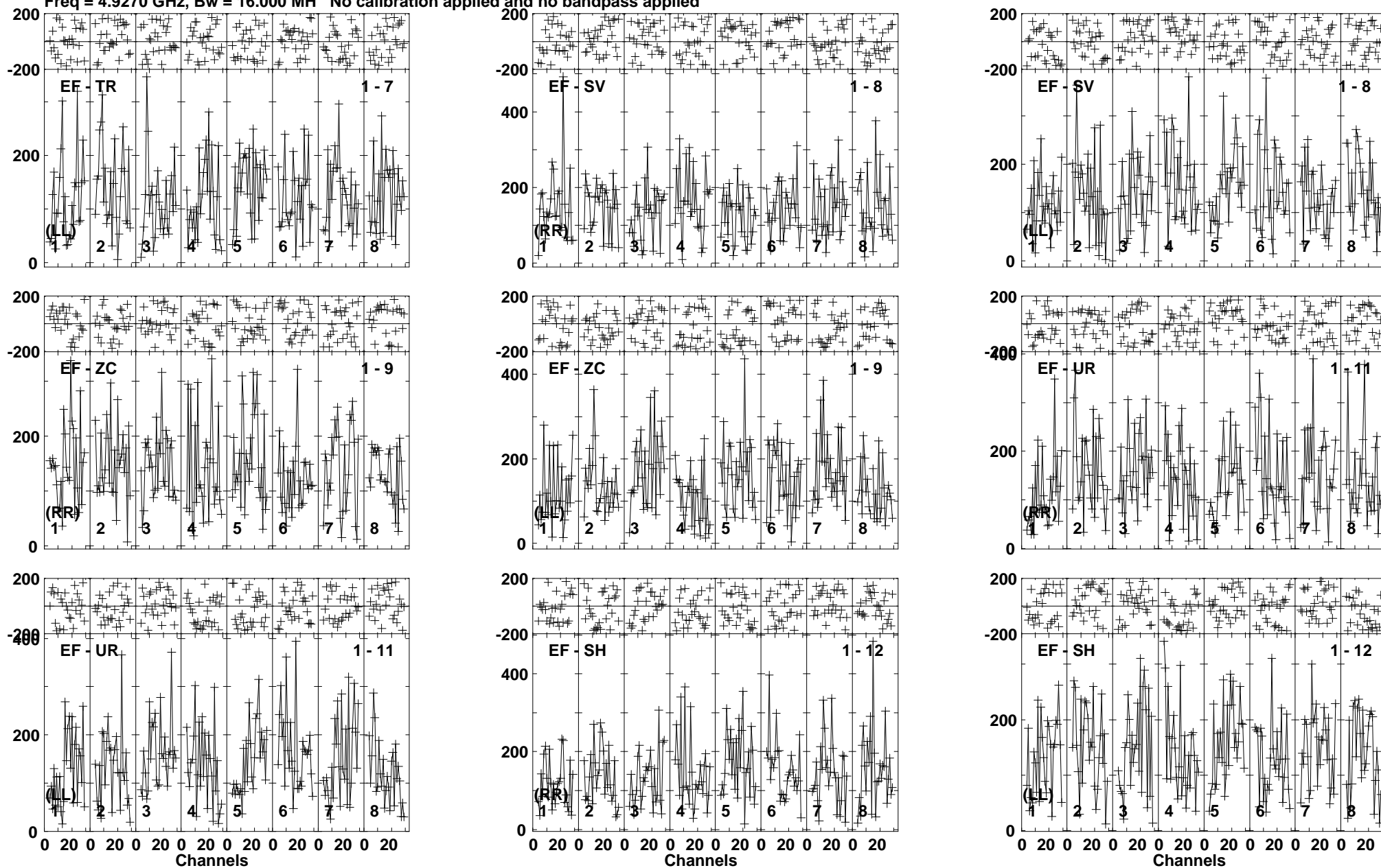
Lower frame: Micro Ampl Jy Top frame: Phas deg Vector averaged cross-power spectrum Baseline: EF (01) - TR (07) Timerange: 01/06:41:49 to 01/06:45:26
