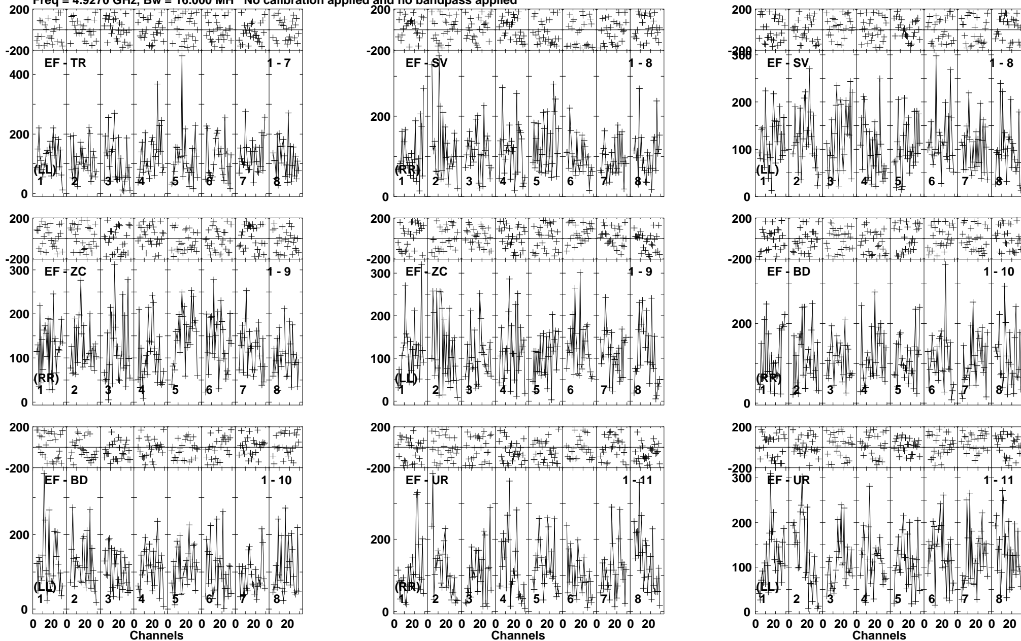
Lower frame: Micro Ampl Jy Top frame: Phas deg Vector averaged cross-power spectrum Baseline: EF (01) - TR (07) Timerange: 00/23:37:07 to 00/23:40:40
