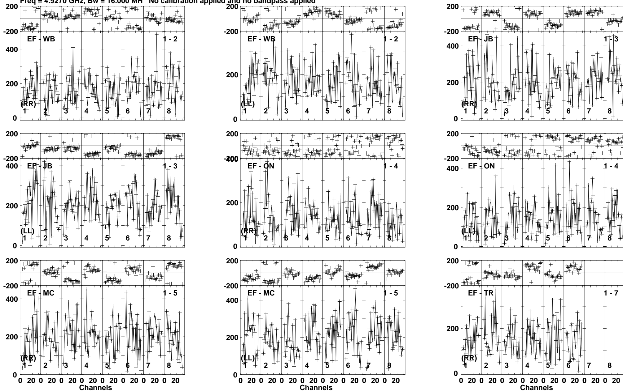
Lower frame: Micro Ampl Jy Top frame: Phas deg Vector averaged cross-power spectrum Baseline: EF (01) - WB (02) Timerange: 00/22:17:51 to 00/22:21:29
