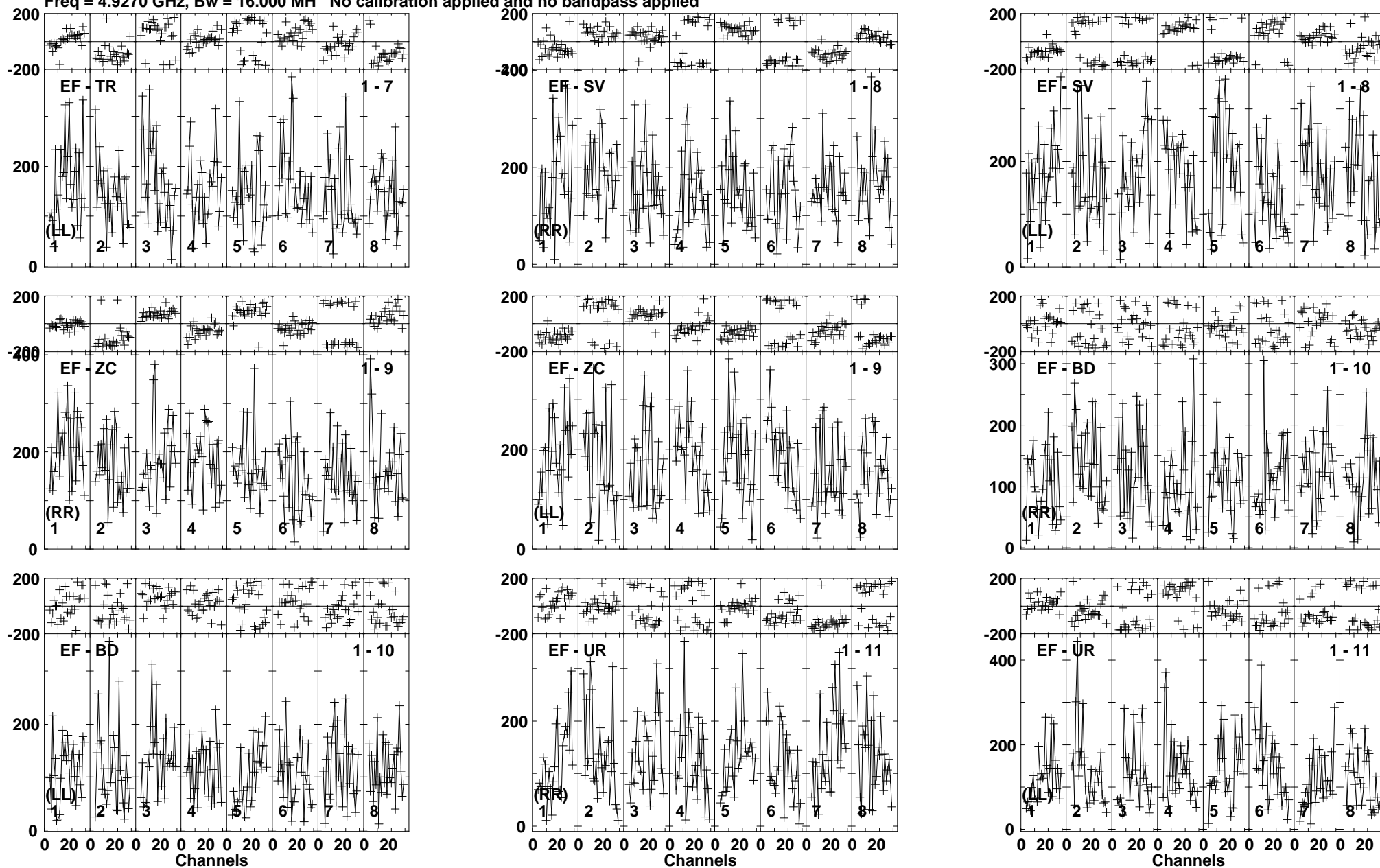
Lower frame: Micro Ampl Jy Top frame: Phas deg Vector averaged cross-power spectrum Baseline: EF (01) - TR (07) Timerange: 00/21:22:51 to 00/21:26:30
