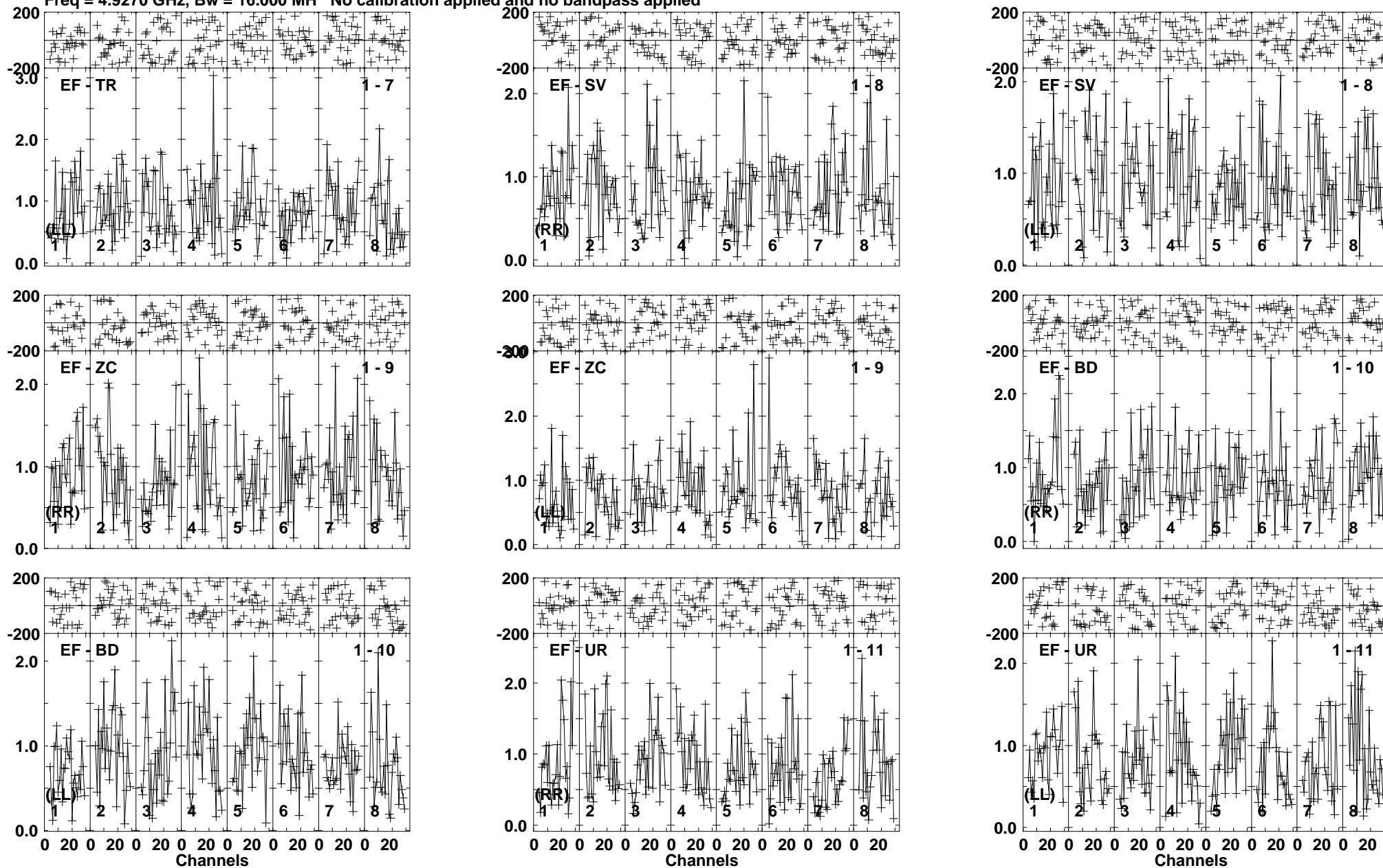
Lower frame: Milli Ampl Jy Top frame: Phas deg Vector averaged cross-power spectrum Baseline: EF (01) - TR (07) Timerange: 00/07:23:00 to 00/07:26:40
