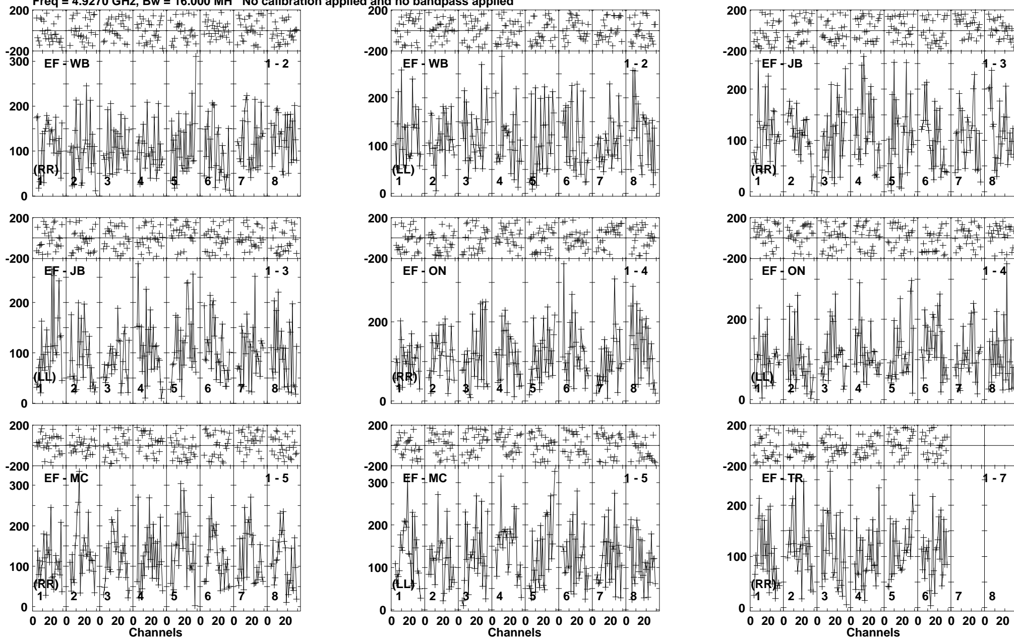
Lower frame: Micro Ampl Jy Top frame: Phas deg Vector averaged cross-power spectrum Baseline: EF (01) - WB (02) Timerange: 00/08:50:00 to 00/08:53:39
