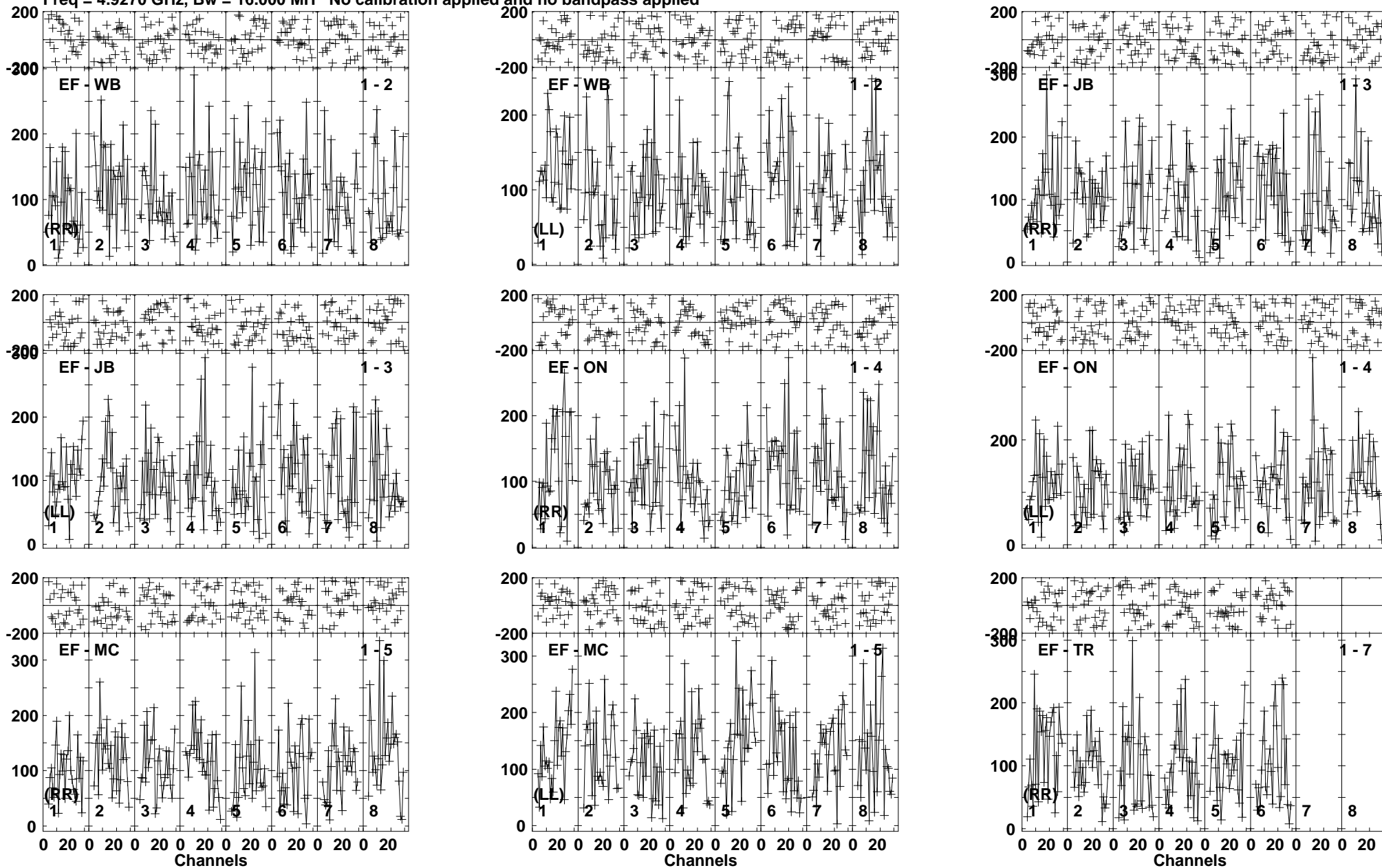
Lower frame: Micro Ampl Jy Top frame: Phas deg Vector averaged cross-power spectrum Baseline: EF (01) - WB (02) Timerange: 00/08:17:00 to 00/08:20:40
