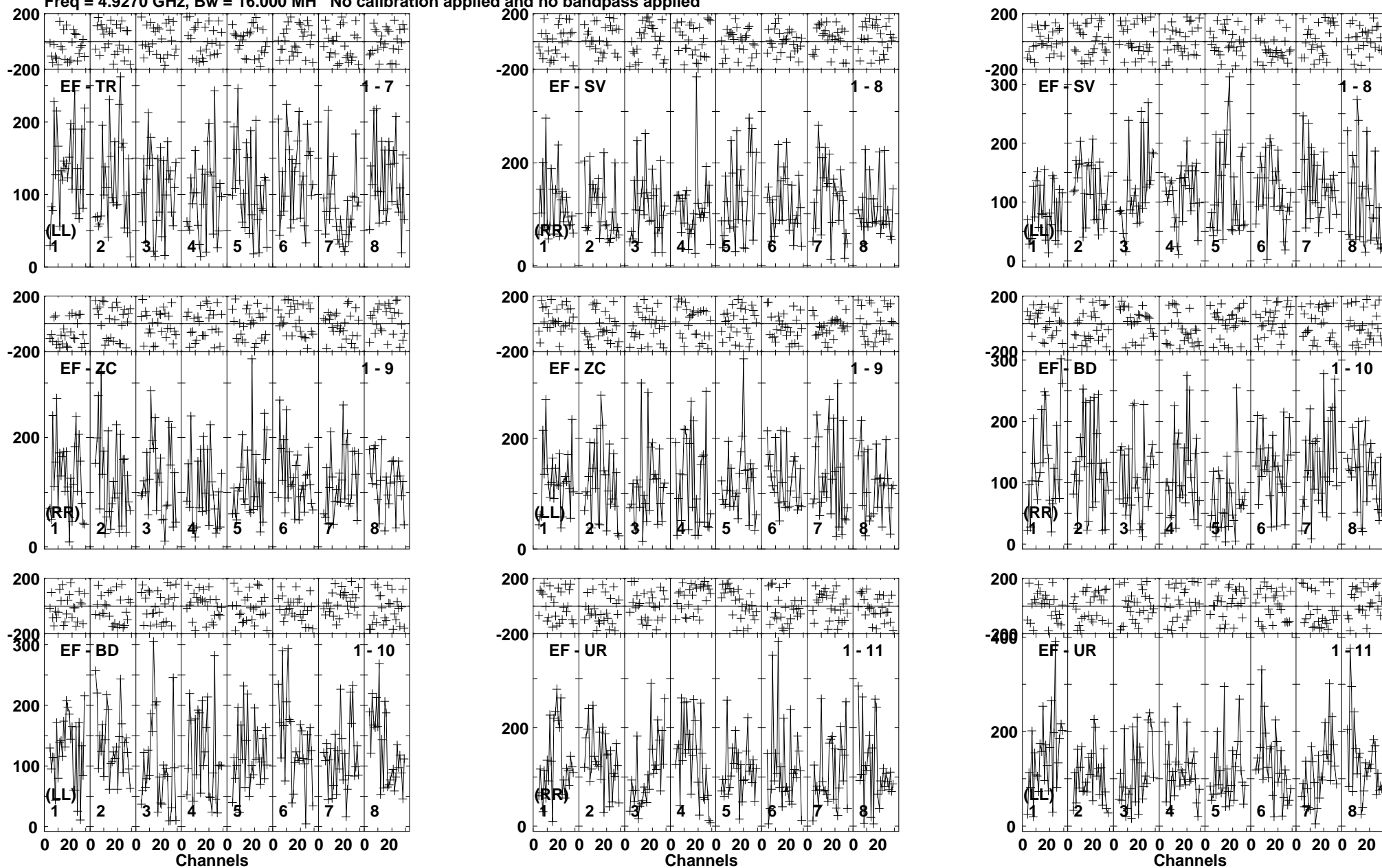
Lower frame: Micro Ampl Jy Top frame: Phas deg Vector averaged cross-power spectrum Baseline: EF (01) - TR (07) Timerange: 00/08:11:10 to 00/08:14:40
