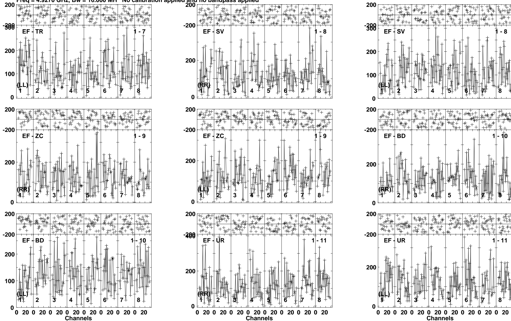
Lower frame: Micro Ampl Jy Top frame: Phas deg Vector averaged cross-power spectrum Baseline: EF (01) - TR (07) Timerange: 00/08:00:10 to 00/08:03:39
