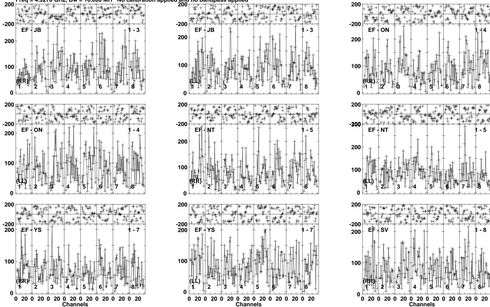
Lower frame: Micro Ampl Jy Top frame: Phas deg Vector averaged cross-power spectrum Baseline: EF (01) - JB (03) Timerange: 00/12:36:03 to 00/12:39:39
