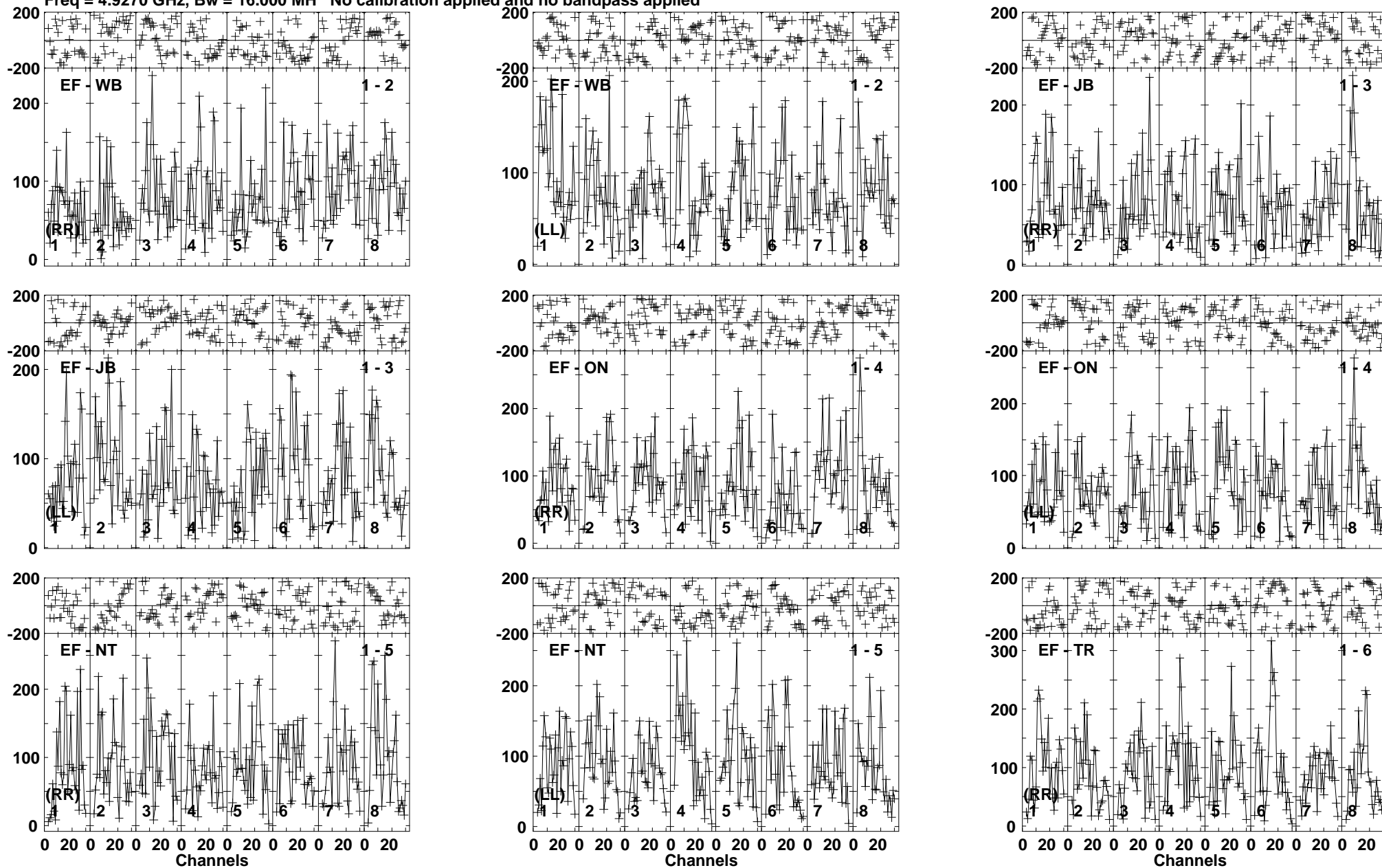
Lower frame: Micro Ampl Jy Top frame: Phas deg Vector averaged cross-power spectrum Baseline: EF (01) - WB (02) Timerange: 00/04:11:32 to 00/04:15:02
