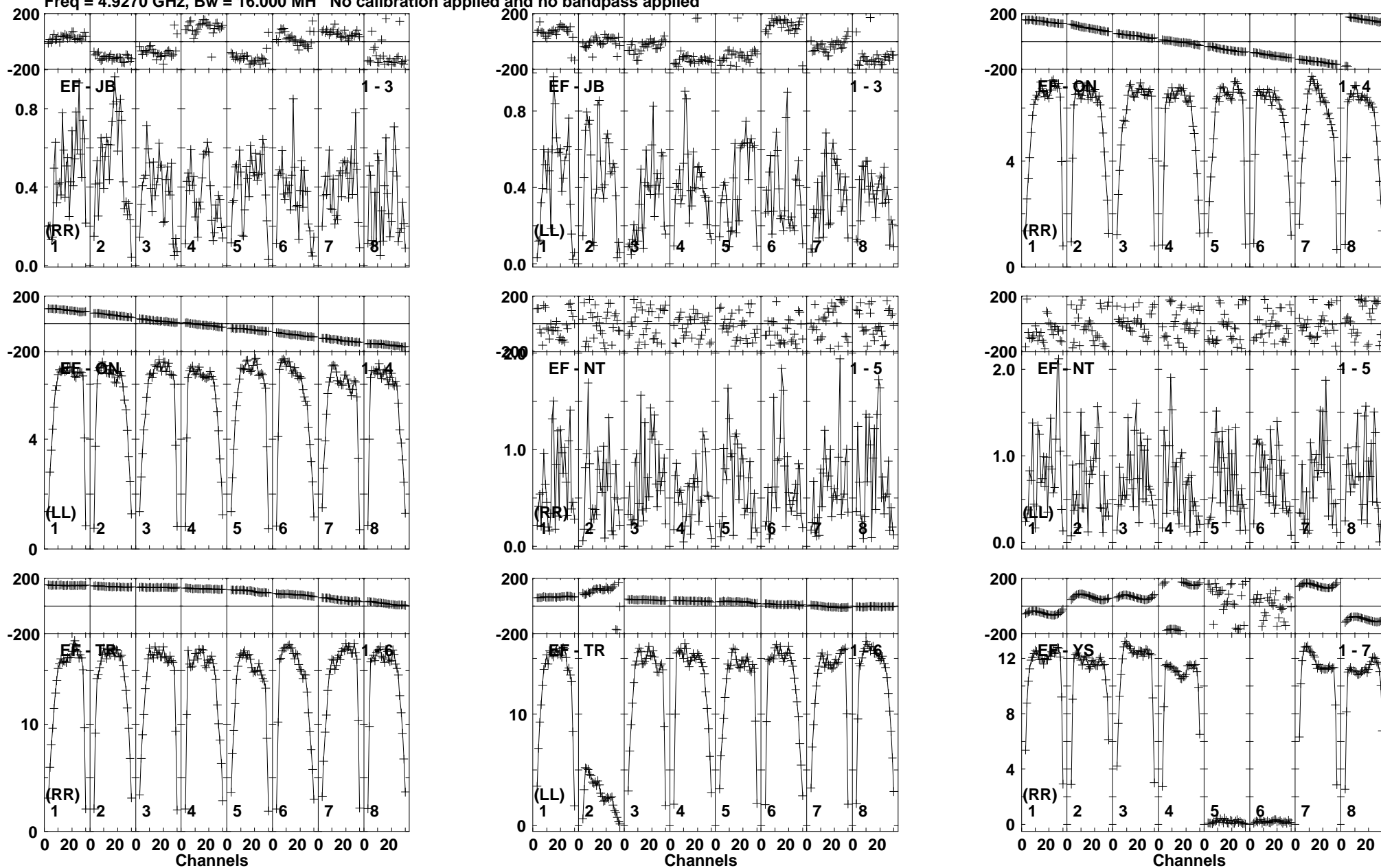
Lower frame: Milli Ampl Jy Top frame: Phas deg Vector averaged cross-power spectrum Baseline: EF (01) - JB (03) Timerange: 00/09:42:50 to 00/09:43:40
