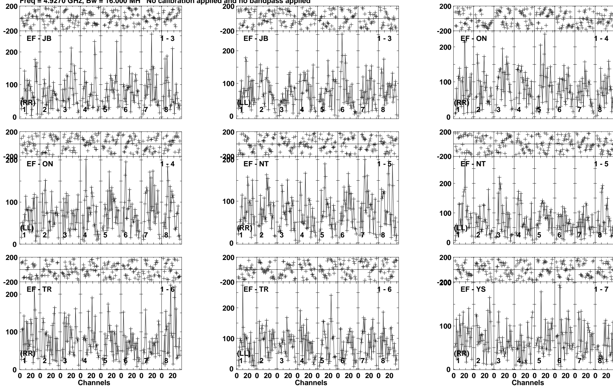
Lower frame: Micro Ampl Jy Top frame: Phas deg Vector averaged cross-power spectrum Baseline: EF (01) - JB (03) Timerange: 00/07:01:33 to 00/07:05:19
