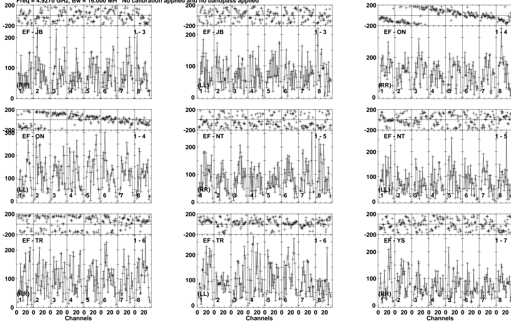
Lower frame: Micro Ampl Jy Top frame: Phas deg Vector averaged cross-power spectrum Baseline: EF (01) - JB (03) Timerange: 00/07:32:57 to 00/07:36:38
