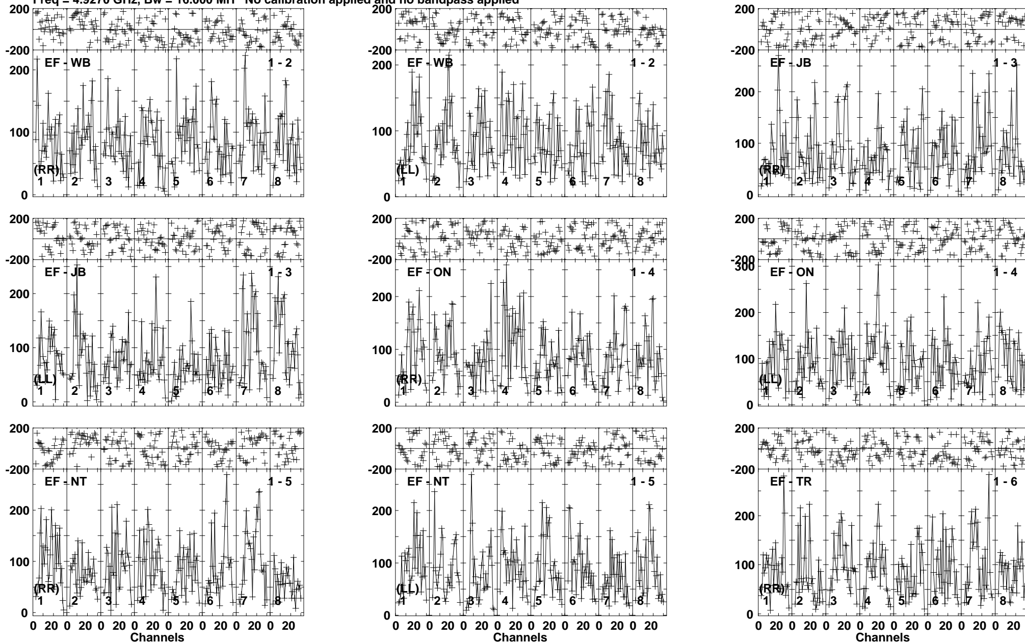
Lower frame: Micro Ampl Jy Top frame: Phas deg Vector averaged cross-power spectrum Baseline: EF (01) - WB (02) Timerange: 00/04:31:31 to 00/04:35:01
