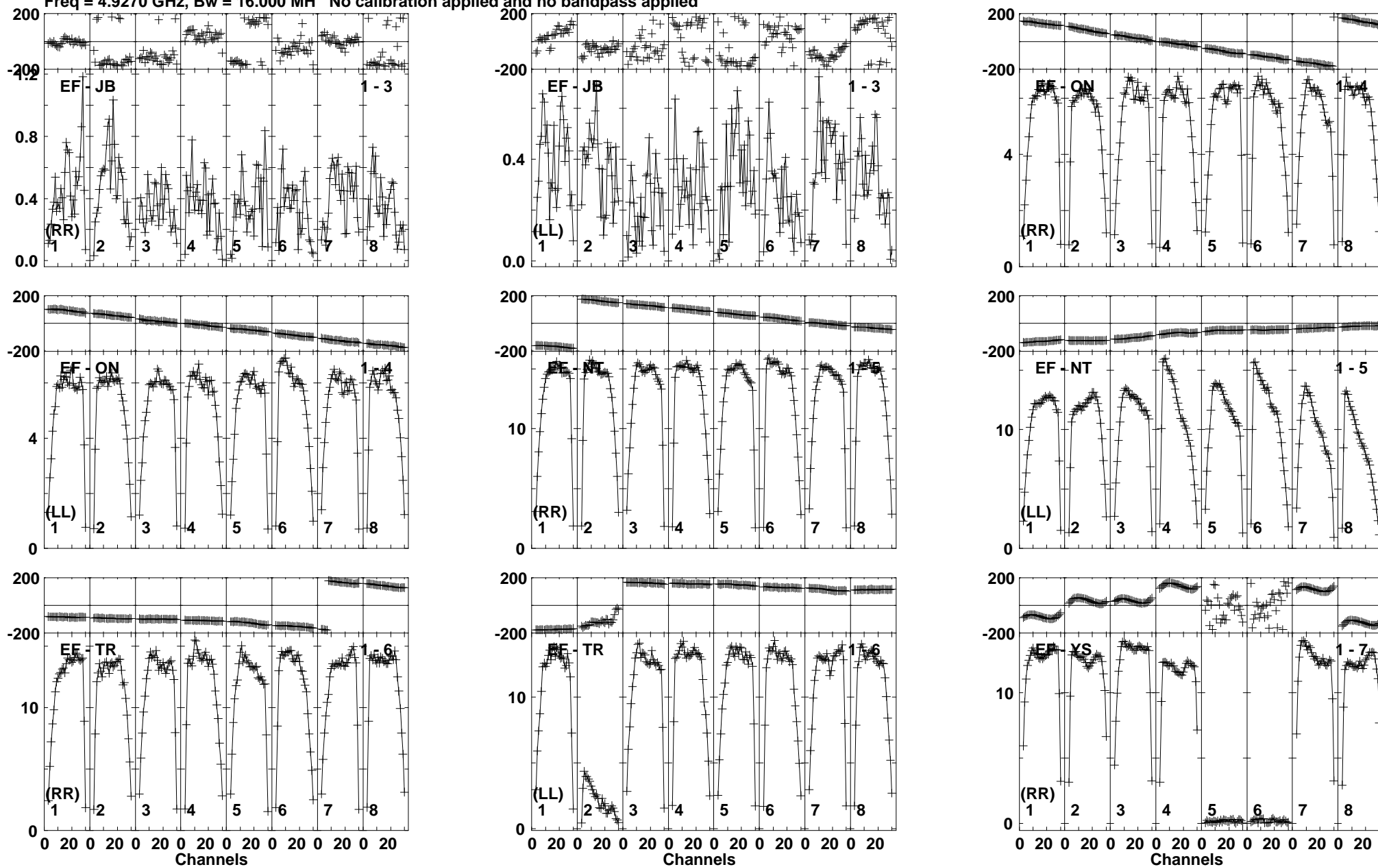
Lower frame: Milli Ampl Jy Top frame: Phas deg Vector averaged cross-power spectrum Baseline: EF (01) - JB (03) Timerange: 00/10:51:23 to 00/10:52:20
