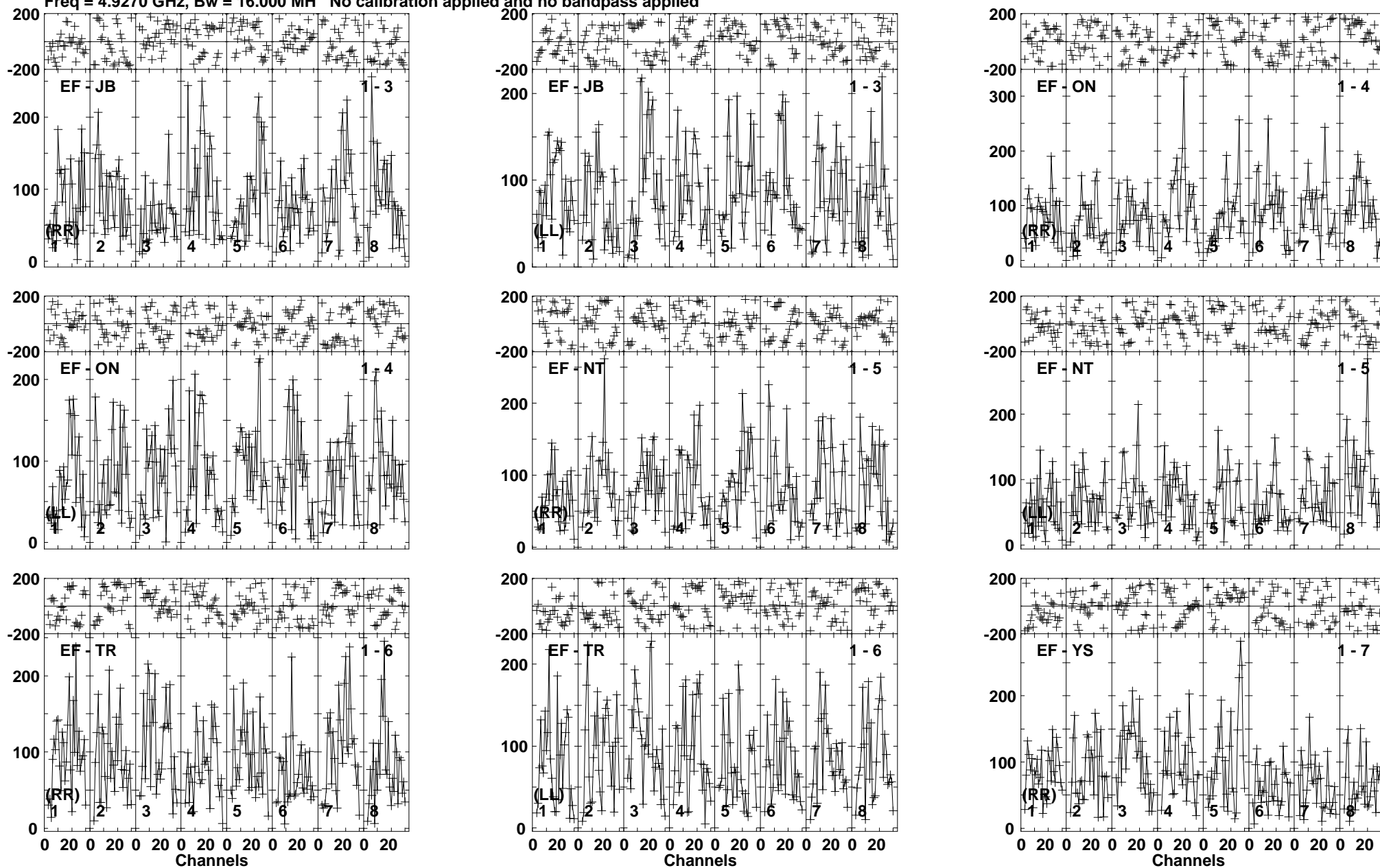
Lower frame: Micro Ampl Jy Top frame: Phas deg Vector averaged cross-power spectrum Baseline: EF (01) - JB (03) Timerange: 00/11:44:09 to 00/11:47:40
