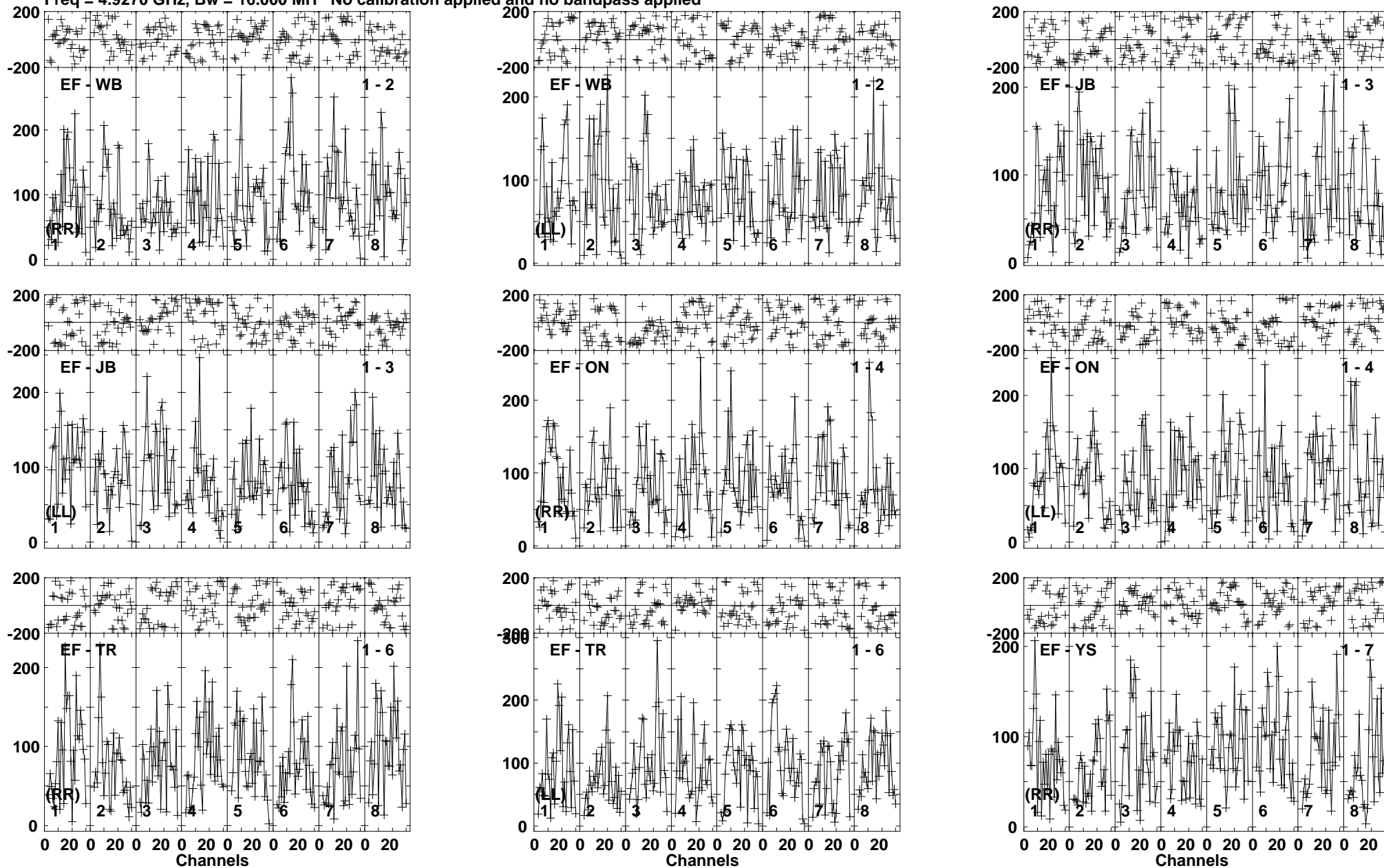
Lower frame: Micro Ampl Jy Top frame: Phas deg Vector averaged cross-power spectrum Baseline: EF (01) - WB (02) Timerange: 00/06:49:58 to 00/06:53:43
