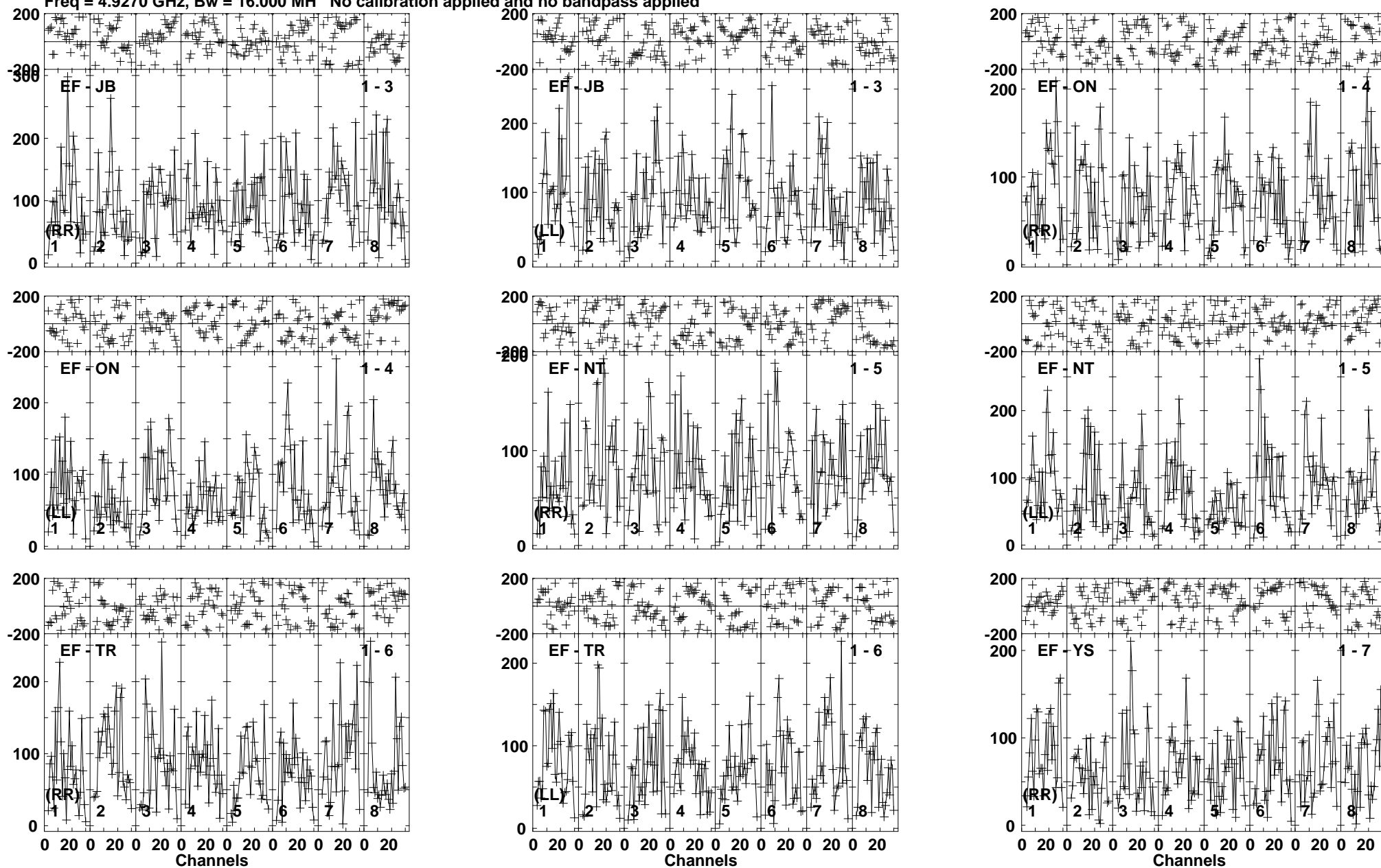
Lower frame: Micro Ampl Jy Top frame: Phas deg Vector averaged cross-power spectrum Baseline: EF (01) - JB (03) Timerange: 00/11:02:02 to 00/11:05:39
