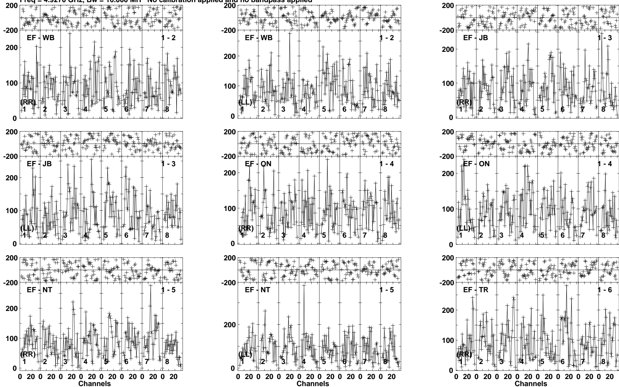
Lower frame: Micro Ampl Jy Top frame: Phas deg Vector averaged cross-power spectrum Baseline: EF (01) - WB (02) Timerange: 00/04:16:21 to 00/04:19:51
