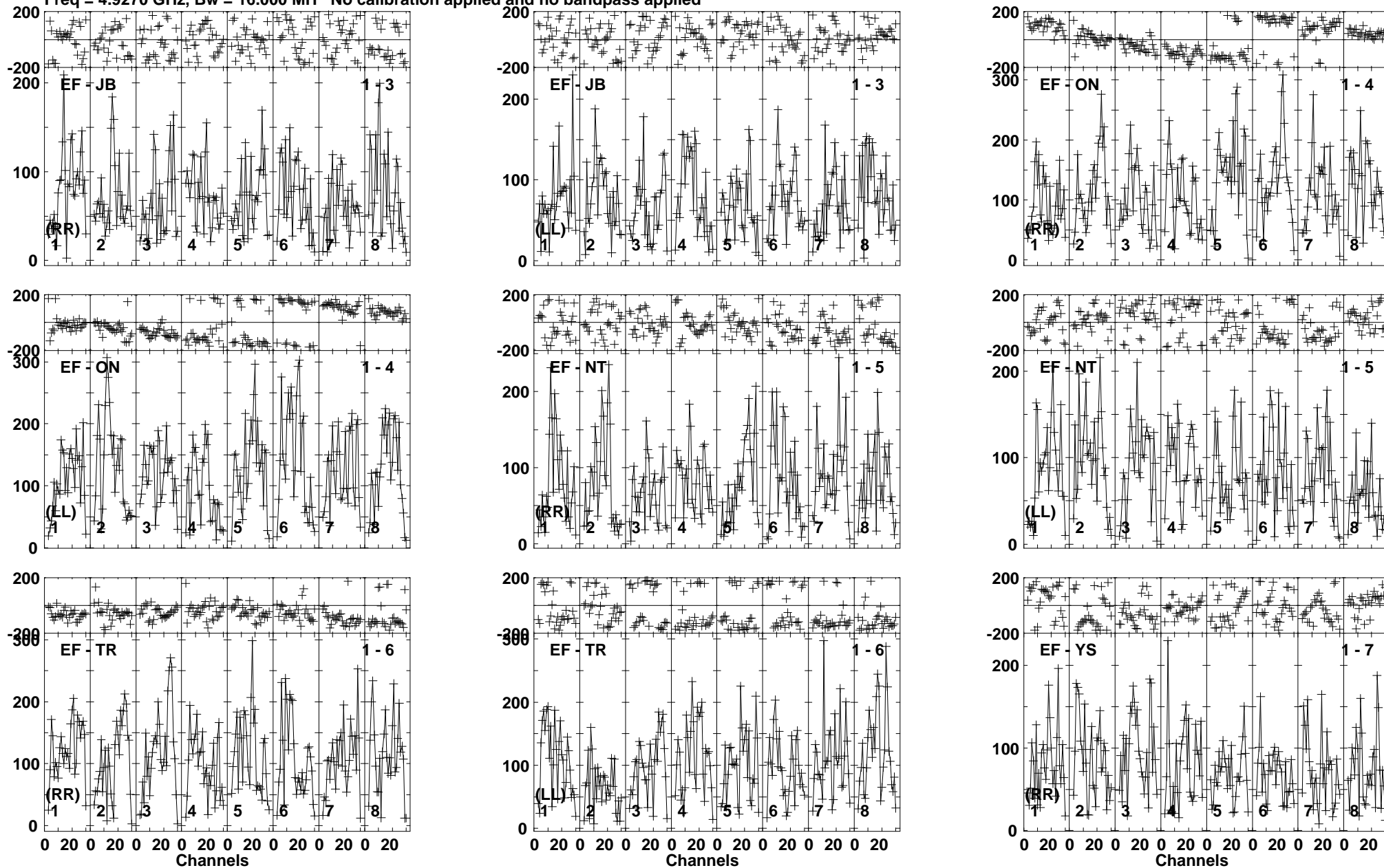
Lower frame: Micro Ampl Jy Top frame: Phas deg Vector averaged cross-power spectrum Baseline: EF (01) - JB (03) Timerange: 00/07:47:42 to 00/07:51:24
