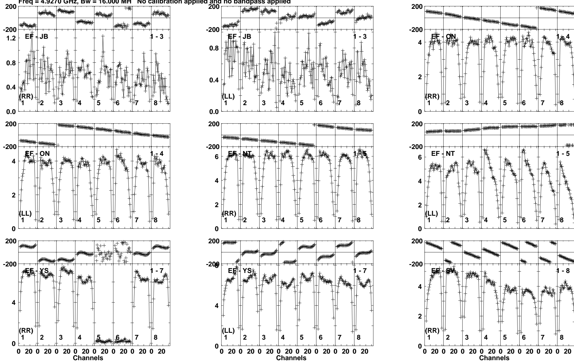
Lower frame: Milli Ampl Jy Top frame: Phas deg Vector averaged cross-power spectrum Baseline: EF (01) - JB (03) Timerange: 00:12:14:10 to 00:12:15:20
