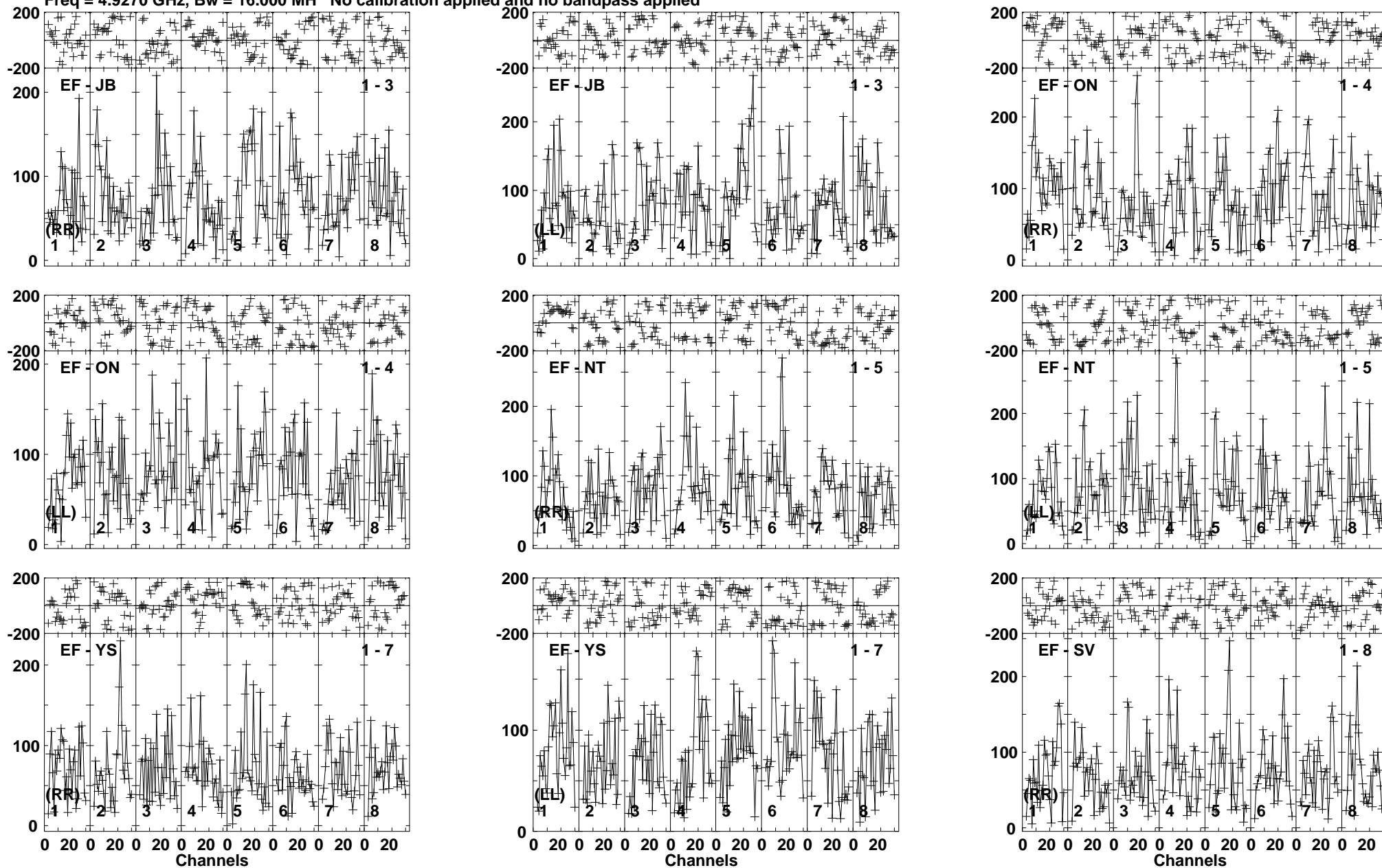
Lower frame: Micro Ampl Jy Top frame: Phas deg Vector averaged cross-power spectrum Baseline: EF (01) - JB (03) Timerange: 00/12:10:21 to 00/12:13:59
