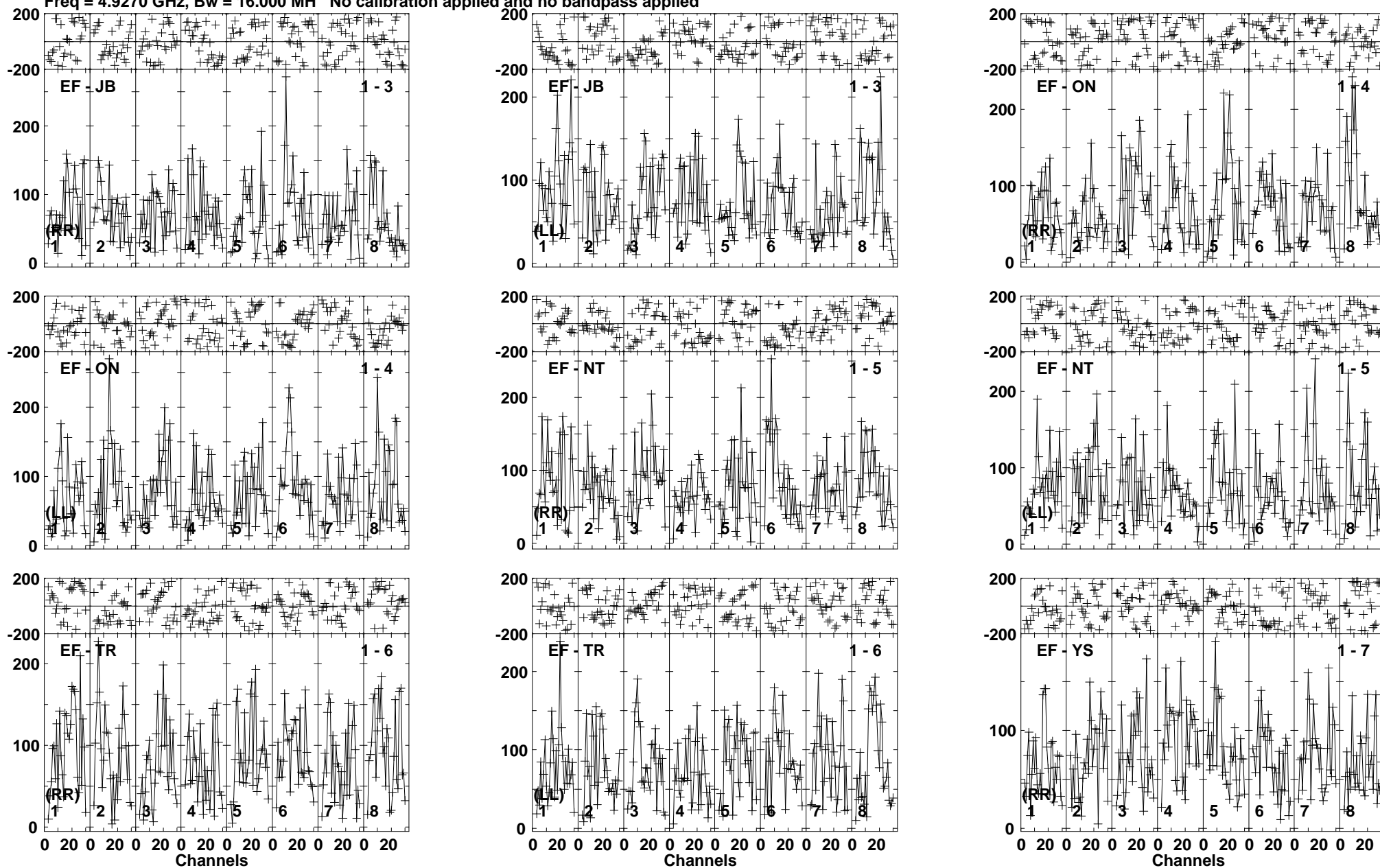
Lower frame: Micro Ampl Jy Top frame: Phas deg Vector averaged cross-power spectrum Baseline: EF (01) - JB (03) Timerange: 00/11:39:00 to 00/11:42:39
