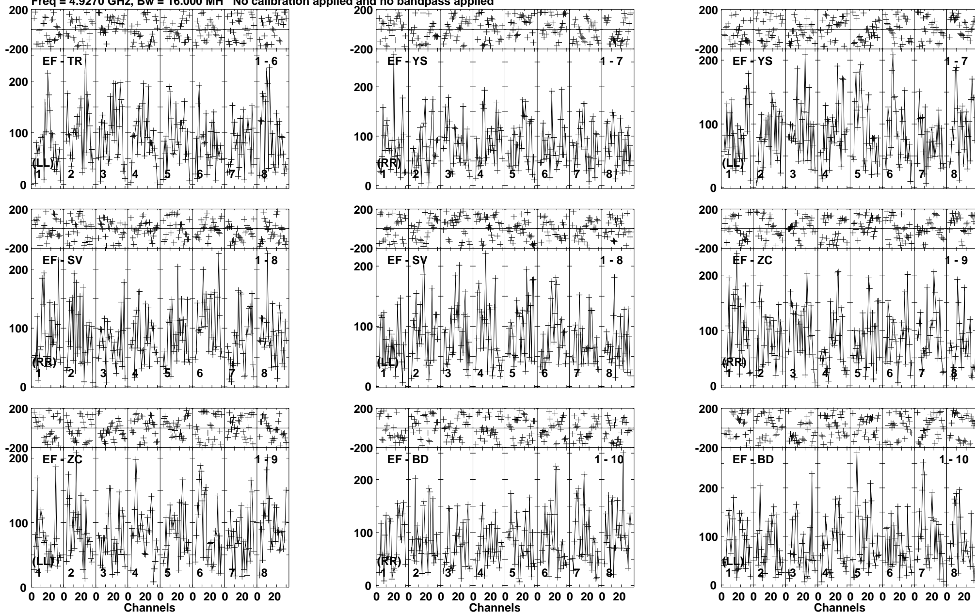
Lower frame: Micro Ampl Jy Top frame: Phas deg Vector averaged cross-power spectrum Baseline: EF (01) - TR (06) Timerange: 00/04:26:41 to 00/04:30:11
