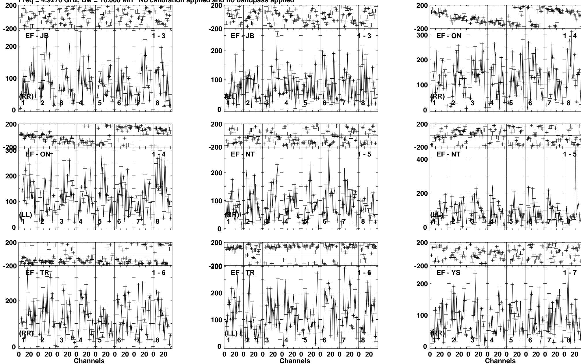
Lower frame: Micro Ampl Jy Top frame: Phas deg Vector averaged cross-power spectrum Baseline: EF (01) - JB (03) Timerange: 00/07:27:37 to 00/07:31:16
