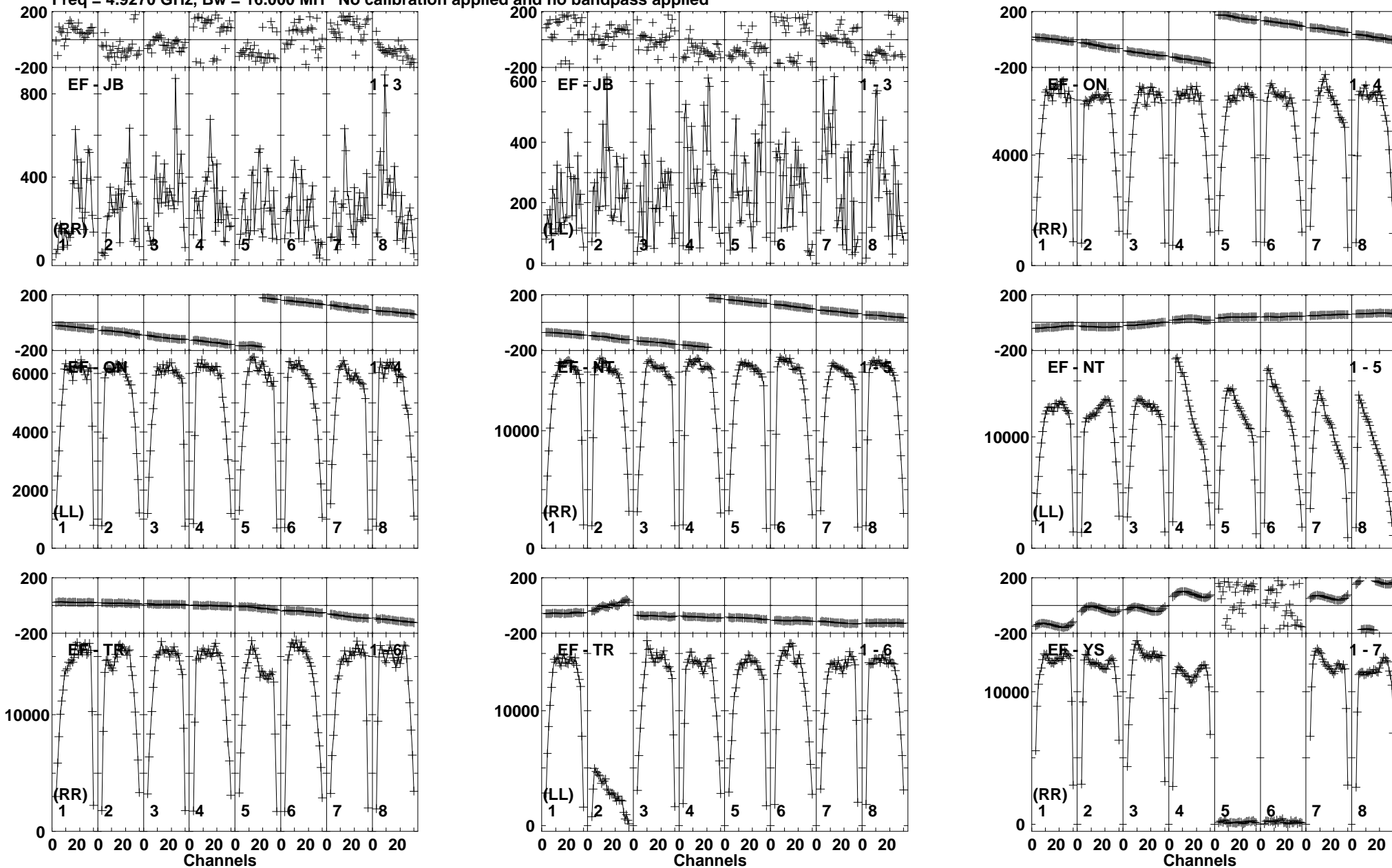
Lower frame: Micro Ampl Jy Top frame: Phas deg Vector averaged cross-power spectrum Baseline: EF (01) - JB (03) Timerange: 00/10:02:04 to 00/10:02:59
