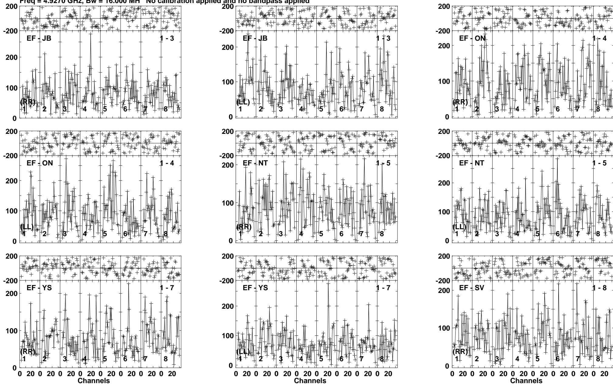
Lower frame: Micro Ampl Jy Top frame: Phas deg Vector averaged cross-power spectrum Baseline: EF (01) - JB (03) Timerange: 00/12:20:22 to 00/12:24:00
