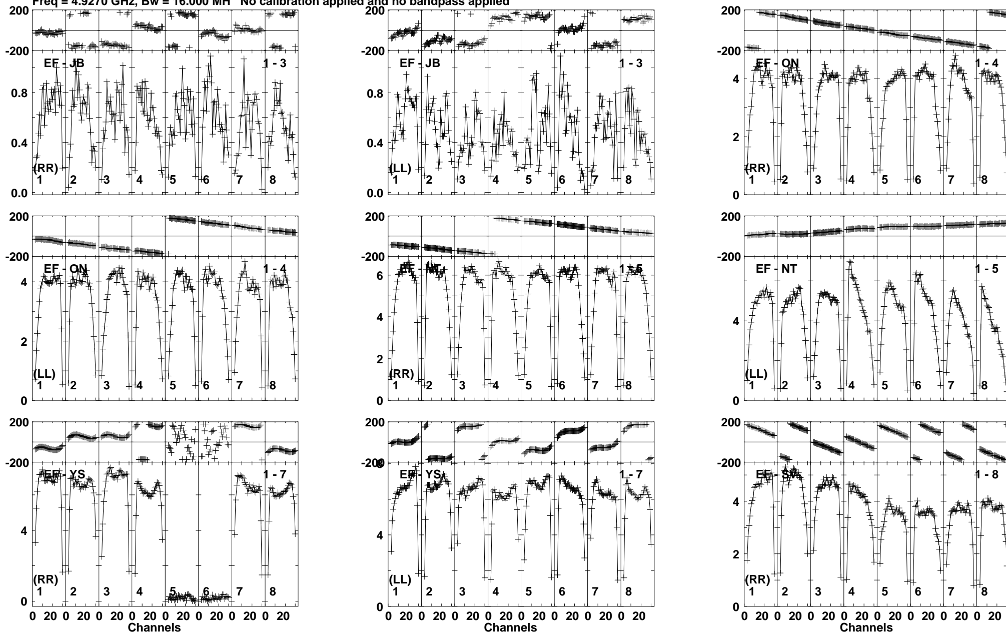
Lower frame: Milli Ampl Jy Top frame: Phas deg Vector averaged cross-power spectrum Baseline: EF (01) - JB (03) Timerange: 00:12:39:50 to 00:12:41:00
