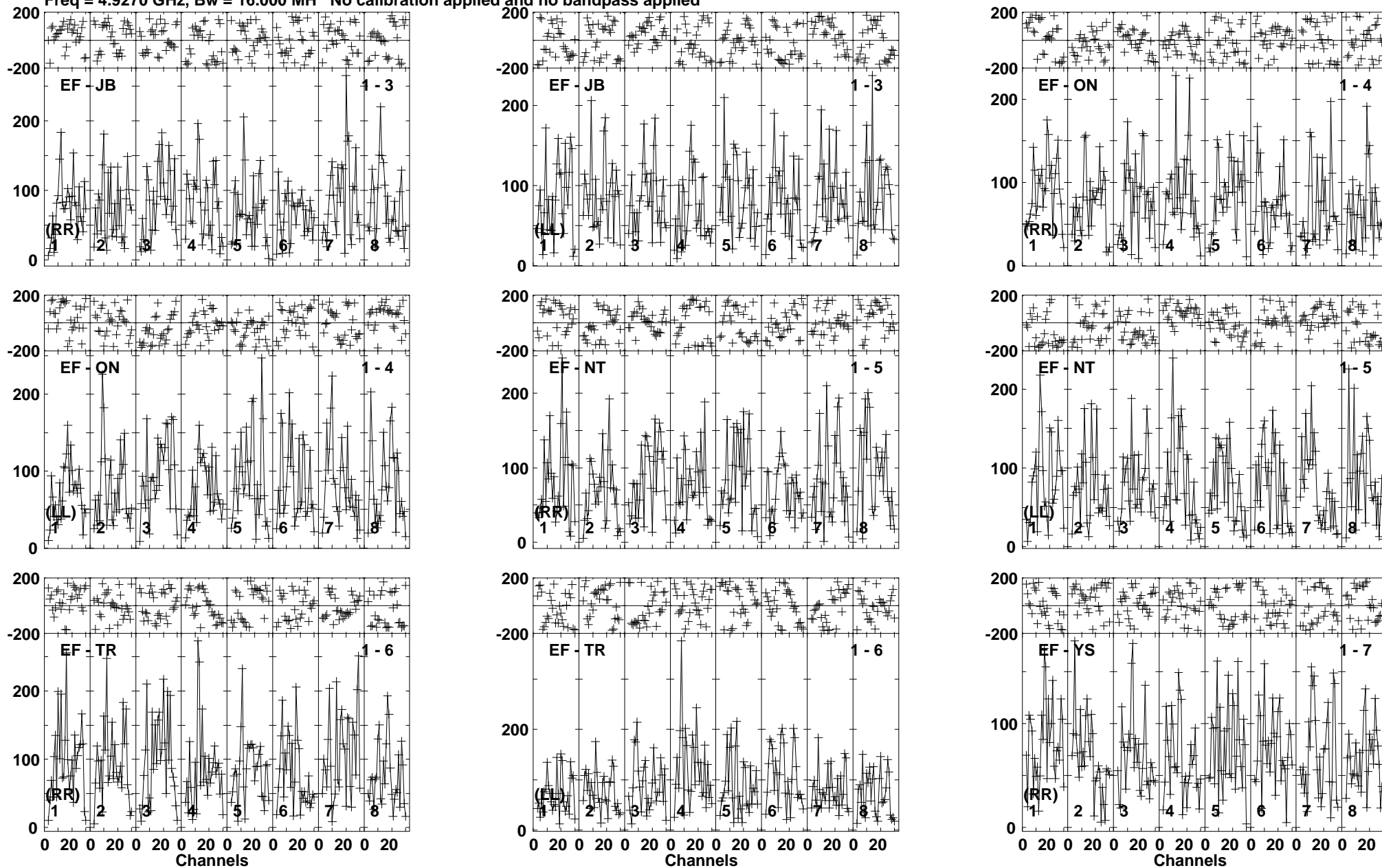
Lower frame: Micro Ampl Jy Top frame: Phas deg Vector averaged cross-power spectrum Baseline: EF (01) - JB (03) Timerange: 00/10:13:04 to 00/10:16:40
