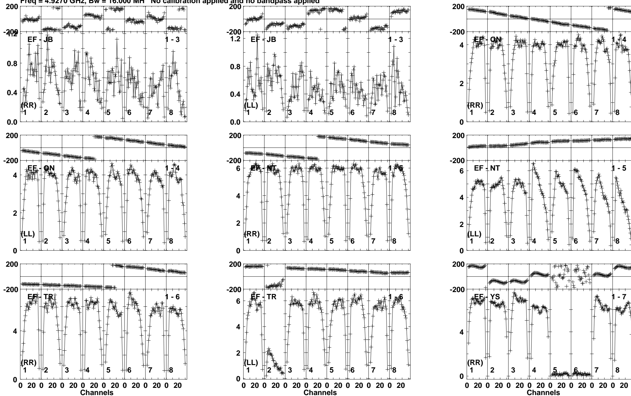
Lower frame: Milli Ampl Jy Top frame: Phas deg Vector averaged cross-power spectrum Baseline: EF (01) - JB (03) Timerange: 00/11:47:49 to 00/11:48:59
