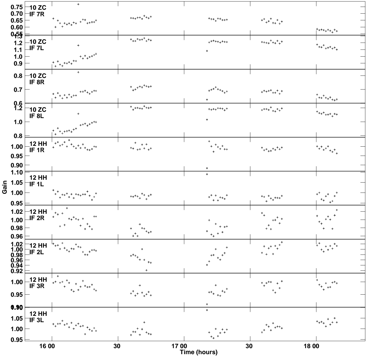
Plot file version 15 created 08-DEC-2015 18:03:45 Gain amp vs UTC time for 0845+04.MULTI.1 SN 2 Rpol & Lpol IF 1 - 8
