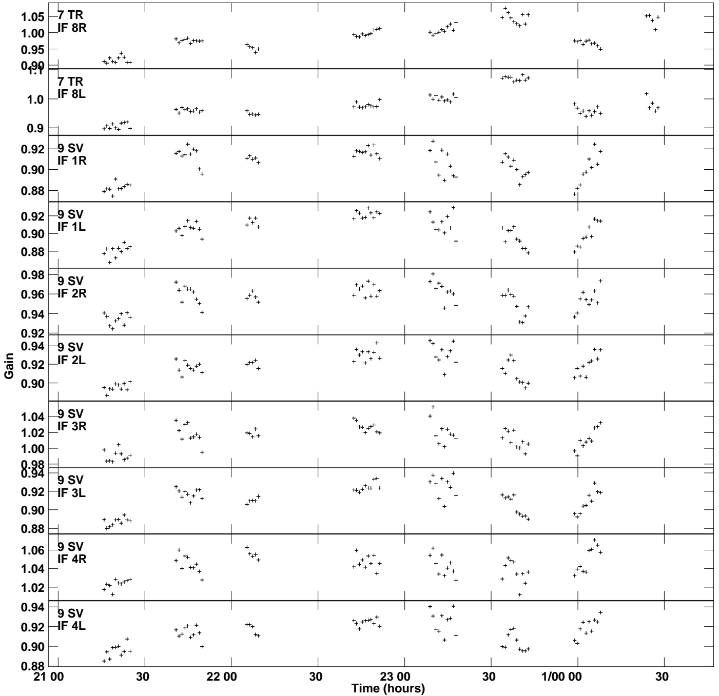
Plot file version 12 created 08-DEC-2015 18:01:55 Gain amp vs UTC time for 1405+04.MULTI.1 SN 2 Rpol & Lpol IF 1 - 8
