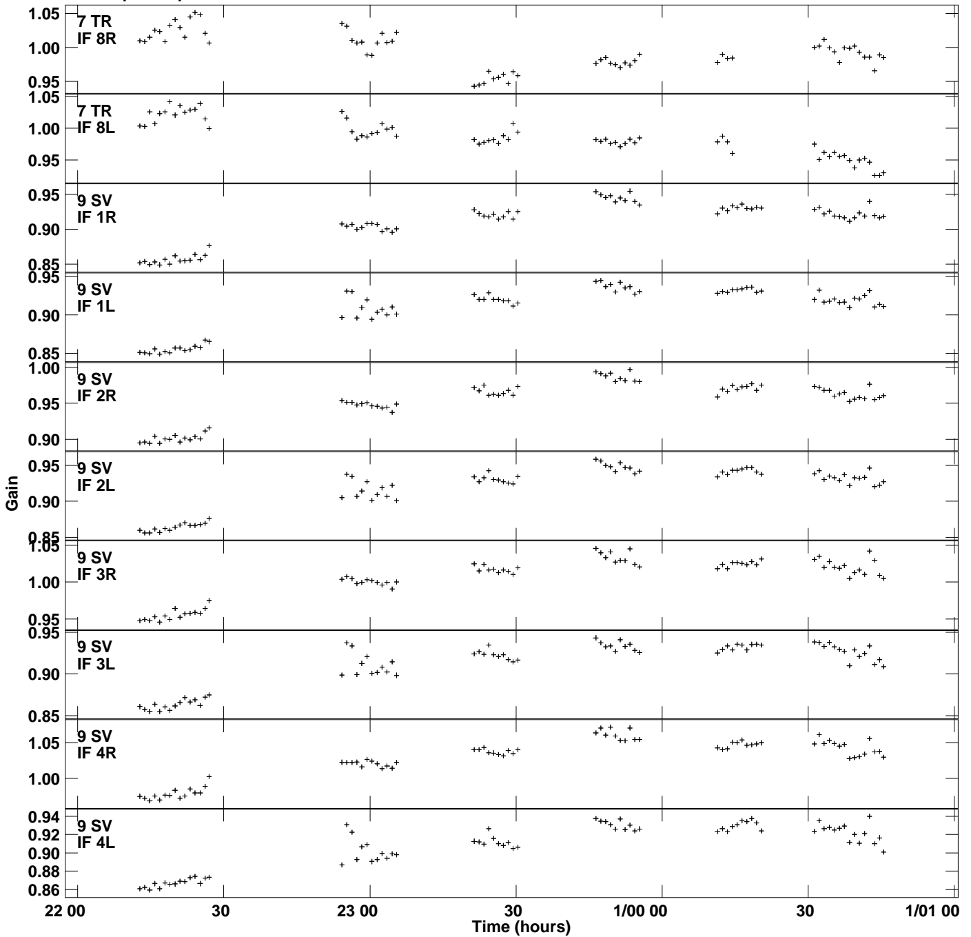
Plot file version 12 created 08-DEC-2015 18:01:35 Gain amp vs UTC time for 1616+04.MULTI.1 SN 2 Rpol & Lpol IF 1 - 8
