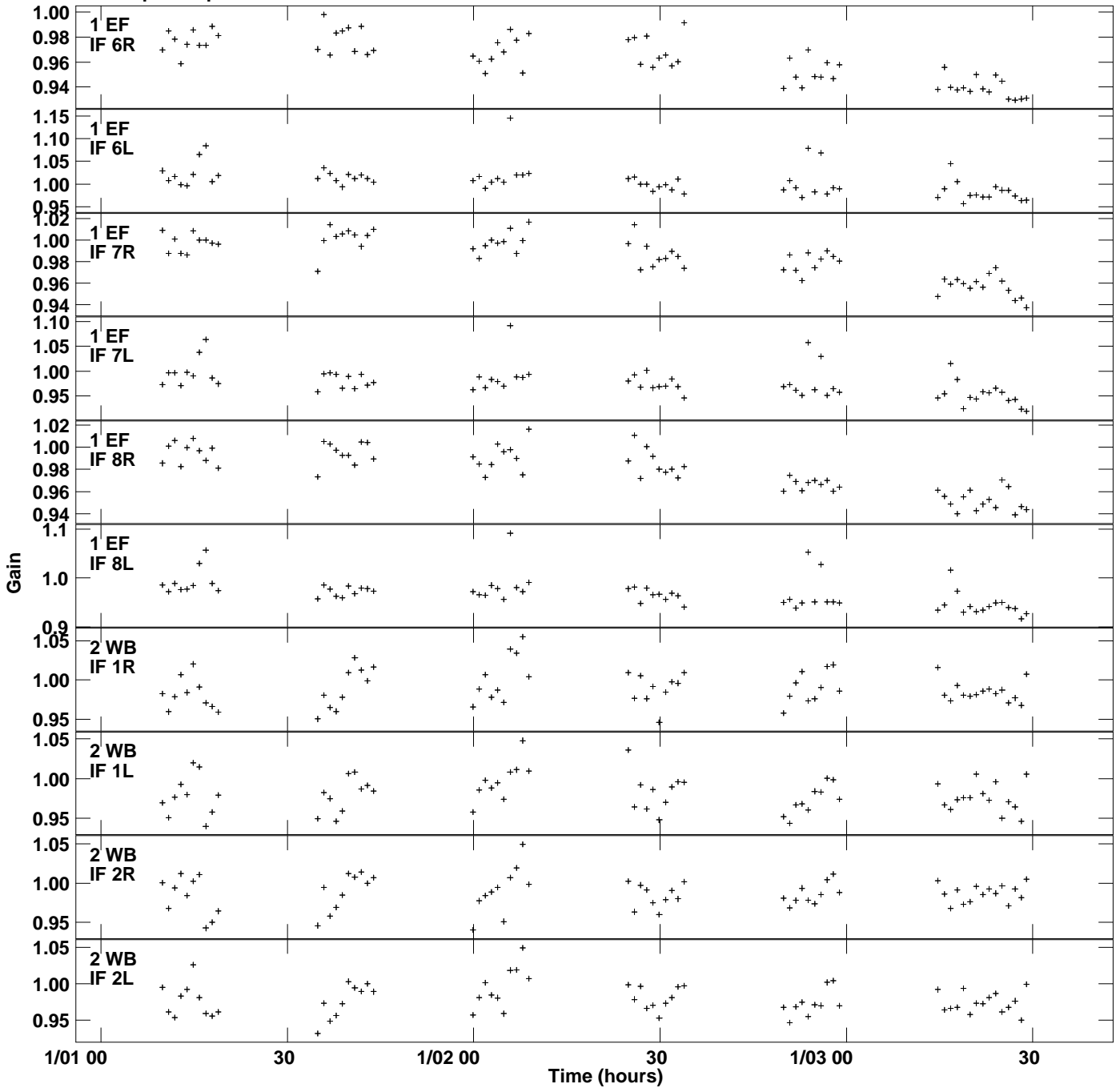
Plot file version 2 created 08-DEC-2015 18:03:24 Gain amp vs UTC time for 2245+03.MULTI.1 SN 2 Rpol & Lpol IF 1 - 8
