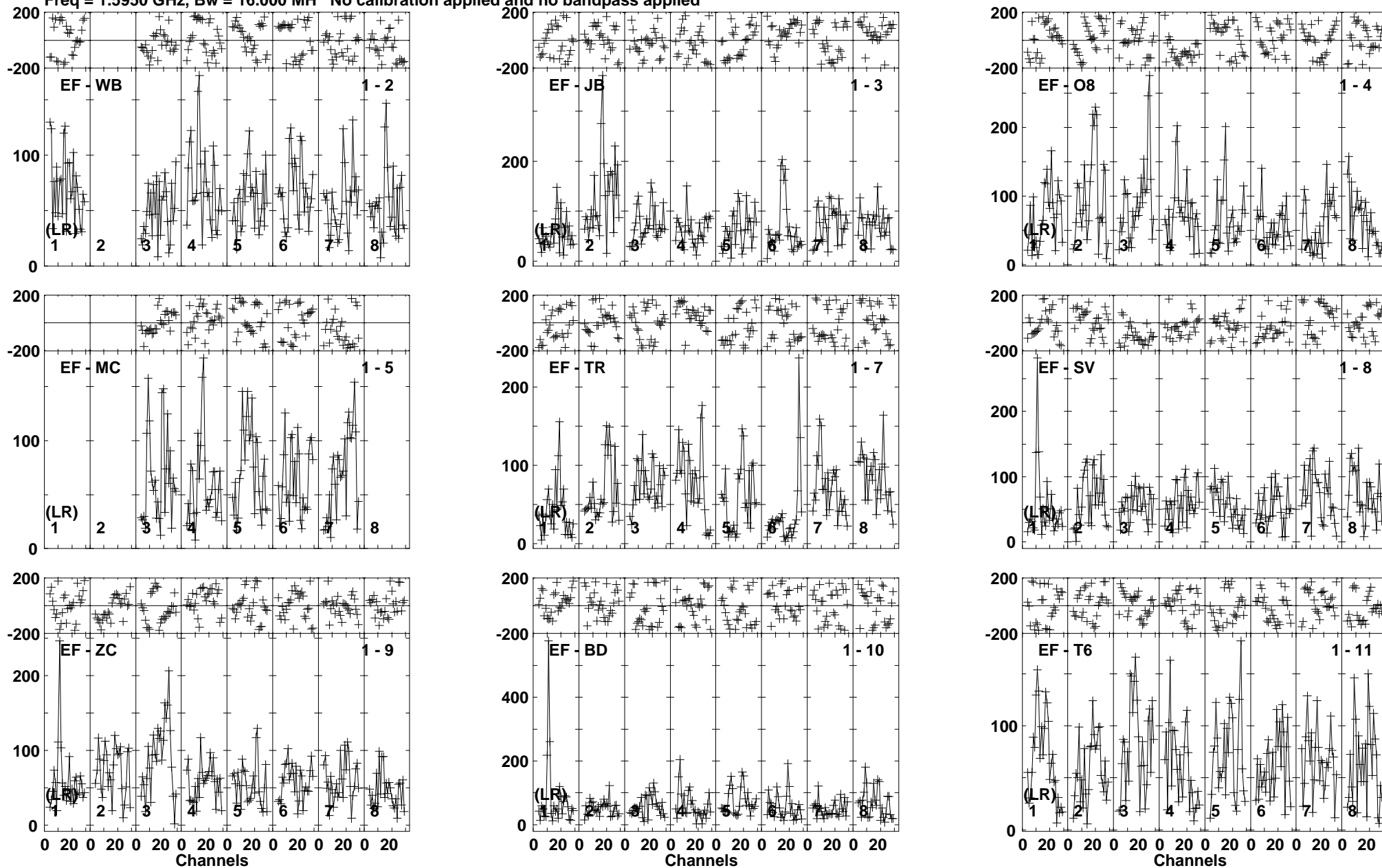
Lower frame: Micro Ampl Jy Top frame: Phas deg Vector averaged cross-power spectrum Baseline: EF (01) - WB (02) Timerange: 00/16:08:22 to 00/16:12:18
