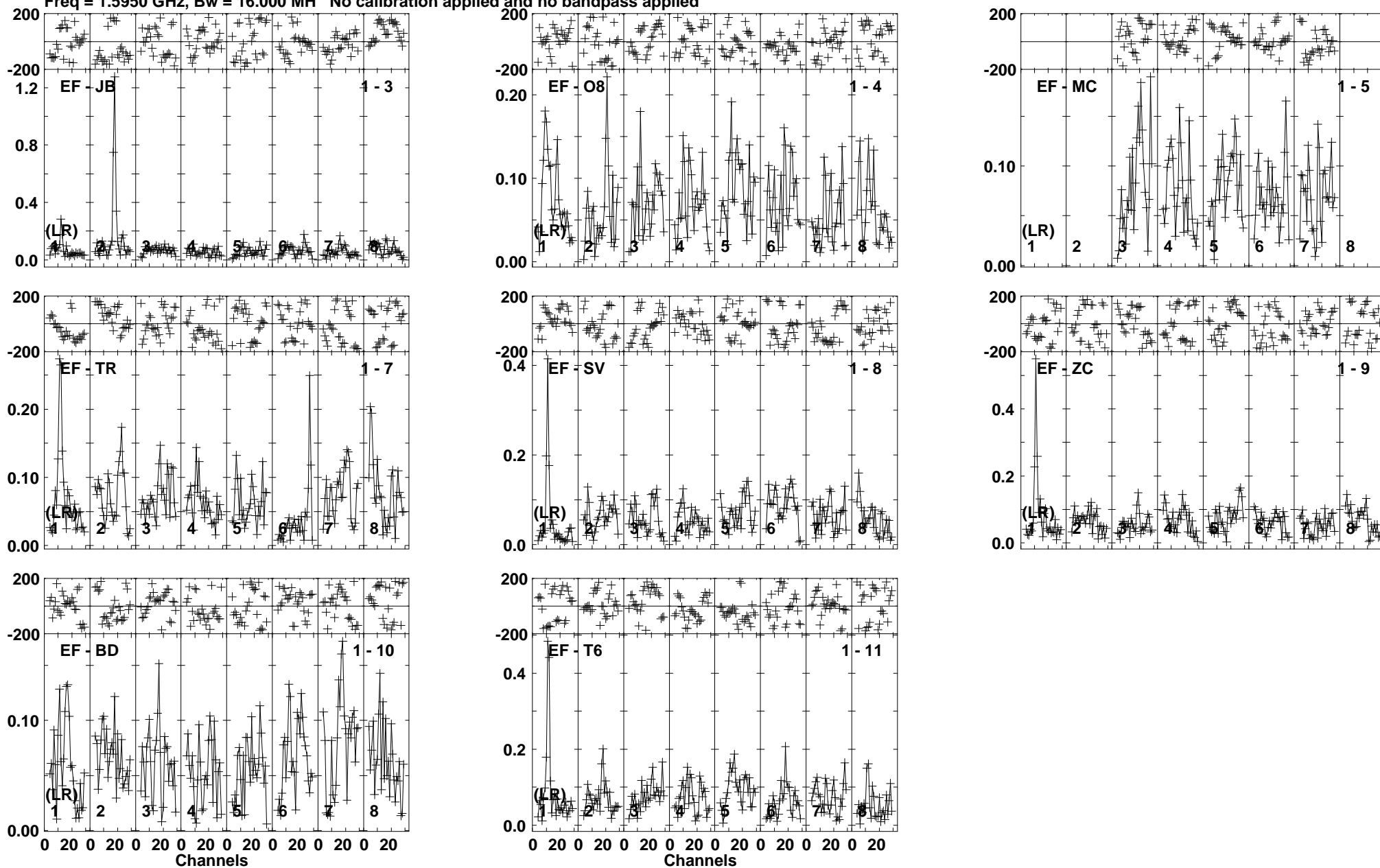
Lower frame: Milli Ampl Jy Top frame: Phas deg Vector averaged cross-power spectrum Baseline: EF (01) - JB (03) Timerange: 00/14:45:43 to 00/14:49:39
