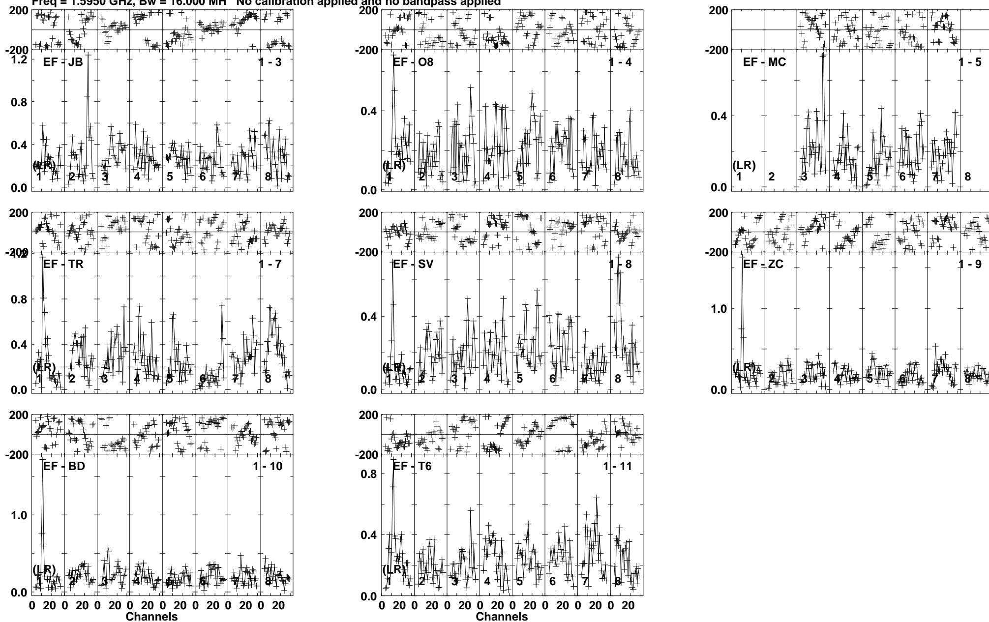
Lower frame: Milli Ampl Jy Top frame: Phas deg Vector averaged cross-power spectrum Baseline: EF (01) - JB (03) Timerange: 00/14:55:26 to 00/14:55:54
