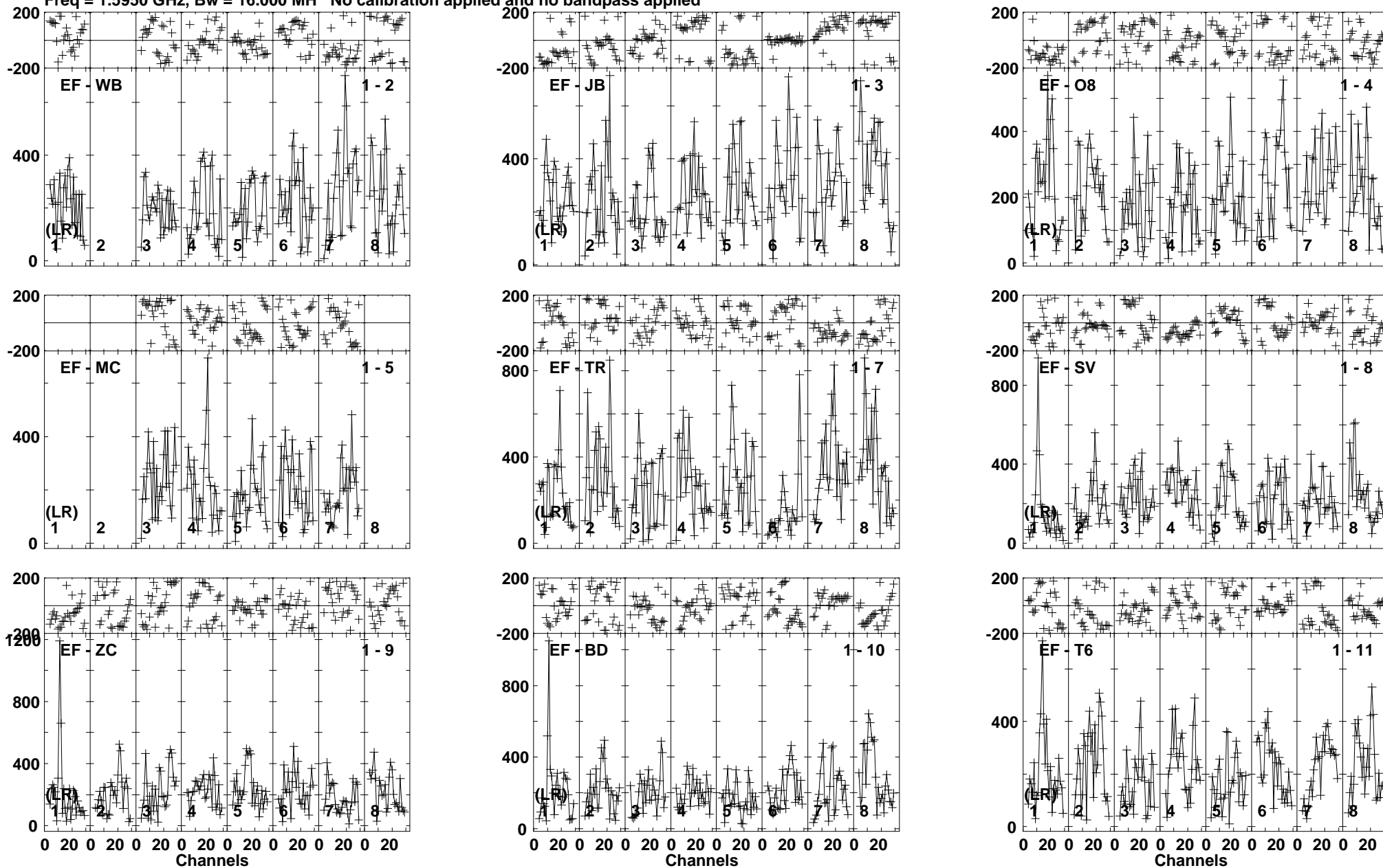
Lower frame: Micro Ampl Jy Top frame: Phas deg Vector averaged cross-power spectrum Baseline: EF (01) - WB (02) Timerange: 00/16:18:08 to 00/16:18:34
