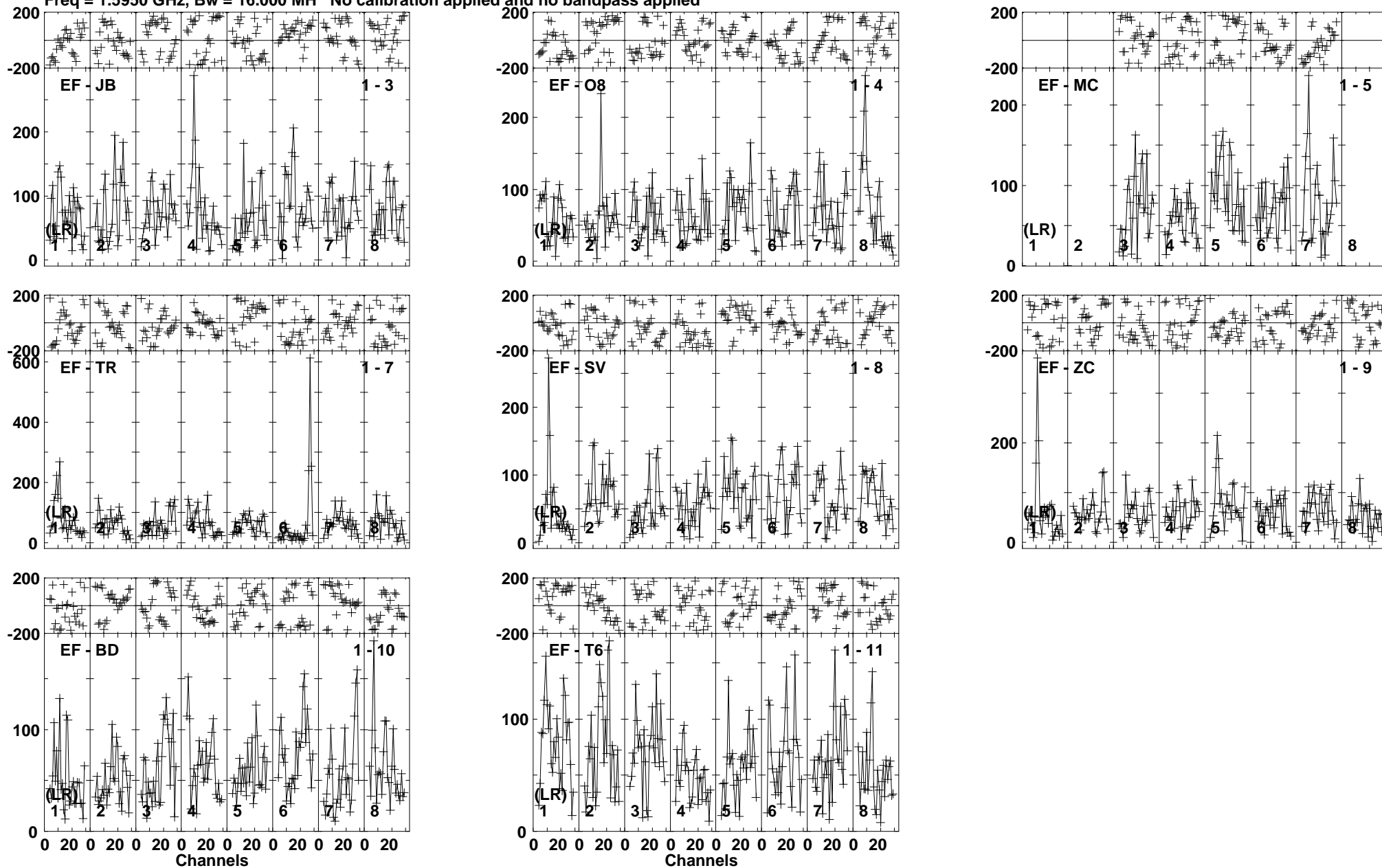
Lower frame: Micro Ampl Jy Top frame: Phas deg Vector averaged cross-power spectrum Baseline: EF (01) - JB (03) Timerange: 00/11:44:44 to 00/11:48:44
