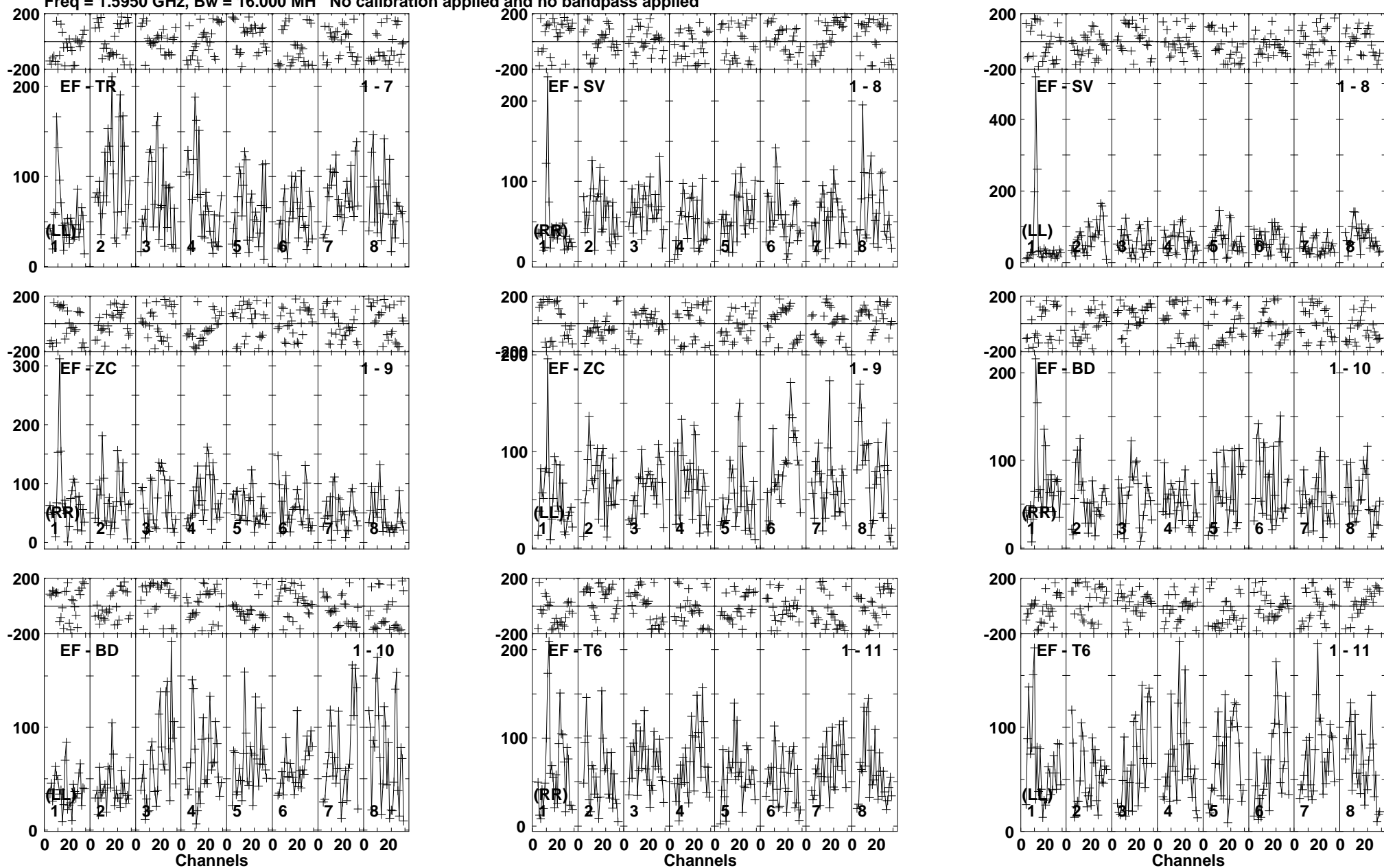
Lower frame: Micro Ampl Jy Top frame: Phas deg Vector averaged cross-power spectrum Baseline: EF (01) - TR (07) Timerange: 00/15:21:44 to 00/15:25:44
