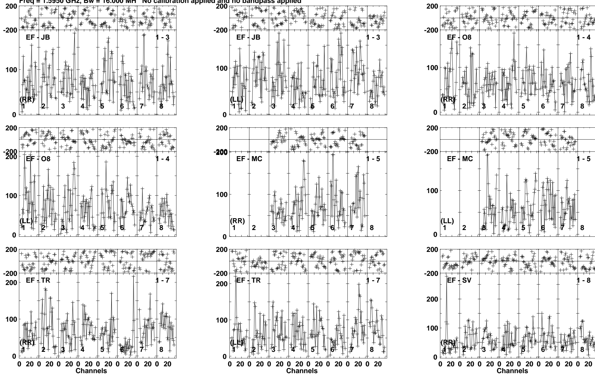
Lower frame: Micro Ampl Jy Top frame: Phas deg Vector averaged cross-power spectrum Baseline: EF (01) - JB (03) Timerange: 00/10:53:04 to 00/10:57:04
