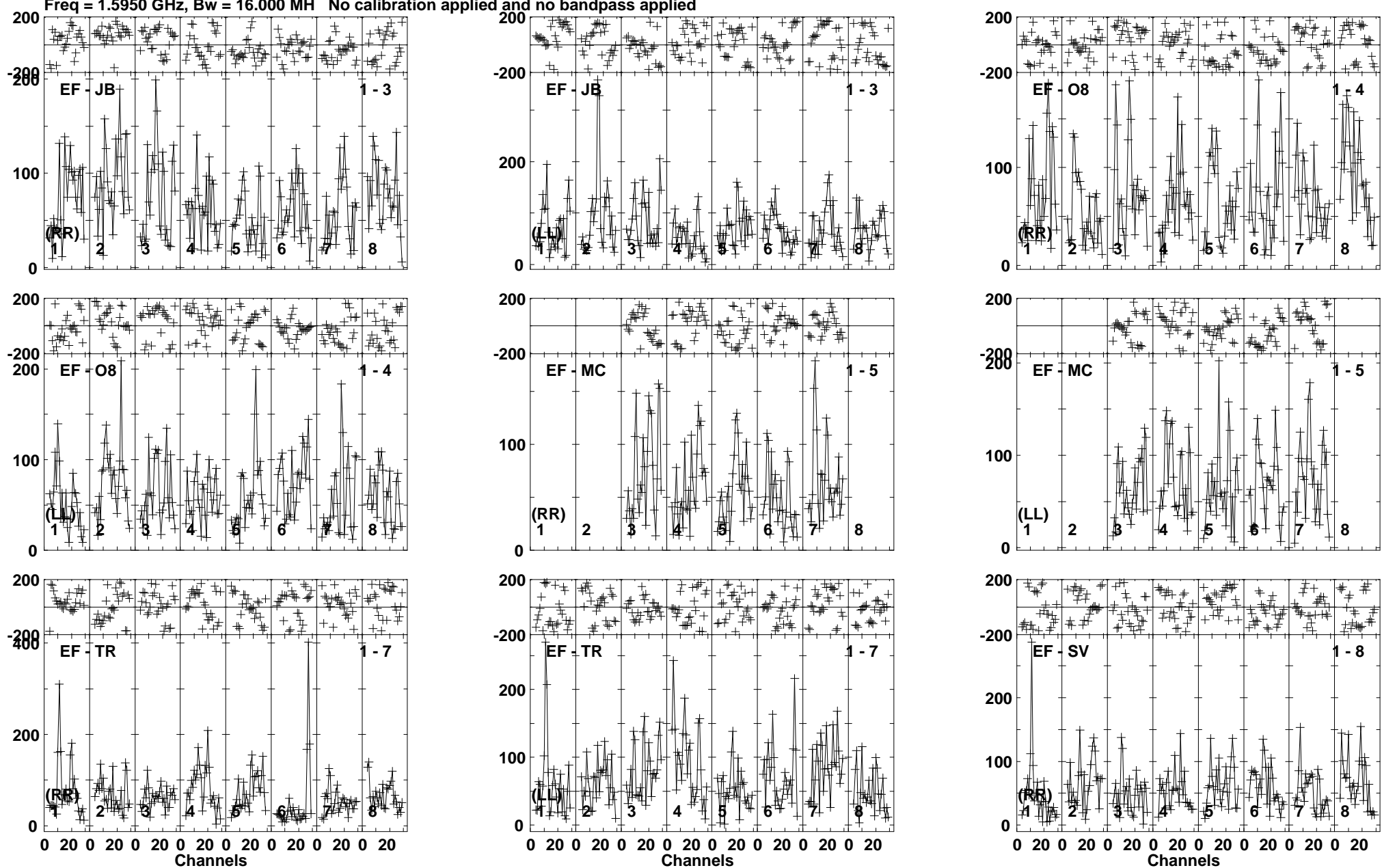
Lower frame: Micro Ampl Jy Top frame: Phas deg Vector averaged cross-power spectrum Baseline: EF (01) - JB (03) Timerange: 00/13:43:43 to 00/13:47:39
