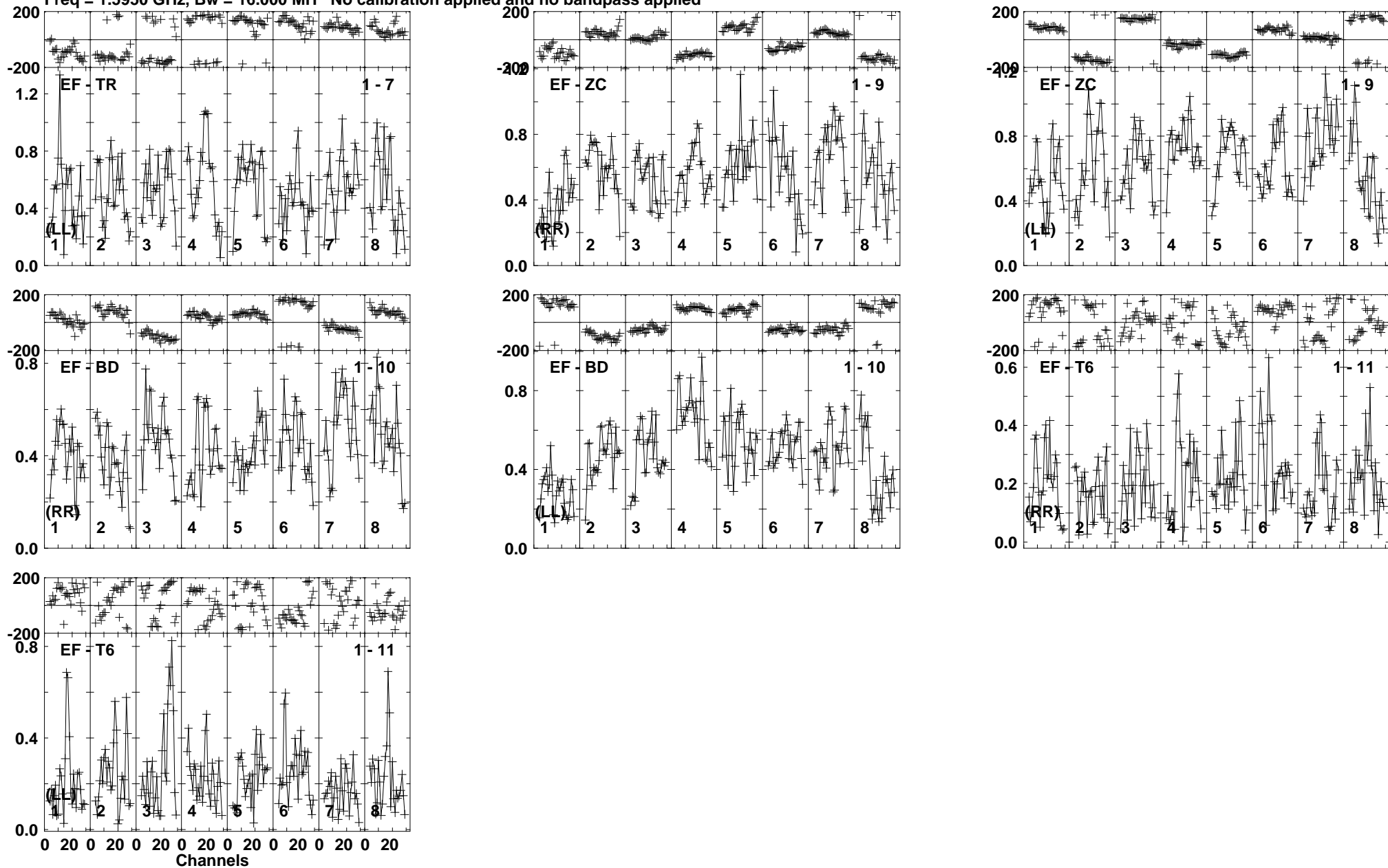
Lower frame: Milli Ampl Jy Top frame: Phas deg Vector averaged cross-power spectrum Baseline: EF (01) - TR (07) Timerange: 00/17:30:28 to 00/17:30:54
