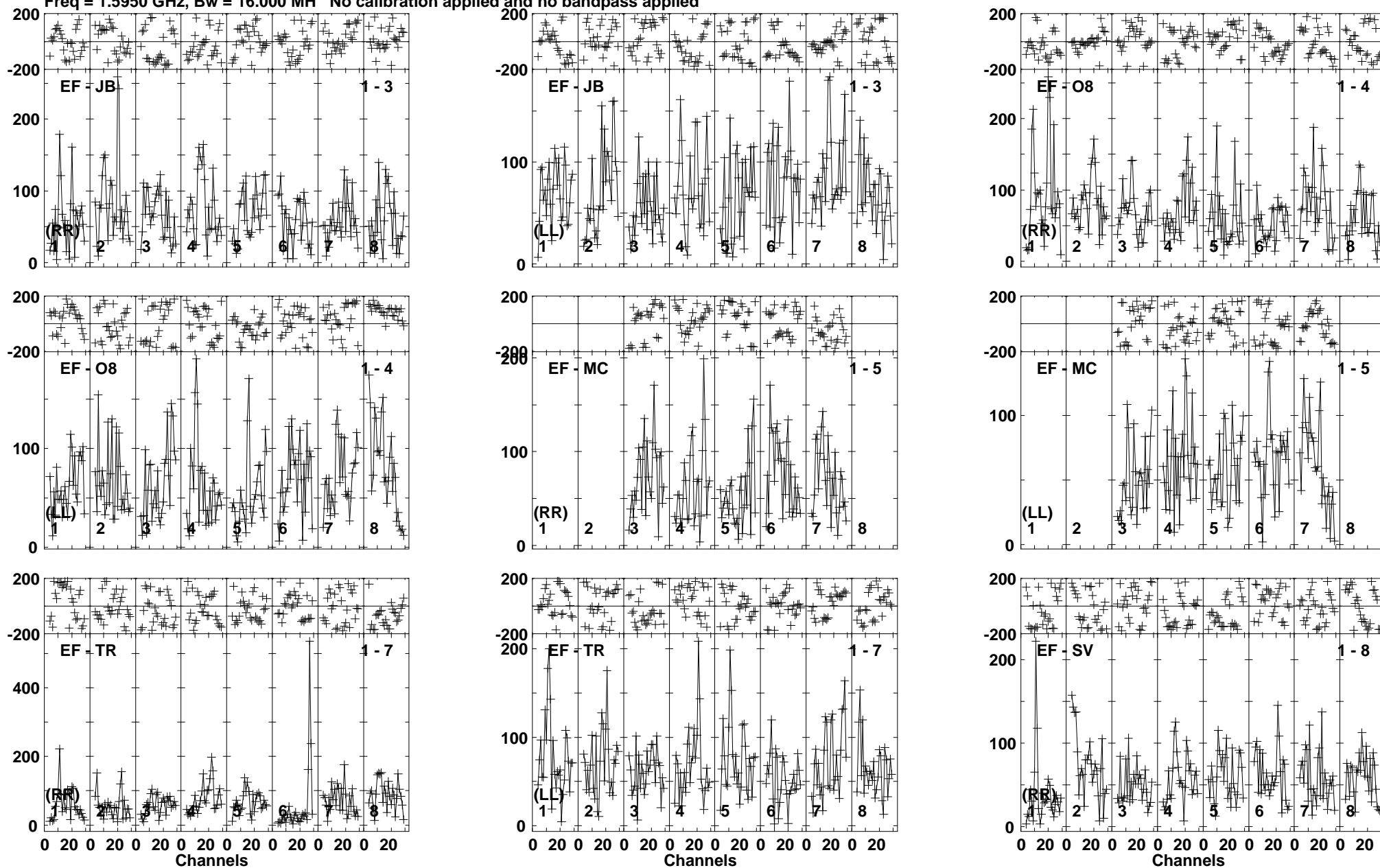
Lower frame: Micro Ampl Jy Top frame: Phas deg Vector averaged cross-power spectrum Baseline: EF (01) - JB (03) Timerange: 00/11:13:44 to 00/11:17:44
