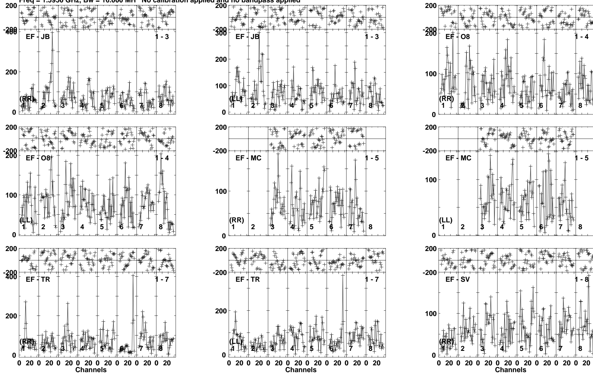
Lower frame: Micro Ampl Jy Top frame: Phas deg Vector averaged cross-power spectrum Baseline: EF (01) - JB (03) Timerange: 00/13:59:04 to 00/14:03:04
