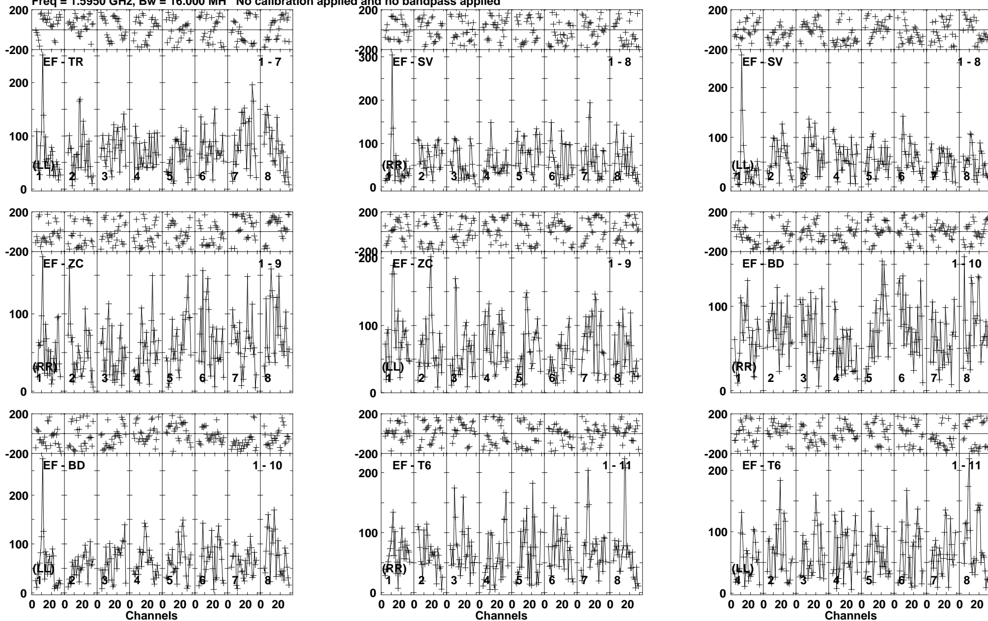
Lower frame: Micro Ampl Jy Top frame: Phas deg Vector averaged cross-power spectrum Baseline: EF (01) - TR (07) Timerange: 00/15:16:42 to 00/15:20:38
