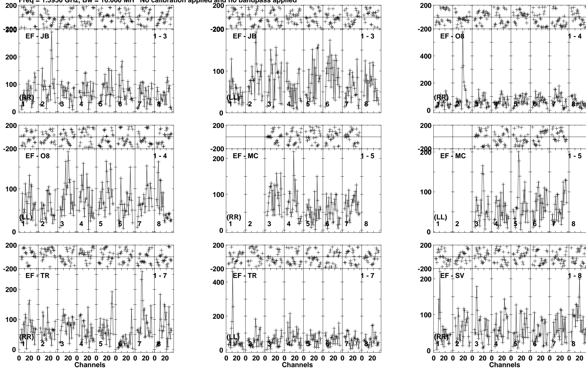
Lower frame: Micro Ampl Jy Top frame: Phas deg Vector averaged cross-power spectrum Baseline: EF (01) - JB (03) Timerange: 00/12:26:04 to 00/12:30:04
