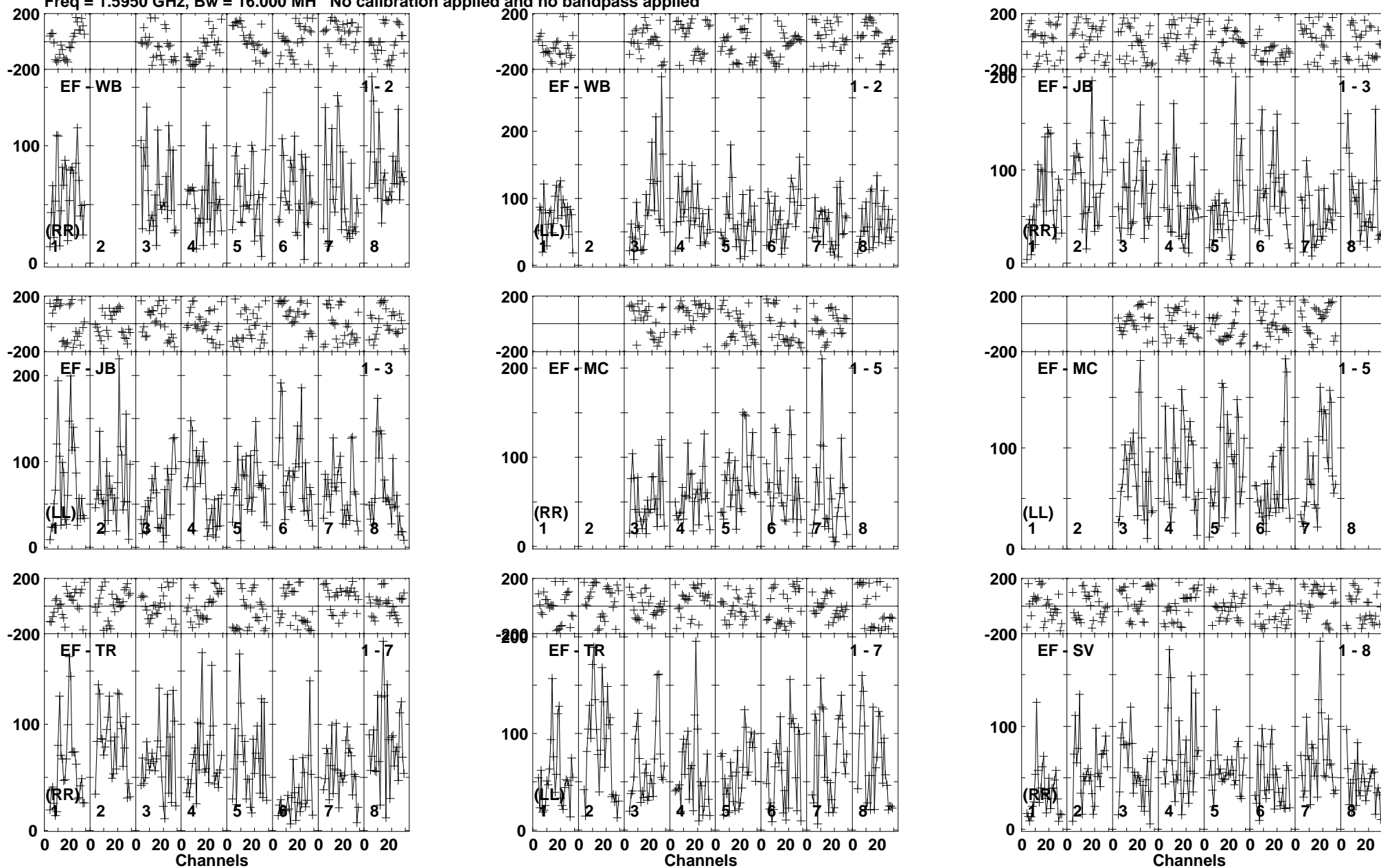
Lower frame: Micro Ampl Jy Top frame: Phas deg Vector averaged cross-power spectrum Baseline: EF (01) - WB (02) Timerange: 00/22:10:04 to 00/22:13:58
