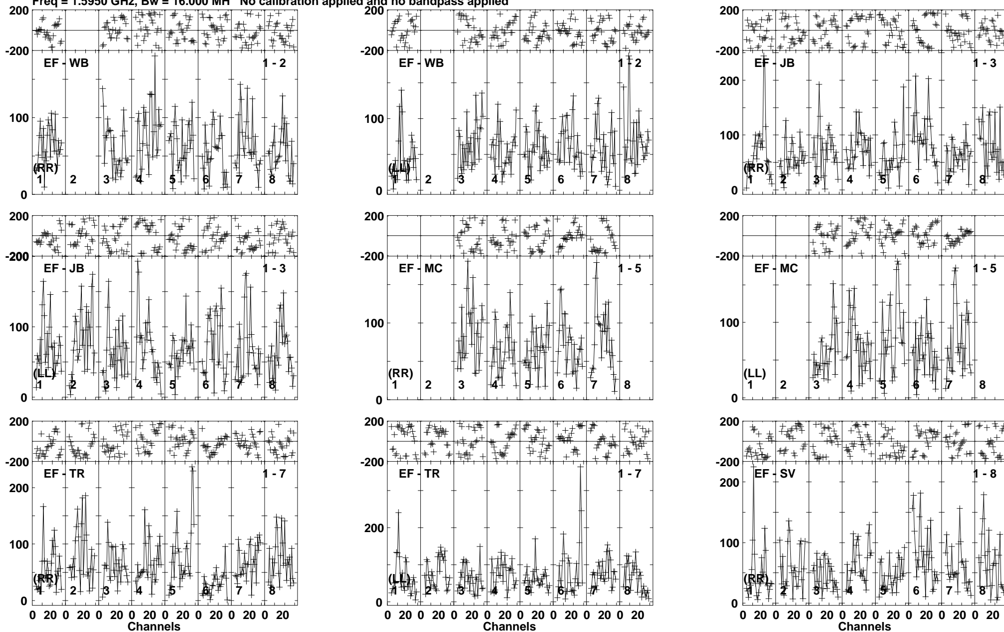
Lower frame: Micro Ampl Jy Top frame: Phas deg Vector averaged cross-power spectrum Baseline: EF (01) - WB (02) Timerange: 00/21:54:24 to 00/21:58:24
