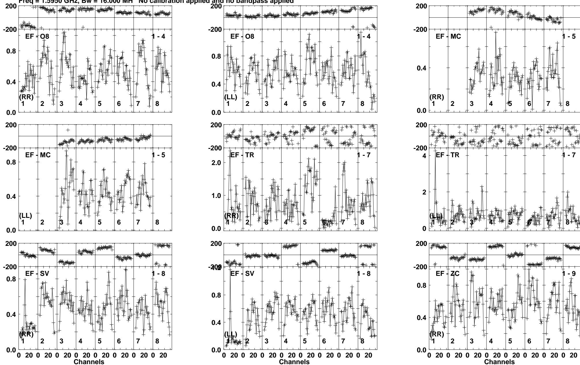
Lower frame: Milli Ampl Jy Top frame: Phas deg Vector averaged cross-power spectrum Baseline: EF (01) - O8 (04) Timerange: 00/13:58:08 to 00/13:58:58
