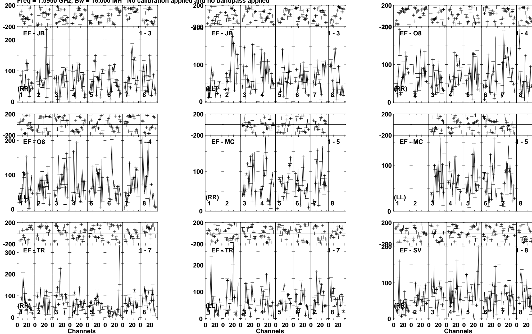
Lower frame: Micro Ampl Jy Top frame: Phas deg Vector averaged cross-power spectrum Baseline: EF (01) - JB (03) Timerange: 00/15:06:22 to 00/15:10:18
