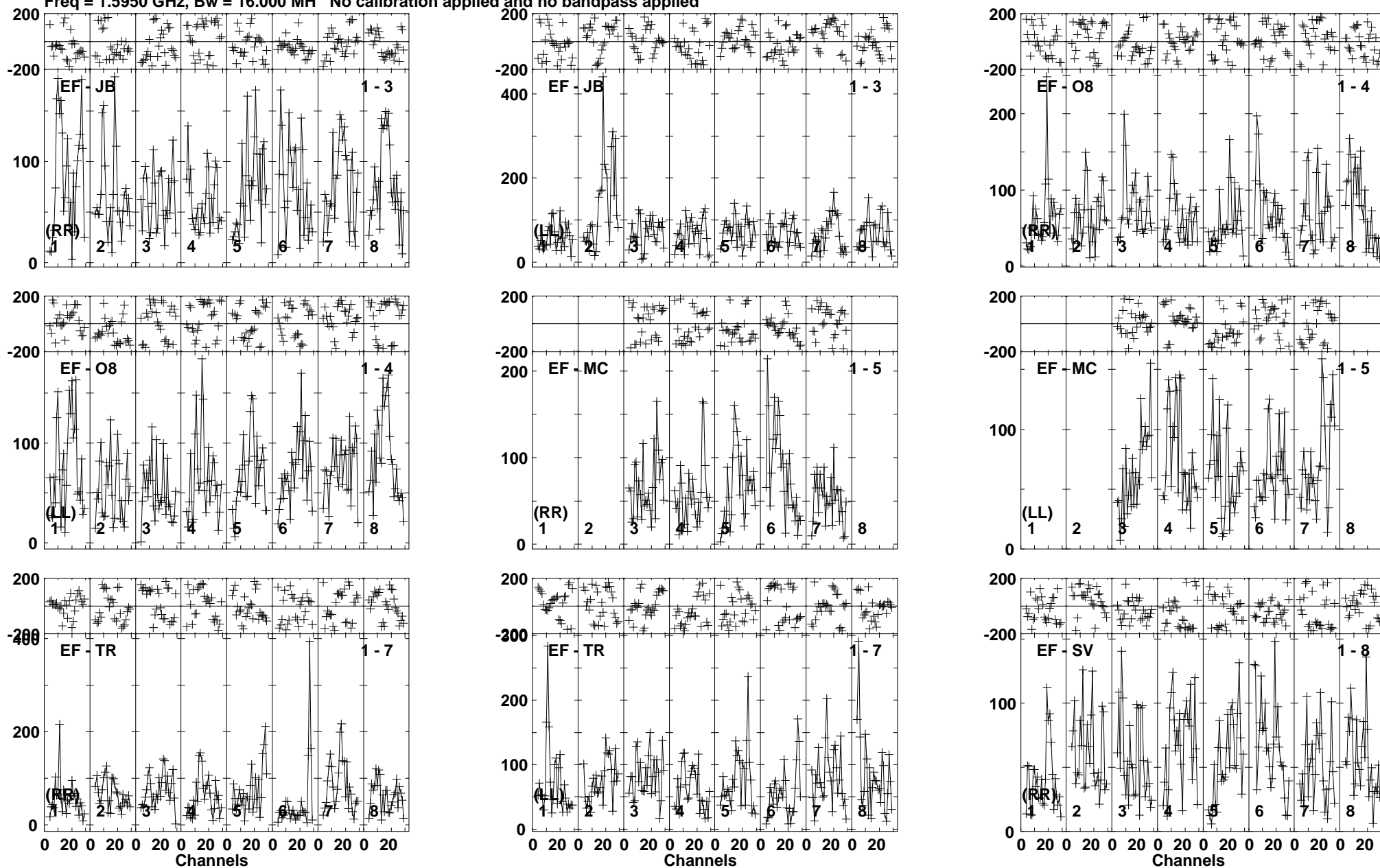
Lower frame: Micro Ampl Jy Top frame: Phas deg Vector averaged cross-power spectrum Baseline: EF (01) - JB (03) Timerange: 00/12:52:03 to 00/12:55:59
