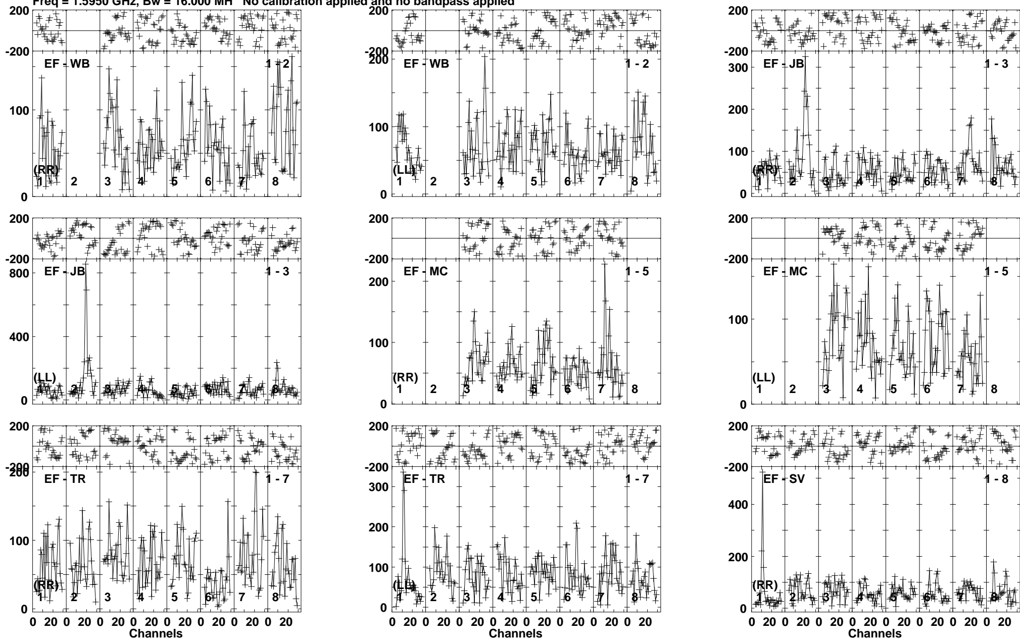
Lower frame: Micro Ampl Jy Top frame: Phas deg Vector averaged cross-power spectrum Baseline: EF (01) - WB (02) Timerange: 00:19:50:24 to 00:19:54:24
