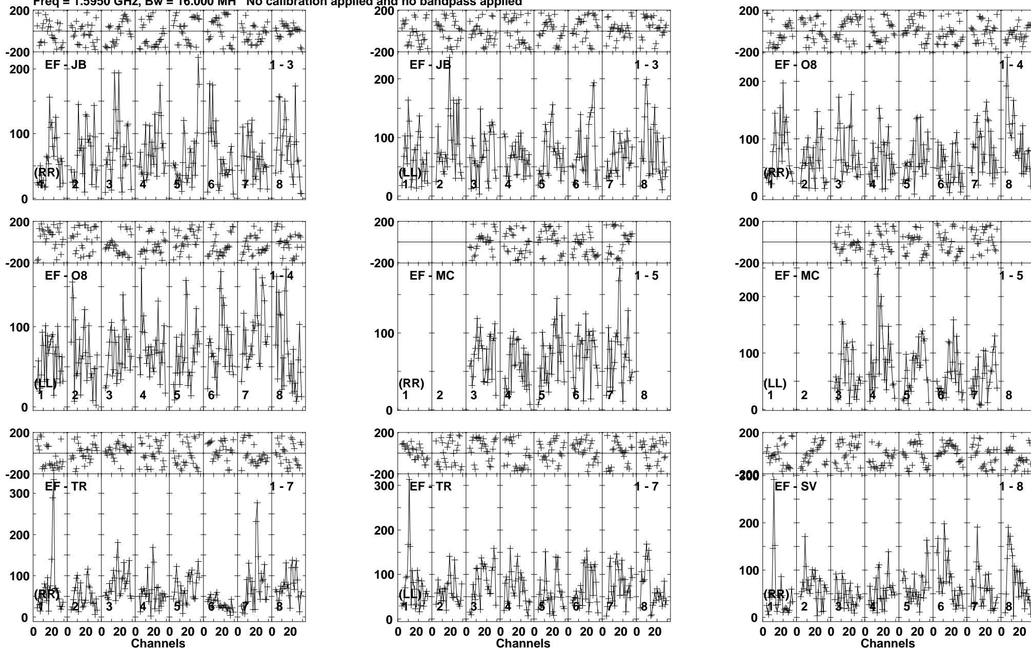
Lower frame: Micro Ampl Jy Top frame: Phas deg Vector averaged cross-power spectrum Baseline: EF (01) - JB (03) Timerange: 00/13:07:24 to 00/13:11:24
