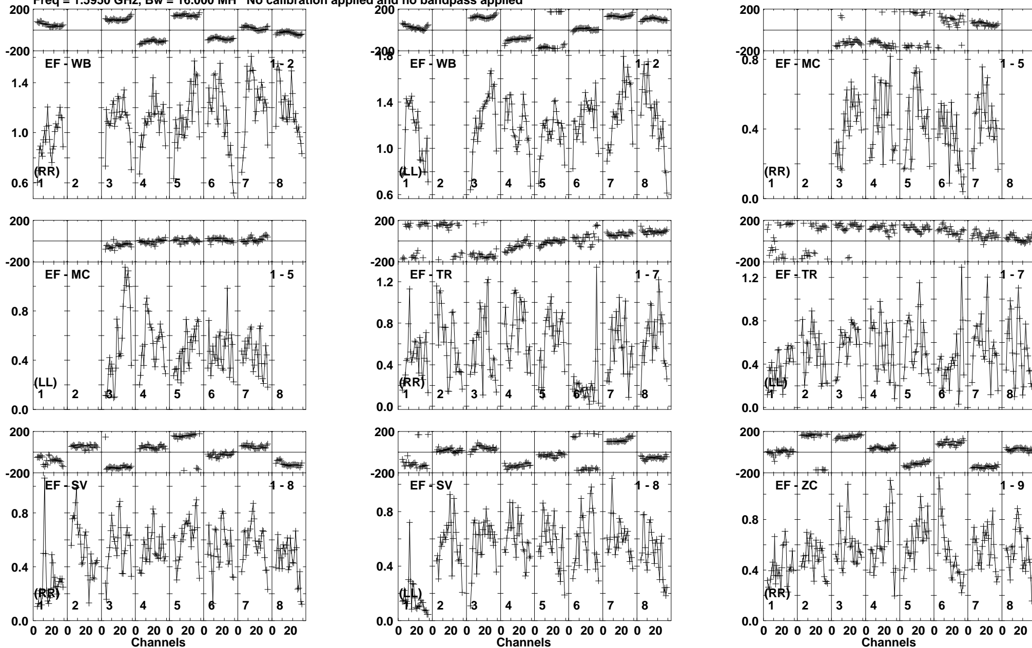
Lower frame: Milli Ampl Jy Top frame: Phas deg Vector averaged cross-power spectrum Baseline: EF (01) - WB (02) Timerange: 00/21:48:46 to 00/21:49:14
