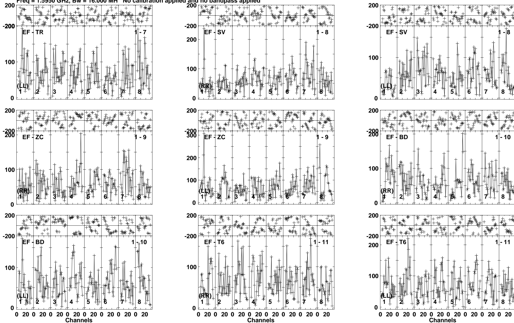
Lower frame: Micro Ampl Jy Top frame: Phas deg Vector averaged cross-power spectrum Baseline: EF (01) - TR (07) Timerange: 00/16:39:22 to 00/16:43:18
