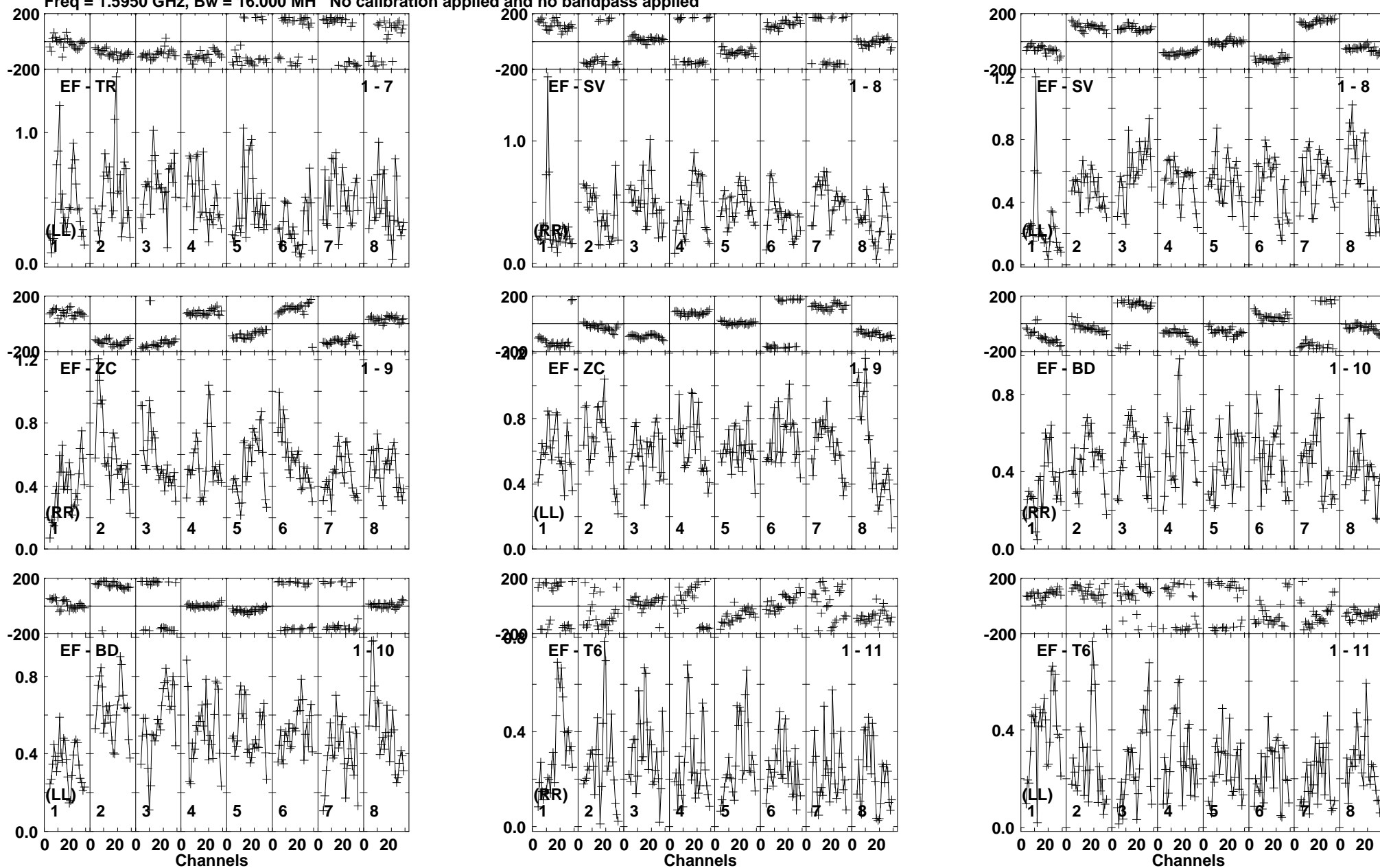
Lower frame: Milli Ampl Jy Top frame: Phas deg Vector averaged cross-power spectrum Baseline: EF (01) - TR (07) Timerange: 00/16:28:26 to 00/16:28:54
