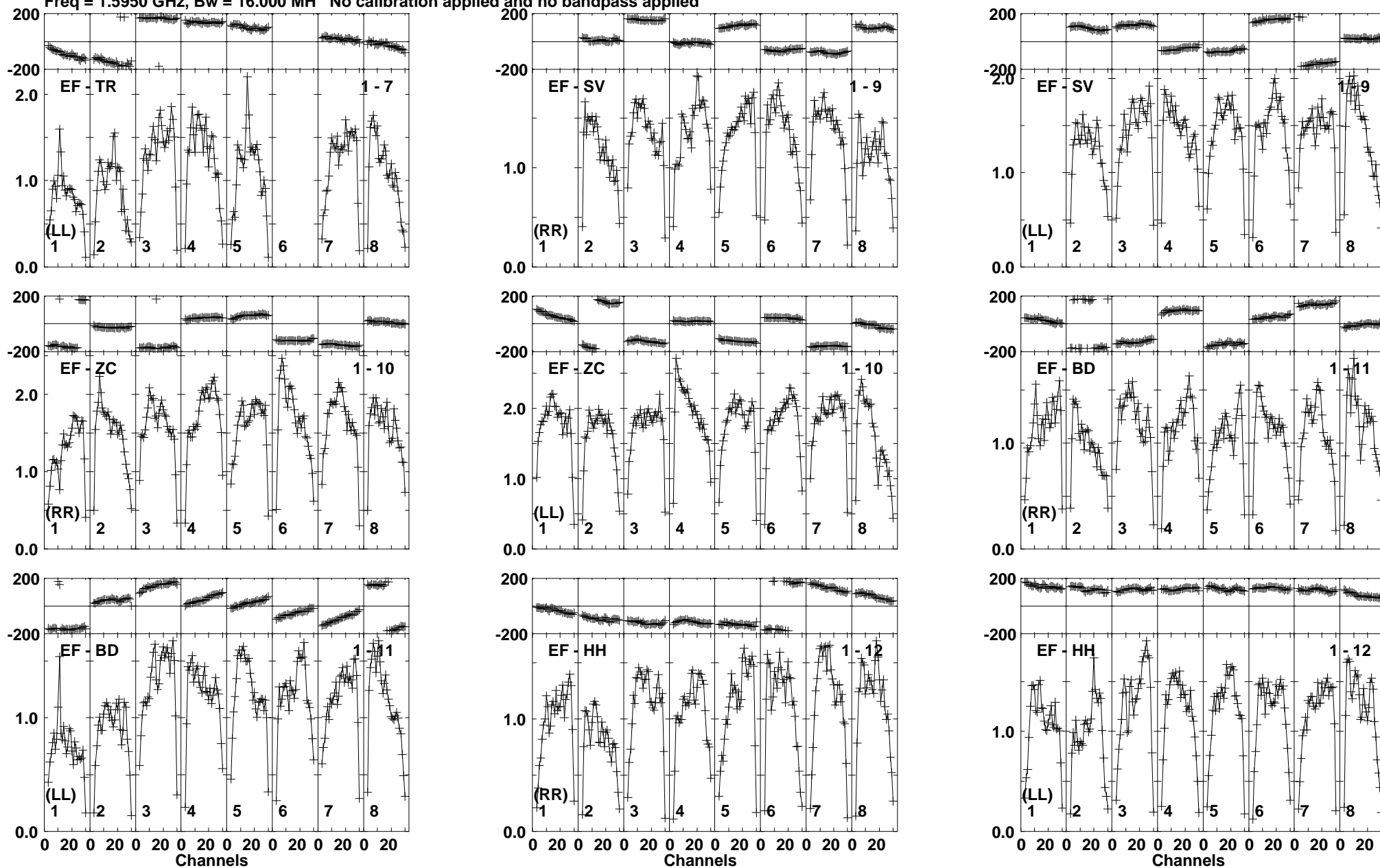
Lower frame: Milli Ampl Jy Top frame: Phas deg Vector averaged cross-power spectrum Baseline: EF (01) - TR (07) Timerange: 00/14:12:39 to 00/14:13:59
