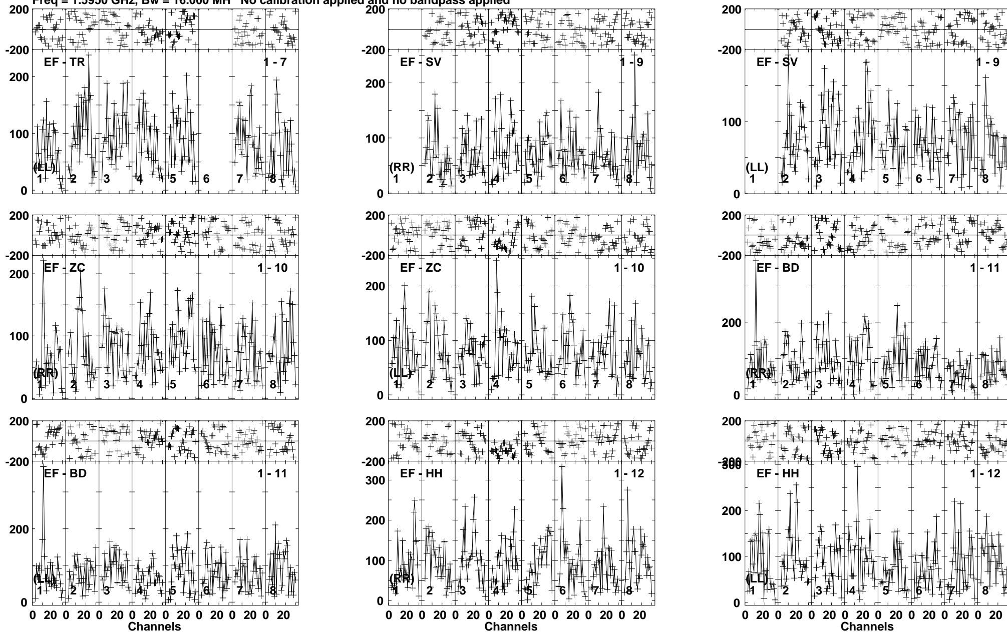
Lower frame: Micro Ampl Jy Top frame: Phas deg Vector averaged cross-power spectrum Baseline: EF (01) - TR (07) Timerange: 00/18:10:07 to 00/18:13:29
