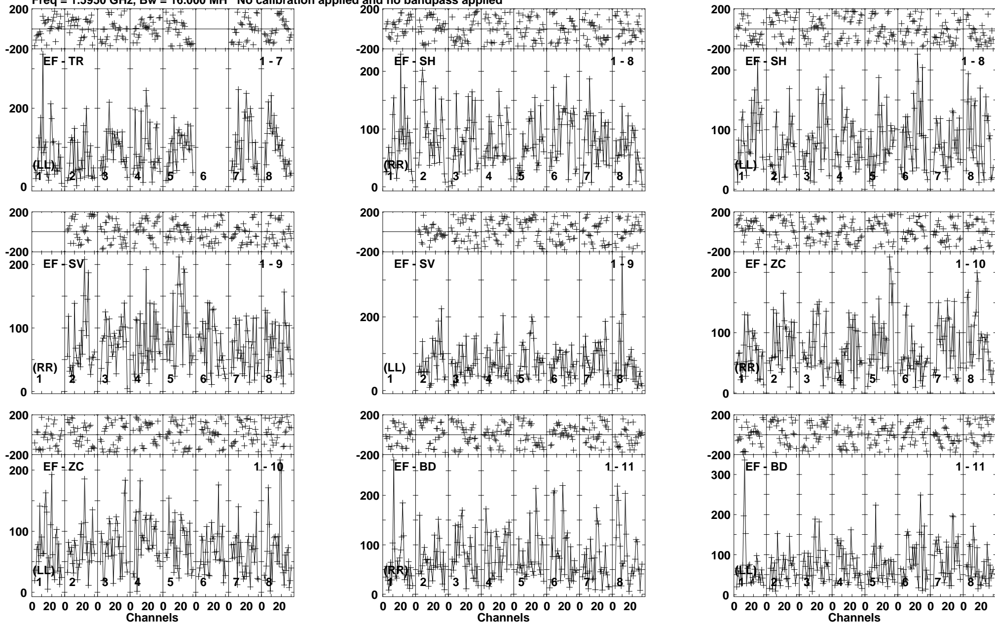
Lower frame: Micro Ampl Jy Top frame: Phas deg Vector averaged cross-power spectrum Baseline: EF (01) - TR (07) Timerange: 00/10:32:04 to 00/10:35:28
