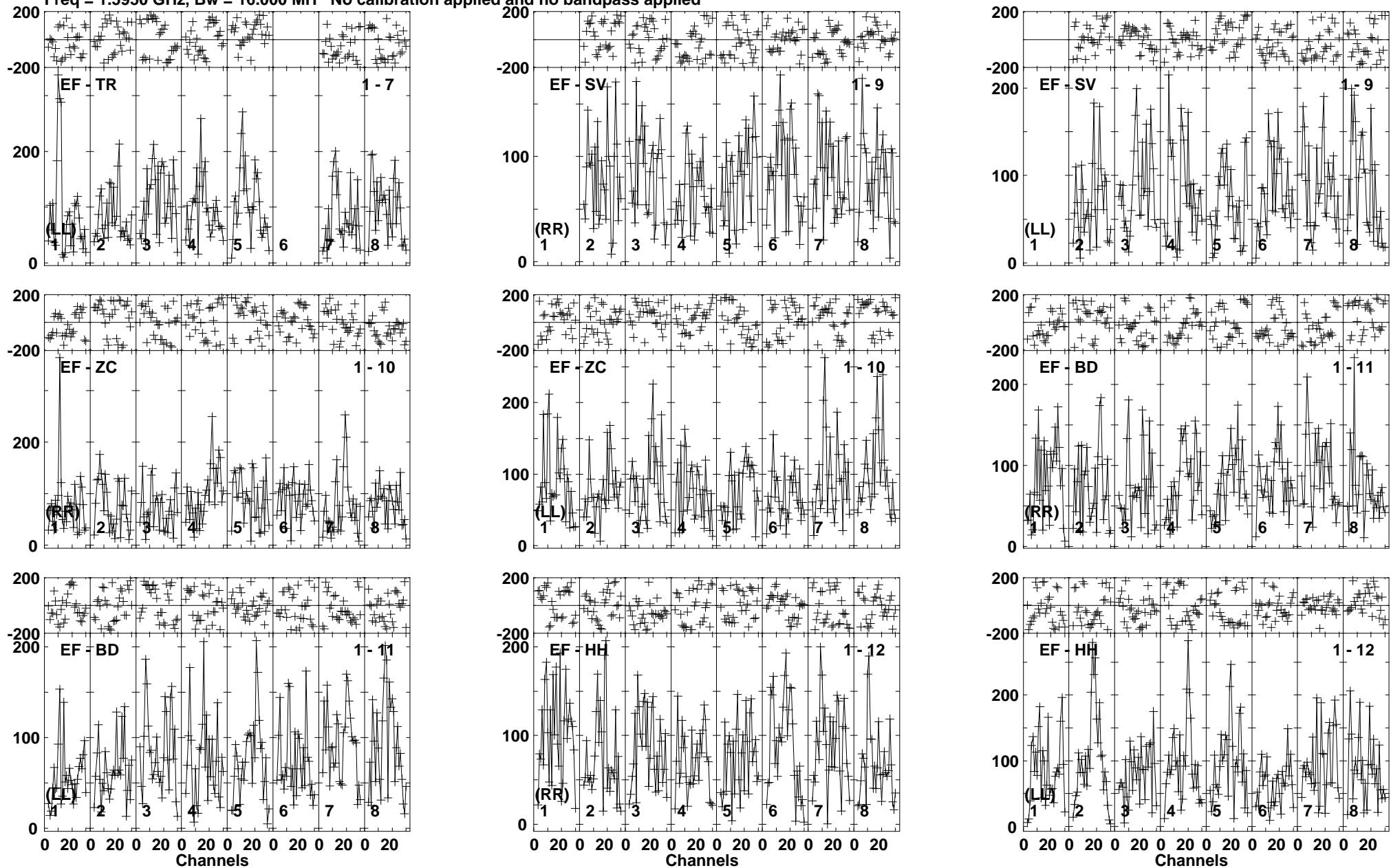
Lower frame: Micro Ampl Jy Top frame: Phas deg Vector averaged cross-power spectrum Baseline: EF (01) - TR (07) Timerange: 00/14:09:04 to 00/14:12:28
