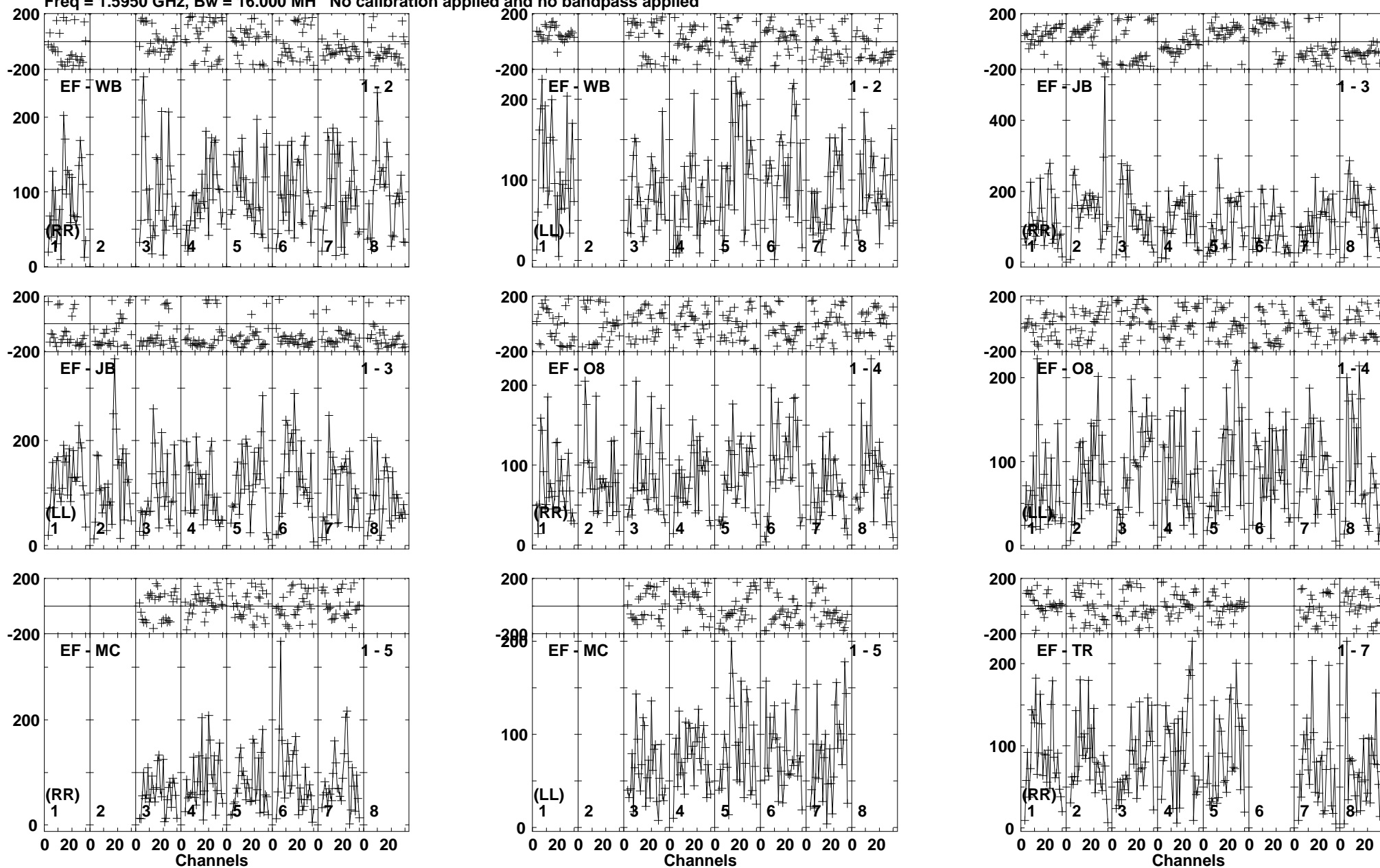
Lower frame: Micro Ampl Jy Top frame: Phas deg Vector averaged cross-power spectrum Baseline: EF (01) - WB (02) Timerange: 00/16:35:04 to 00/16:38:28
