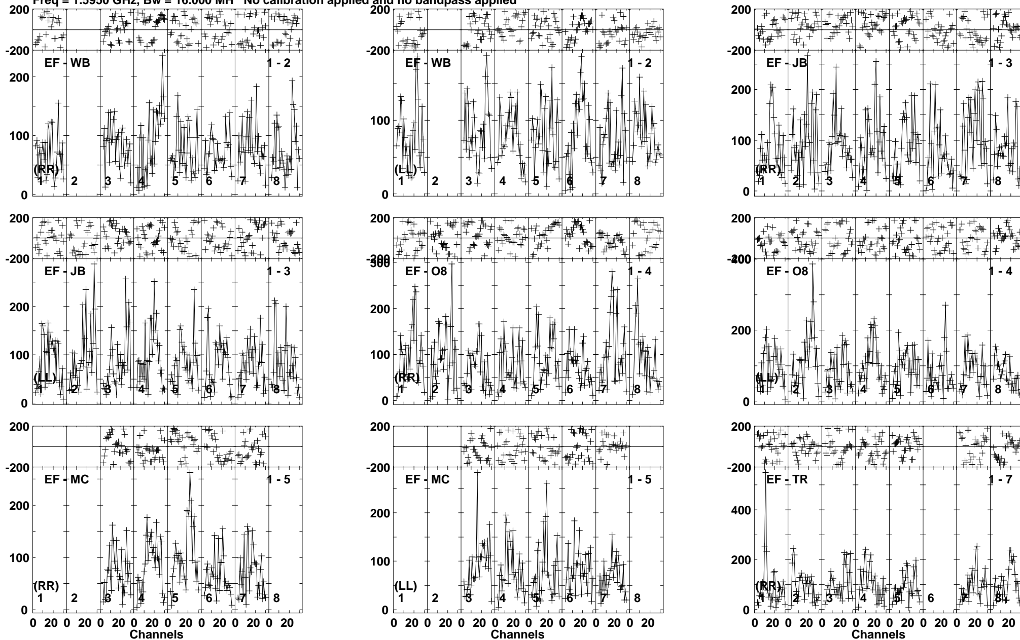
Lower frame: Micro Ampl Jy Top frame: Phas deg Vector averaged cross-power spectrum Baseline: EF (01) - WB (02) Timerange: 00/09:34:04 to 00/09:37:28
