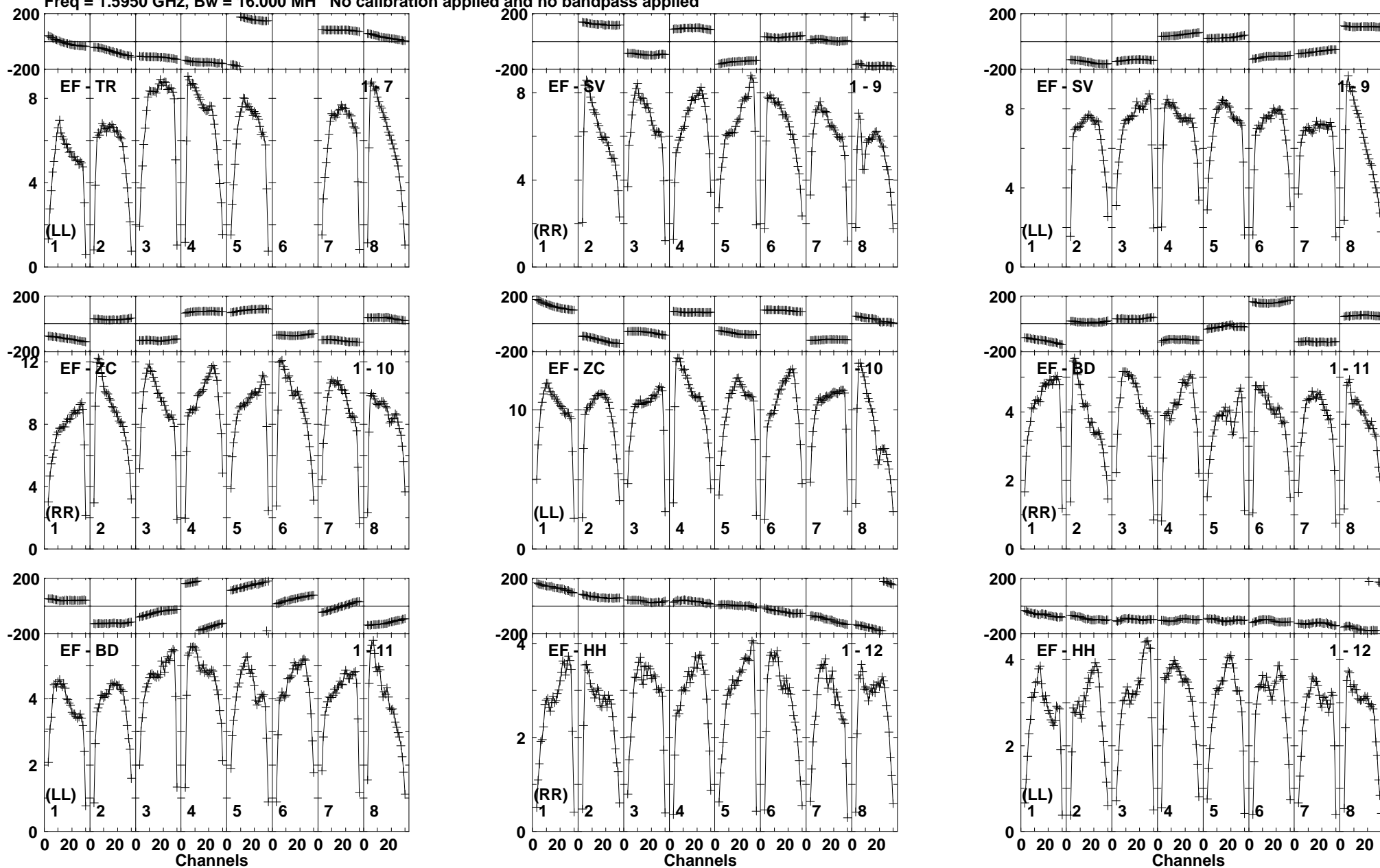
Lower frame: Milli Ampl Jy Top frame: Phas deg Vector averaged cross-power spectrum Baseline: EF (01) - TR (07) Timerange: 00/13:41:03 to 00/13:41:59
