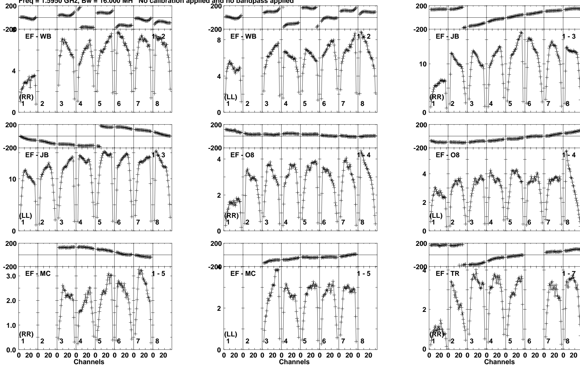
Lower frame: Milli Ampl Jy Top frame: Phas deg Vector averaged cross-power spectrum Baseline: EF (01) - WB (02) Timerange: 00/11:05:35 to 00/11:06:59
