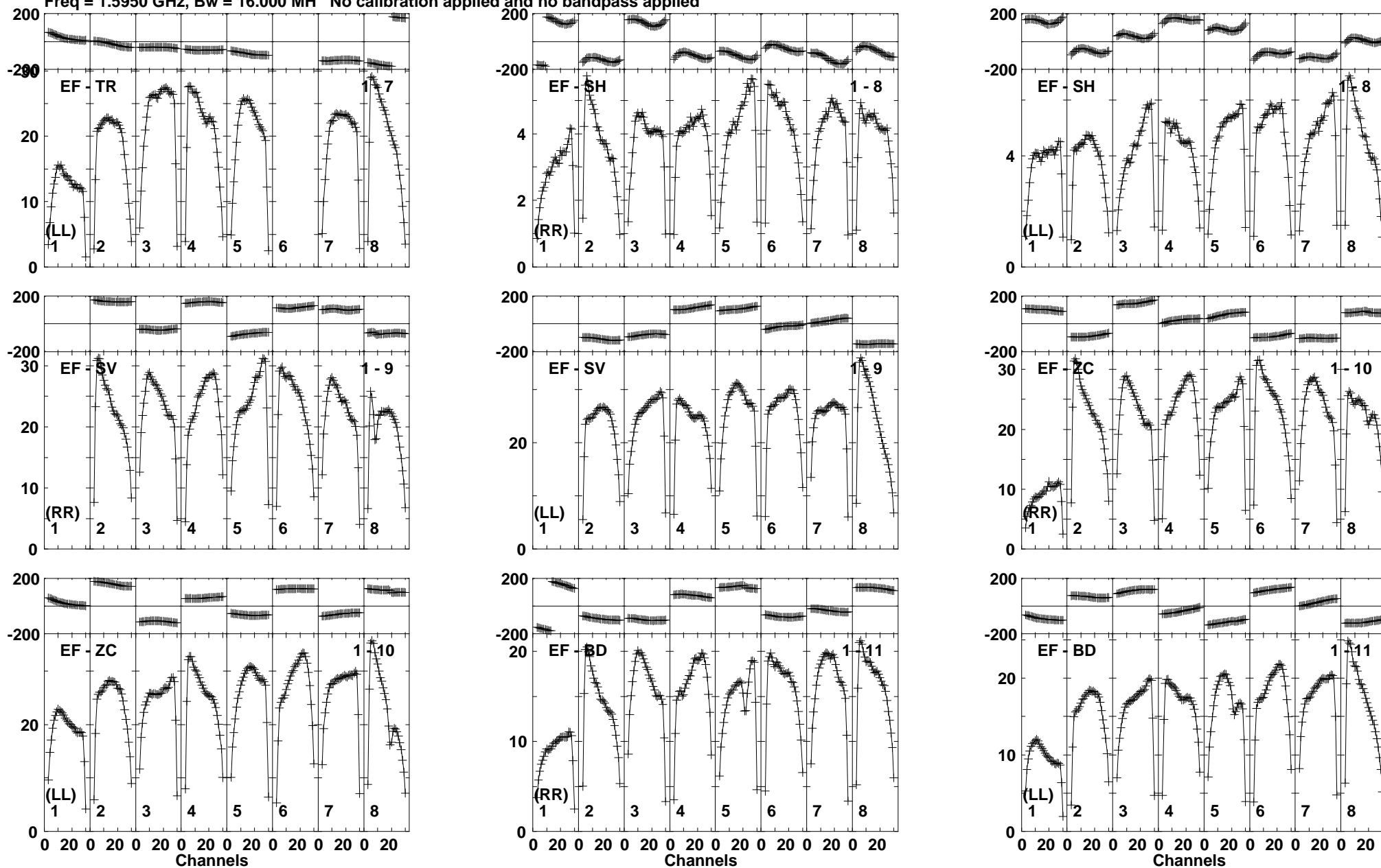
Lower frame: Milli Ampl Jy Top frame: Phas deg Vector averaged cross-power spectrum Baseline: EF (01) - TR (07) Timerange: 00/10:07:36 to 00/10:08:58
