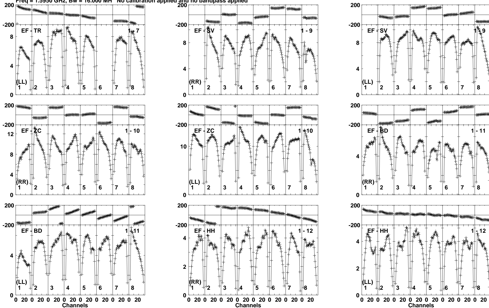
Lower frame: Milli Ampl Jy Top frame: Phas deg Vector averaged cross-power spectrum Baseline: EF (01) - TR (07) Timerange: 00/14:25:03 to 00/14:25:59
