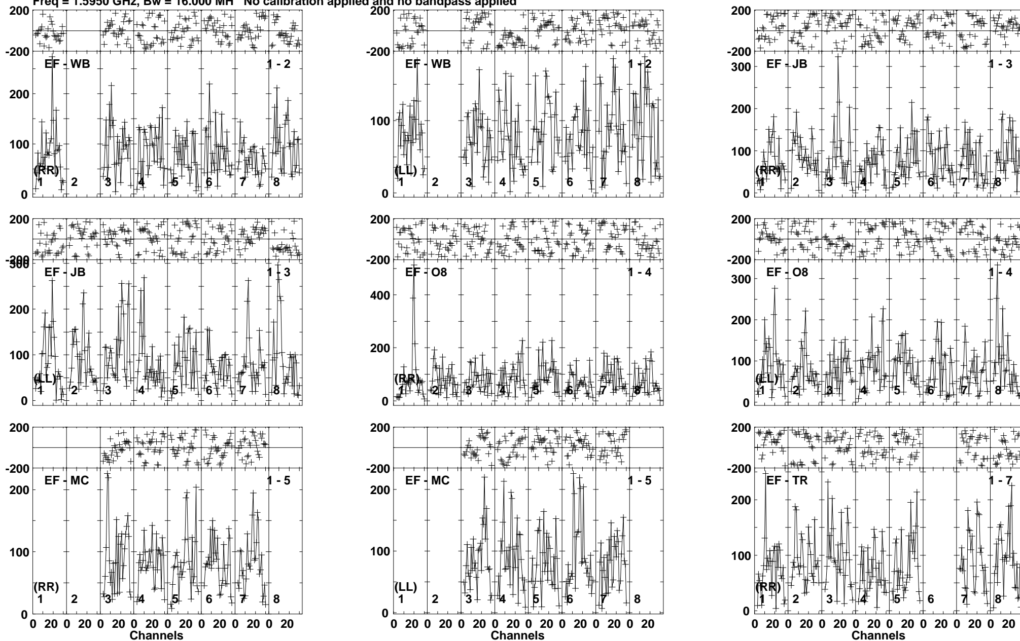
Lower frame: Micro Ampl Jy Top frame: Phas deg Vector averaged cross-power spectrum Baseline: EF (01) - WB (02) Timerange: 00/10:57:05 to 00/11:00:29
