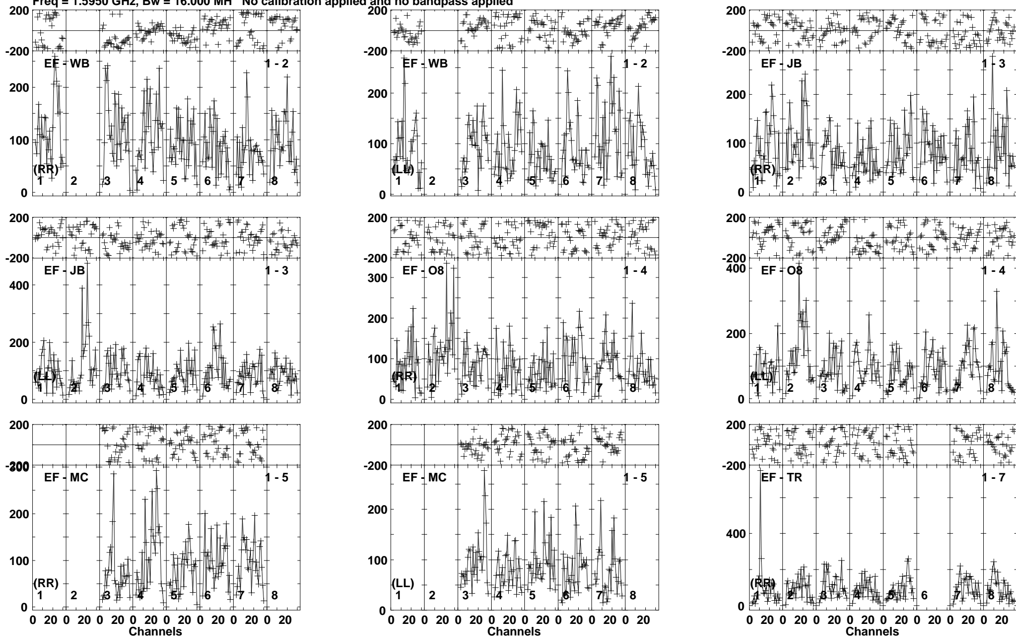
Lower frame: Micro Ampl Jy Top frame: Phas deg Vector averaged cross-power spectrum Baseline: EF (01) - WB (02) Timerange: 00/15:28:09 to 00/15:31:29
