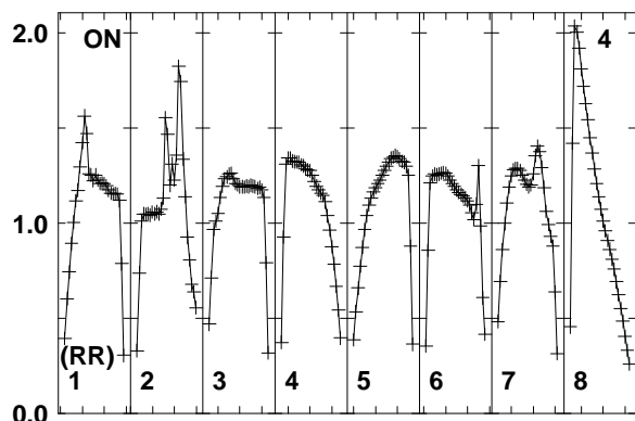
Lower frame: Real Jy Total-power spectrum Antenna: EF (01) Timerange: 00/17:35:01 to 00/17:38:29
