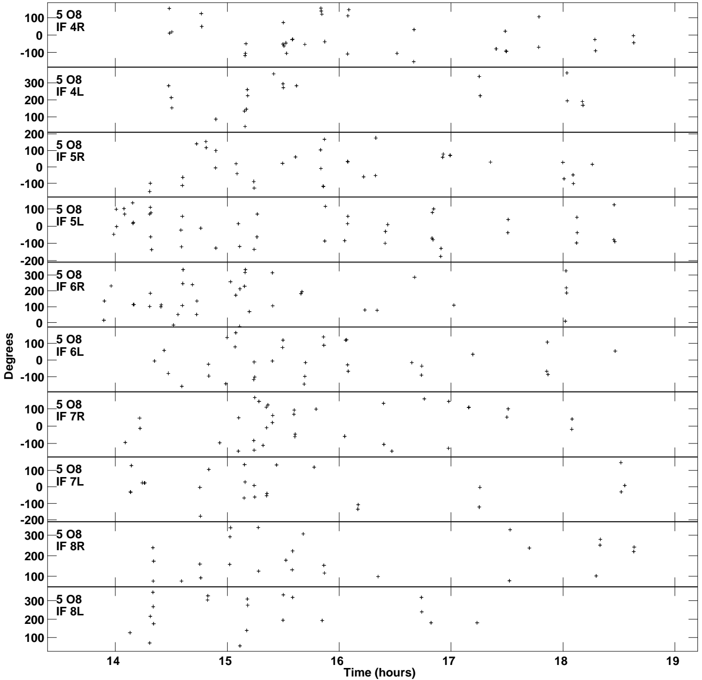
Plot file version 8 created 16-OCT-2015 11:38:20 Gain phs vs UTC time for ASASSN-14LI.MULTI.1 SN 1 Rpol & Lpol IF 1 - 8
