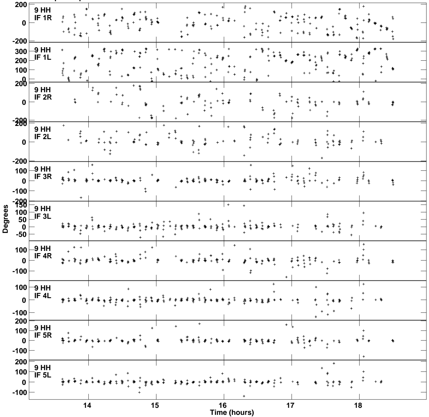
Plot file version 12 created 15-OCT-2015 11:48:16 Gain phs vs UTC time for J1250+1621.MULTI.1 SN 1 Rpol & Lpol IF 1 - 8
