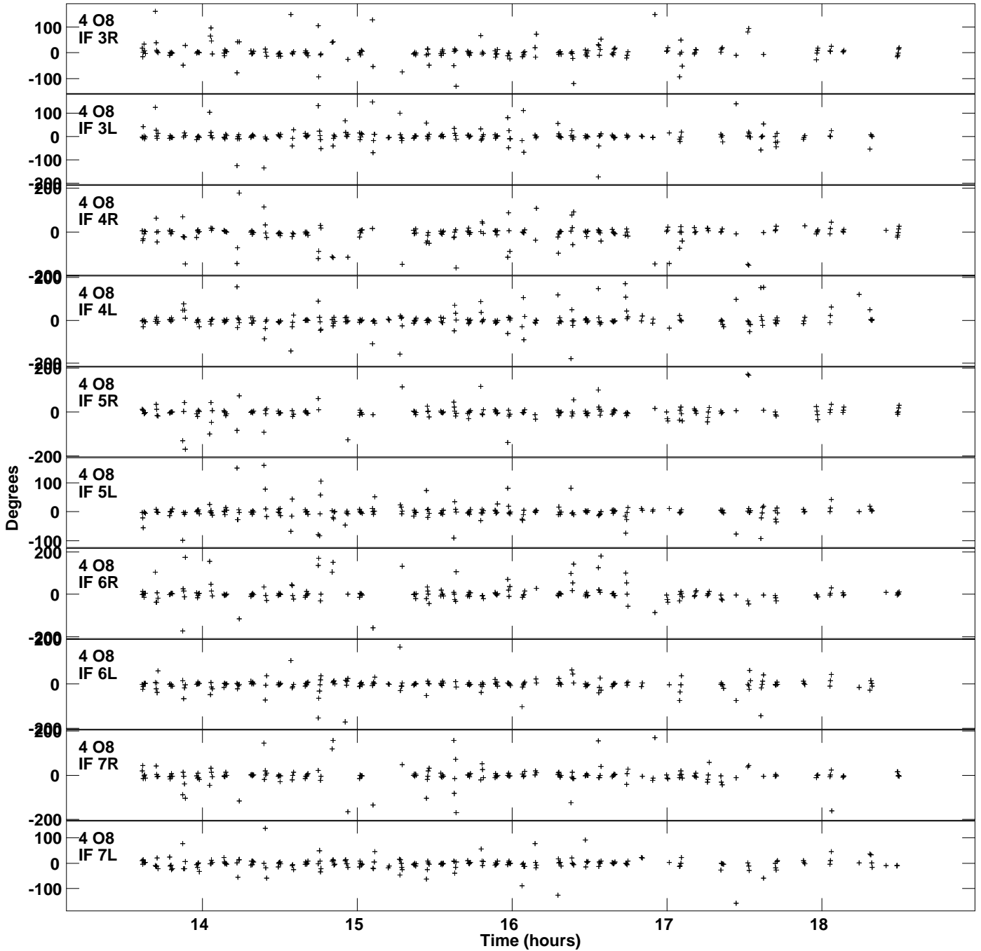
Plot file version 6 created 15-OCT-2015 11:48:16 Gain phs vs UTC time for J1250+1621.MULTI.1 SN 1 Rpol & Lpol IF 1 - 8
