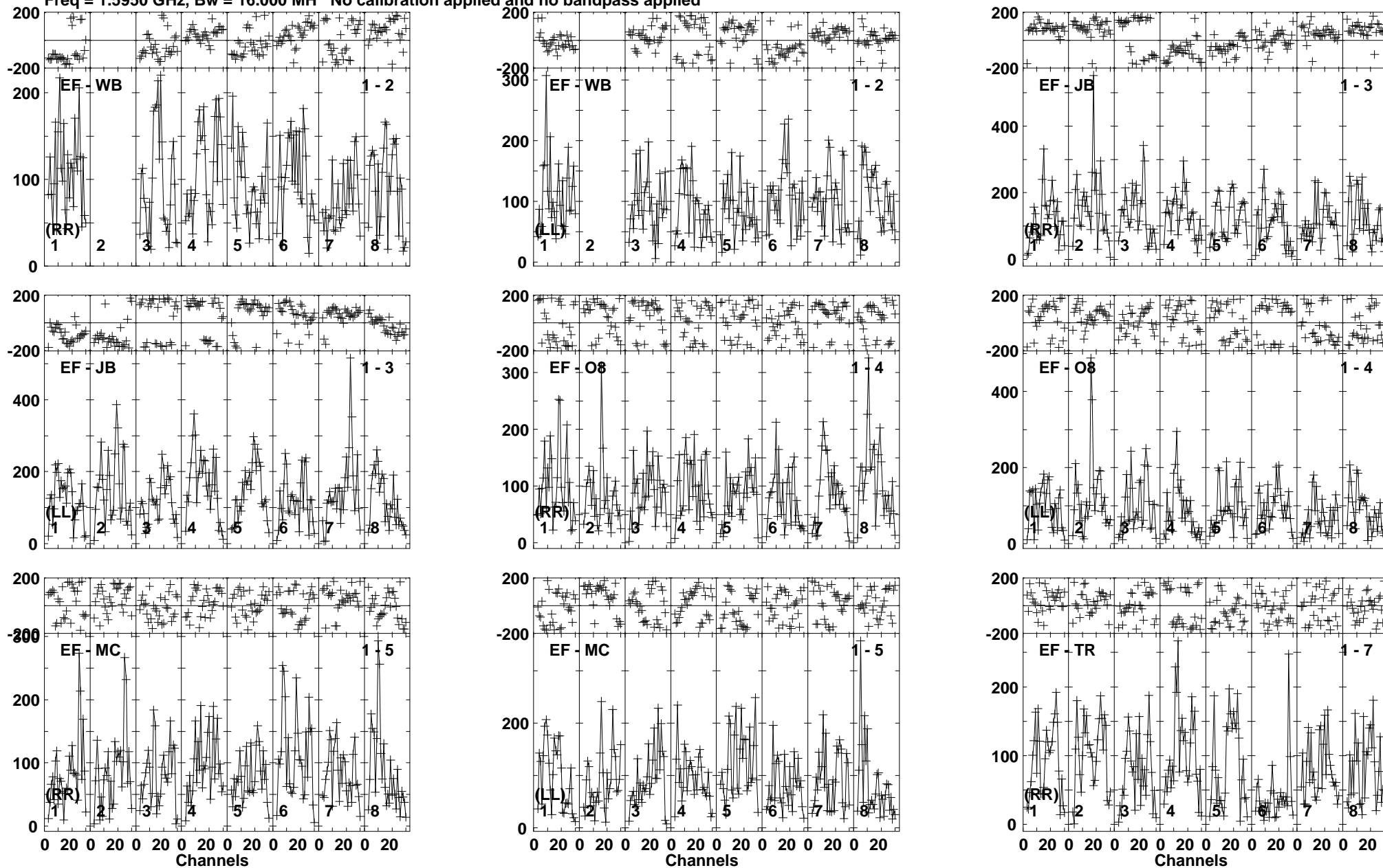
Lower frame: Micro Ampl Jy Top frame: Phas deg Vector averaged cross-power spectrum Baseline: EF (01) - WB (02) Timerange: 00/16:50:36 to 00/16:53:58
