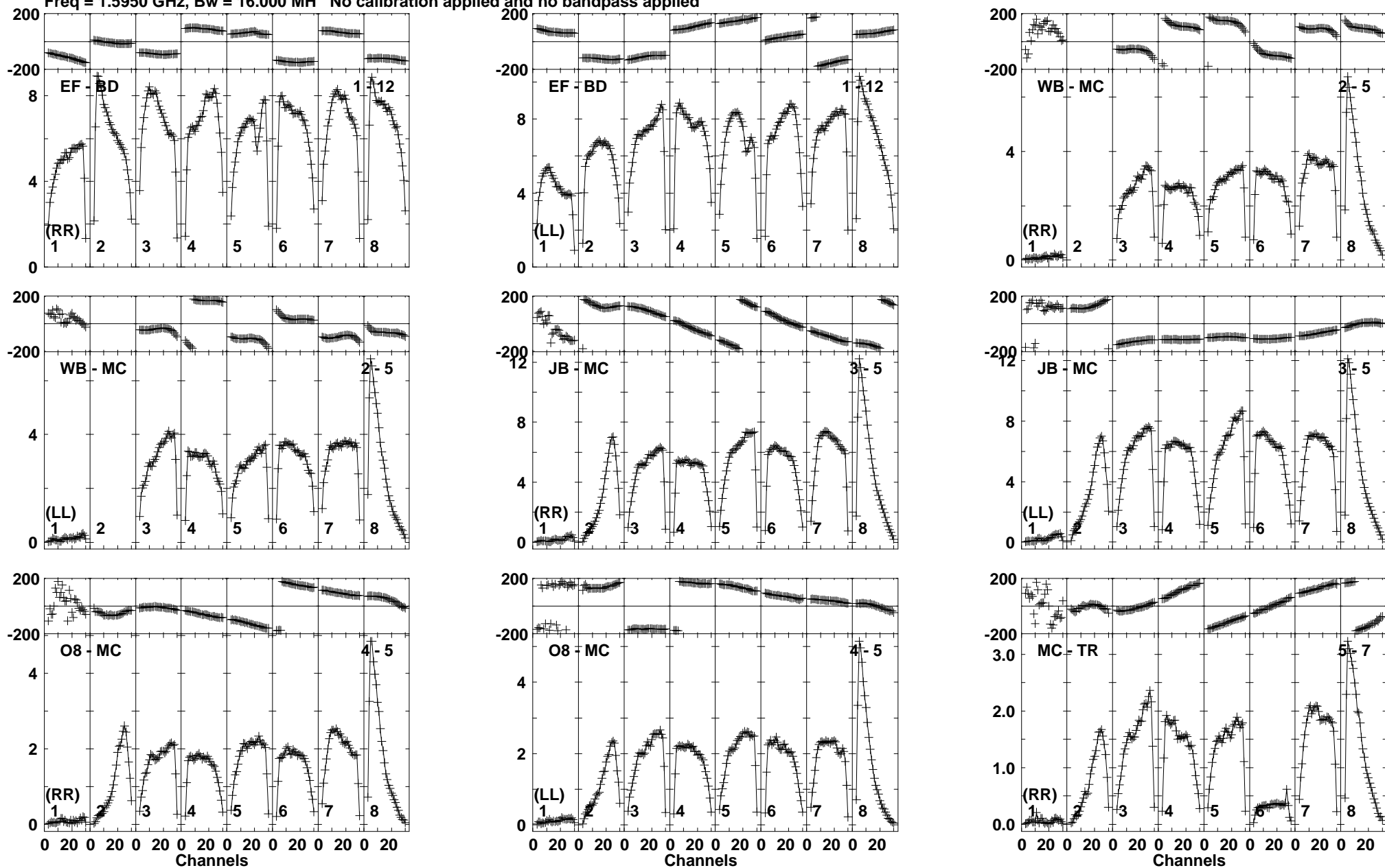
Lower frame: Milli Ampl Jy Top frame: Phas deg Vector averaged cross-power spectrum Baseline: EF (01) - BD (12) Timerange: 00/16:11:33 to 00/16:15:59
