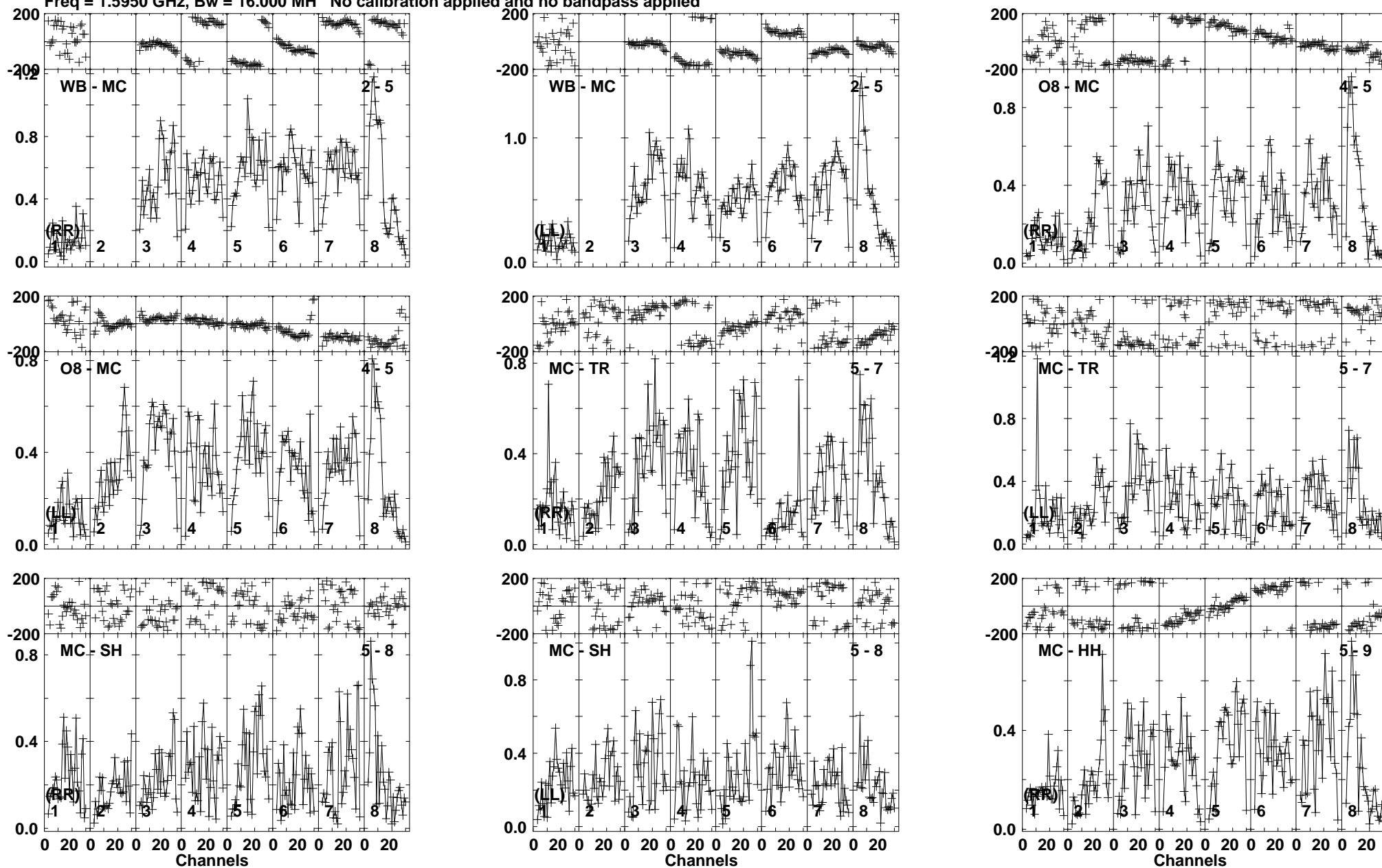
Lower frame: Milli Ampl Jy Top frame: Phas deg Vector averaged cross-power spectrum Baseline: WB (02) - MC (05) Timerange: 00/14:55:07 to 00/14:56:29
