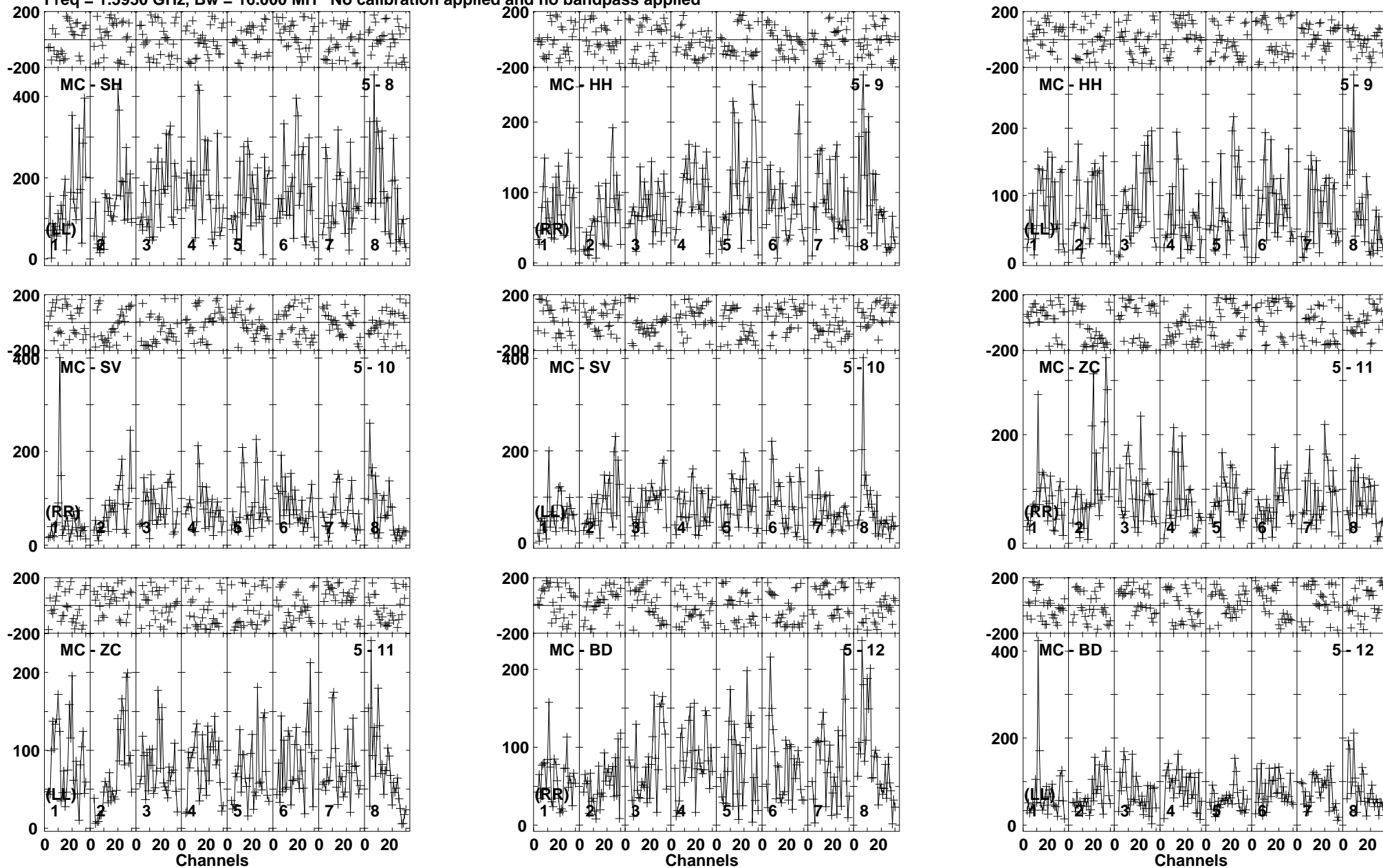
Lower frame: Micro Ampl Jy Top frame: Phas deg Vector averaged cross-power spectrum Baseline: MC (05) - SH (08) Timerange: 00/14:30:37 to 00/14:33:59
