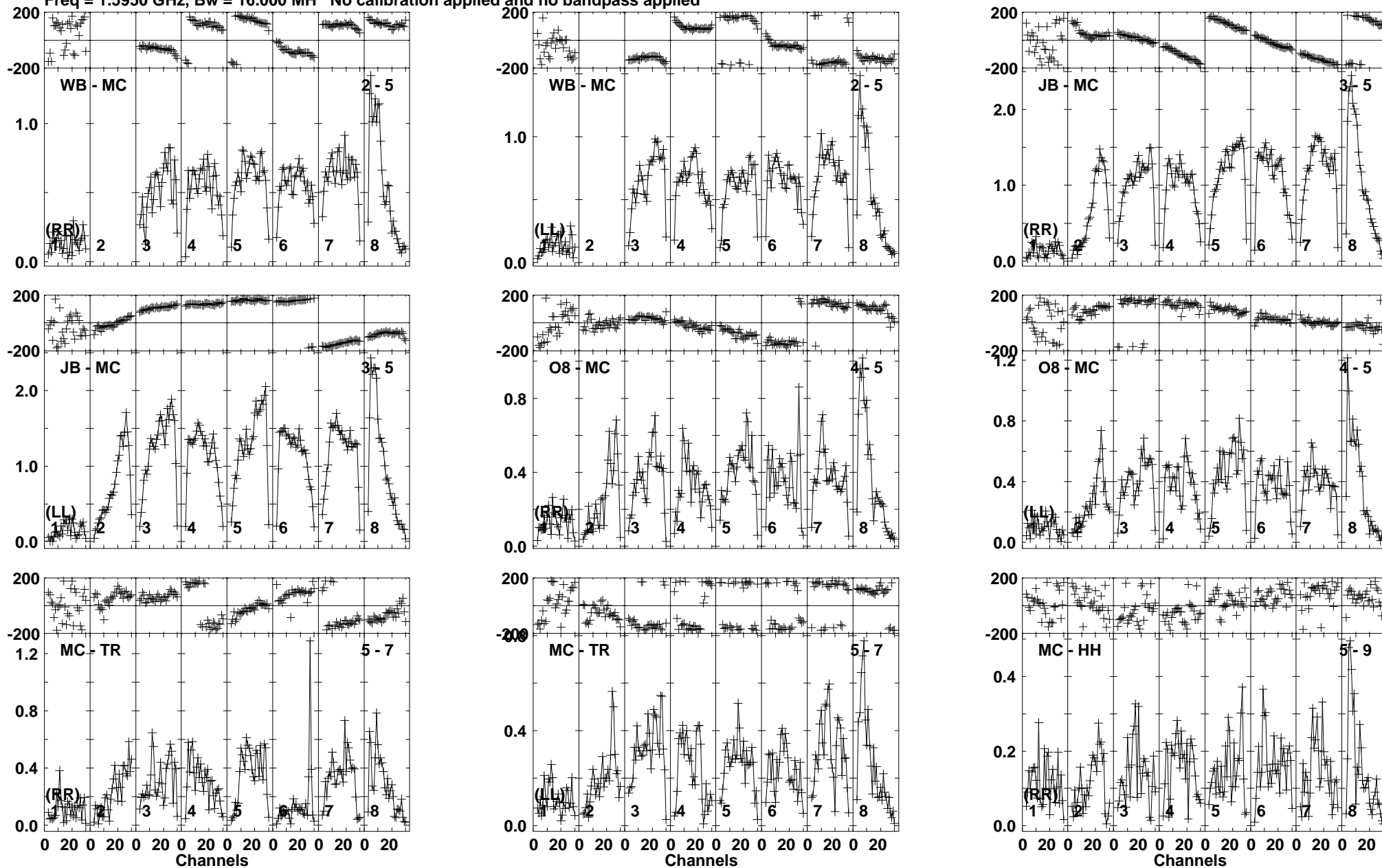
Lower frame: Milli Ampl Jy Top frame: Phas deg Vector averaged cross-power spectrum Baseline: WB (02) - MC (05) Timerange: 00/18:13:13 to 00/18:14:29
