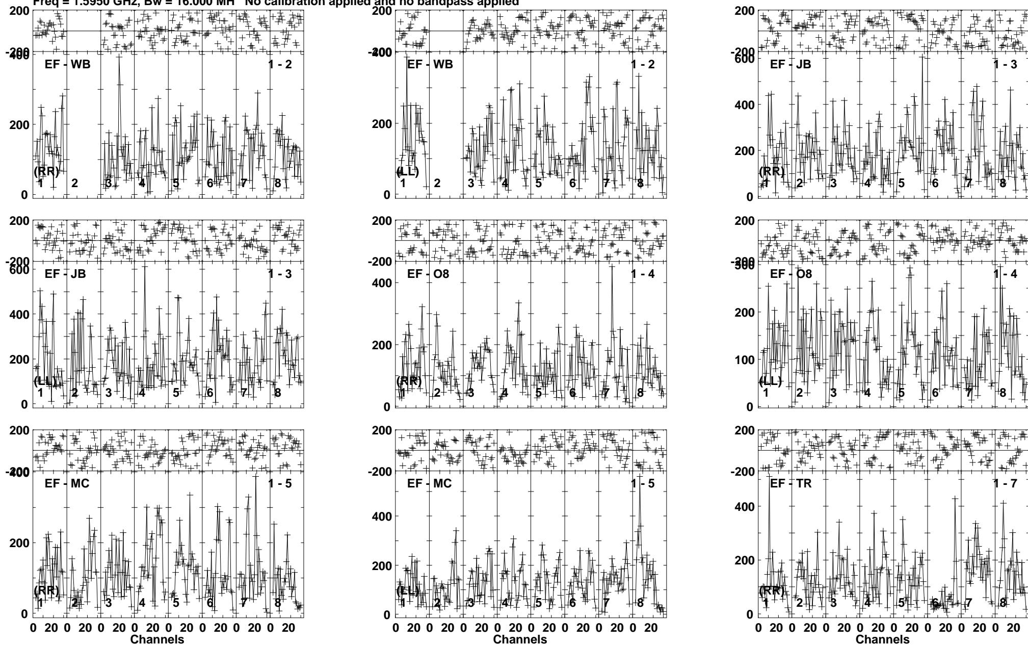
Lower frame: Micro Ampl Jy Top frame: Phas deg Vector averaged cross-power spectrum Baseline: EF (01) - WB (02) Timerange: 00/16:17:33 to 00/16:18:59
