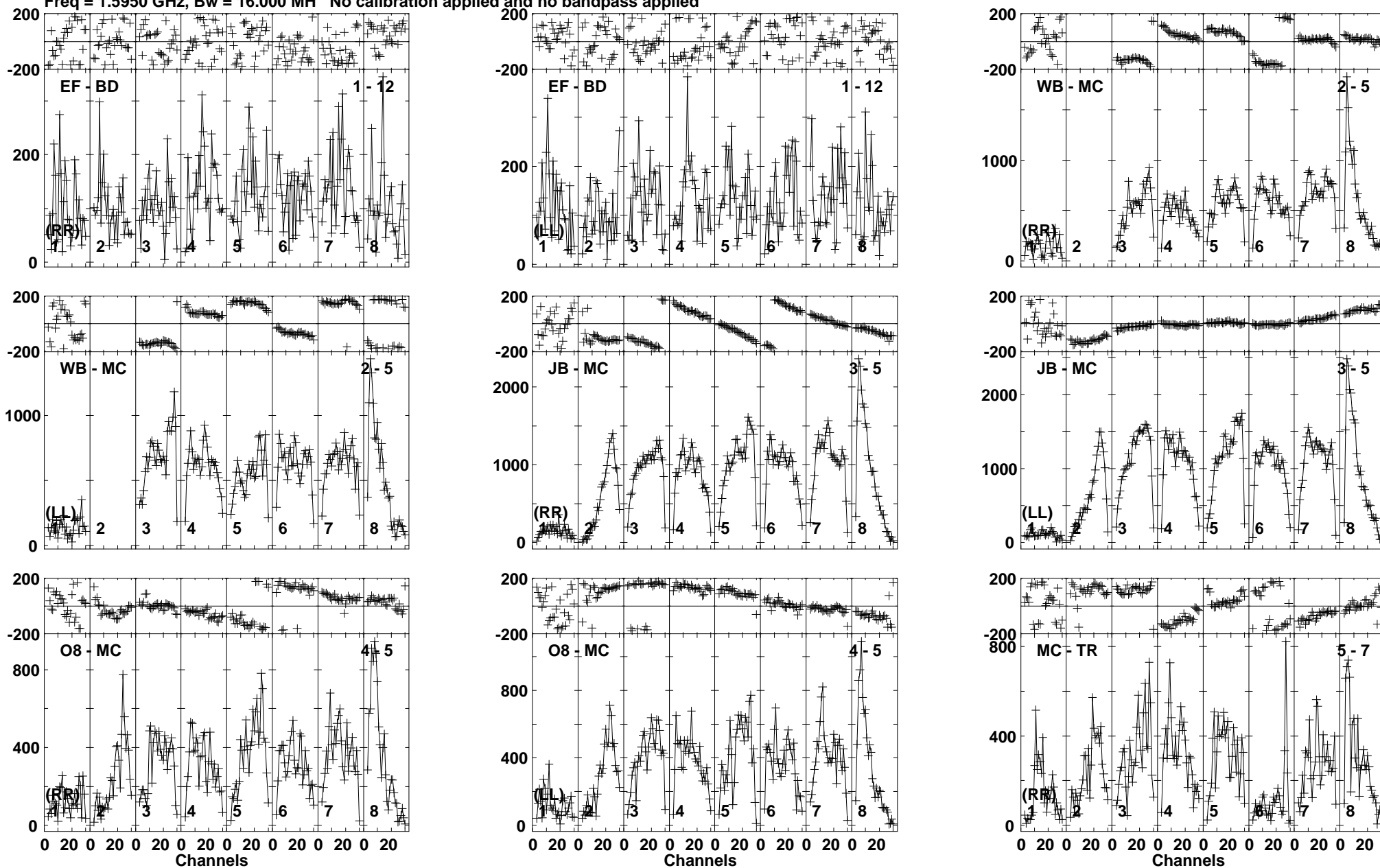
Lower frame: Micro Ampl Jy Top frame: Phas deg Vector averaged cross-power spectrum Baseline: EF (01) - BD (12) Timerange: 00/16:28:13 to 00/16:29:29
