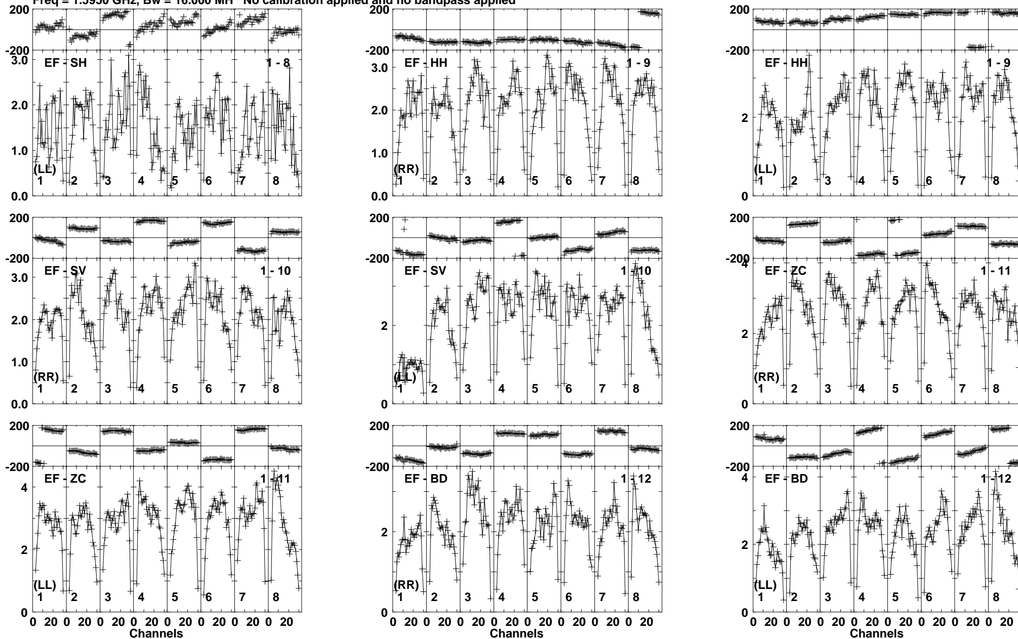
Lower frame: Milli Ampl Jy Top frame: Phas deg Vector averaged cross-power spectrum Baseline: EF (01) - SH (08) Timerange: 00/15:58:07 to 00/15:59:29
