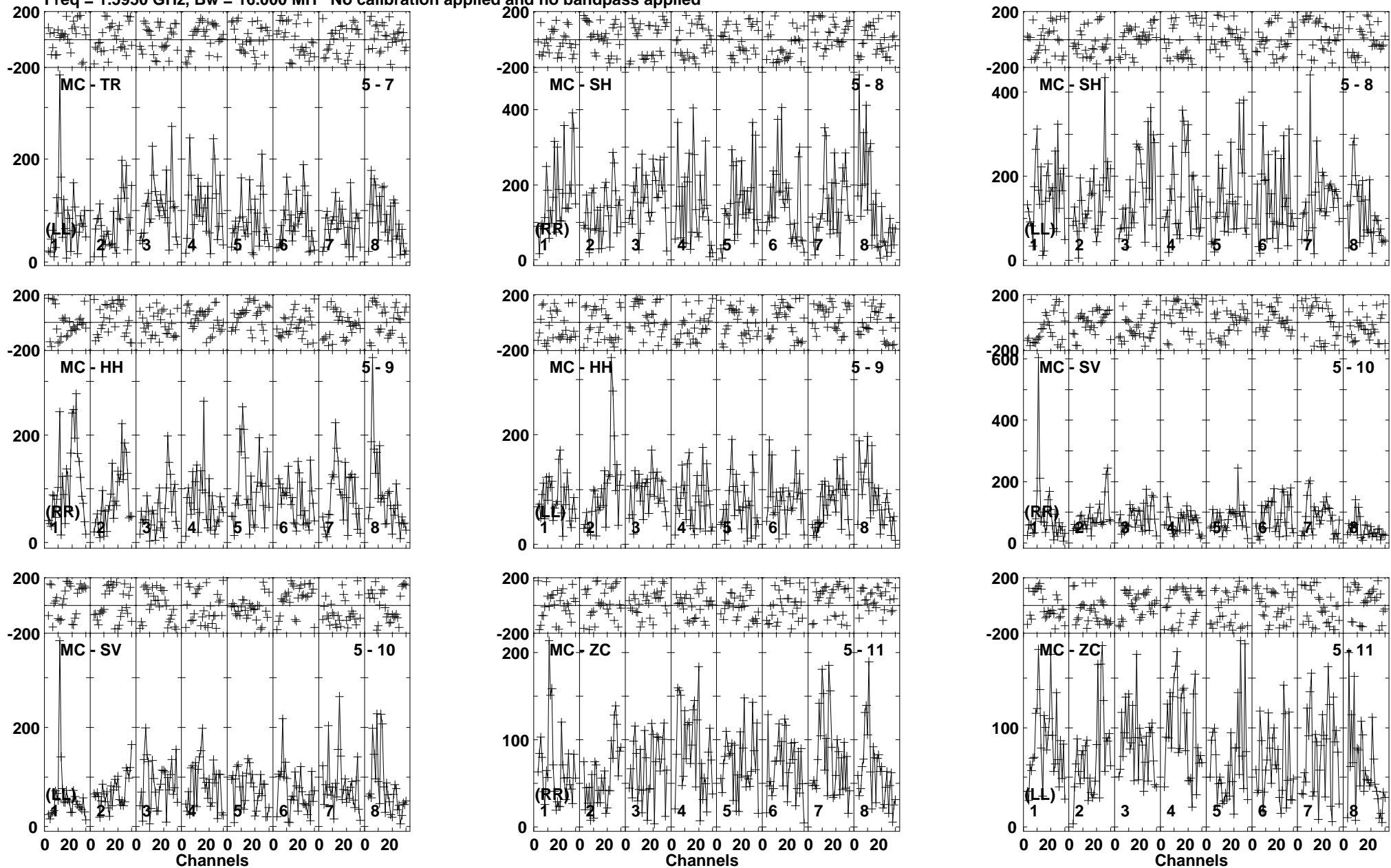
Lower frame: Micro Ampl Jy Top frame: Phas deg Vector averaged cross-power spectrum Baseline: MC (05) - TR (07) Timerange: 00/16:19:07 to 00/16:22:29
