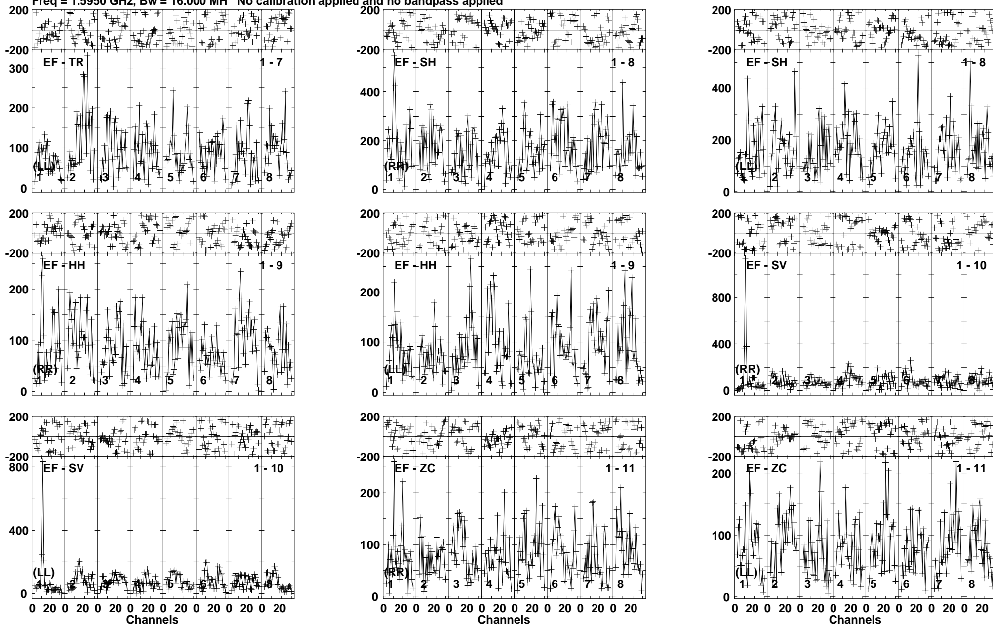
Lower frame: Micro Ampl Jy Top frame: Phas deg Vector averaged cross-power spectrum Baseline: EF (01) - TR (07) Timerange: 00/16:55:34 to 00/16:58:58
