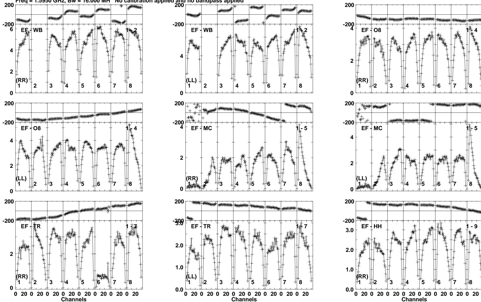
Lower frame: Milli Ampl Jy Top frame: Phas deg Vector averaged cross-power spectrum Baseline: EF (01) - WB (02) Timerange: 00:17:46:39 to 00:17:47:59
