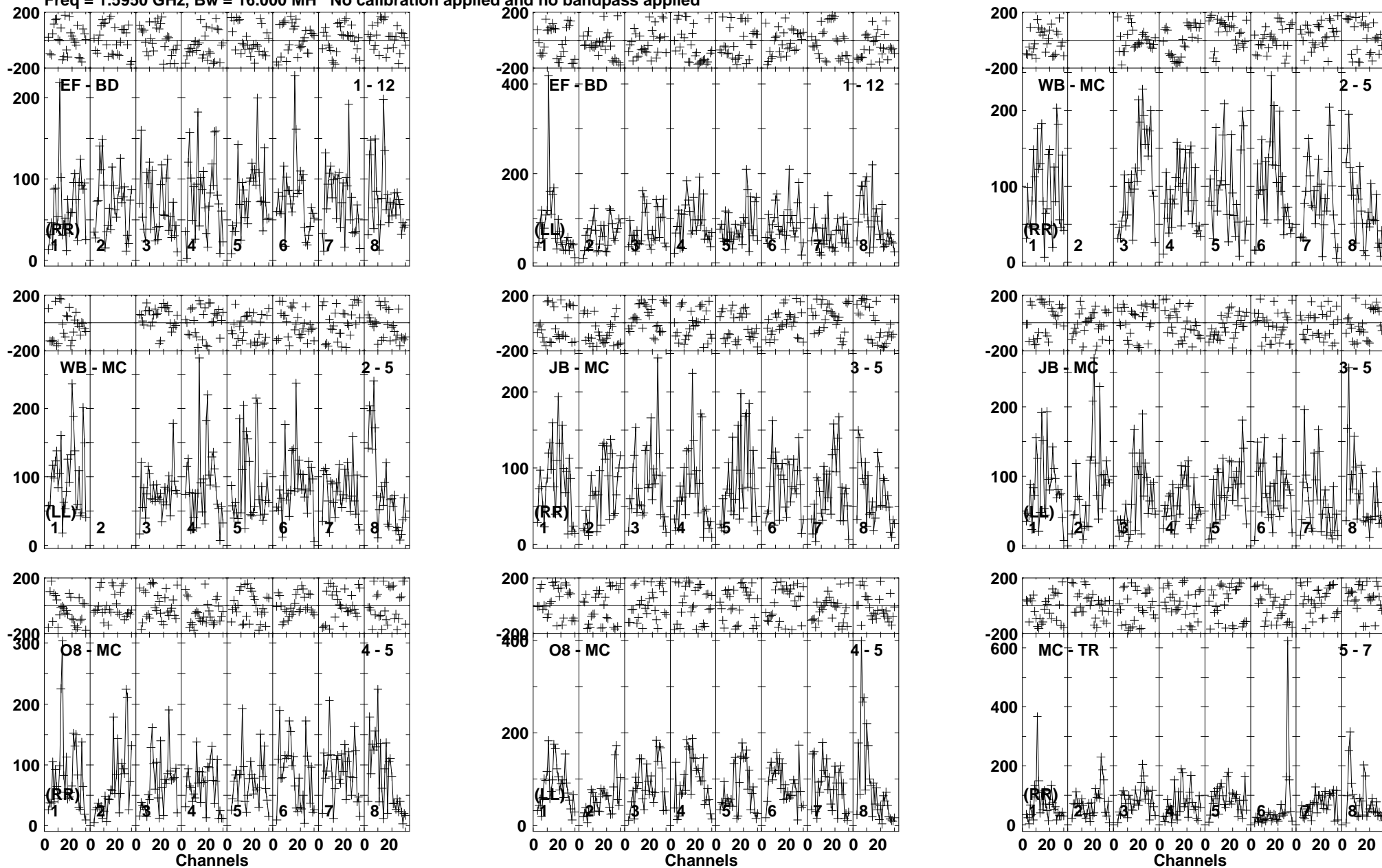
Lower frame: Micro Ampl Jy Top frame: Phas deg Vector averaged cross-power spectrum Baseline: EF (01) - BD (12) Timerange: 00/16:34:34 to 00/16:37:58
