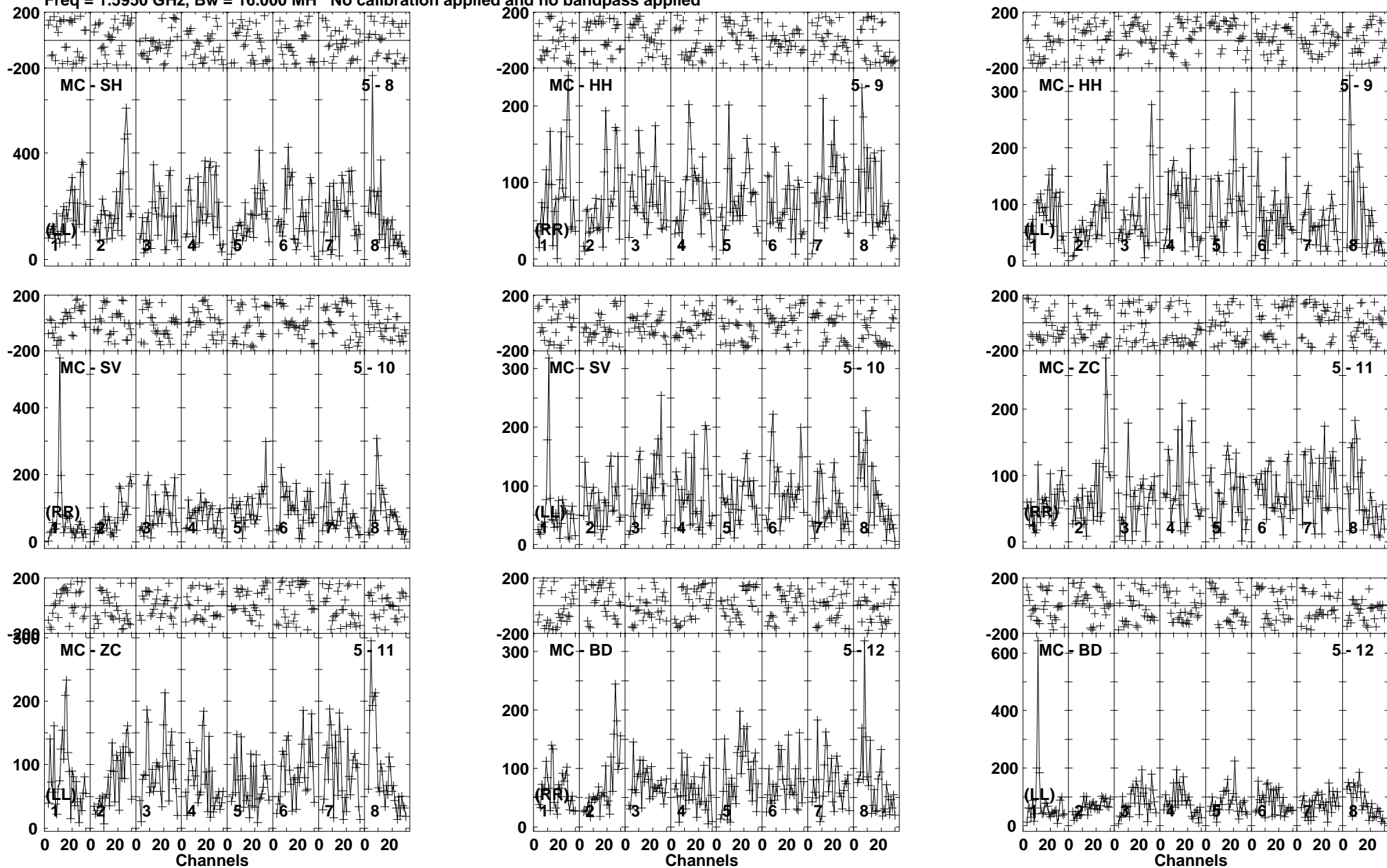
Lower frame: Micro Ampl Jy Top frame: Phas deg Vector averaged cross-power spectrum Baseline: MC (05) - SH (08) Timerange: 00/14:56:34 to 00/14:59:58
