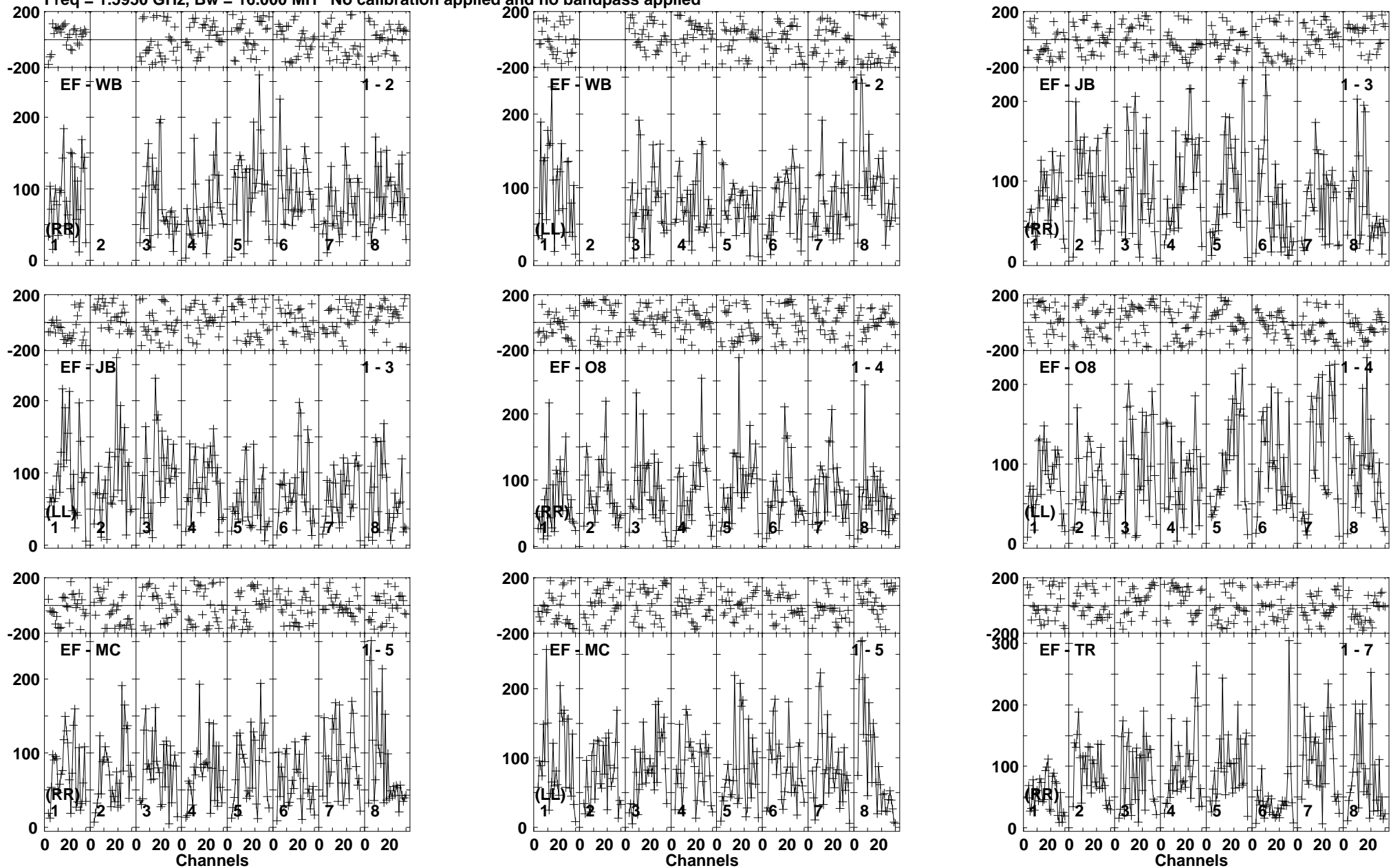
Lower frame: Micro Ampl Jy Top frame: Phas deg Vector averaged cross-power spectrum Baseline: EF (01) - WB (02) Timerange: 00/16:24:04 to 00/16:27:28
