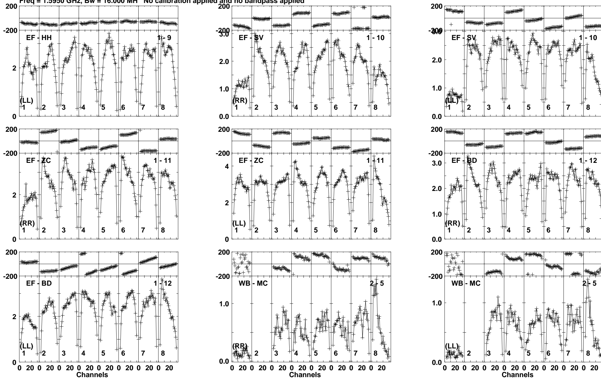
Lower frame: Milli Amply Jy Top frame: Phas deg Vector averaged cross-power spectrum Baseline: EF (01) - HH (09) Timerange: 00:18:07:39 to 00:18:08:59
