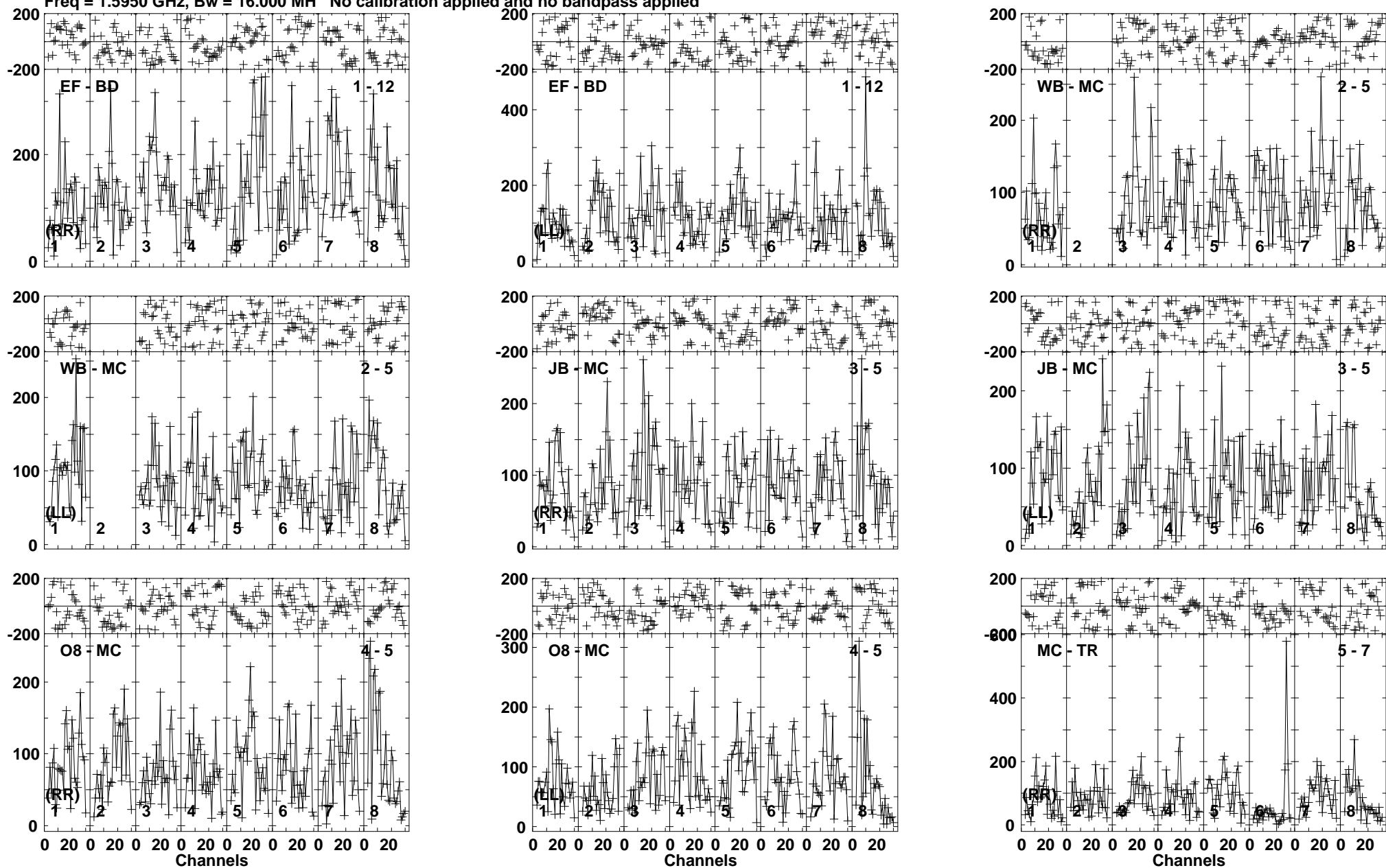
Lower frame: Micro Ampl Jy Top frame: Phas deg Vector averaged cross-power spectrum Baseline: EF (01) - BD (12) Timerange: 00/15:54:37 to 00/15:57:59
