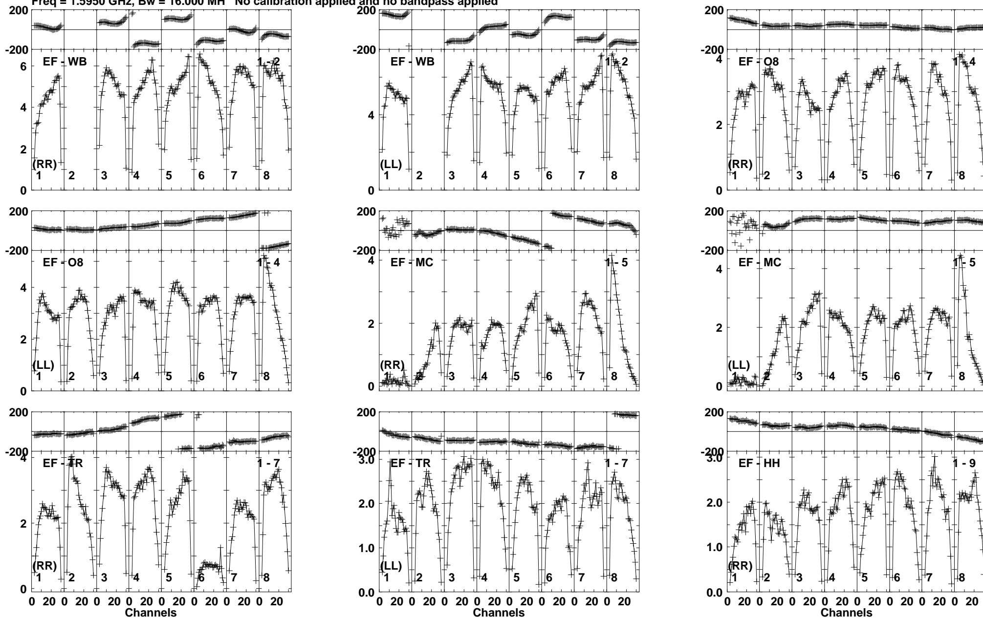
Lower frame: Milli Ampl Jy Top frame: Phas deg Vector averaged cross-power spectrum Baseline: EF (01) - WB (02) Timerange: 00/18:18:09 to 00/18:19:29
