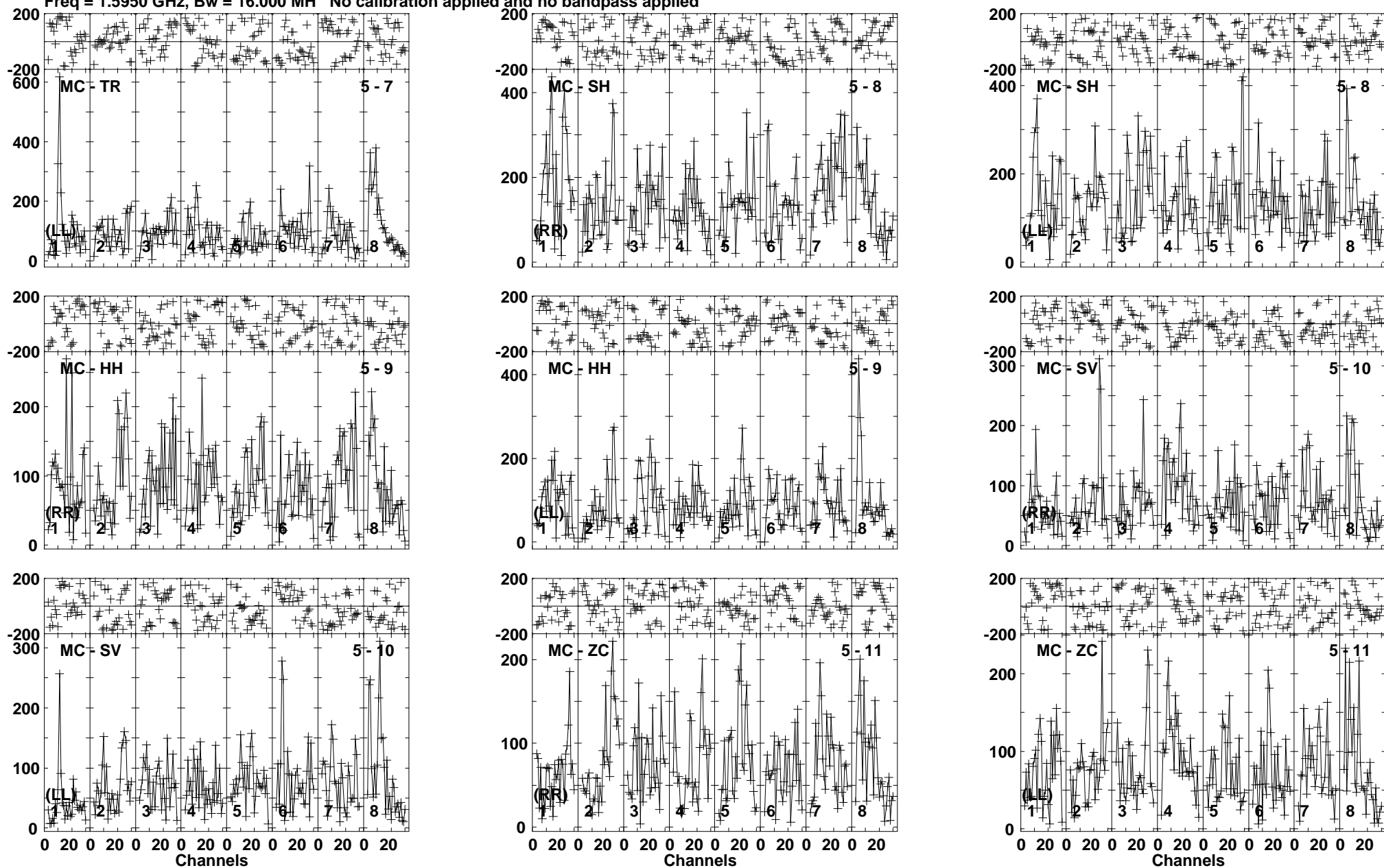
Lower frame: Micro Ampl Jy Top frame: Phas deg Vector averaged cross-power spectrum Baseline: MC (05) - TR (07) Timerange: 00:16:50:36 to 00:16:53:58
