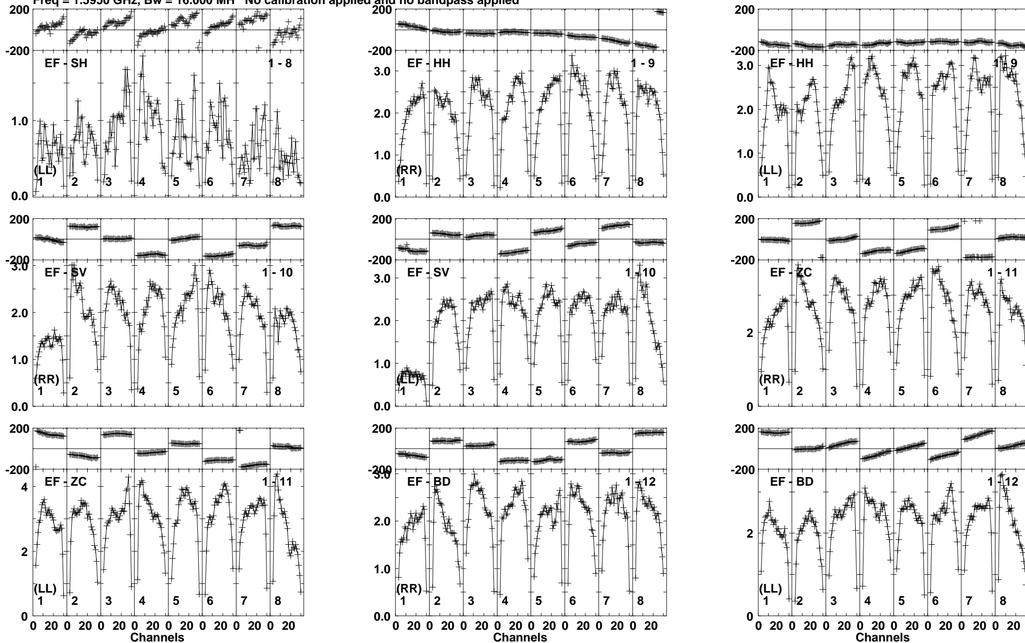
Lower frame: Milli Ampl Jy Top frame: Phas deg Vector averaged cross-power spectrum Baseline: EF (01) - SH (08) Timerange: 00/17:25:36 to 00/17:26:58
