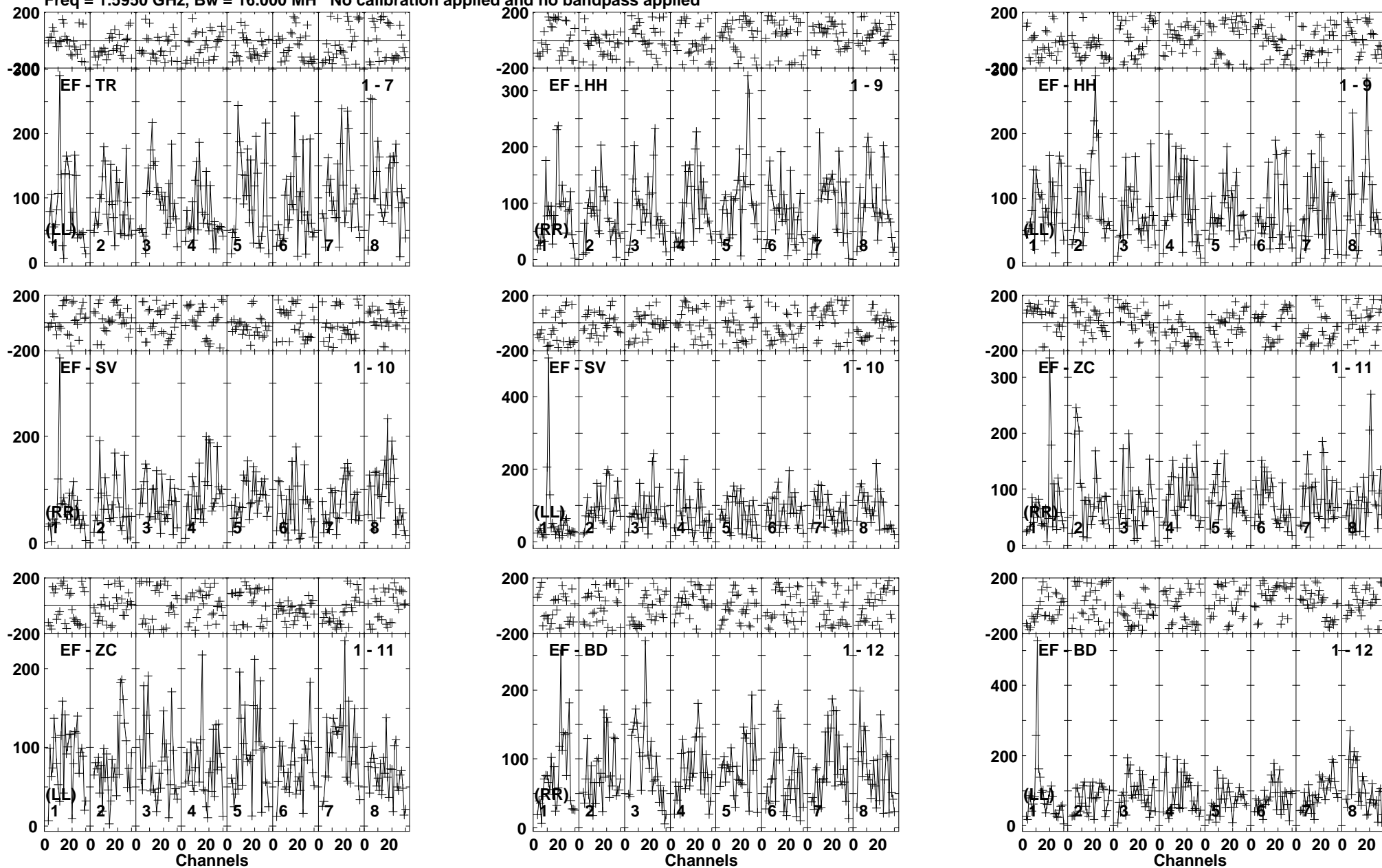
Lower frame: Micro Ampl Jy Top frame: Phas deg Vector averaged cross-power spectrum Baseline: EF (01) - TR (07) Timerange: 00:18:14:39 to 00:18:17:59
