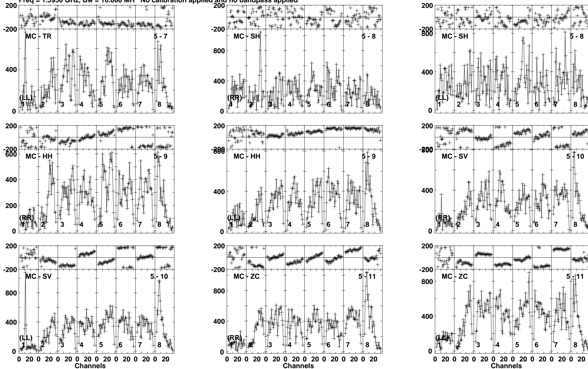
Lower frame: Micro Ampl Jy Top frame: Phas deg Vector averaged cross-power spectrum Baseline: MC (05) - TR (07) Timerange: 00/16:17:33 to 00/16:18:59
