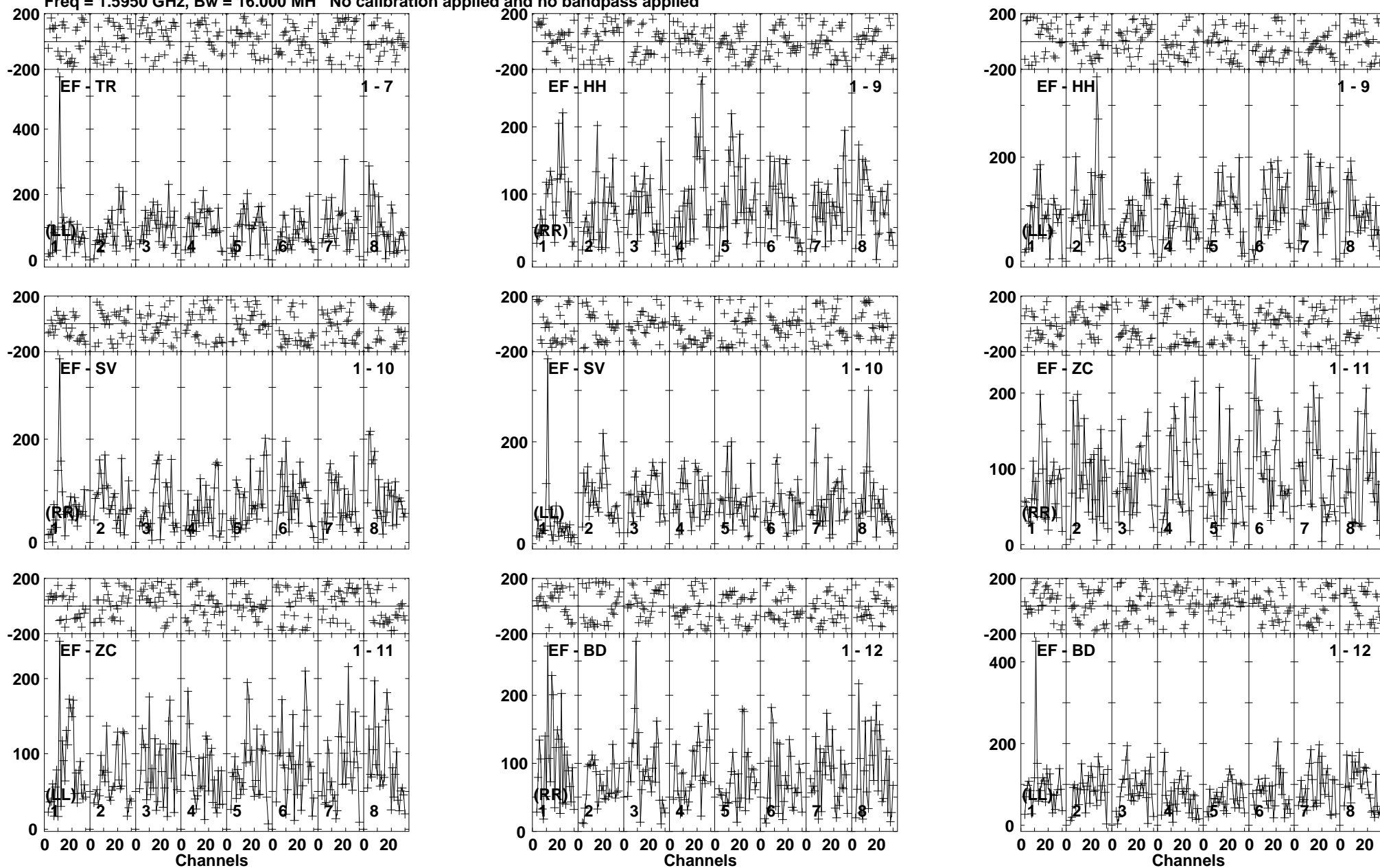
Lower frame: Micro Ampl Jy Top frame: Phas deg Vector averaged cross-power spectrum Baseline: EF (01) - TR (07) Timerange: 00/17:43:09 to 00/17:46:29
