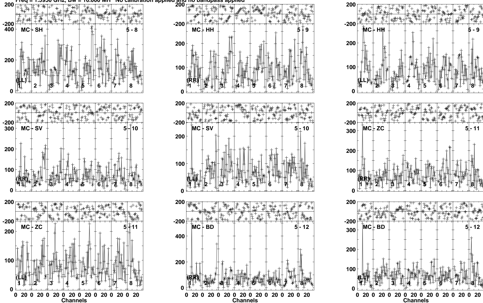
Lower frame: Micro Ampl Jy Top frame: Phas deg Vector averaged cross-power spectrum Baseline: MC (05) - SH (08) Timerange: 00/15:28:04 to 00/15:31:28
