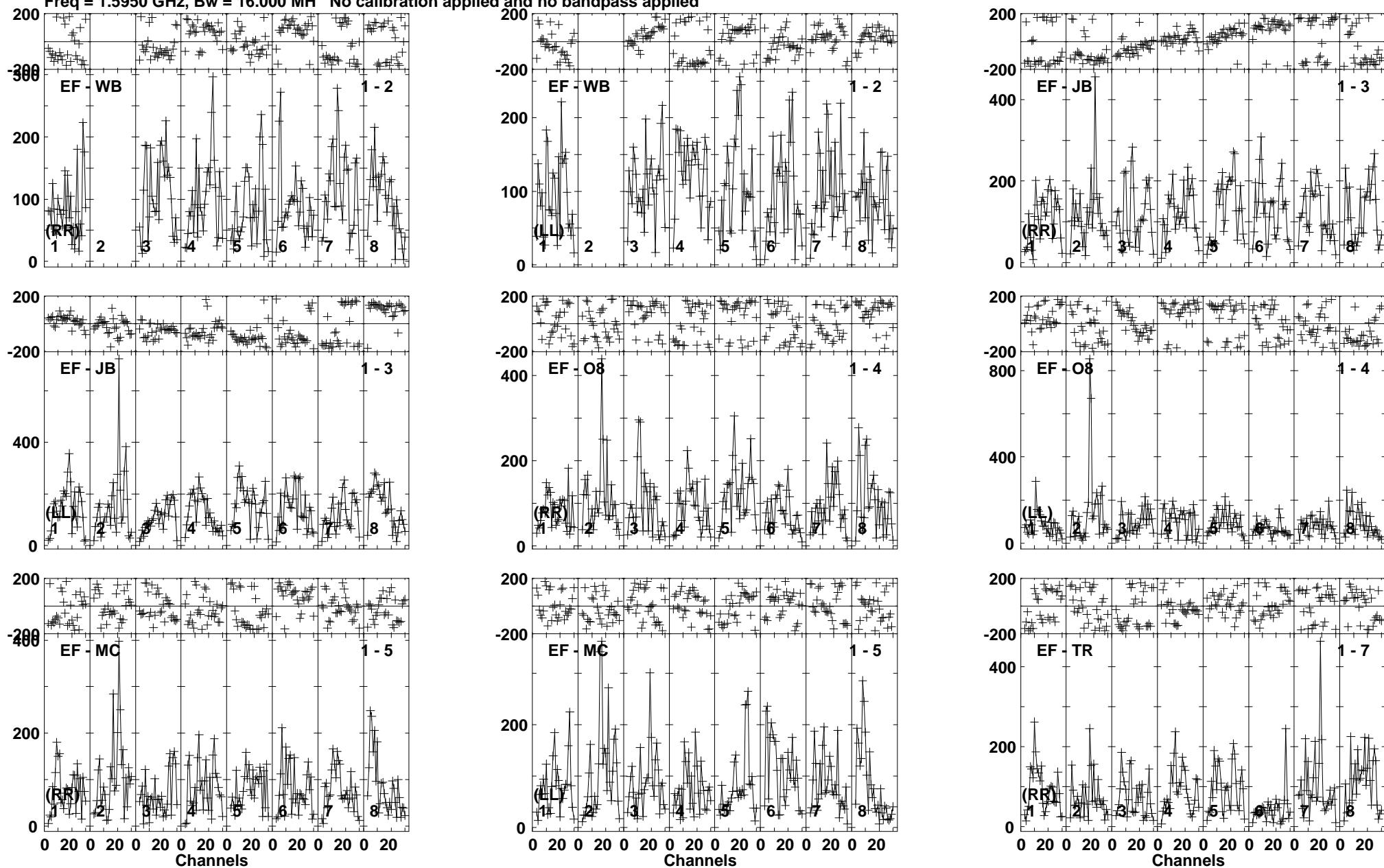
Lower frame: Micro Ampl Jy Top frame: Phas deg Vector averaged cross-power spectrum Baseline: EF (01) - WB (02) Timerange: 00/17:06:04 to 00/17:09:28
