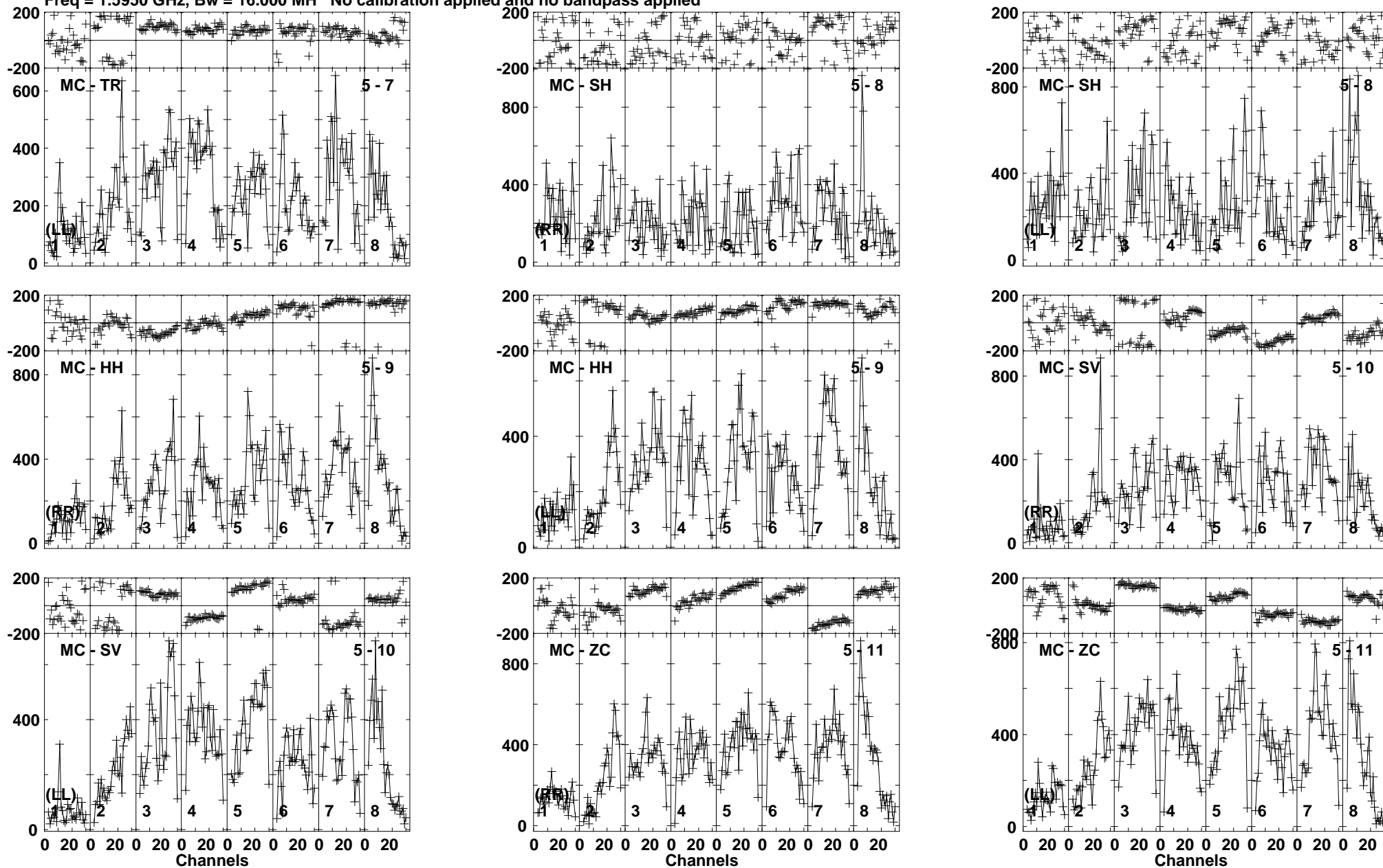
Lower frame: Micro Ampl Jy Top frame: Phas deg Vector averaged cross-power spectrum Baseline: MC (05) - TR (07) Timerange: 00/17:10:13 to 00/17:11:29
