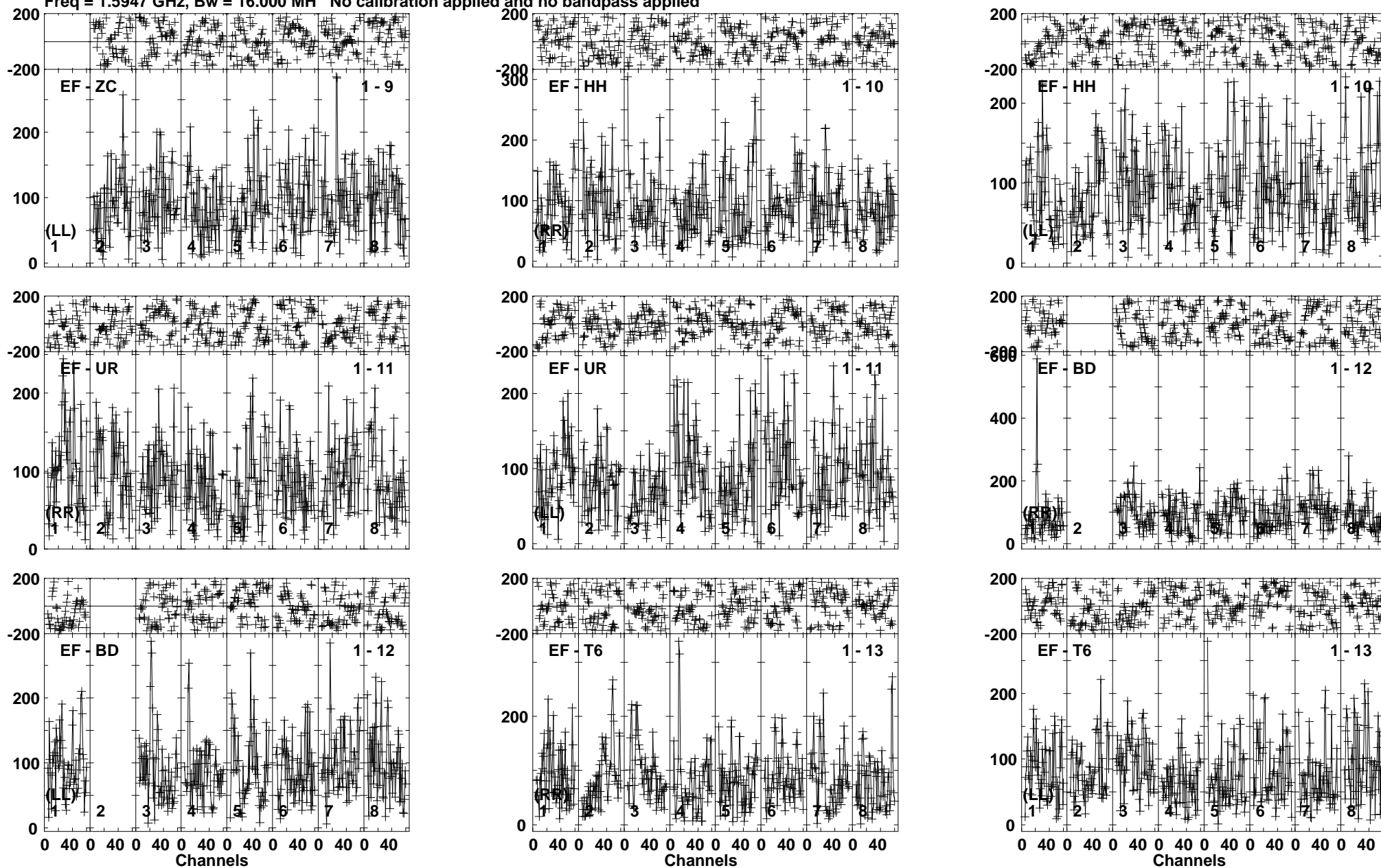
Lower frame: Micro Ampl Jy Top frame: Phas deg Vector averaged cross-power spectrum Baseline: EF (01) - ZC (09) Timerange: 00/17:55:12 to 00/17:58:39
