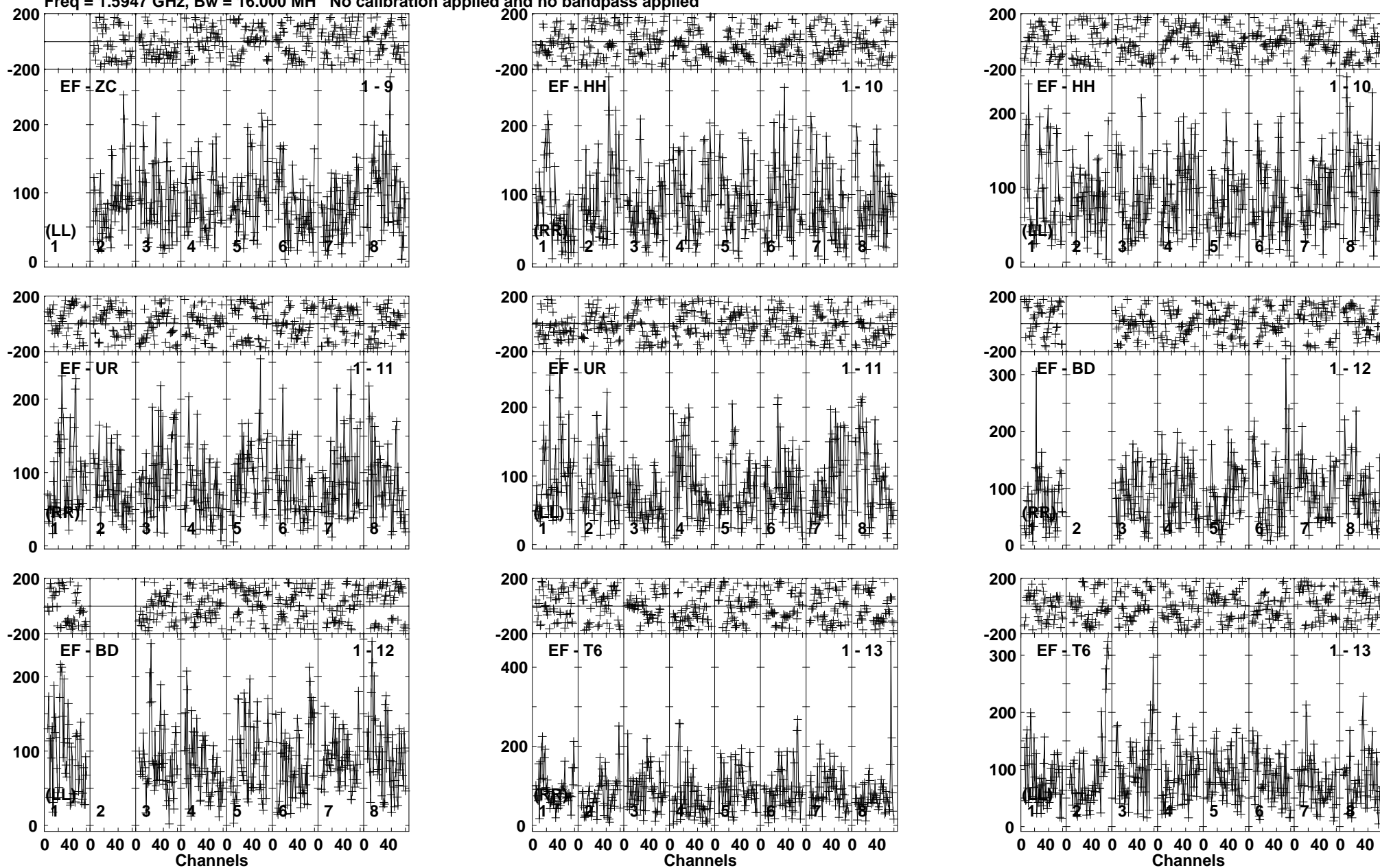
Lower frame: Micro Ampl Jy Top frame: Phas deg Vector averaged cross-power spectrum Baseline: EF (01) - ZC (09) Timerange: 00/18:35:02 to 00/18:38:29
