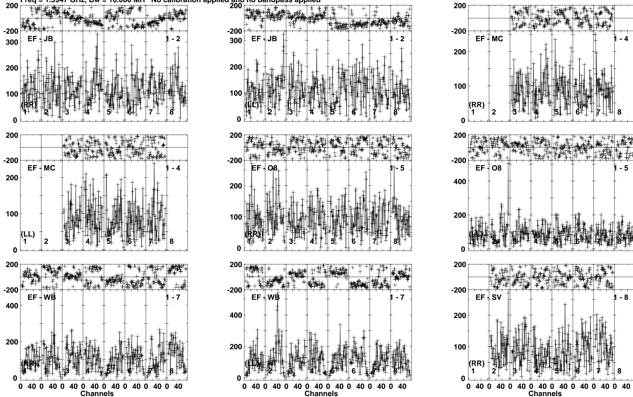
Lower frame: Micro Ampl Jy Top frame: Phas deg Vector averaged cross-power spectrum Baseline: EF (01) - JB (02) Timerange: 01/00:15:13 to 01/00:18:40
