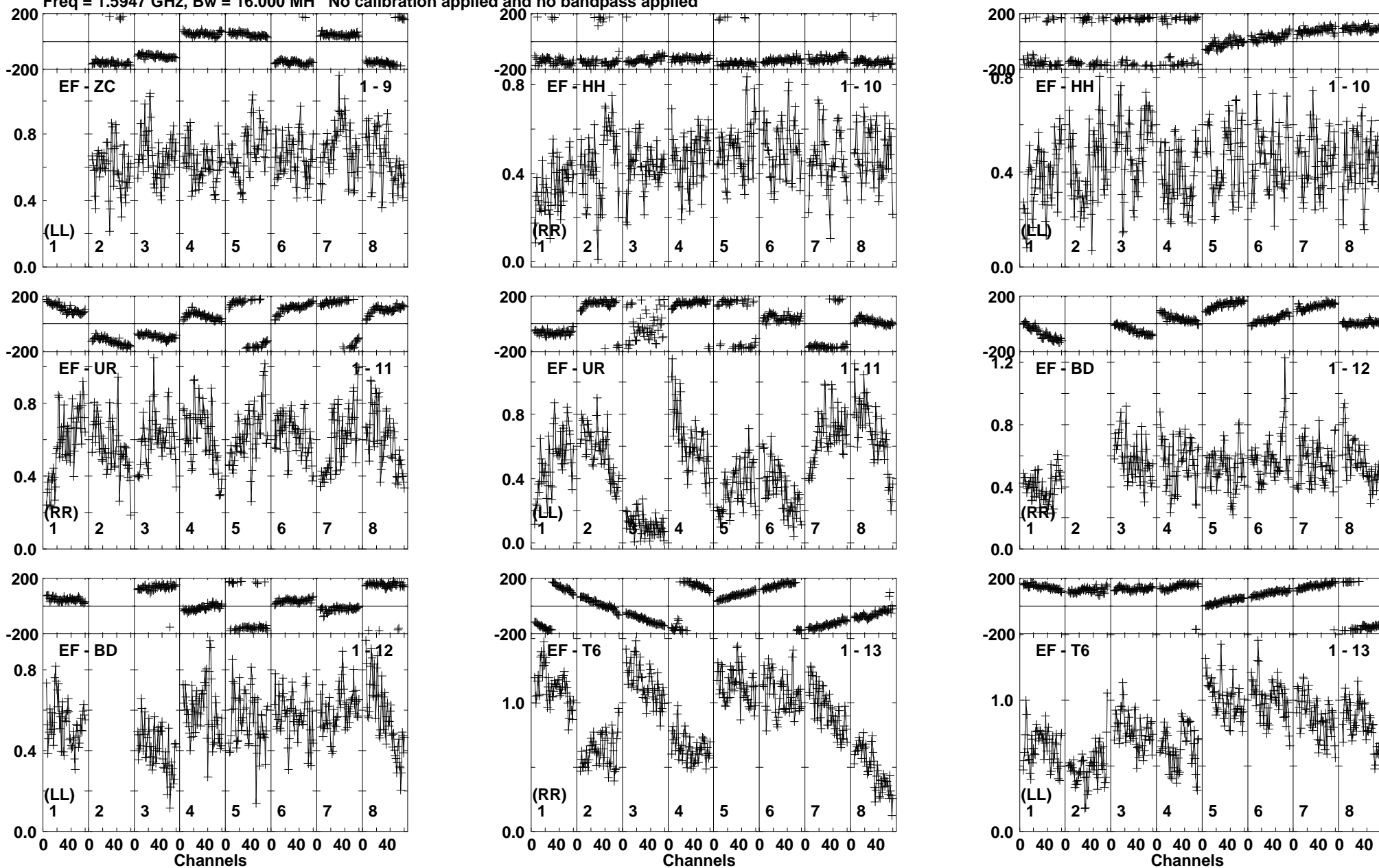
Lower frame: Milli Ampl Jy Top frame: Phas deg Vector averaged cross-power spectrum Baseline: EF (01) - ZC (09) Timerange: 00/17:54:11 to 00/17:55:09
