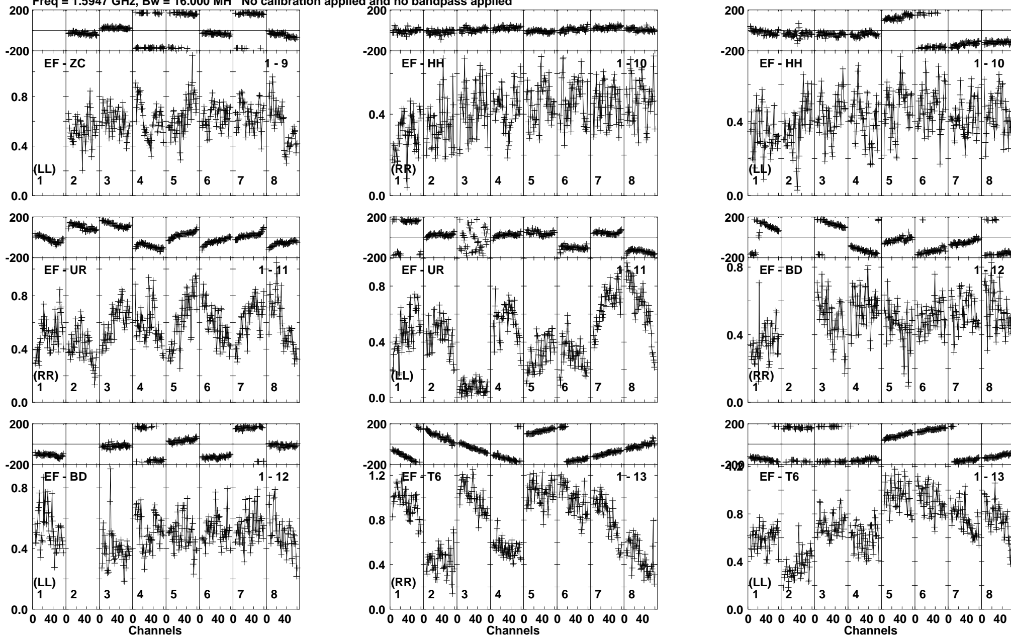
Lower frame: Milli Ampl Jy Top frame: Phas deg Vector averaged cross-power spectrum Baseline: EF (01) - ZC (09) Timerange: 00/17:43:31 to 00/17:44:59
