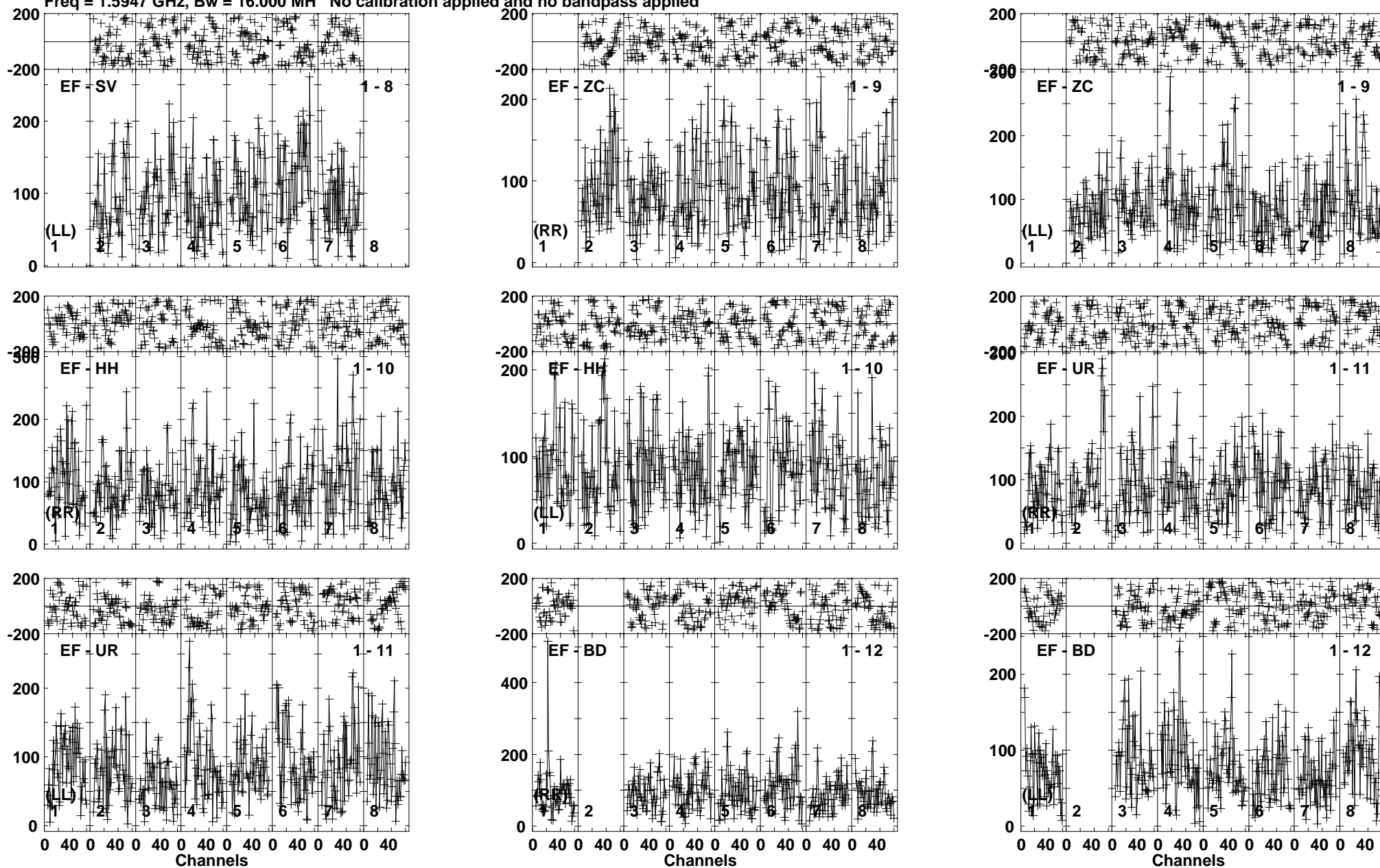
Lower frame: Micro Ampl Jy Top frame: Phas deg Vector averaged cross-power spectrum Baseline: EF (01) - SV (08) Timerange: 00/20:15:02 to 00/20:18:30
