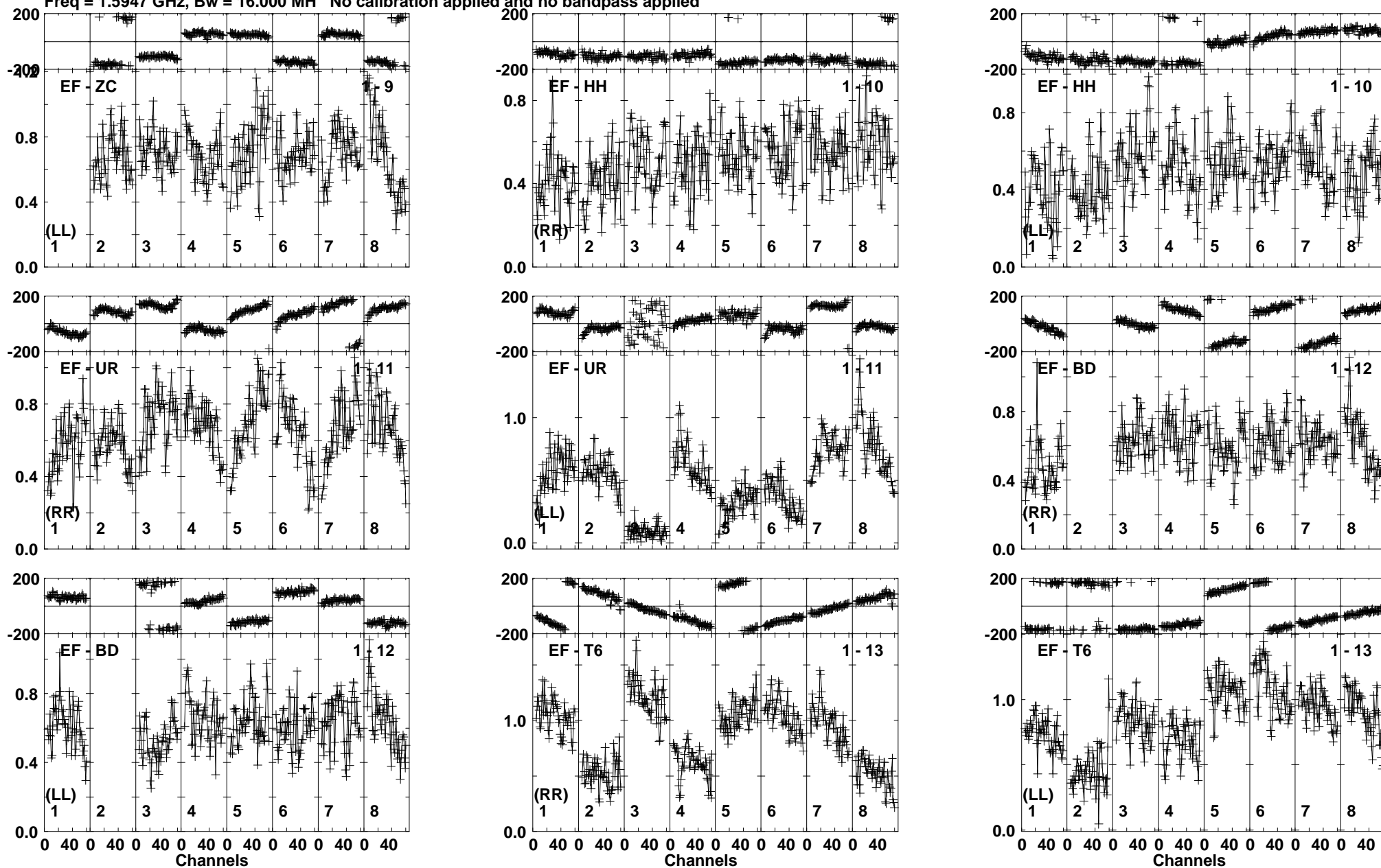
Lower frame: Milli Ampl Jy Top frame: Phas deg Vector averaged cross-power spectrum Baseline: EF (01) - ZC (09) Timerange: 00/18:44:10 to 00/18:45:09
