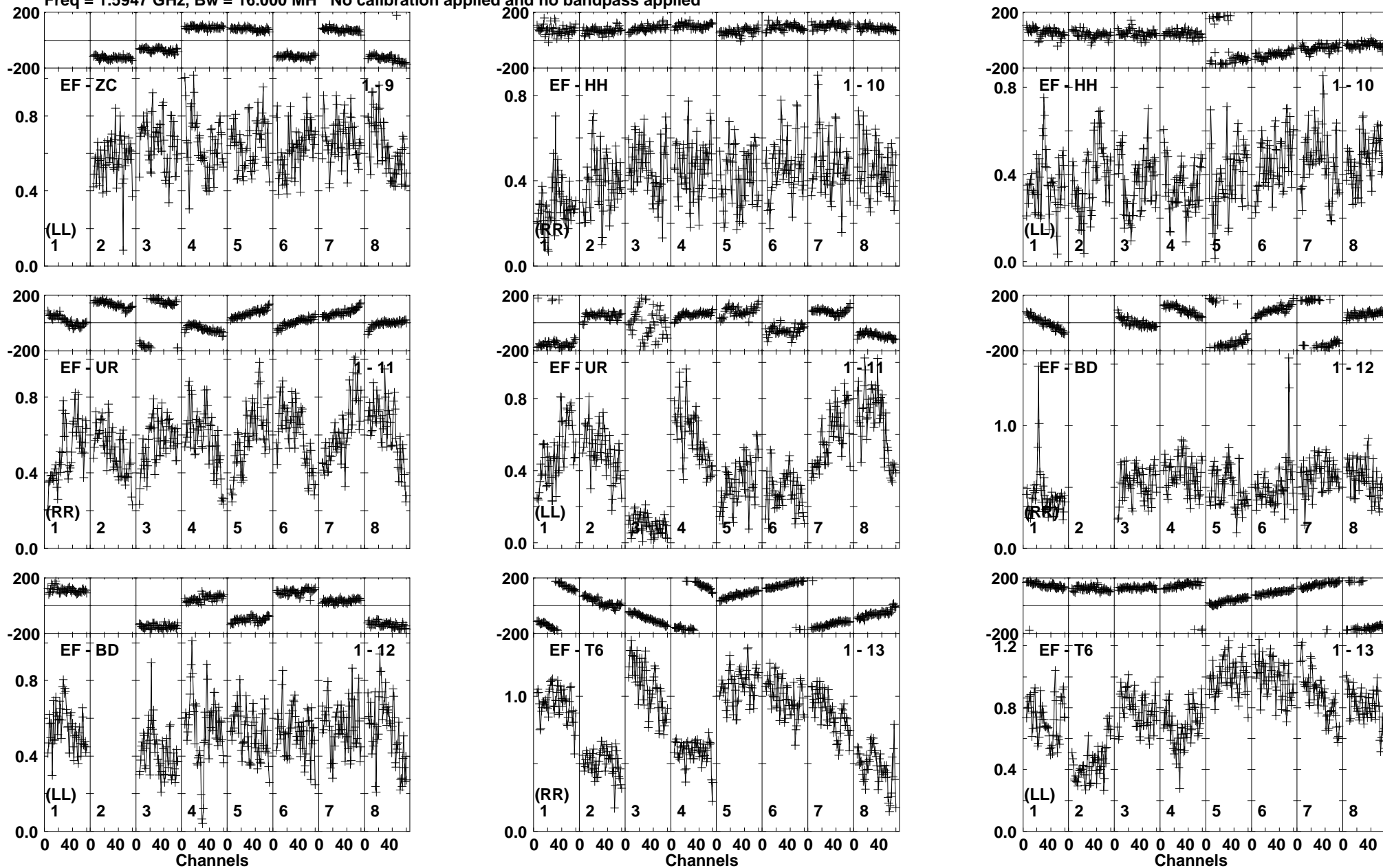
Lower frame: Milli Amp Jy Top frame: Phas deg Vector averaged cross-power spectrum Baseline: EF (01) - ZC (09) Timerange: 00/17:48:35 to 00/17:50:00
