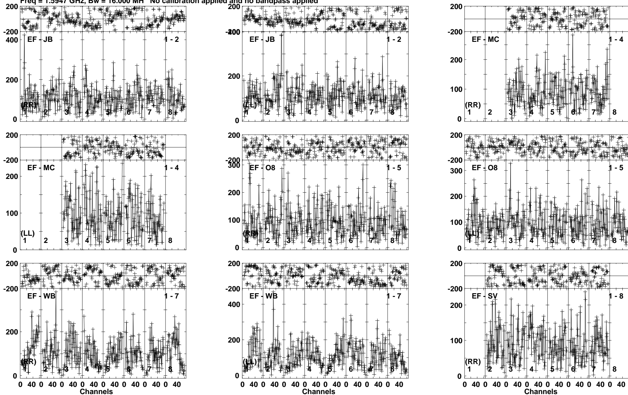
Lower frame: Micro Ampl Jy Top frame: Phas deg Vector averaged cross-power spectrum Baseline: EF (01) - JB (02) Timerange: 01/03:00:07 to 01/03:03:29
