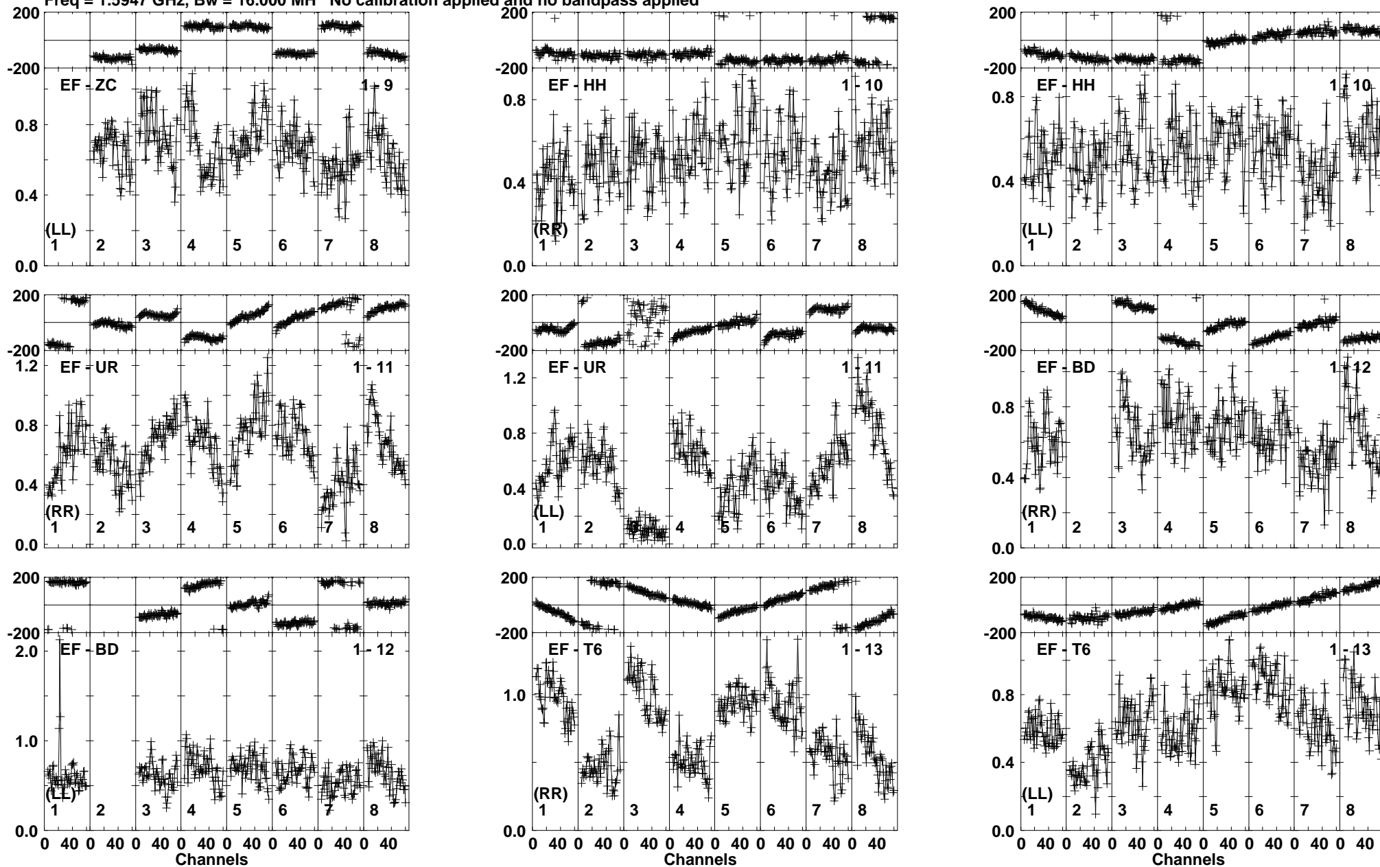
Lower frame: Milli Ampl Jy Top frame: Phas deg Vector averaged cross-power spectrum Baseline: EF (01) - ZC (09) Timerange: 00:19:38:45 to 00:19:40:09
