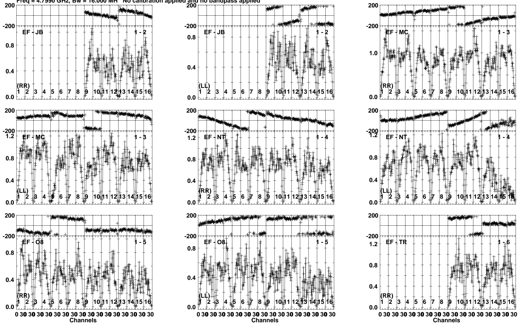
Lower frame: Milli Ampl Jy Top frame: Phas deg Vector averaged cross-power spectrum Baseline: EF (01) - JB (02) Timerange: 00/15:27:47 to 00/15:29:09
