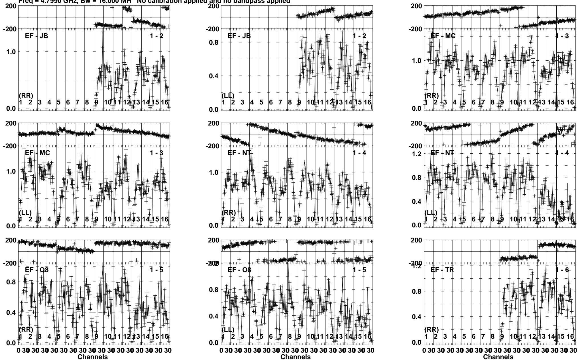
Lower frame: Milli Ampl Jy Top frame: Phas deg Vector averaged cross-power spectrum Baseline: EF (01) - JB (02) Timerange: 00/19:25:05 to 00/19:26:29
