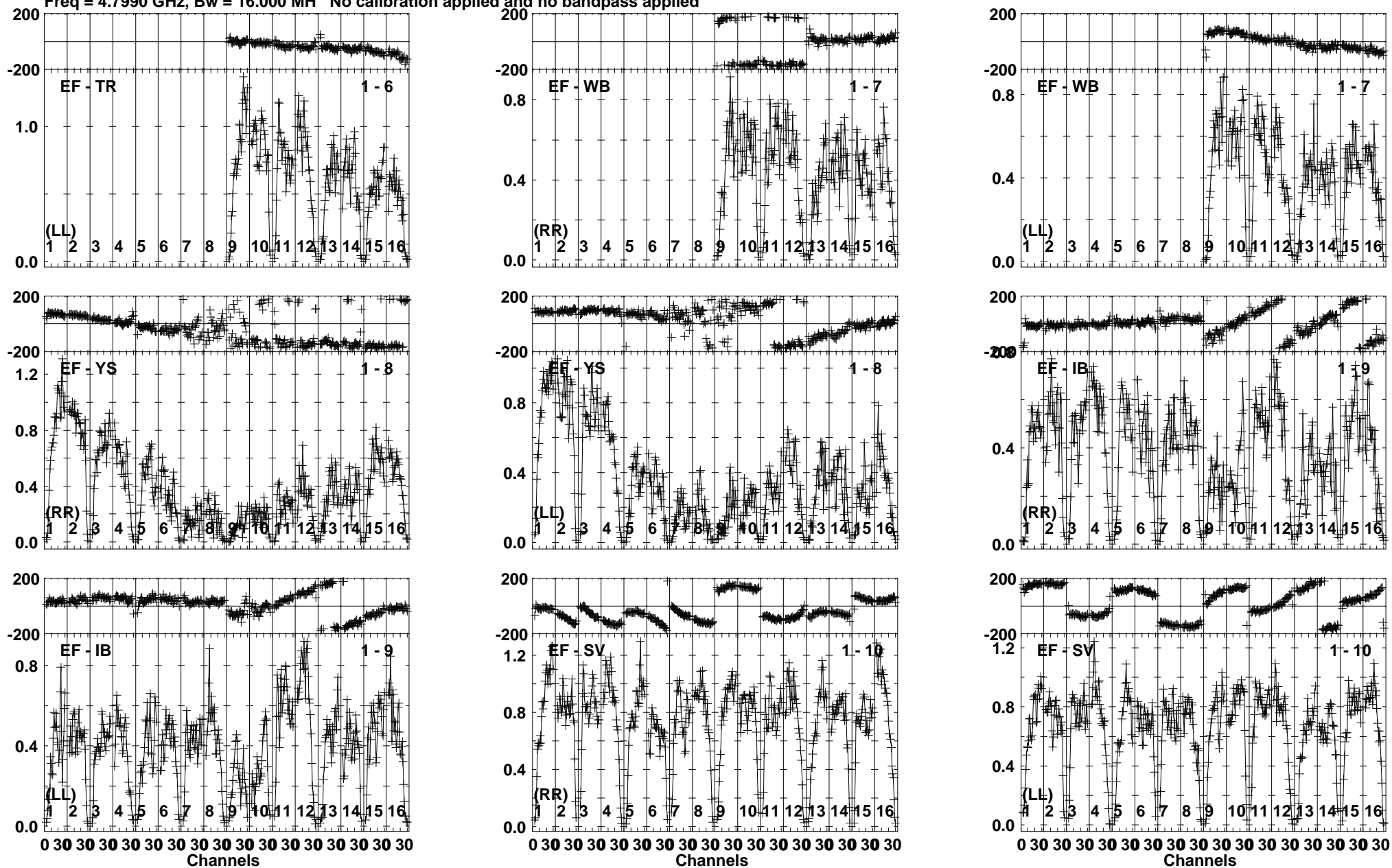
Lower frame: Milli Ampl Jy Top frame: Phas deg Vector averaged cross-power spectrum Baseline: EF (01) - TR (06) Timerange: 00/19:14:45 to 00/19:16:09
