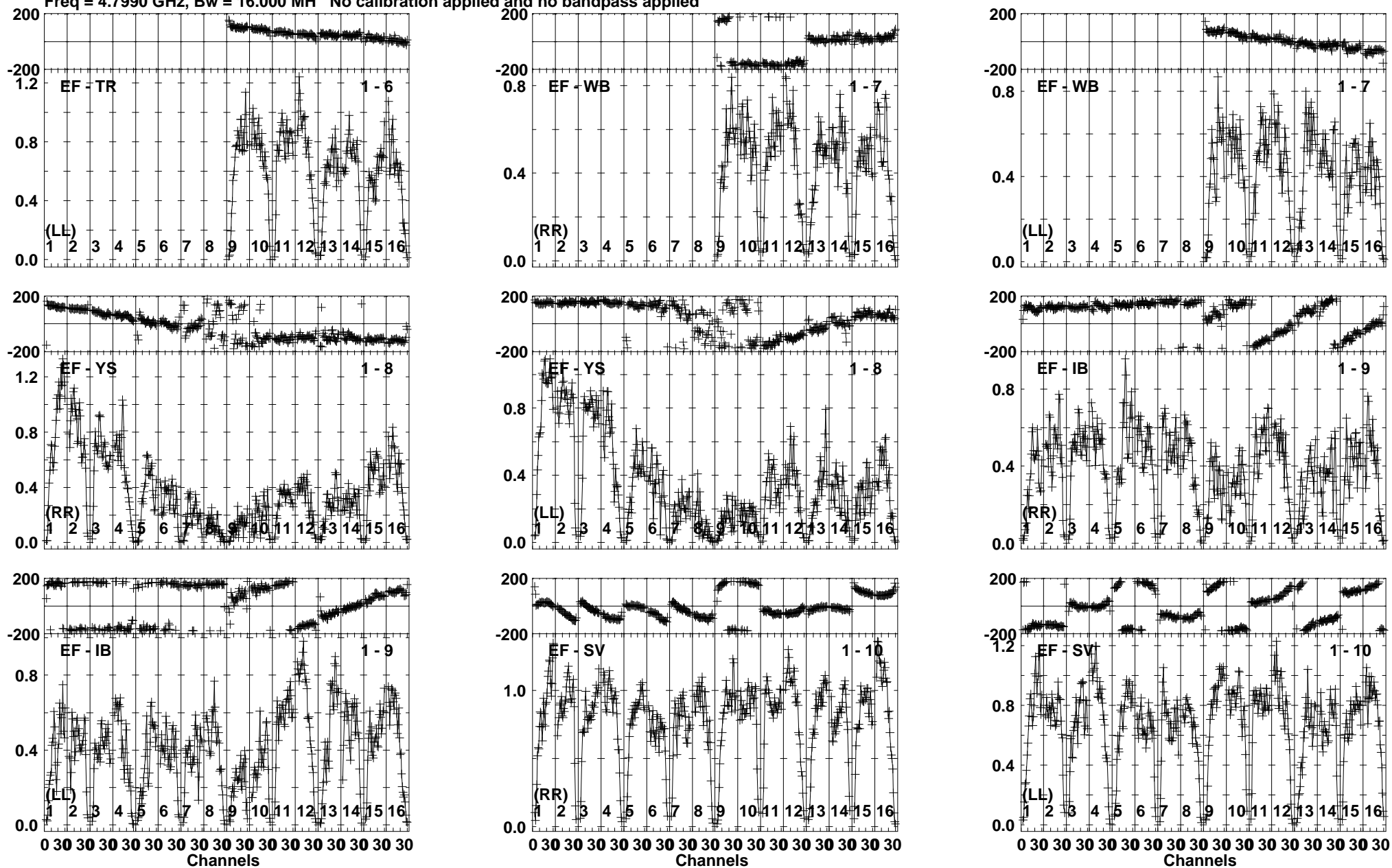
Lower frame: Milli Ampl Jy Top frame: Phas deg Vector averaged cross-power spectrum Baseline: EF (01) - TR (06) Timerange: 00/19:10:11 to 00/19:11:09
