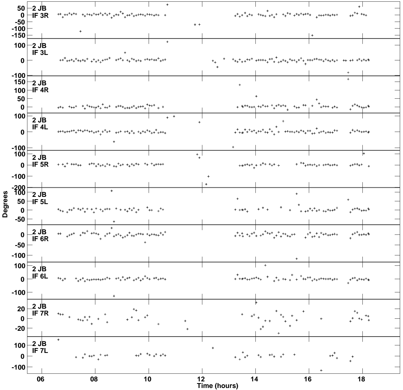
Plot file version 3 created 12-JAN-2018 16:11:49 Gain phs vs UTC time for J0529+3209.MULTI.1 SN 1 Rpol & Lpol IF 1 - 8
