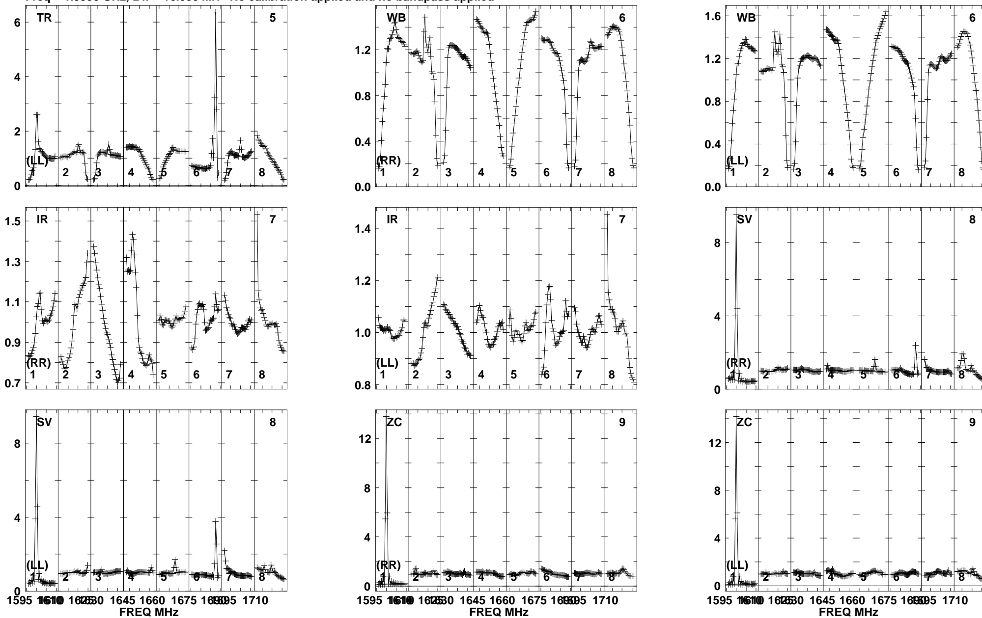
Lower frame: Real Jy Total-power spectrum Antenna: TR (05) Timerange: 00/13:15:41 to 00/13:18:39
