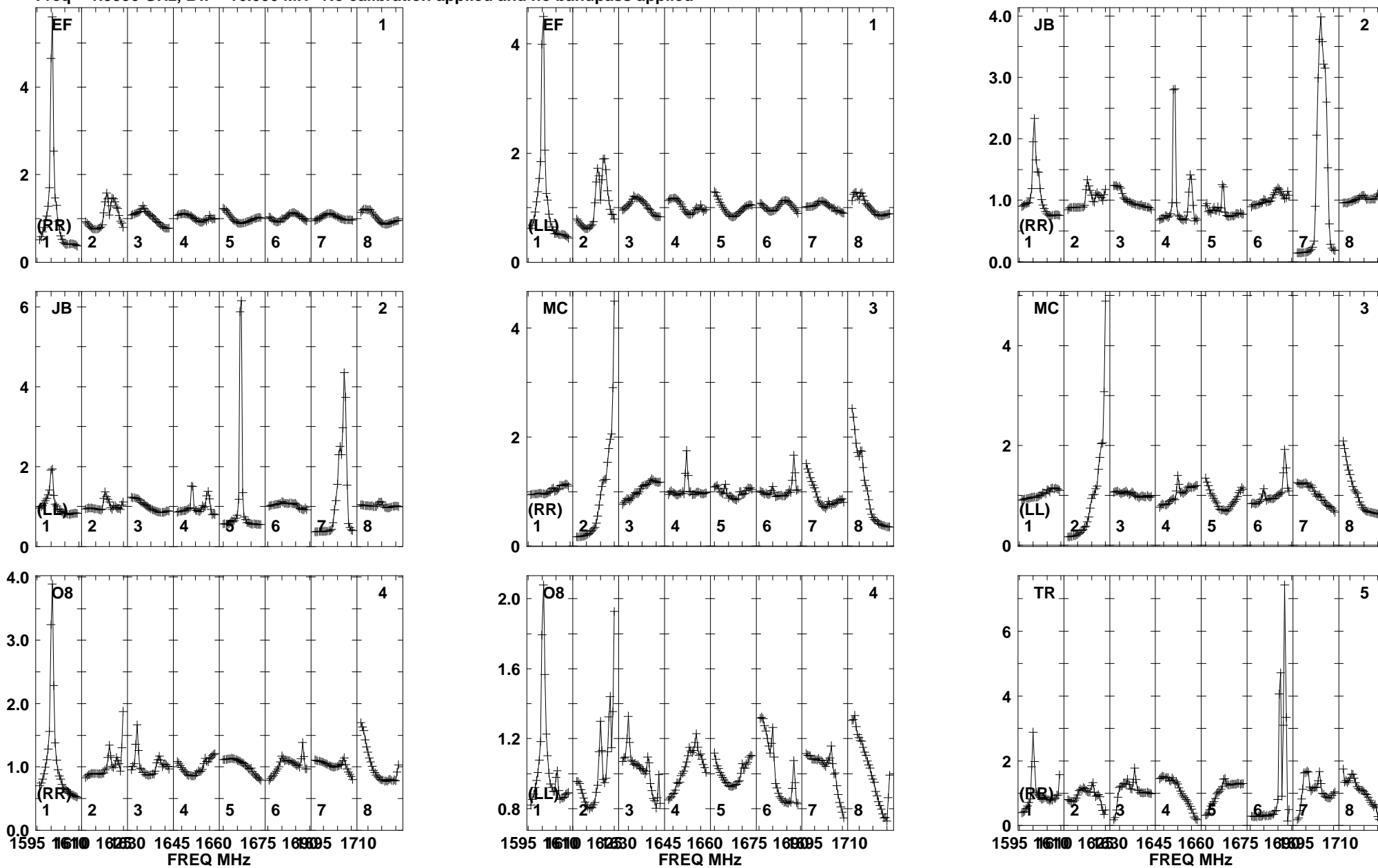
Lower frame: Real Jy Total-power spectrum Antenna: EF (01) Timerange: 00/13:35:33 to 00/13:36:59
