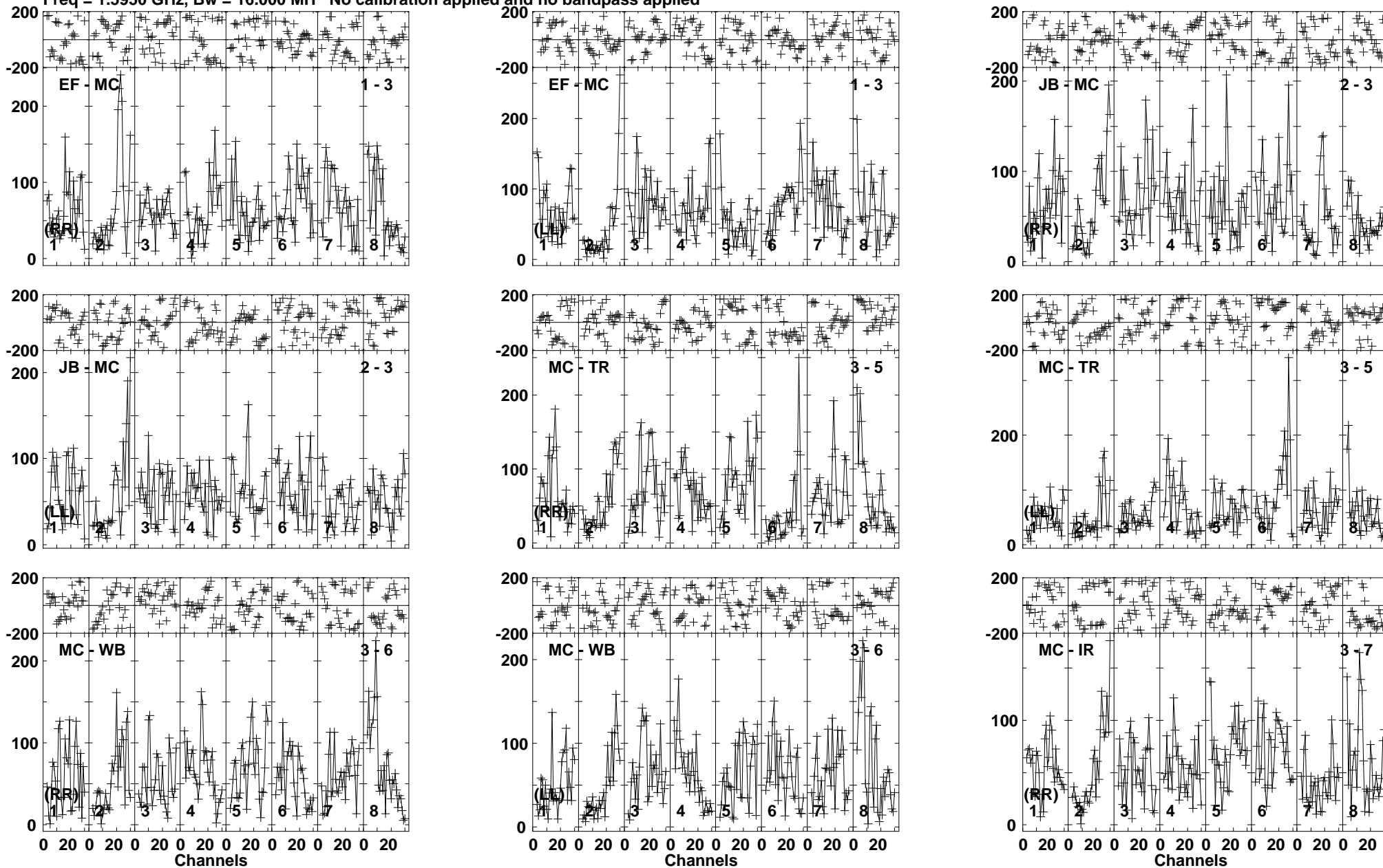
Lower frame: Micro Ampl Jy Top frame: Phas deg Vector averaged cross-power spectrum Baseline: EF (01) - MC (03) Timerange: 00/08:12:33 to 00/08:15:59
