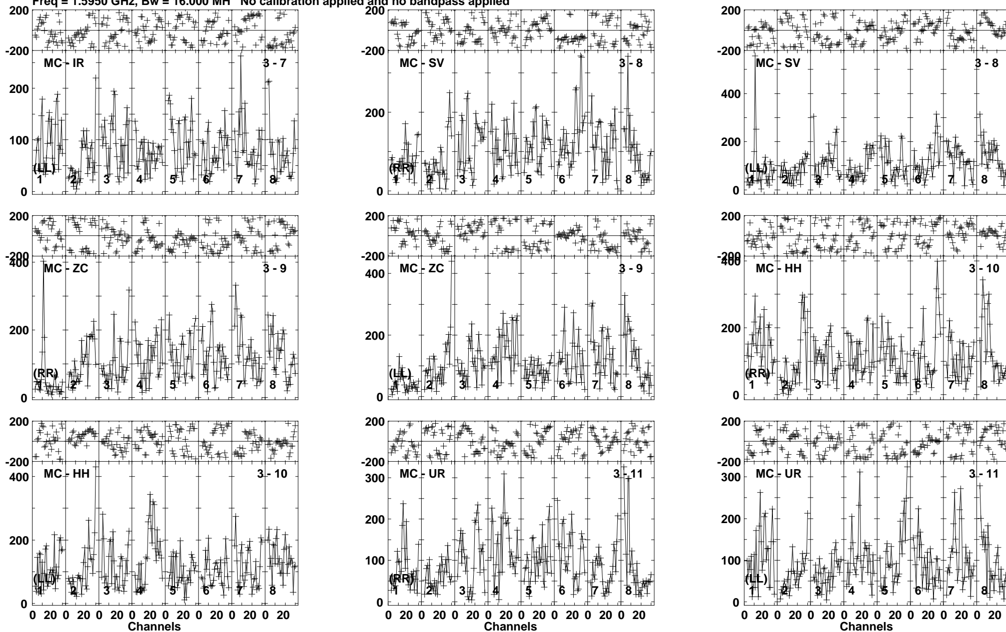
Lower frame: Micro Ampl Jy Top frame: Phas deg Vector averaged cross-power spectrum Baseline: MC (03) - IR (07) Timerange: 00/12:33:21 to 00/12:34:49
