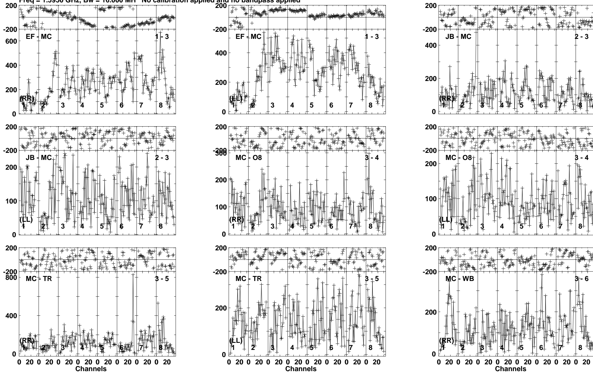
Lower frame: Micro Ampl Jy Top frame: Phas deg Vector averaged cross-power spectrum Baseline: EF (01) - MC (03) Timerange: 00/18:07:03 to 00/18:08:29
