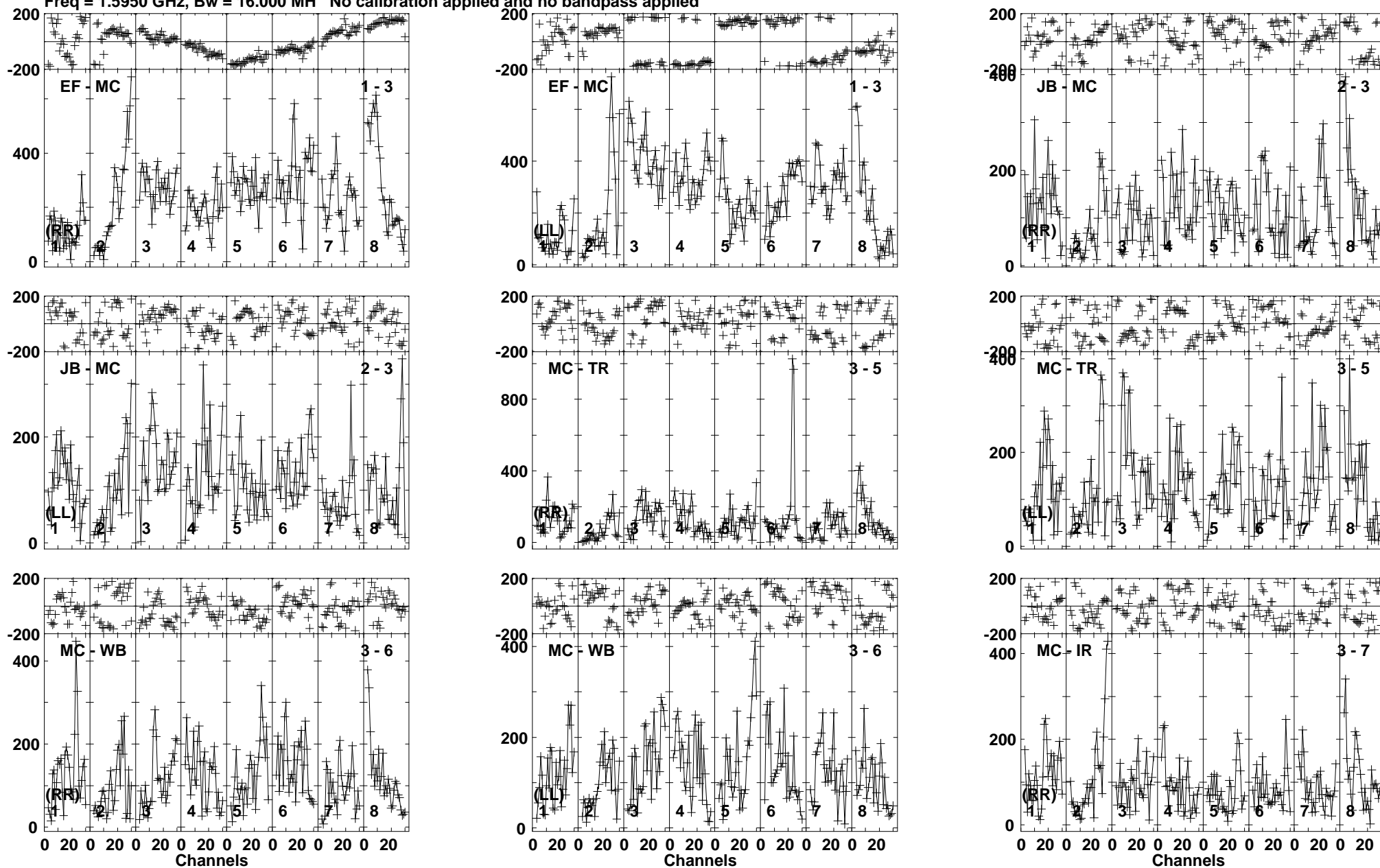
Lower frame: Micro Ampl Jy Top frame: Phas deg Vector averaged cross-power spectrum Baseline: EF (01) - MC (03) Timerange: 00/07:11:03 to 00/07:12:29
