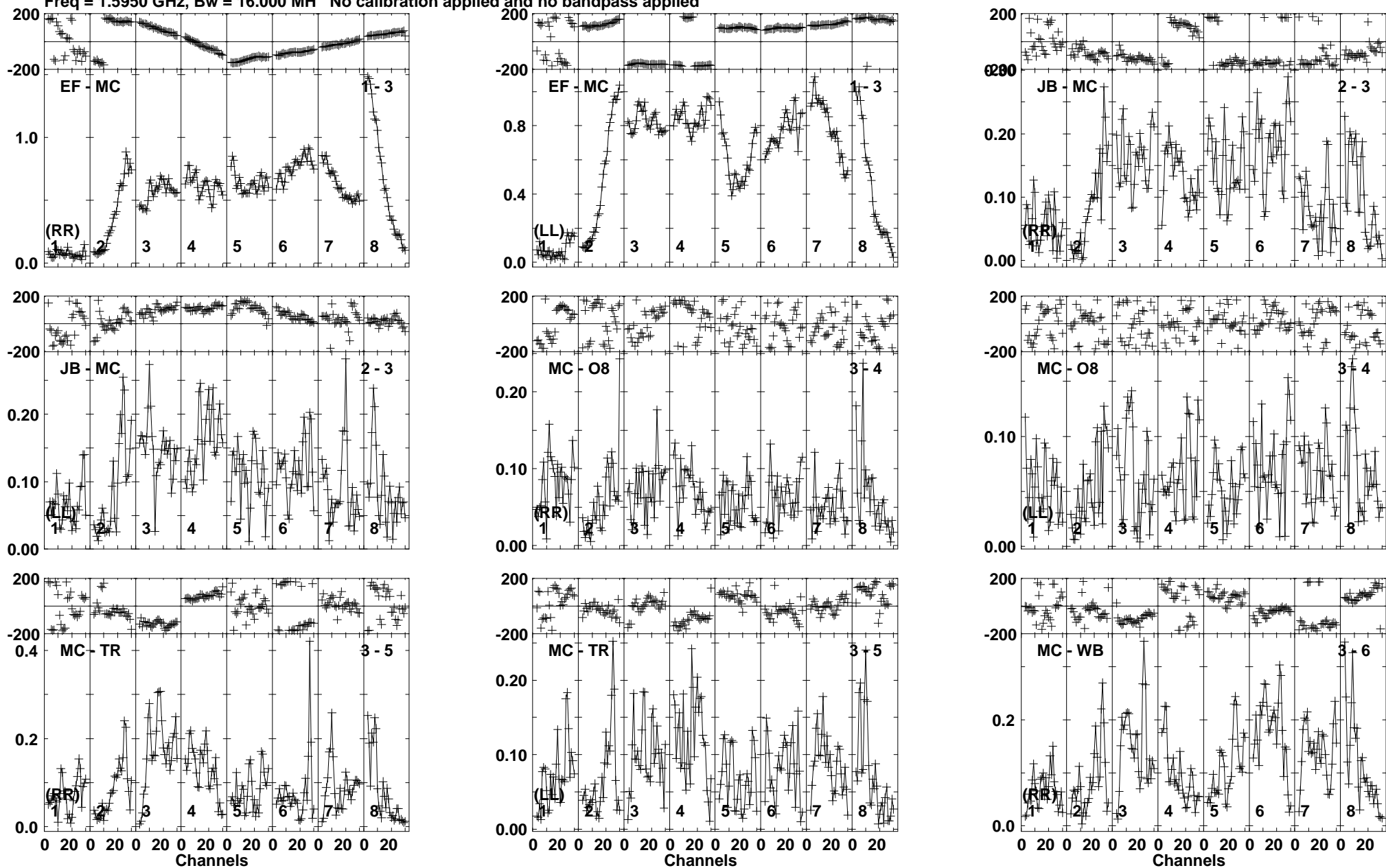
Lower frame: Milli Ampl Jy Top frame: Phas deg Vector averaged cross-power spectrum Baseline: EF (01) - MC (03) Timerange: 00:17:39:01 to 00:17:41:59
