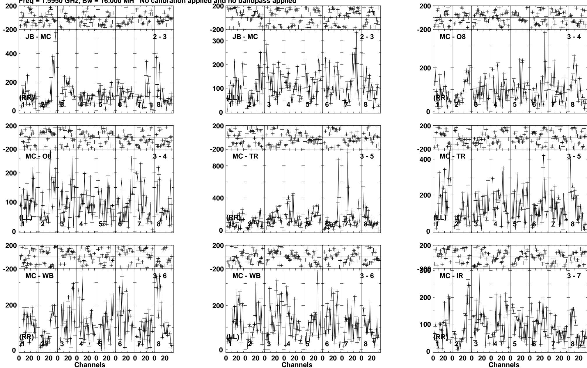
Lower frame: Micro Ampl Jy Top frame: Phas deg Vector averaged cross-power spectrum Baseline: JB (02) - MC (03) Timerange: 00/17:21:51 to 00/17:23:19
