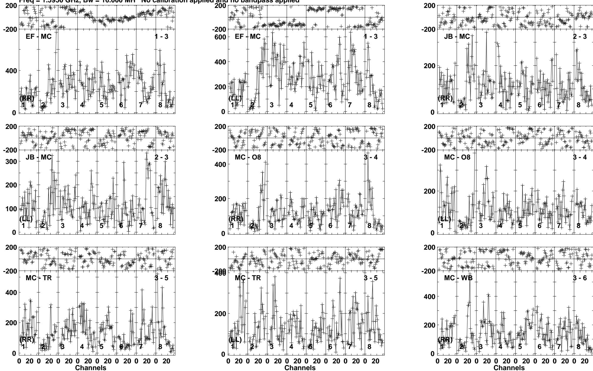
Lower frame: Micro Ampl Jy Top frame: Phas deg Vector averaged cross-power spectrum Baseline: EF (01) - MC (03) Timerange: 00/17:32:21 to 00/17:33:19
