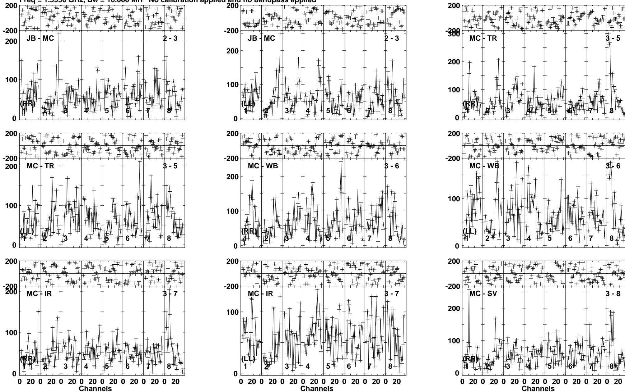
Lower frame: Micro Ampl Jy Top frame: Phas deg Vector averaged cross-power spectrum Baseline: JB (02) - MC (03) Timerange: 00/10:47:31 to 00/10:50:59
