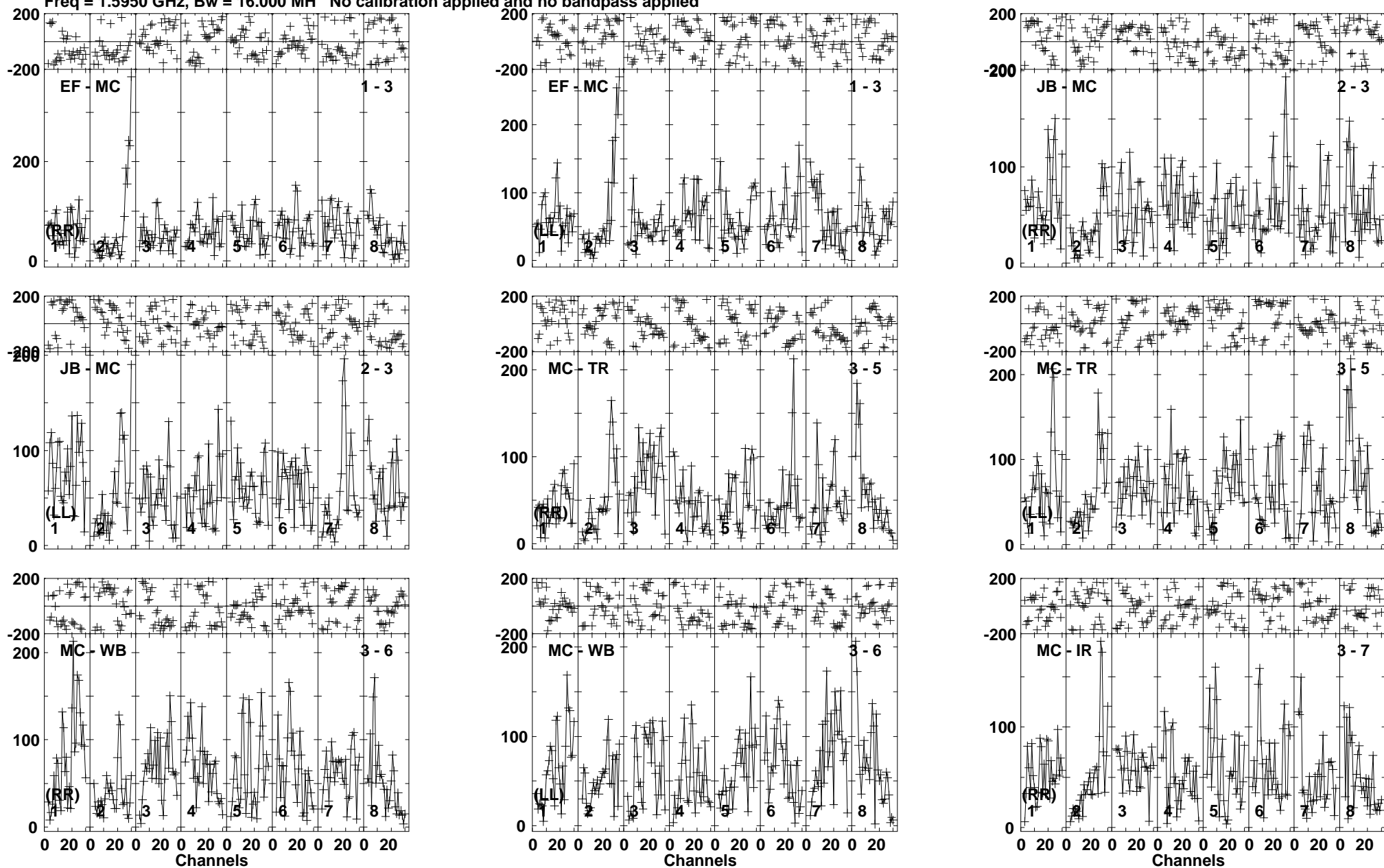
Lower frame: Micro Ampl Jy Top frame: Phas deg Vector averaged cross-power spectrum Baseline: EF (01) - MC (03) Timerange: 00/07:07:33 to 00/07:10:59
