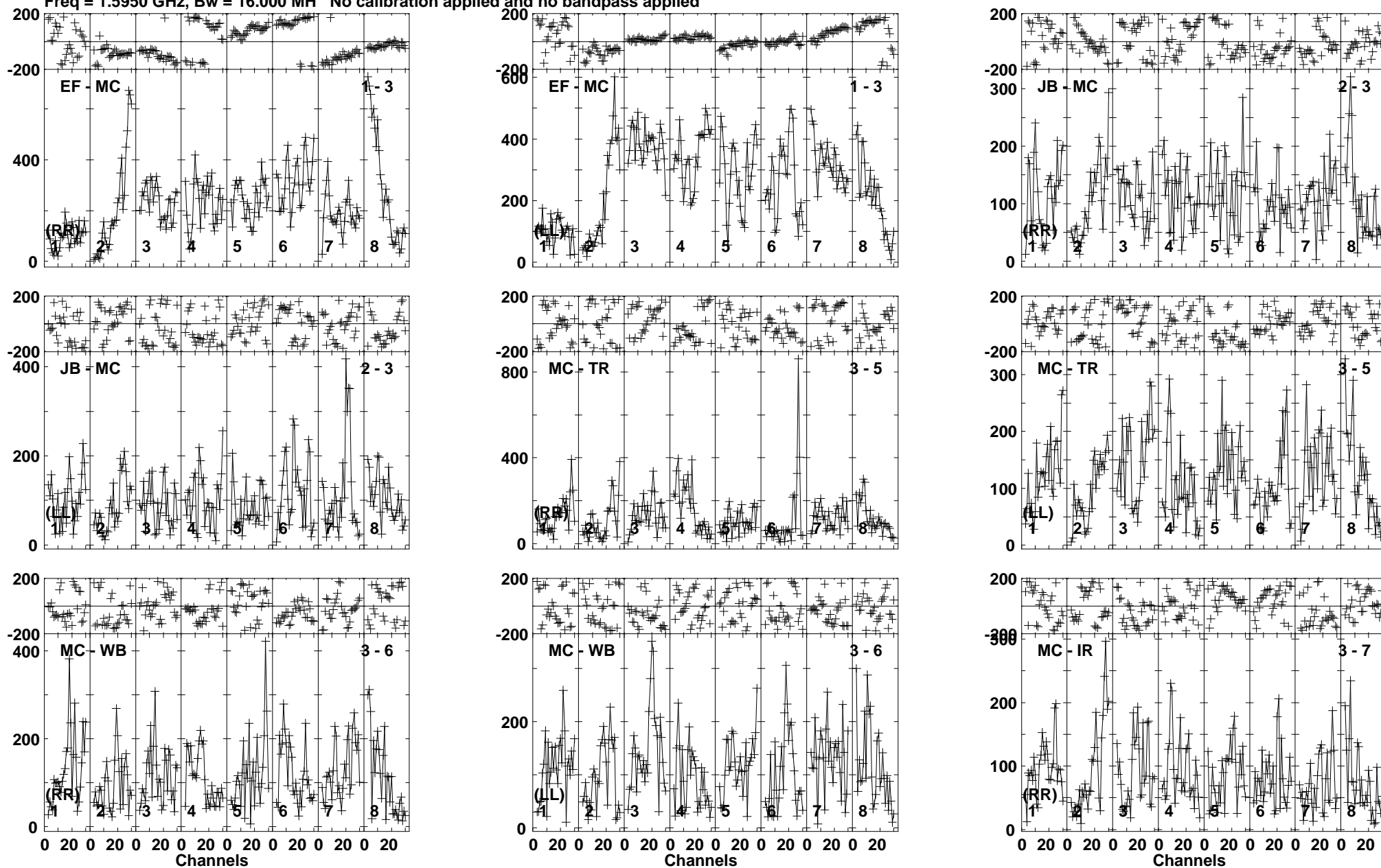
Lower frame: Micro Ampl Jy Top frame: Phas deg Vector averaged cross-power spectrum Baseline: EF (01) - MC (03) Timerange: 00/07:26:01 to 00/07:27:29
