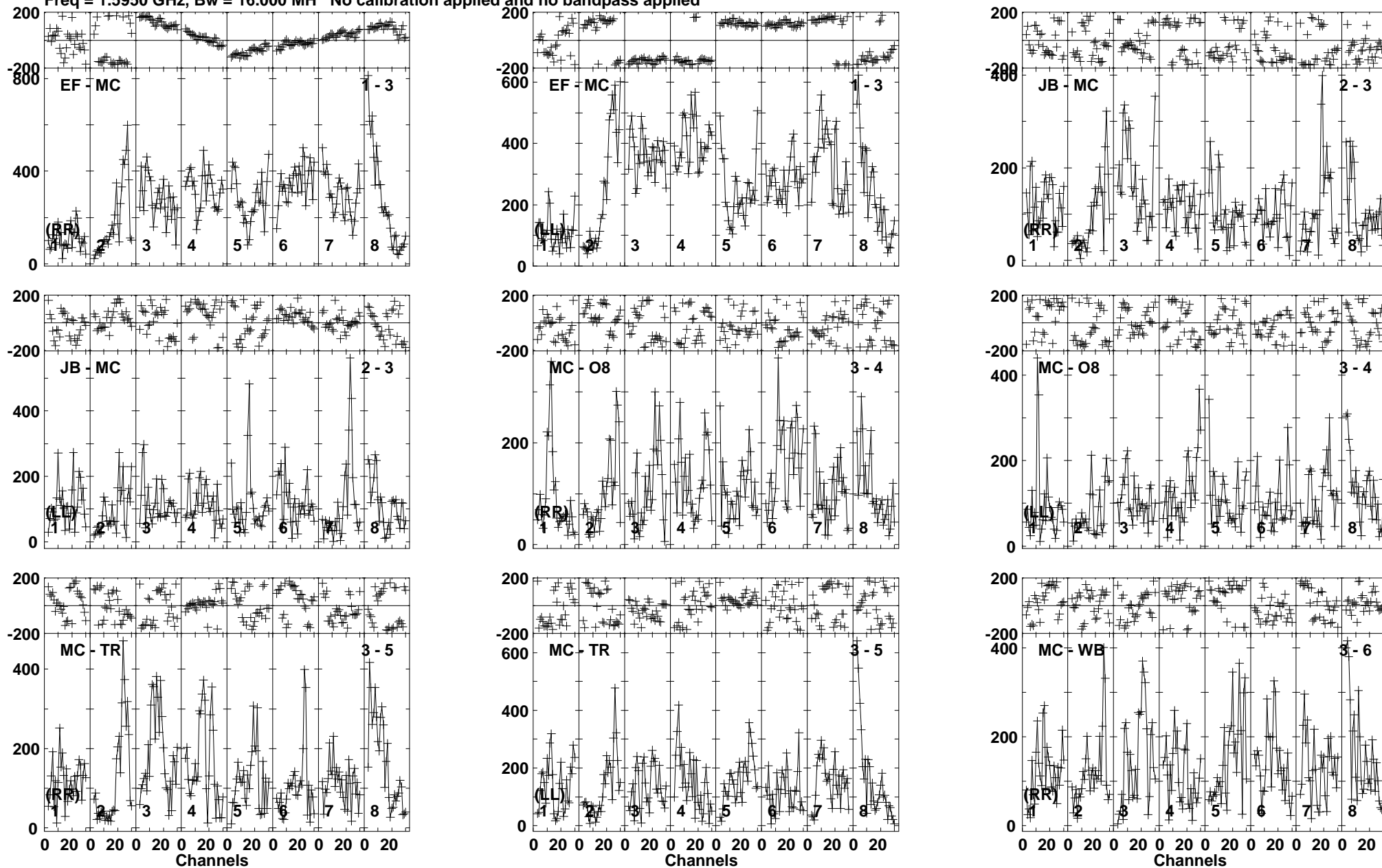
Lower frame: Micro Ampl Jy Top frame: Phas deg Vector averaged cross-power spectrum Baseline: EF (01) - MC (03) Timerange: 00/13:51:01 to 00/13:51:59
