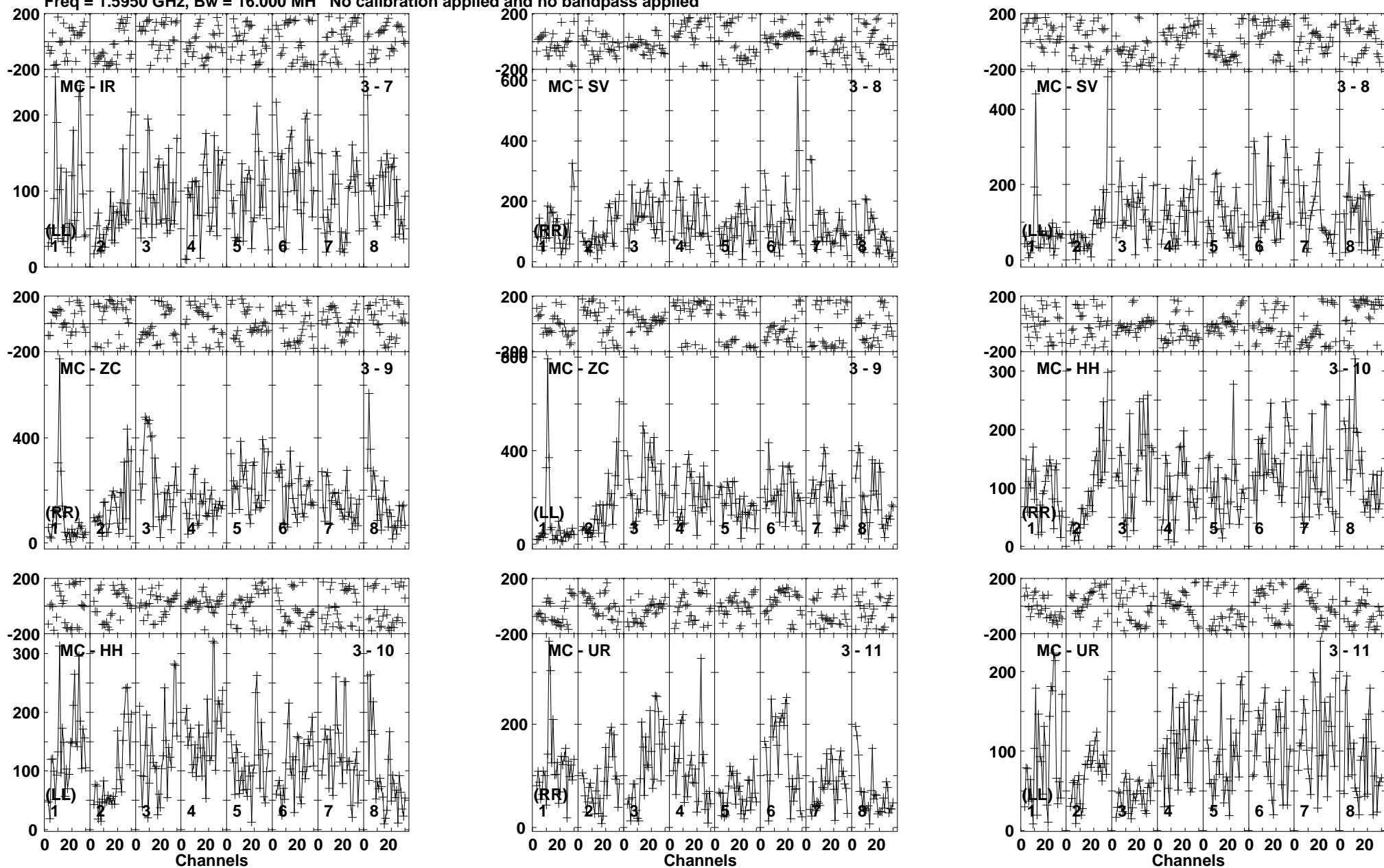
Lower frame: Micro Ampl Jy Top frame: Phas deg Vector averaged cross-power spectrum Baseline: MC (03) - IR (07) Timerange: 00/09:51:03 to 00/09:52:29
