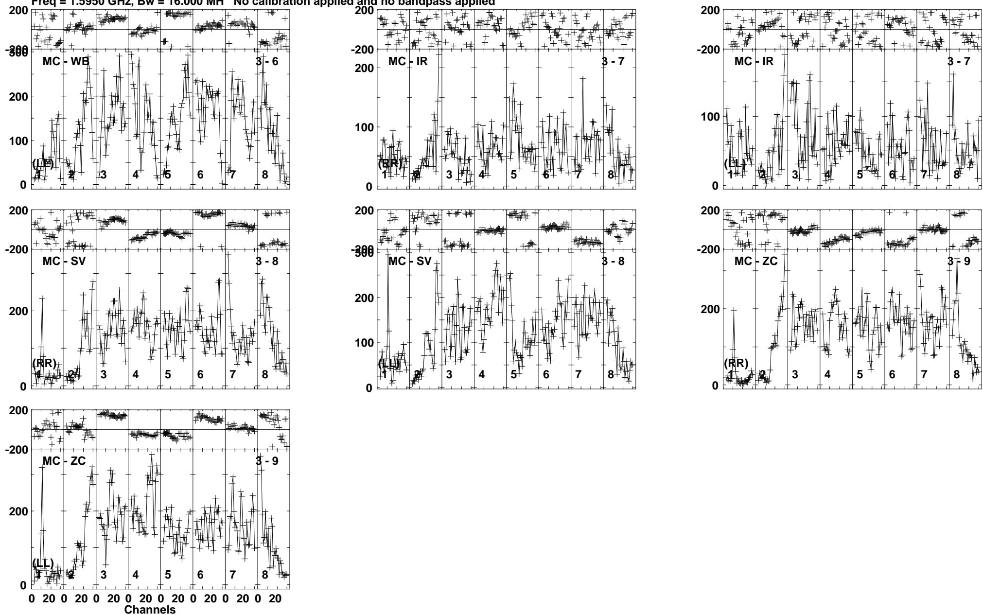
Lower frame: Micro Ampl Jy Top frame: Phas deg Vector averaged cross-power spectrum Baseline: MC (03) - WB (06) Timerange: 00/16:08:31 to 00/16:11:29
