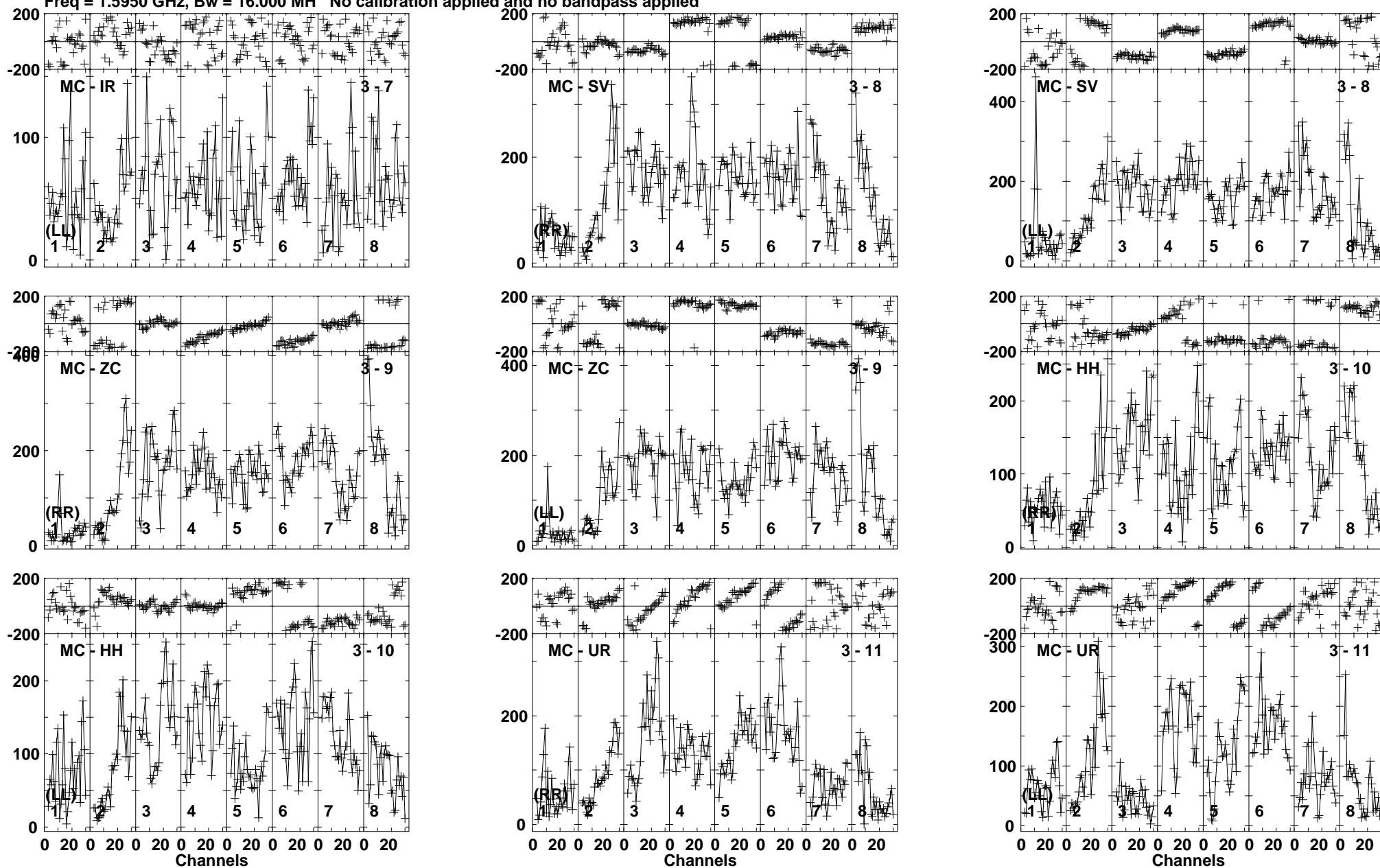
Lower frame: Micro Ampl Jy Top frame: Phas deg Vector averaged cross-power spectrum Baseline: MC (03) - IR (07) Timerange: 00/11:03:01 to 00/11:05:59
