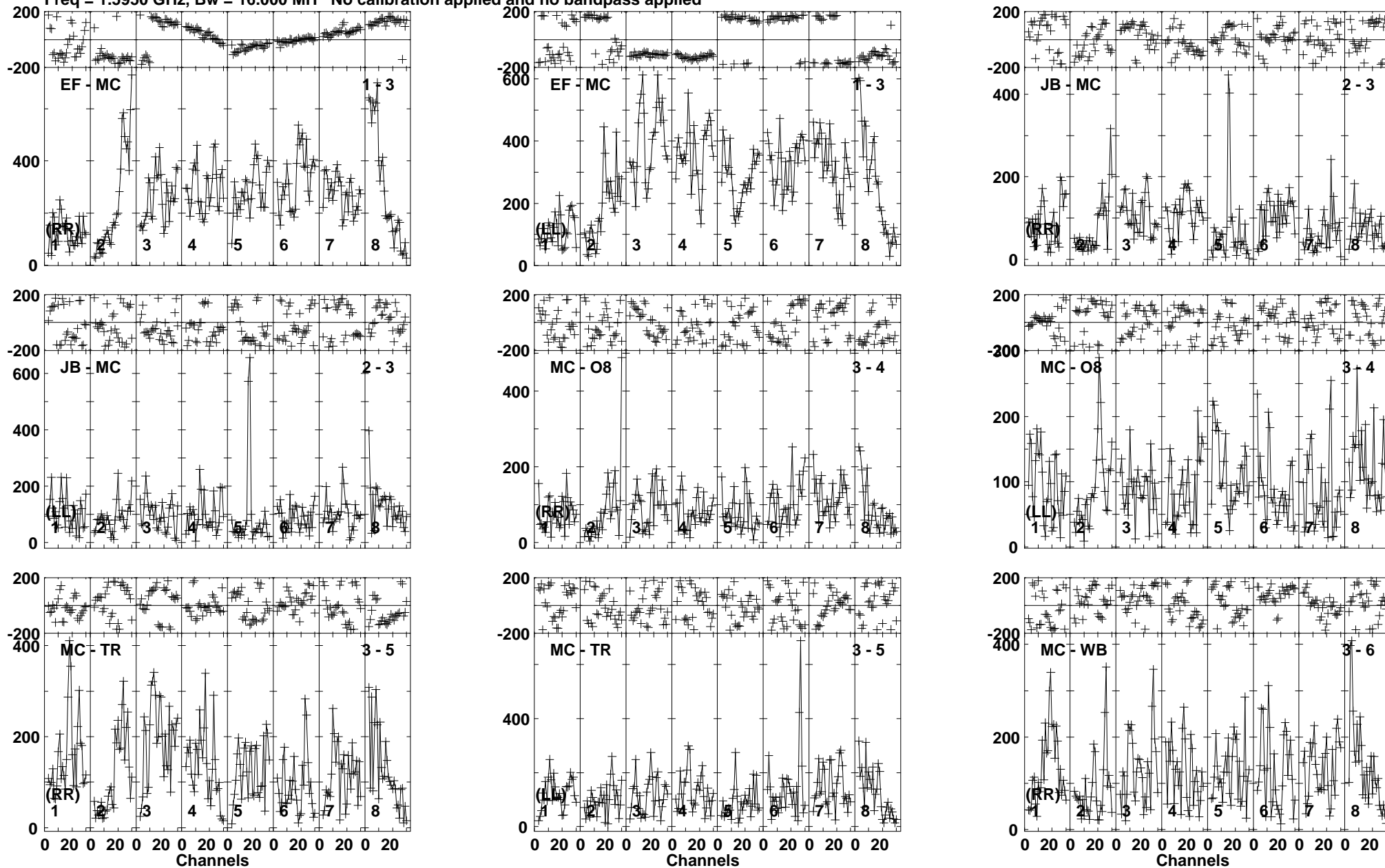
Lower frame: Micro Ampl Jy Top frame: Phas deg Vector averaged cross-power spectrum Baseline: EF (01) - MC (03) Timerange: 00/15:01:03 to 00/15:02:29
