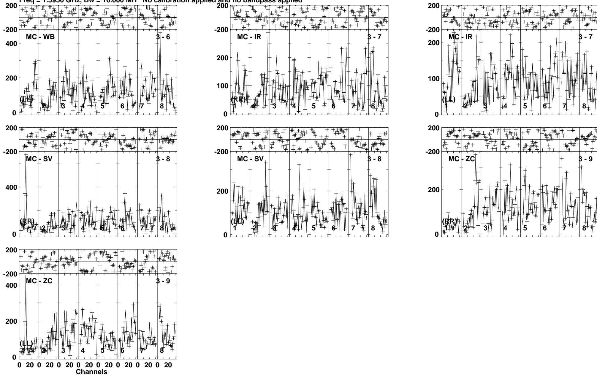
Lower frame: Micro Ampl Jy Top frame: Phas deg Vector averaged cross-power spectrum Baseline: MC (03) - WB (06) Timerange: 00/14:30:53 to 00/14:32:19
