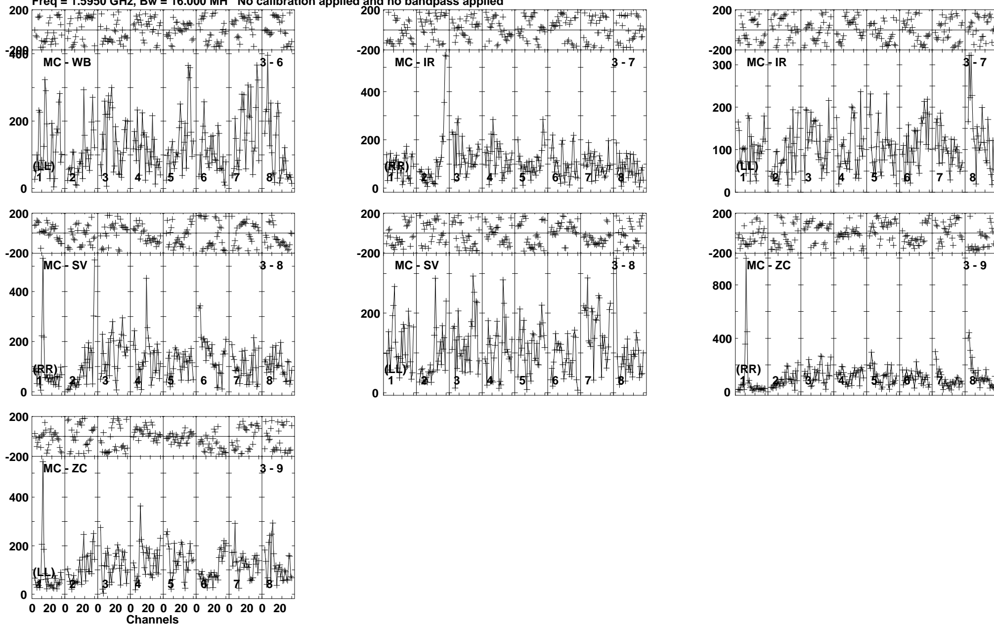
Lower frame: Micro Ampl Jy Top frame: Phas deg Vector averaged cross-power spectrum Baseline: MC (03) - WB (06) Timerange: 00/15:36:41 to 00/15:37:39
