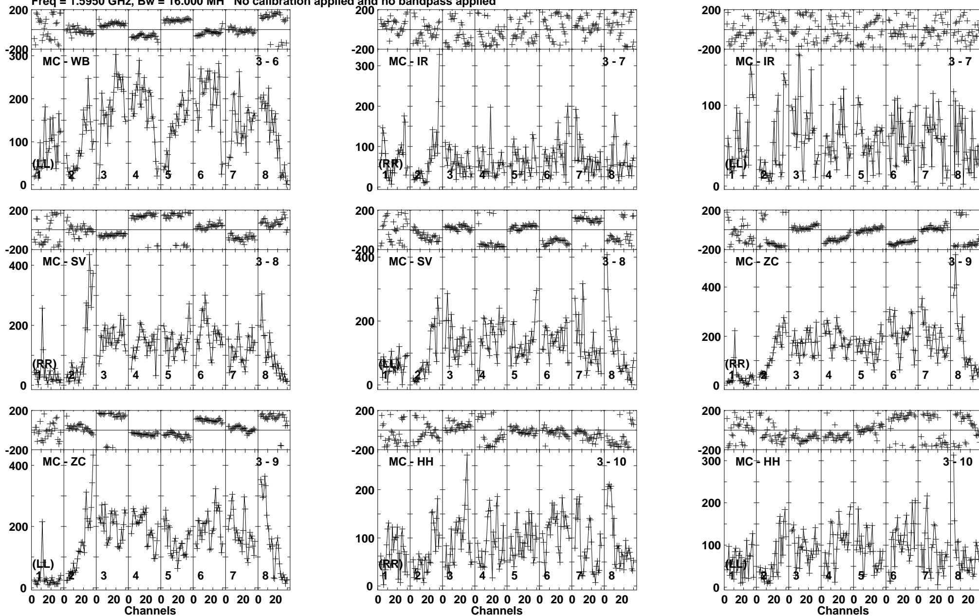
Lower frame: Micro Ampl Jy Top frame: Phas deg Vector averaged cross-power spectrum Baseline: MC (03) - WB (06) Timerange: 00/14:17:51 to 00/14:20:49
