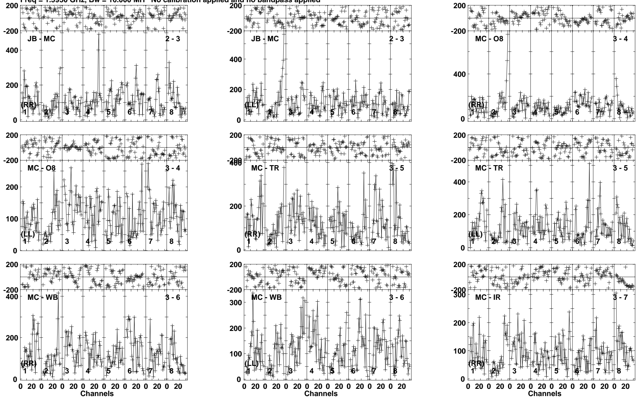
Lower frame: Micro Ampl Jy Top frame: Phas deg Vector averaged cross-power spectrum Baseline: JB (02) - MC (03) Timerange: 00/11:21:03 to 00/11:22:29
