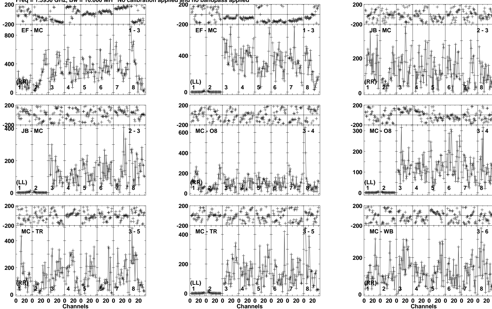
Lower frame: Micro Ampl Jy Top frame: Phas deg Vector averaged cross-power spectrum Baseline: EF (01) - MC (03) Timerange: 00/13:18:43 to 00/13:20:09
