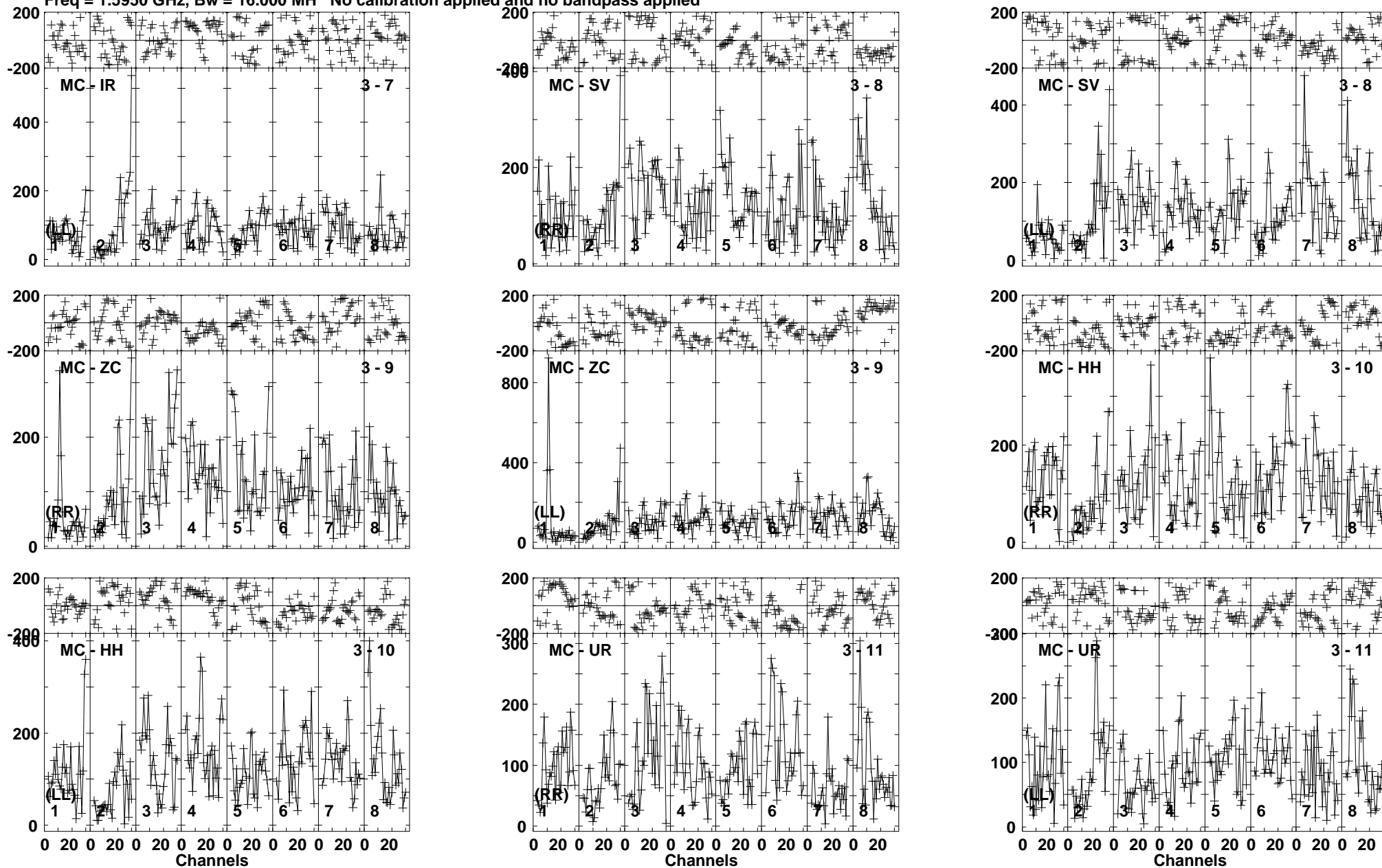
Lower frame: Micro Ampl Jy Top frame: Phas deg Vector averaged cross-power spectrum Baseline: MC (03) - IR (07) Timerange: 00/11:53:03 to 00/11:54:29
