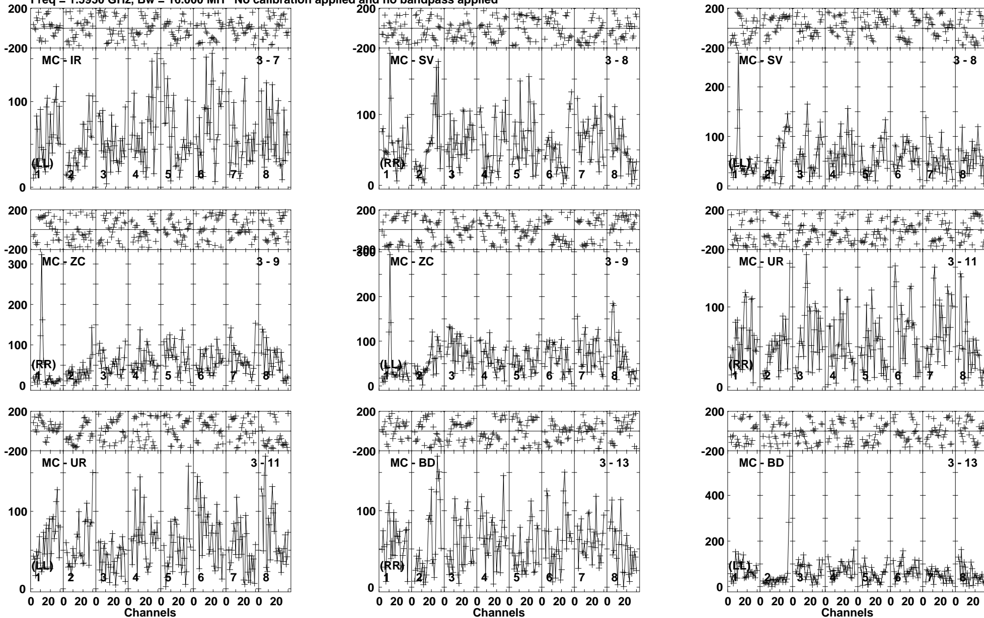
Lower frame: Micro Ampl Jy Top frame: Phas deg Vector averaged cross-power spectrum Baseline: MC (03) - IR (07) Timerange: 00/08:17:31 to 00/08:20:59
