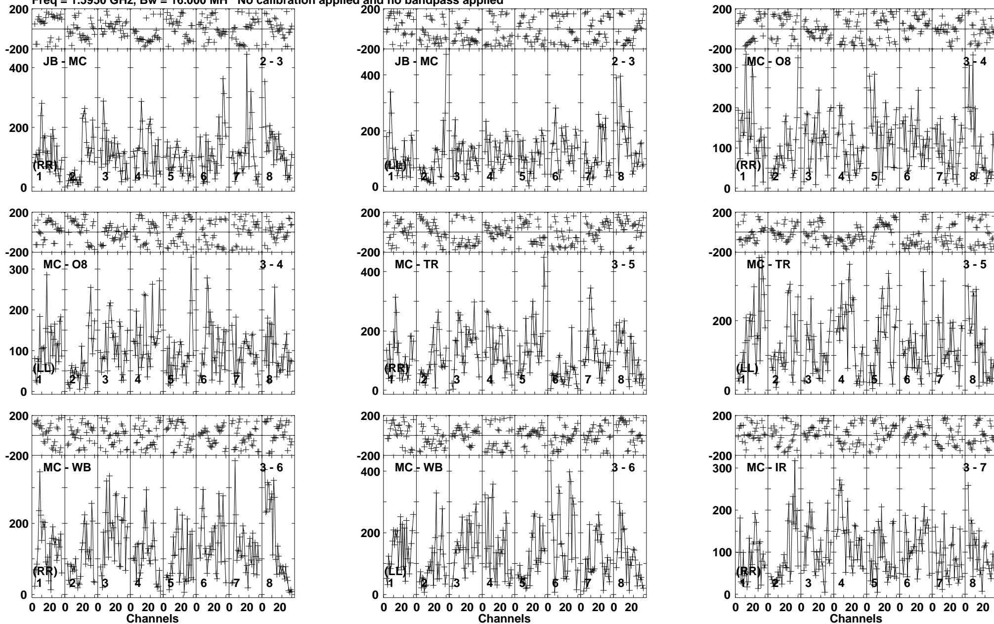
Lower frame: Micro Ampl Jy Top frame: Phas deg Vector averaged cross-power spectrum Baseline: JB (02) - MC (03) Timerange: 00/17:17:21 to 00/17:18:19
