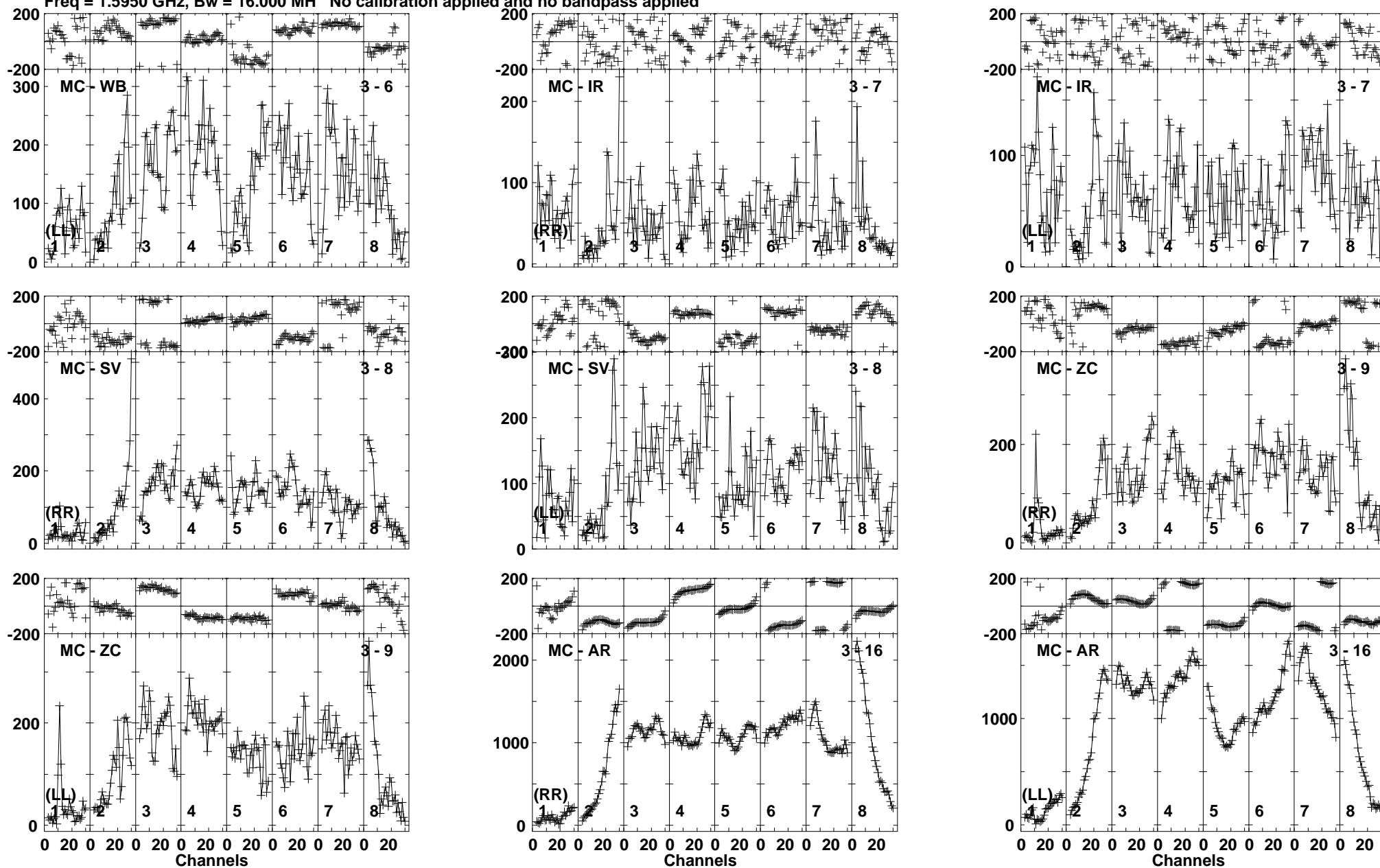
Lower frame: Micro Ampl Jy Top frame: Phas deg Vector averaged cross-power spectrum Baseline: MC (03) - WB (06) Timerange: 00/16:33:41 to 00/16:36:39
