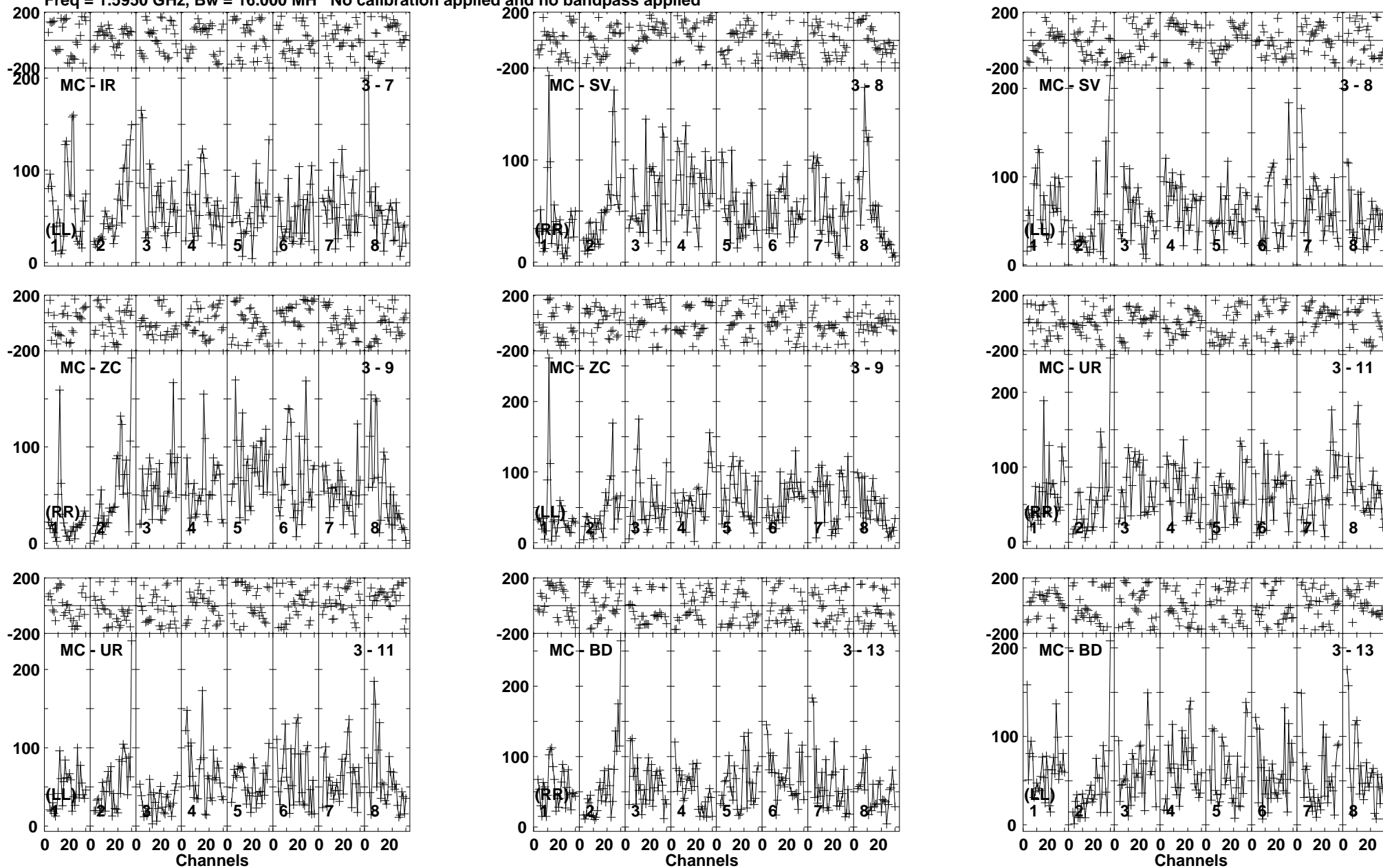
Lower frame: Micro Ampl Jy Top frame: Phas deg Vector averaged cross-power spectrum Baseline: MC (03) - IR (07) Timerange: 00/06:57:33 to 00/07:00:59
