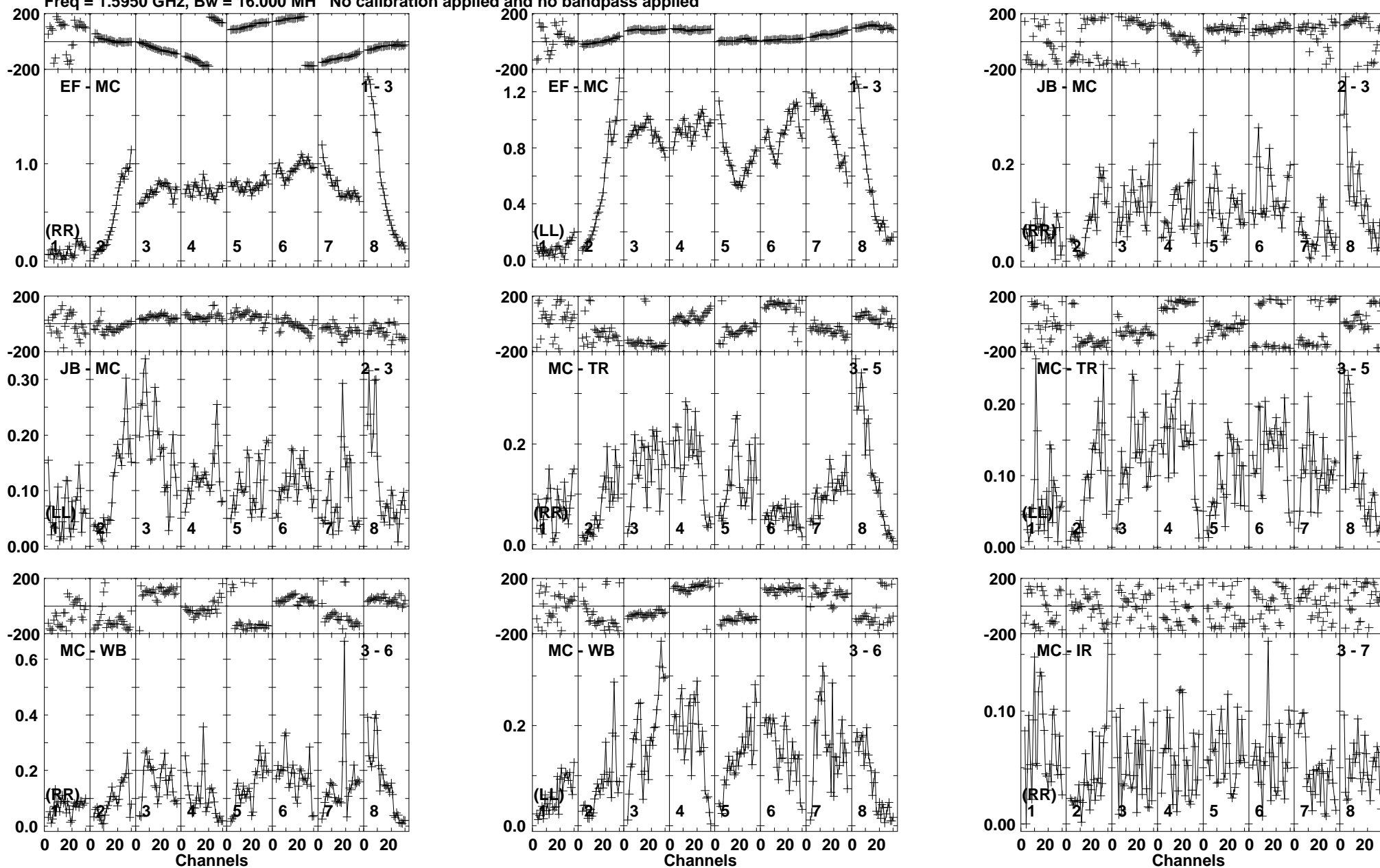
Lower frame: Milli Ampl Jy Top frame: Phas deg Vector averaged cross-power spectrum Baseline: EF (01) - MC (03) Timerange: 00/10:13:03 to 00/10:15:59
