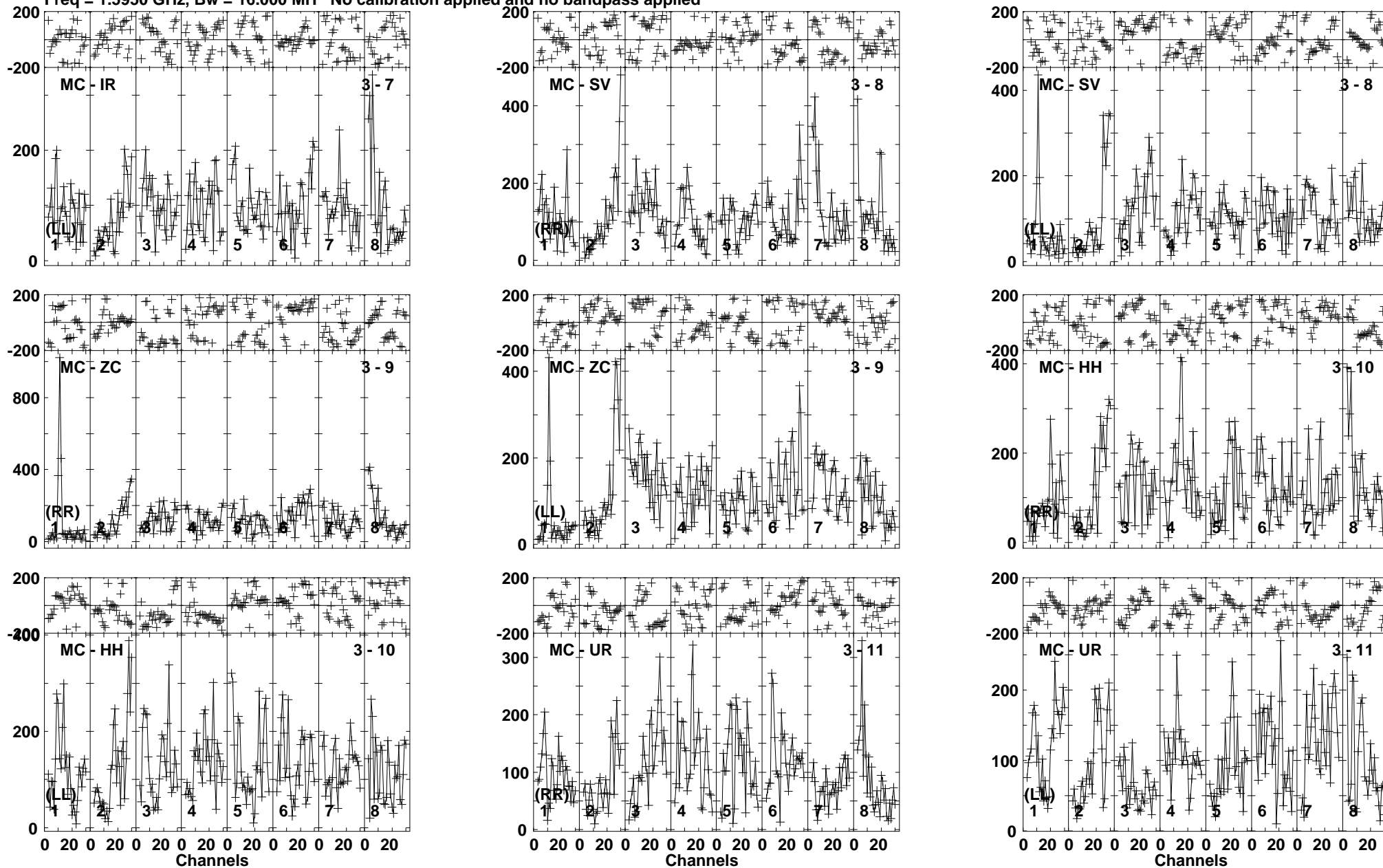
Lower frame: Micro Ampl Jy Top frame: Phas deg Vector averaged cross-power spectrum Baseline: MC (03) - IR (07) Timerange: 00/11:21:03 to 00/11:22:29
