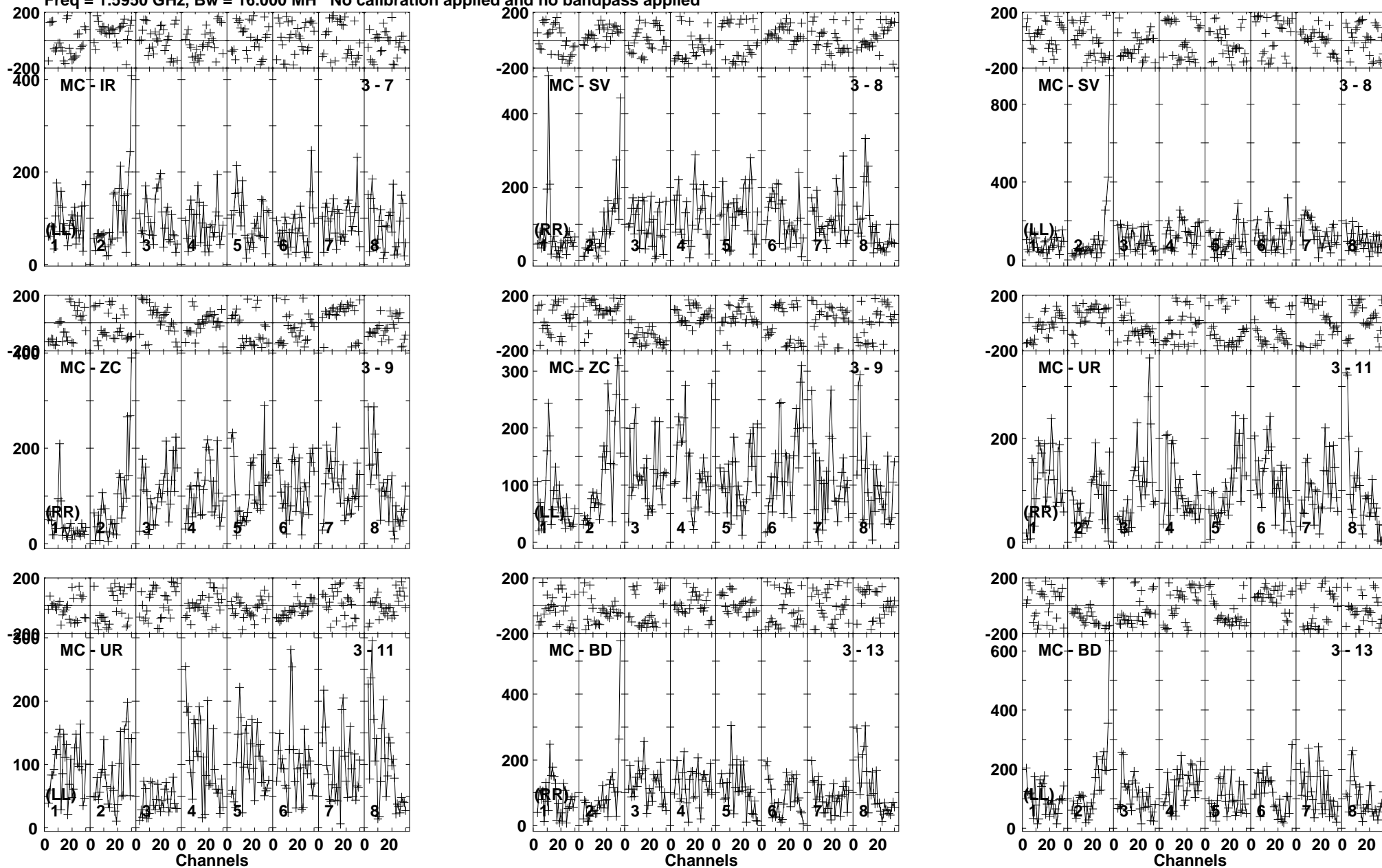
Lower frame: Micro Ampl Jy Top frame: Phas deg Vector averaged cross-power spectrum Baseline: MC (03) - IR (07) Timerange: 00/07:11:03 to 00/07:12:29
