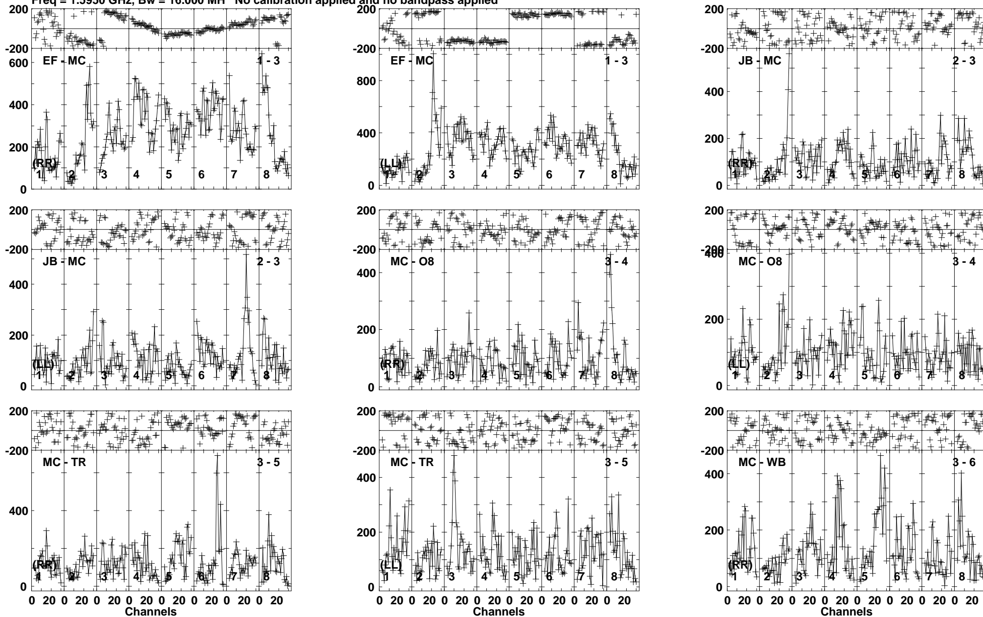
Lower frame: Micro Ampl Jy Top frame: Phas deg Vector averaged cross-power spectrum Baseline: EF (01) - MC (03) Timerange: 00/14:30:53 to 00/14:32:19
