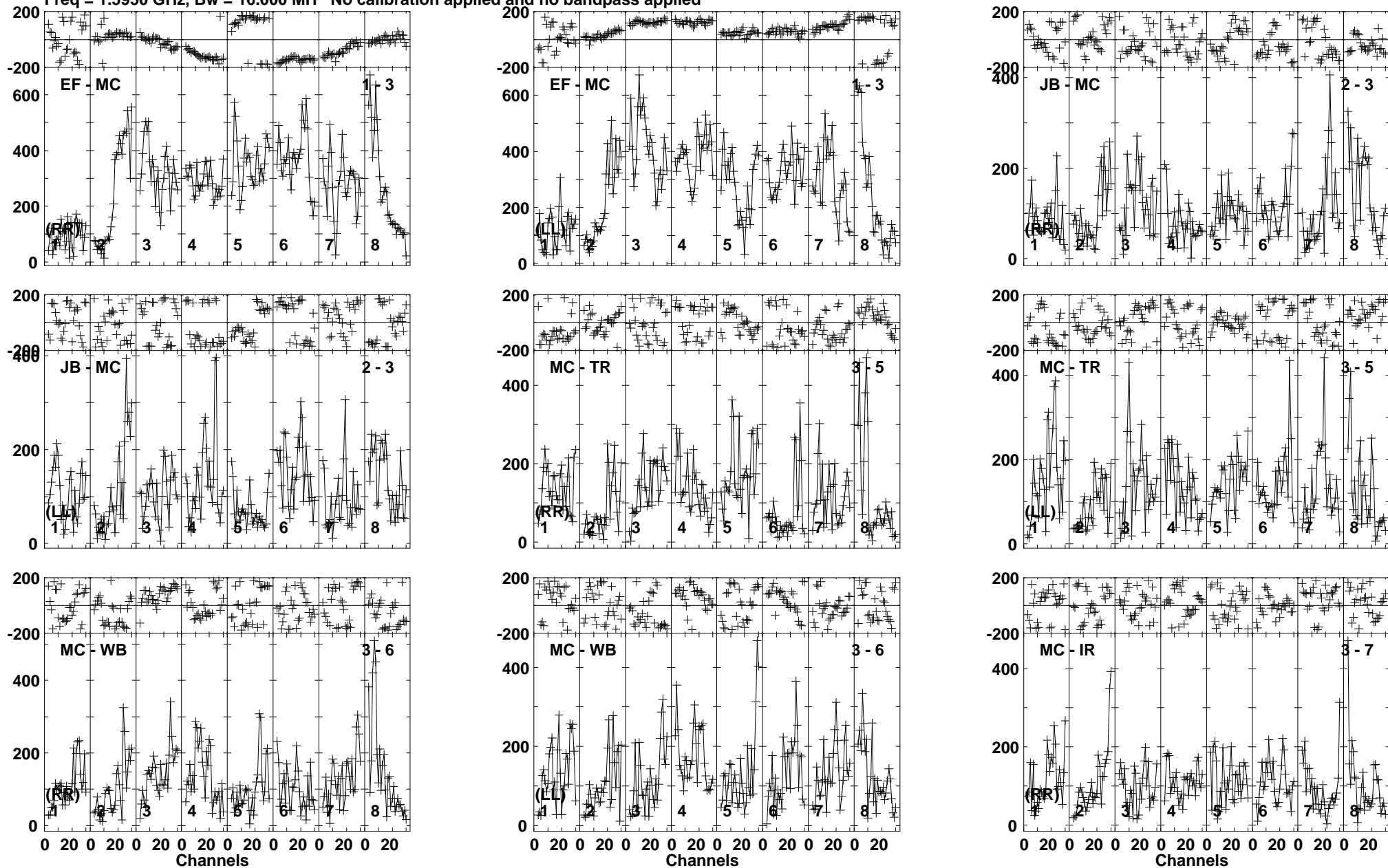
Lower frame: Micro Ampl Jy Top frame: Phas deg Vector averaged cross-power spectrum Baseline: EF (01) - MC (03) Timerange: 00/09:21:31 to 00/09:22:29
