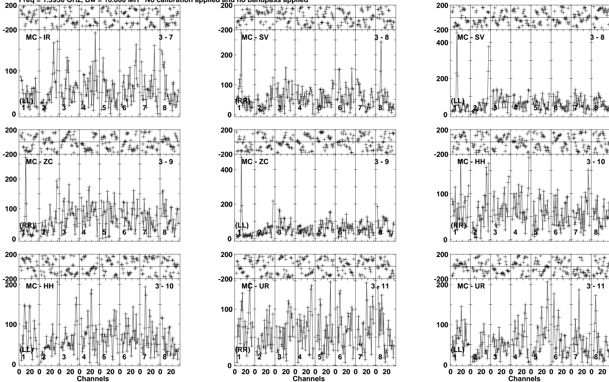
Lower frame: Micro Ampl Jy Top frame: Phas deg Vector averaged cross-power spectrum Baseline: MC (03) - IR (07) Timerange: 00/10/02:31 to 00/10/05:59
