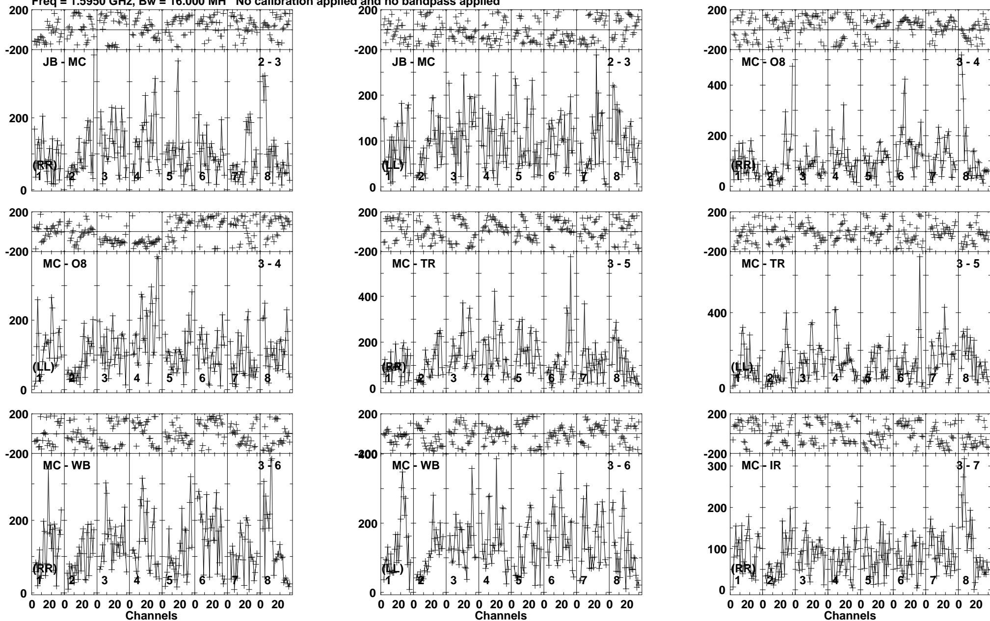
Lower frame: Micro Ampl Jy Top frame: Phas deg Vector averaged cross-power spectrum Baseline: JB (02) - MC (03) Timerange: 00/12:43:23 to 00/12:44:49
