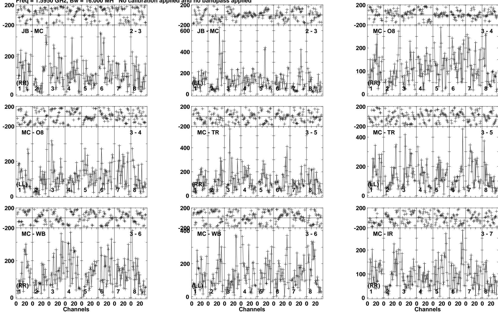
Lower frame: Micro Ampl Jy Top frame: Phas deg Vector averaged cross-power spectrum Baseline: JB (02) - MC (03) Timerange: 00/12:08:11 to 00/12:09:39
