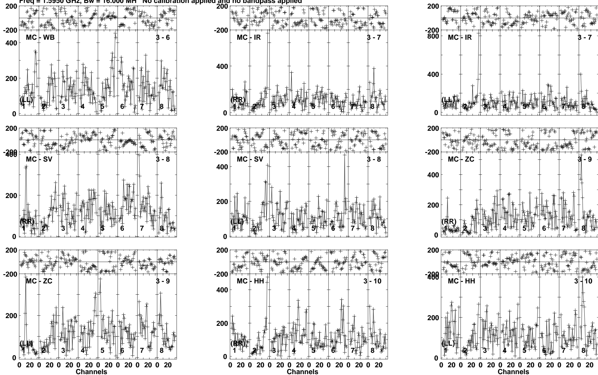
Lower frame: Micro Ampl Jy Top frame: Phas deg Vector averaged cross-power spectrum Baseline: MC (03) - WB (06) Timerange: 00/13:51:01 to 00/13:51:59
