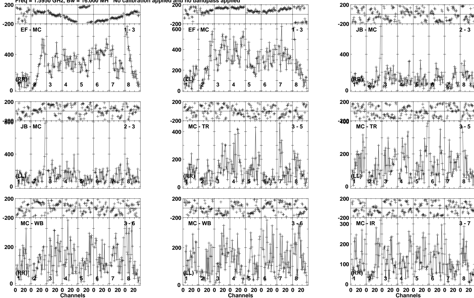
Lower frame: Micro Ampl Jy Top frame: Phas deg Vector averaged cross-power spectrum Baseline: EF (01) - MC (03) Timerange: 00/10:11:31 to 00/10:12:29
