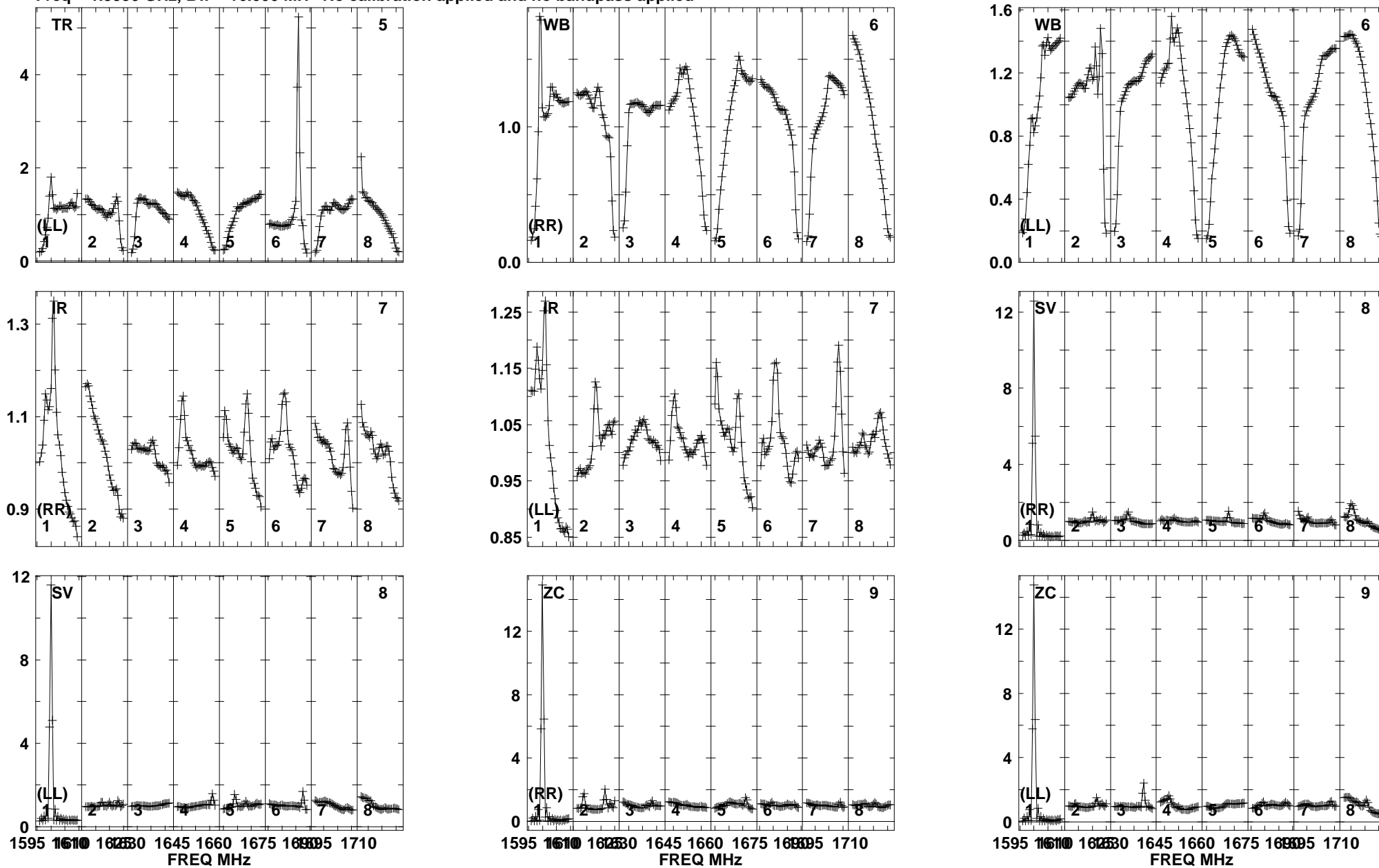
Lower frame: Real Jy Total-power spectrum Antenna: TR (05) Timerange: 01/04:39:01 to 01/04:39:59
