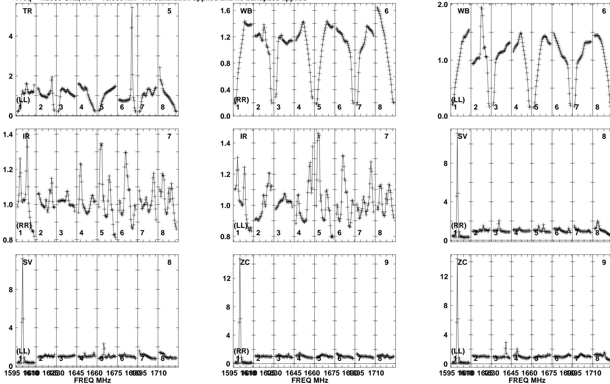
Lower frame: Real Jy Total-power spectrum Antenna: TR (05) Timerange: 00/22:25:03 to 00/22:28:29
