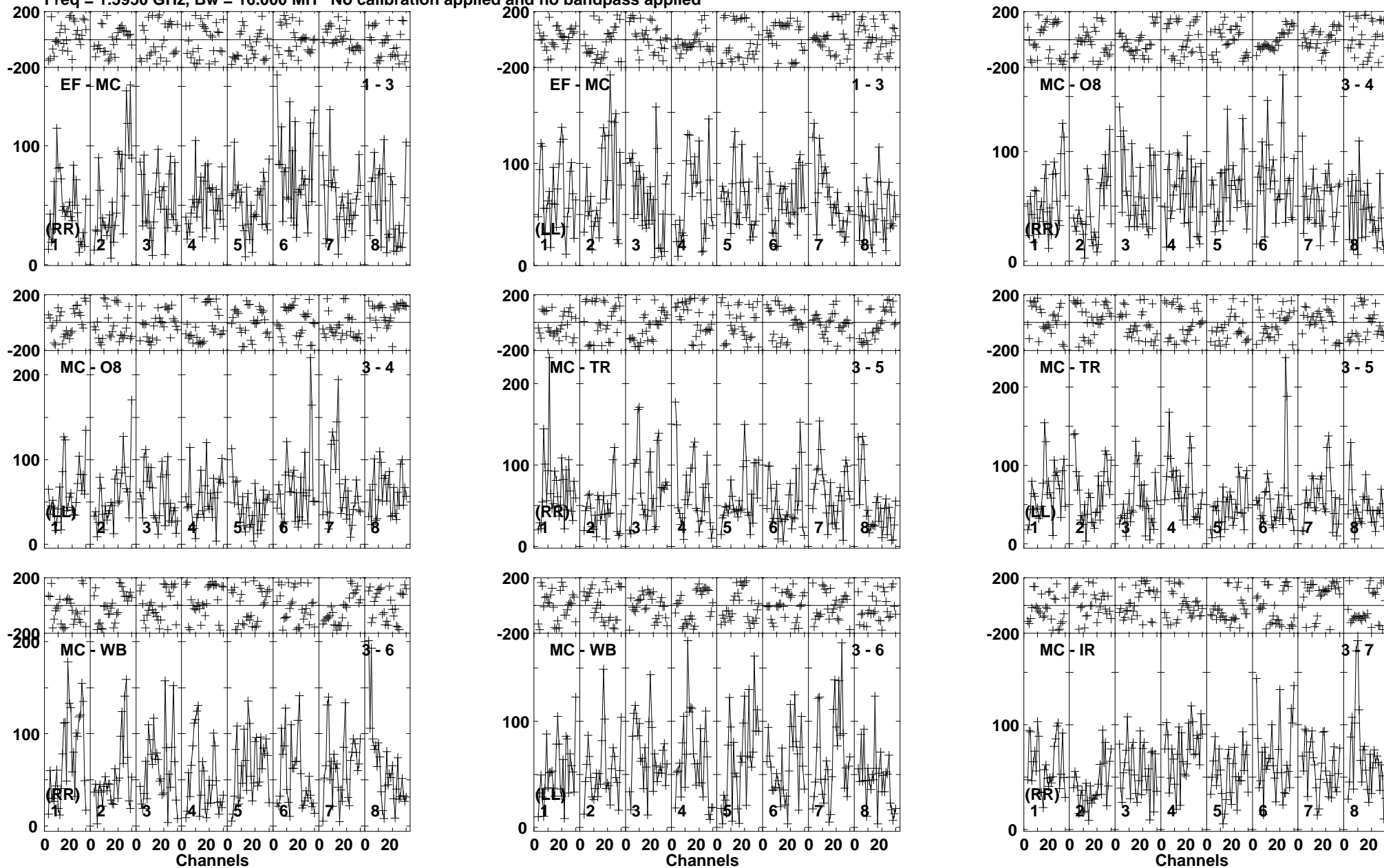
Lower frame: Micro Ampl Jy Top frame: Phas deg Vector averaged cross-power spectrum Baseline: EF (01) - MC (03) Timerange: 00/21:05:03 to 00/21:08:29
