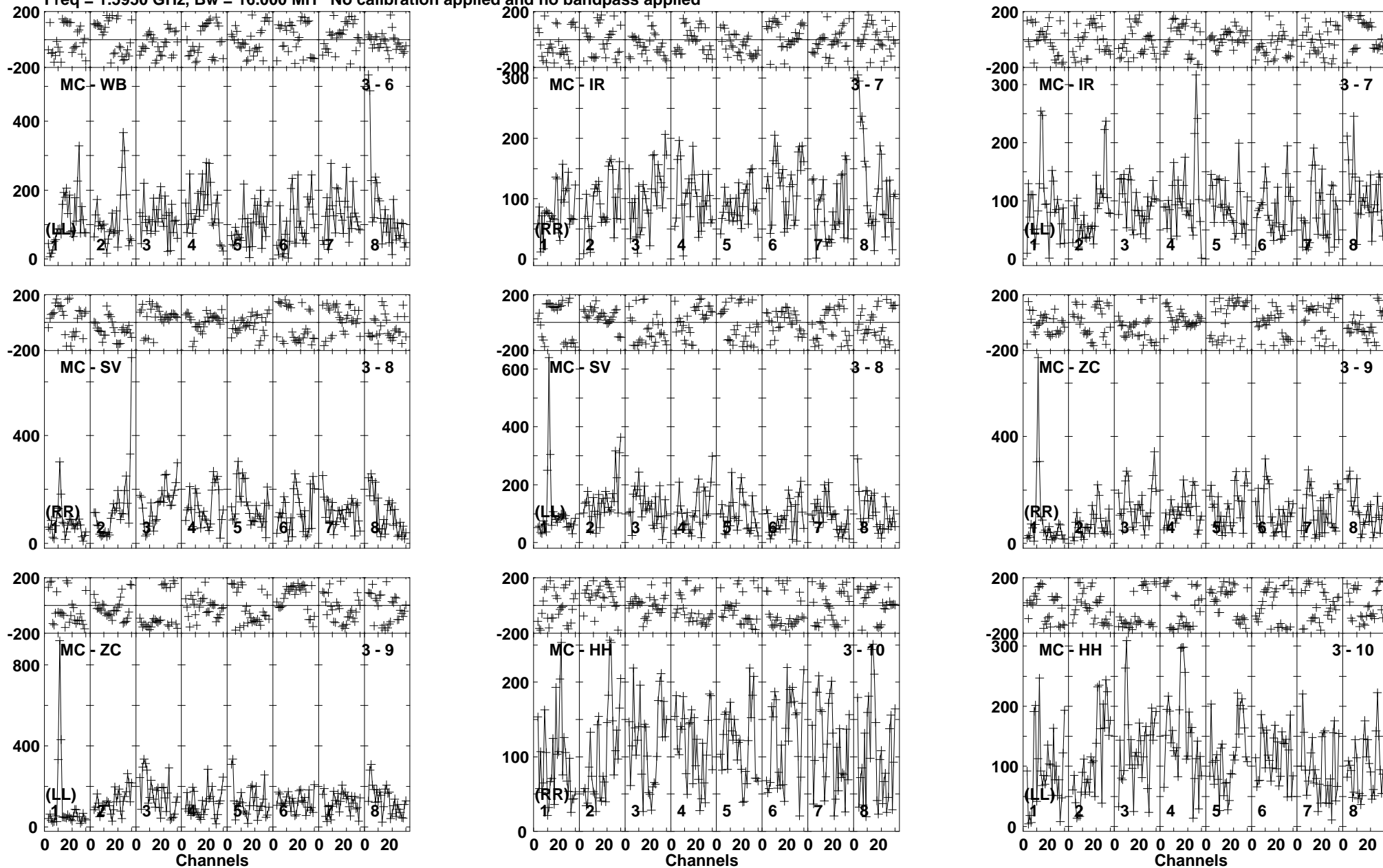
Lower frame: Micro Ampl Jy Top frame: Phas deg Vector averaged cross-power spectrum Baseline: MC (03) - WB (06) Timerange: 01/00:53:31 to 01/00:54:59
