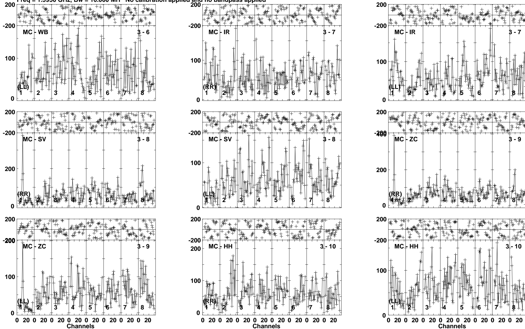
Lower frame: Micro Ampl Jy Top frame: Phas deg Vector averaged cross-power spectrum Baseline: MC (03) - WB (06) Timerange: 00/23:40:01 to 00/23:43:29
