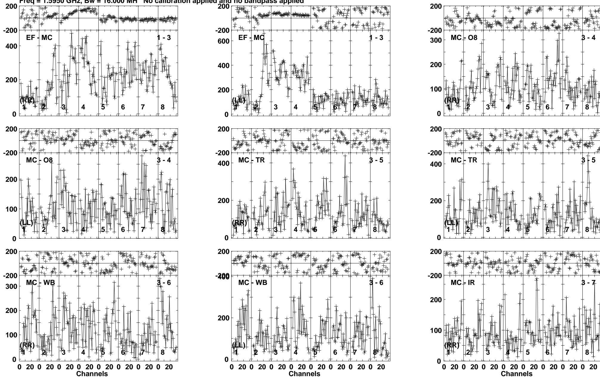
Lower frame: Micro Ampl Jy Top frame: Phas deg Vector averaged cross-power spectrum Baseline: EF (01) - MC (03) Timerange: 00/21:43:33 to 00/21:44:59
