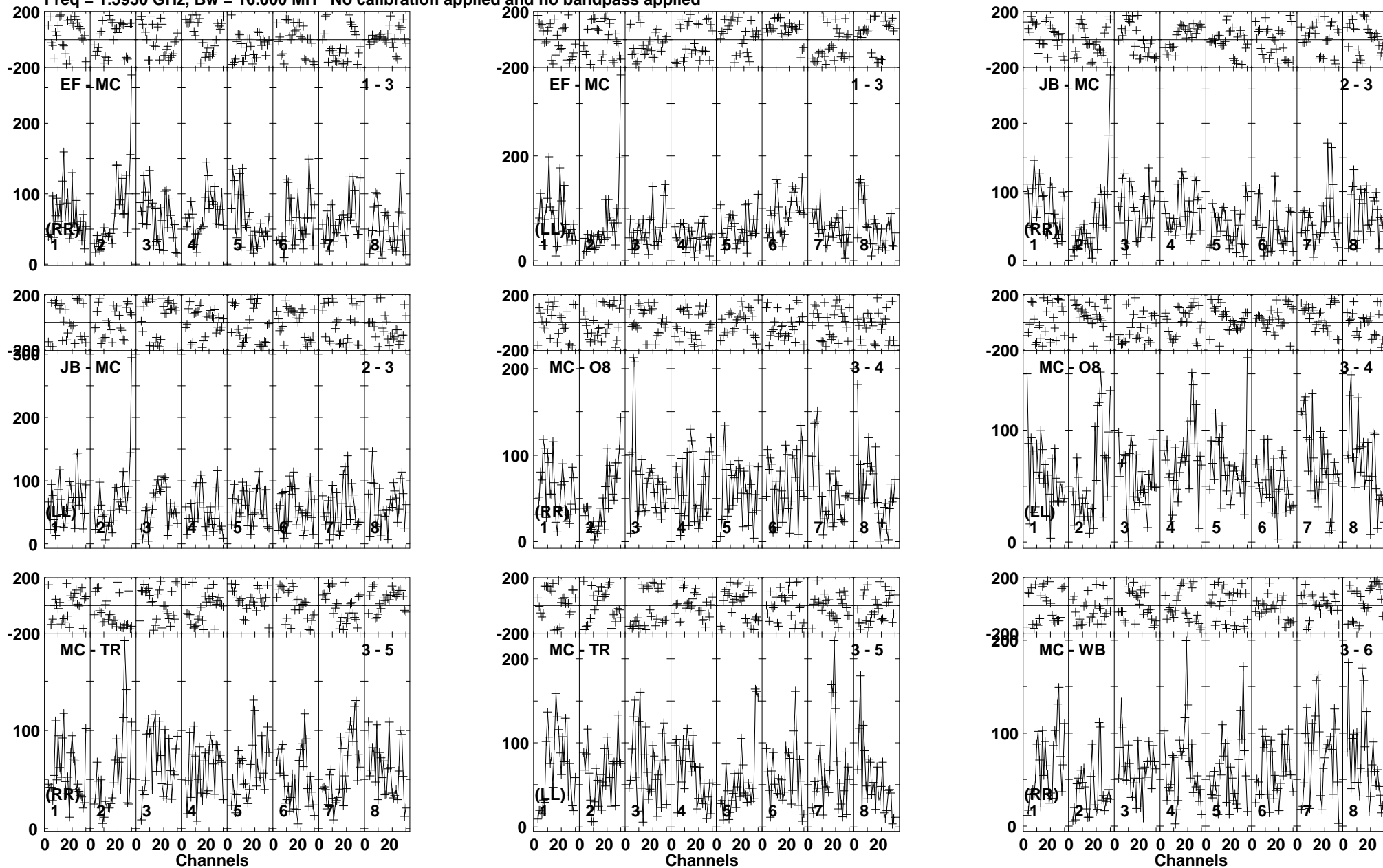
Lower frame: Micro Ampl Jy Top frame: Phas deg Vector averaged cross-power spectrum Baseline: EF (01) - MC (03) Timerange: 01/07:31:03 to 01/07:34:29
