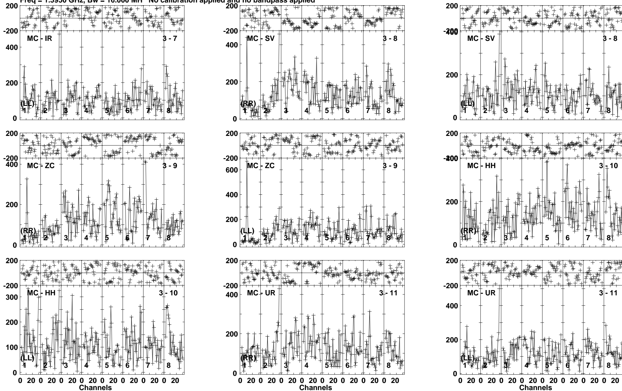
Lower frame: Micro Ampl Jy Top frame: Phas deg Vector averaged cross-power spectrum Baseline: MC (03) - IR (07) Timerange: 00/21:24:01 to 00/21:24:59
