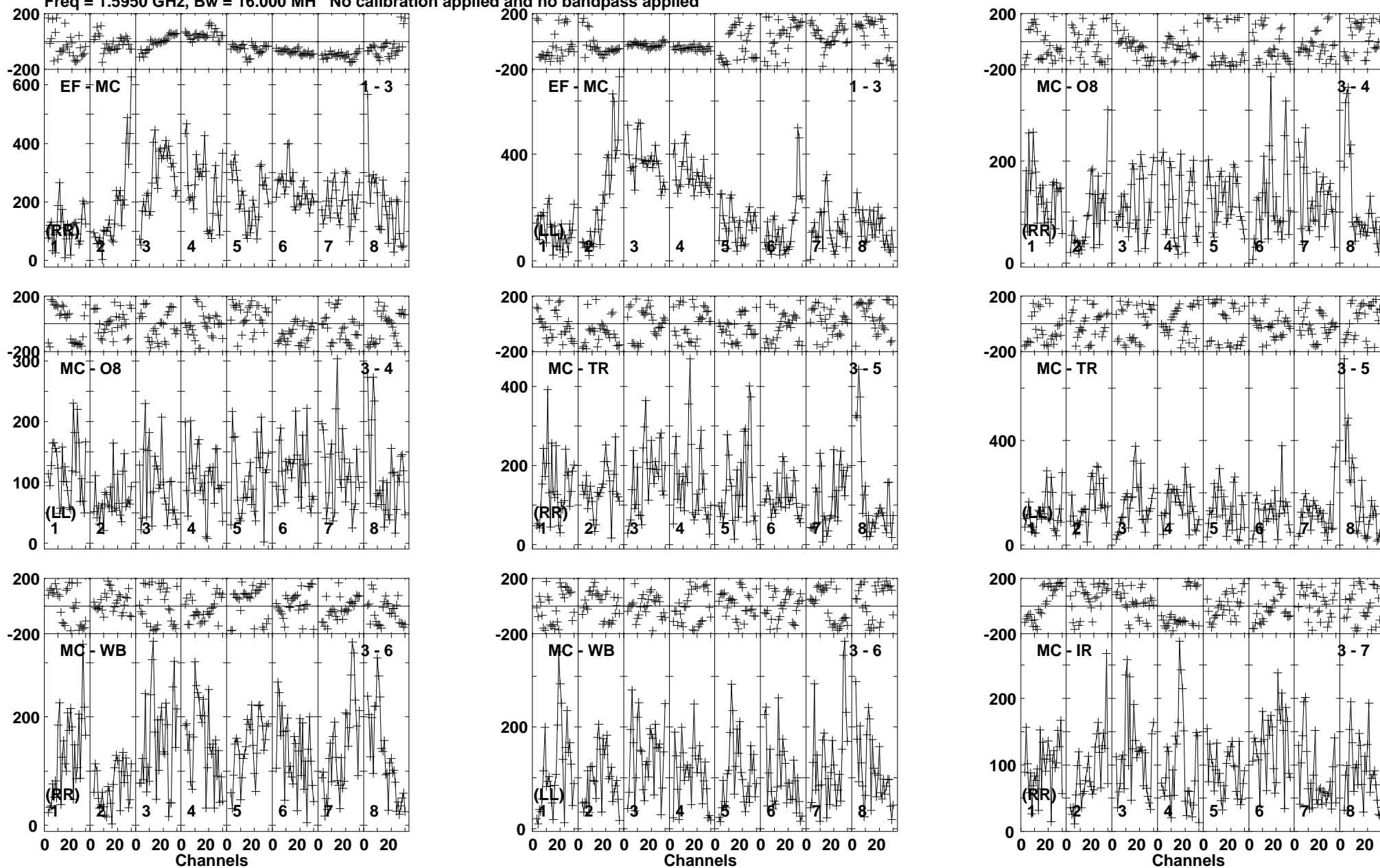
Lower frame: Micro Ampl Jy Top frame: Phas deg Vector averaged cross-power spectrum Baseline: EF (01) - MC (03) Timerange: 01/07:24:33 to 01/07:25:59
