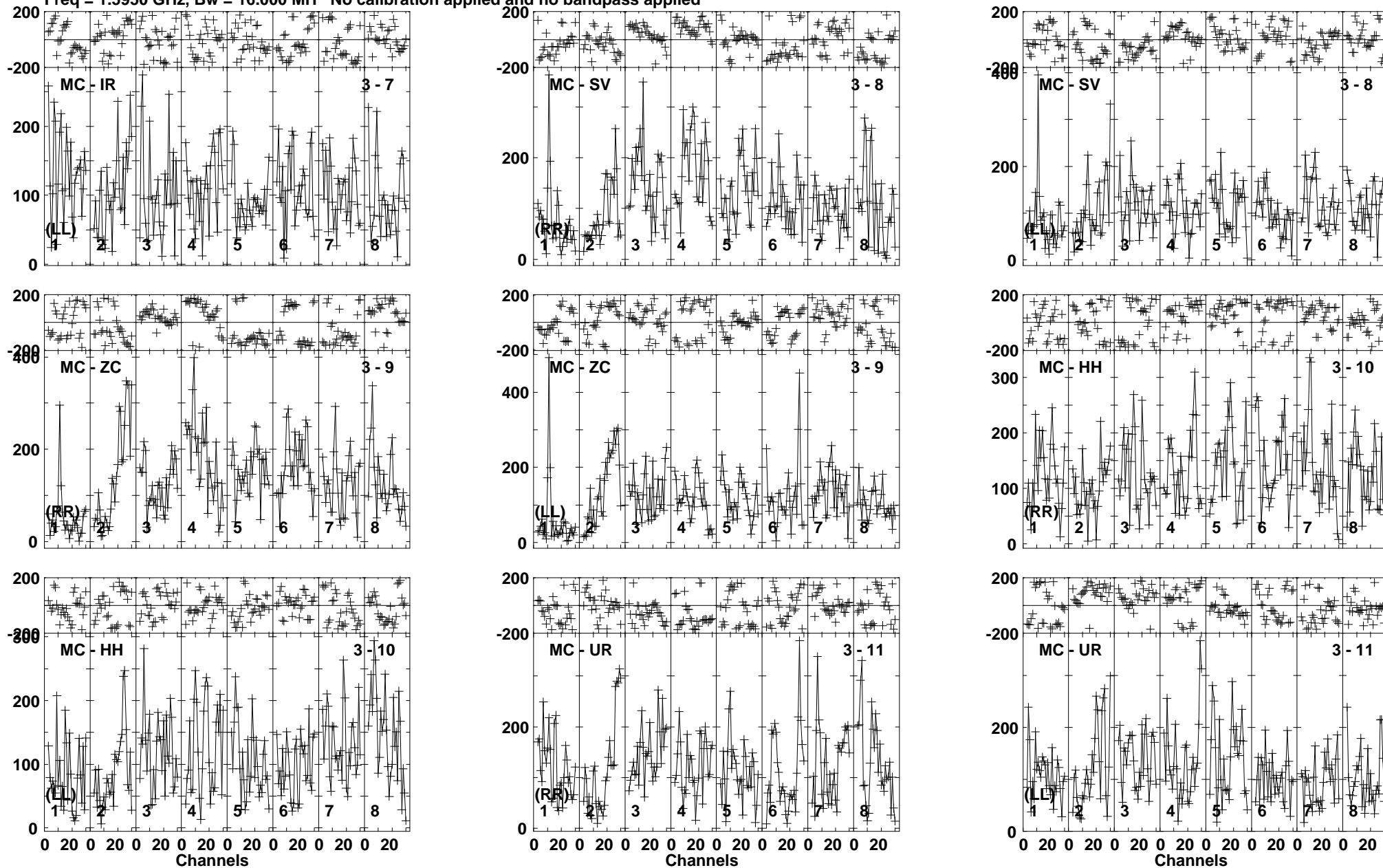
Lower frame: Micro Ampl Jy Top frame: Phas deg Vector averaged cross-power spectrum Baseline: MC (03) - IR (07) Timerange: 00/22:54:01 to 00/22:54:59
