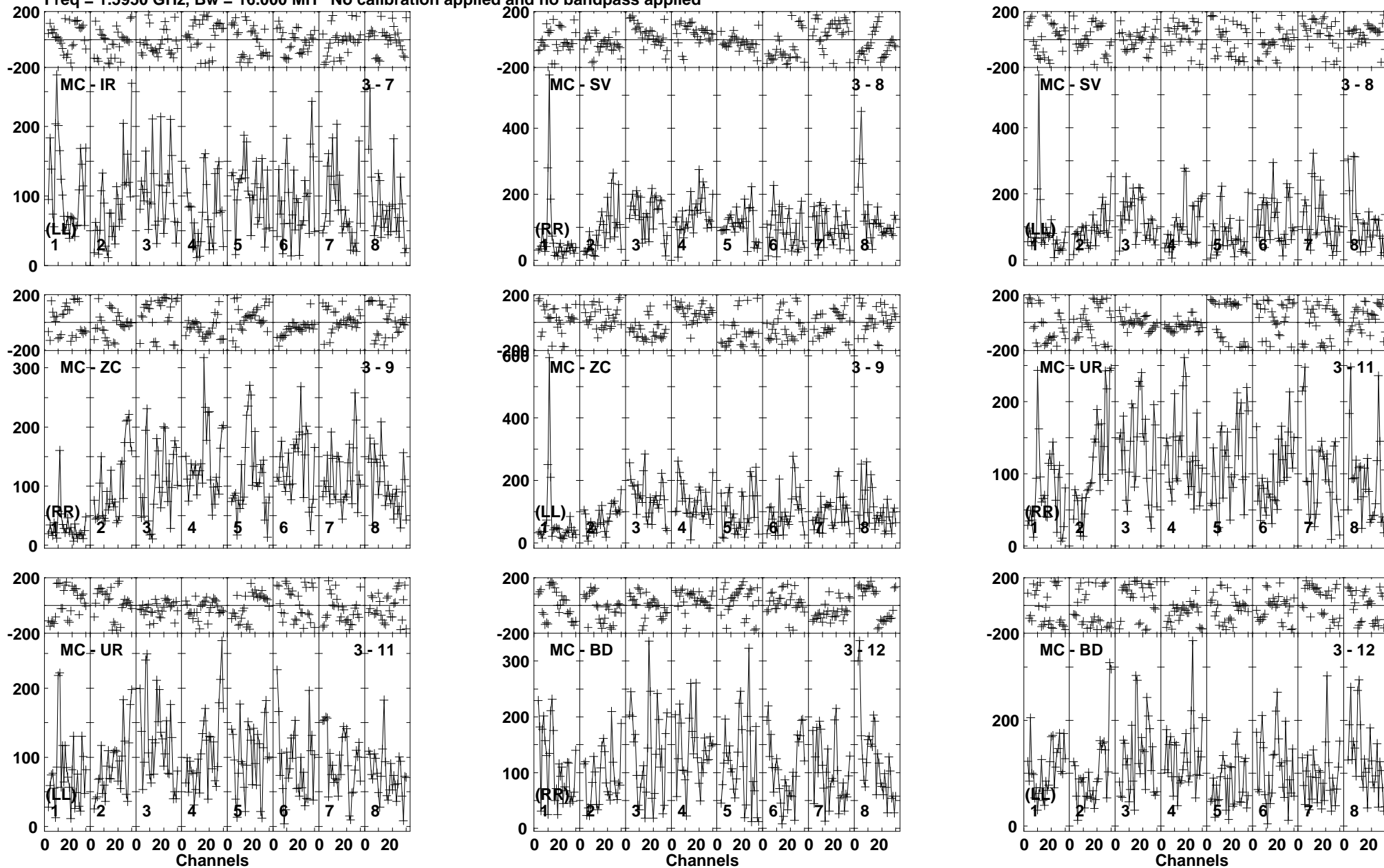
Lower frame: Micro Ampl Jy Top frame: Phas deg Vector averaged cross-power spectrum Baseline: MC (03) - IR (07) Timerange: 00/20:26:01 to 00/20:27:29
