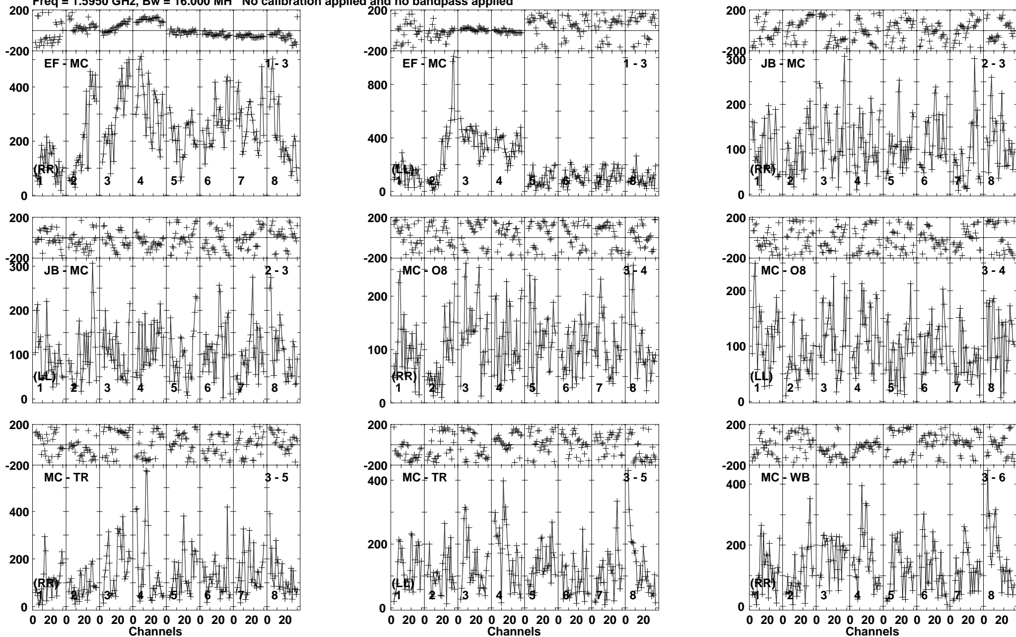
Lower frame: Micro Ampl Jy Top frame: Phas deg Vector averaged cross-power spectrum Baseline: EF (01) - MC (03) Timerange: 01/03:43:11 to 01/03:44:39
