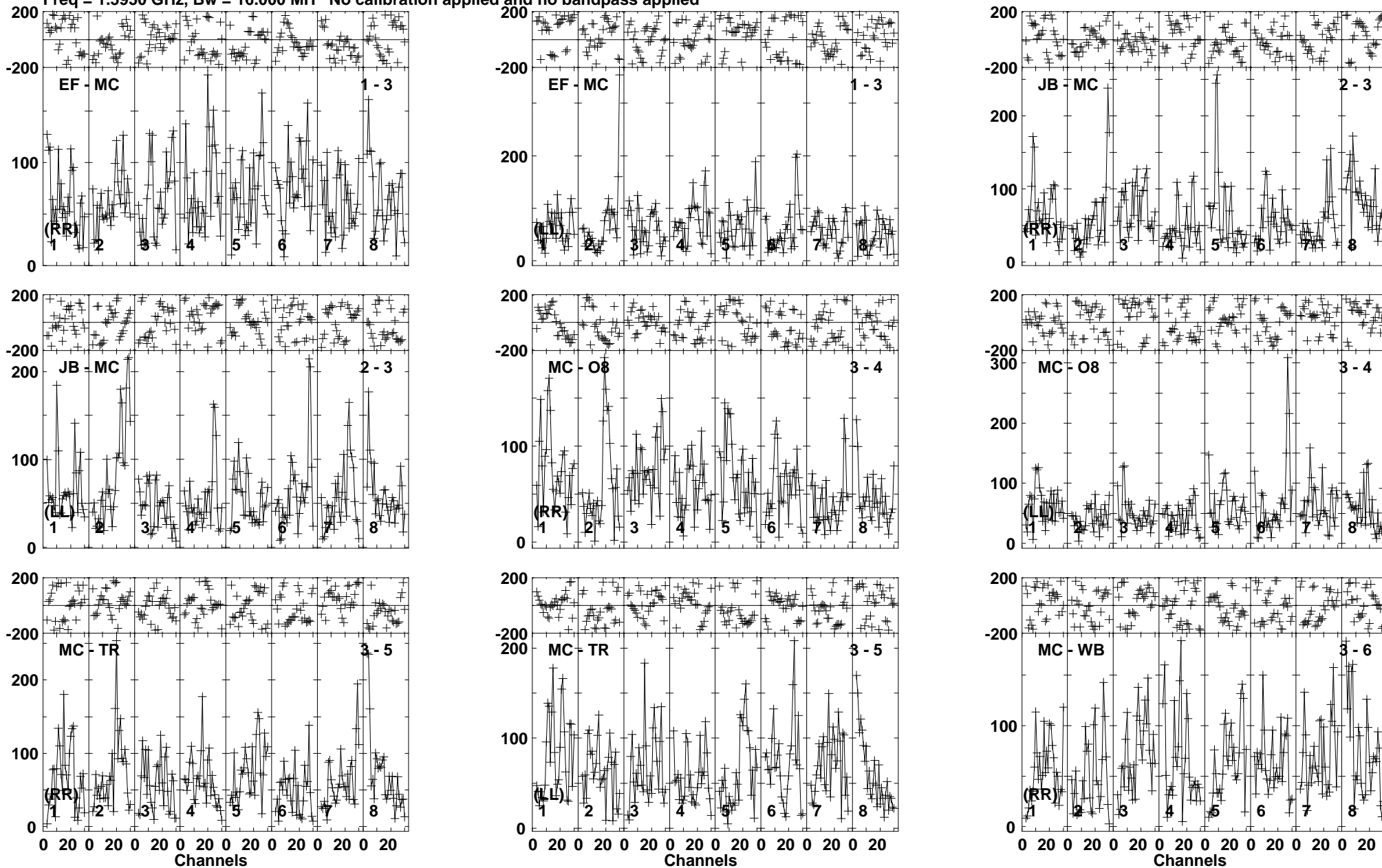
Lower frame: Micro Ampl Jy Top frame: Phas deg Vector averaged cross-power spectrum Baseline: EF (01) - MC (03) Timerange: 01/00:35:03 to 01/00:38:29
