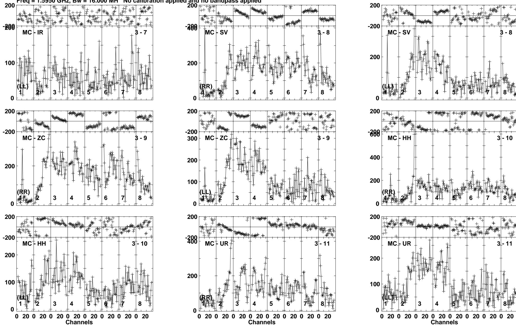
Lower frame: Micro Ampl Jy Top frame: Phas deg Vector averaged cross-power spectrum Baseline: MC (03) - IR (07) Timerange: 00:22:15:31 to 00:22:18:29
