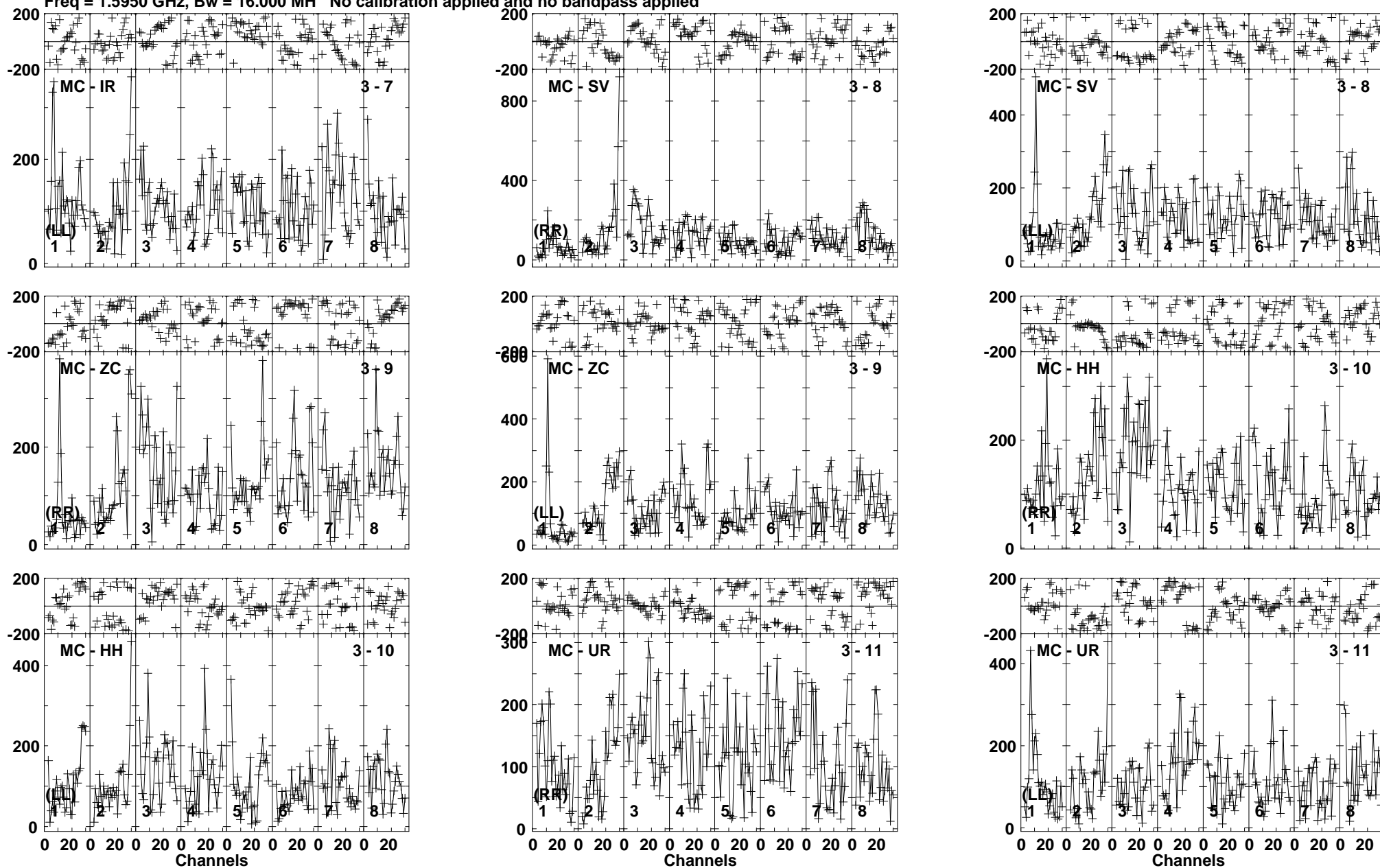
Lower frame: Micro Ampl Jy Top frame: Phas deg Vector averaged cross-power spectrum Baseline: MC (03) - IR (07) Timerange: 00/23:19:01 to 00/23:19:59
