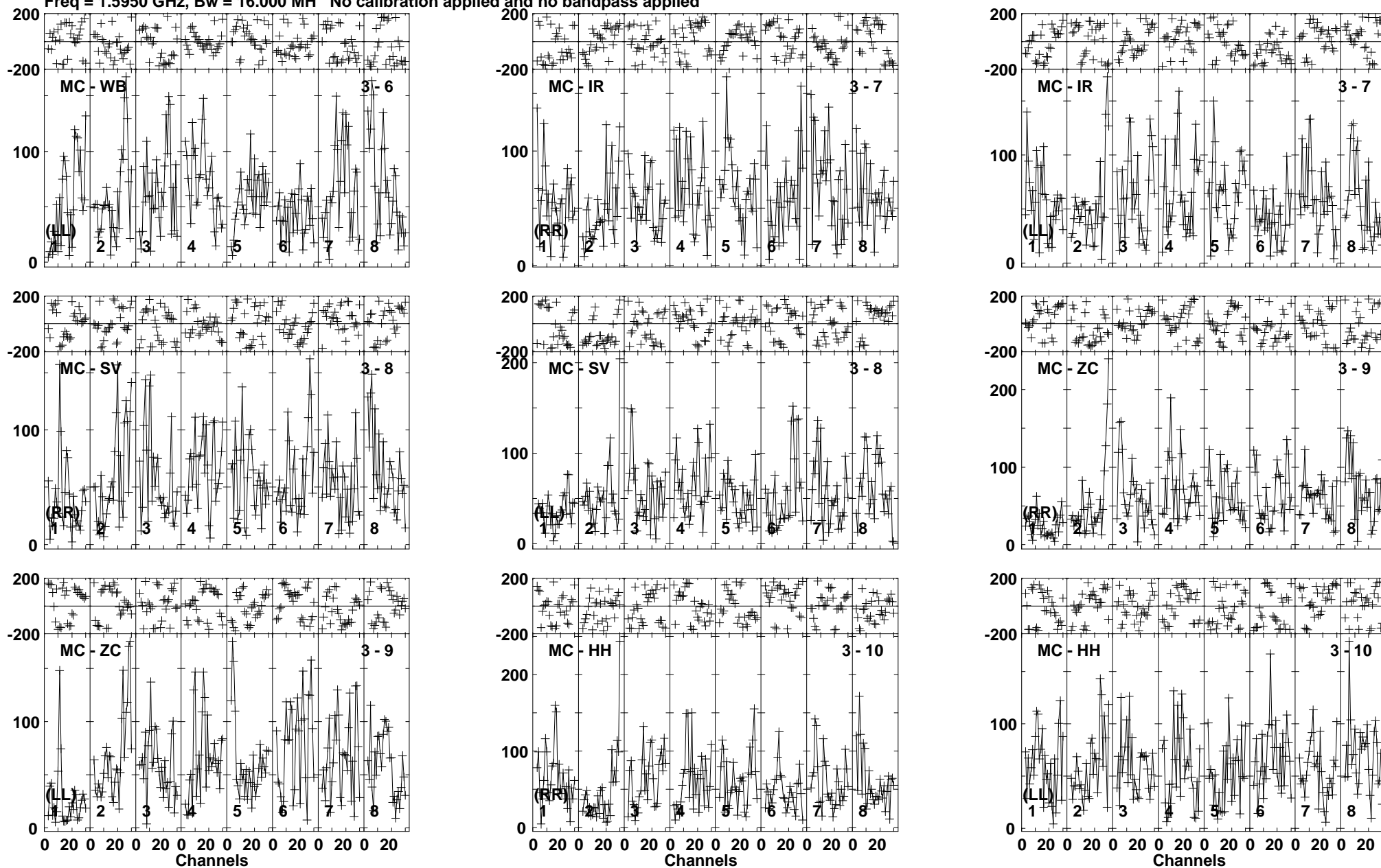
Lower frame: Micro Ampl Jy Top frame: Phas deg Vector averaged cross-power spectrum Baseline: MC (03) - WB (06) Timerange: 01/00:05:03 to 01/00:08:29
