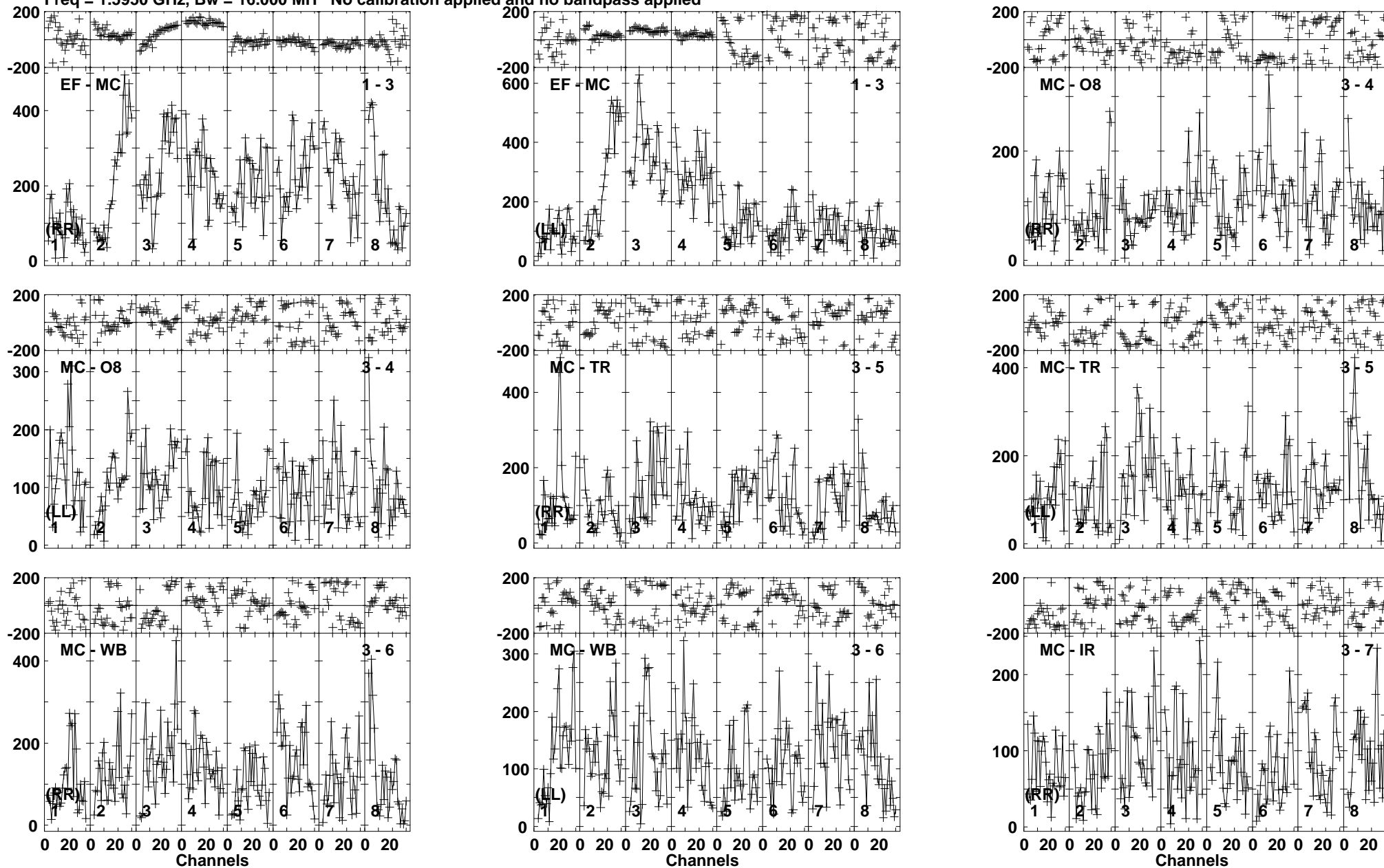
Lower frame: Micro Ampl Jy Top frame: Phas deg Vector averaged cross-power spectrum Baseline: EF (01) - MC (03) Timerange: 00/21:33:31 to 00/21:34:59
