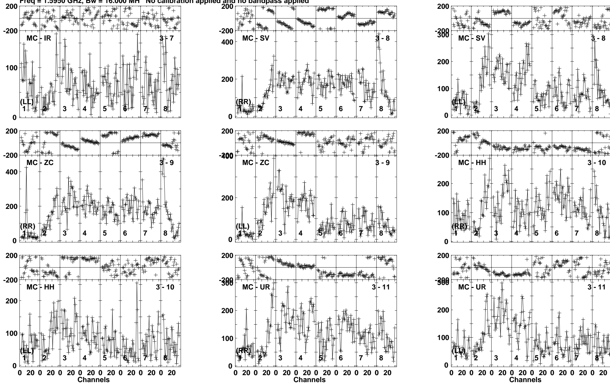
Lower frame: Micro Ampl Jy Top frame: Phas deg Vector averaged cross-power spectrum Baseline: MC (03) - IR (07) Timerange: 00/21:25:31 to 00/21:28:29
