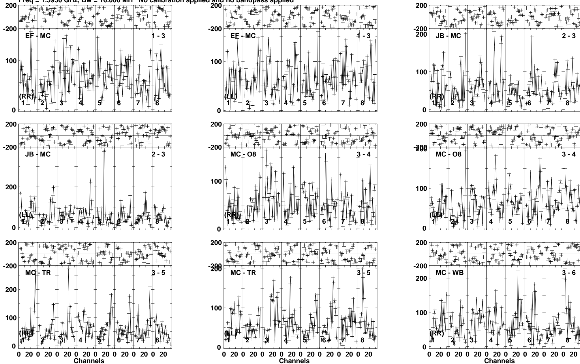
Lower frame: Micro Ampl Jy Top frame: Phas deg Vector averaged cross-power spectrum Baseline: EF (01) - MC (03) Timerange: 01/00:25:03 to 01/00:28:29
