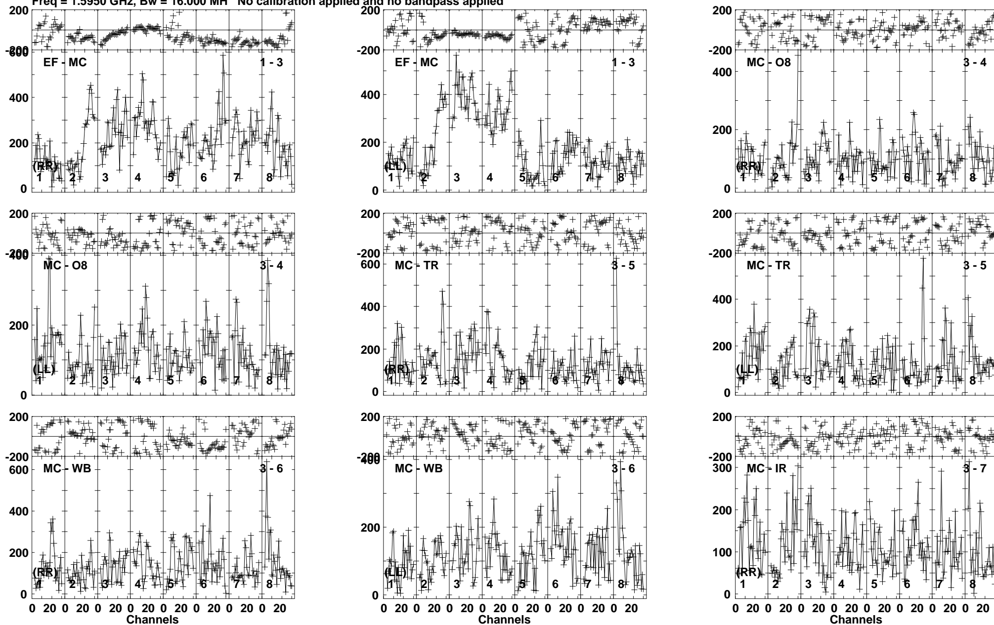
Lower frame: Micro Ampl Jy Top frame: Phas deg Vector averaged cross-power spectrum Baseline: EF (01) - MC (03) Timerange: 00/21:14:01 to 00/21:14:59
