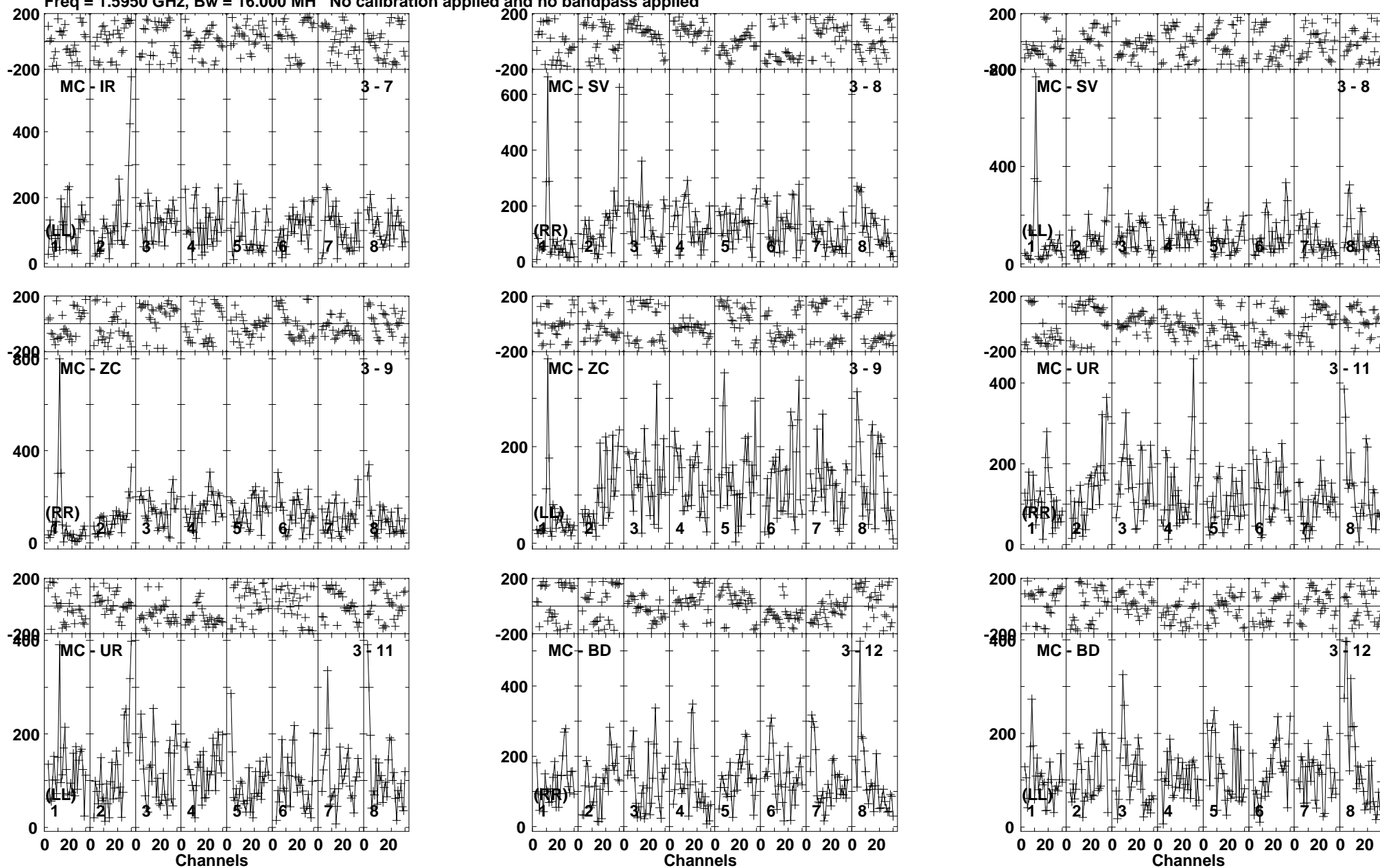
Lower frame: Micro Ampl Jy Top frame: Phas deg Vector averaged cross-power spectrum Baseline: MC (03) - IR (07) Timerange: 00/20:59:01 to 00/20:59:59
