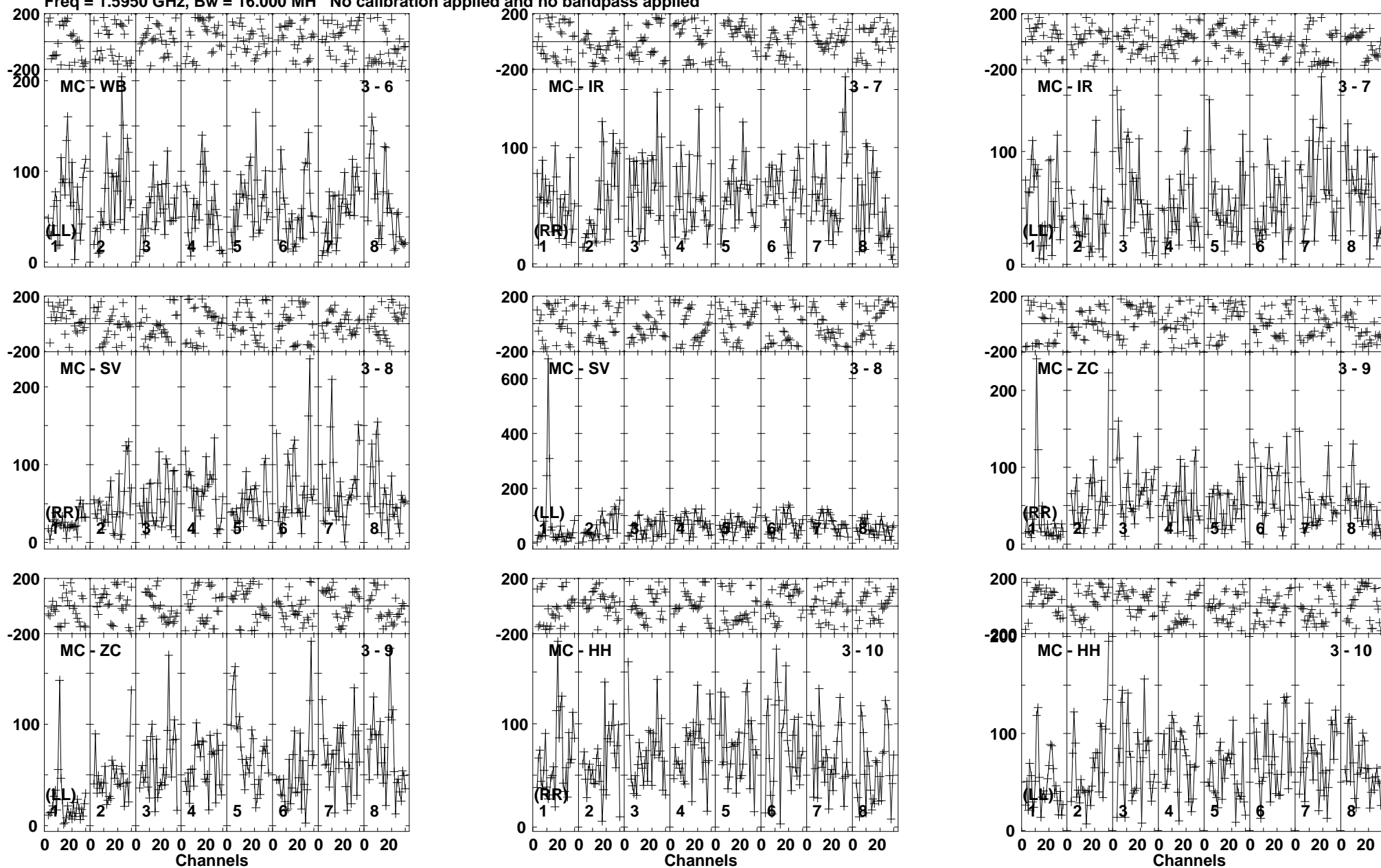
Lower frame: Micro Ampl Jy Top frame: Phas deg Vector averaged cross-power spectrum Baseline: MC (03) - WB (06) Timerange: 01/01:27:01 to 01/01:30:29
