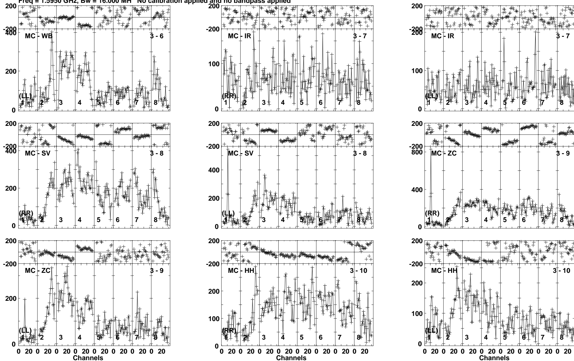
Lower frame: Micro Ampl Jy Top frame: Phas deg Vector averaged cross-power spectrum Baseline: MC (03) - WB (06) Timerange: 01/00:20:31 to 01/00:23:29
