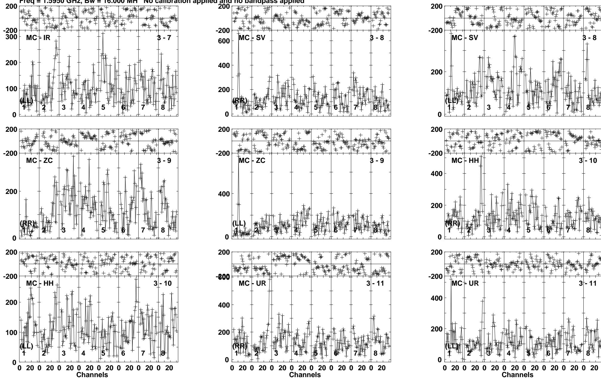
Lower frame: Micro Ampl Jy Top frame: Phas deg Vector averaged cross-power spectrum Baseline: MC (03) - IR (07) Timerange: 00/21:39:01 to 00/21:39:59
