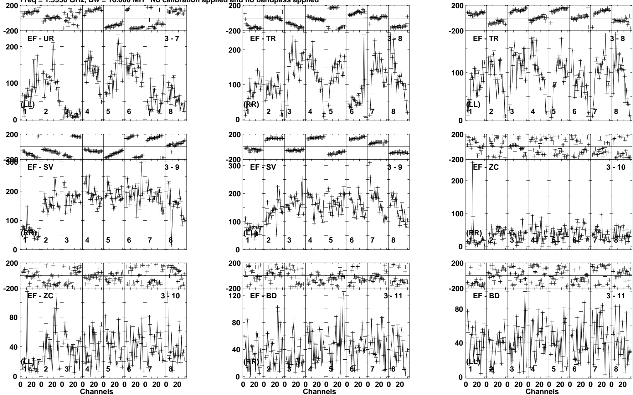
Lower frame: Micro Ampl Jy Top frame: Phas deg Vector averaged cross-power spectrum Baseline: EF (03) - UR (07) Timerange: 01/00:26:01 to 01/00:39:59
