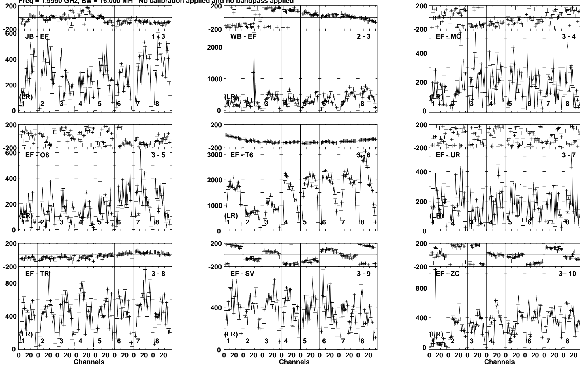
Lower frame: Micro Ampl Jy Top frame: Phas deg Vector averaged cross-power spectrum Baseline: JB (01) - EF (03) Timerange: 00/20:25:01 to 00/20:26:09
