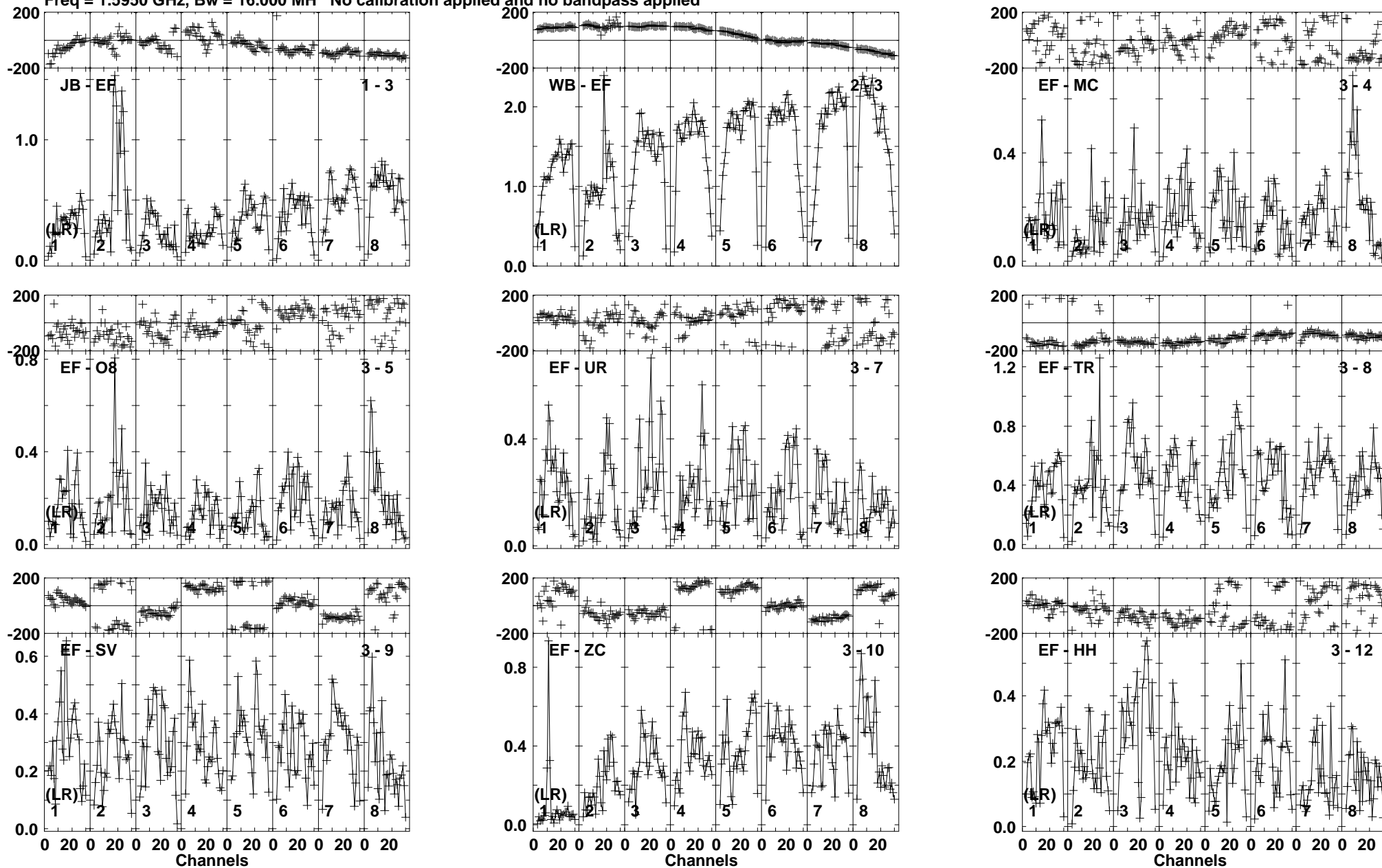
Lower frame: Milli Ampl Jy Top frame: Phas deg Vector averaged cross-power spectrum Baseline: JB (01) - EF (03) Timerange: 00/21:51:01 to 00/21:52:09
