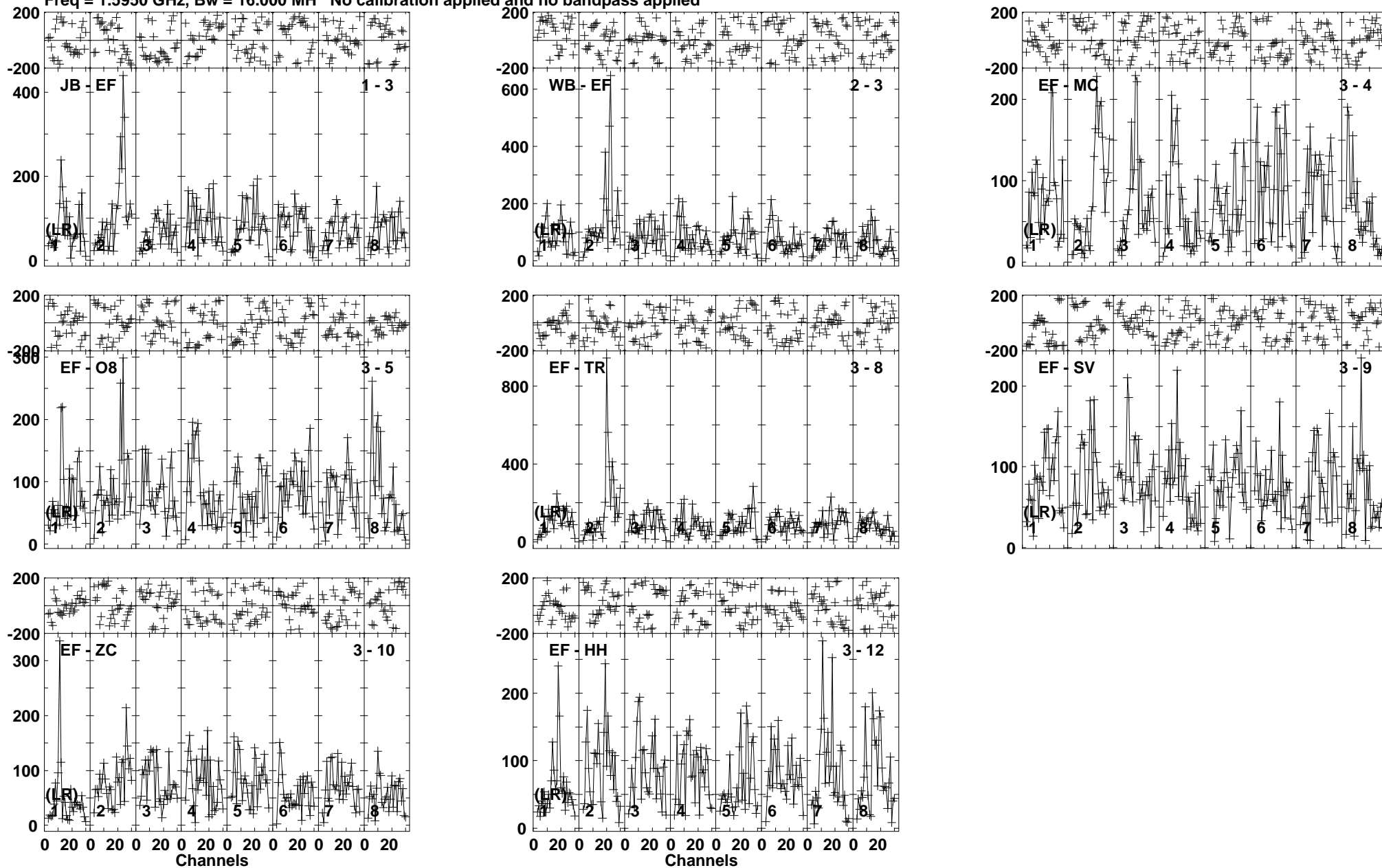
Lower frame: Micro Ampl Jy Top frame: Phas deg Vector averaged cross-power spectrum Baseline: JB (01) - EF (03) Timerange: 01/00:57:41 to 01/01:01:29
