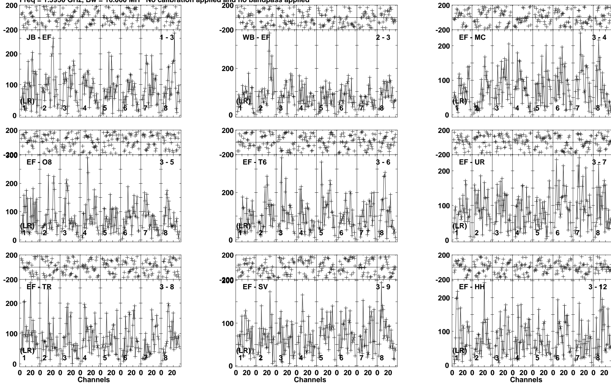
Lower frame: Micro Ampl Jy Top frame: Phas deg Vector averaged cross-power spectrum Baseline: JB (01) - EF (03) Timerange: 00/19:44:11 to 00/19:47:59
