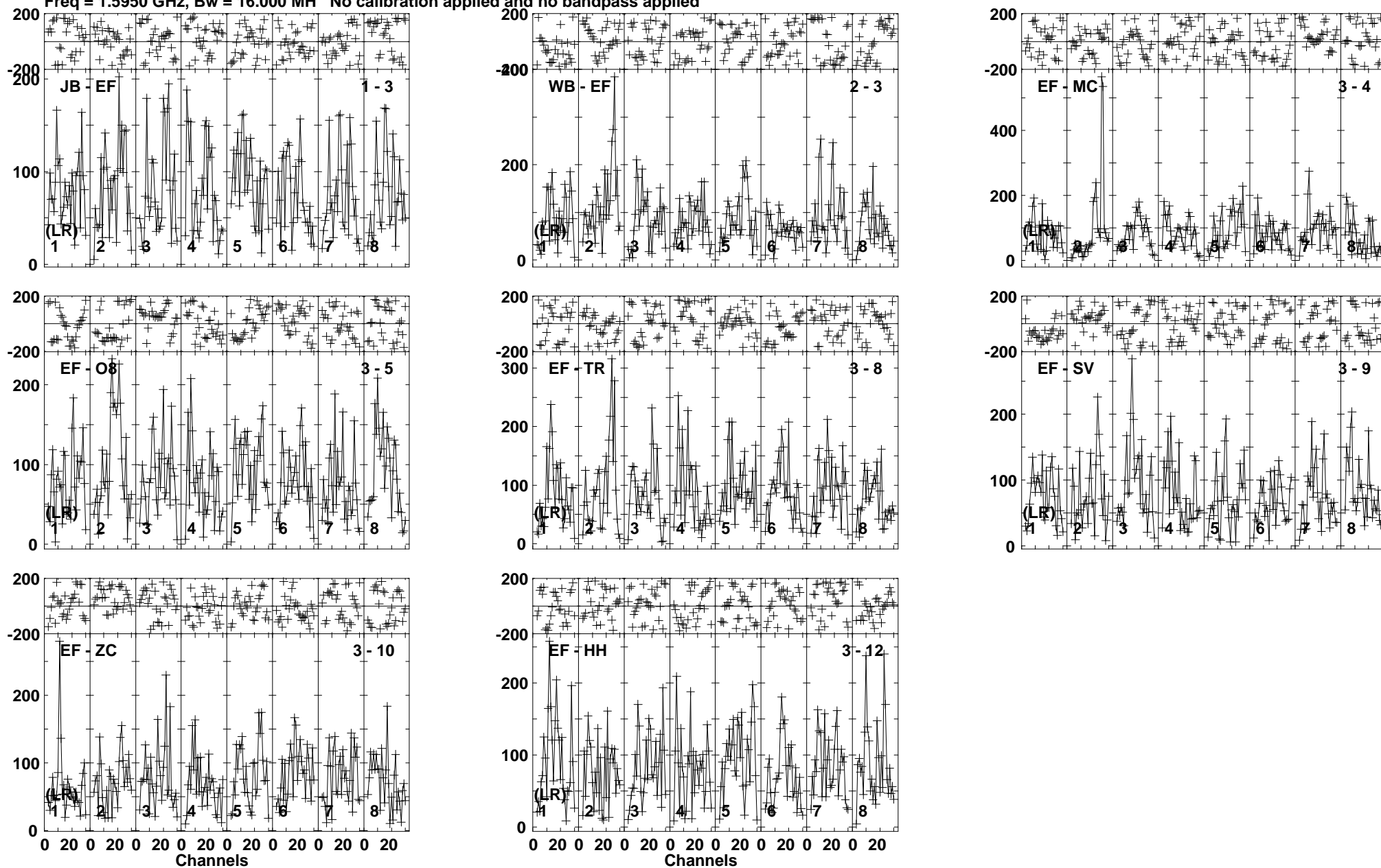
Lower frame: Micro Ampl Jy Top frame: Phas deg Vector averaged cross-power spectrum Baseline: JB (01) - EF (03) Timerange: 00/23:10:41 to 00/23:14:29
