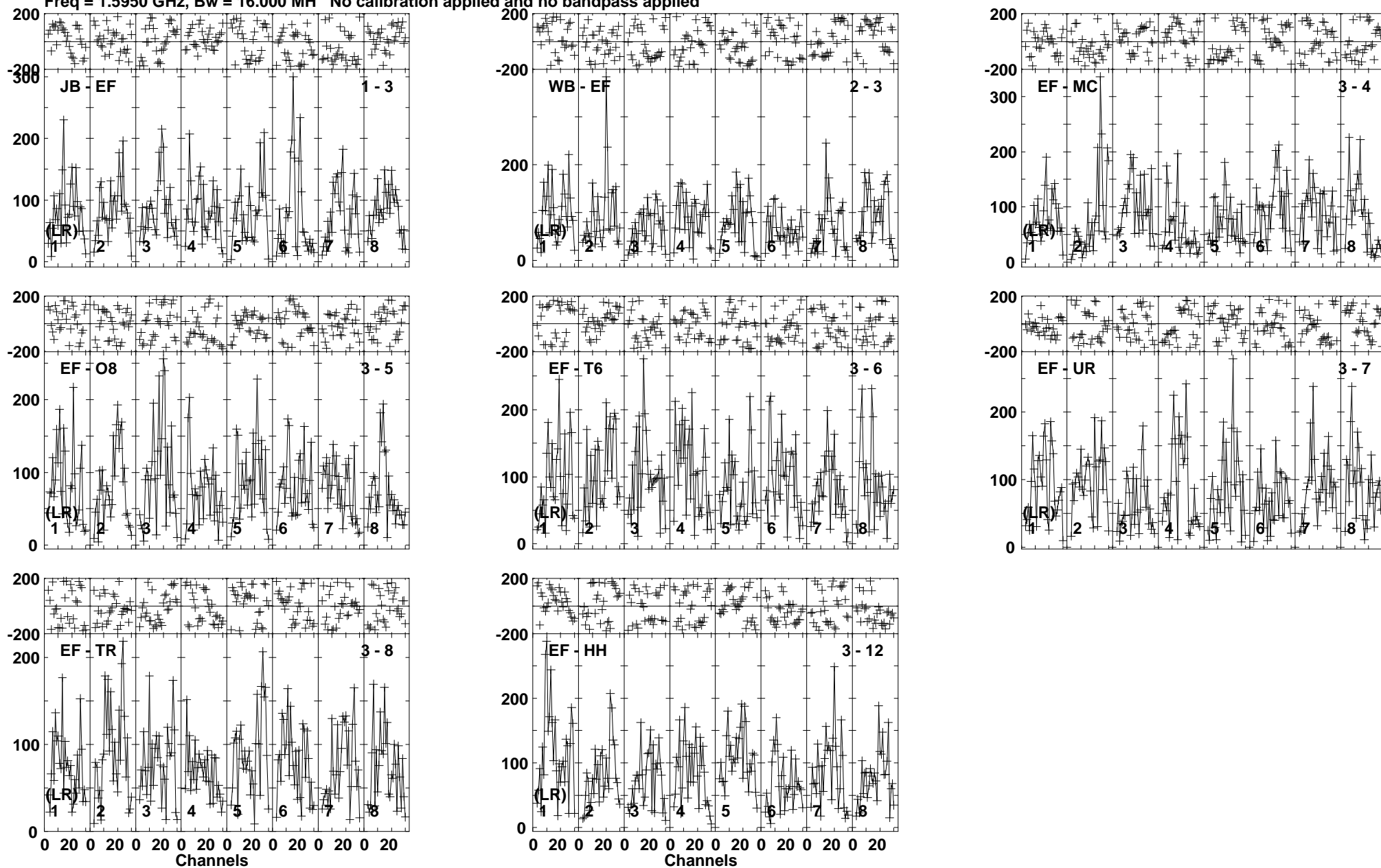
Lower frame: Micro Ampl Jy Top frame: Phas deg Vector averaged cross-power spectrum Baseline: JB (01) - EF (03) Timerange: 00/19:33:41 to 00/19:37:29
