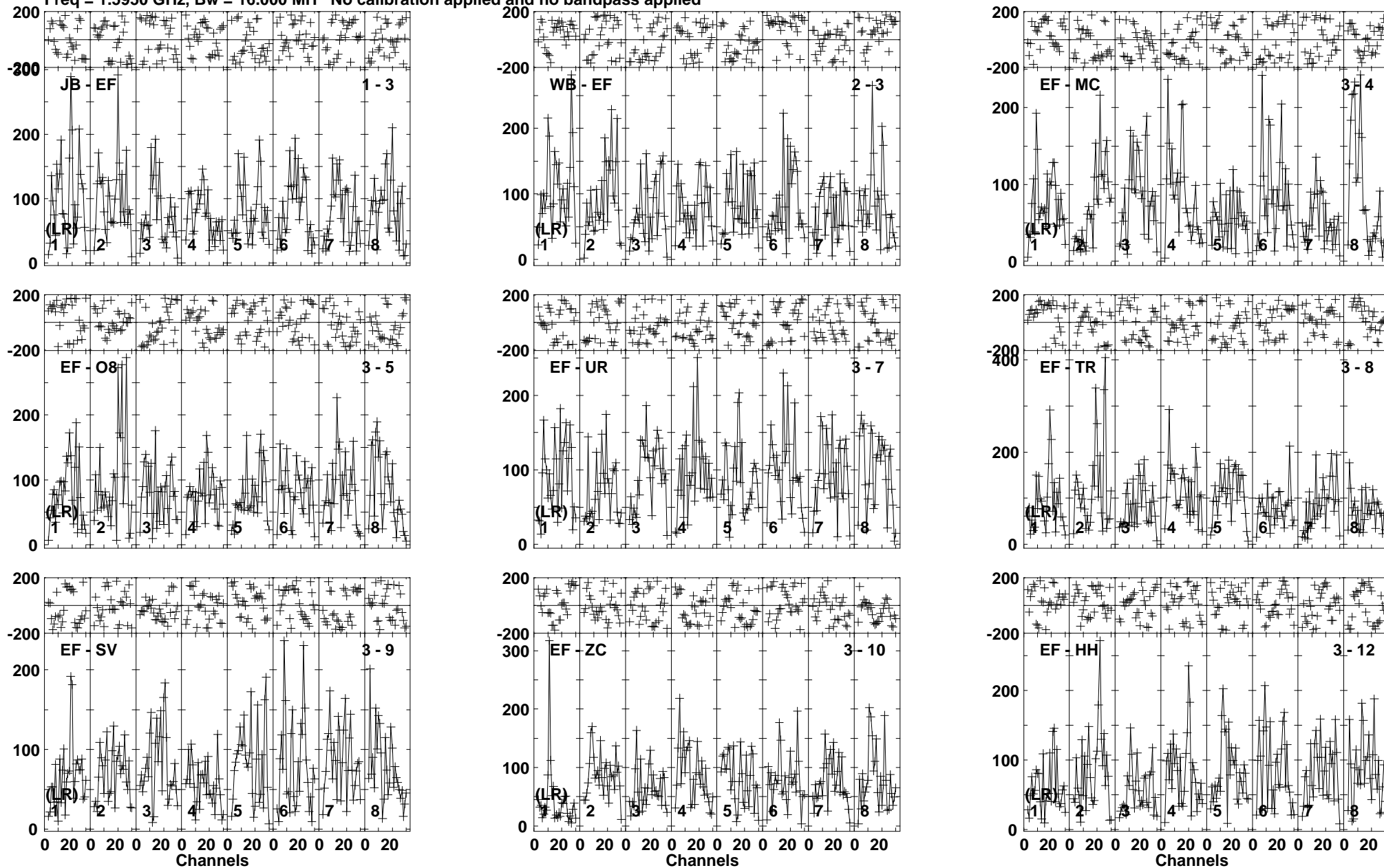
Lower frame: Micro Ampl Jy Top frame: Phas deg Vector averaged cross-power spectrum Baseline: JB (01) - EF (03) Timerange: 00/22:23:41 to 00/22:27:29
