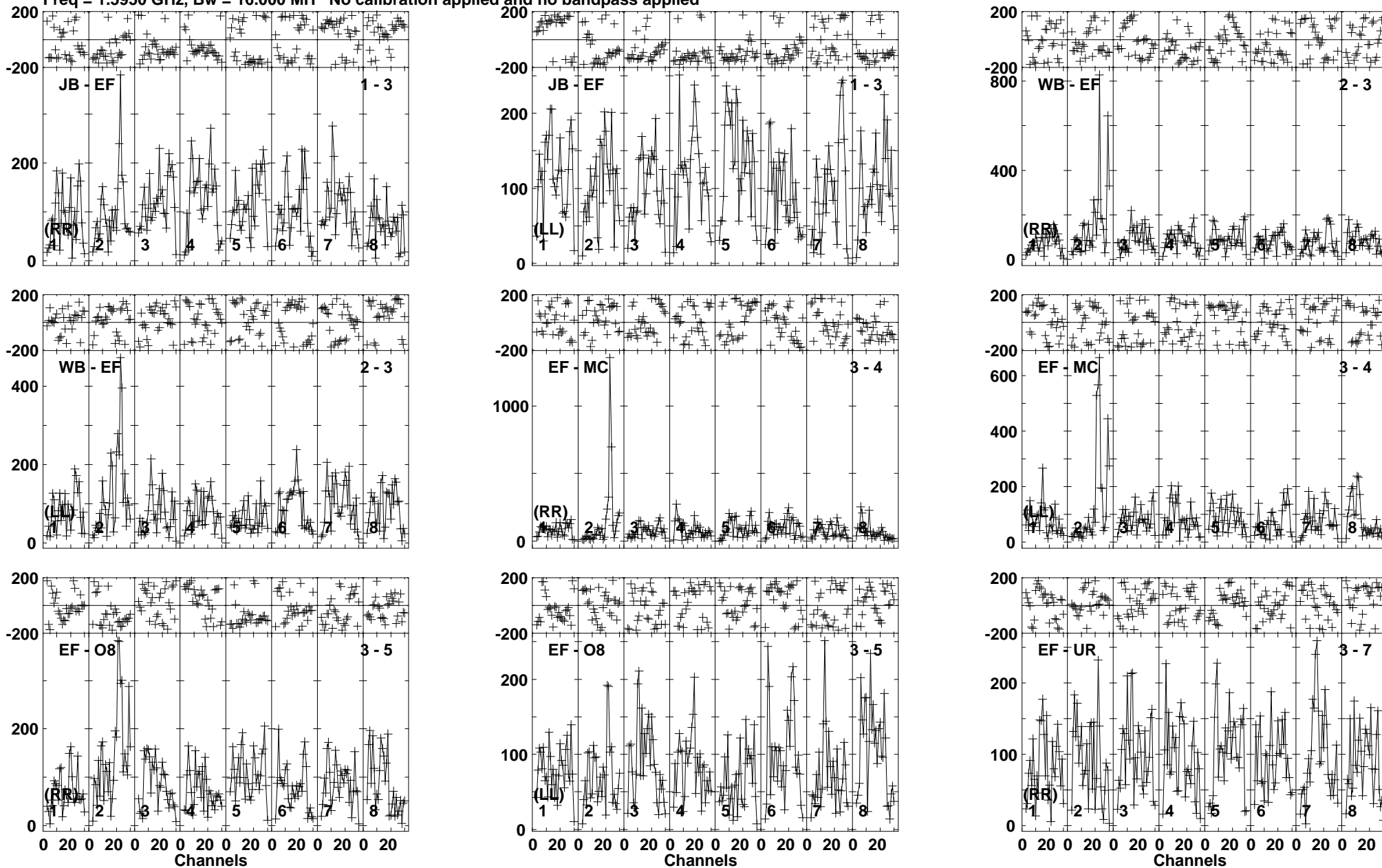
Lower frame: Micro Ampl Jy Top frame: Phas deg Vector averaged cross-power spectrum Baseline: JB (01) - EF (03) Timerange: 00/21:18:41 to 00/21:22:29
