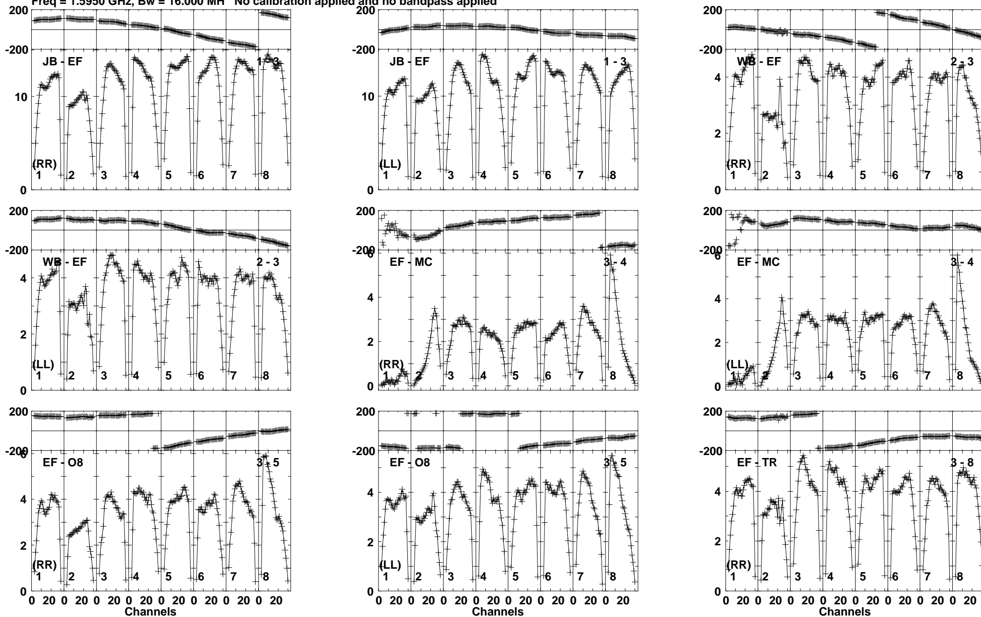
Lower frame: Milli Ampl Jy Top frame: Phas deg Vector averaged cross-power spectrum Baseline: JB (01) - EF (03) Timerange: 01/00:41:01 to 01/00:42:09
