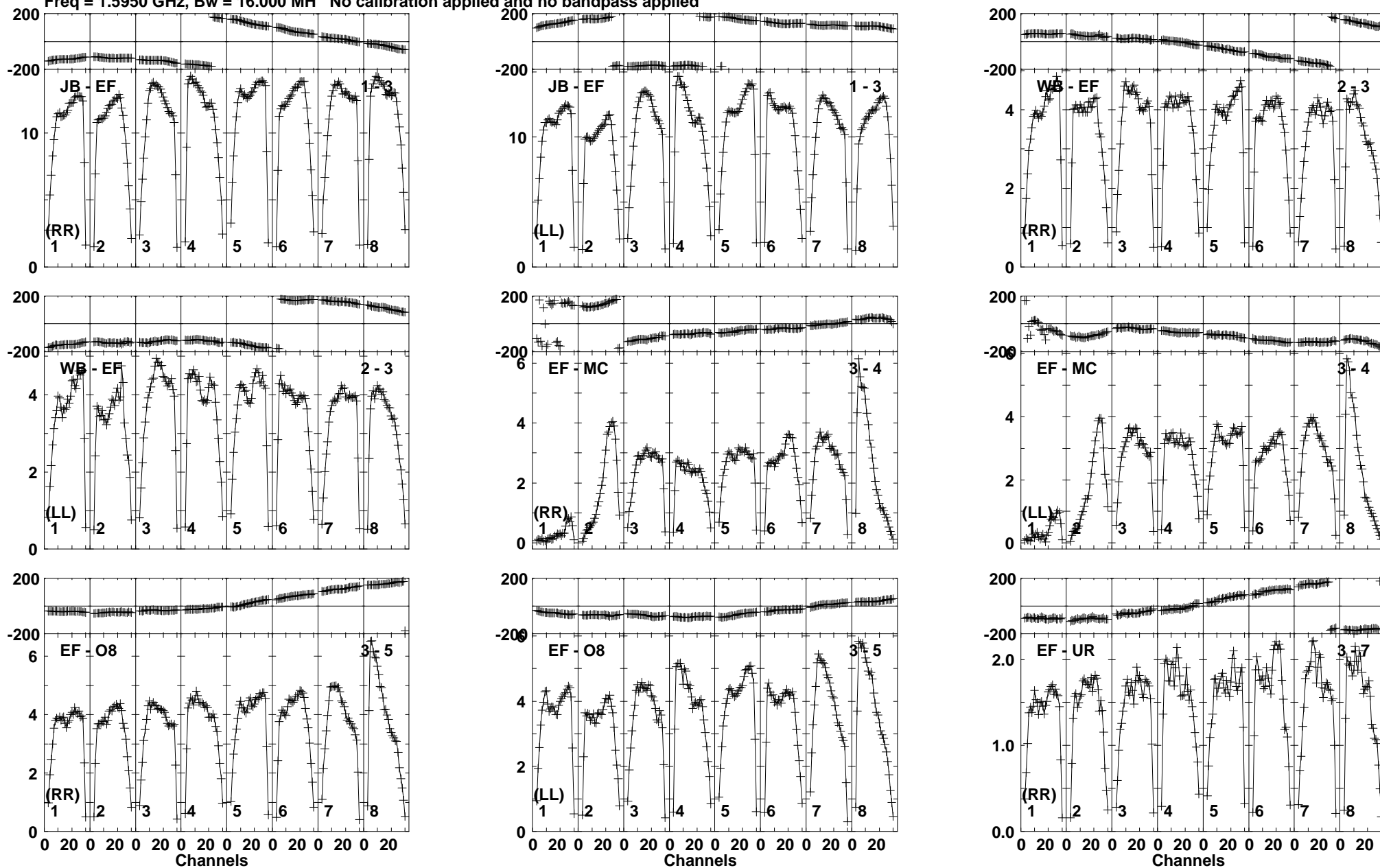
Lower frame: Milli Ampl Jy Top frame: Phas deg Vector averaged cross-power spectrum Baseline: JB (01) - EF (03) Timerange: 00:22:12:01 to 00:22:13:09
