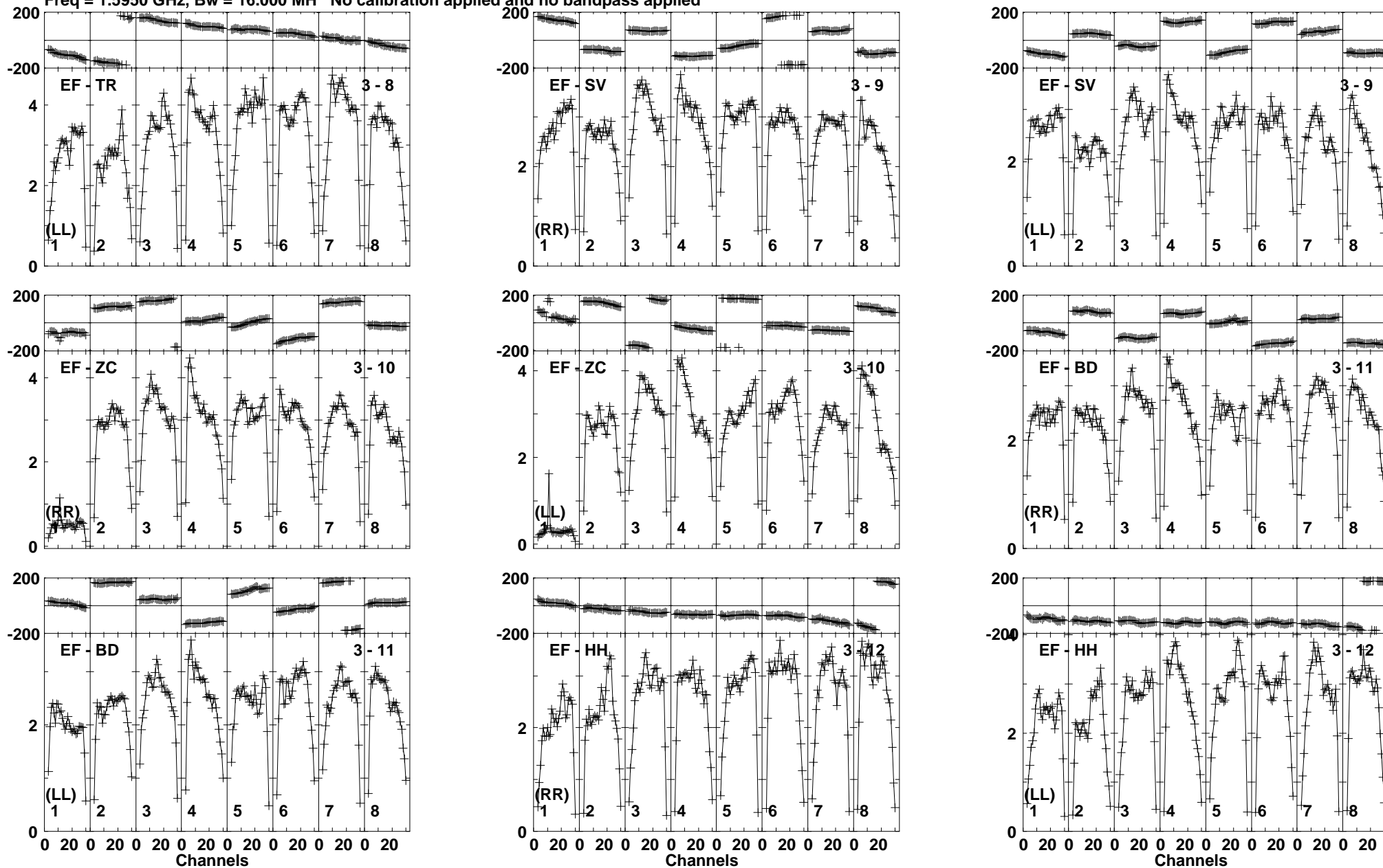
Lower frame: Milli Ampl Jy Top frame: Phas deg Vector averaged cross-power spectrum Baseline: EF (03) - TR (08) Timerange: 00/21:22:31 to 00/21:23:39
