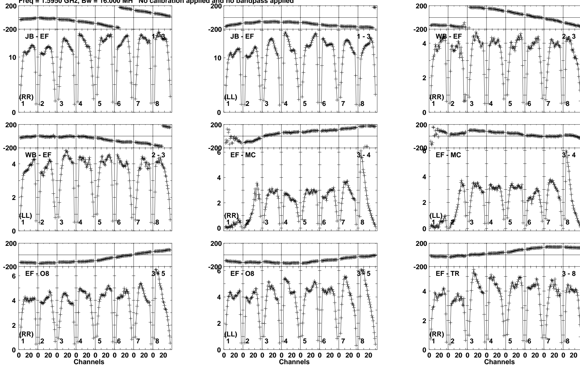
Lower frame: Milli Ampl Jy Top frame: Phas deg Vector averaged cross-power spectrum Baseline: JB (01) - EF (03) Timerange: 00/23:25:31 to 00/23:26:39
