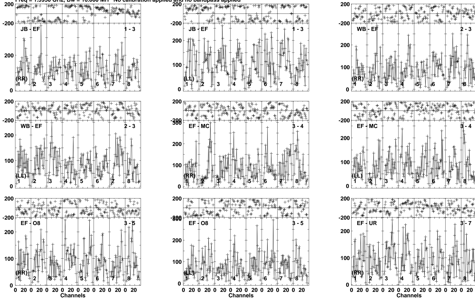
Lower frame: Micro Ampl Jy Top frame: Phas deg Vector averaged cross-power spectrum Baseline: JB (01) - EF (03) Timerange: 00/21:23:41 to 00/21:27:29
