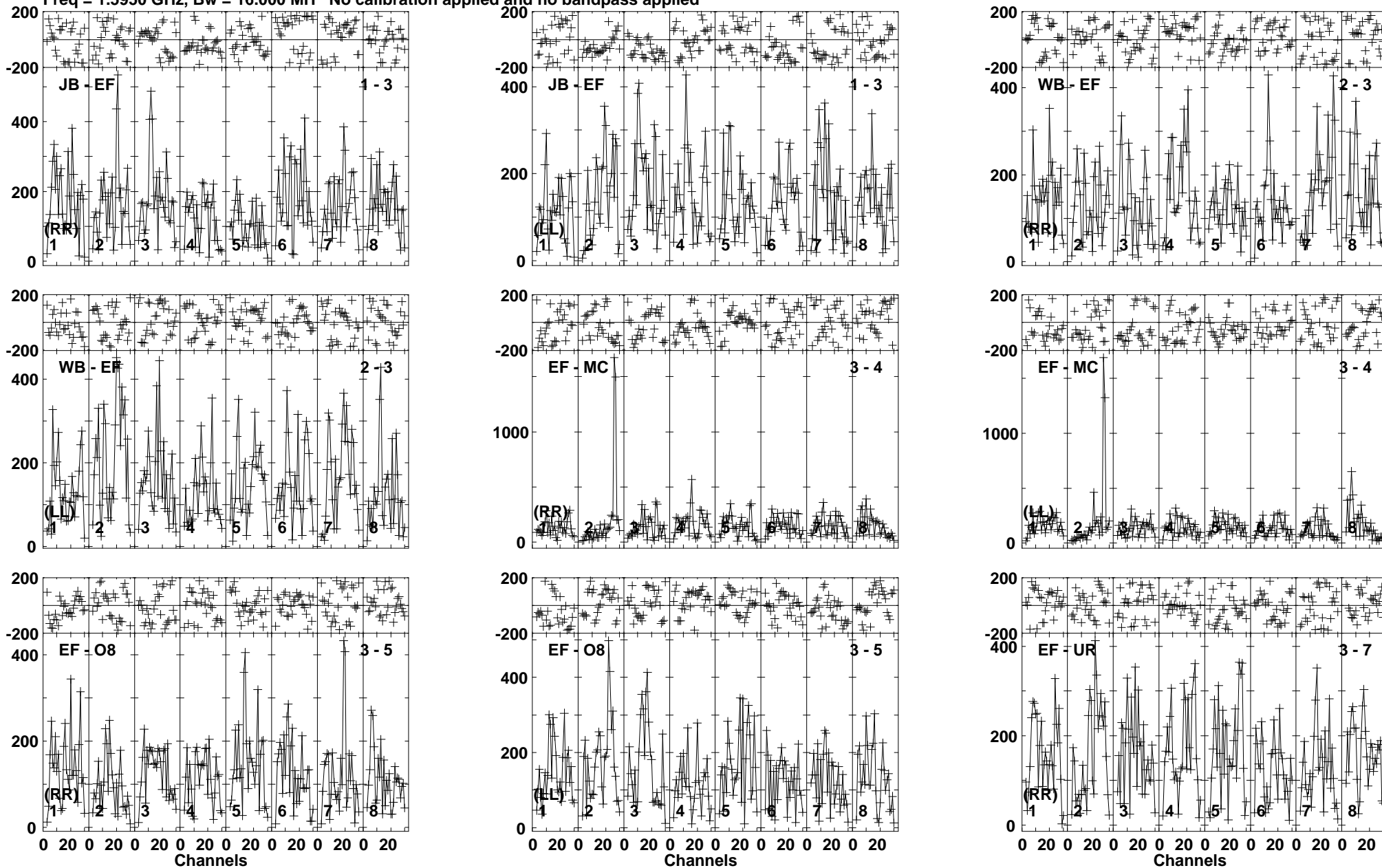
Lower frame: Micro Ampl Jy Top frame: Phas deg Vector averaged cross-power spectrum Baseline: JB (01) - EF (03) Timerange: 00/23:04:31 to 00/23:05:39
