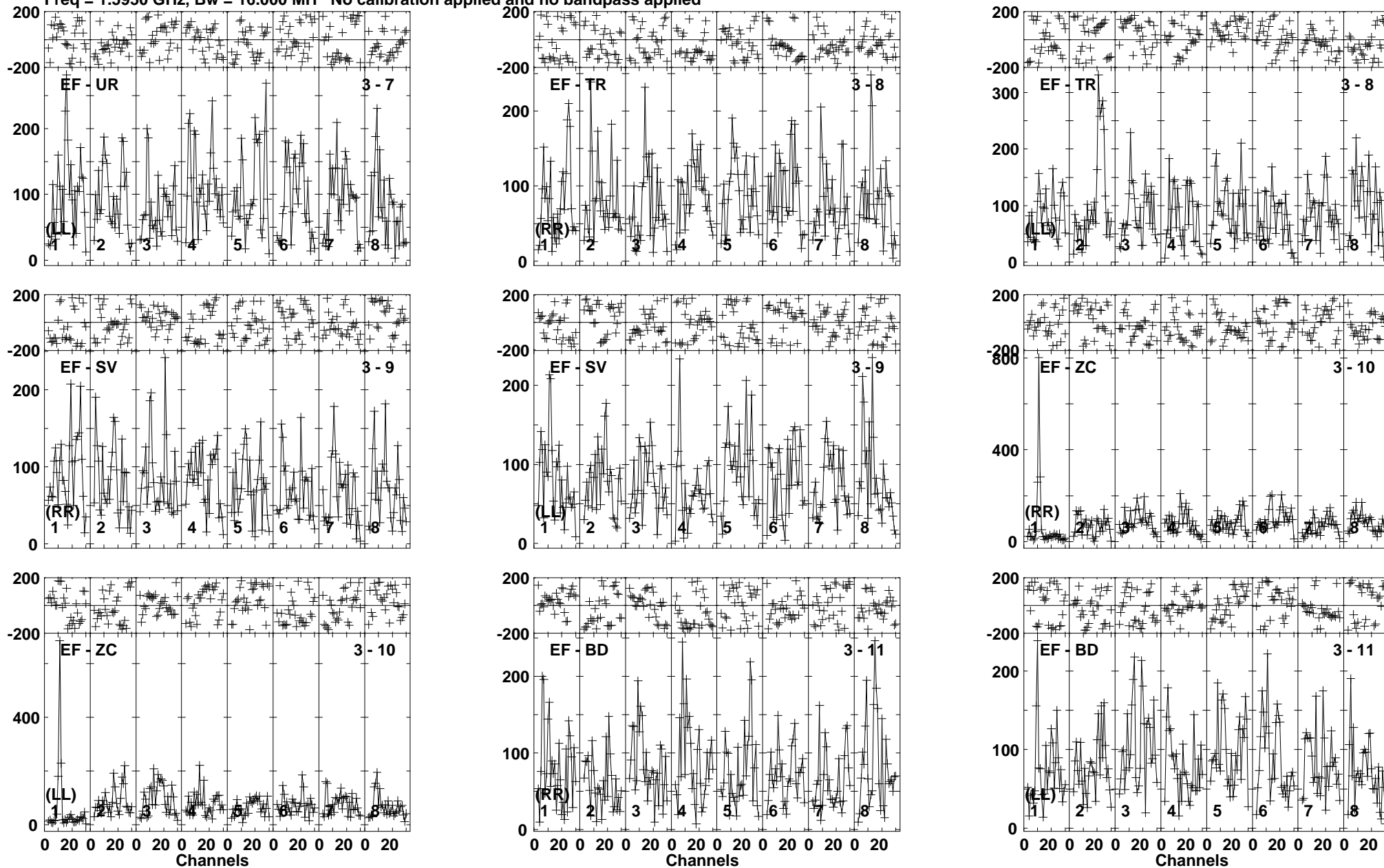
Lower frame: Micro Ampl Jy Top frame: Phas deg Vector averaged cross-power spectrum Baseline: EF (03) - UR (07) Timerange: 00/21:18:41 to 00/21:22:29
