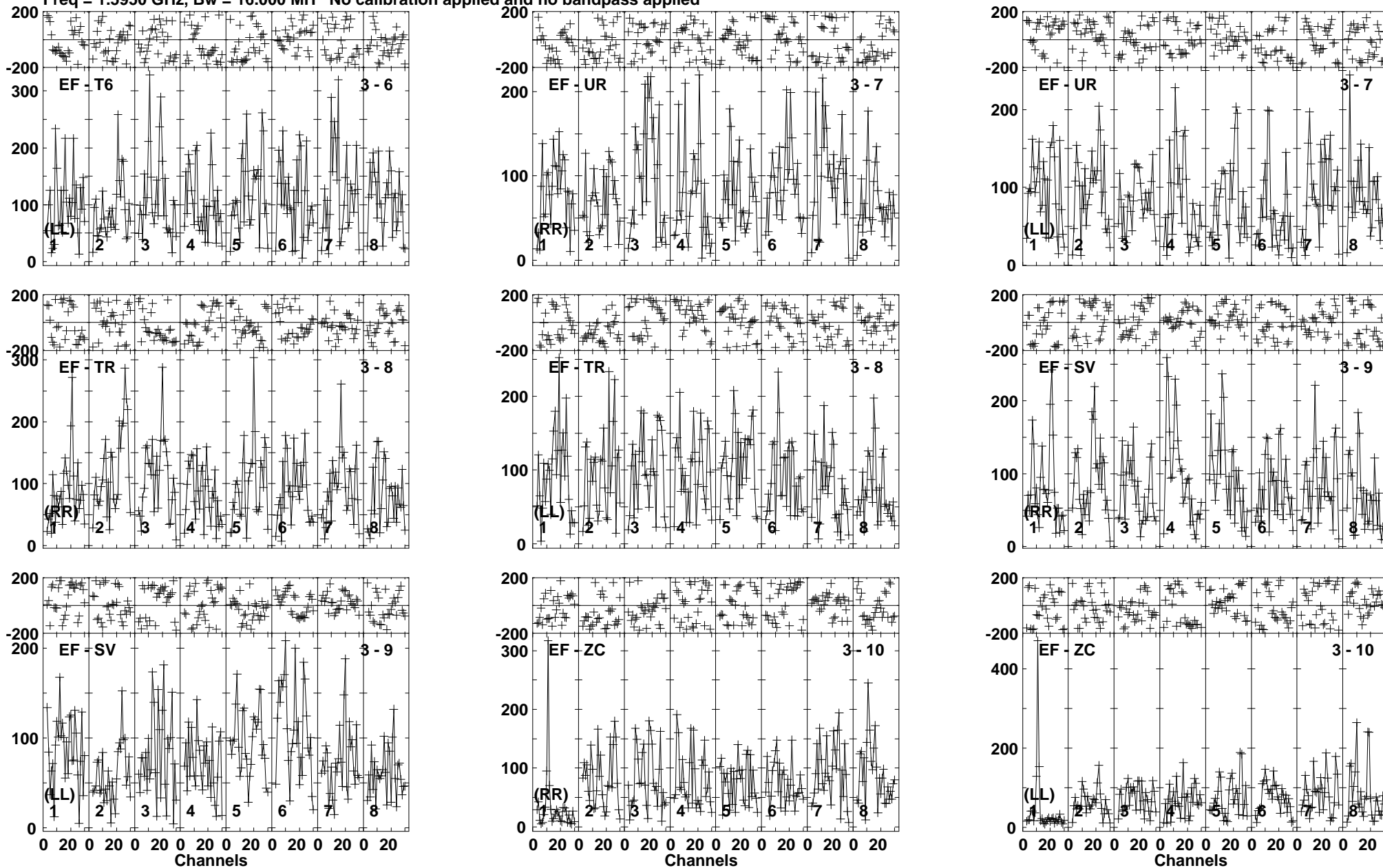
Lower frame: Micro Ampl Jy Top frame: Phas deg Vector averaged cross-power spectrum Baseline: EF (03) - T6 (06) Timerange: 00/20:05:11 to 00/20:08:59
