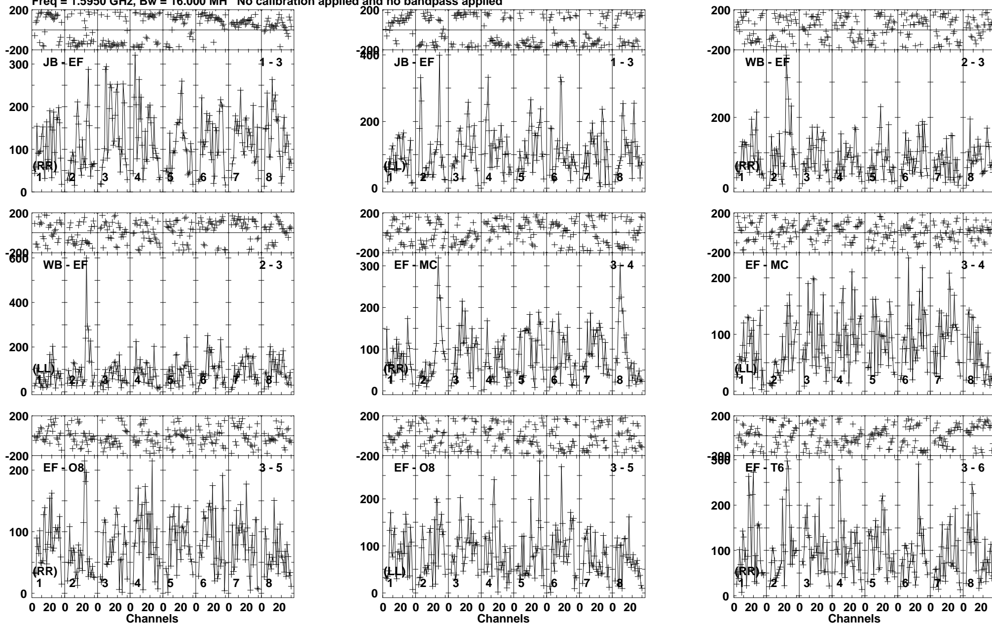
Lower frame: Micro Ampl Jy Top frame: Phas deg Vector averaged cross-power spectrum Baseline: JB (01) - EF (03) Timerange: 00/20:20:41 to 00/20:24:29
