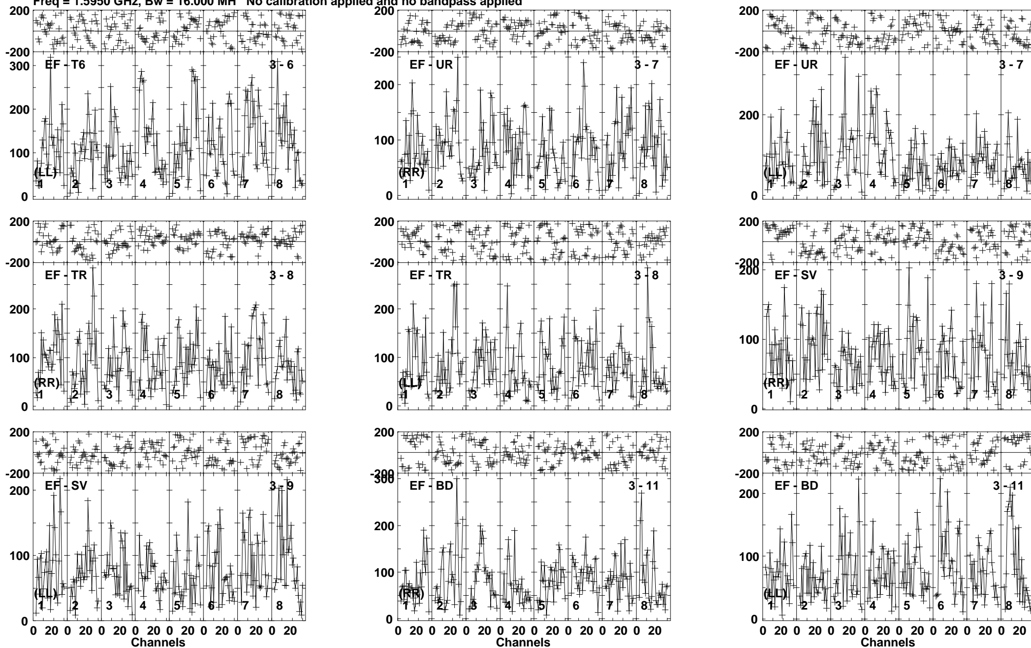
Lower frame: Micro Ampl Jy Top frame: Phas deg Vector averaged cross-power spectrum Baseline: EF (03) - T6 (06) Timerange: 00:19:54:41 to 00:19:58:29
