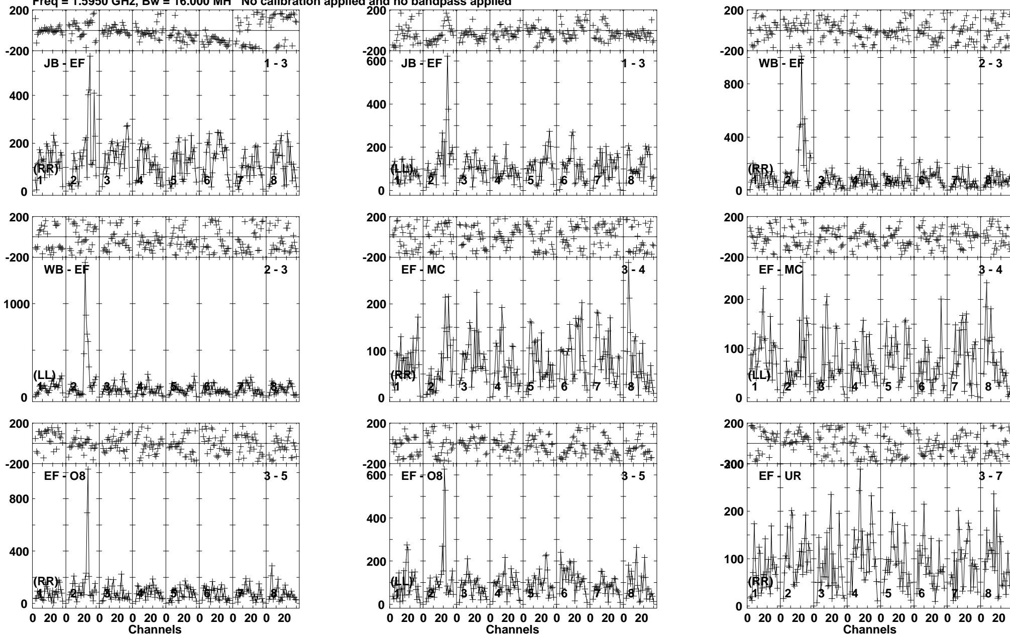
Lower frame: Micro Ampl Jy Top frame: Phas deg Vector averaged cross-power spectrum Baseline: JB (01) - EF (03) Timerange: 00/22:07:41 to 00/22:11:29
