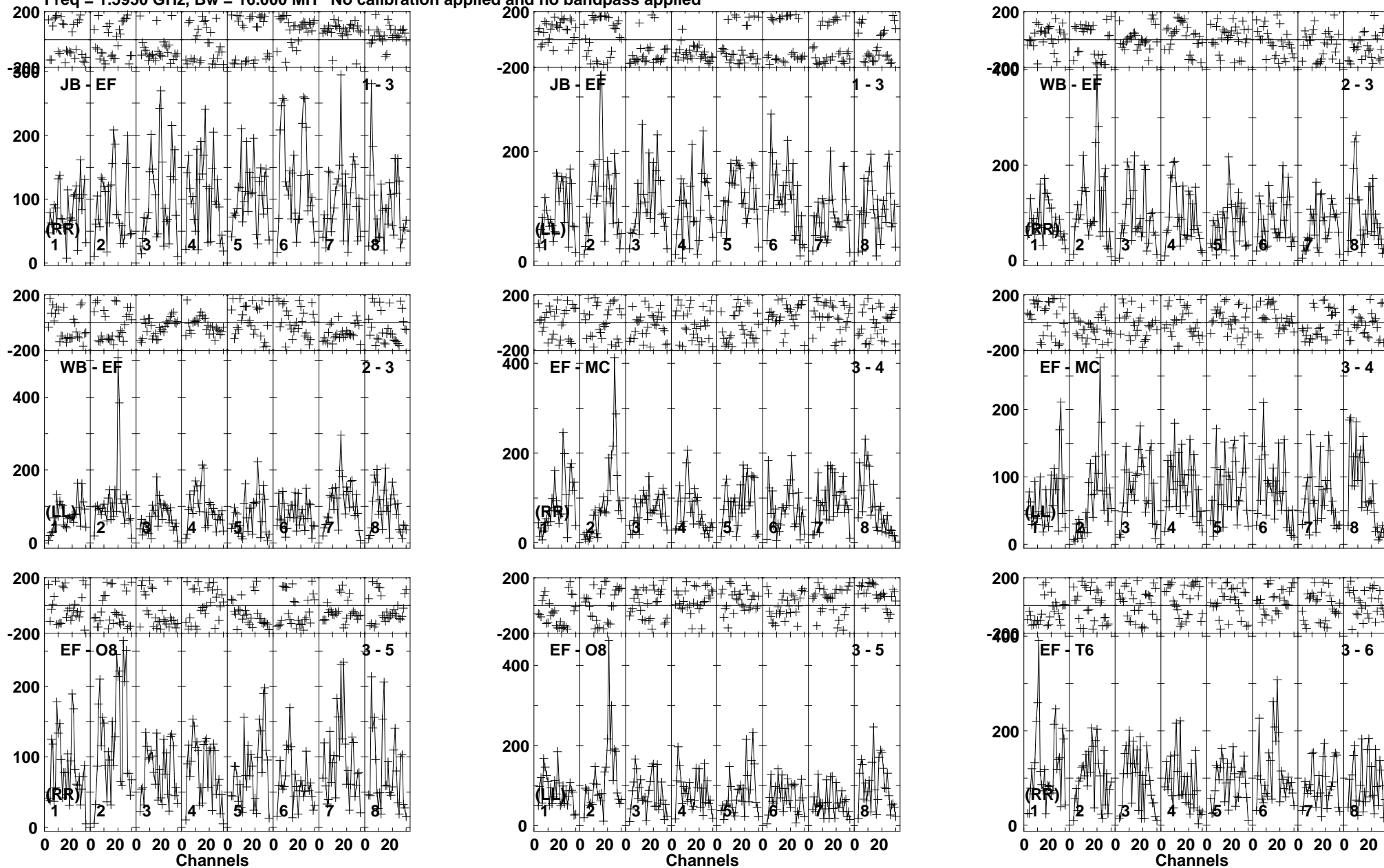
Lower frame: Micro Ampl Jy Top frame: Phas deg Vector averaged cross-power spectrum Baseline: JB (01) - EF (03) Timerange: 00/20:41:41 to 00/20:45:29
