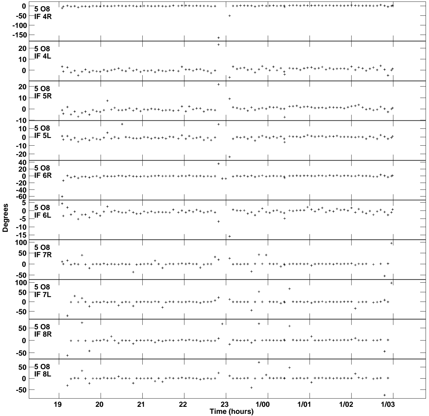
Plot file version 8 created 12-AUG-2019 17:21:24 Gain phs vs UTC time for 0205-010.MULTI.1 SN 1 Rpol & Lpol IF 1 - 8
