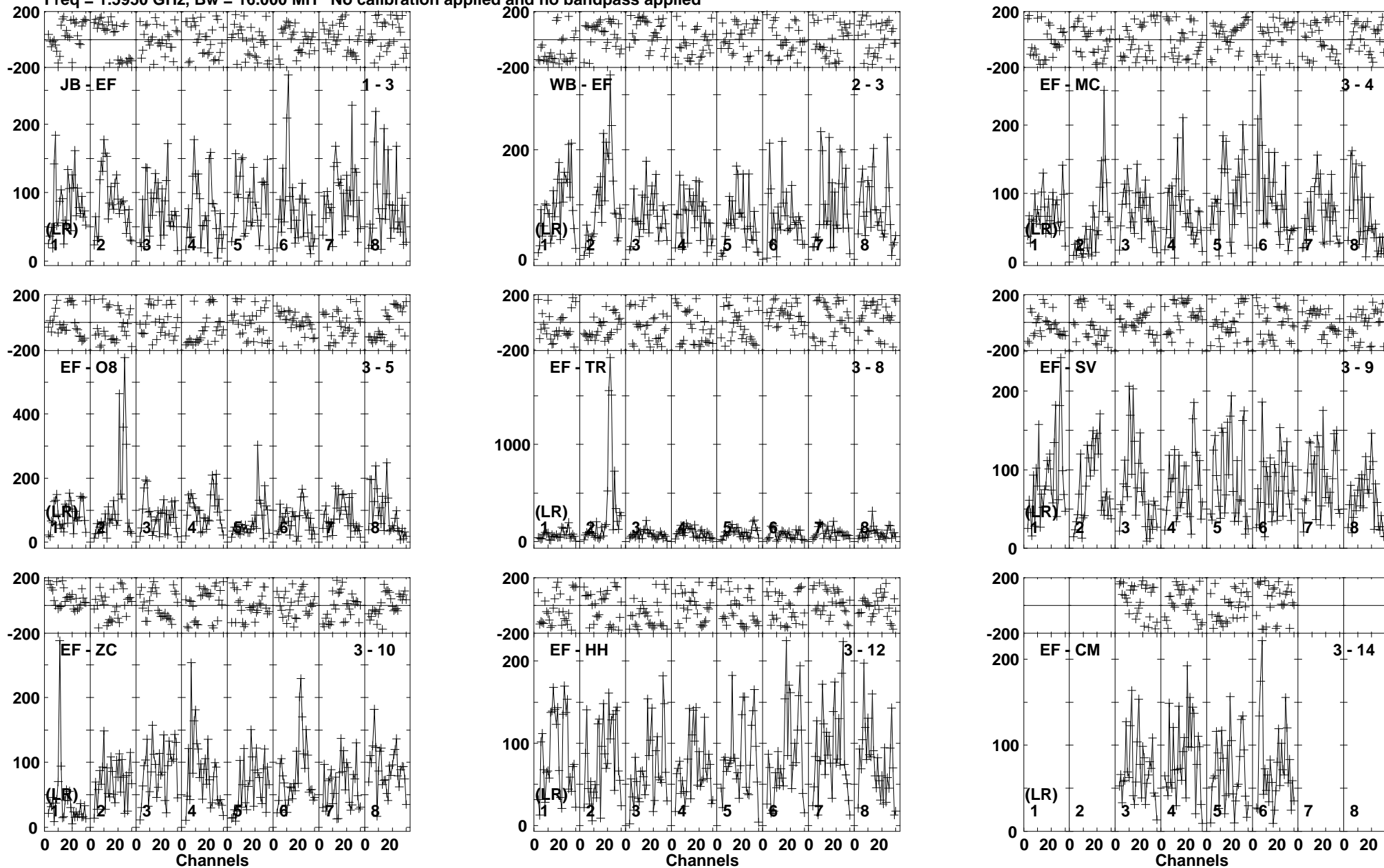
Lower frame: Micro Ampl Jy Top frame: Phas deg Vector averaged cross-power spectrum Baseline: JB (01) - EF (03) Timerange: 01/01:08:11 to 01/01:11:59
