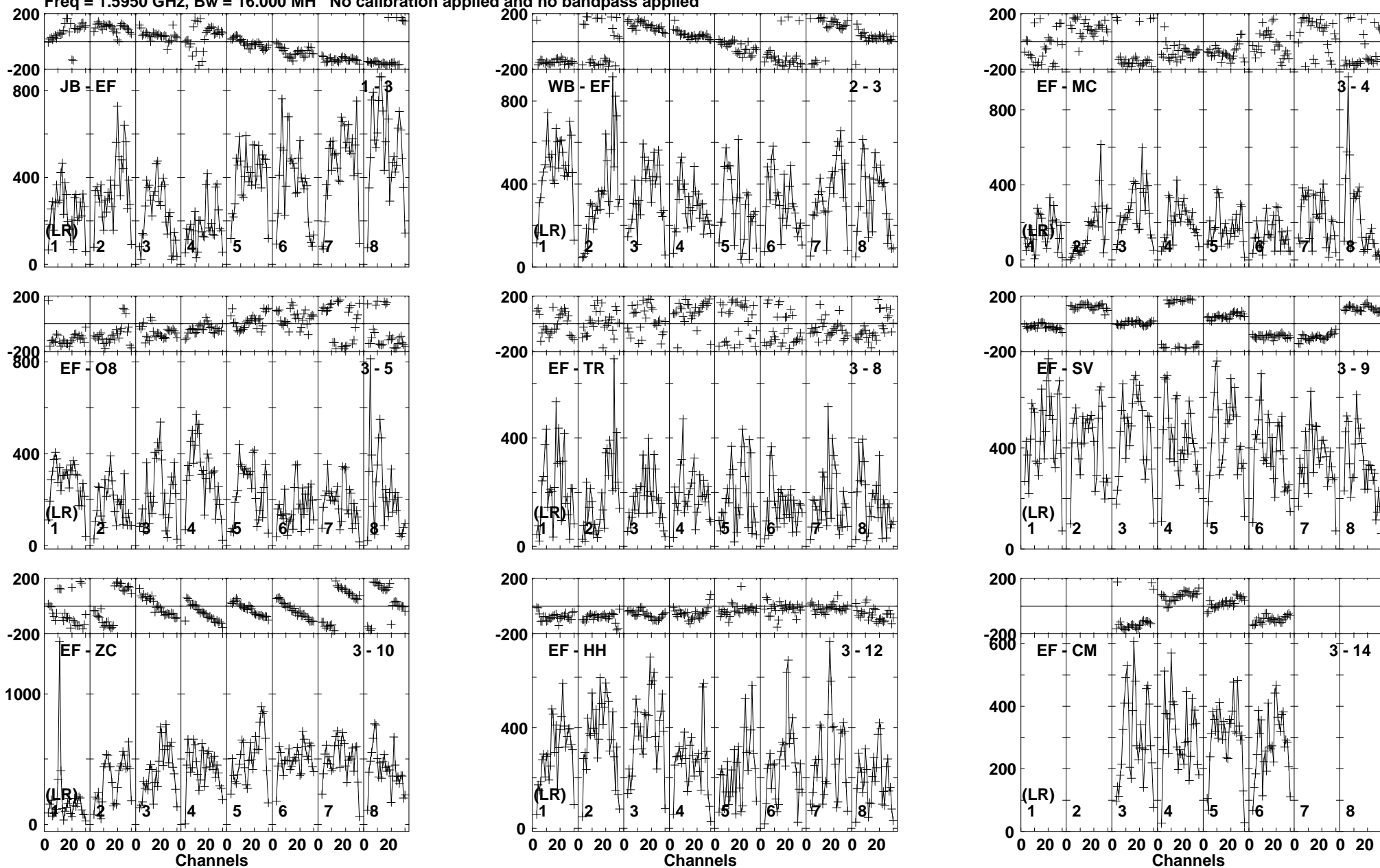
Lower frame: Micro Ampl Jy Top frame: Phas deg Vector averaged cross-power spectrum Baseline: JB (01) - EF (03) Timerange: 01/01:12:31 to 01/01:13:39
