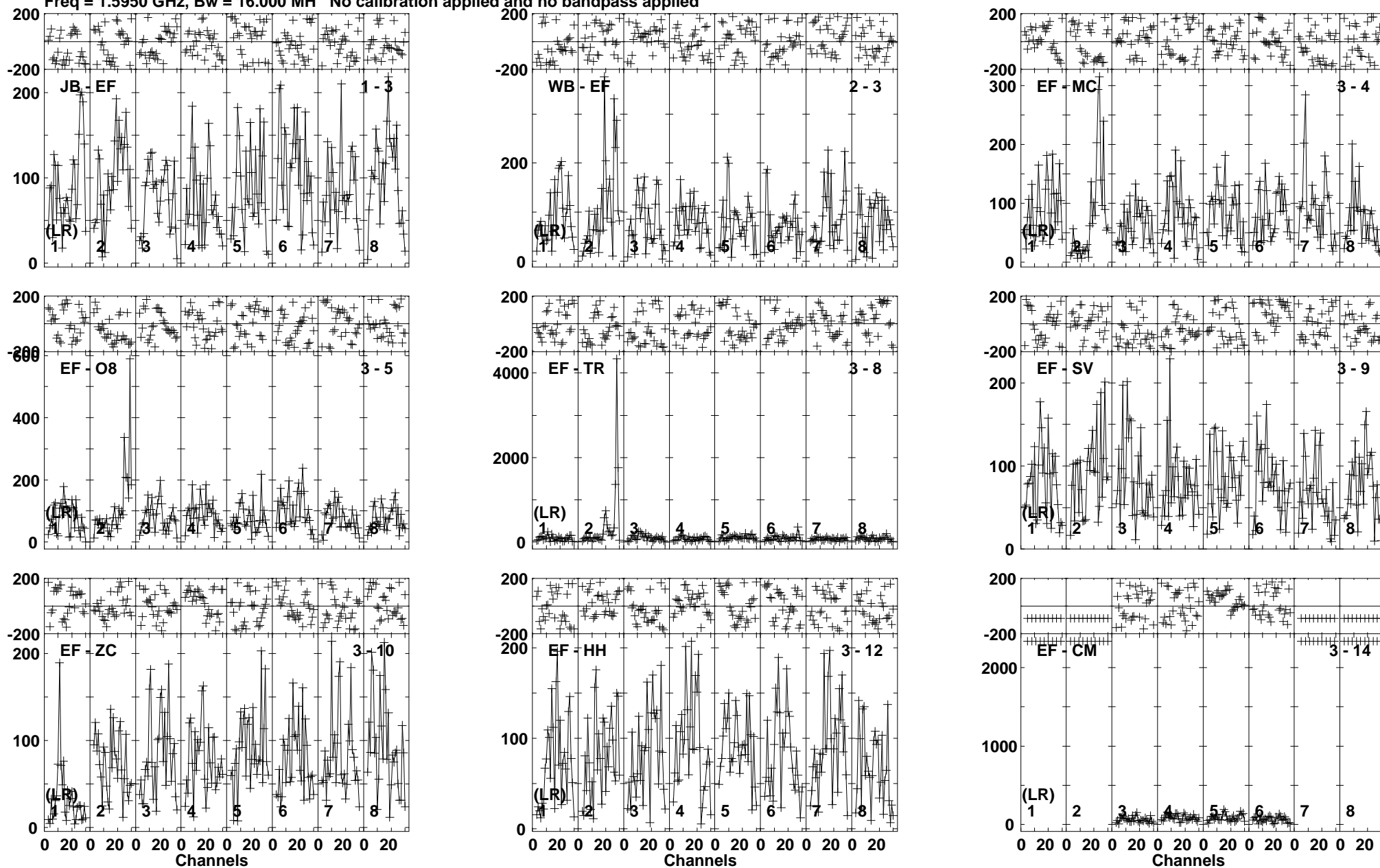
Lower frame: Micro Ampl Jy Top frame: Phas deg Vector averaged cross-power spectrum Baseline: JB (01) - EF (03) Timerange: 01/00:42:11 to 01/00:45:59
