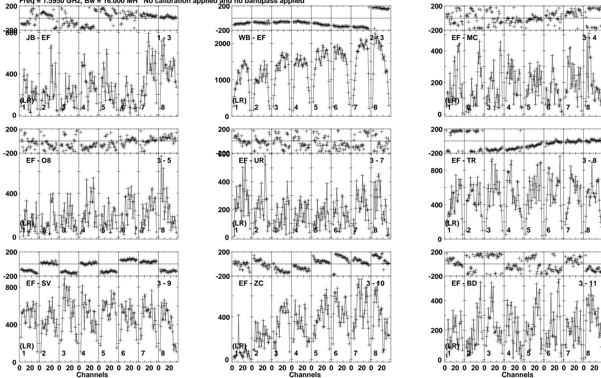
Lower frame: Micro Ampl Jy Top frame: Phas deg Vector averaged cross-power spectrum Baseline: JB (01) - EF (03) Timerange: 00/19:22:01 to 00/19:23:09
