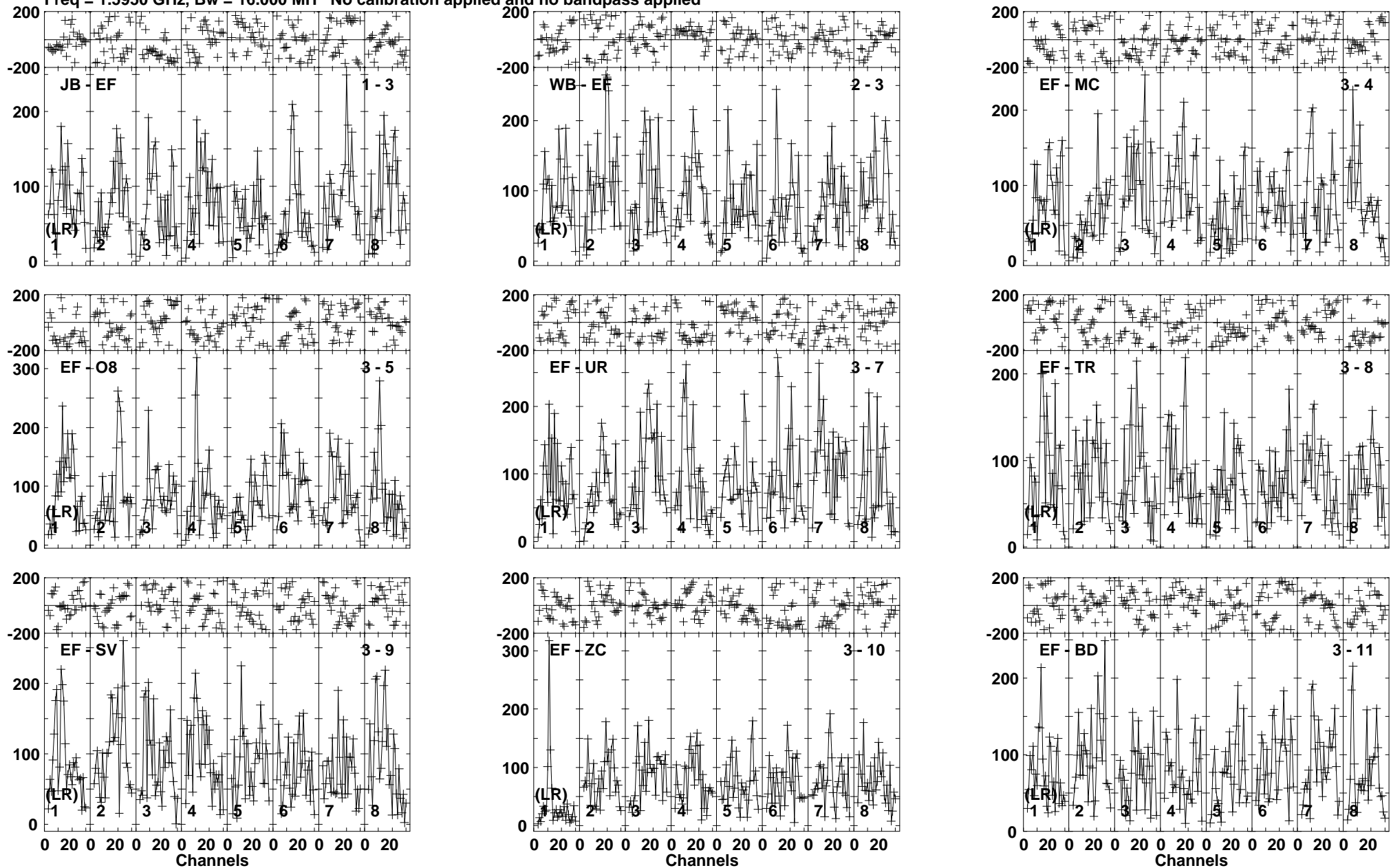
Lower frame: Micro Ampl Jy Top frame: Phas deg Vector averaged cross-power spectrum Baseline: JB (01) - EF (03) Timerange: 00:19:38:41 to 00:19:42:29
