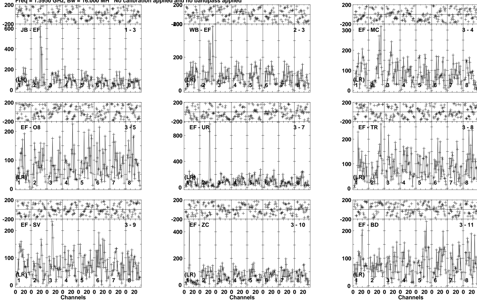
Lower frame: Micro Ampl Jy Top frame: Phas deg Vector averaged cross-power spectrum Baseline: JB (01) - EF (03) Timerange: 00/20:57:41 to 00/21:01:29
