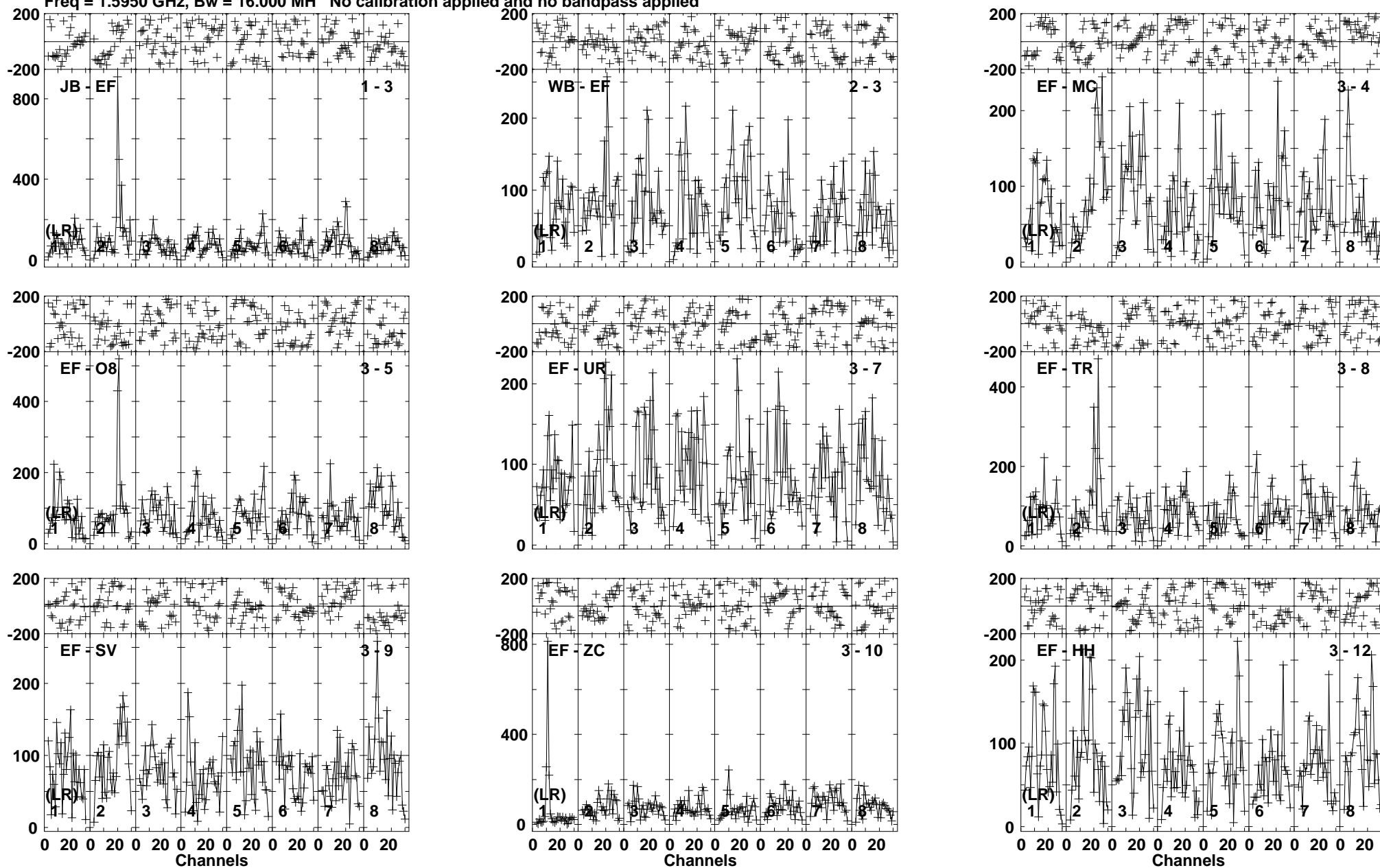
Lower frame: Micro Ampl Jy Top frame: Phas deg Vector averaged cross-power spectrum Baseline: JB (01) - EF (03) Timerange: 00/22:02:41 to 00/22:06:29
