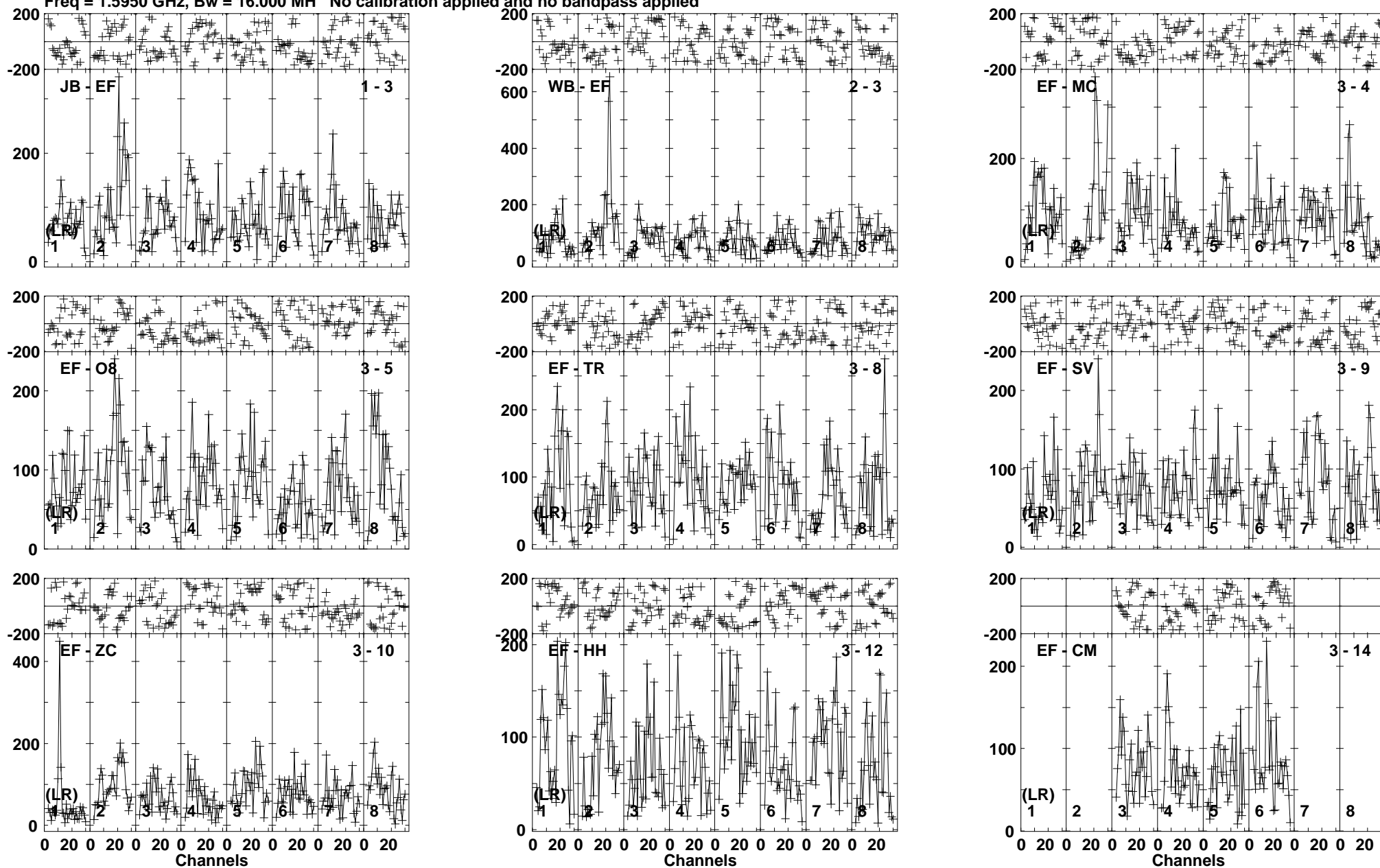
Lower frame: Micro Ampl Jy Top frame: Phas deg Vector averaged cross-power spectrum Baseline: JB (01) - EF (03) Timerange: 01/01:29:11 to 01/01:32:59
