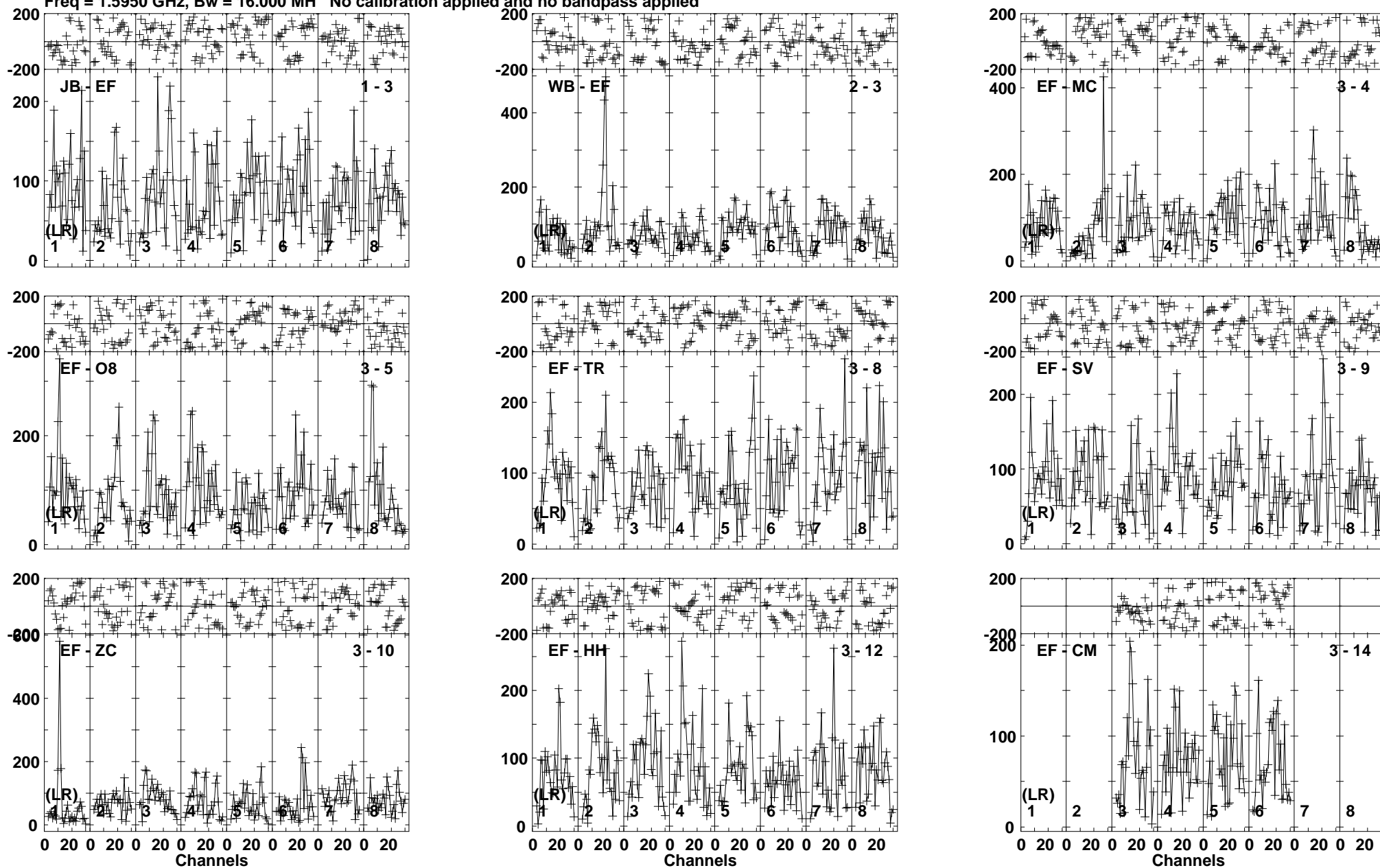
Lower frame: Micro Ampl Jy Top frame: Phas deg Vector averaged cross-power spectrum Baseline: JB (01) - EF (03) Timerange: 01/01:24:11 to 01/01:27:59
