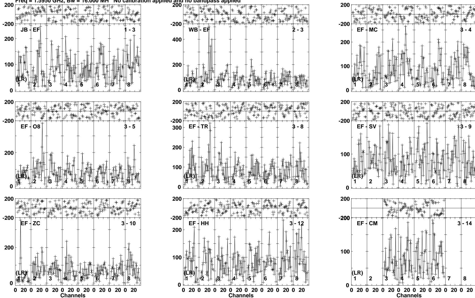
Lower frame: Micro Ampl Jy Top frame: Phas deg Vector average cross-power spectrum Baseline: JB (01) - EF (03) Timerange: 00/23:42:11 to 00/23:45:59
