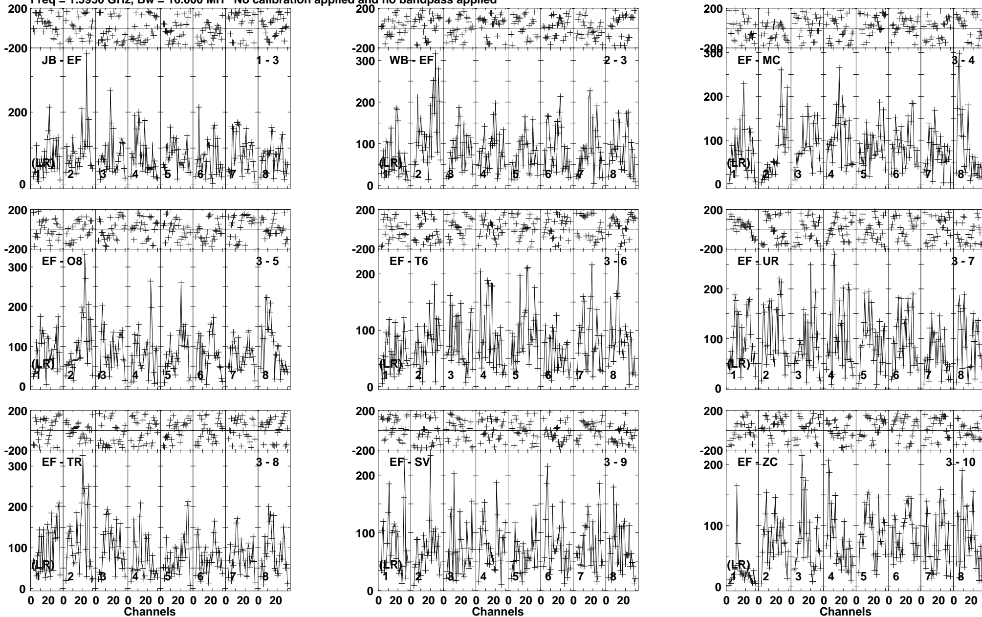
Lower frame: Micro Ampl Jy Top frame: Phas deg Vector averaged cross-power spectrum Baseline: JB (01) - EF (03) Timerange: 00/20:36:41 to 00/20:40:29
