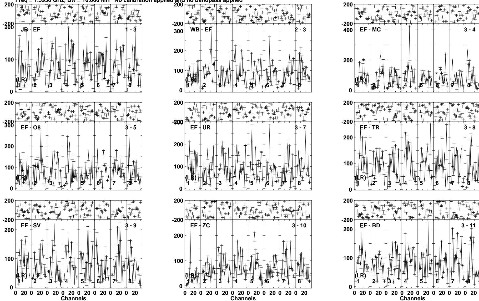
Lower frame: Micro Ampl Jy Top frame: Phas deg Vector averaged cross-power spectrum Baseline: JB (01) - EF (03) Timerange: 00:19:54:41 to 00:19:58:29
