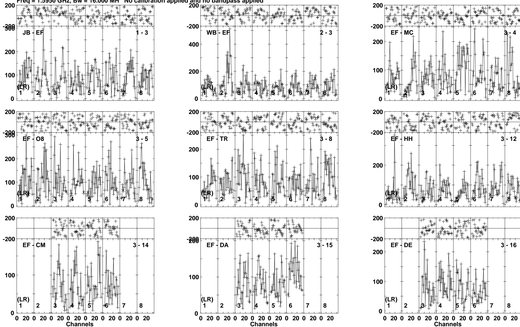
Lower frame: Micro Ampl Jy Top frame: Phas deg Vector averaged cross-power spectrum Baseline: JB (01) - EF (03) Timerange: 01/02:11:11 to 01/02:14:59
