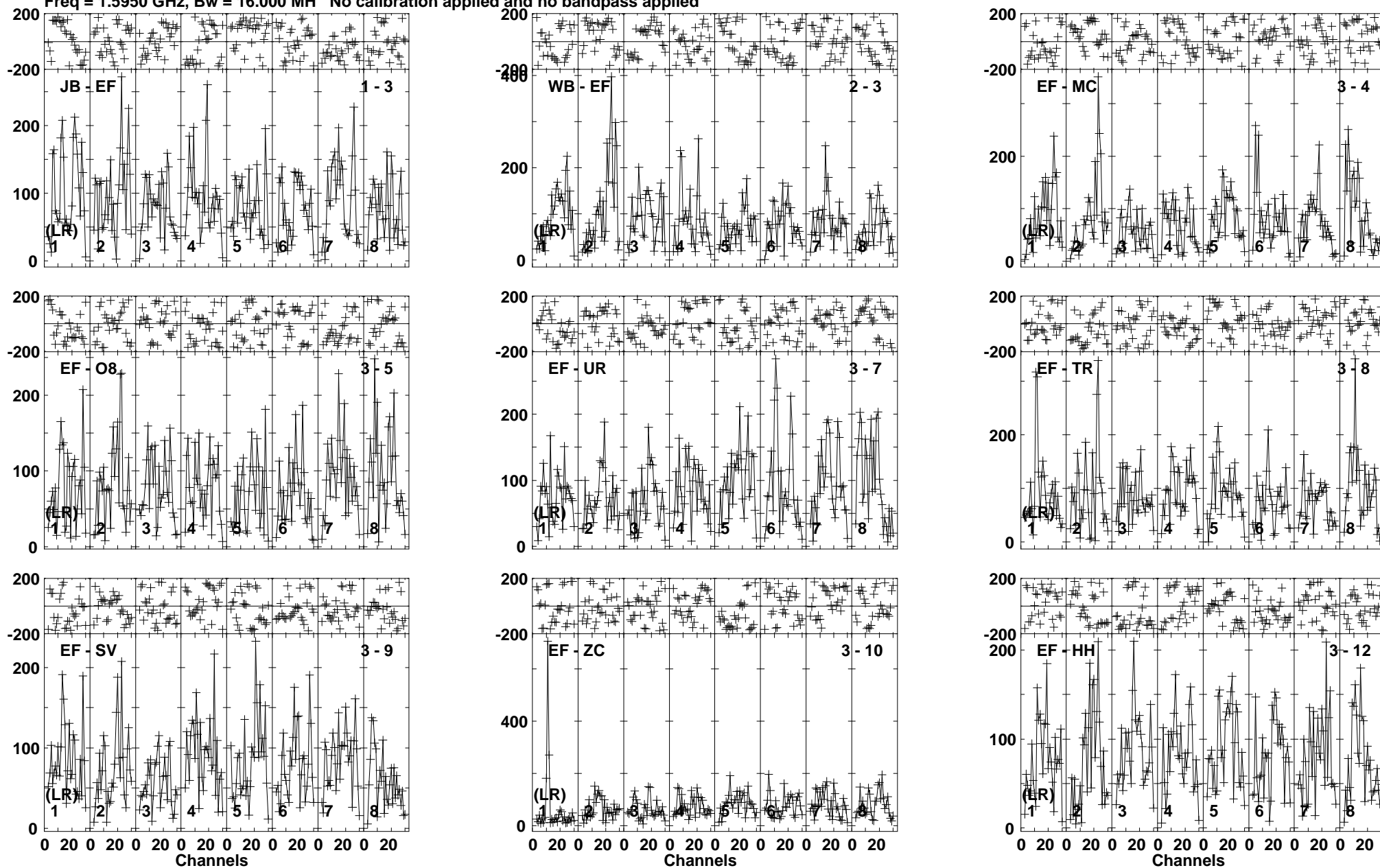
Lower frame: Micro Ampl Jy Top frame: Phas deg Vector averaged cross-power spectrum Baseline: JB (01) - EF (03) Timerange: 00/22:34:11 to 00/22:37:59
