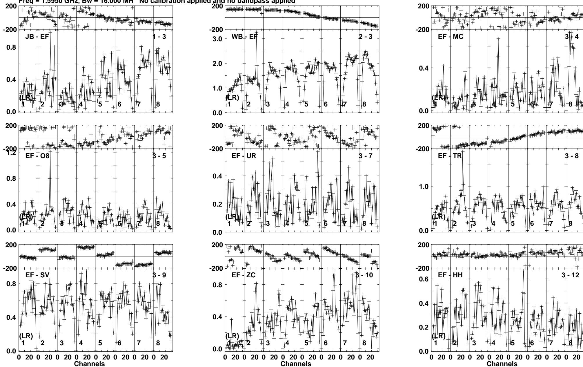
Lower frame: Milli Ampl Jy Top frame: Phas deg Vector averaged cross-power spectrum Baseline: JB (01) - EF (03) Timerange: 00/22:01:31 to 00/22:02:39
