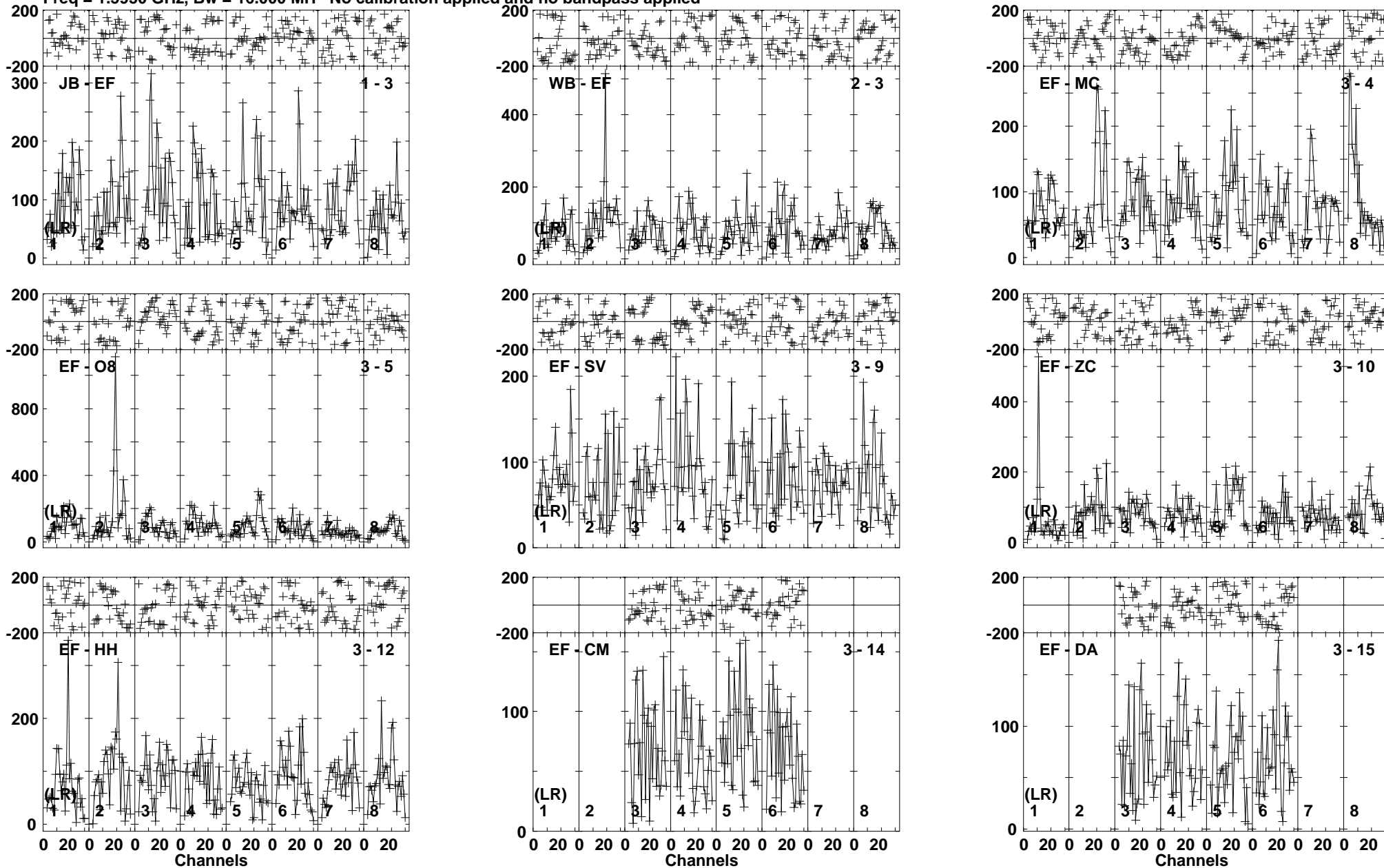
Lower frame: Micro Ampl Jy Top frame: Phas deg Vector averaged cross-power spectrum Baseline: JB (01) - EF (03) Timerange: 01/00:47:11 to 01/00:50:59
