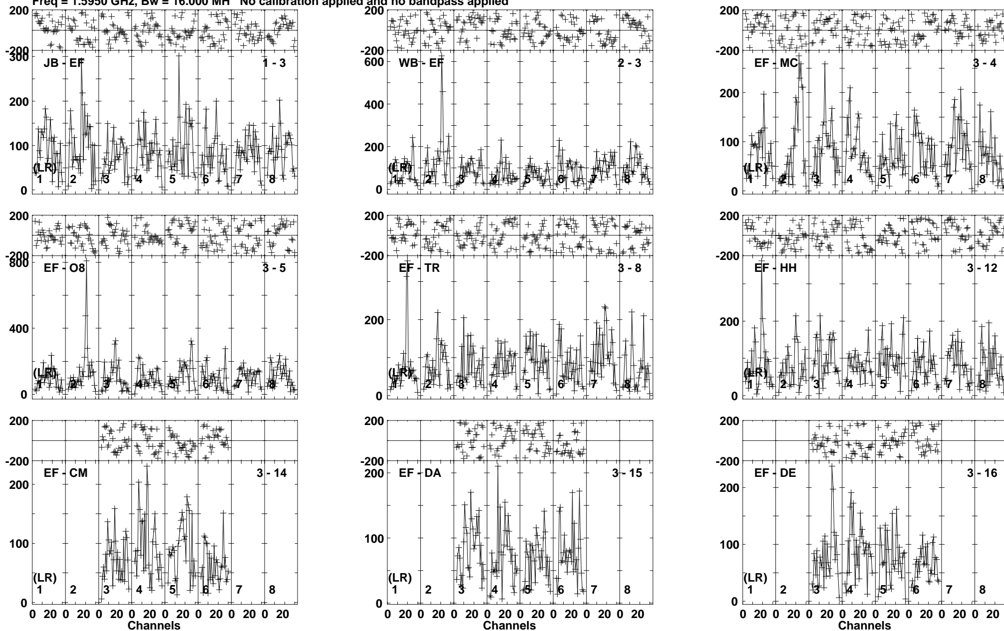
Lower frame: Micro Ampl Jy Top frame: Phas deg Vector averaged cross-power spectrum Baseline: JB (01) - EF (03) Timerange: 01/02:37:41 to 01/02:41:29
