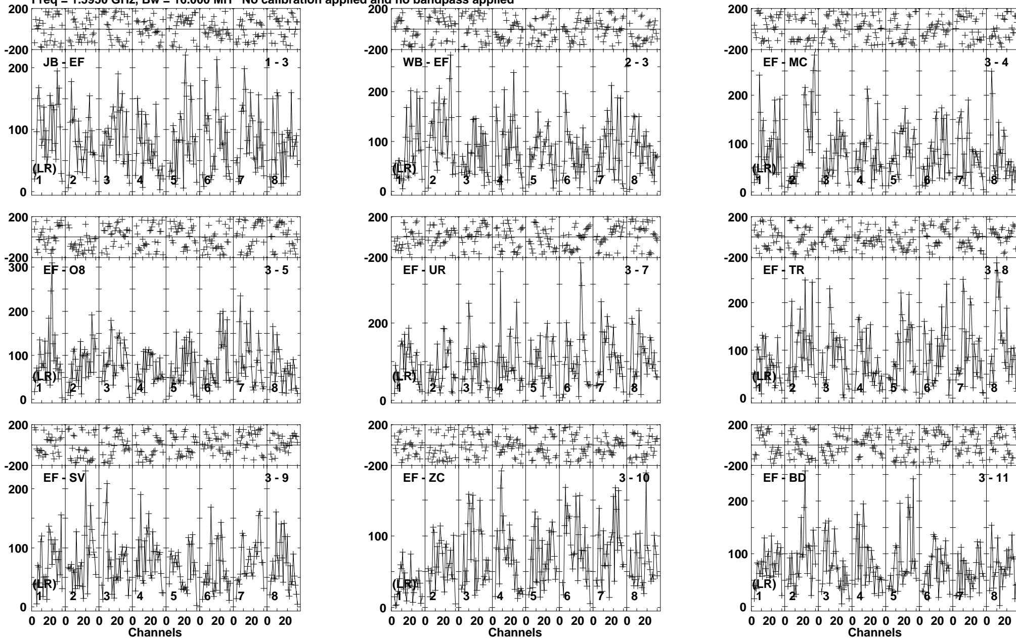
Lower frame: Micro Ampl Jy Top frame: Phas deg Vector averaged cross-power spectrum Baseline: JB (01) - EF (03) Timerange: 00/21:02:41 to 00/21:06:29
