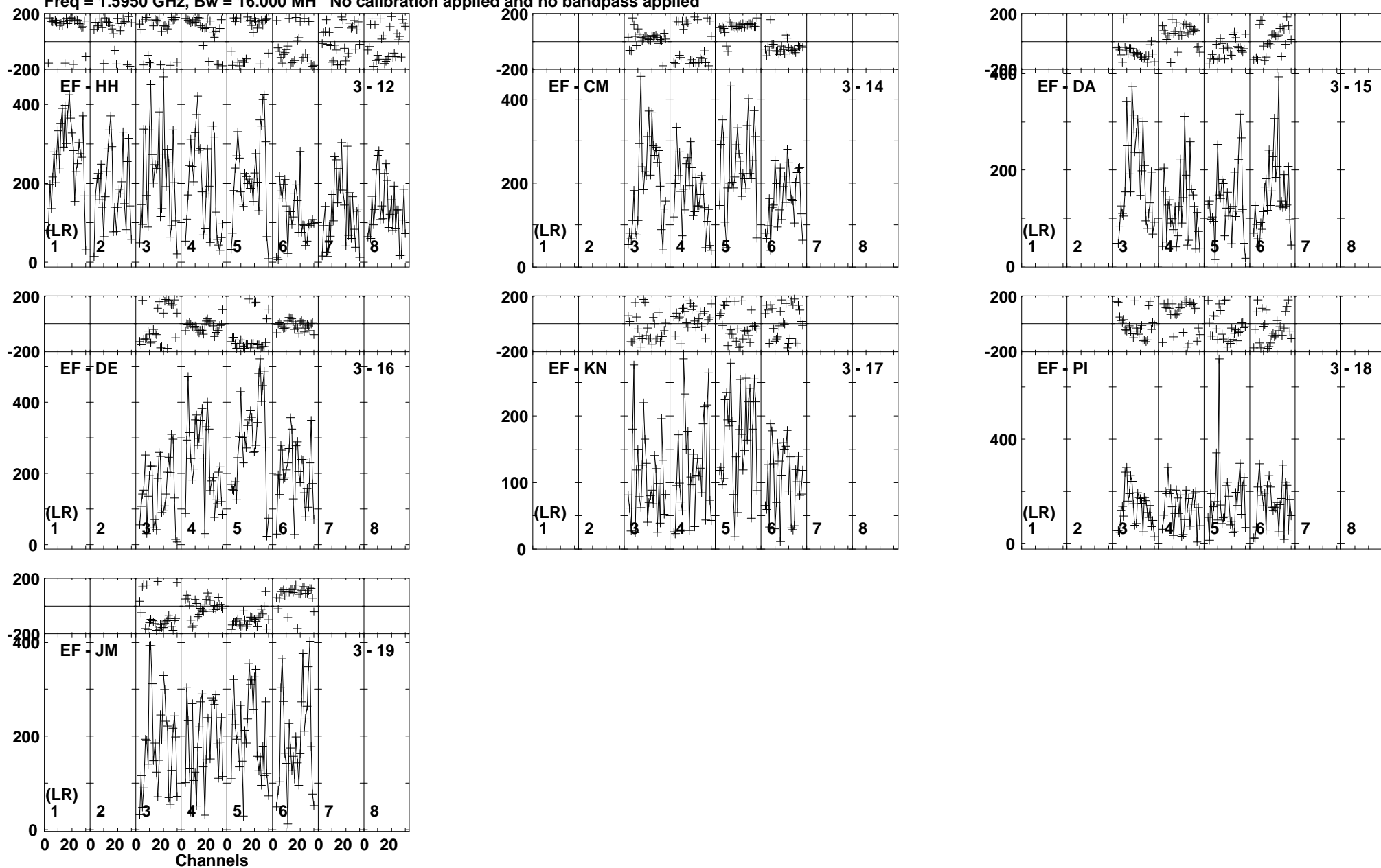
Lower frame: Micro Ampl Jy Top frame: Phas deg Vector averaged cross-power spectrum Baseline: EF (03) - HH (12) Timerange: 00/19:22:01 to 00/19:23:09
