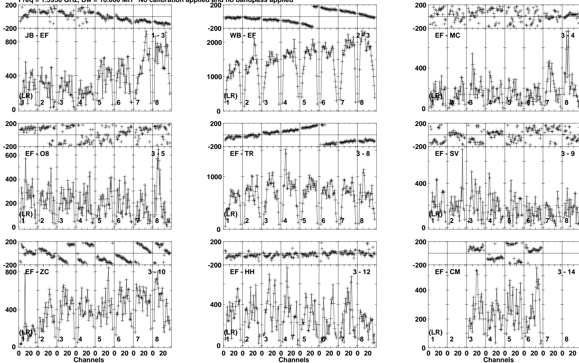
Lower frame: Micro Ampl Jy Top frame: Phas deg Vector averaged cross-power spectrum Baseline: JB (01) - EF (03) Timerange: 00/23:15:01 to 00/23:16:09
