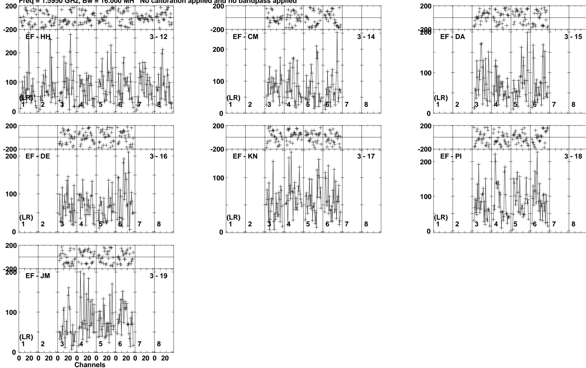
Lower frame: Micro Ampl Jy Top frame: Phas deg Vector averaged cross-power spectrum Baseline: EF (03) - HH (12) Timerange: 00/20:52:11 to 00/20:55:59
