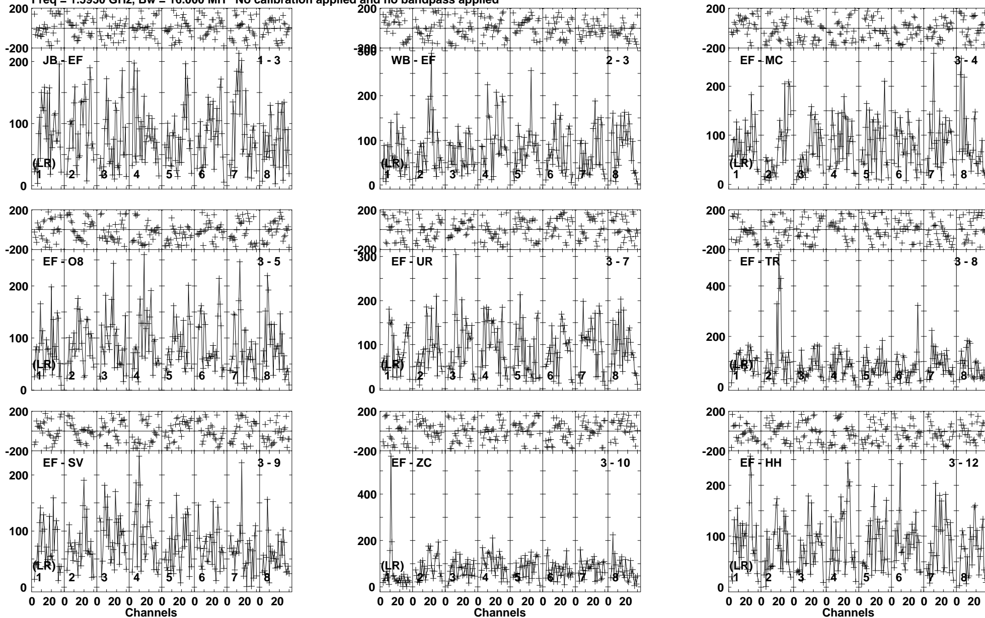
Lower frame: Micro Ampl Jy Top frame: Phas deg Vector averaged cross-power spectrum Baseline: JB (01) - EF (03) Timerange: 00/22:55:11 to 00/22:58:59
