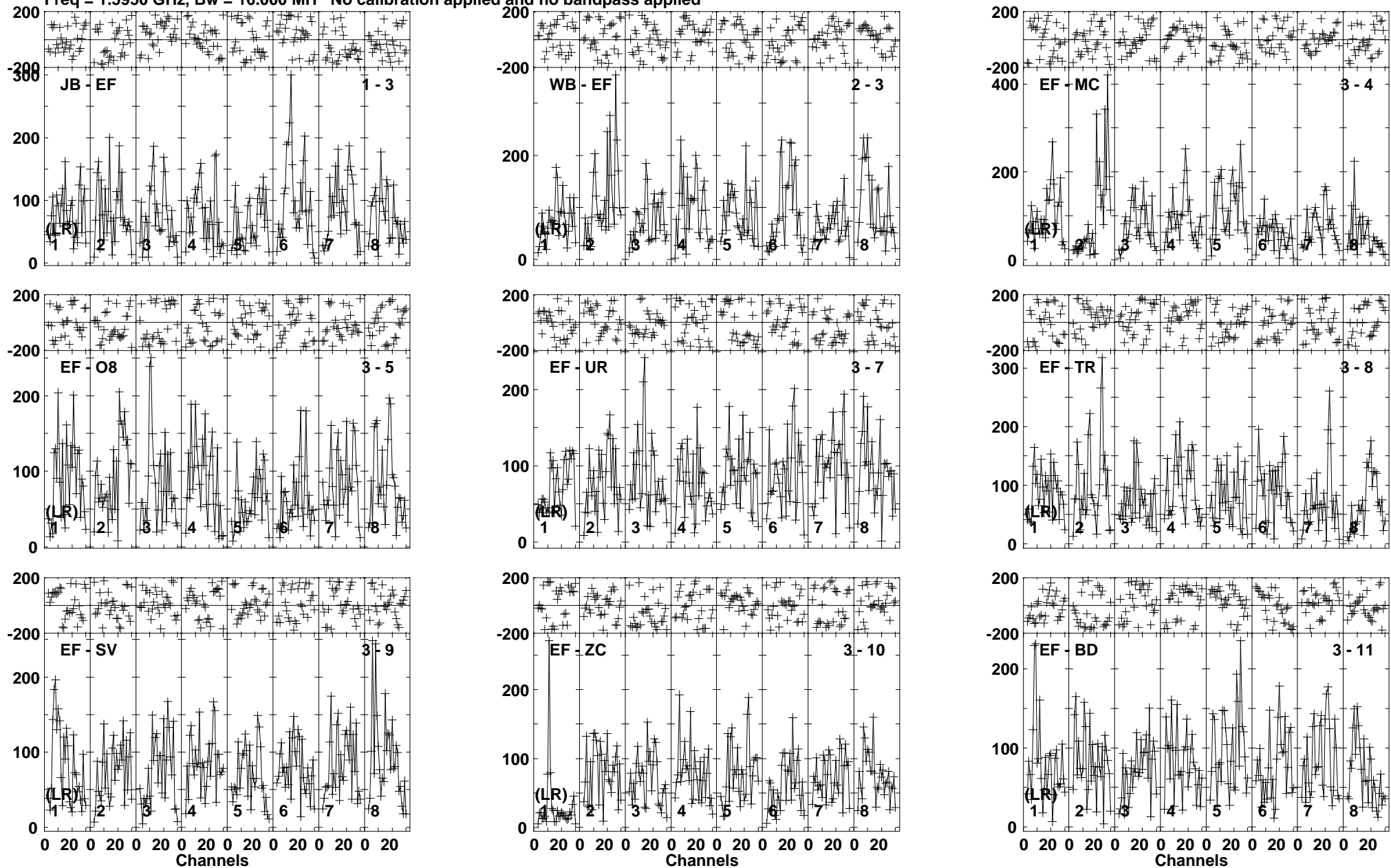
Lower frame: Micro Ampl Jy Top frame: Phas deg Vector averaged cross-power spectrum Baseline: JB (01) - EF (03) Timerange: 00/19:07:11 to 00/19:10:59
