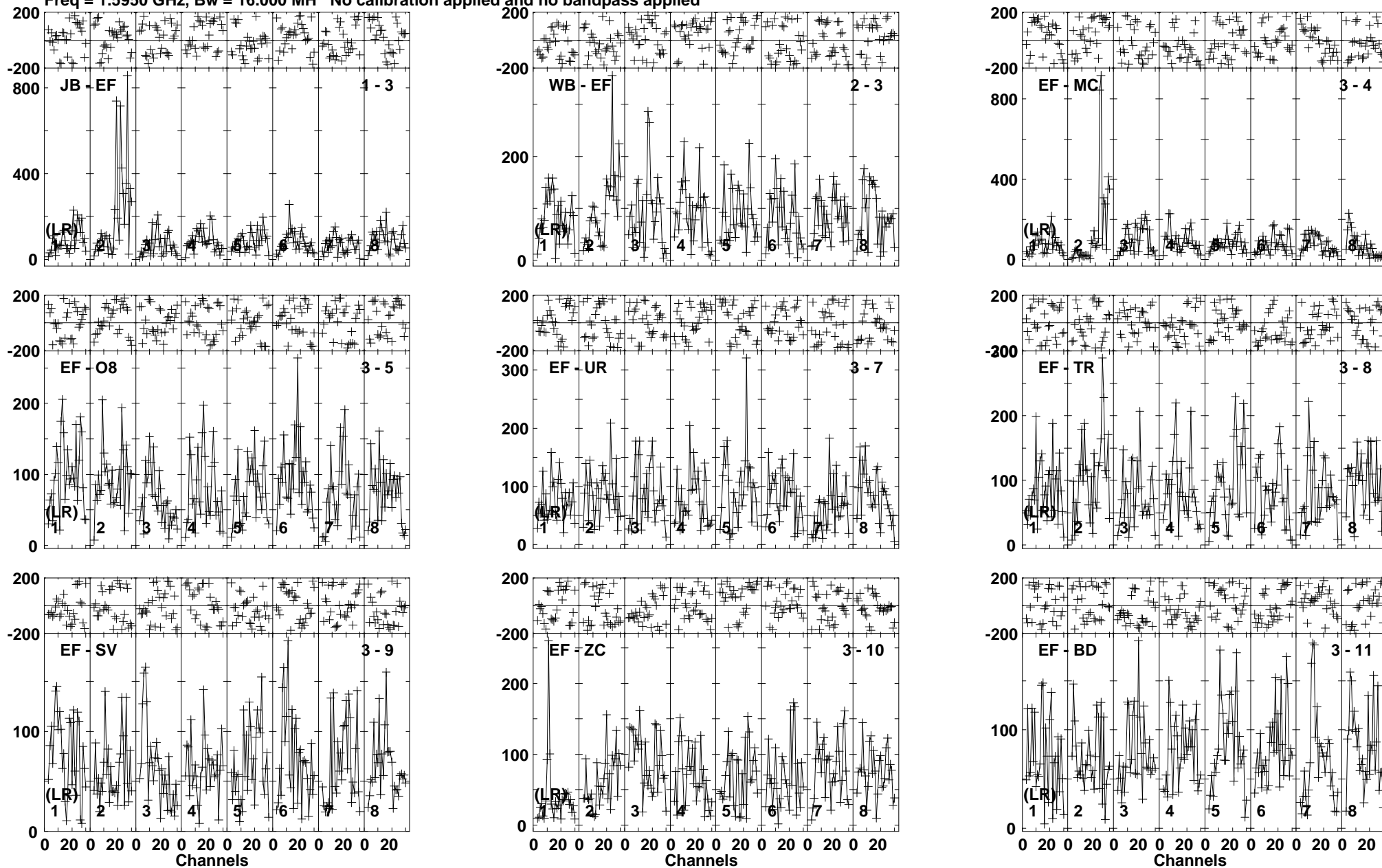
Lower frame: Micro Ampl Jy Top frame: Phas deg Vector averaged cross-power spectrum Baseline: JB (01) - EF (03) Timerange: 00/19:23:11 to 00/19:26:59
