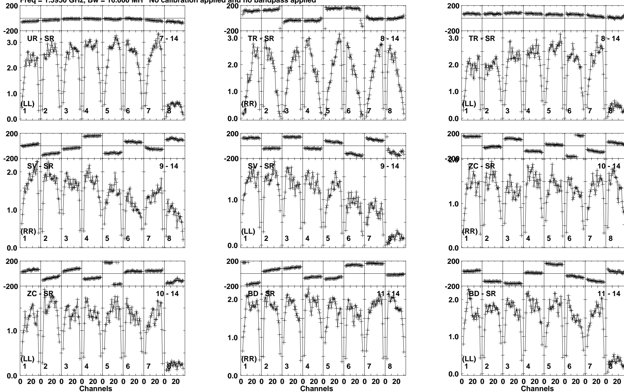
Lower frame: Milli Ampl Jy Top frame: Phas deg Vector averaged cross-power spectrum Baseline: UR (07) - SR (14) Timerange: 00/13:03:21 to 00/13:04:29
