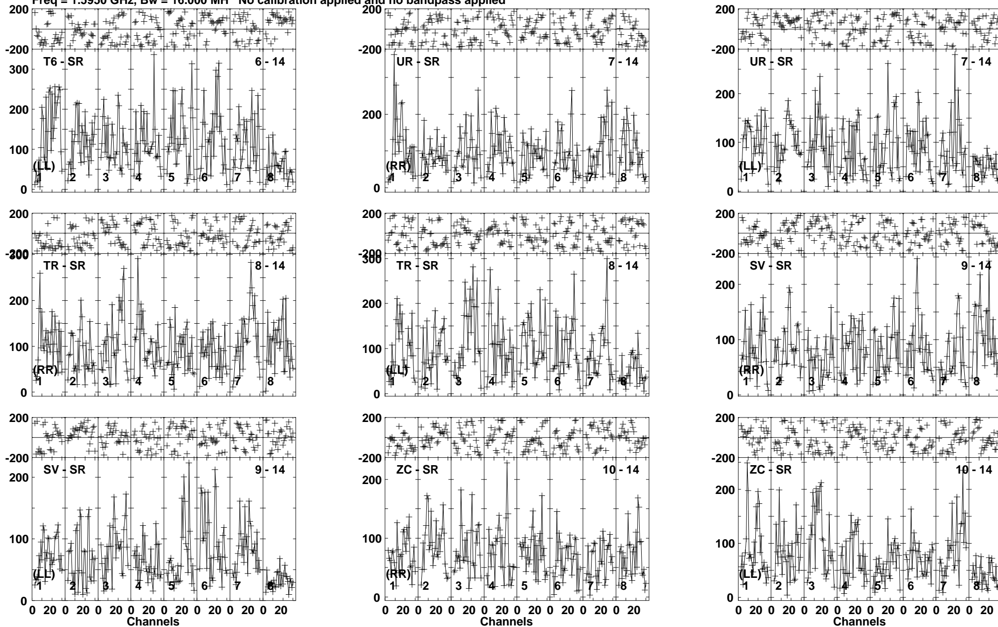
Lower frame: Micro Ampl Jy Top frame: Phas deg Vector averaged cross-power spectrum Baseline: T6 (06) - SR (14) Timerange: 00:12:17:31 to 00:12:21:19
