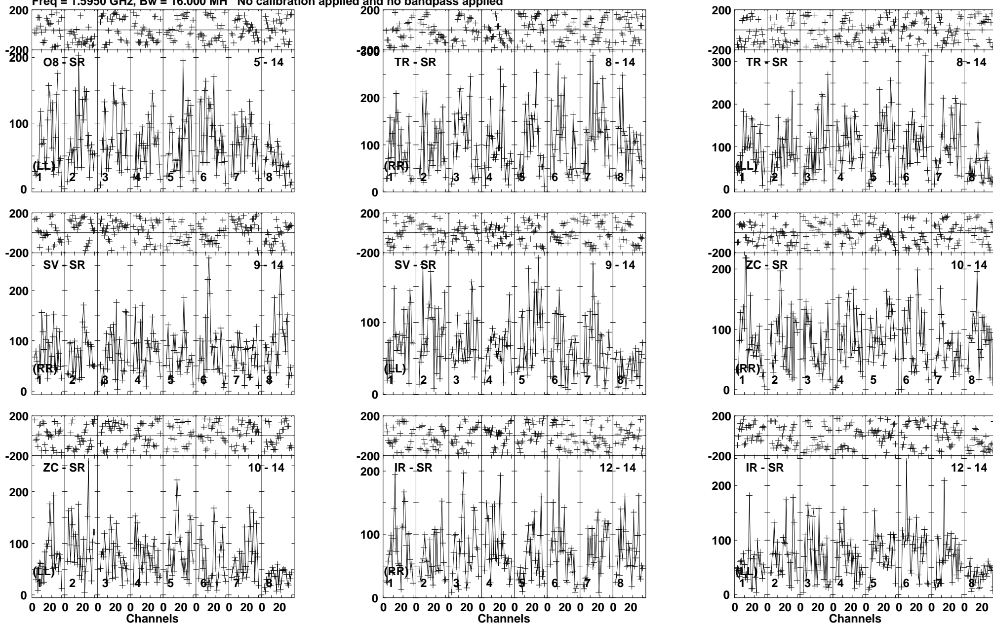
Lower frame: Micro Ampl Jy Top frame: Phas deg Vector averaged cross-power spectrum Baseline: O8 (05) - SR (14) Timerange: 00/15:39:01 to 00/15:42:49
