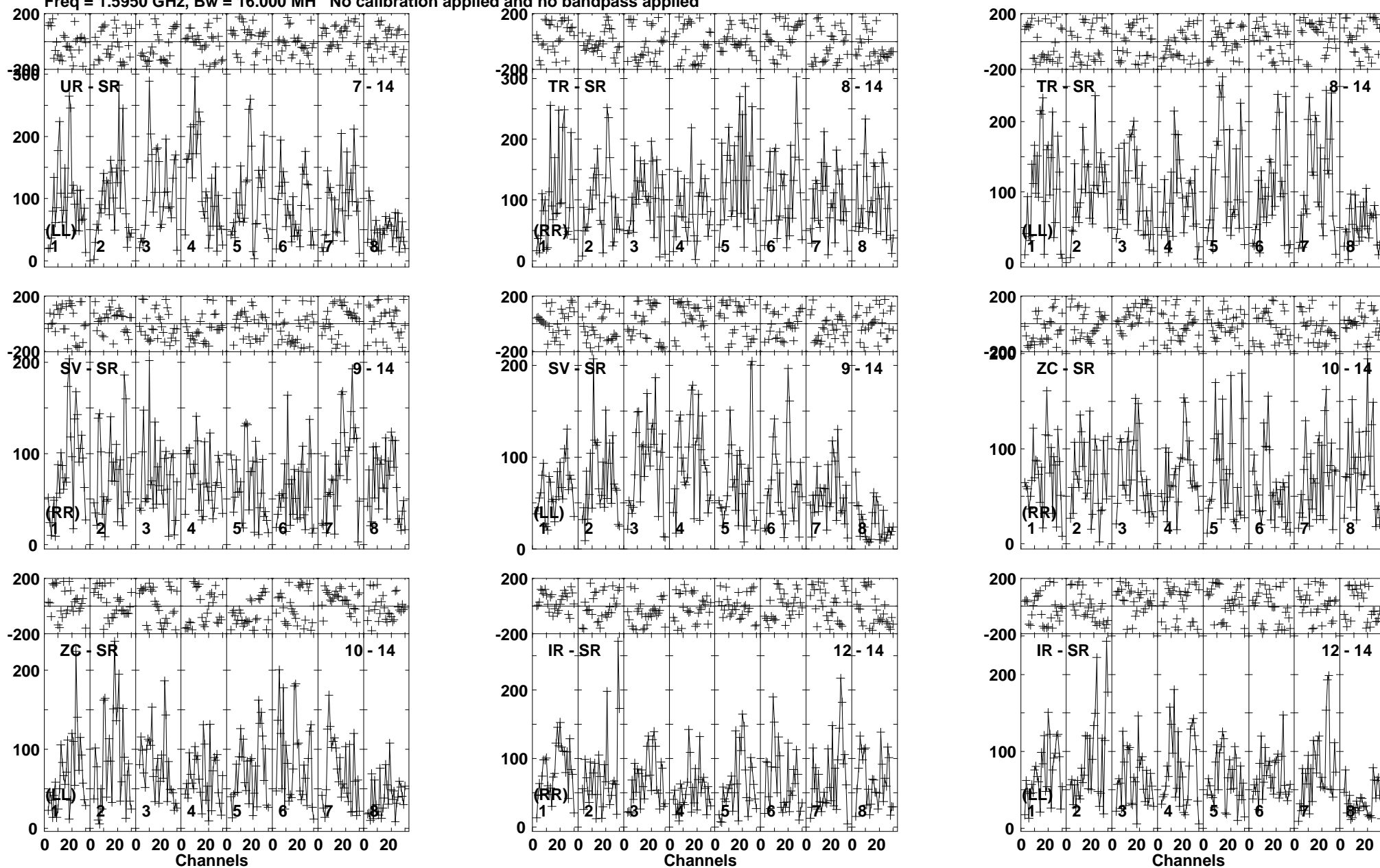
Lower frame: Micro Ampl Jy Top frame: Phas deg Vector averaged cross-power spectrum Baseline: UR (07) - SR (14) Timerange: 00/13:54:01 to 00/13:57:49
