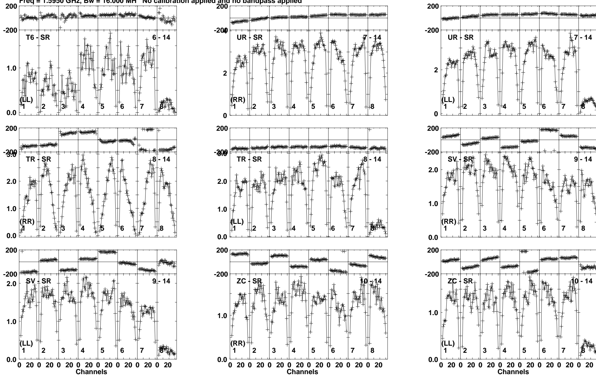
Lower frame: Milli Ampl Jy Top frame: Phas deg Vector averaged cross-power spectrum Baseline: T6 (06) - SR (14) Timerange: 00/12:00:21 to 00/12:01:29
