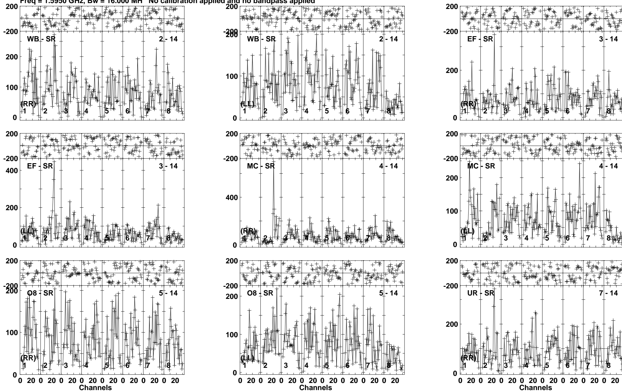
Lower frame: Micro Ampl Jy Top frame: Phas deg Vector averaged cross-power spectrum Baseline: WB (02) - SR (14) Timerange: 00/13:54:01 to 00/13:57:49
