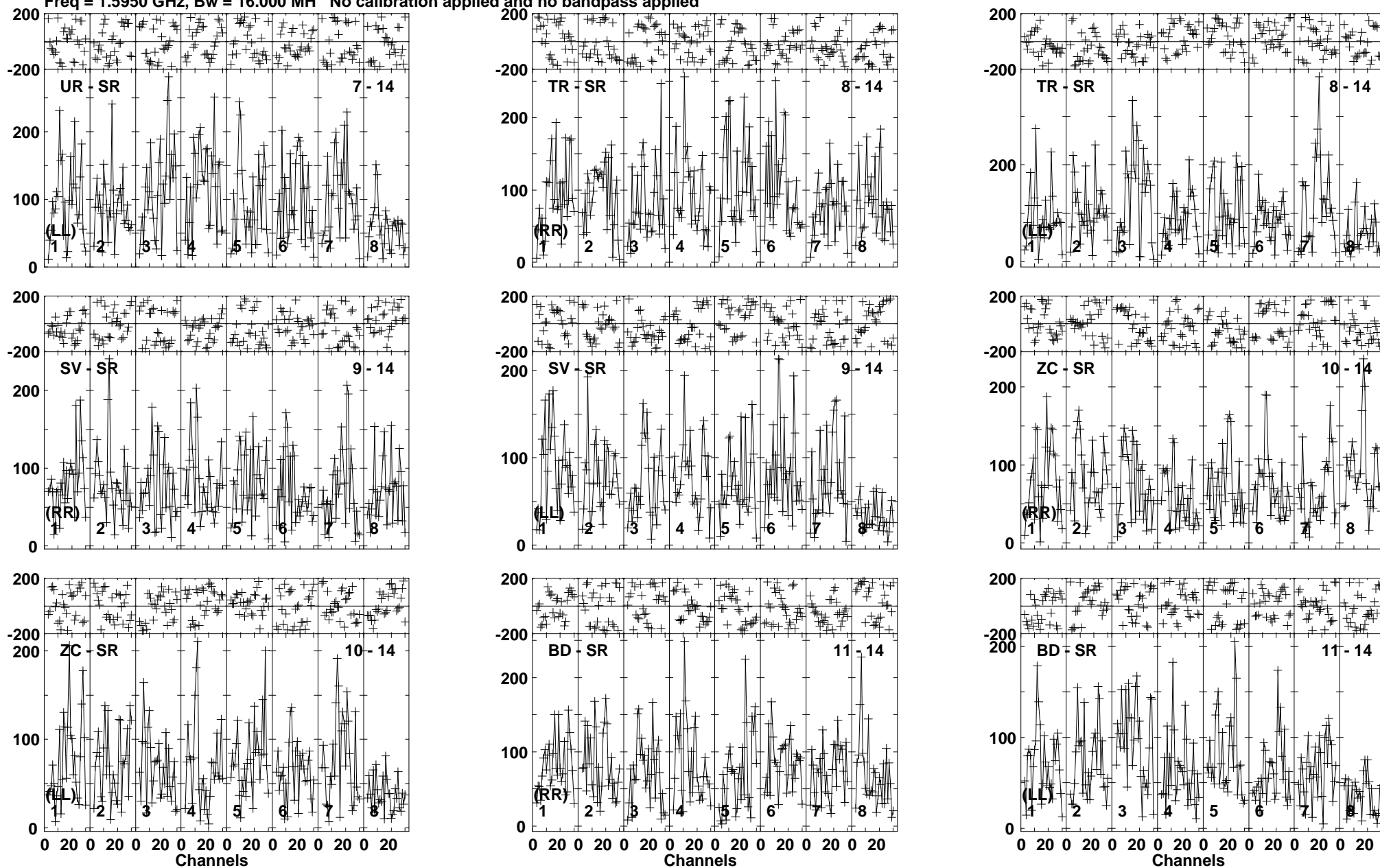
Lower frame: Micro Ampl Jy Top frame: Phas deg Vector averaged cross-power spectrum Baseline: UR (07) - SR (14) Timerange: 00:12:38:31 to 00:12:42:19
