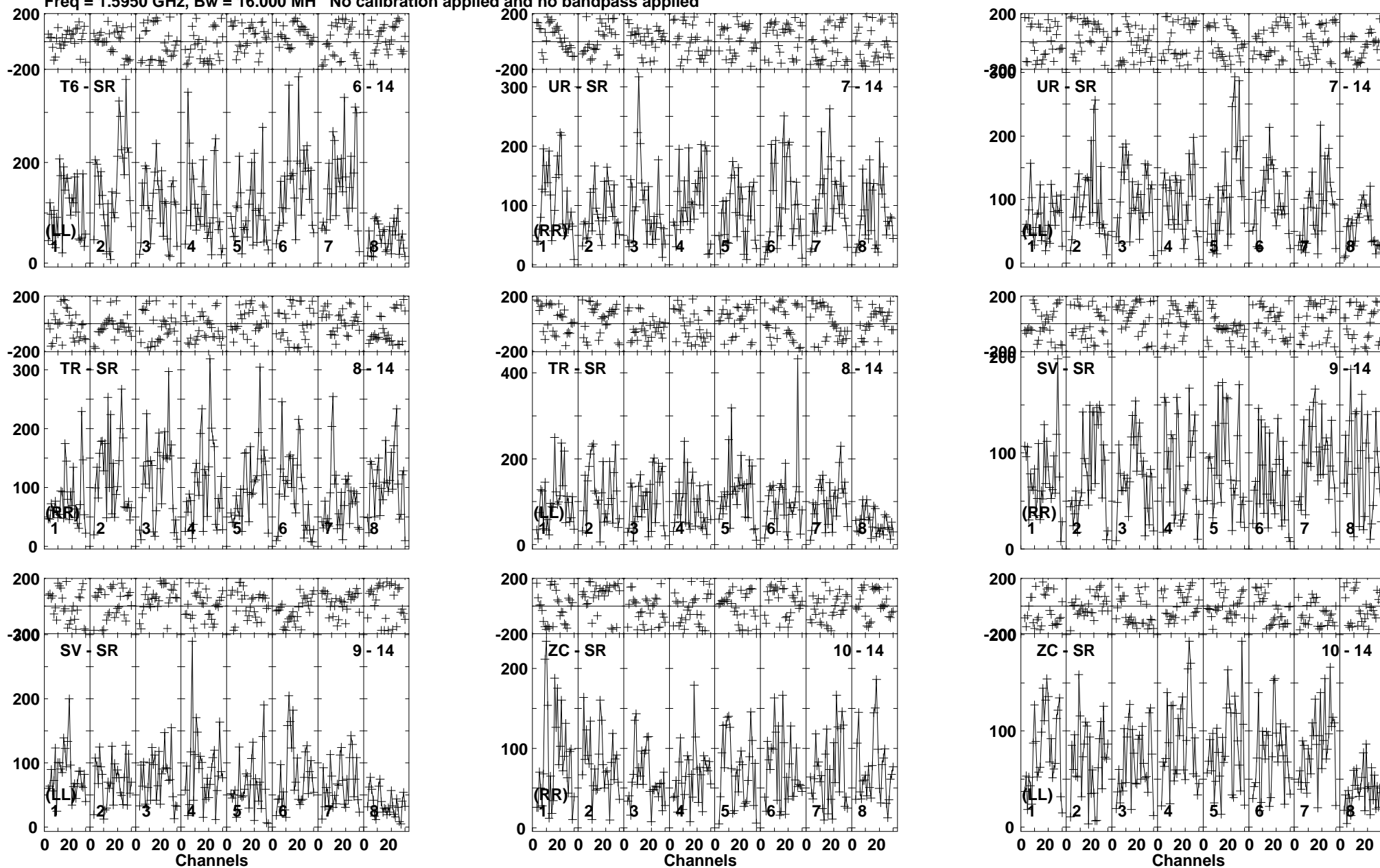
Lower frame: Micro Ampl Jy Top frame: Phas deg Vector averaged cross-power spectrum Baseline: T6 (06) - SR (14) Timerange: 00:12:12:01 to 00:12:15:49
