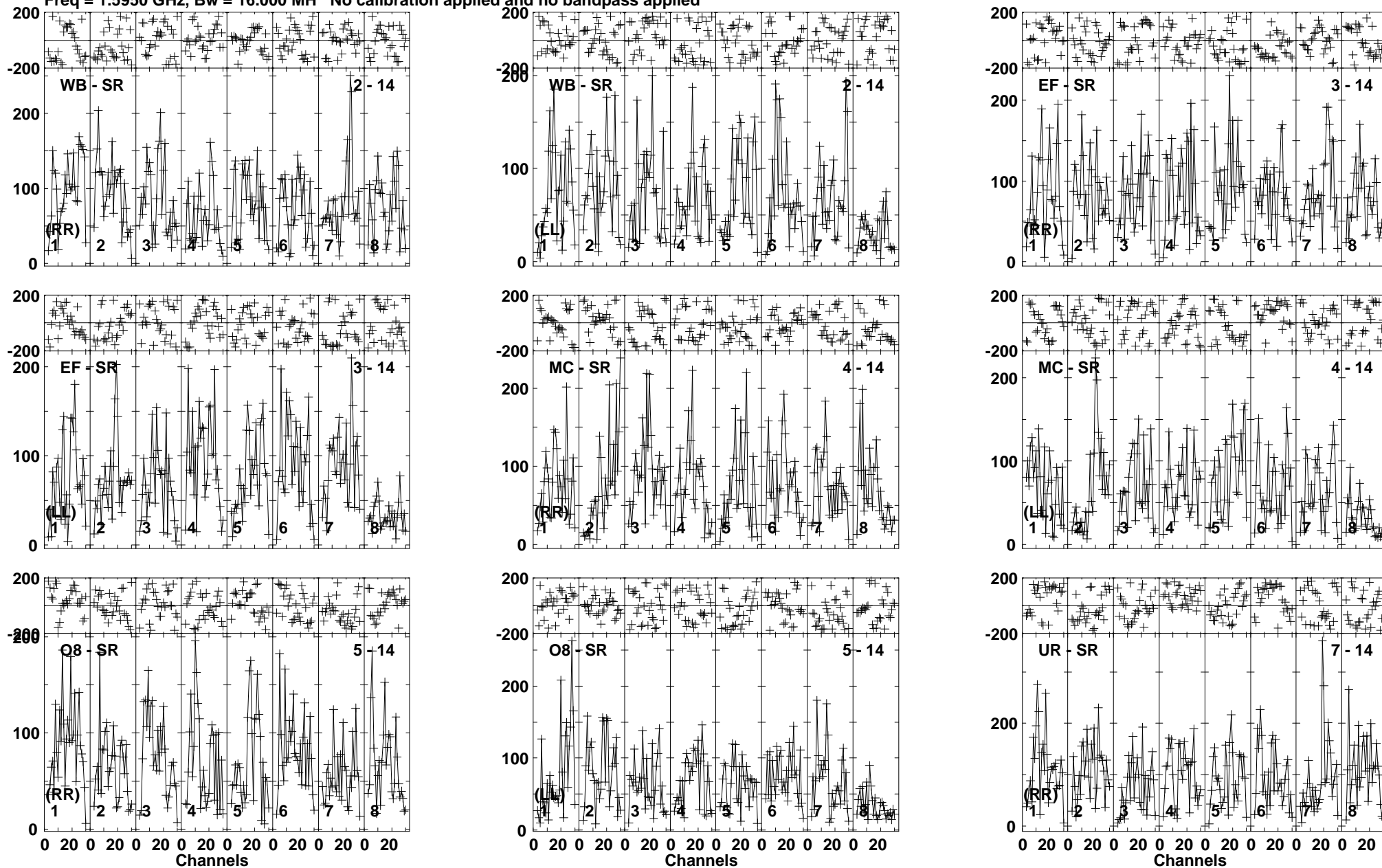
Lower frame: Micro Ampl Jy Top frame: Phas deg Vector averaged cross-power spectrum Baseline: WB (02) - SR (14) Timerange: 00/12:59:31 to 00/13:03:19
