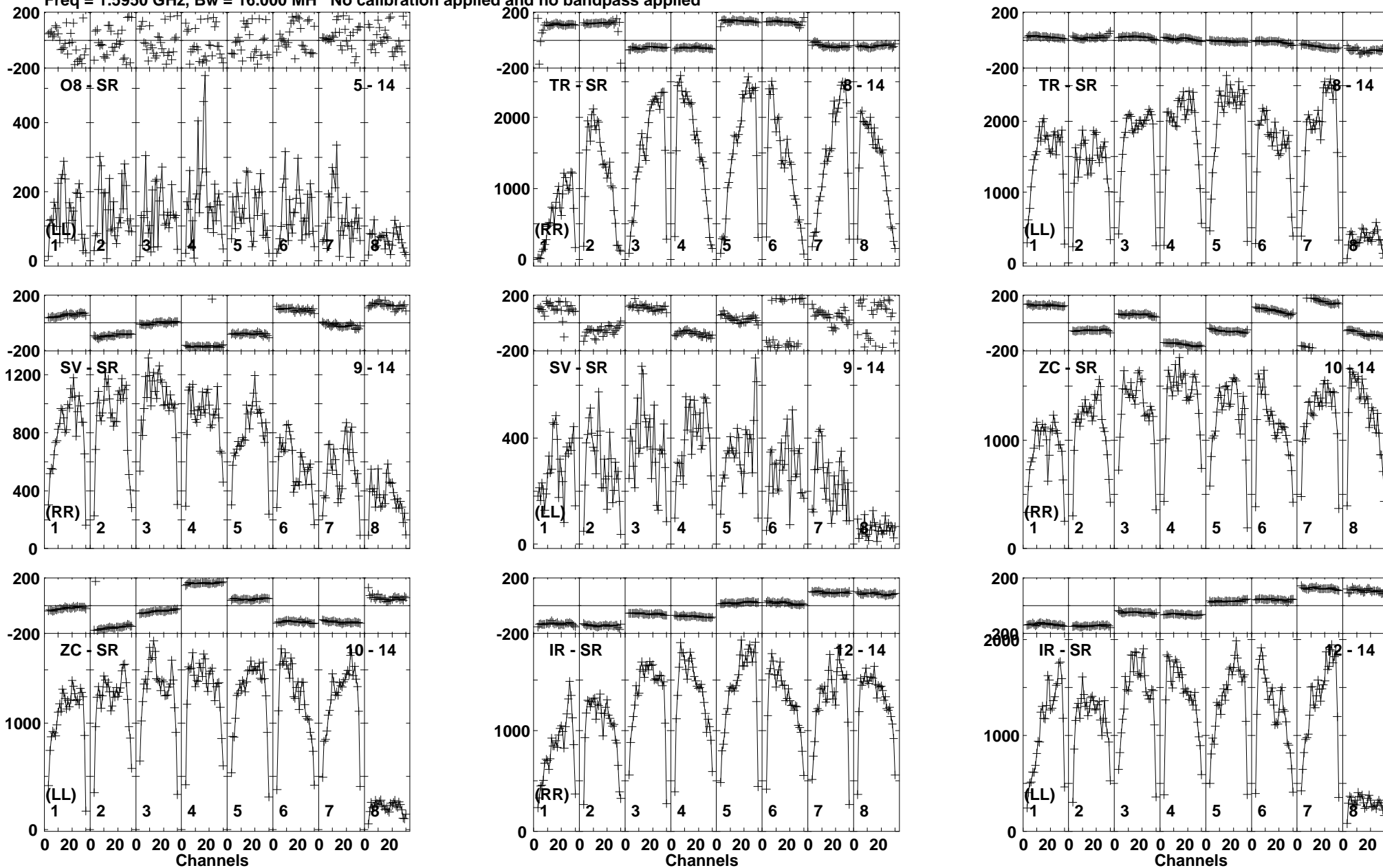
Lower frame: Micro Ampl Jy Top frame: Phas deg Vector averaged cross-power spectrum Baseline: O8 (05) - SR (14) Timerange: 00/16:42:51 to 00/16:43:59
