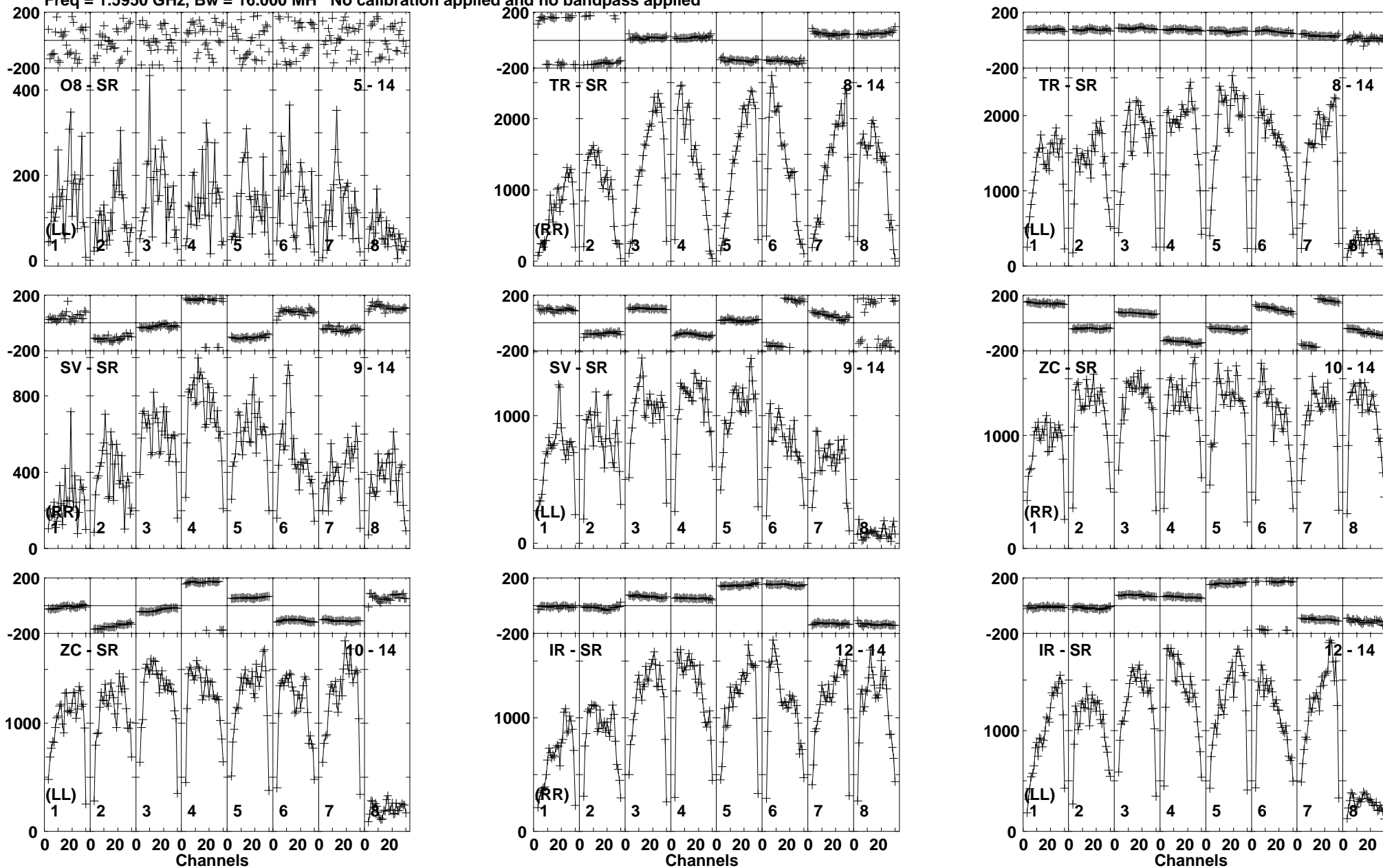
Lower frame: Micro Ampl Jy Top frame: Phas deg Vector averaged cross-power spectrum Baseline: O8 (05) - SR (14) Timerange: 00/17:03:51 to 00/17:04:59
