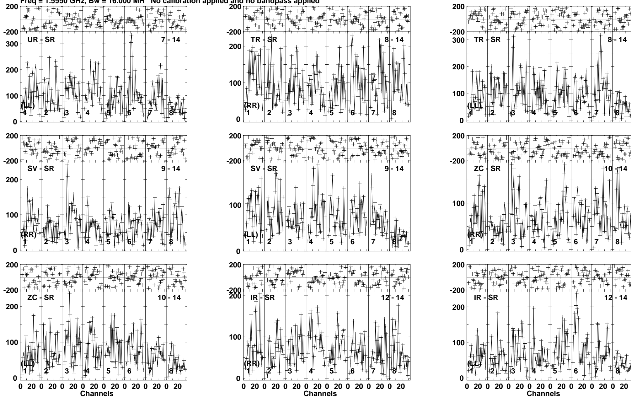
Lower frame: Micro Ampl Jy Top frame: Phas deg Vector averaged cross-power spectrum Baseline: UR (07) - SR (14) Timerange: 00/13:17:01 to 00/13:20:49
