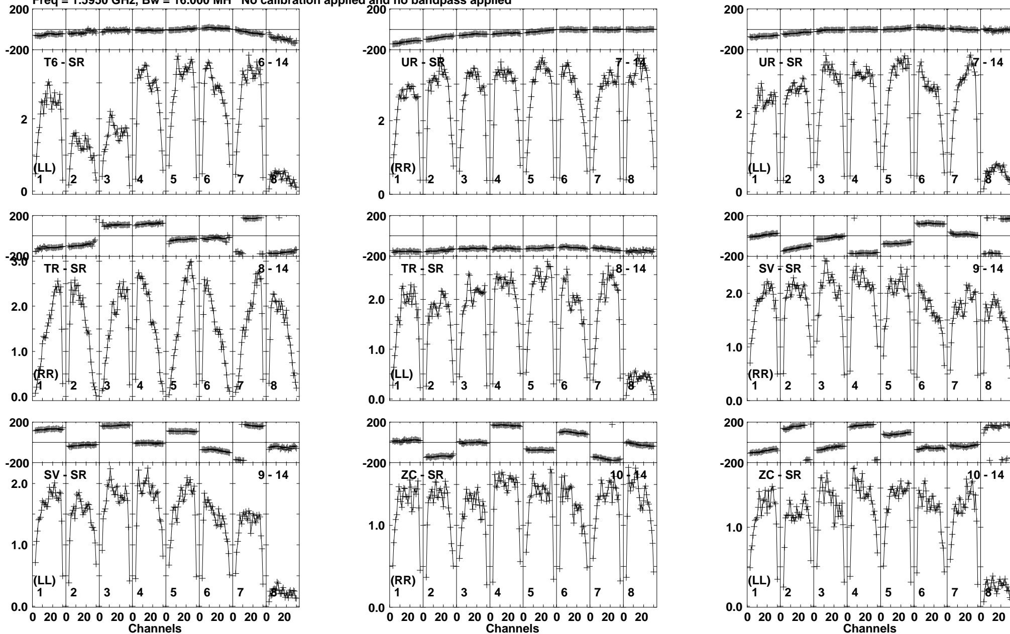
Lower frame: Milli Ampl Jy Top frame: Phas deg Vector averaged cross-power spectrum Baseline: T6 (06) - SR (14) Timerange: 00/11:55:21 to 00/11:56:29
