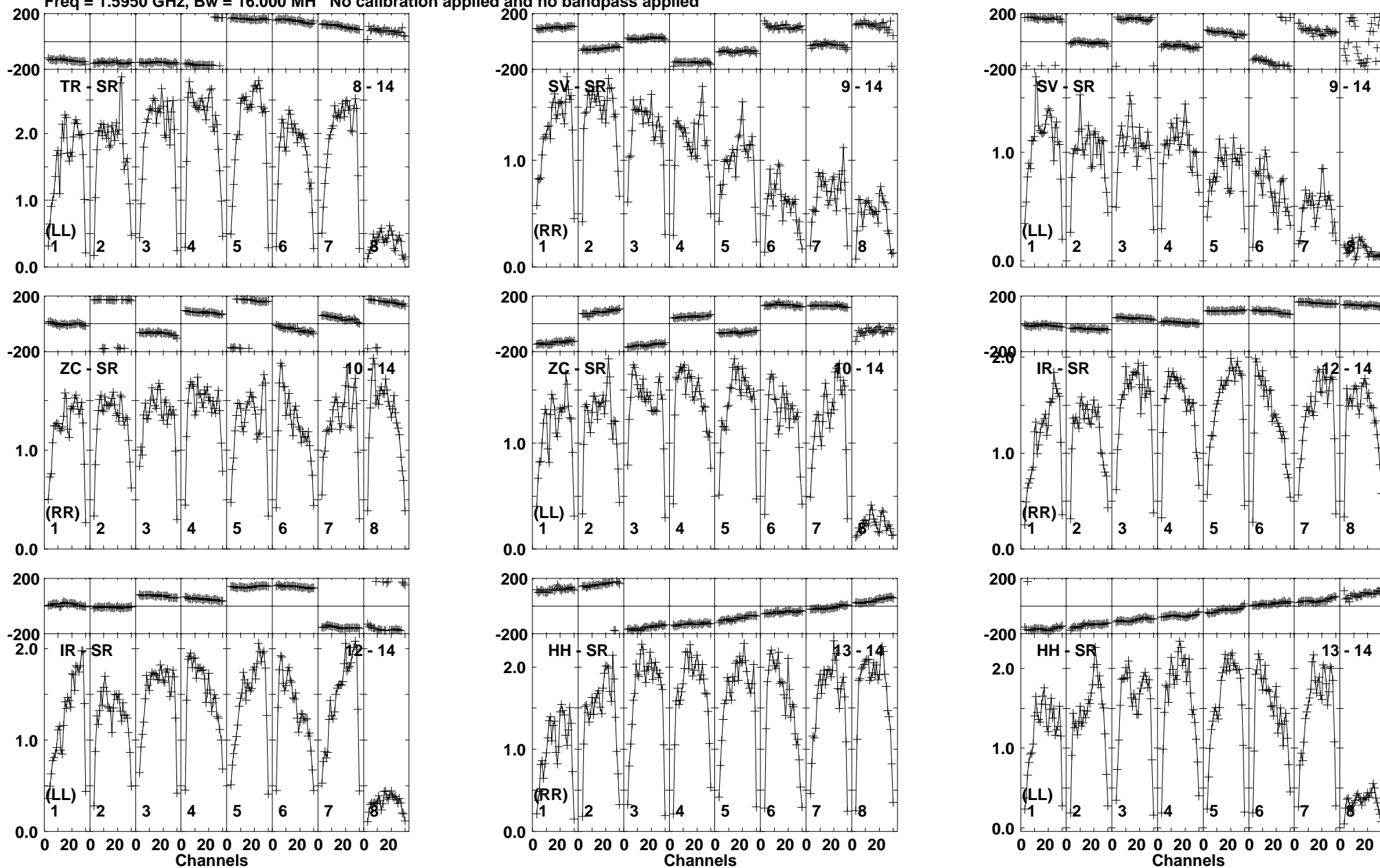
Lower frame: Milli Ampl Jy Top frame: Phas deg Vector averaged cross-power spectrum Baseline: TR (08) - SR (14) Timerange: 00/15:32:21 to 00/15:33:29
