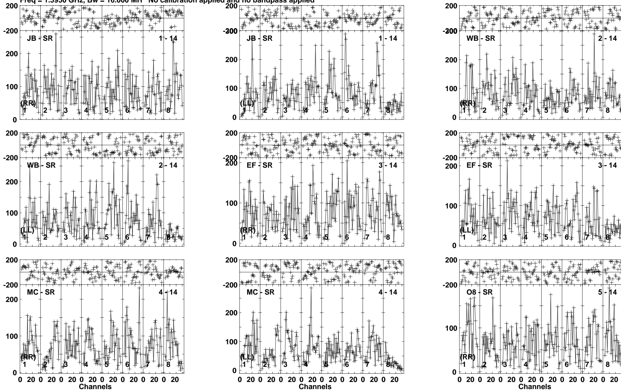
Lower frame: Micro Ampl Jy Top frame: Phas deg Vector averaged cross-power spectrum Baseline: JB (01) - SR (14) Timerange: 00/15:33:31 to 00/15:37:19
