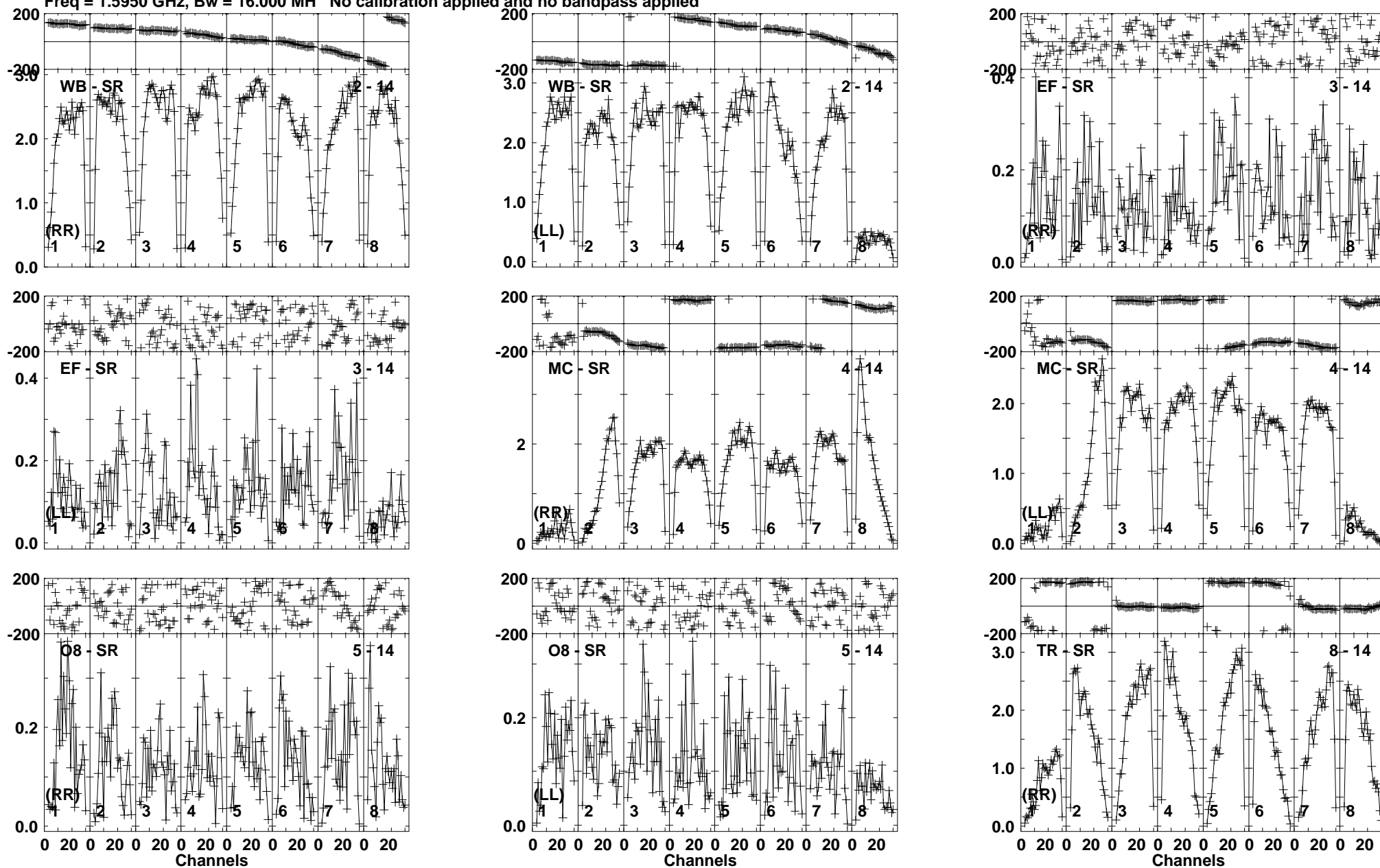
Lower frame: Milli Ampl Jy Top frame: Phas deg Vector averaged cross-power spectrum Baseline: WB (02) - SR (14) Timerange: 00/15:11:21 to 00/15:12:29
