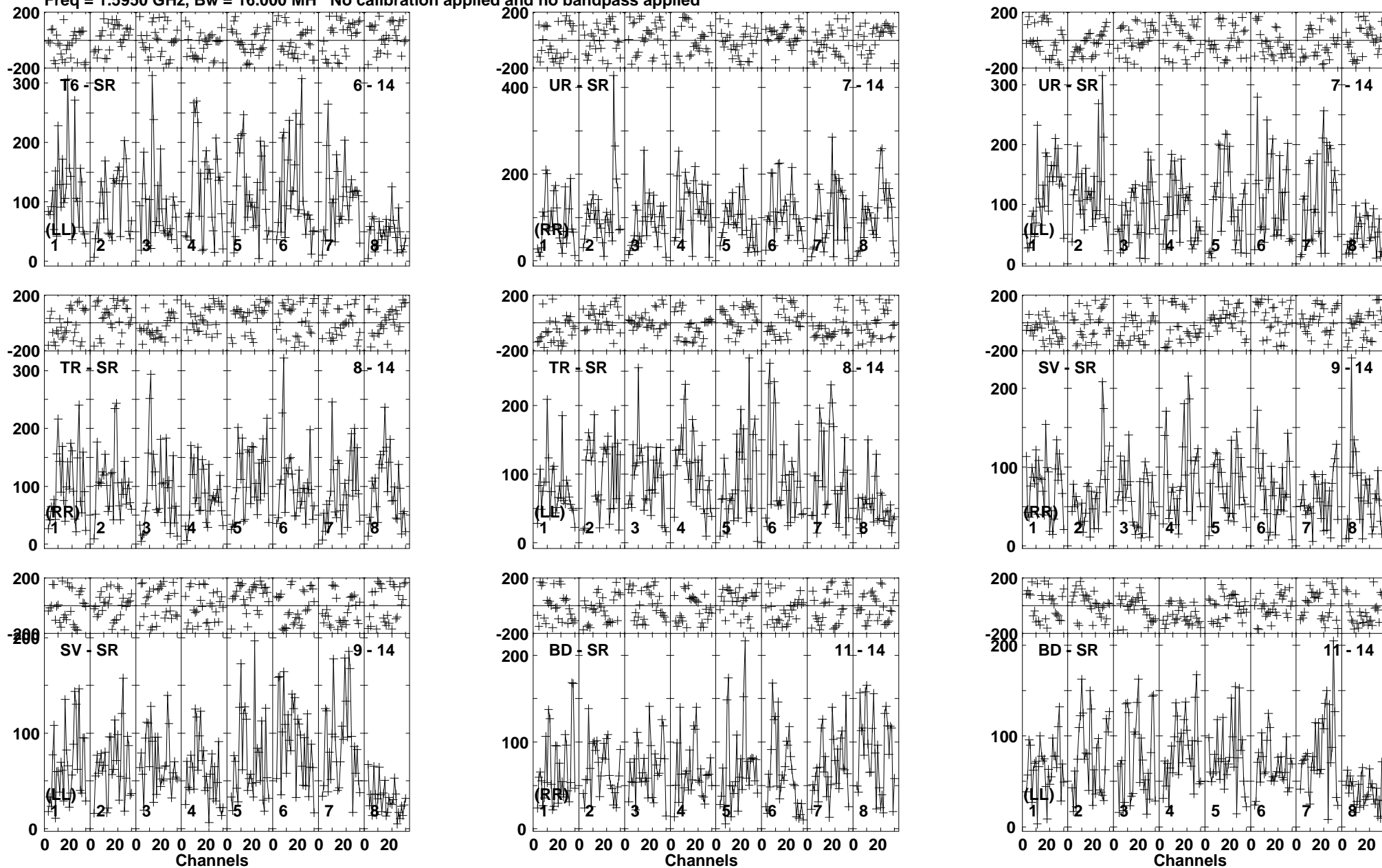
Lower frame: Micro Ampl Jy Top frame: Phas deg Vector averaged cross-power spectrum Baseline: T6 (06) - SR (14) Timerange: 00/11:30:01 to 00/11:33:49
