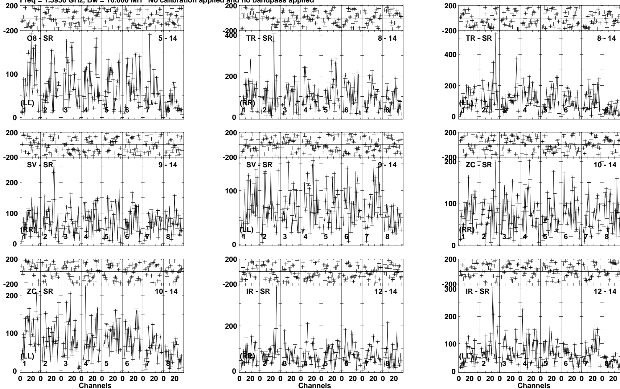
Lower frame: Micro Ampl Jy Top frame: Phas deg Vector averaged cross-power spectrum Baseline: O8 (05) - SR (14) Timerange: 00/16:23:01 to 00/16:26:49
