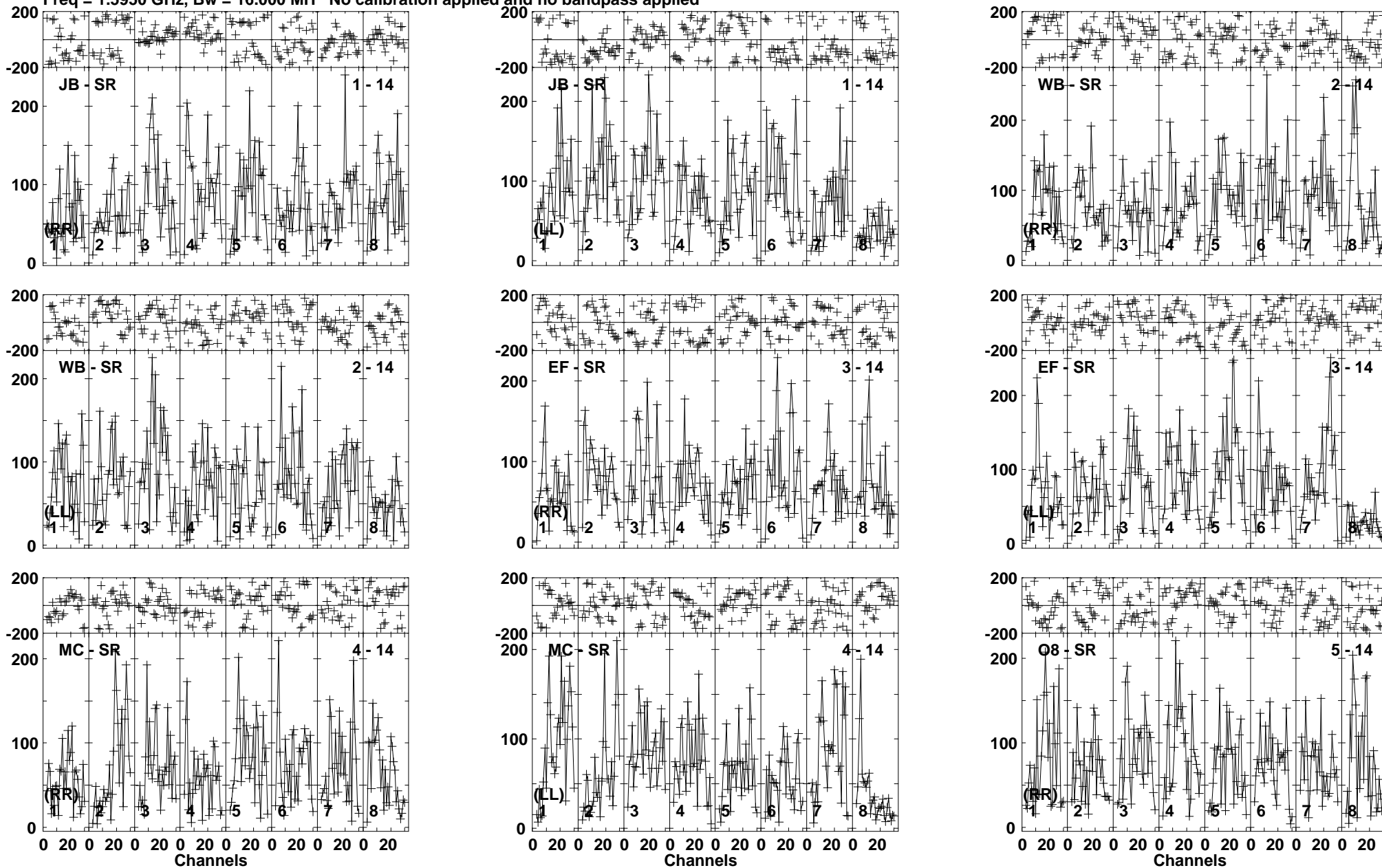
Lower frame: Micro Ampl Jy Top frame: Phas deg Vector averaged cross-power spectrum Baseline: JB (01) - SR (14) Timerange: 00/17:10:01 to 00/17:13:49
