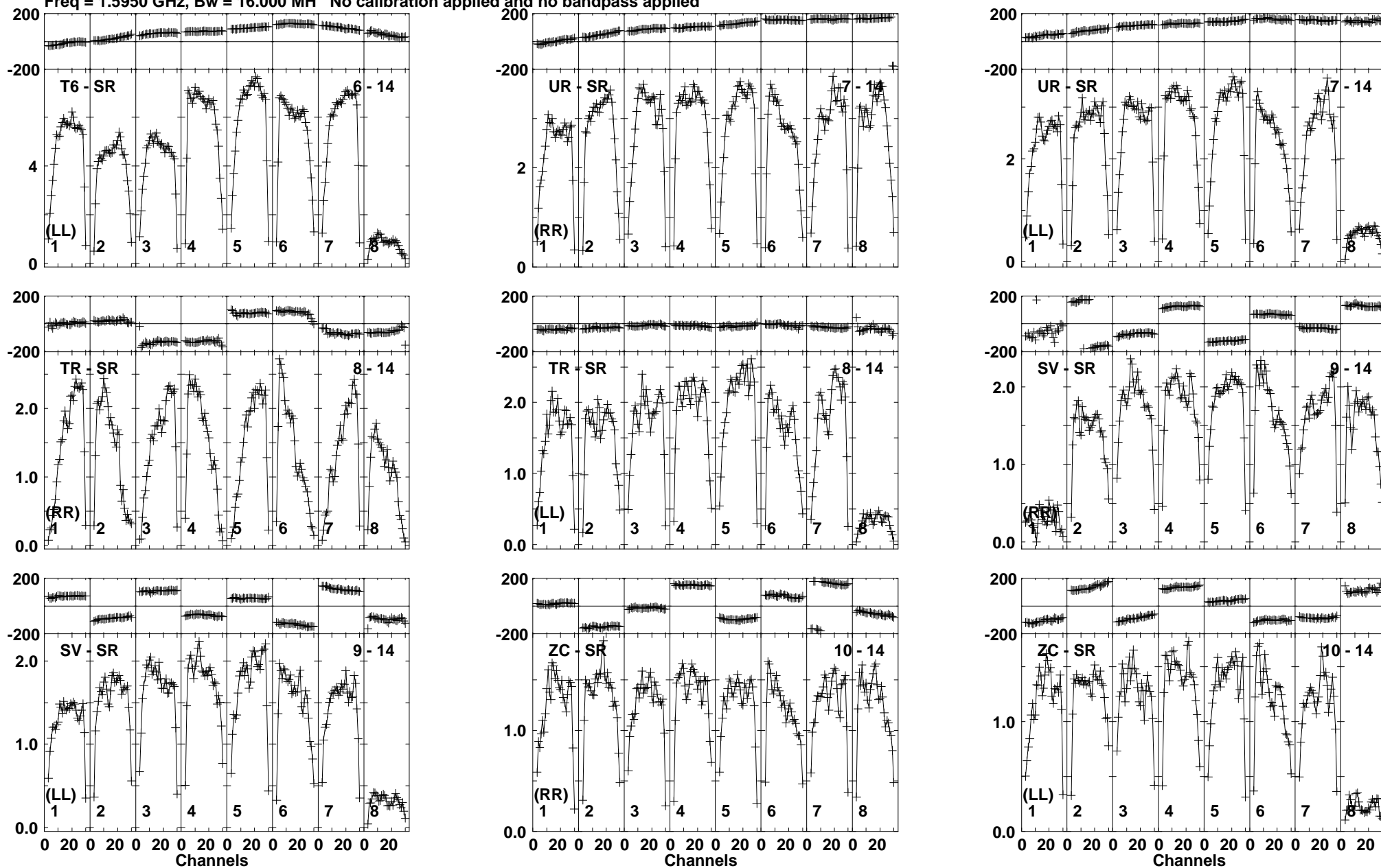
Lower frame: Milli Ampl Jy Top frame: Phas deg Vector averaged cross-power spectrum Baseline: T6 (06) - SR (14) Timerange: 00/10:41:51 to 00/10:42:59
