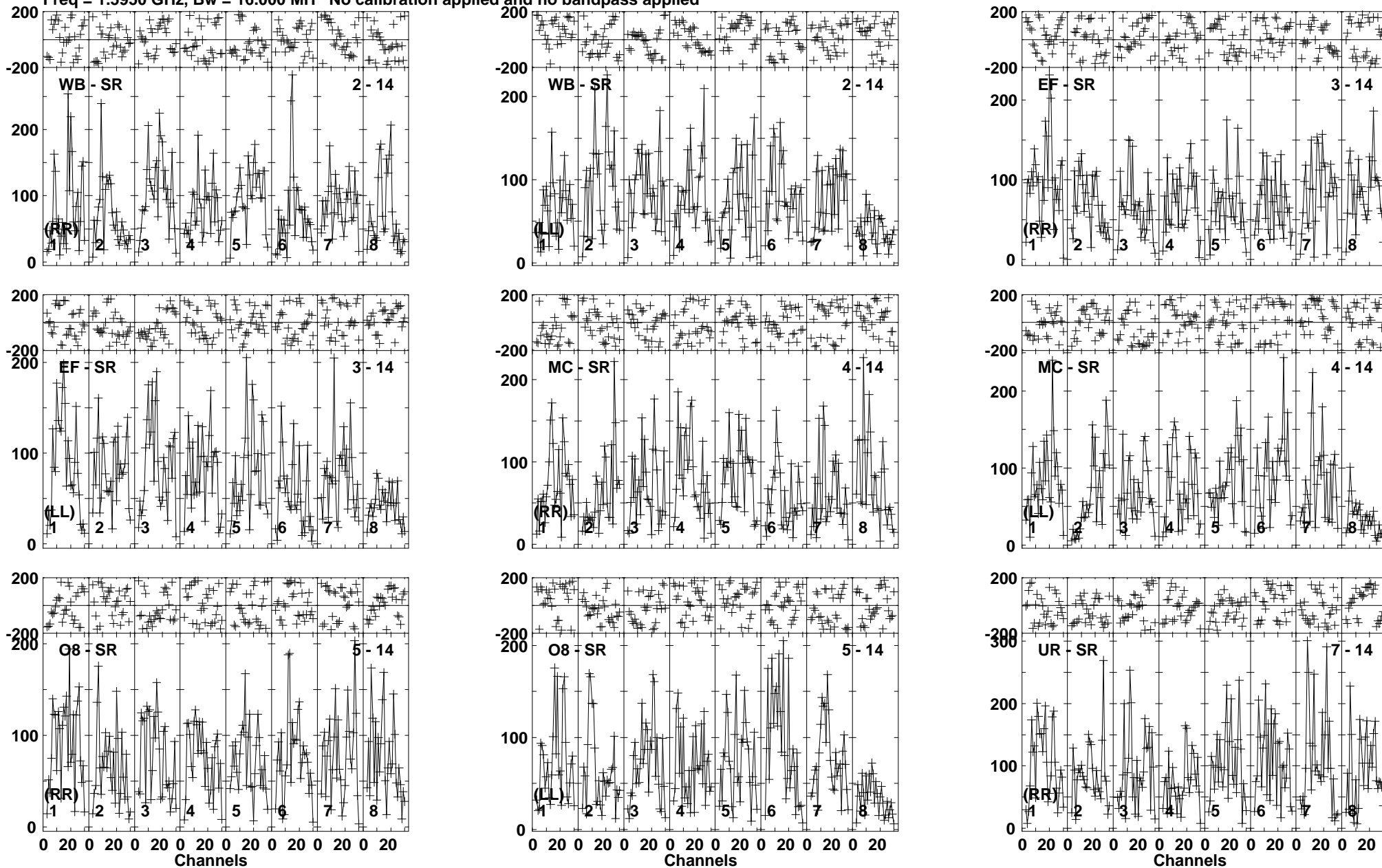
Lower frame: Micro Ampl Jy Top frame: Phas deg Vector averaged cross-power spectrum Baseline: WB (02) - SR (14) Timerange: 00/13:22:31 to 00/13:26:19
