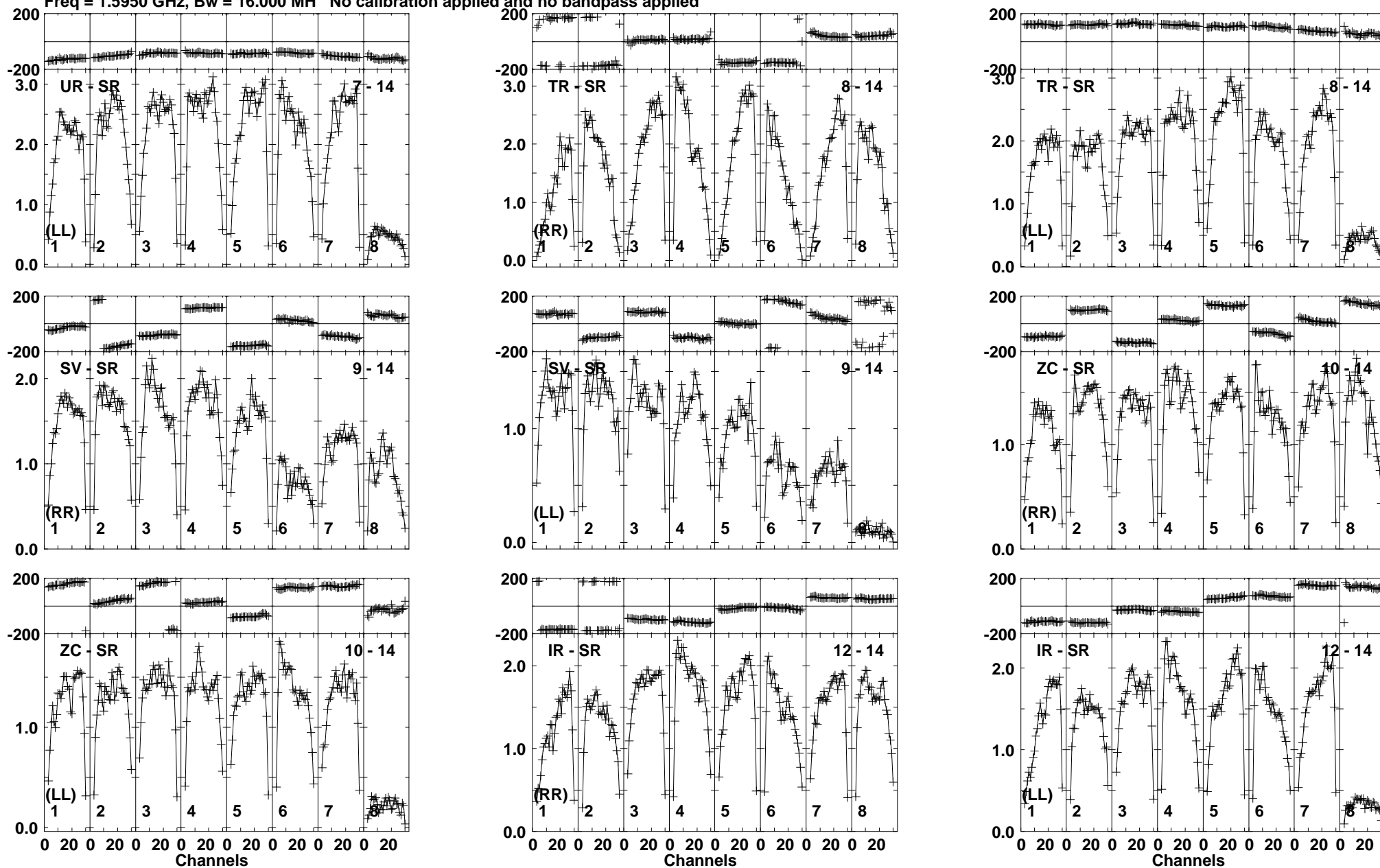
Lower frame: Milli Ampl Jy Top frame: Phas deg Vector averaged cross-power spectrum Baseline: UR (07) - SR (14) Timerange: 00/13:31:51 to 00/13:32:59
