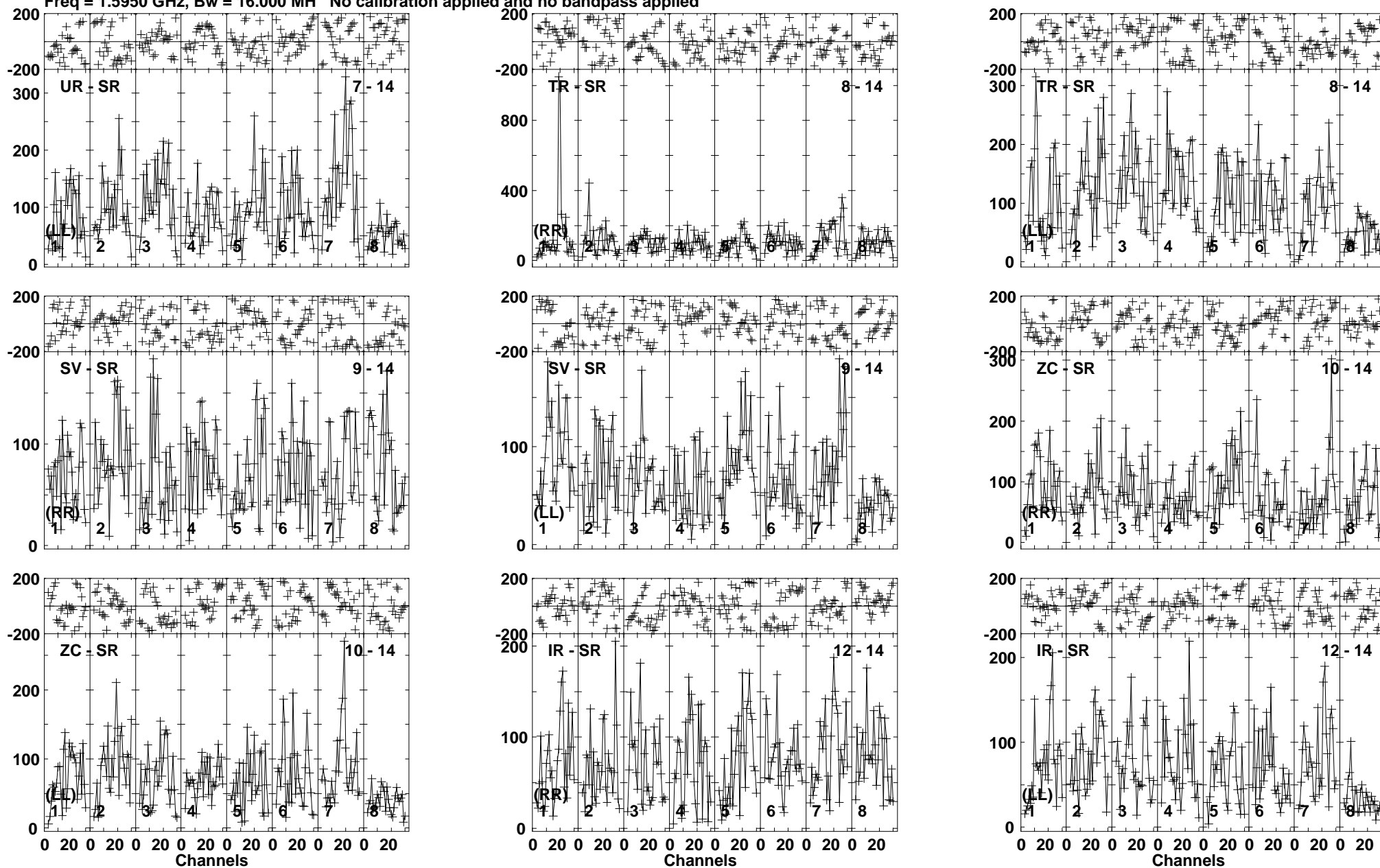
Lower frame: Micro Ampl Jy Top frame: Phas deg Vector averaged cross-power spectrum Baseline: UR (07) - SR (14) Timerange: 00/13:33:01 to 00/13:36:49
