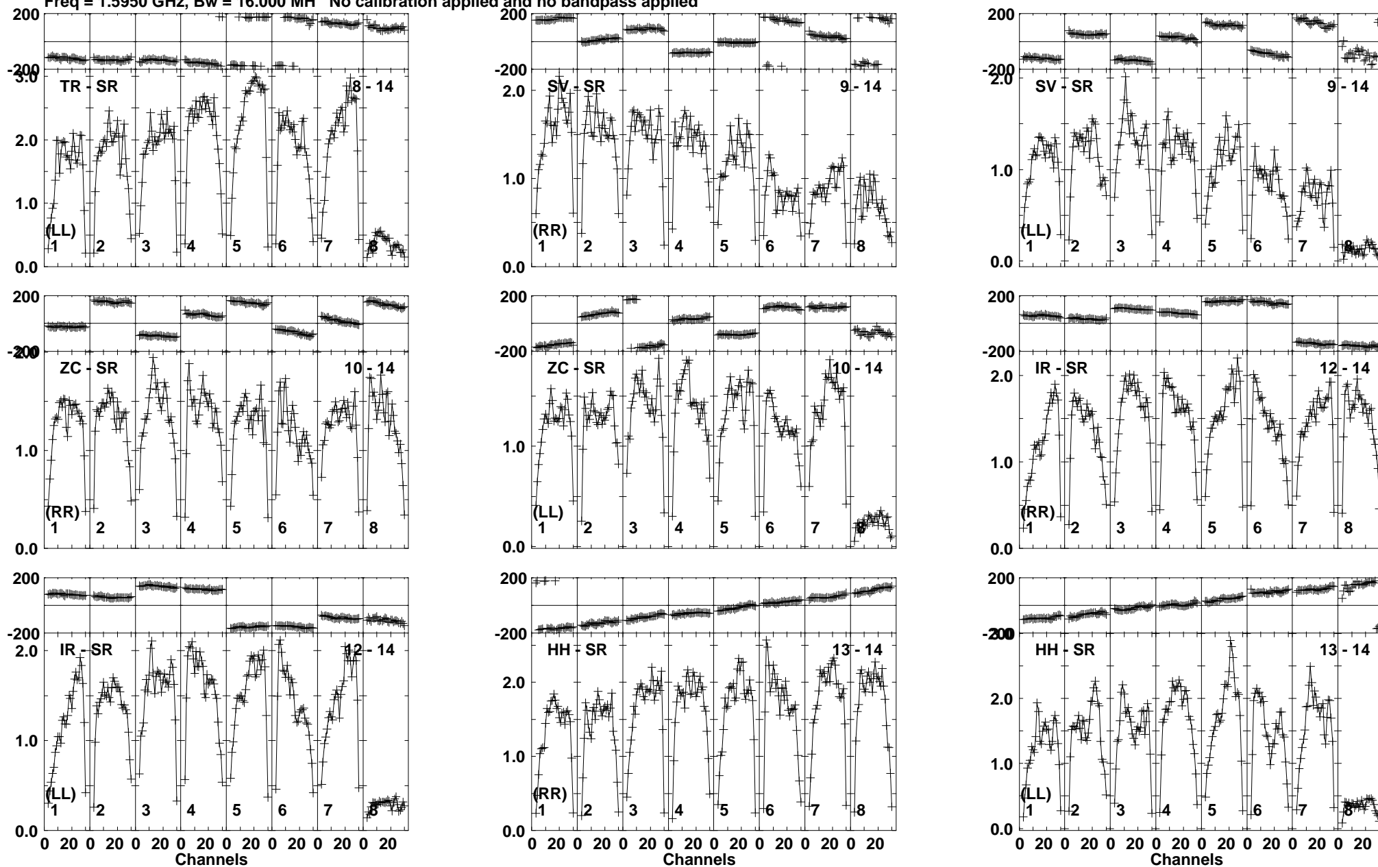
Lower frame: Milli Ampl Jy Top frame: Phas deg Vector averaged cross-power spectrum Baseline: TR (08) - SR (14) Timerange: 00/15:21:51 to 00/15:22:59
