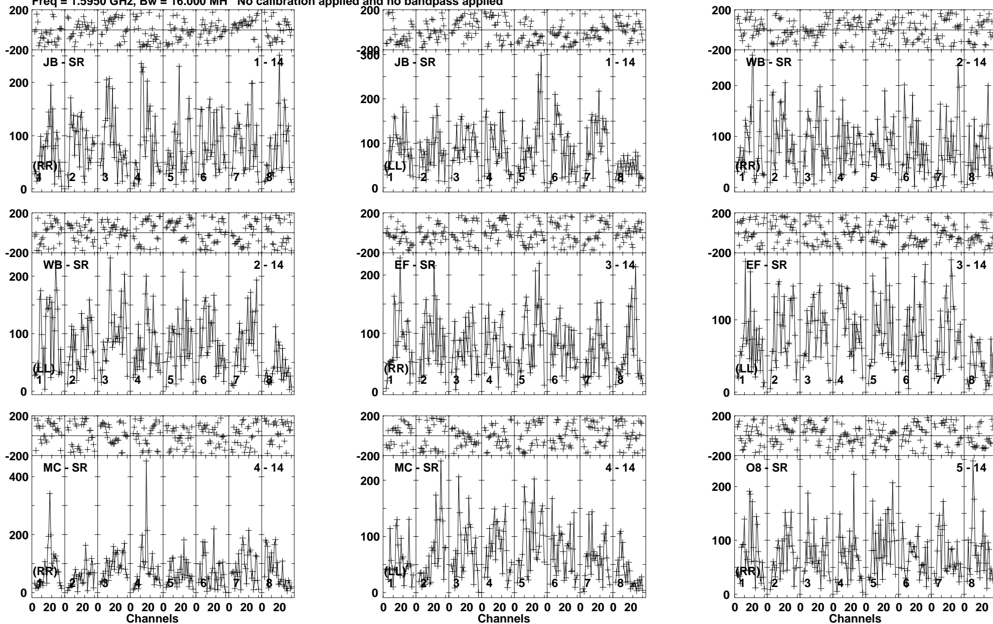
Lower frame: Micro Ampl Jy Top frame: Phas deg Vector averaged cross-power spectrum Baseline: JB (01) - SR (14) Timerange: 00/17:05:01 to 00/17:08:49
