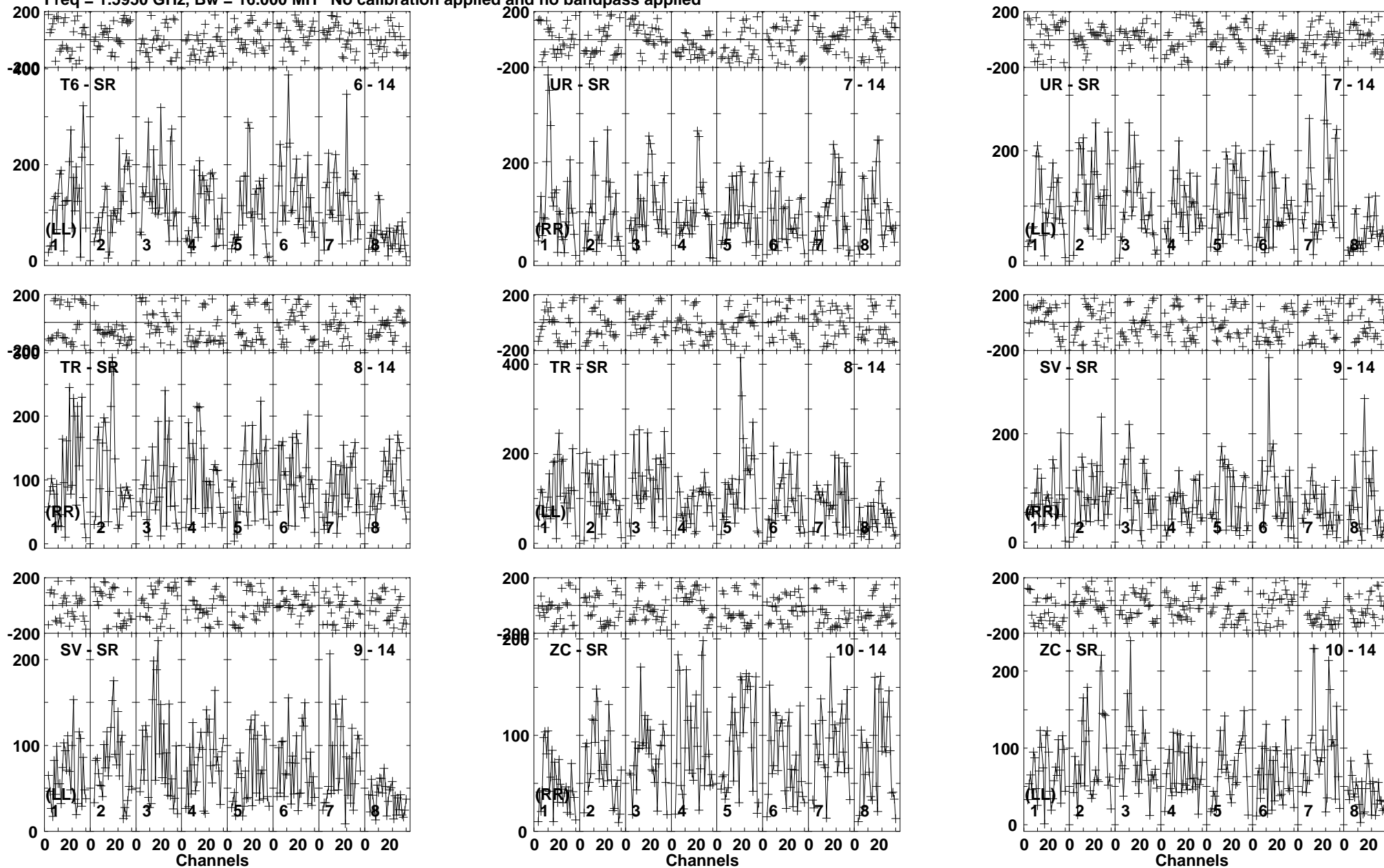
Lower frame: Micro Ampl Jy Top frame: Phas deg Vector averaged cross-power spectrum Baseline: T6 (06) - SR (14) Timerange: 00/11:46:01 to 00/11:49:49
