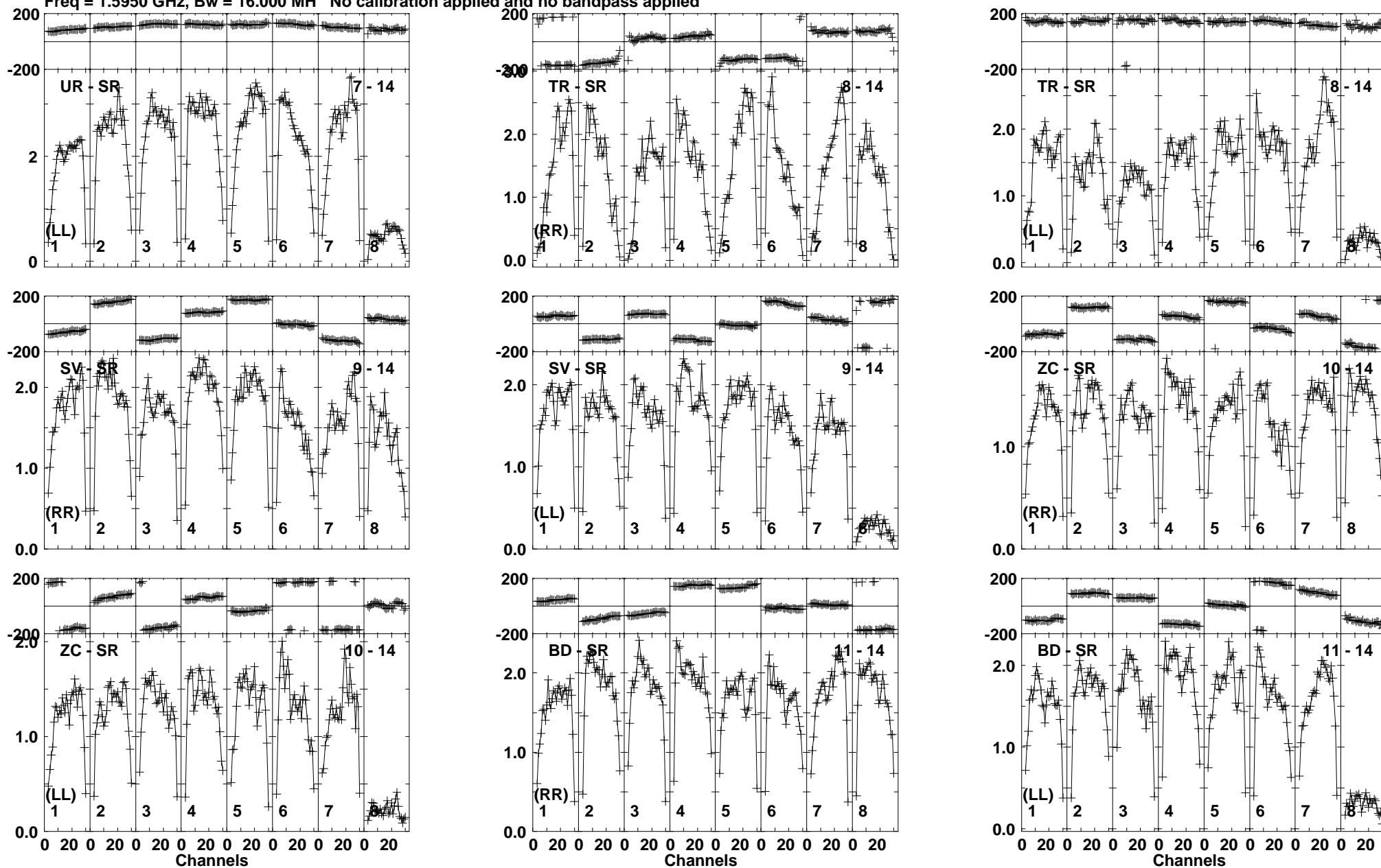
Lower frame: Milli Ampl Jy Top frame: Phas deg Vector averaged cross-power spectrum Baseline: UR (07) - SR (14) Timerange: 00:12:42:21 to 00:12:43:29
