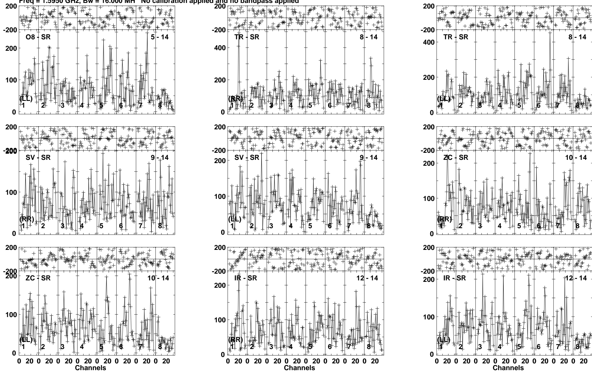
Lower frame: Micro Ampl Jy Top frame: Phas deg Vector averaged cross-power spectrum Baseline: O8 (05) - SR (14) Timerange: 00/16:38:31 to 00/16:42:19
