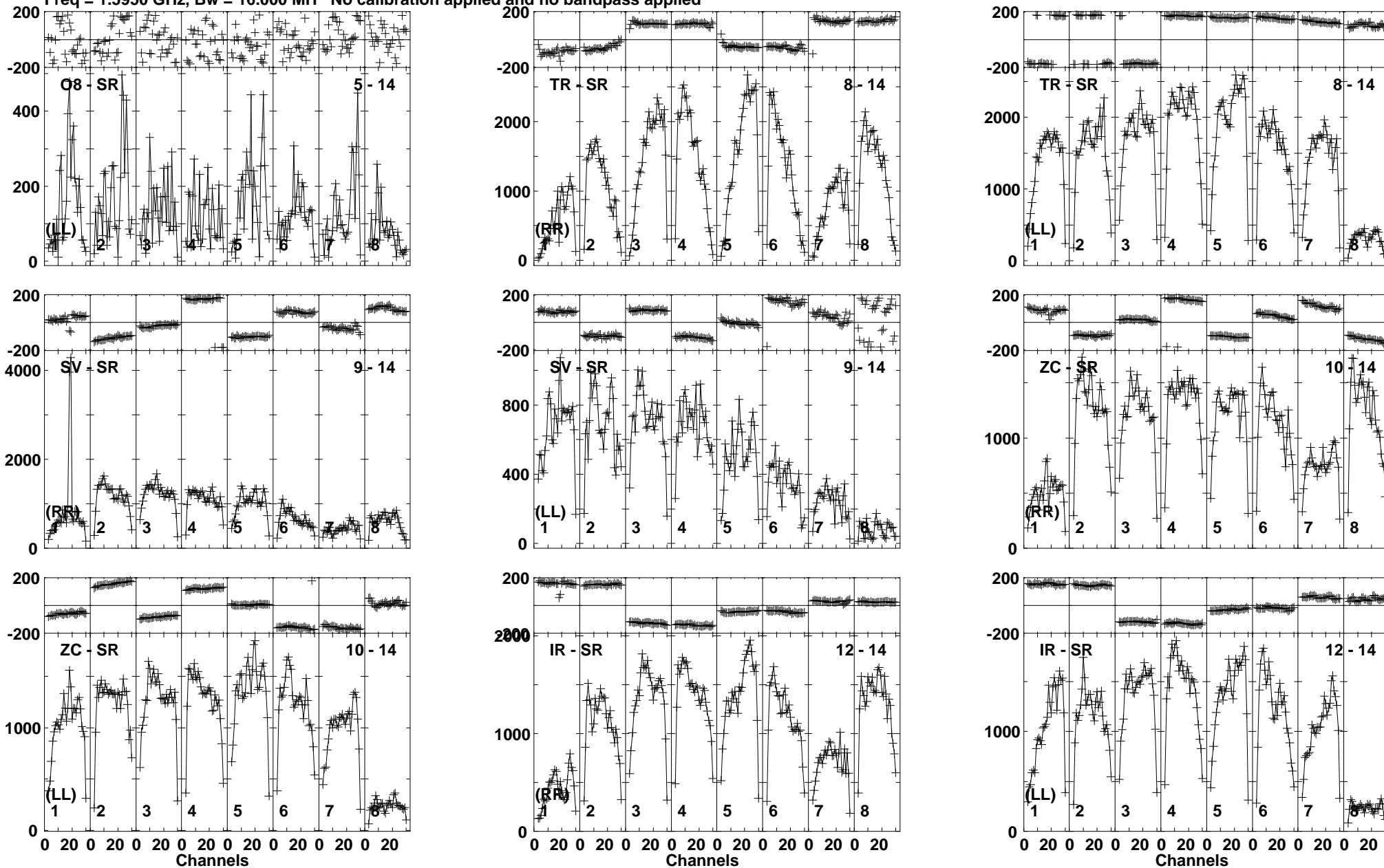
Lower frame: Micro Ampl Jy Top frame: Phas deg Vector averaged cross-power spectrum Baseline: O8 (05) - SR (14) Timerange: 00/16:53:21 to 00/16:54:29
