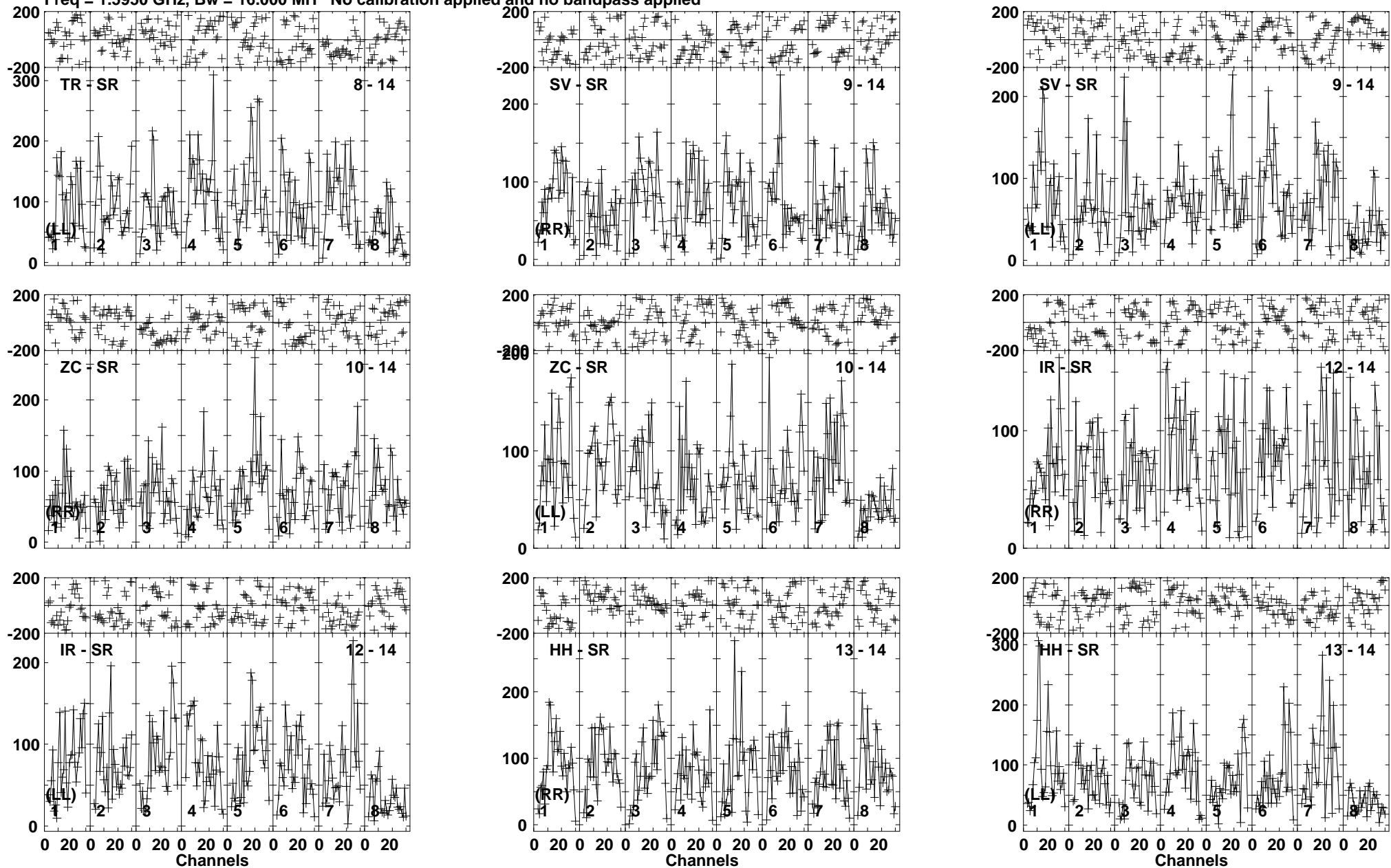
Lower frame: Micro Ampl Jy Top frame: Phas deg Vector averaged cross-power spectrum Baseline: TR (08) - SR (14) Timerange: 00/14:57:01 to 00/15:00:49
