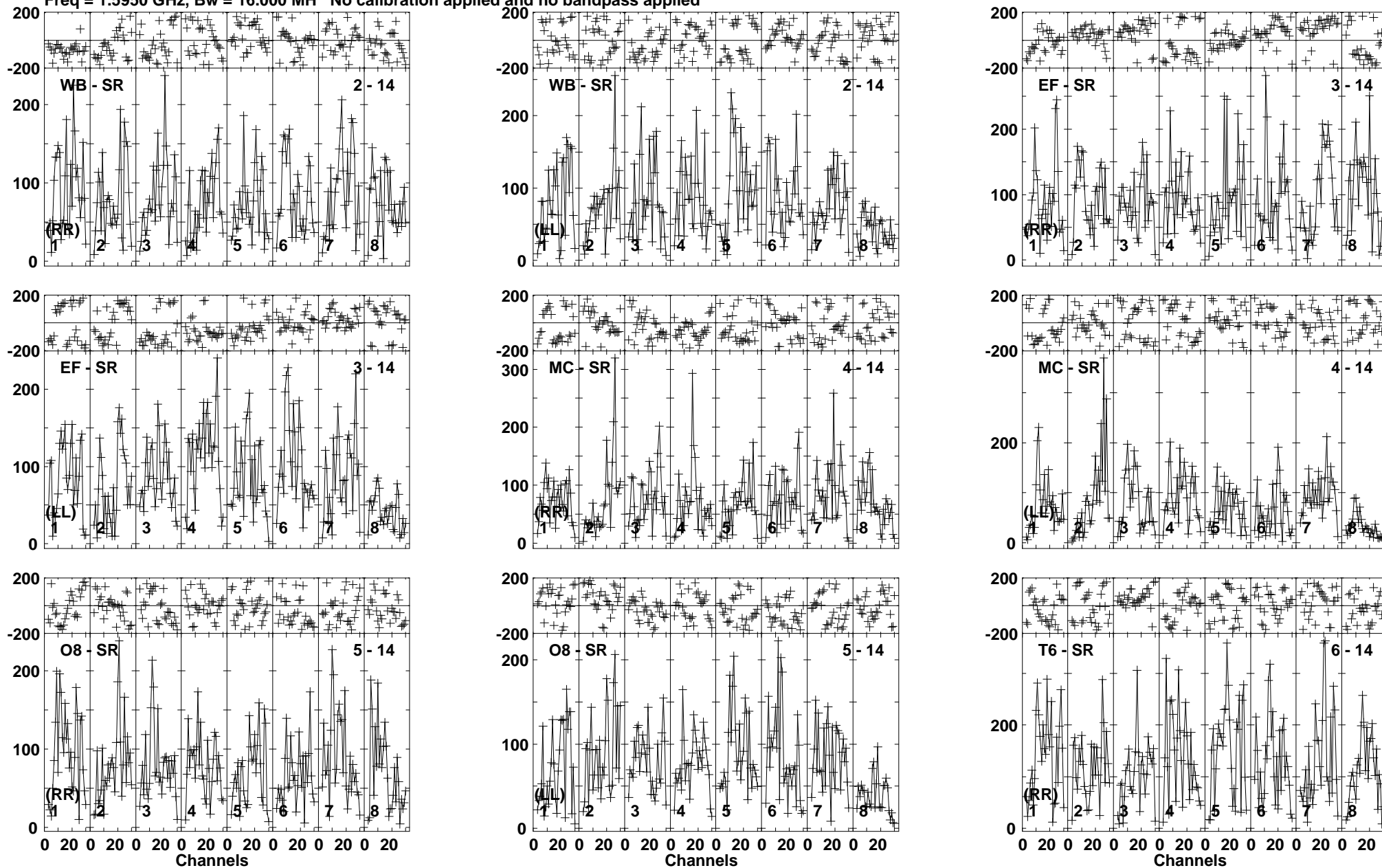
Lower frame: Micro Ampl Jy Top frame: Phas deg Vector averaged cross-power spectrum Baseline: WB (02) - SR (14) Timerange: 00/10:53:31 to 00/10:57:19
