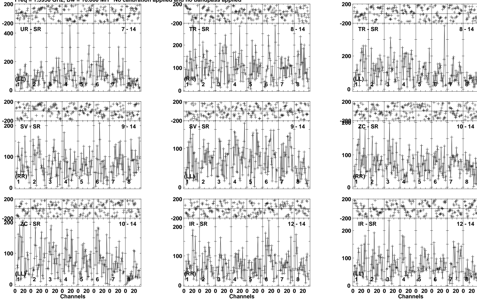
Lower frame: Micro Ampl Jy Top frame: Phas deg Vector averaged cross-power spectrum Baseline: UR (07) - SR (14) Timerange: 00/14:04:31 to 00/14:08:19
