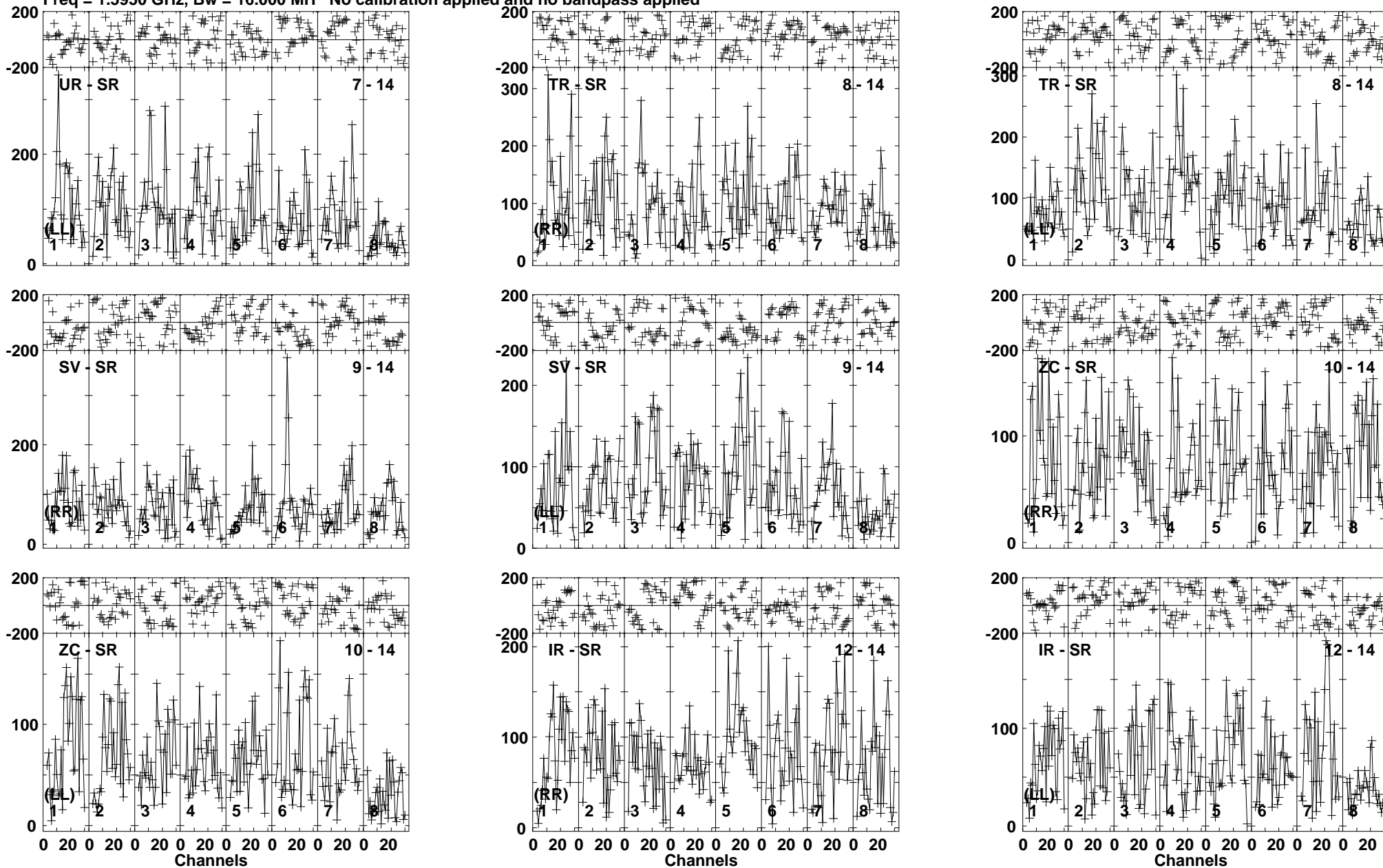
Lower frame: Micro Ampl Jy Top frame: Phas deg Vector averaged cross-power spectrum Baseline: UR (07) - SR (14) Timerange: 00/14:36:01 to 00/14:39:49
