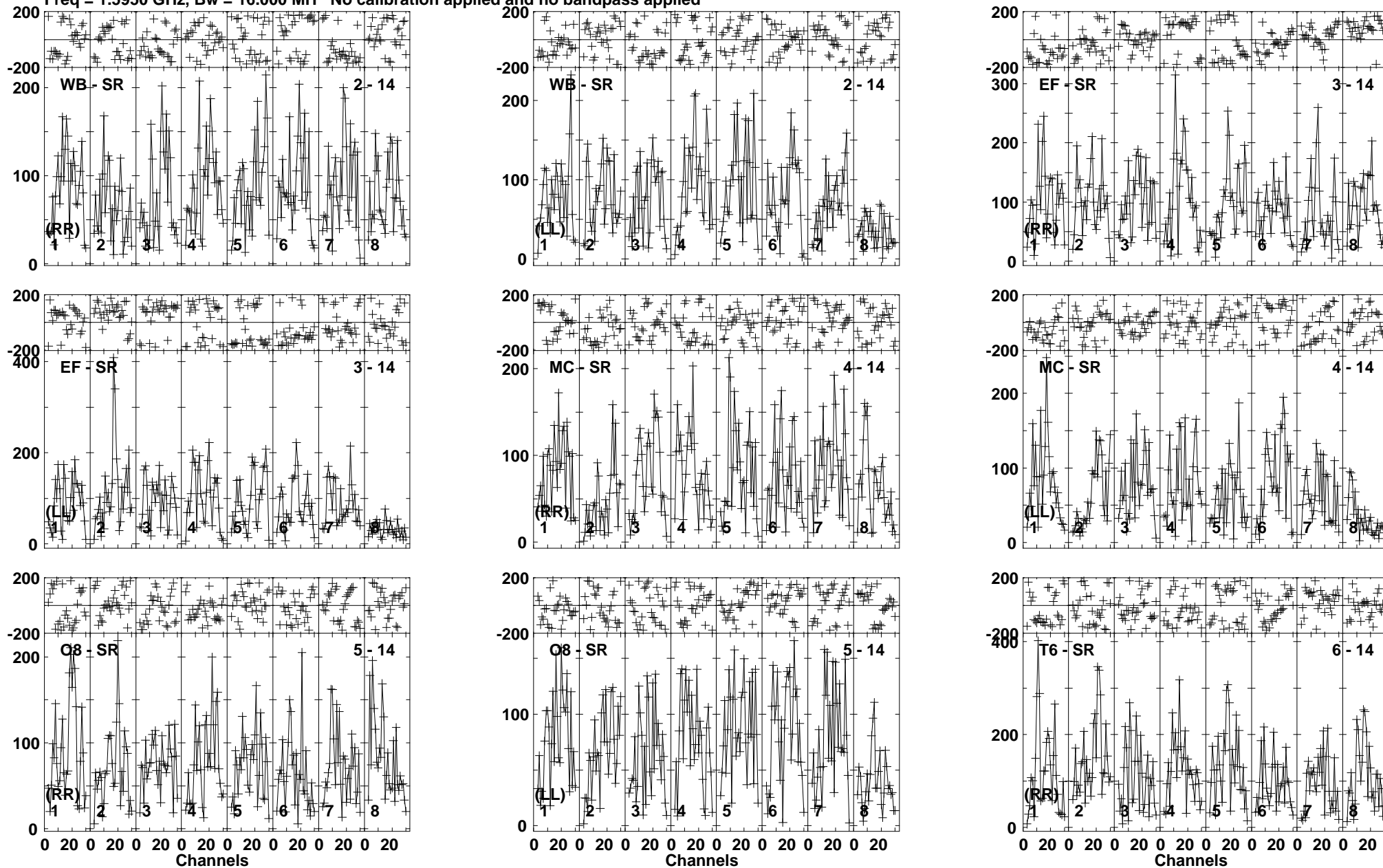
Lower frame: Micro Ampl Jy Top frame: Phas deg Vector averaged cross-power spectrum Baseline: WB (02) - SR (14) Timerange: 00/10:48:01 to 00/10:51:49
