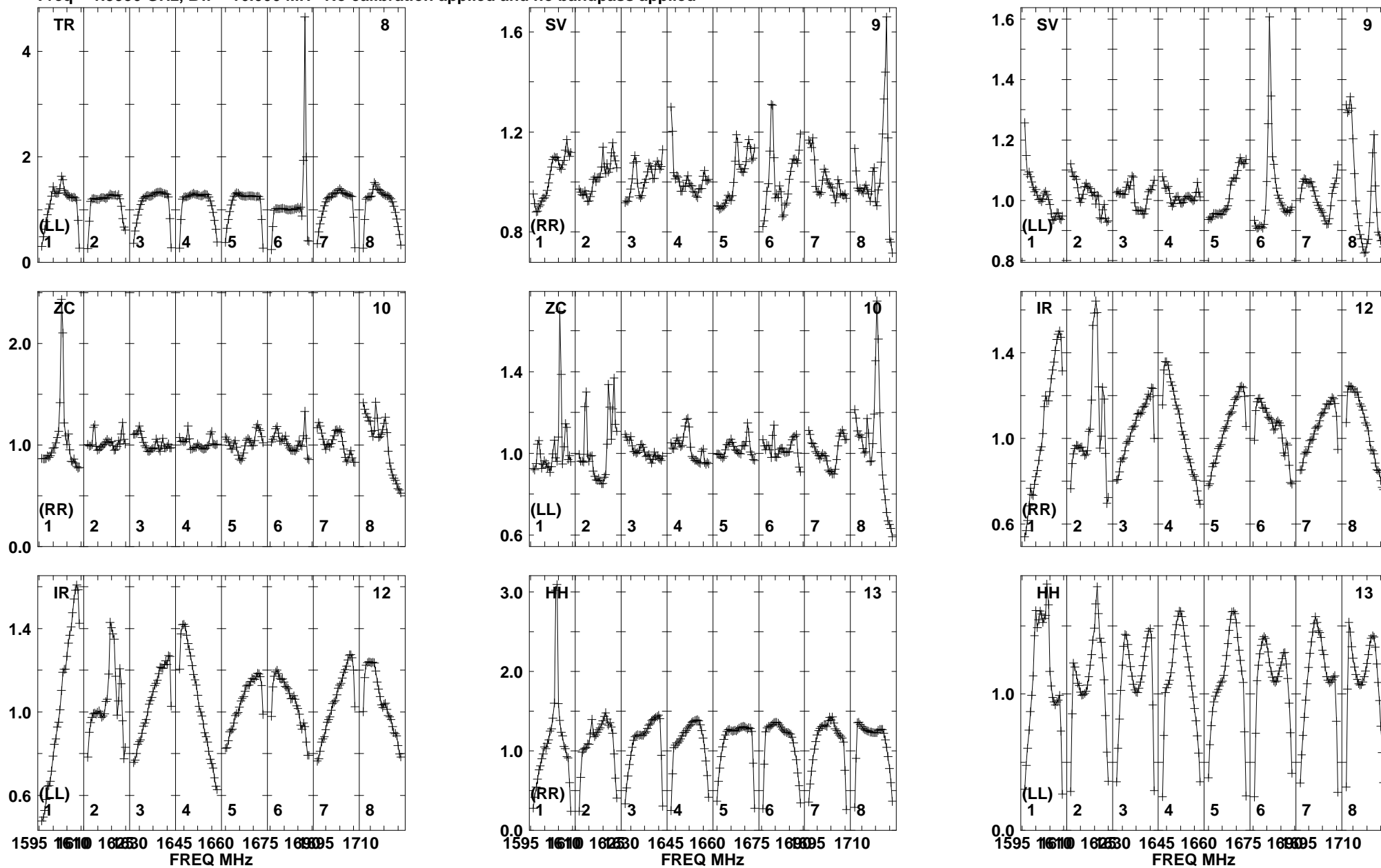
Lower frame: Real Jy Total-power spectrum Antenna: TR (08) Timerange: 00/16:33:31 to 00/16:37:19
