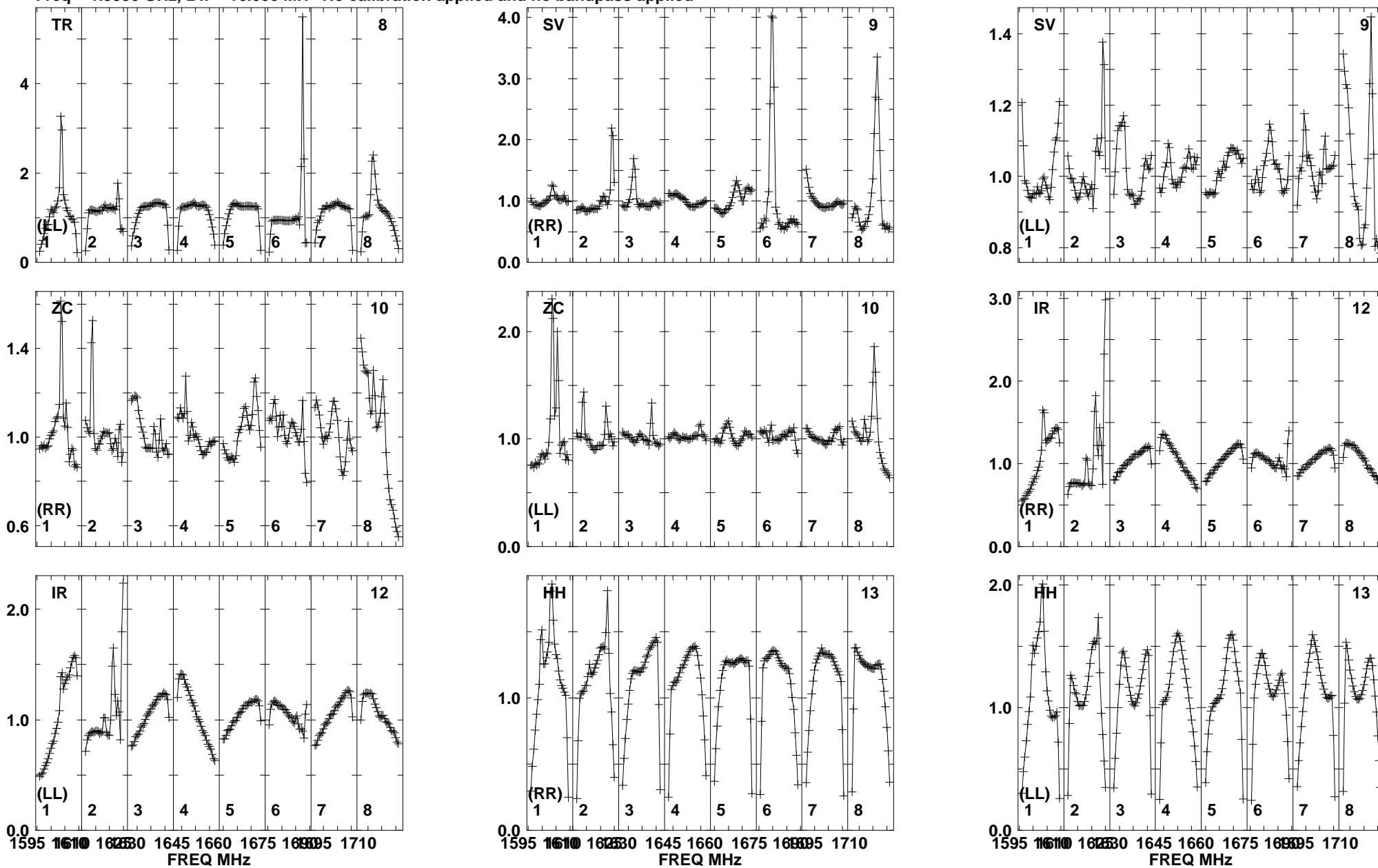
Lower frame: Real Jy Total-power spectrum Antenna: TR (08) Timerange: 00/15:27:21 to 00/15:28:29
