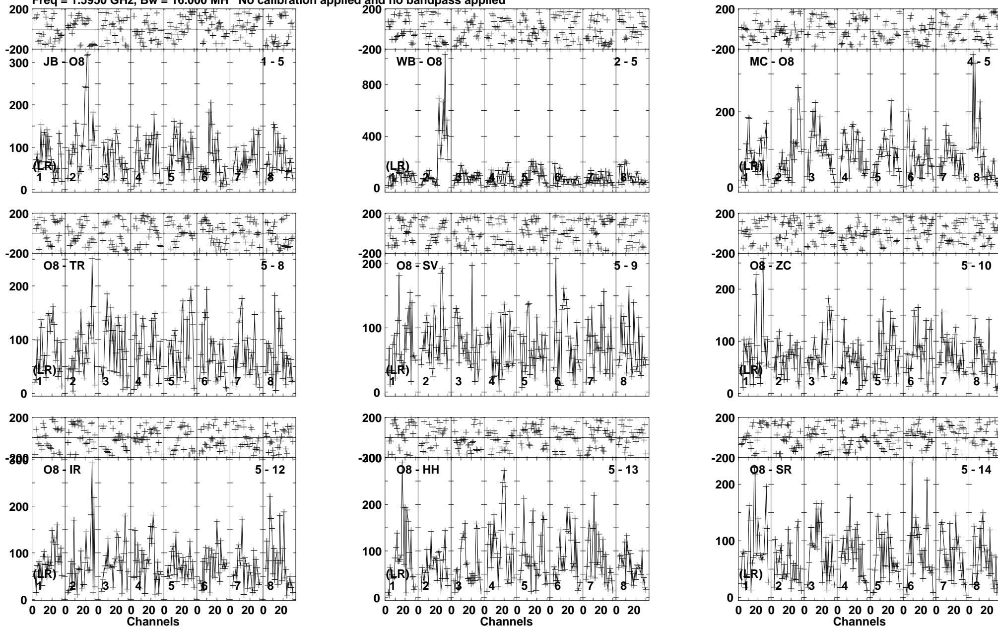
Lower frame: Micro Ampl Jy Top frame: Phas deg Vector averaged cross-power spectrum Baseline: JB (01) - O8 (05) Timerange: 00/16:28:01 to 00/16:31:49
