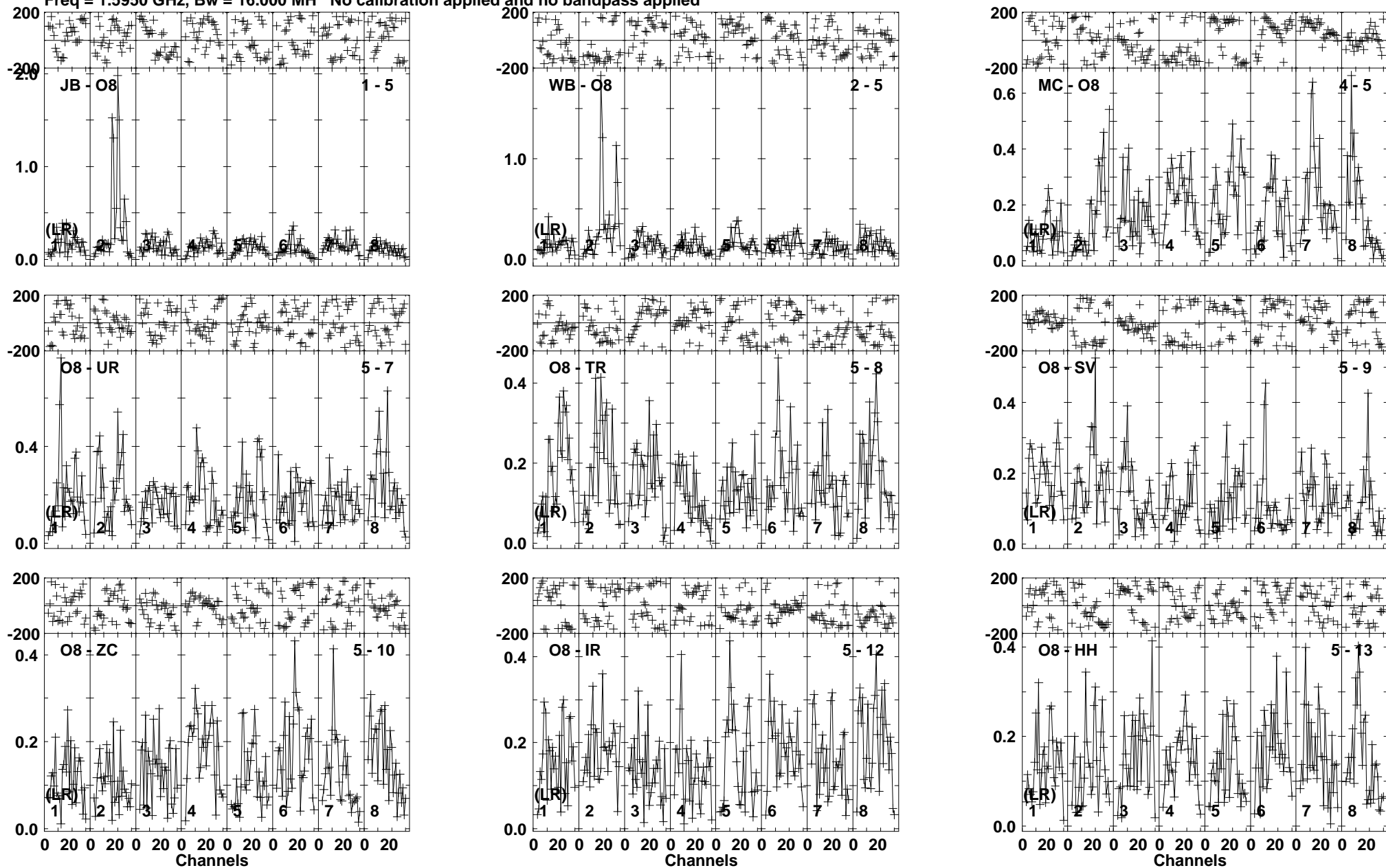
Lower frame: Milli Ampl Jy Top frame: Phas deg Vector averaged cross-power spectrum Baseline: JB (01) - O8 (05) Timerange: 00/14:34:51 to 00/14:35:59
