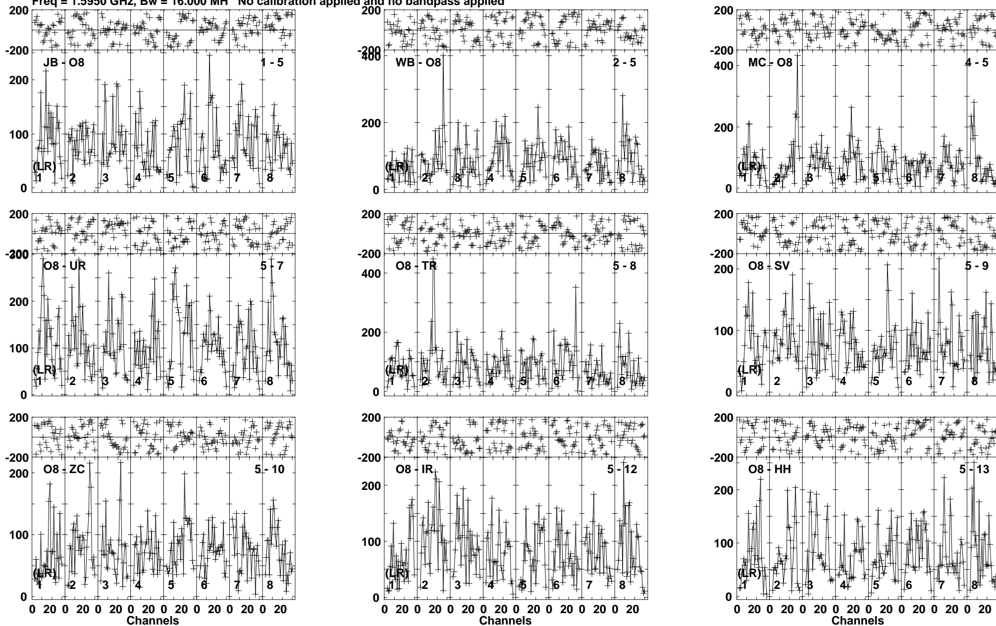
Lower frame: Micro Ampl Jy Top frame: Phas deg Vector averaged cross-power spectrum Baseline: JB (01) - O8 (05) Timerange: 00/13:17:01 to 00/13:20:49
