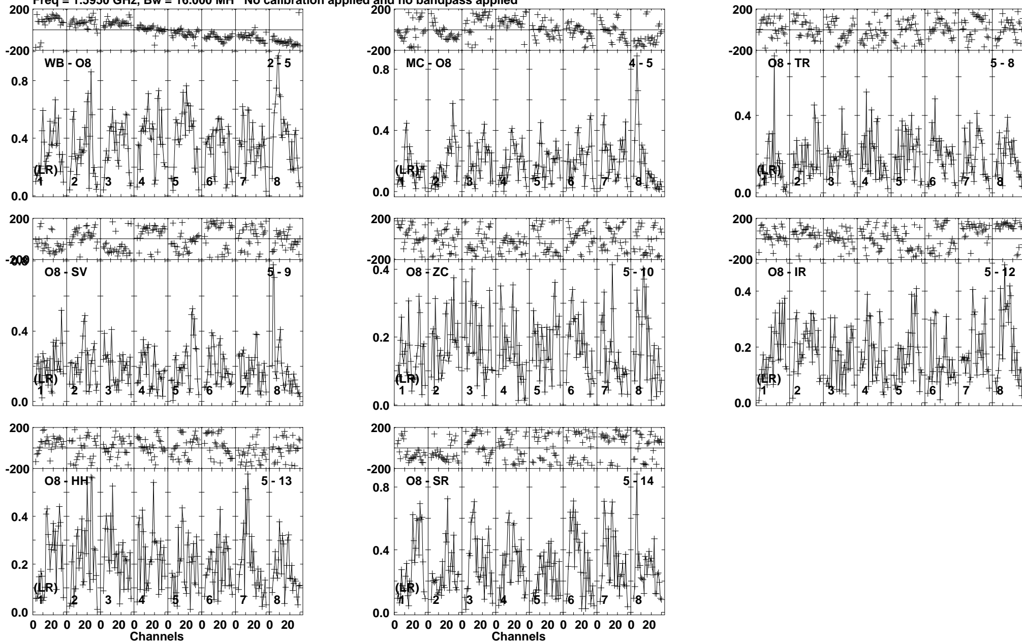
Lower frame: Milli Ampl Jy Top frame: Phas deg Vector averaged cross-power spectrum Baseline: WB (02) - O8 (05) Timerange: 00/15:21:51 to 00/15:22:59
