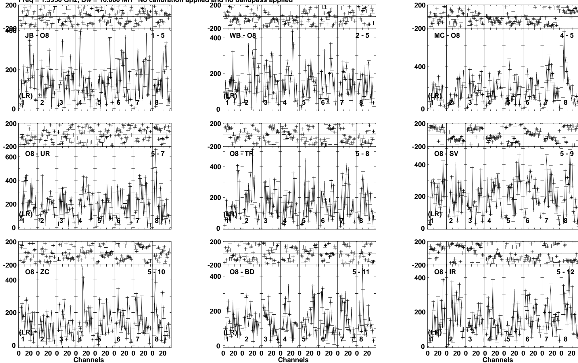
Lower frame: Micro Ampl Jy Top frame: Phas deg Vector averaged cross-power spectrum Baseline: JB (01) - O8 (05) Timerange: 00/12:47:51 to 00/12:48:59
