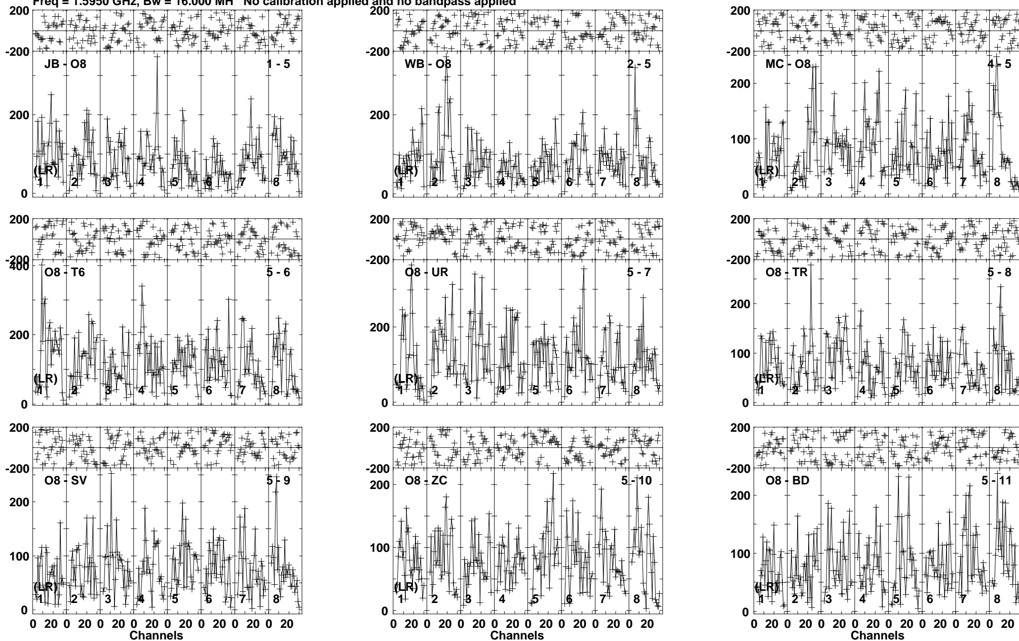
Lower frame: Micro Ampl Jy Top frame: Phas deg Vector averaged cross-power spectrum Baseline: JB (01) - O8 (05) Timerange: 00/11:04:01 to 00/11:07:49
