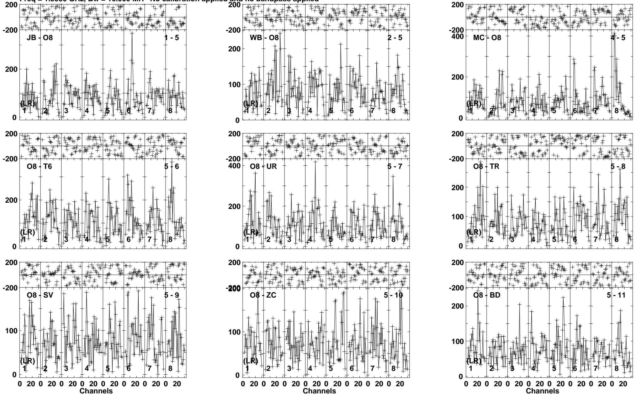
Lower frame: Micro Ampl Jy Top frame: Phas deg Vector averaged cross-power spectrum Baseline: JB (01) - O8 (05) Timerange: 00/12:01:31 to 00/12:05:19
