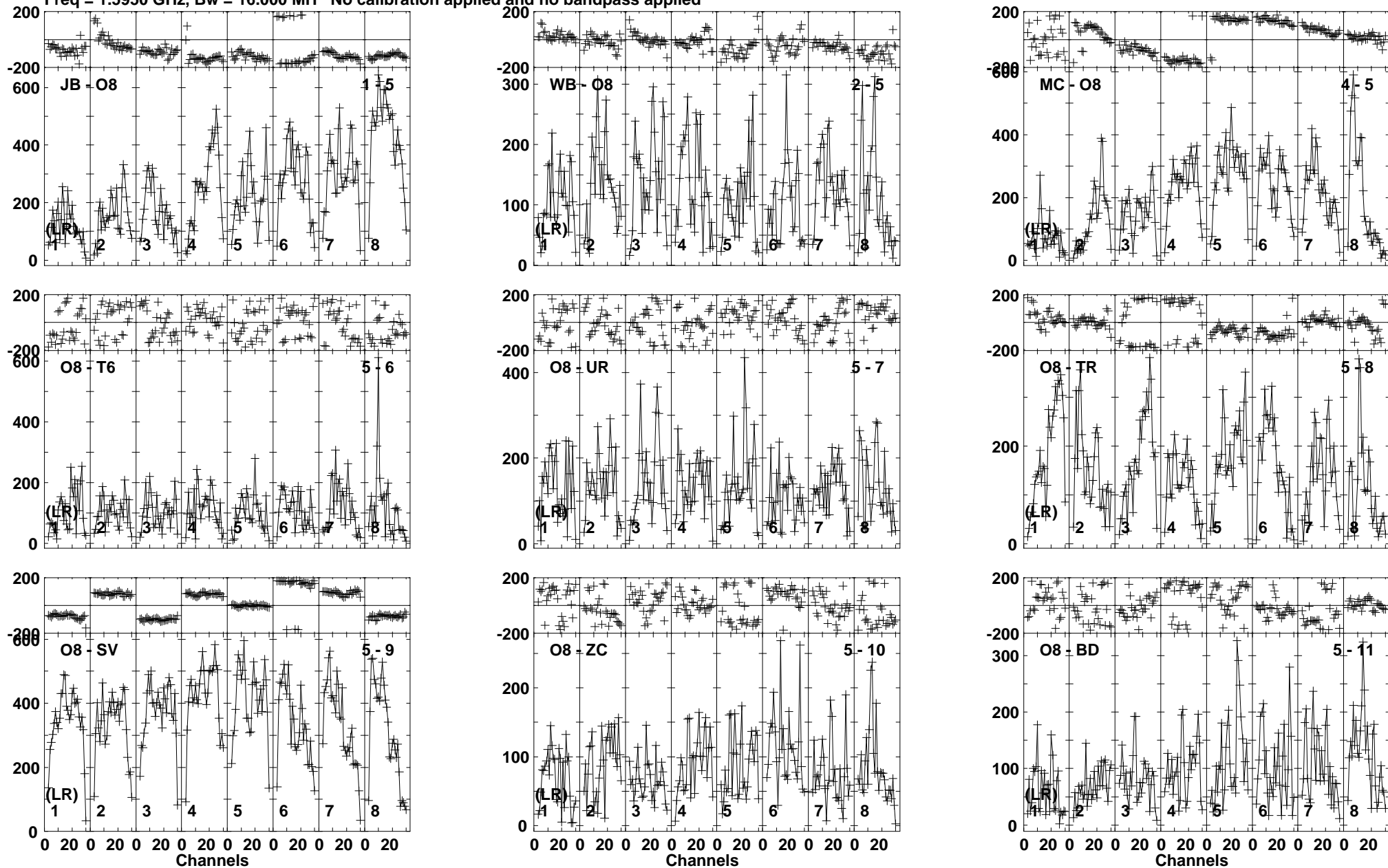
Lower frame: Micro Ampl Jy Top frame: Phas deg Vector averaged cross-power spectrum Baseline: JB (01) - O8 (05) Timerange: 00/10:30:01 to 00/10:33:29
