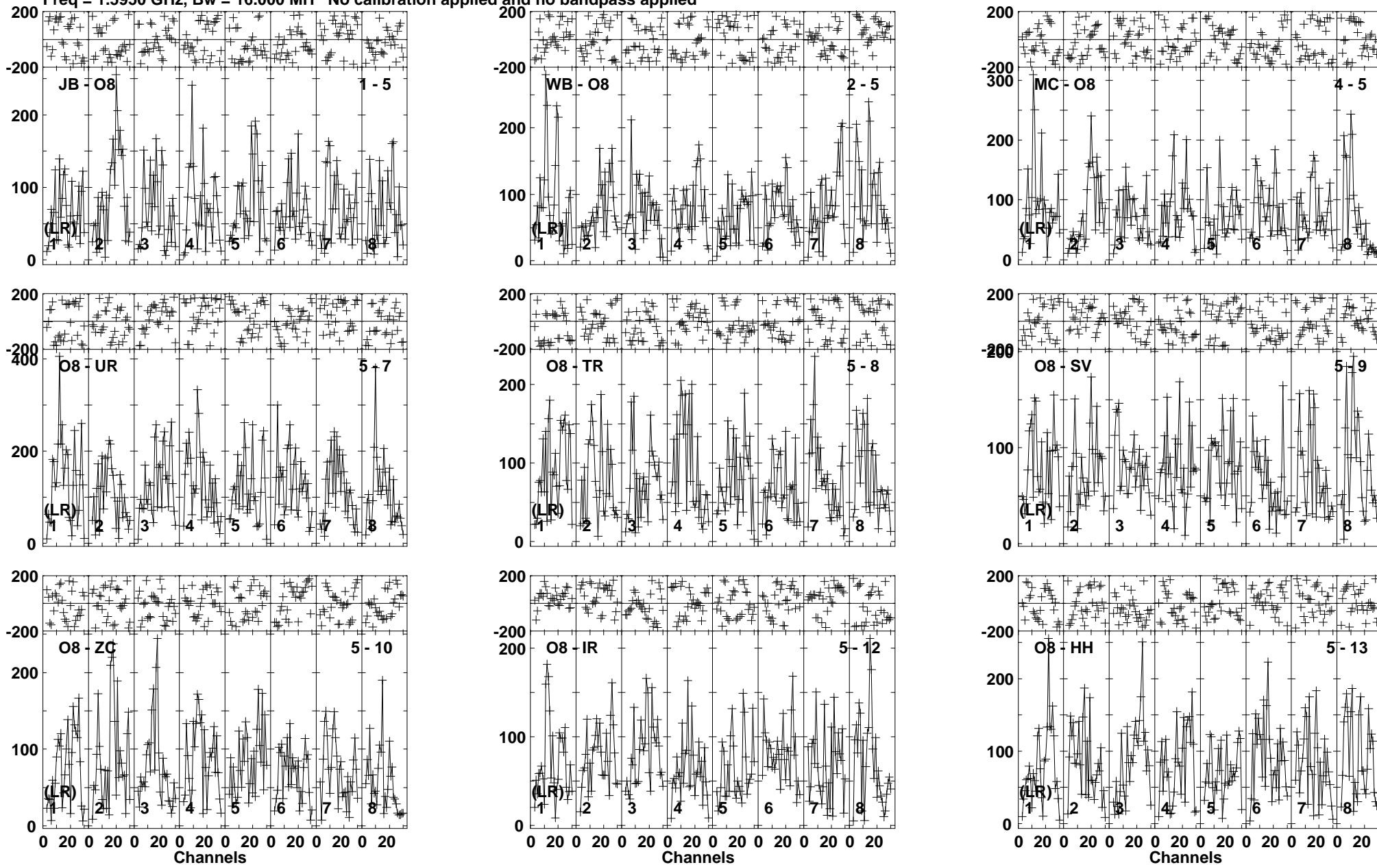
Lower frame: Micro Ampl Jy Top frame: Phas deg Vector averaged cross-power spectrum Baseline: JB (01) - O8 (05) Timerange: 00/14:20:01 to 00/14:23:49
