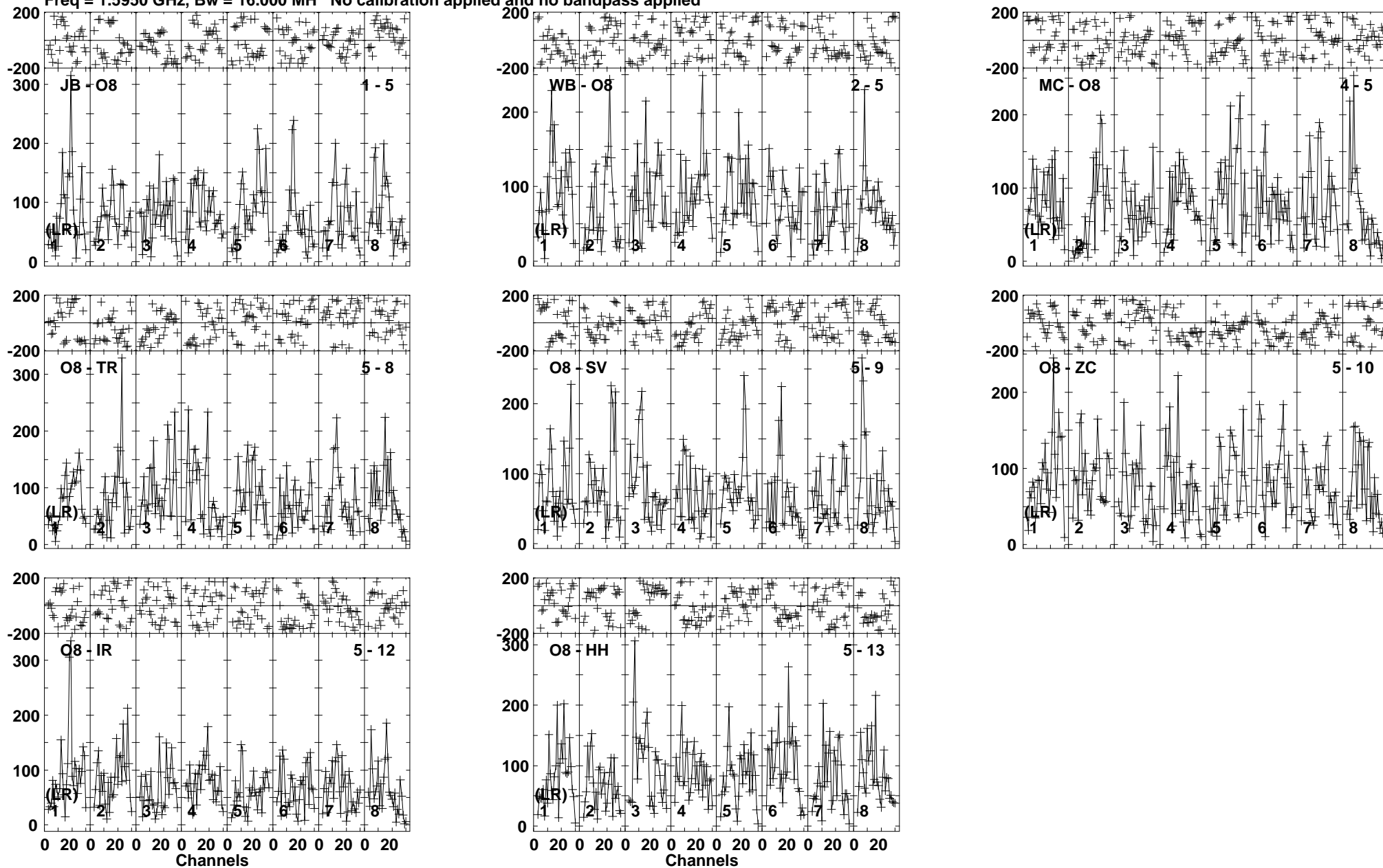
Lower frame: Micro Ampl Jy Top frame: Phas deg Vector averaged cross-power spectrum Baseline: JB (01) - O8 (05) Timerange: 00/15:33:31 to 00/15:37:19
