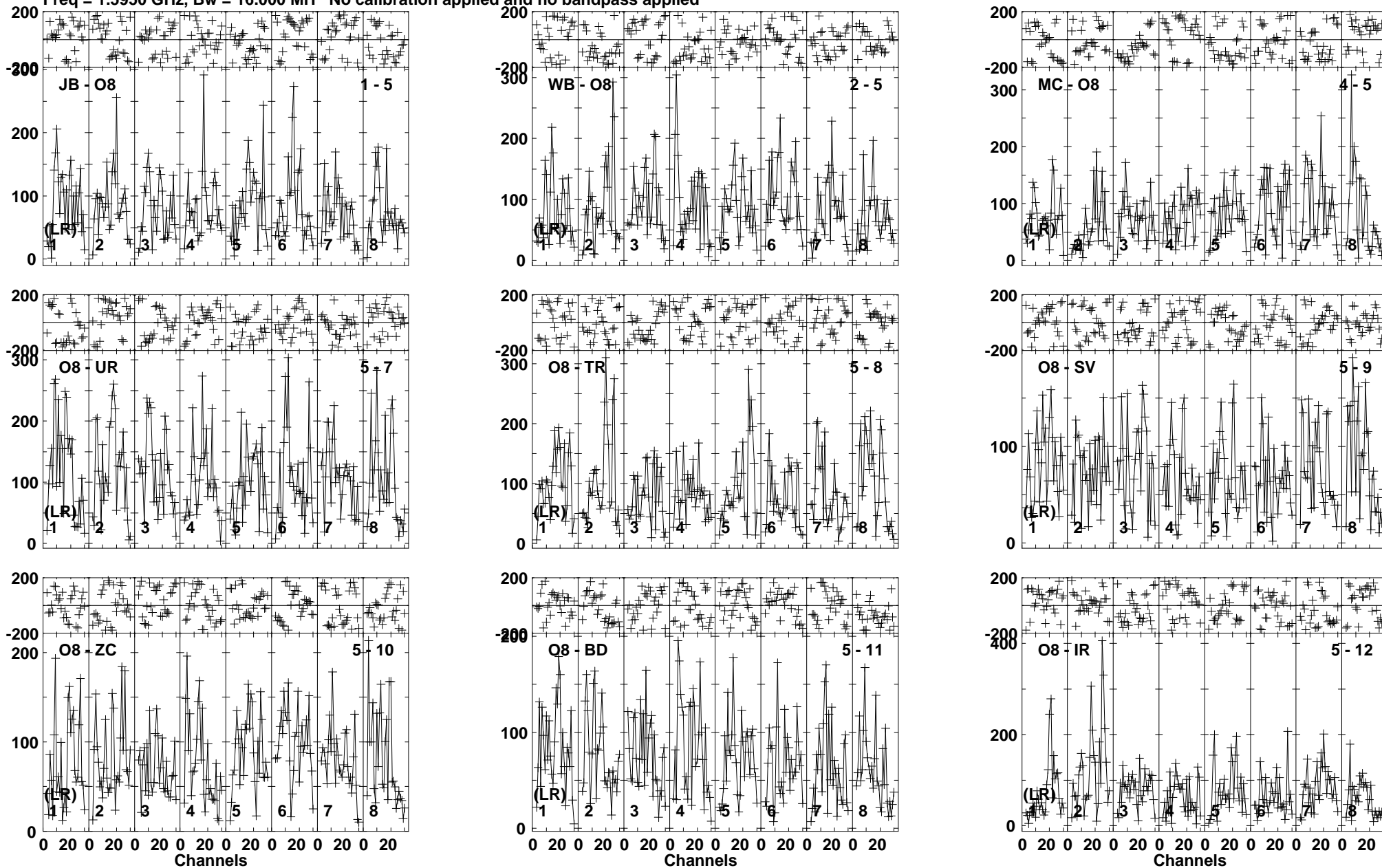
Lower frame: Micro Ampl Jy Top frame: Phas deg Vector averaged cross-power spectrum Baseline: JB (01) - O8 (05) Timerange: 00/12:59:31 to 00/13:03:19
