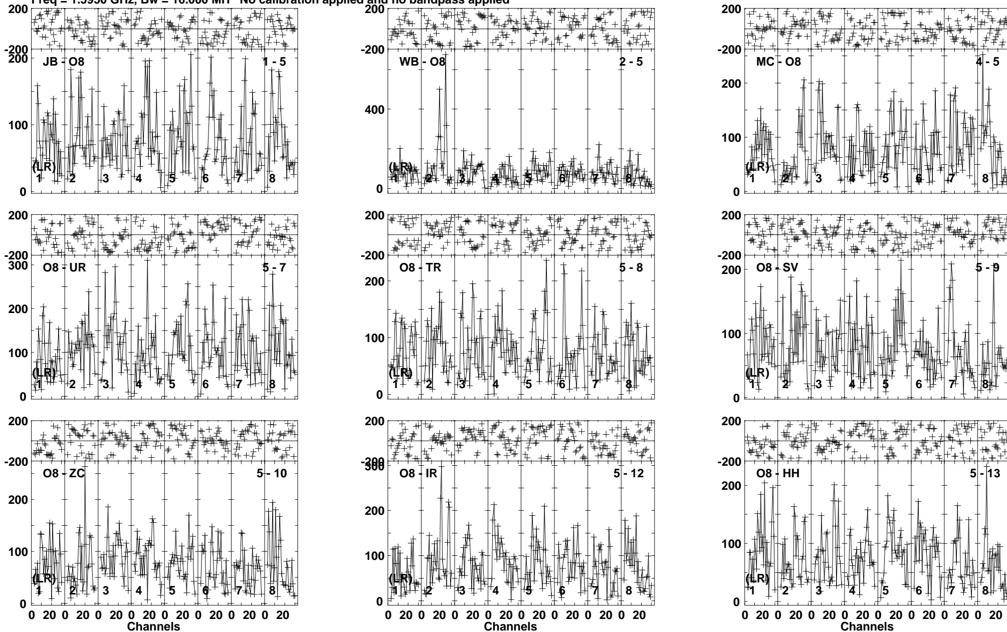
Lower frame: Micro Ampl Jy Top frame: Phas deg Vector averaged cross-power spectrum Baseline: JB (01) - O8 (05) Timerange: 00/14:25:31 to 00/14:29:19
