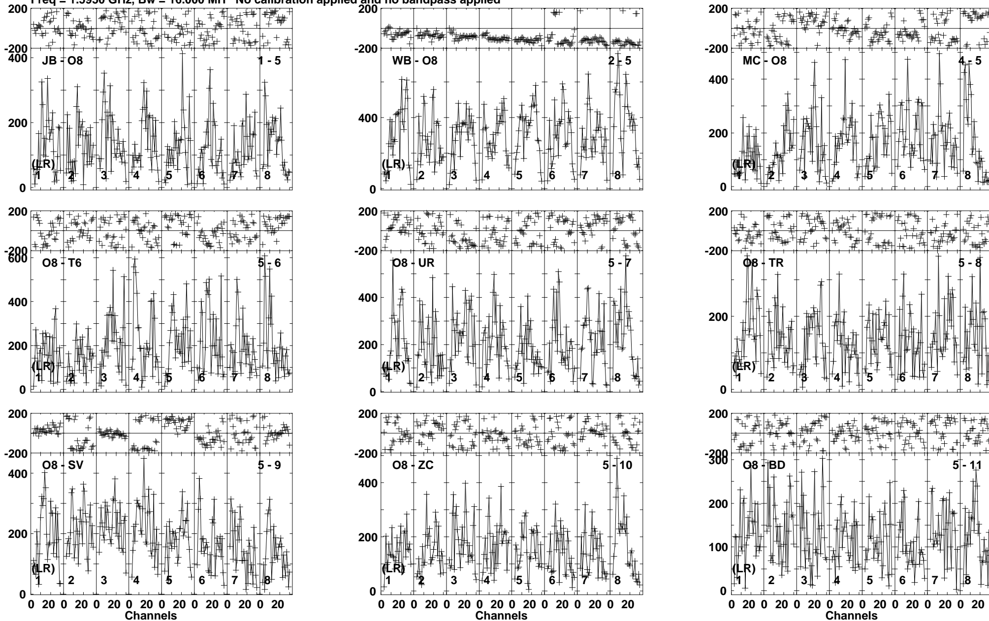
Lower frame: Micro Ampl Jy Top frame: Phas deg Vector averaged cross-power spectrum Baseline: JB (01) - O8 (05) Timerange: 00/11:55:21 to 00/11:56:29
