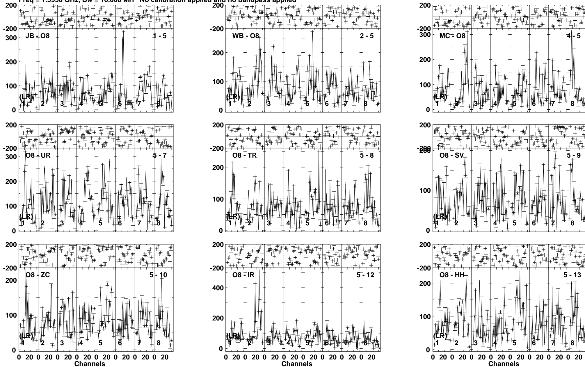
Lower frame: Micro Ampl Jy Top frame: Phas deg Vector averaged cross-power spectrum Baseline: JB (01) - O8 (05) Timerange: 00/13:38:01 to 00/13:41:49
