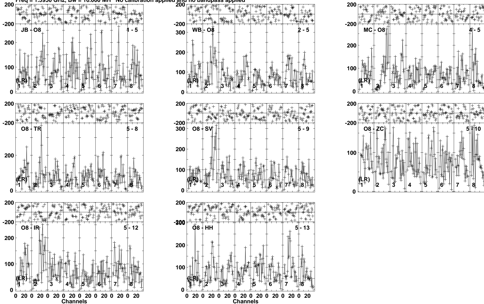
Lower frame: Micro Ampl Jy Top frame: Phas deg Vector averaged cross-power spectrum Baseline: JB (01) - O8 (05) Timerange: 00/16:02:01 to 00/16:05:49
