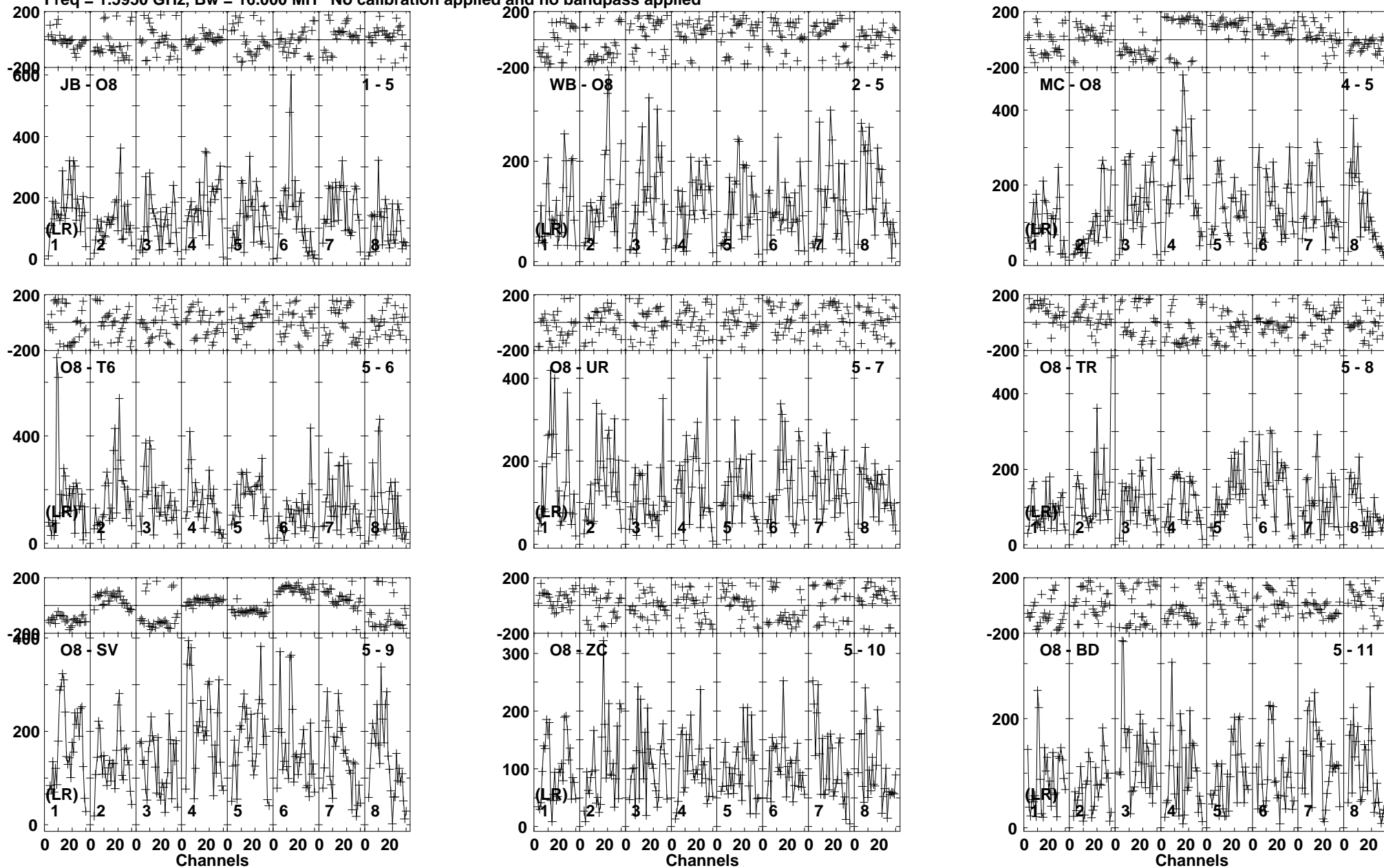
Lower frame: Micro Ampl Jy Top frame: Phas deg Vector averaged cross-power spectrum Baseline: JB (01) - O8 (05) Timerange: 00/10:33:31 to 00/10:37:29
