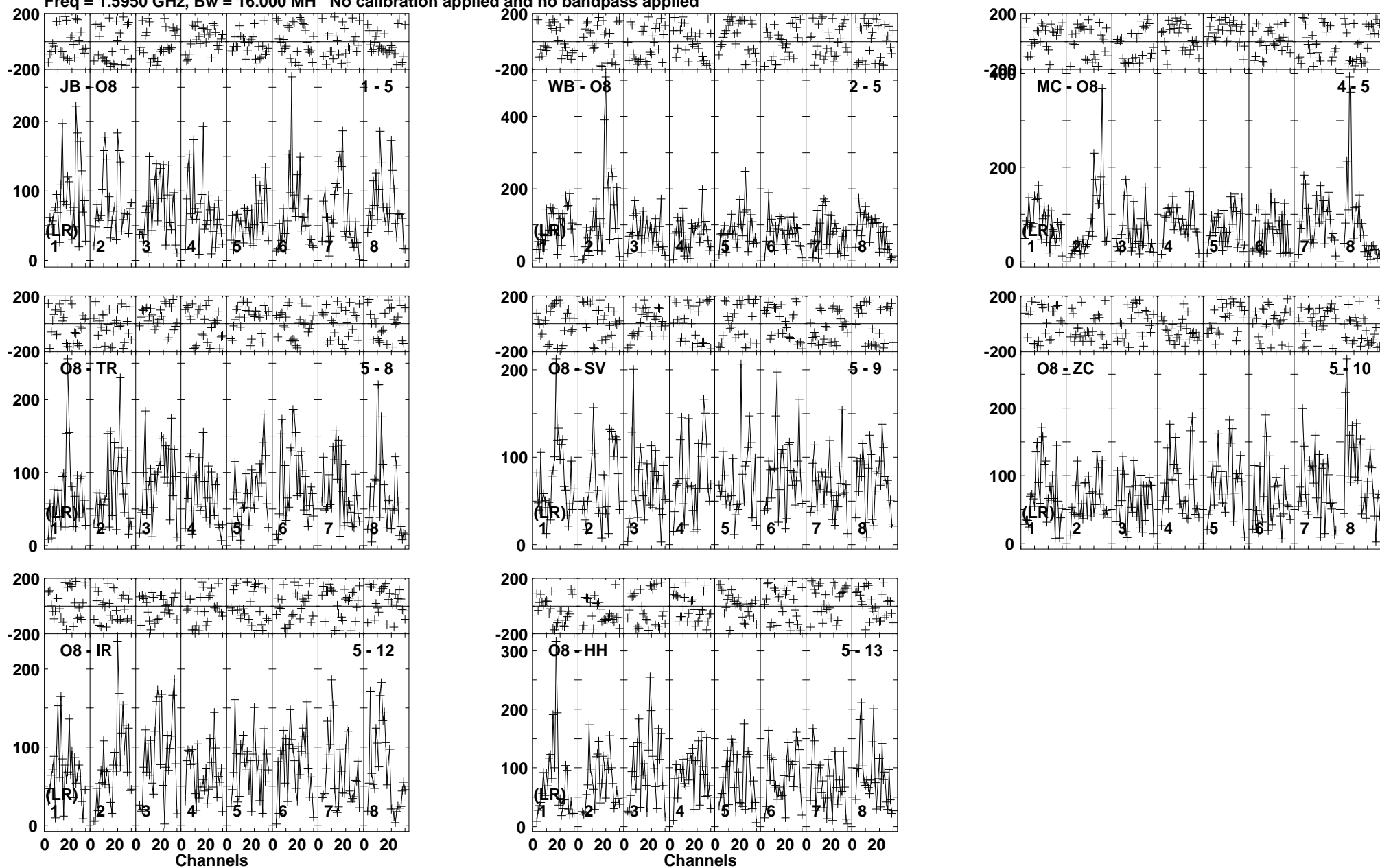
Lower frame: Micro Ampl Jy Top frame: Phas deg Vector averaged cross-power spectrum Baseline: JB (01) - O8 (05) Timerange: 00/16:17:31 to 00/16:21:19
