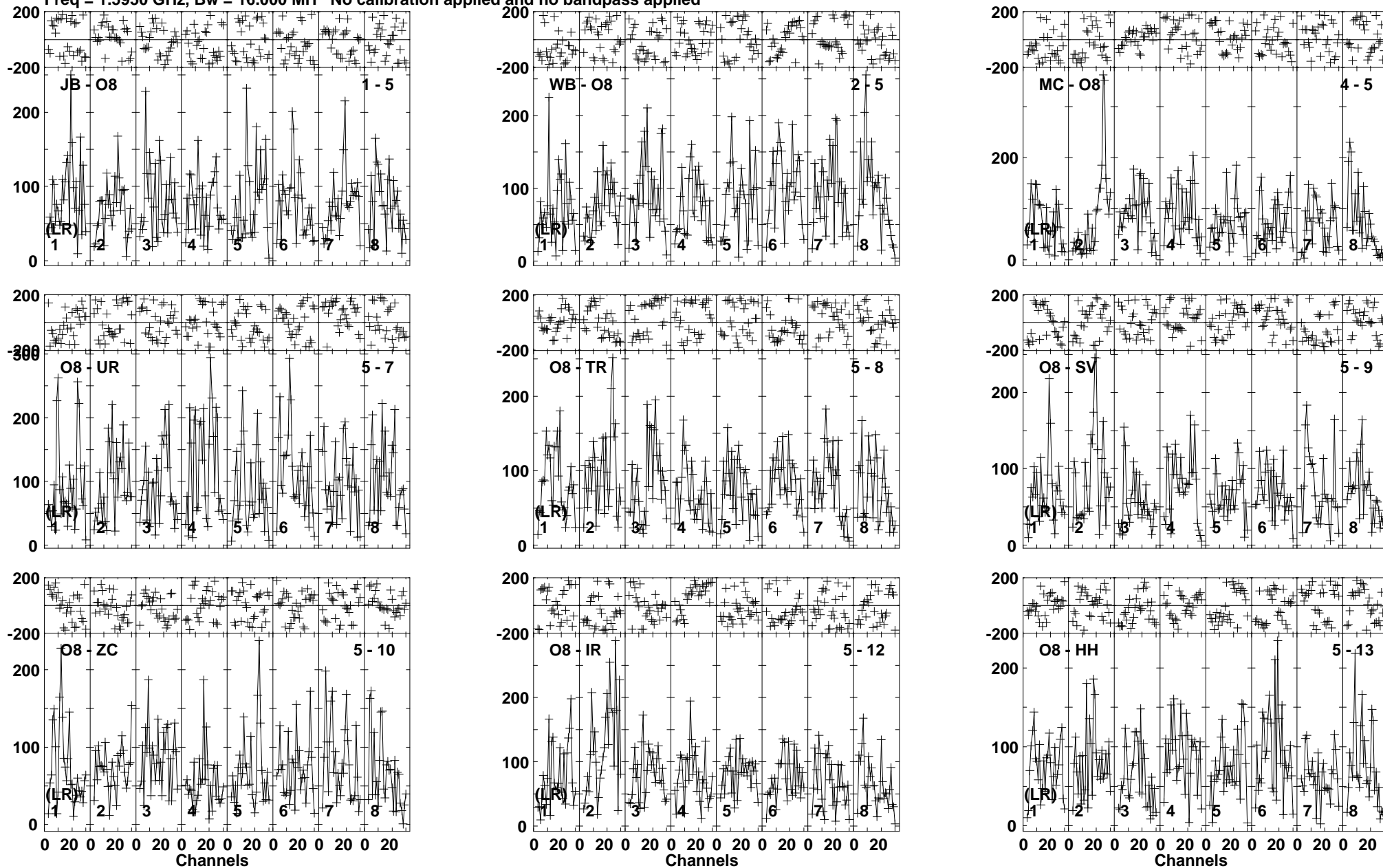
Lower frame: Micro Ampl Jy Top frame: Phas deg Vector averaged cross-power spectrum Baseline: JB (01) - O8 (05) Timerange: 00/13:10:01 to 00/13:13:49
