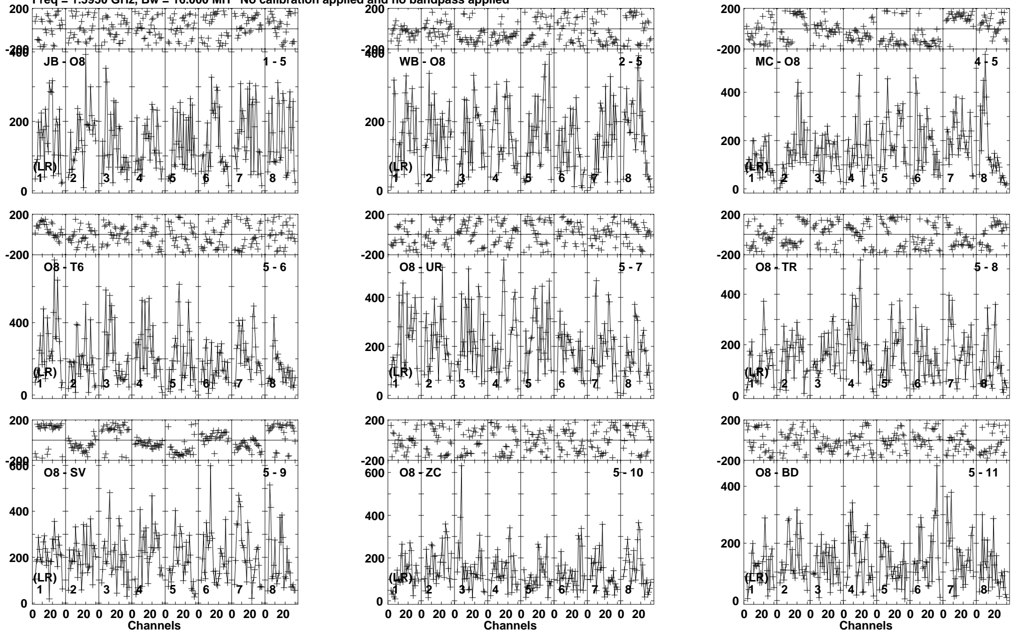
Lower frame: Micro Ampl Jy Top frame: Phas deg Vector averaged cross-power spectrum Baseline: JB (01) - O8 (05) Timerange: 00/12:16:21 to 00/12:17:29
