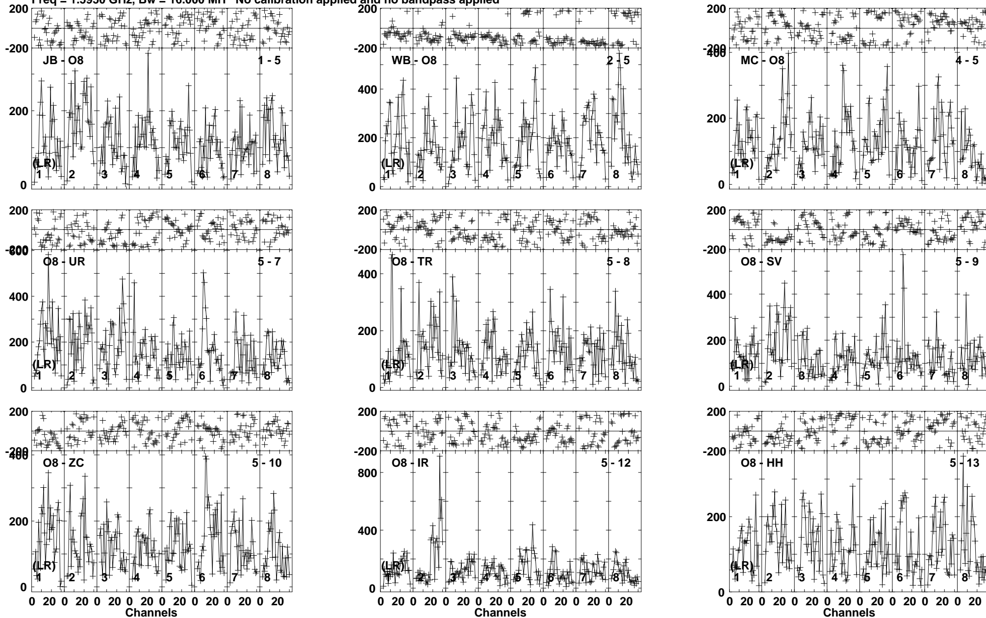
Lower frame: Micro Ampl Jy Top frame: Phas deg Vector averaged cross-power spectrum Baseline: JB (01) - O8 (05) Timerange: 00/13:15:01 to 00/13:16:59
