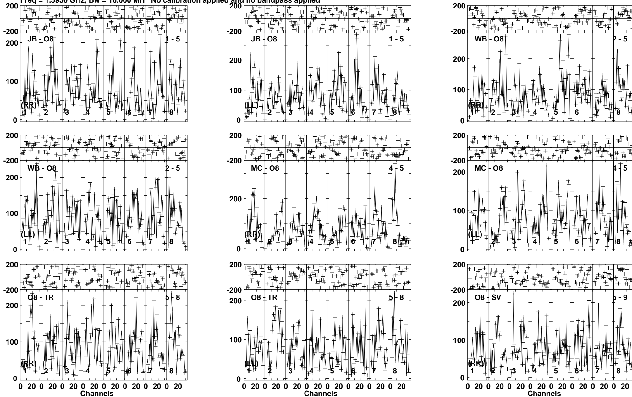
Lower frame: Micro Ampl Jy Top frame: Phas deg Vector averaged cross-power spectrum Baseline: JB (01) - O8 (05) Timerange: 00/16:33:31 to 00/16:37:19
