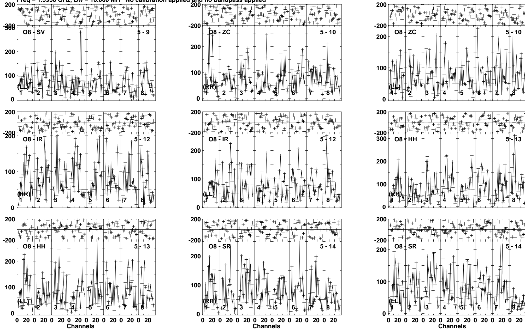
Lower frame: Micro Ampl Jy Top frame: Phas deg Vector averaged cross-power spectrum Baseline: O8 (05) - SV (09) Timerange: 00/15:12:31 to 00/15:16:19
