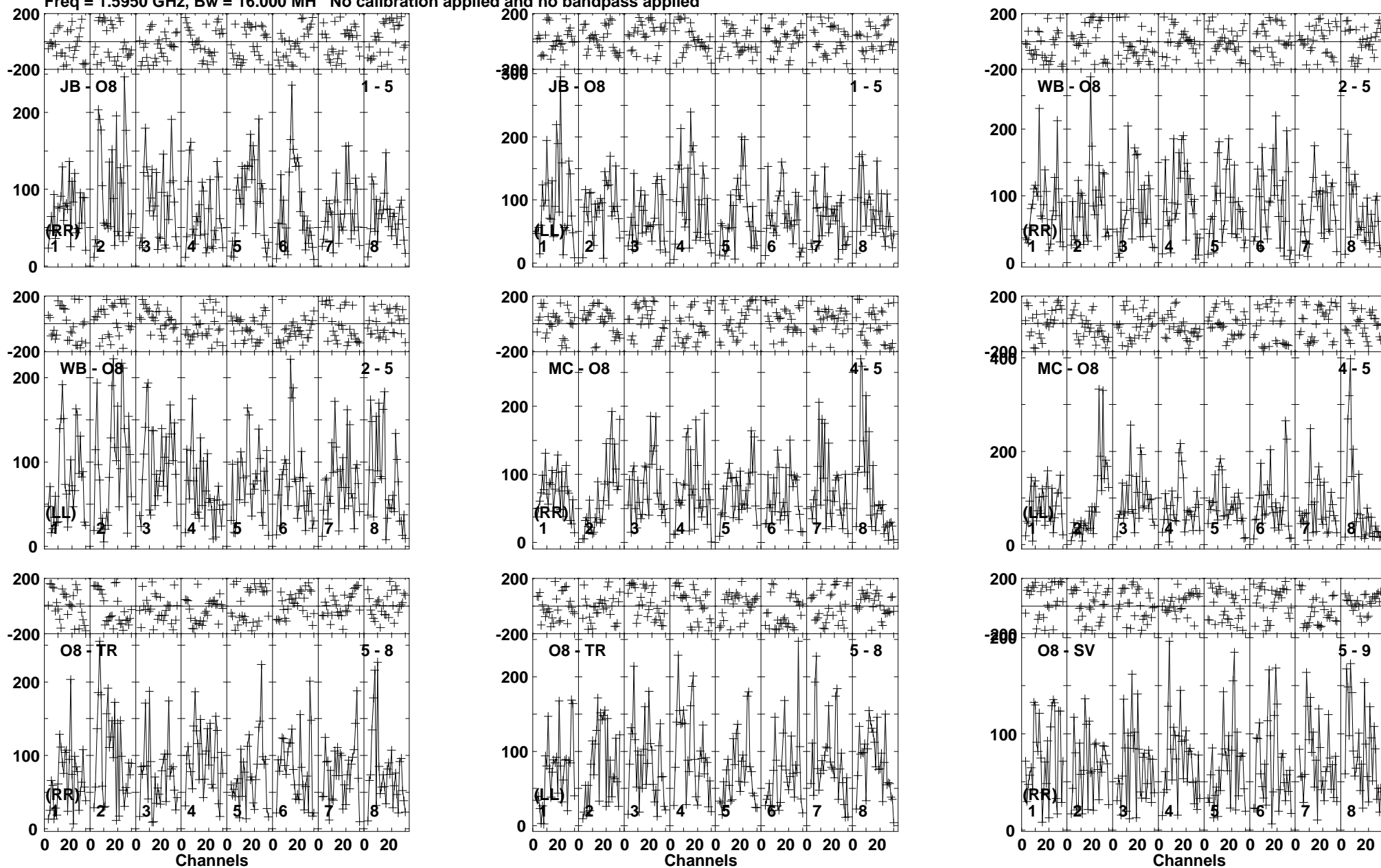
Lower frame: Micro Ampl Jy Top frame: Phas deg Vector averaged cross-power spectrum Baseline: JB (01) - O8 (05) Timerange: 00/15:02:01 to 00/15:05:49
