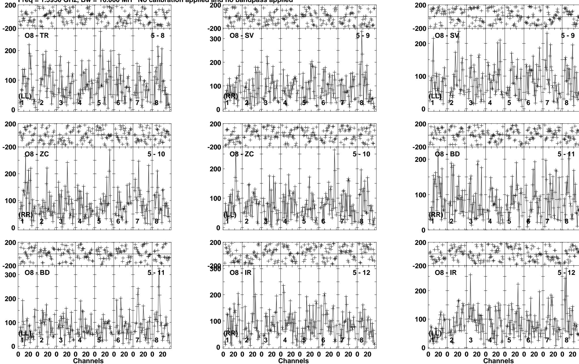
Lower frame: Micro Ampl Jy Top frame: Phas deg Vector averaged cross-power spectrum Baseline: O8 (05) - TR (08) Timerange: 00:12:22:31 to 00:12:26:19
