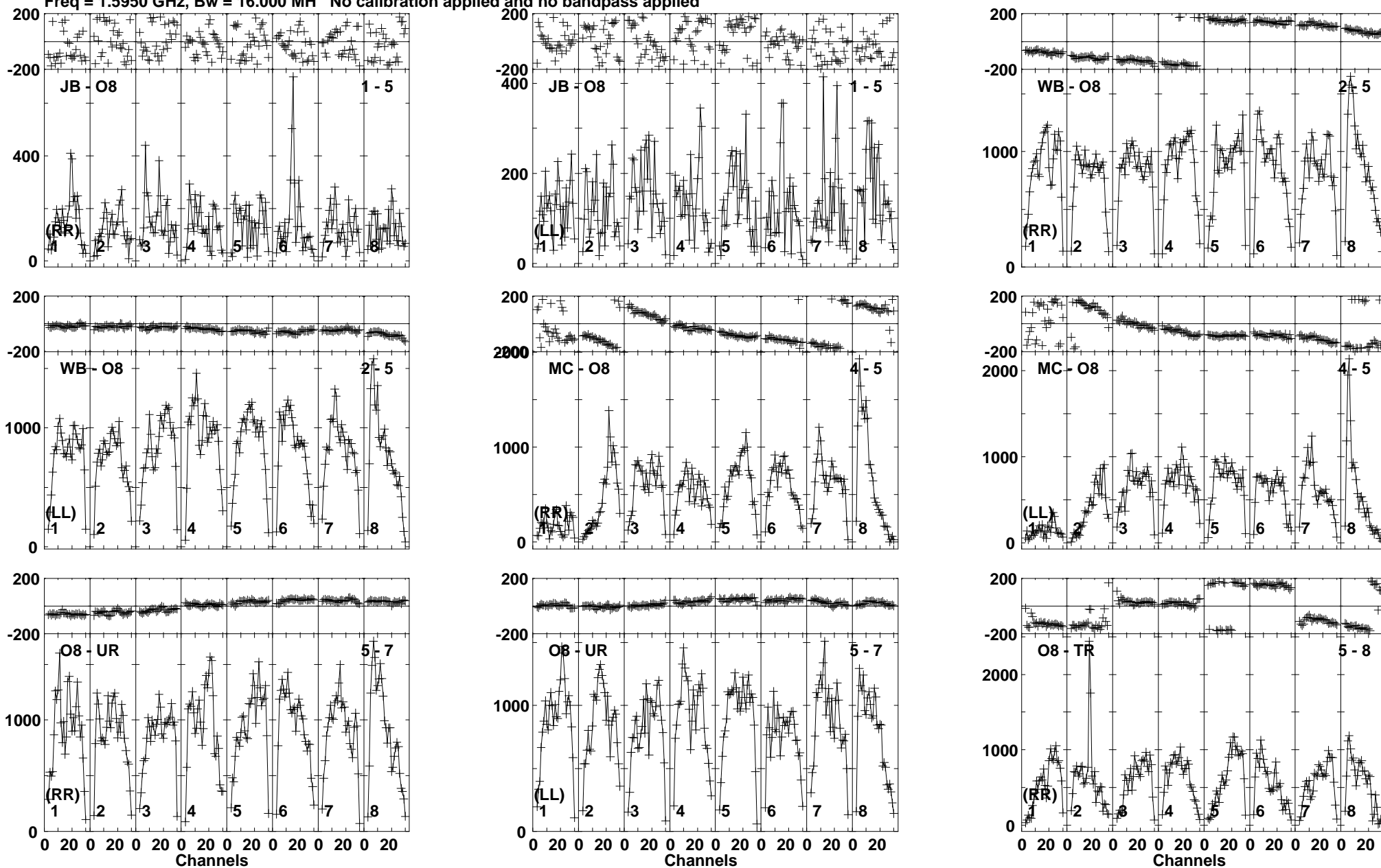
Lower frame: Micro Ampl Jy Top frame: Phas deg Vector averaged cross-power spectrum Baseline: JB (01) - O8 (05) Timerange: 00/13:21:21 to 00/13:22:29
