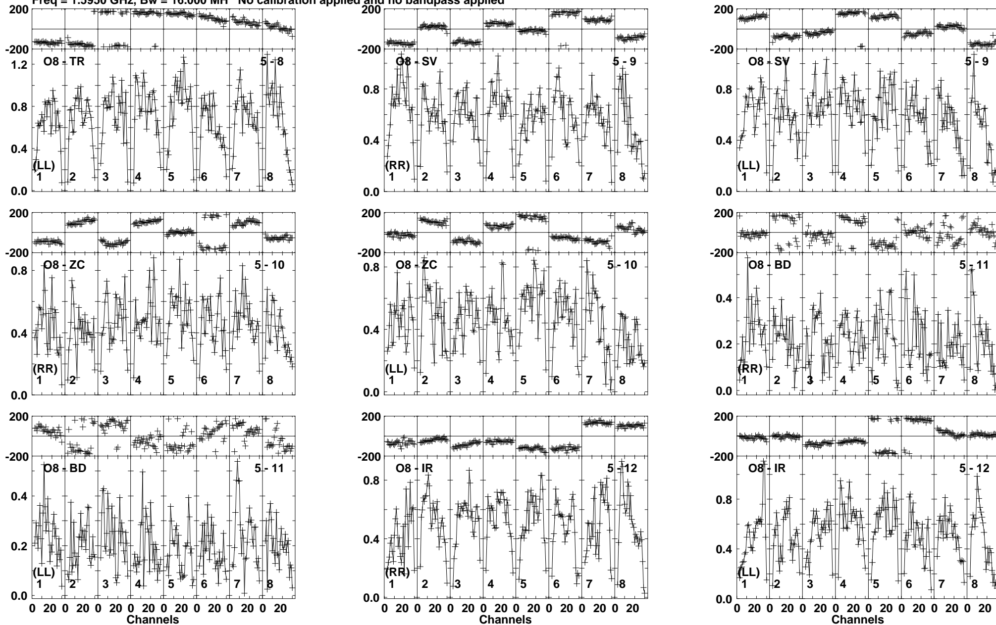
Lower frame: Milli Ampl Jy Top frame: Phas deg Vector averaged cross-power spectrum Baseline: O8 (05) - TR (08) Timerange: 00/12:00:21 to 00/12:01:29
