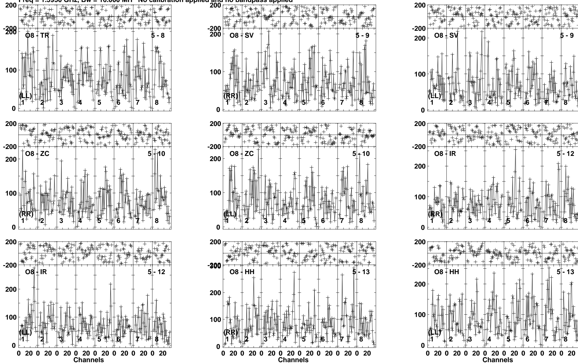
Lower frame: Micro Ampl Jy Top frame: Phas deg Vector averaged cross-power spectrum Baseline: O8 (05) - TR (08) Timerange: 00/14:20:01 to 00/14:23:49
