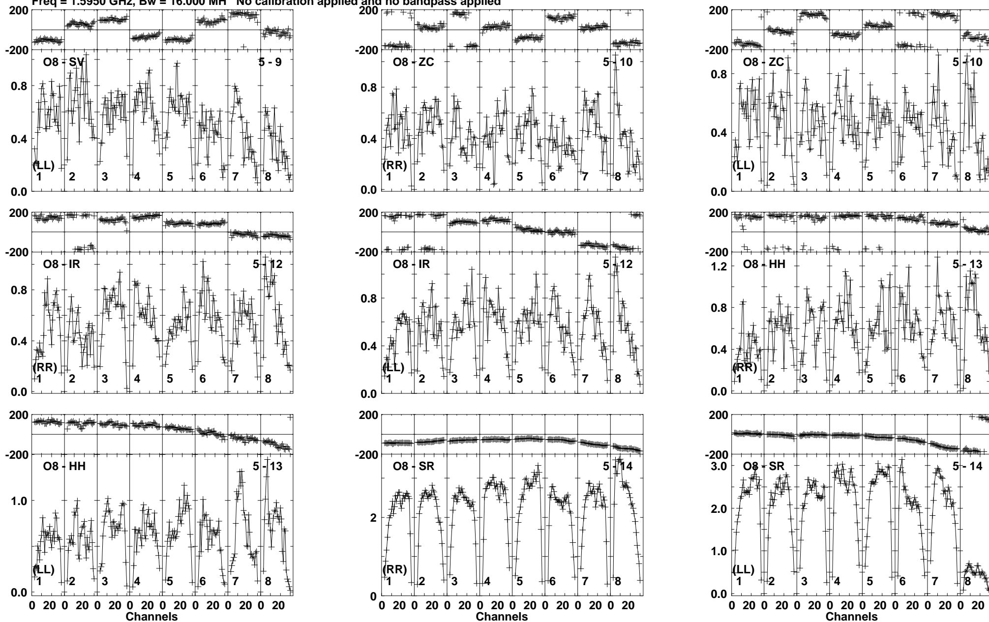
Lower frame: Milli Ampl Jy Top frame: Phas deg Vector averaged cross-power spectrum Baseline: O8 (05) - SV (09) Timerange: 00/13:26:21 to 00/13:27:29
