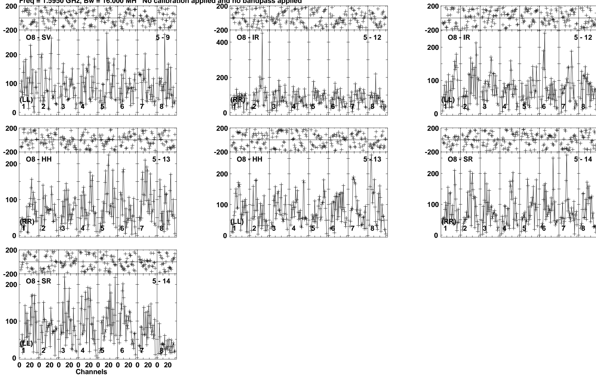
Lower frame: Micro Ampl Jy Top frame: Phas deg Vector averaged cross-power spectrum Baseline: O8 (05) - SV (09) Timerange: 00/17:31:01 to 00/17:34:49
