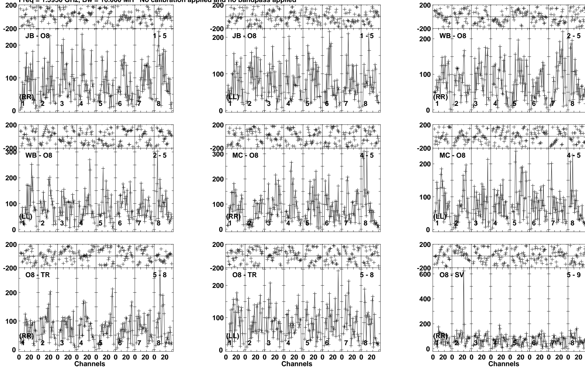
Lower frame: Micro Ampl Jy Top frame: Phas deg Vector averaged cross-power spectrum Baseline: JB (01) - O8 (05) Timerange: 00/15:12:31 to 00/15:16:19
