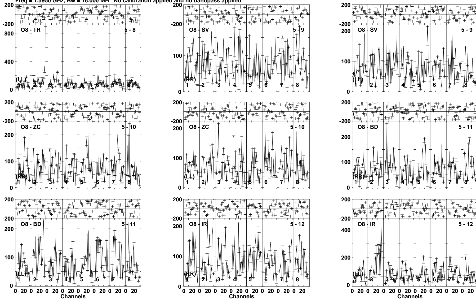
Lower frame: Micro Ampl Jy Top frame: Phas deg Vector averaged cross-power spectrum Baseline: O8 (05) - TR (08) Timerange: 00/11:25:01 to 00/11:28:49
