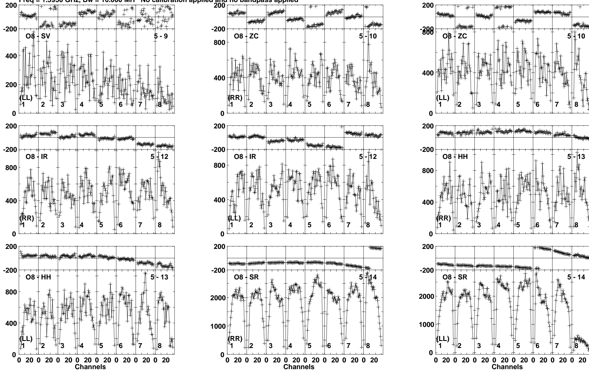
Lower frame: Micro Ampl Jy Top frame: Phas deg Vector averaged cross-power spectrum Baseline: O8 (05) - SV (09) Timerange: 00/17:03:51 to 00/17:04:59
