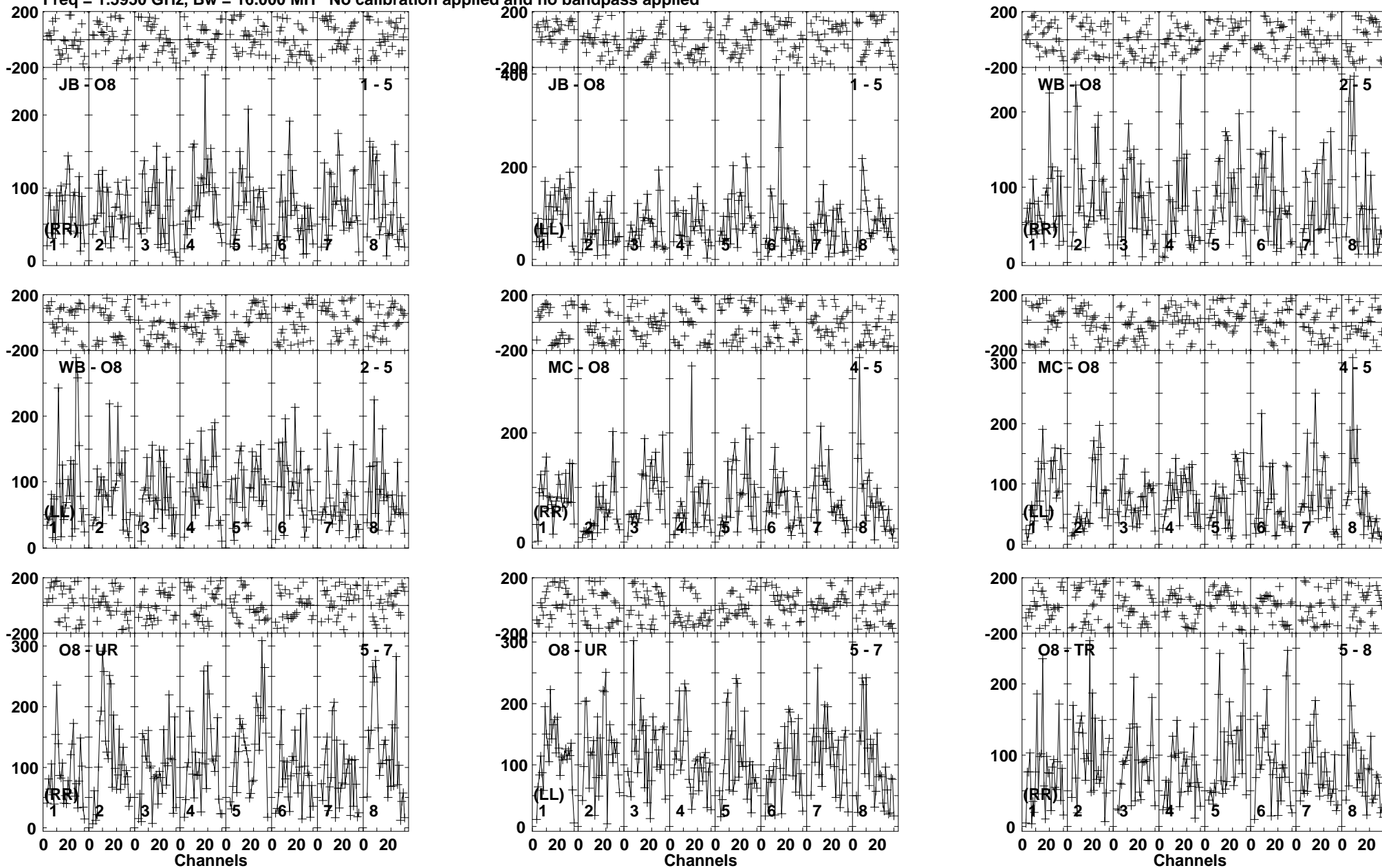
Lower frame: Micro Ampl Jy Top frame: Phas deg Vector averaged cross-power spectrum Baseline: JB (01) - O8 (05) Timerange: 00:12:54:01 to 00:12:57:49
