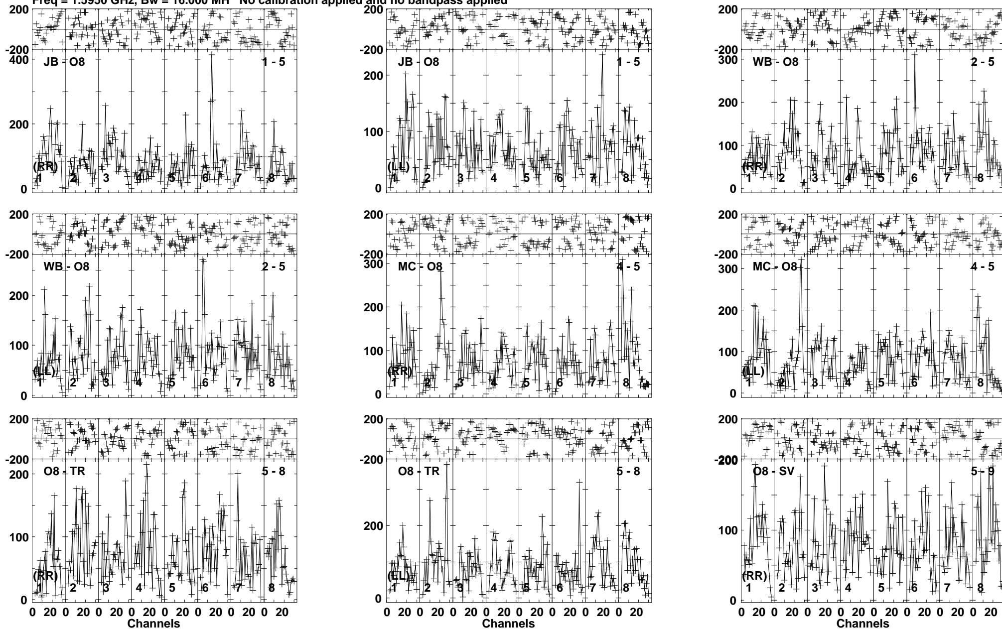
Lower frame: Micro Ampl Jy Top frame: Phas deg Vector averaged cross-power spectrum Baseline: JB (01) - O8 (05) Timerange: 00/15:07:31 to 00/15:11:19
