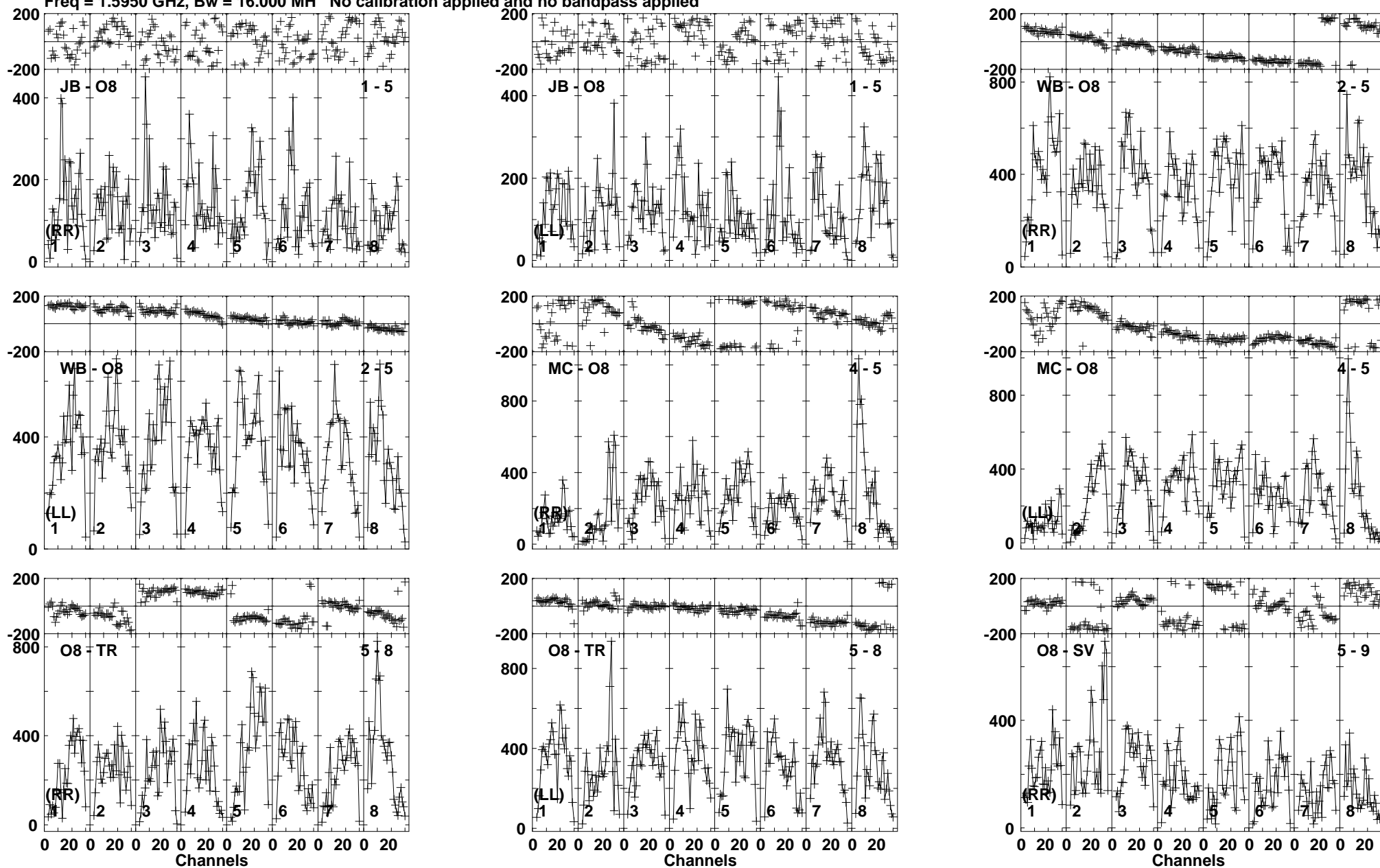
Lower frame: Micro Ampl Jy Top frame: Phas deg Vector averaged cross-power spectrum Baseline: JB (01) - O8 (05) Timerange: 00/15:54:31 to 00/15:56:29
