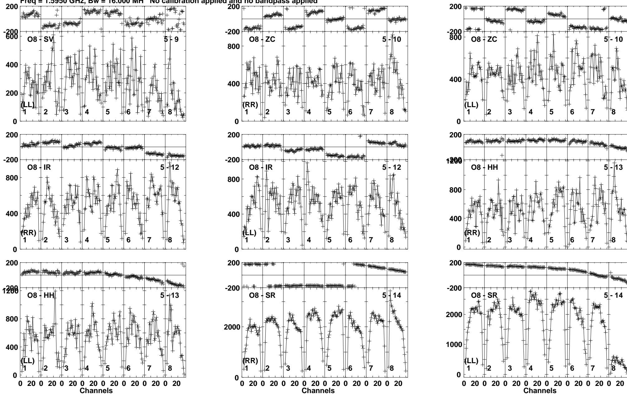
Lower frame: Micro Ampl Jy Top frame: Phas deg Vector averaged cross-power spectrum Baseline: O8 (05) - SV (09) Timerange: 00/16:53:21 to 00/16:54:29
