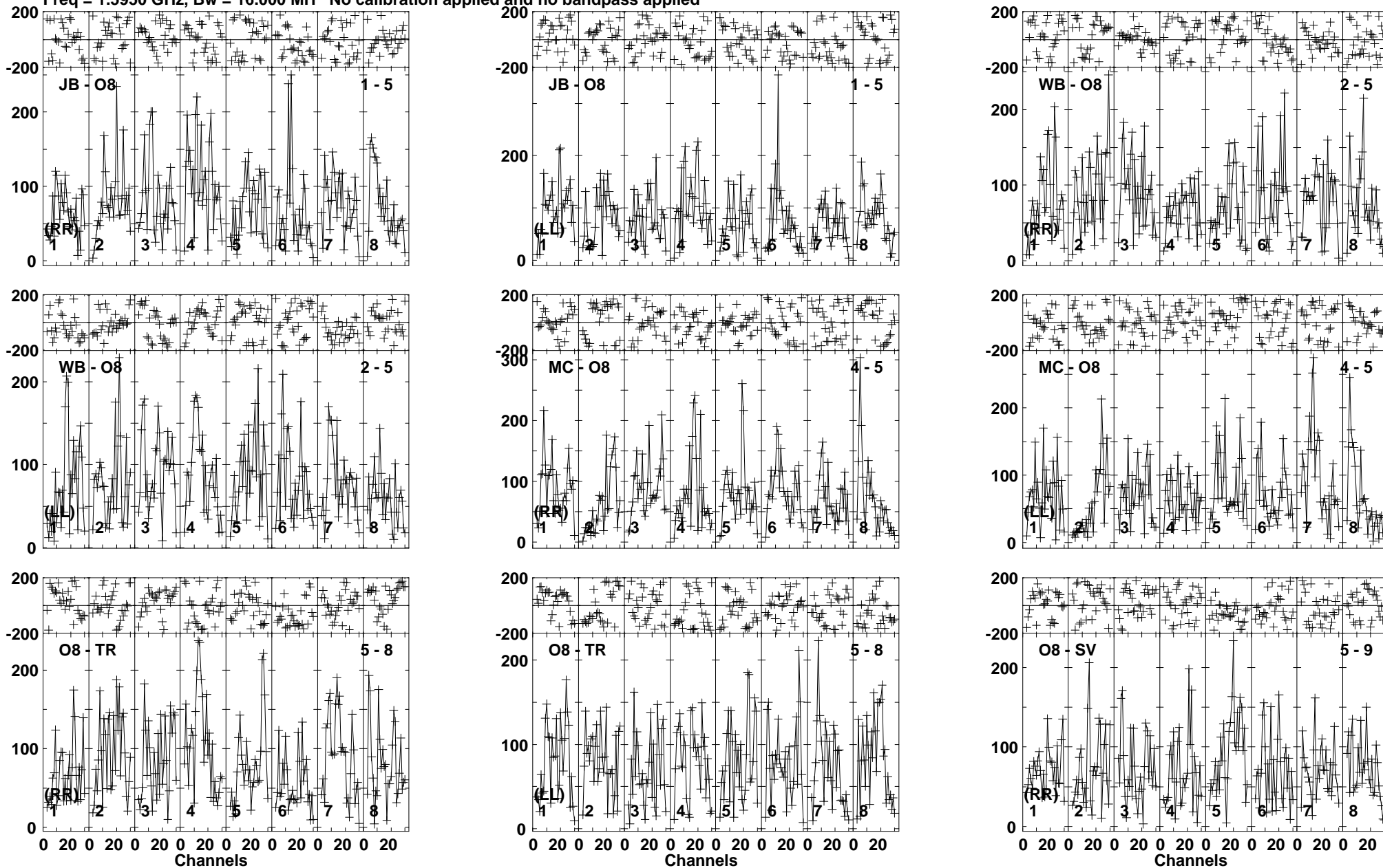
Lower frame: Micro Ampl Jy Top frame: Phas deg Vector averaged cross-power spectrum Baseline: JB (01) - O8 (05) Timerange: 00/16:07:01 to 00/16:10:49
