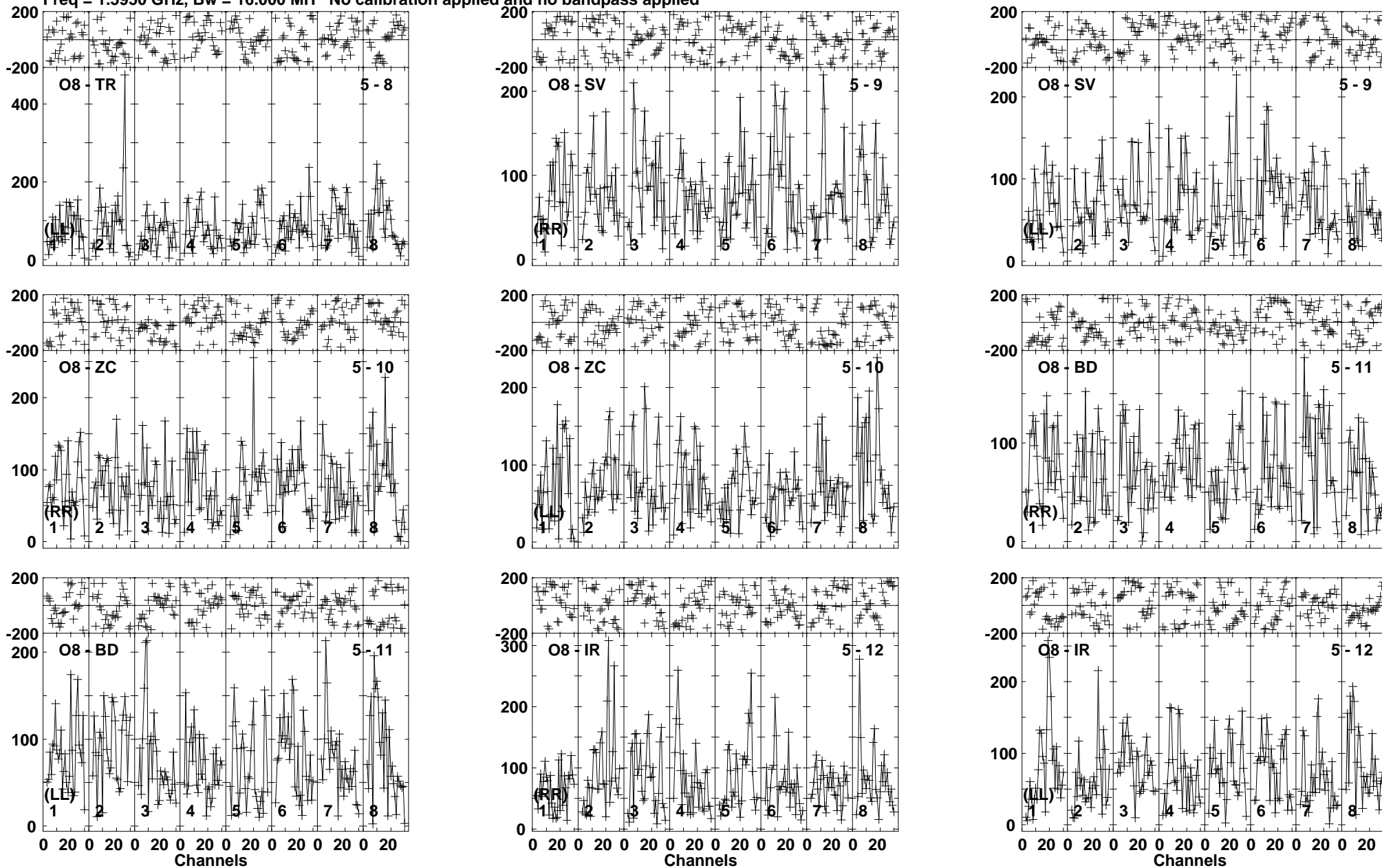
Lower frame: Micro Ampl Jy Top frame: Phas deg Vector averaged cross-power spectrum Baseline: O8 (05) - TR (08) Timerange: 00:12:43:31 to 00:12:47:19
