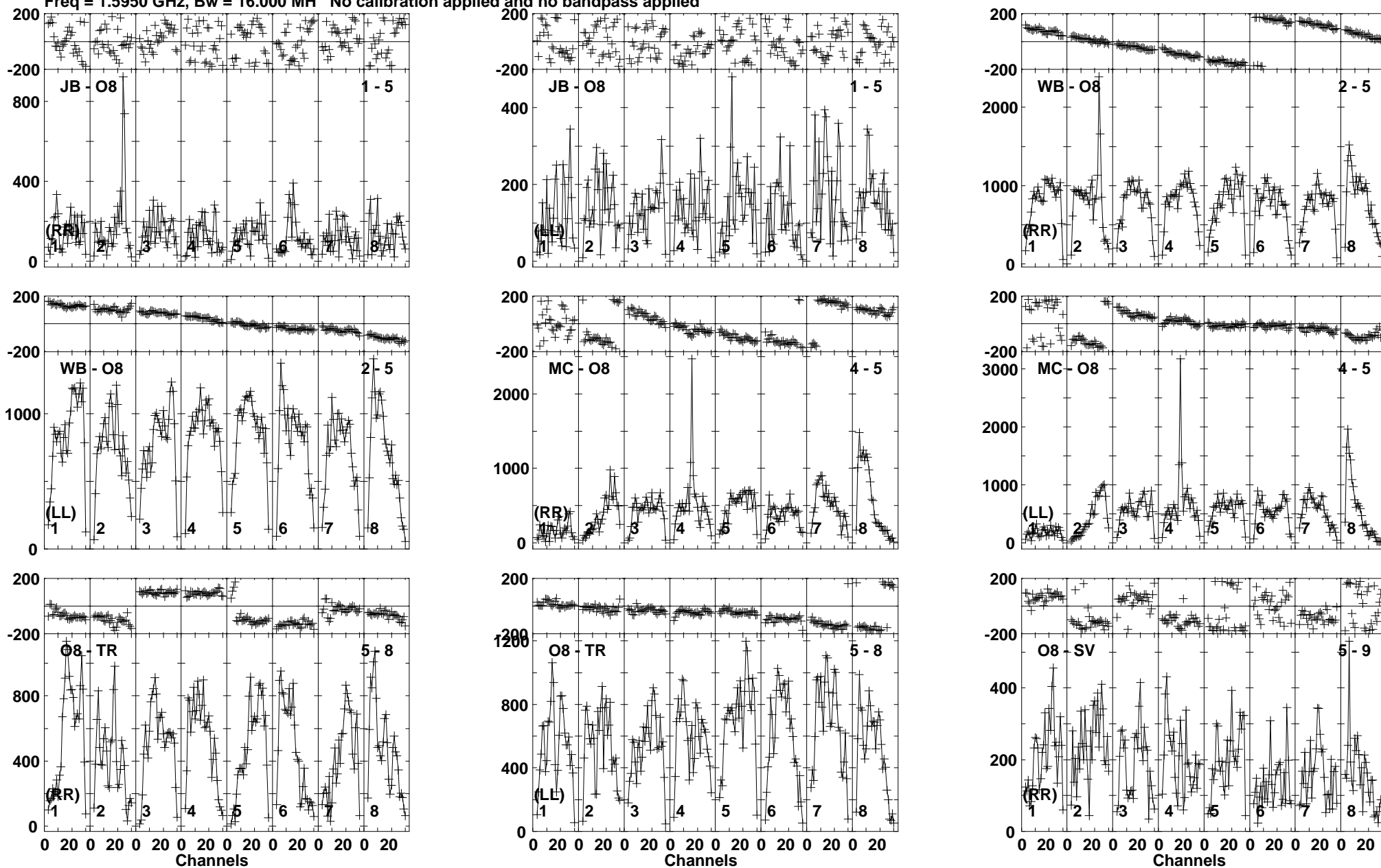
Lower frame: Micro Ampl Jy Top frame: Phas deg Vector averaged cross-power spectrum Baseline: JB (01) - O8 (05) Timerange: 00/17:14:21 to 00/17:15:29
