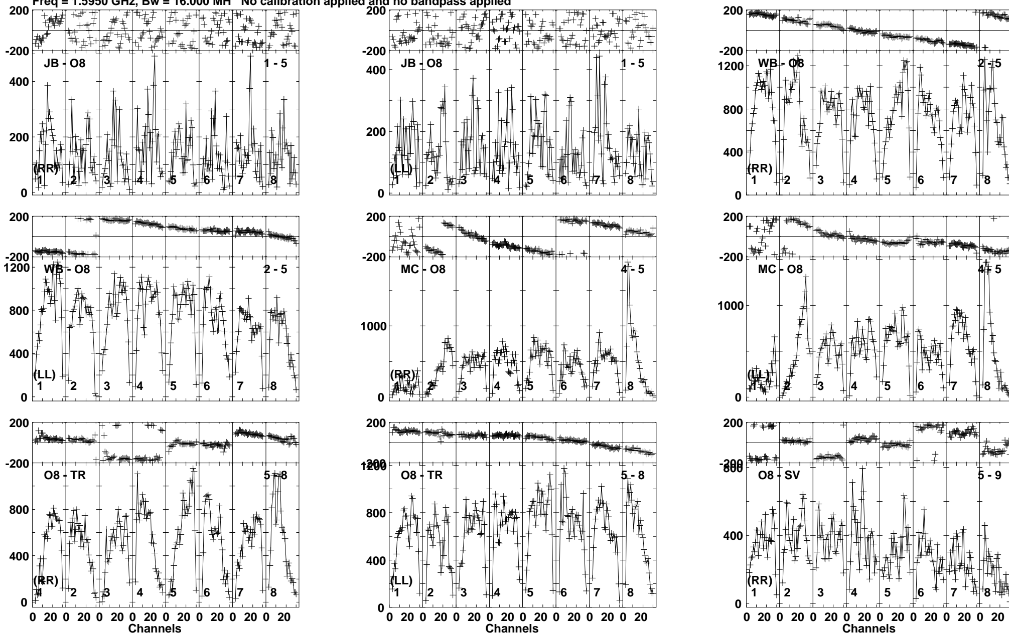
Lower frame: Micro Ampl Jy Top frame: Phas deg Vector averaged cross-power spectrum Baseline: JB (01) - O8 (05) Timerange: 00/17:03:51 to 00/17:04:59
