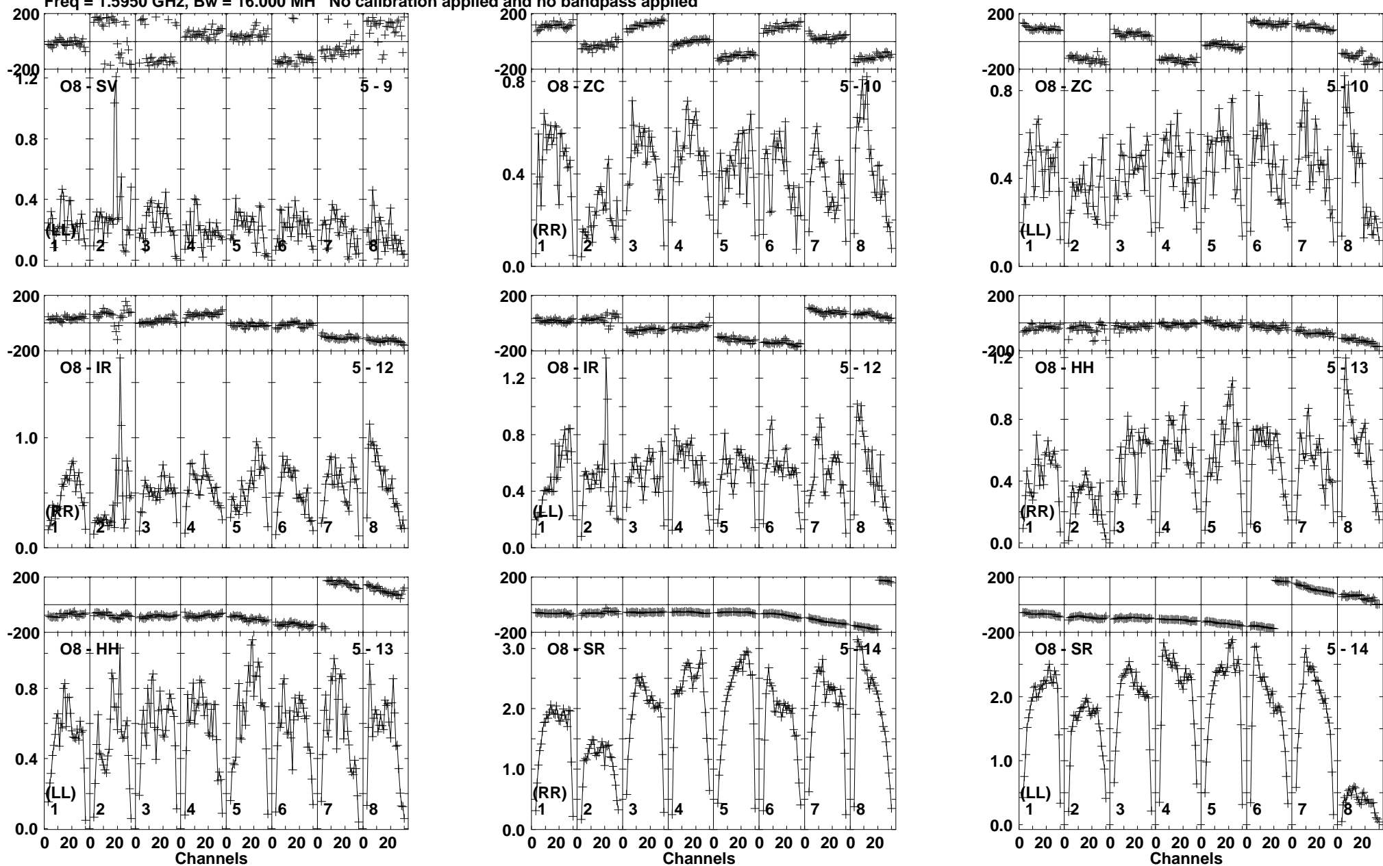
Lower frame: Milli Ampl Jy Top frame: Phas deg Vector averaged cross-power spectrum Baseline: O8 (05) - SV (09) Timerange: 00/16:32:21 to 00/16:33:29
