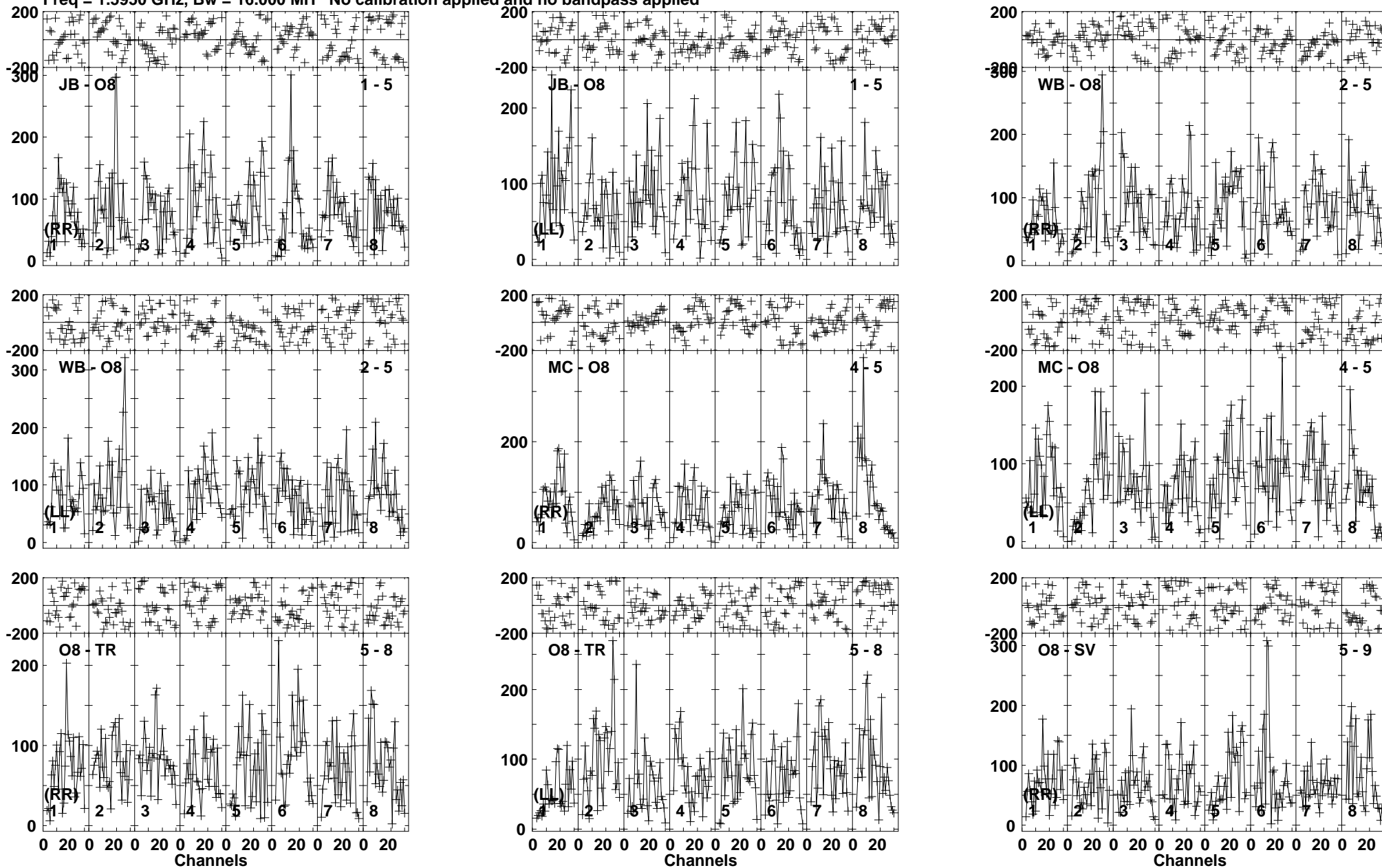
Lower frame: Micro Ampl Jy Top frame: Phas deg Vector averaged cross-power spectrum Baseline: JB (01) - O8 (05) Timerange: 00/14:41:01 to 00/14:44:49
