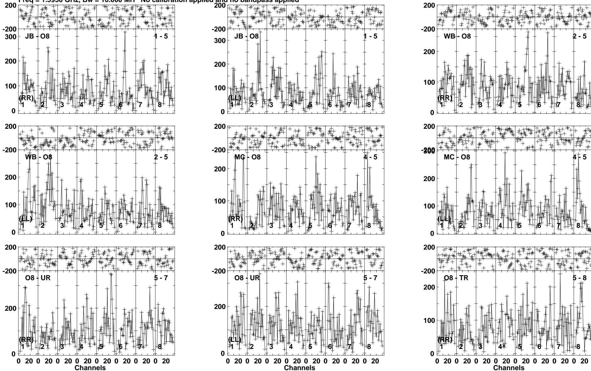
Lower frame: Micro Ampl Jy Top frame: Phas deg Vector averaged cross-power spectrum Baseline: JB (01) - O8 (05) Timerange: 00/14:36:01 to 00/14:39:49
