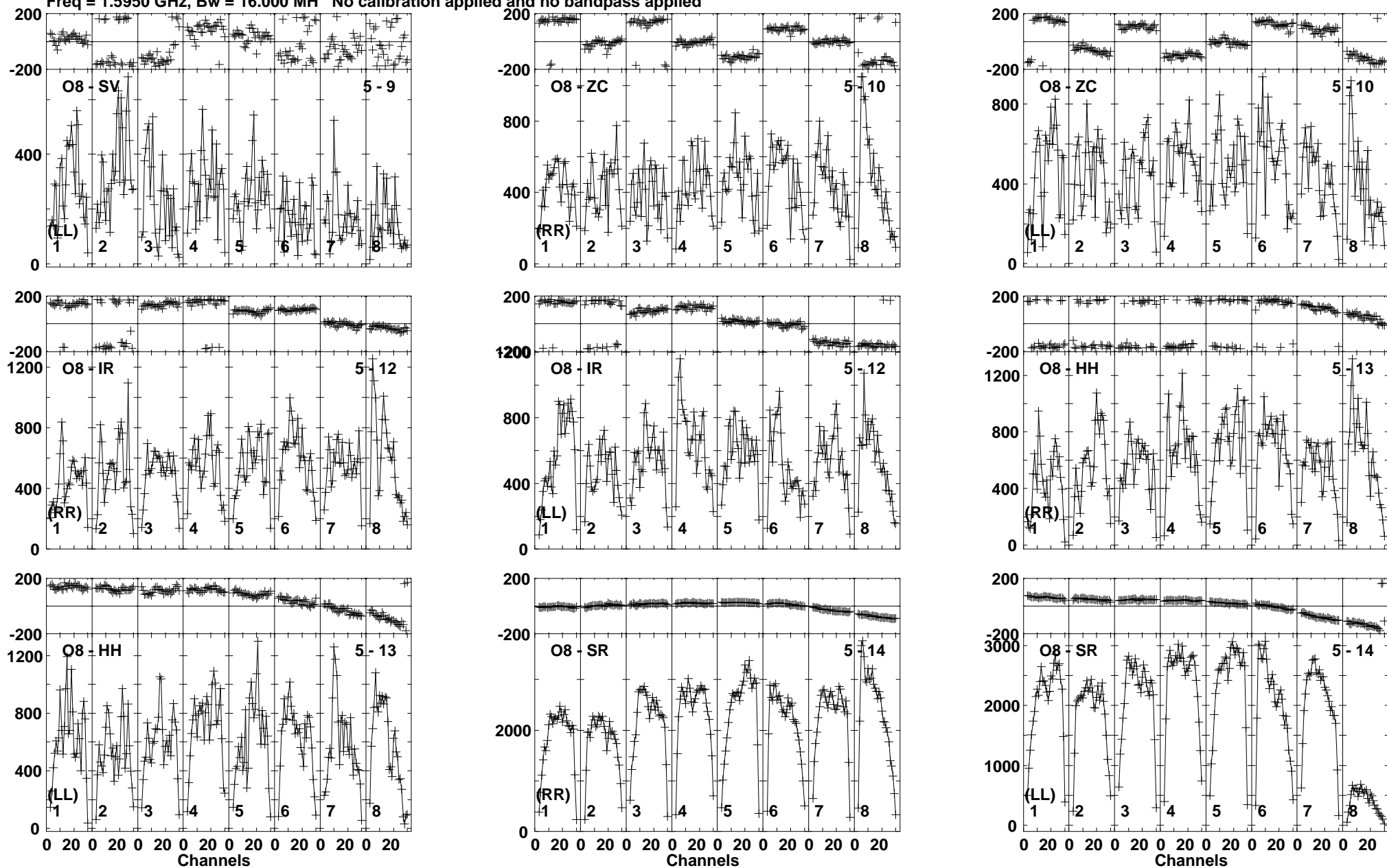
Lower frame: Micro Ampl Jy Top frame: Phas deg Vector averaged cross-power spectrum Baseline: O8 (05) - SV (09) Timerange: 00/13:57:51 to 00/13:58:59
