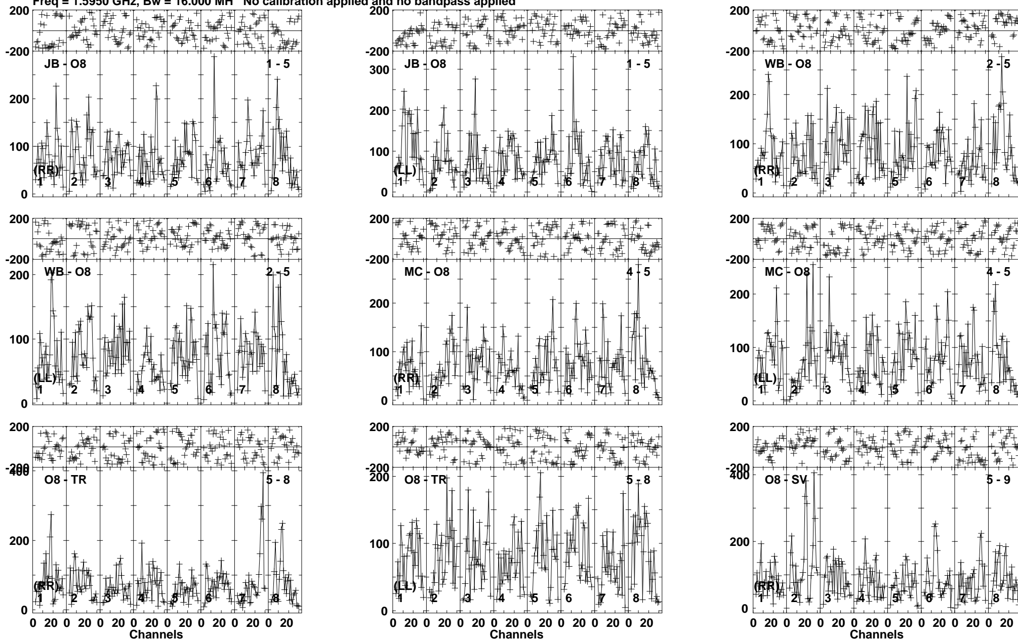
Lower frame: Micro Ampl Jy Top frame: Phas deg Vector averaged cross-power spectrum Baseline: JB (01) - O8 (05) Timerange: 00/16:23:01 to 00/16:26:49
