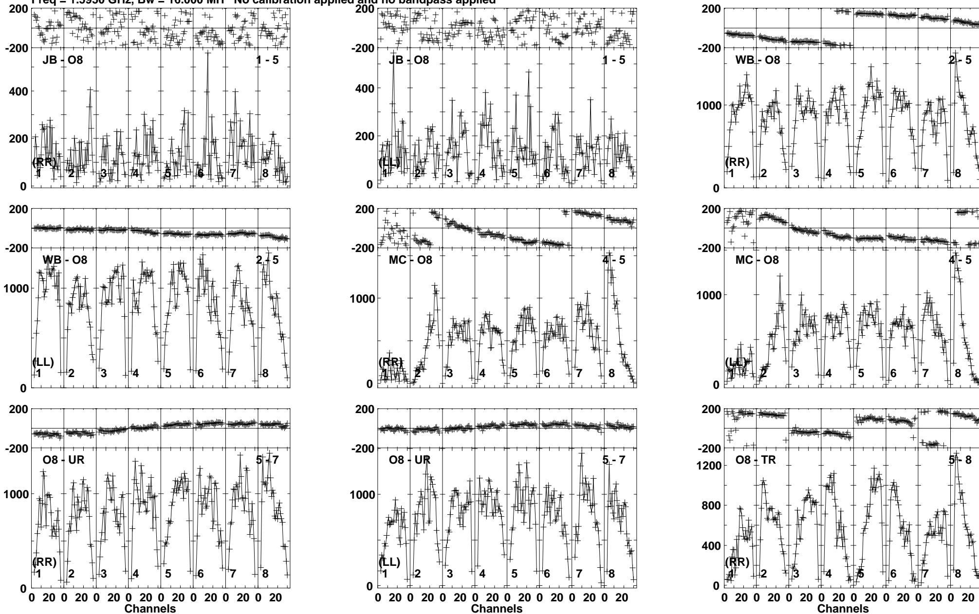
Lower frame: Micro Ampl Jy Top frame: Phas deg Vector averaged cross-power spectrum Baseline: JB (01) - O8 (05) Timerange: 00/13:52:51 to 00/13:53:59
