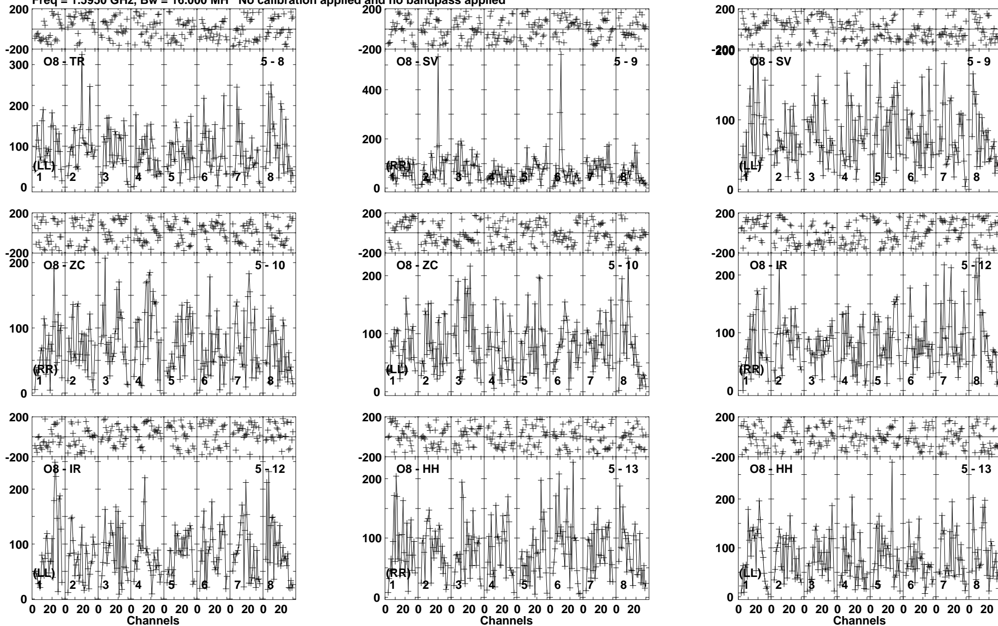
Lower frame: Micro Ampl Jy Top frame: Phas deg Vector averaged cross-power spectrum Baseline: O8 (05) - TR (08) Timerange: 00/14:30:31 to 00/14:34:19
