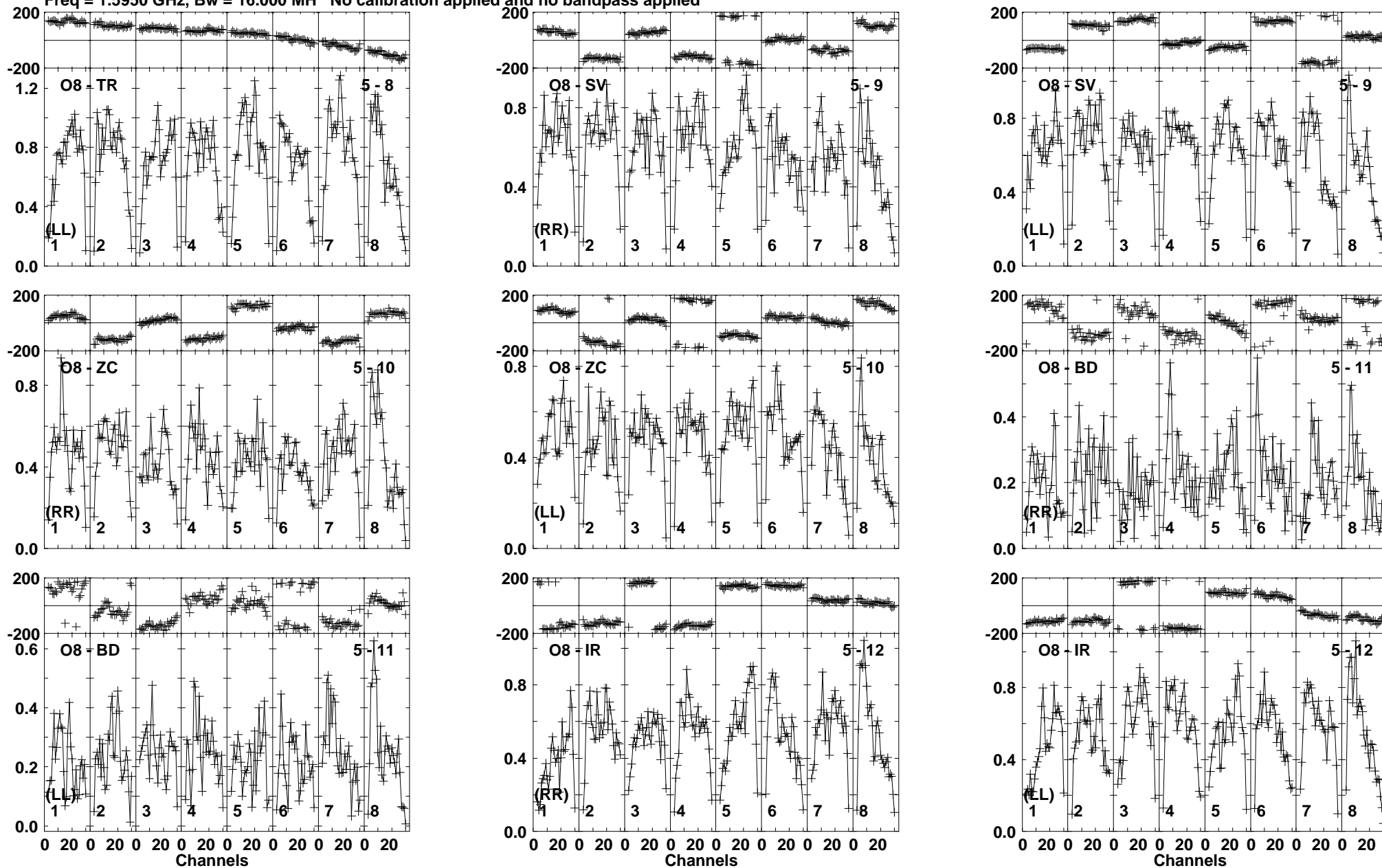
Lower frame: Milli Ampl Jy Top frame: Phas deg Vector averaged cross-power spectrum Baseline: O8 (05) - TR (08) Timerange: 00:12:47:51 to 00:12:48:59
