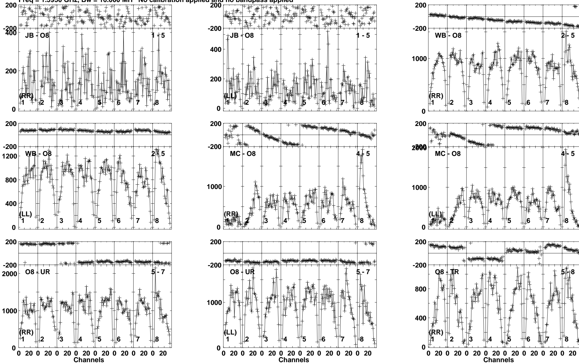
Lower frame: Micro Ampl Jy Top frame: Phas deg Vector averaged cross-power spectrum Baseline: JB (01) - O8 (05) Timerange: 00:12:37:21 to 00:12:38:29
