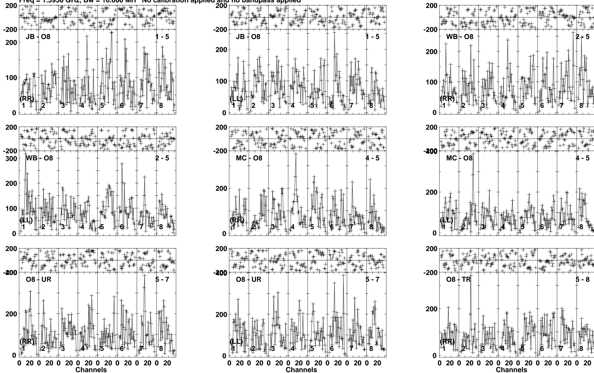
Lower frame: Micro Ampl Jy Top frame: Phas deg Vector averaged cross-power spectrum Baseline: JB (01) - O8 (05) Timerange: 00/13:22:31 to 00/13:26:19
