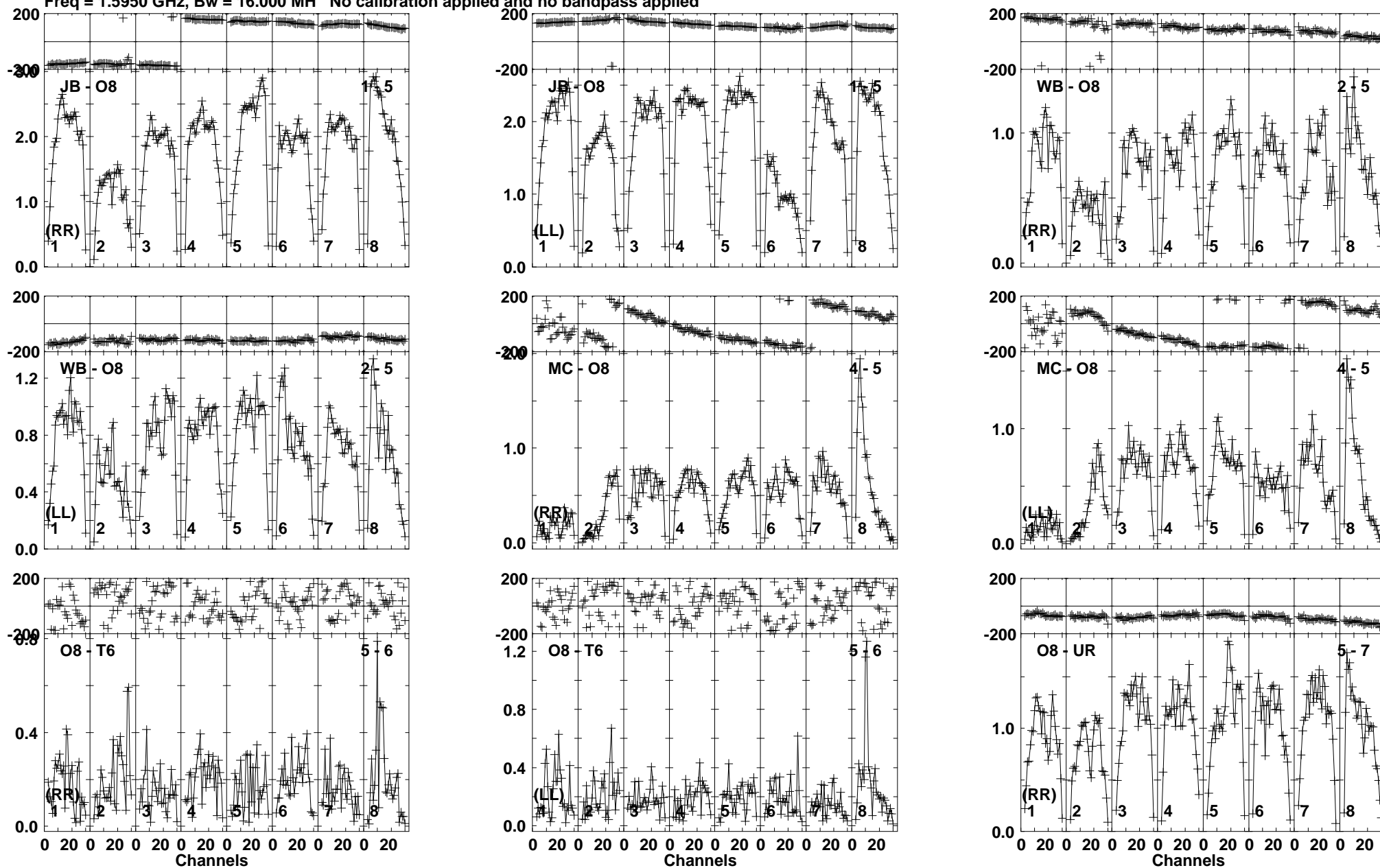
Lower frame: Milli Ampl Jy Top frame: Phas deg Vector averaged cross-power spectrum Baseline: JB (01) - O8 (05) Timerange: 00/11:02:51 to 00/11:03:59
