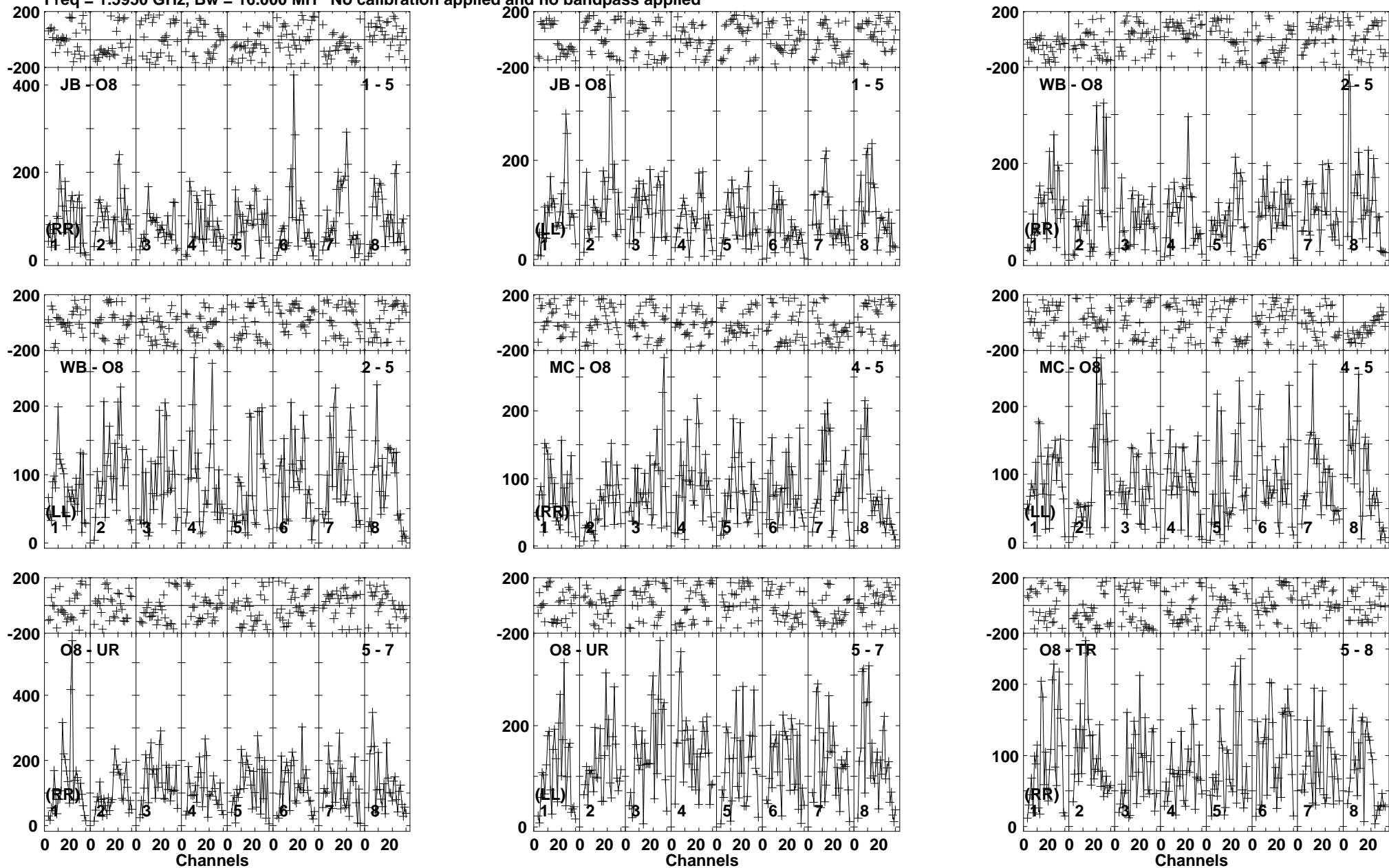
Lower frame: Micro Ampl Jy Top frame: Phas deg Vector averaged cross-power spectrum Baseline: JB (01) - O8 (05) Timerange: 00/12:22:31 to 00/12:26:19
