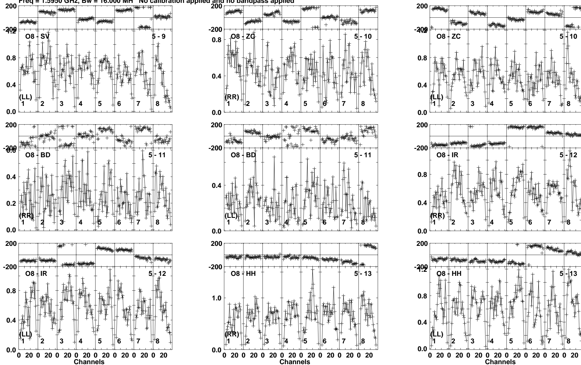
Lower frame: Milli Ampl Jy Top frame: Phas deg Vector averaged cross-power spectrum Baseline: O8 (05) - SV (09) Timerange: 00:12:42:21 to 00:12:43:29
