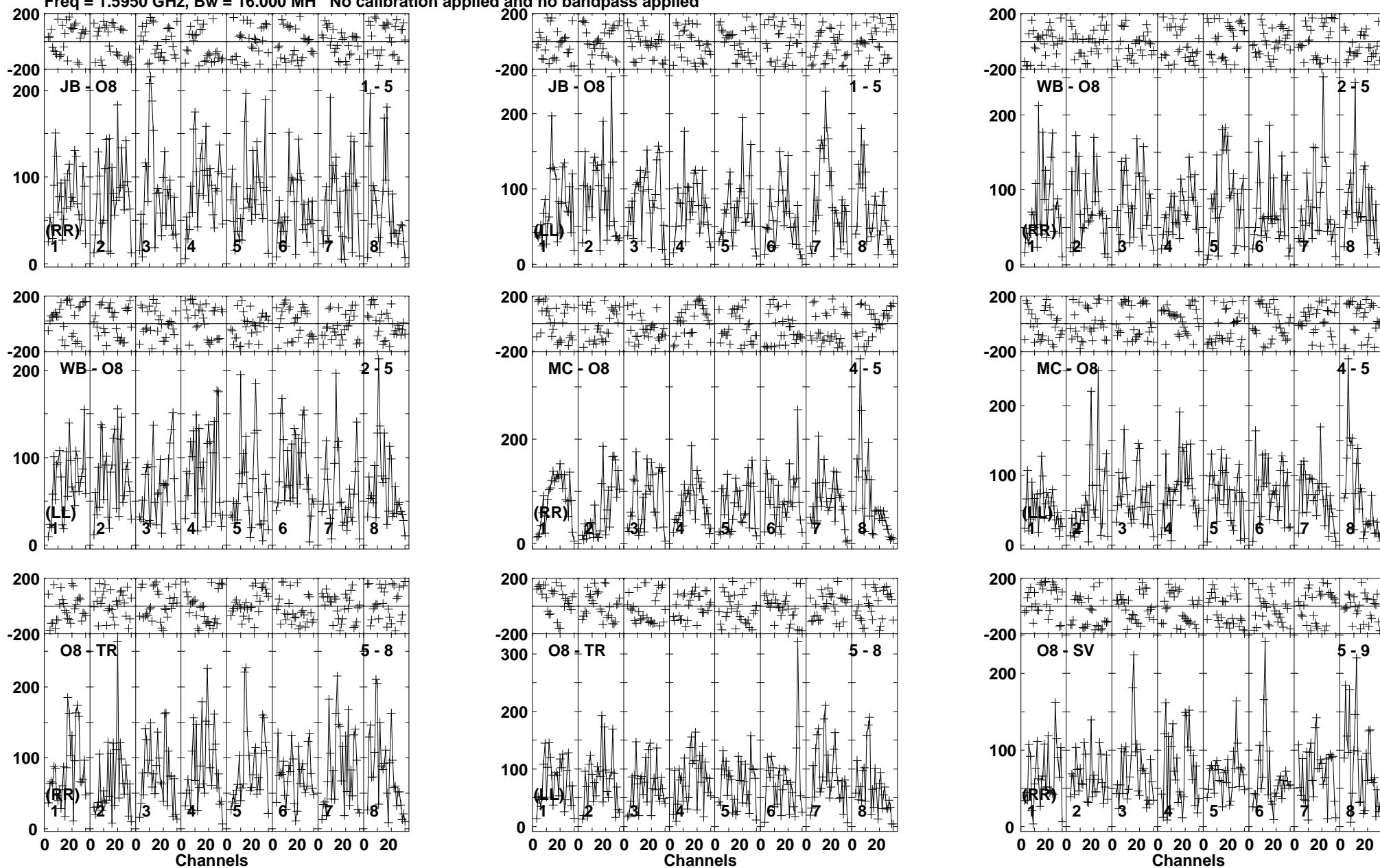
Lower frame: Micro Ampl Jy Top frame: Phas deg Vector averaged cross-power spectrum Baseline: JB (01) - O8 (05) Timerange: 00/15:49:31 to 00/15:53:19
