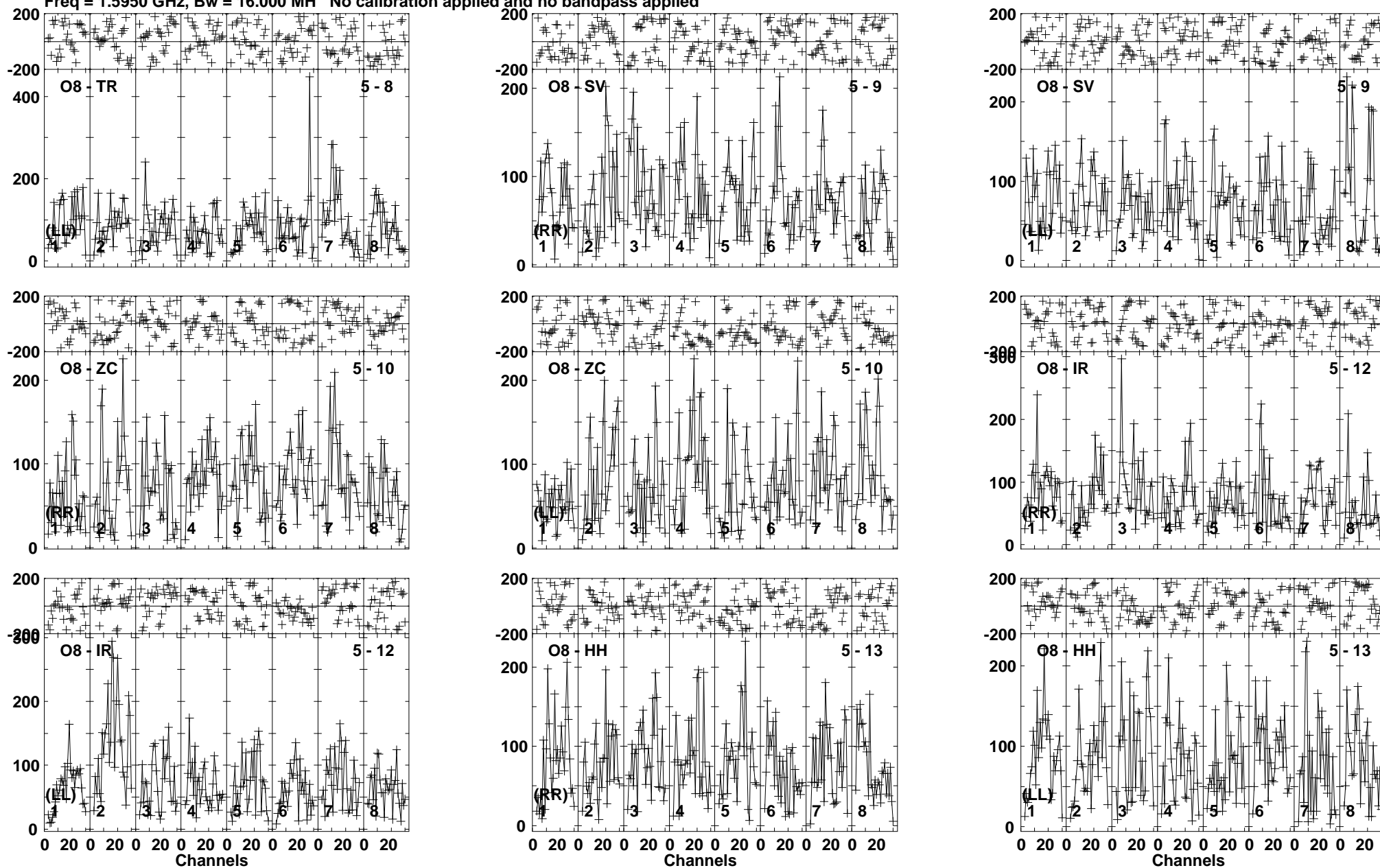
Lower frame: Micro Ampl Jy Top frame: Phas deg Vector averaged cross-power spectrum Baseline: O8 (05) - TR (08) Timerange: 00/14:15:01 to 00/14:18:49
