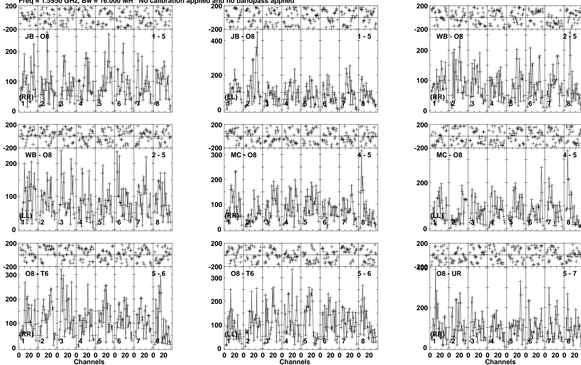
Lower frame: Micro Ampl Jy Top frame: Phas deg Vector averaged cross-power spectrum Baseline: JB (01) - O8 (05) Timerange: 00/10:37:31 to 00/10:41:19
