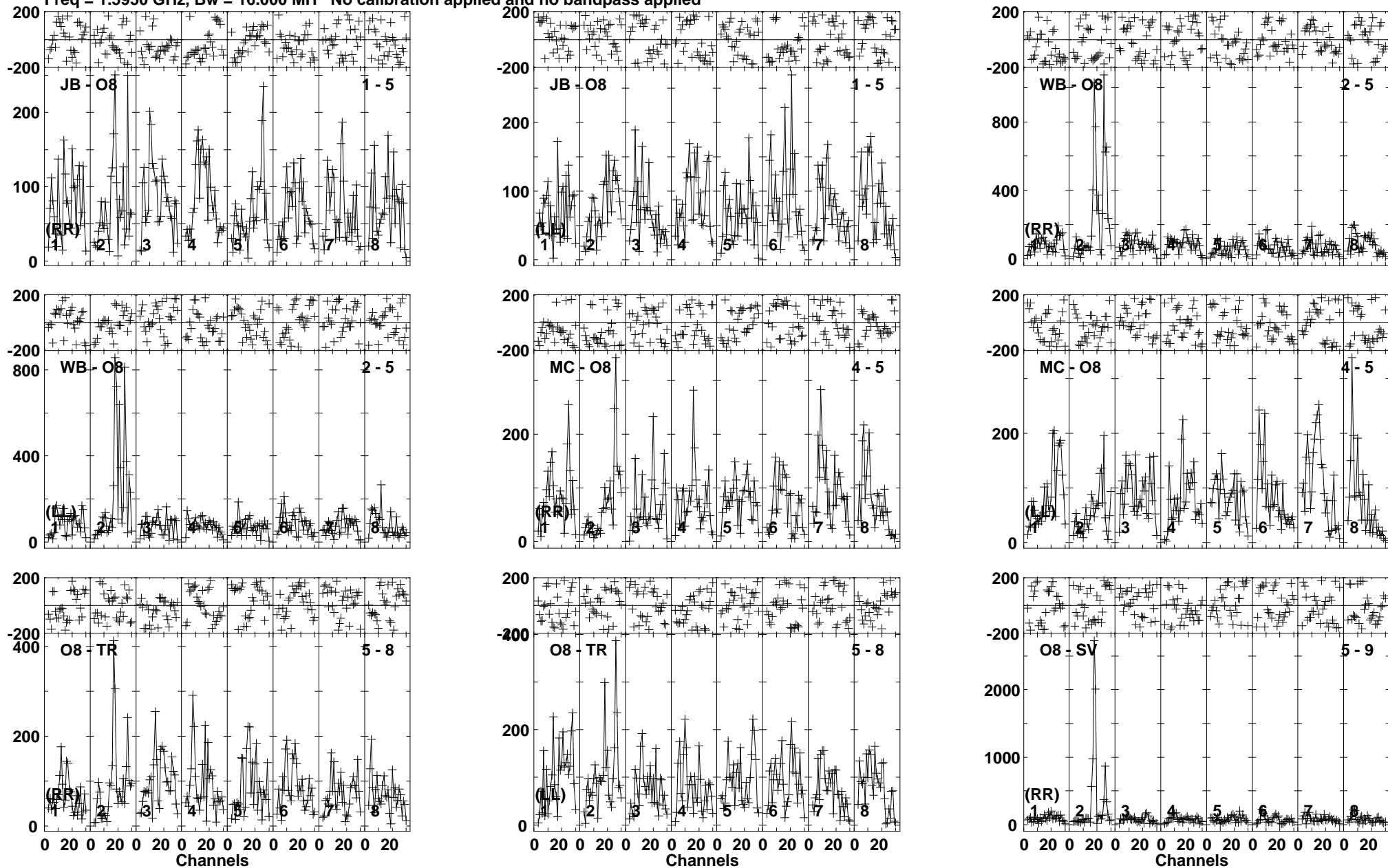
Lower frame: Micro Ampl Jy Top frame: Phas deg Vector averaged cross-power spectrum Baseline: JB (01) - O8 (05) Timerange: 00/16:38:31 to 00/16:42:19
