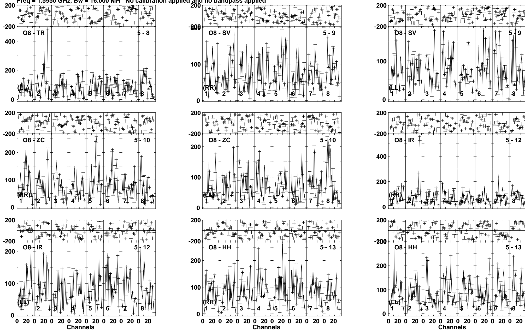
Lower frame: Micro Ampl Jy Top frame: Phas deg Vector averaged cross-power spectrum Baseline: O8 (05) - TR (08) Timerange: 00/13:22:31 to 00/13:26:19
