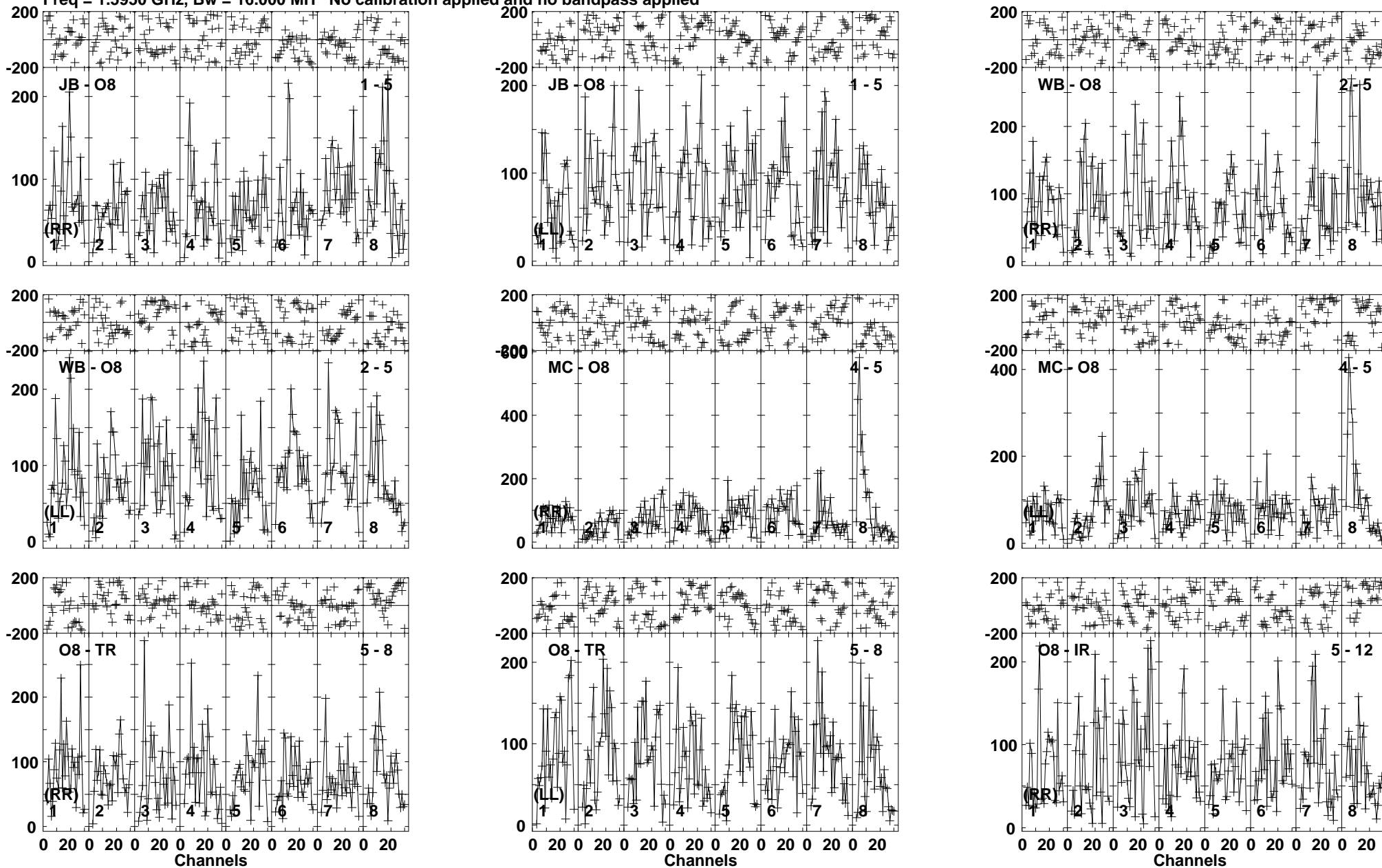
Lower frame: Micro Ampl Jy Top frame: Phas deg Vector averaged cross-power spectrum Baseline: JB (01) - O8 (05) Timerange: 00/17:57:31 to 00/18:01:19
