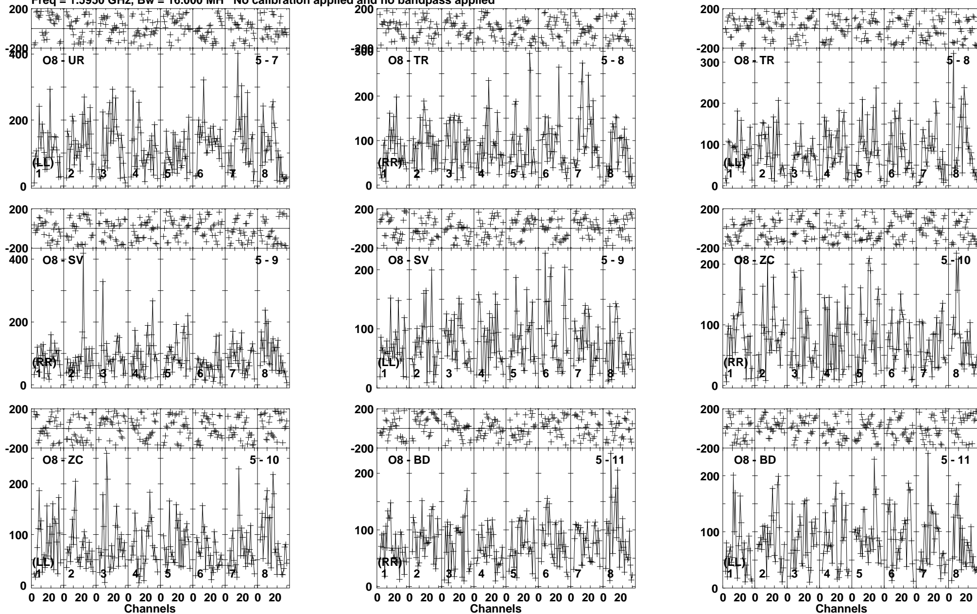
Lower frame: Micro Ampl Jy Top frame: Phas deg Vector averaged cross-power spectrum Baseline: O8 (05) - UR (07) Timerange: 00/11:35:31 to 00/11:39:19
