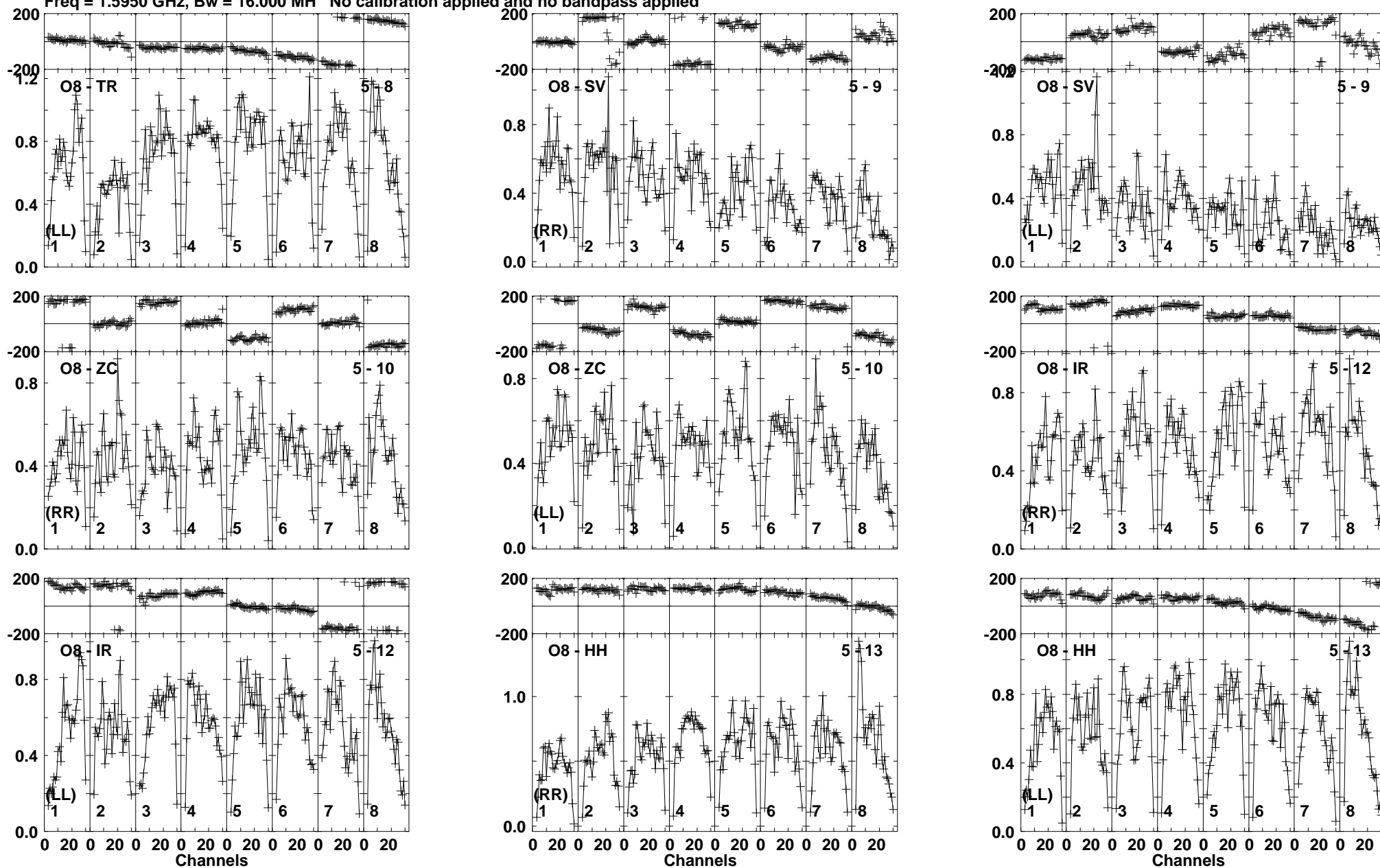
Lower frame: Milli Ampl Jy Top frame: Phas deg Vector averaged cross-power spectrum Baseline: O8 (05) - TR (08) Timerange: 00/13:31:51 to 00/13:32:59
