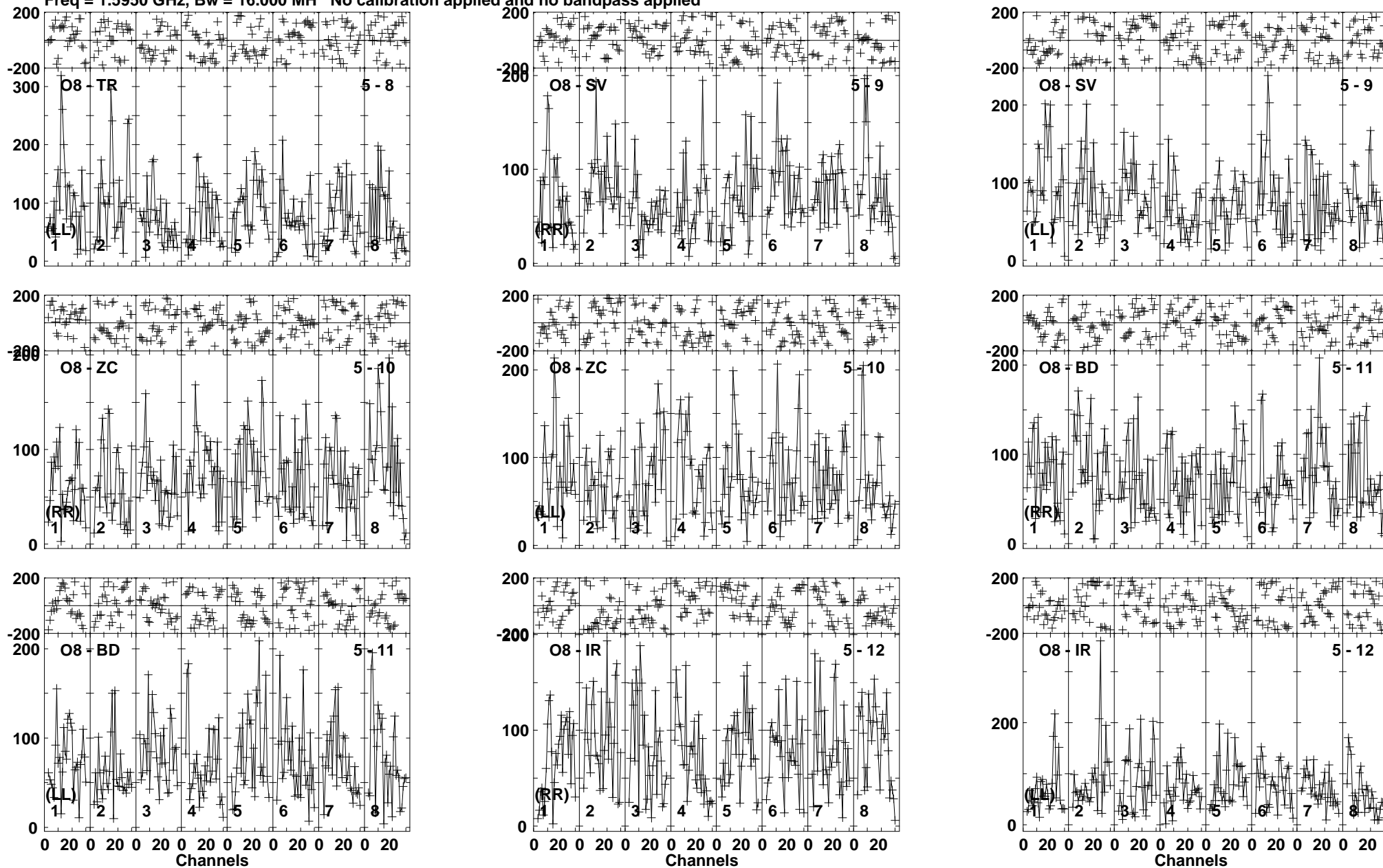
Lower frame: Micro Ampl Jy Top frame: Phas deg Vector averaged cross-power spectrum Baseline: O8 (05) - TR (08) Timerange: 00/12:54:01 to 00/12:57:49
