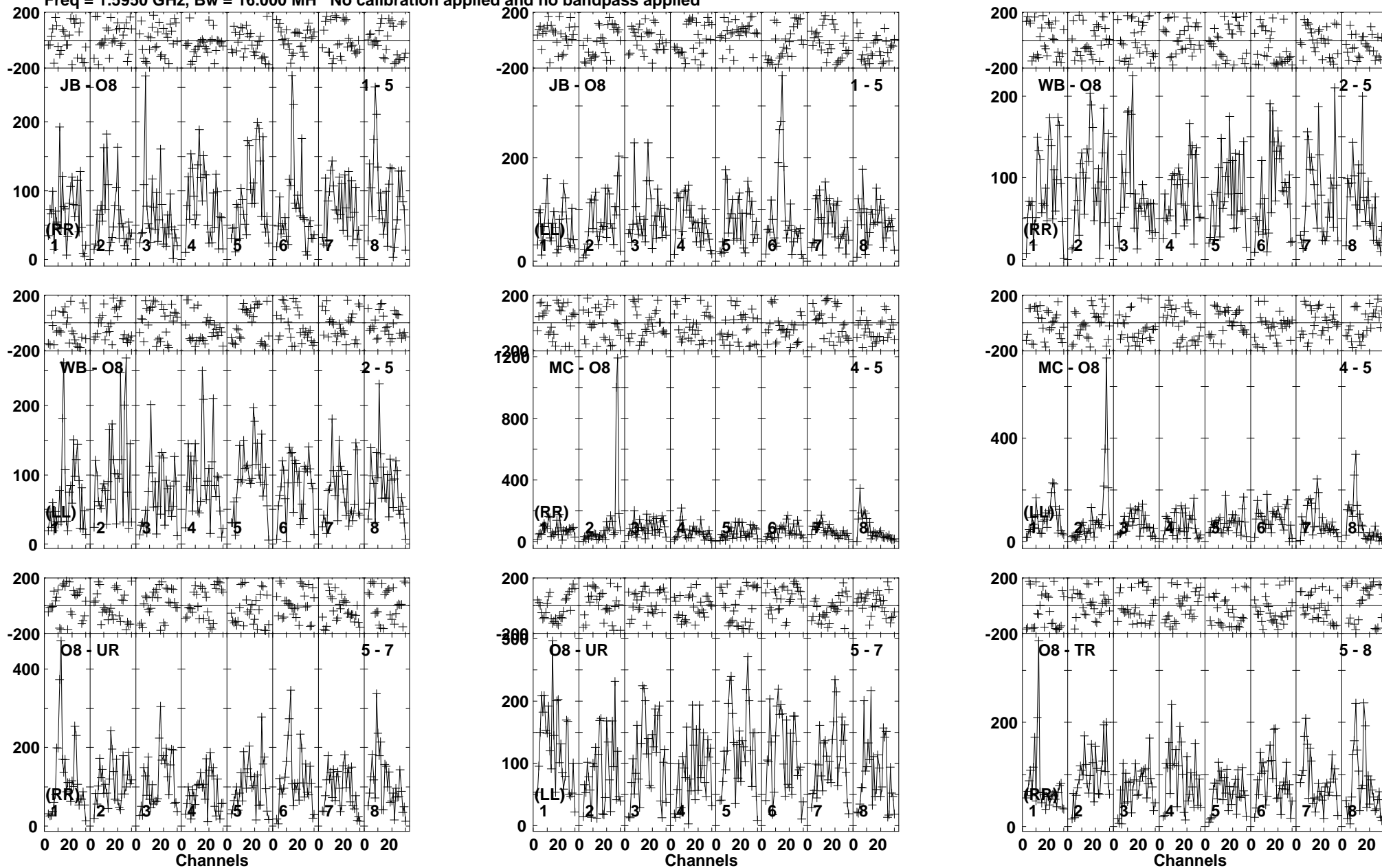
Lower frame: Micro Ampl Jy Top frame: Phas deg Vector averaged cross-power spectrum Baseline: JB (01) - O8 (05) Timerange: 00/13:48:31 to 00/13:52:19
