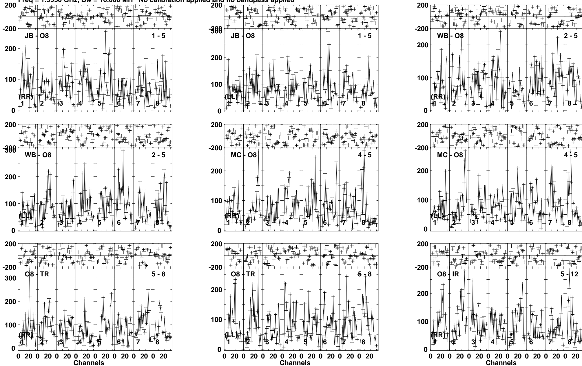
Lower frame: Micro Ampl Jy Top frame: Phas deg Vector averaged cross-power spectrum Baseline: JB (01) - O8 (05) Timerange: 00/17:47:01 to 00/17:50:49
