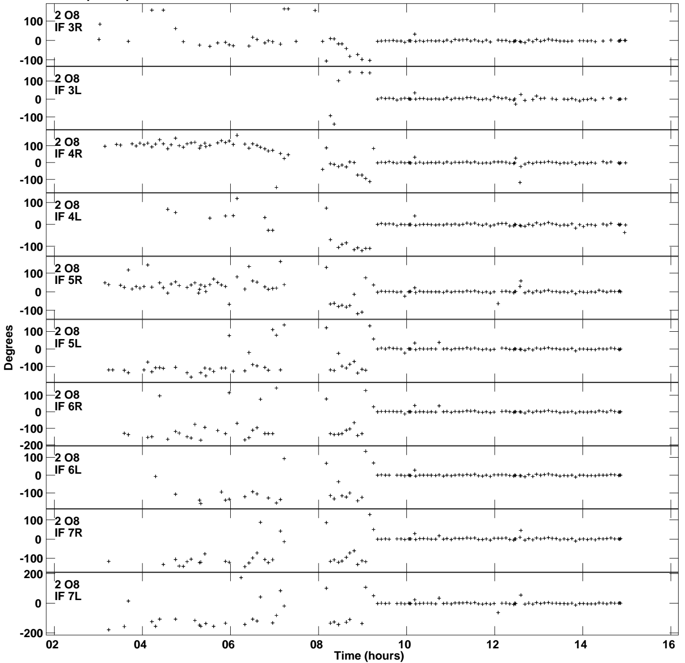
Plot file version 3 created 03-SEP-2018 10:35:08 Gain phs vs UTC time for J1312+2531.MULTI.1 SN 1 Rpol & Lpol IF 1 - 8
