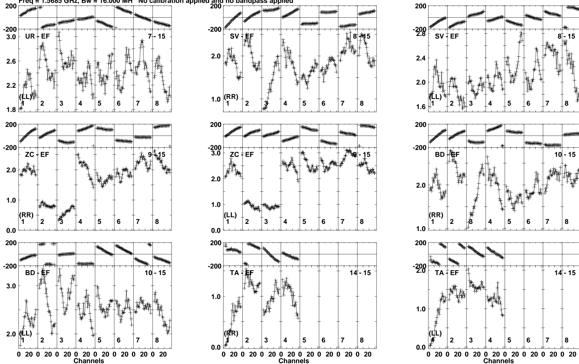
Lower frame: Milli Ampl Jy Top frame: Phas deg Vector averaged cross-power spectrum Baseline: UR (07) - EF (15) Timerange: 00/09:30:11 to 00/09:31:39
