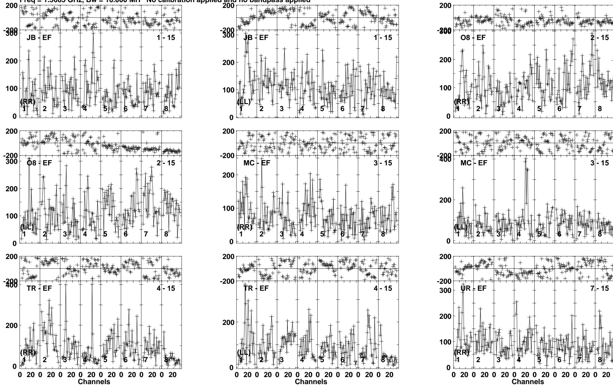
Lower frame: Micro Ampl Jy Top frame: Phas deg Vector averaged cross-power spectrum Baseline: JB (01) - EF (15) Timerange: 00/10:55:43 to 00/10:59:09
