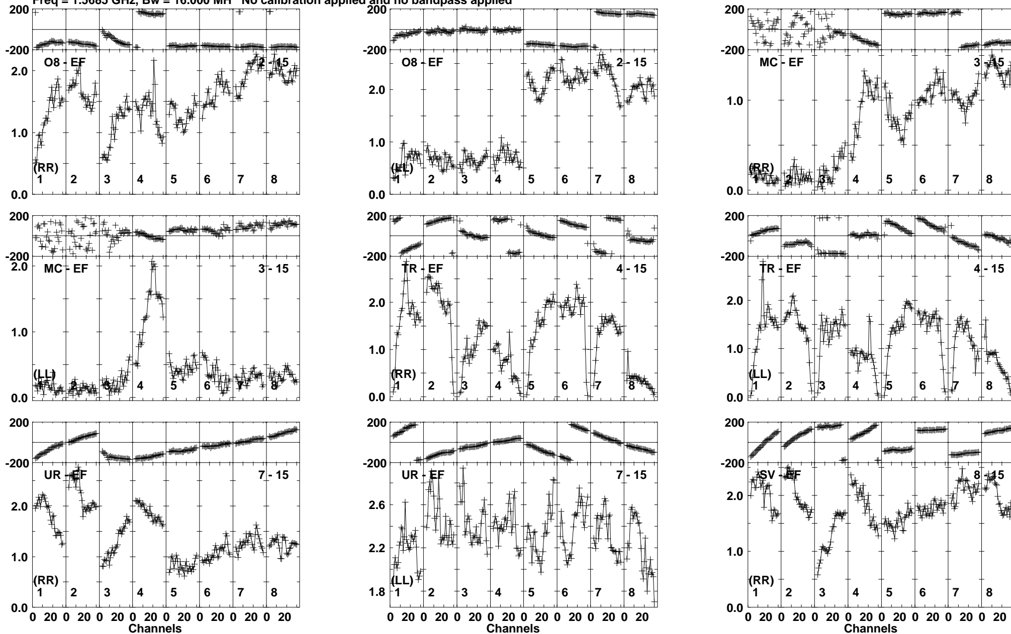
Lower frame: Milli Ampl Jy Top frame: Phas deg Vector averaged cross-power spectrum Baseline: O8 (02) - EF (15) Timerange: 00/10:22:13 to 00/10:23:39
