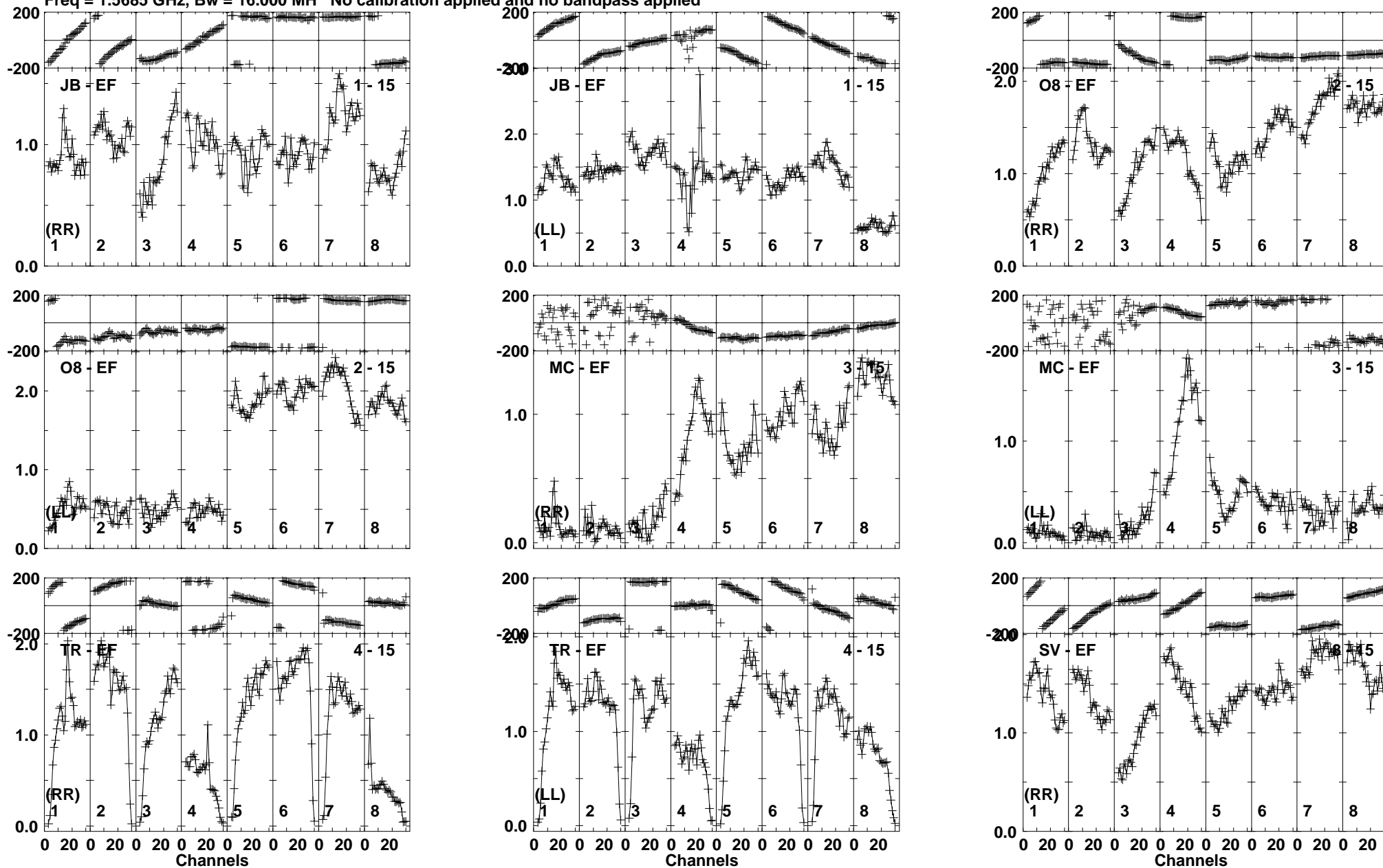
Lower frame: Milli Ampl Jy Top frame: Phas deg Vector averaged cross-power spectrum Baseline: JB (01) - EF (15) Timerange: 00/13:01:31 to 00/13:02:59
