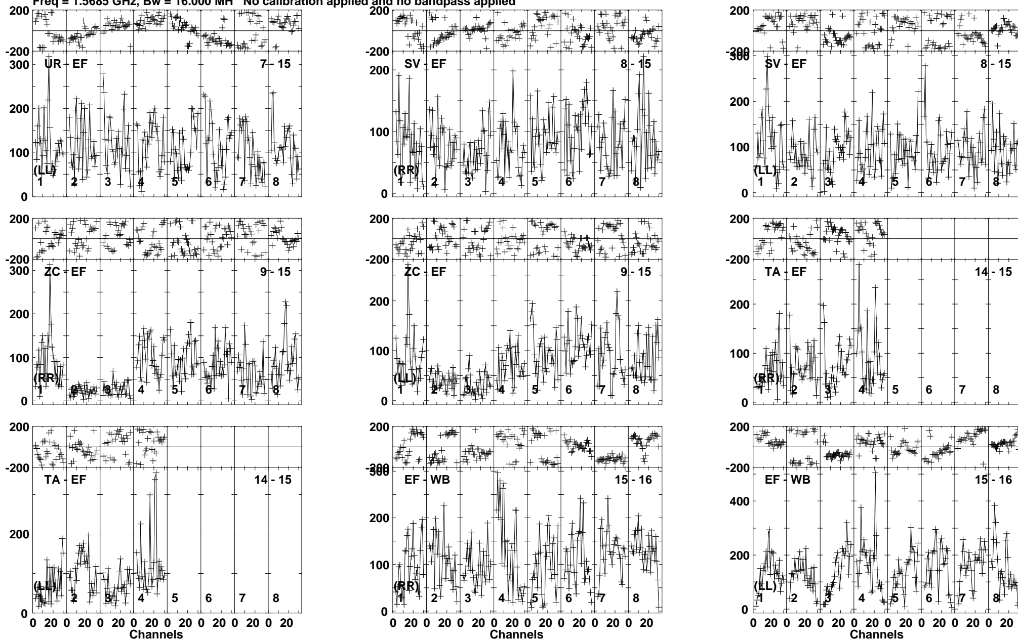
Lower frame: Micro Ampl Jy Top frame: Phas deg Vector averaged cross-power spectrum Baseline: UR (07) - EF (15) Timerange: 00/11:17:03 to 00/11:20:29
