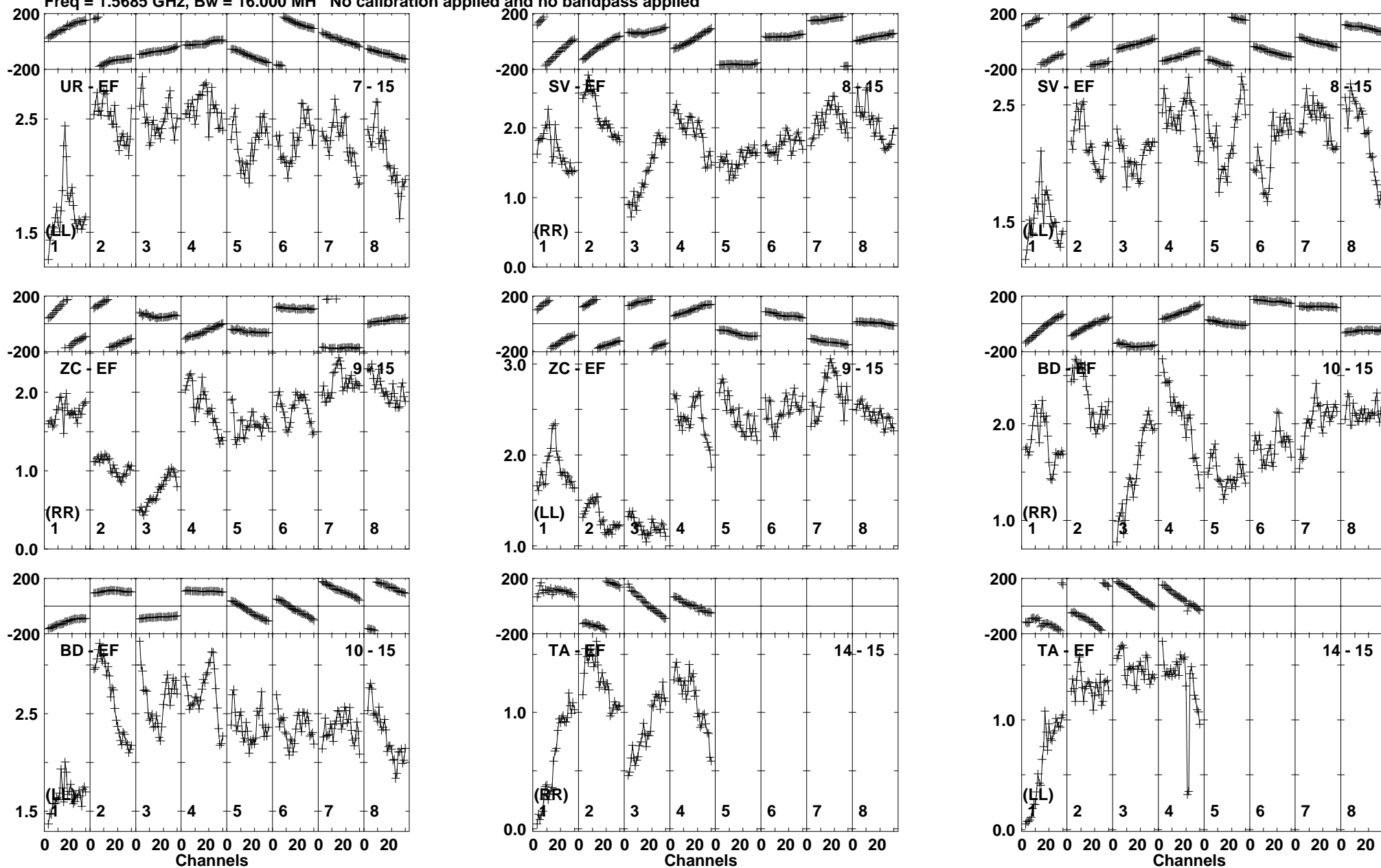
Lower frame: Milli Ampl Jy Top frame: Phas deg Vector averaged cross-power spectrum Baseline: UR (07) - EF (15) Timerange: 00/10:10:03 to 00/10:12:59
