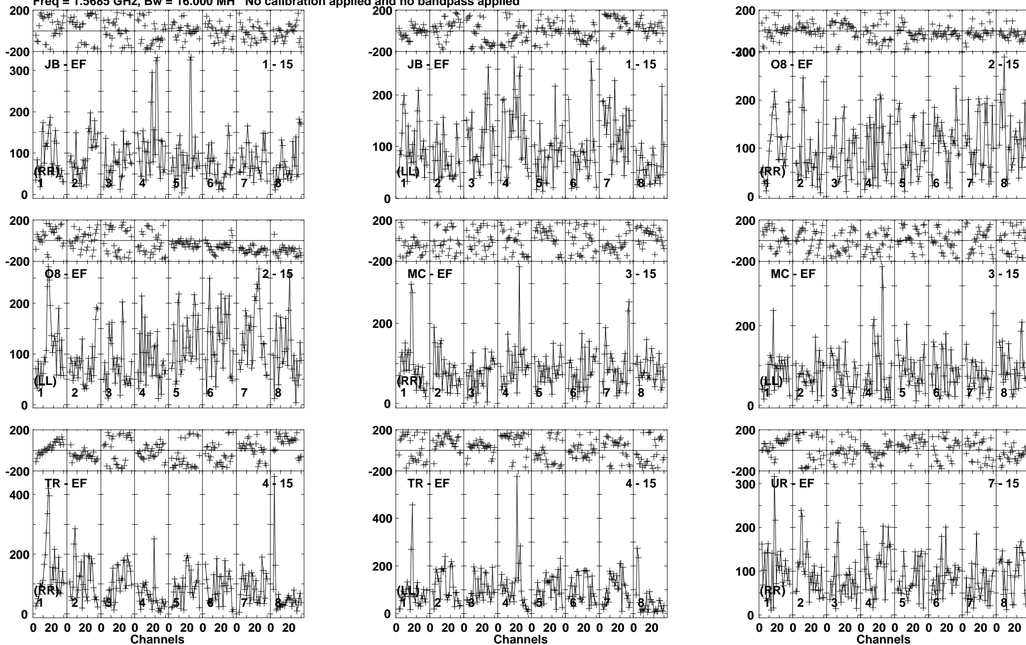
Lower frame: Micro Ampl Jy Top frame: Phas deg Vector averaged cross-power spectrum Baseline: JB (01) - EF (15) Timerange: 00/11:12:03 to 00/11:15:29
