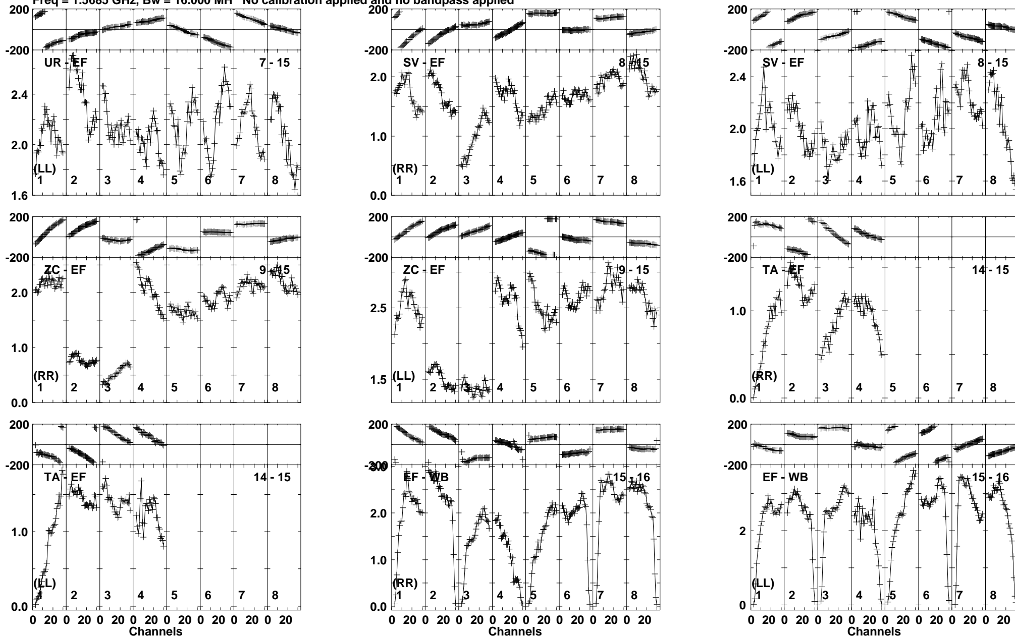
Lower frame: Milli Ampl Jy Top frame: Phas deg Vector averaged cross-power spectrum Baseline: UR (07) - EF (15) Timerange: 00/10:59:51 to 00/11:01:19
