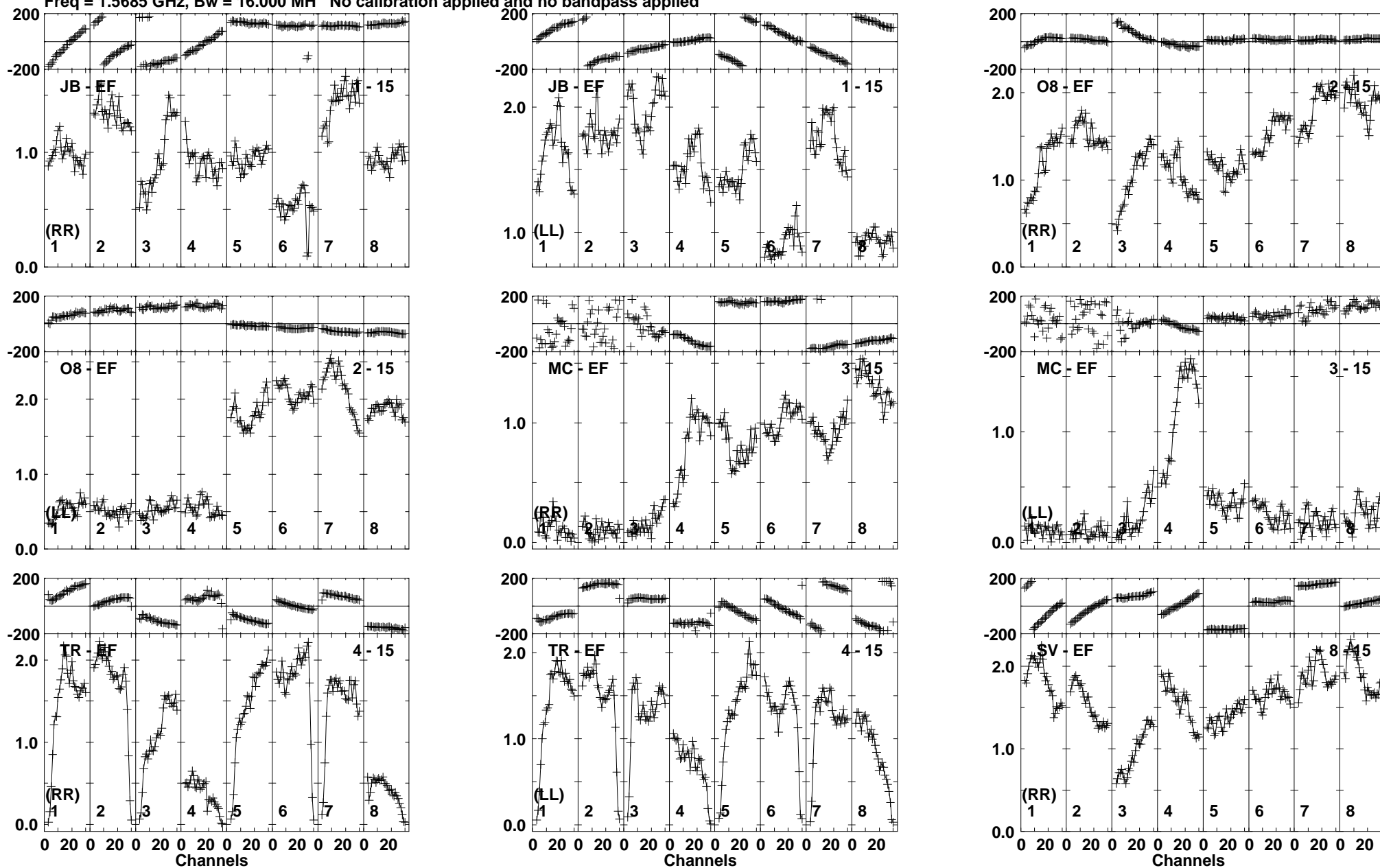
Lower frame: Milli Ampl Jy Top frame: Phas deg Vector averaged cross-power spectrum Baseline: JB (01) - EF (15) Timerange: 00/11:53:11 to 00/11:54:39
