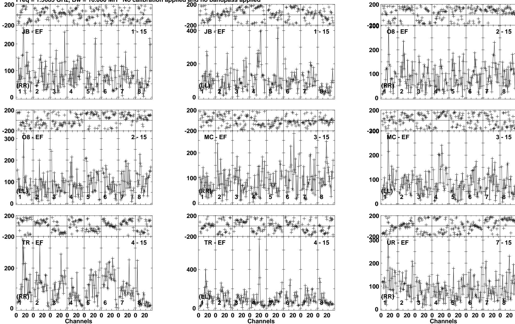
Lower frame: Micro Ampl Jy Top frame: Phas deg Vector averaged cross-power spectrum Baseline: JB (01) - EF (15) Timerange: 00/09:31:43 to 00/09:35:09
