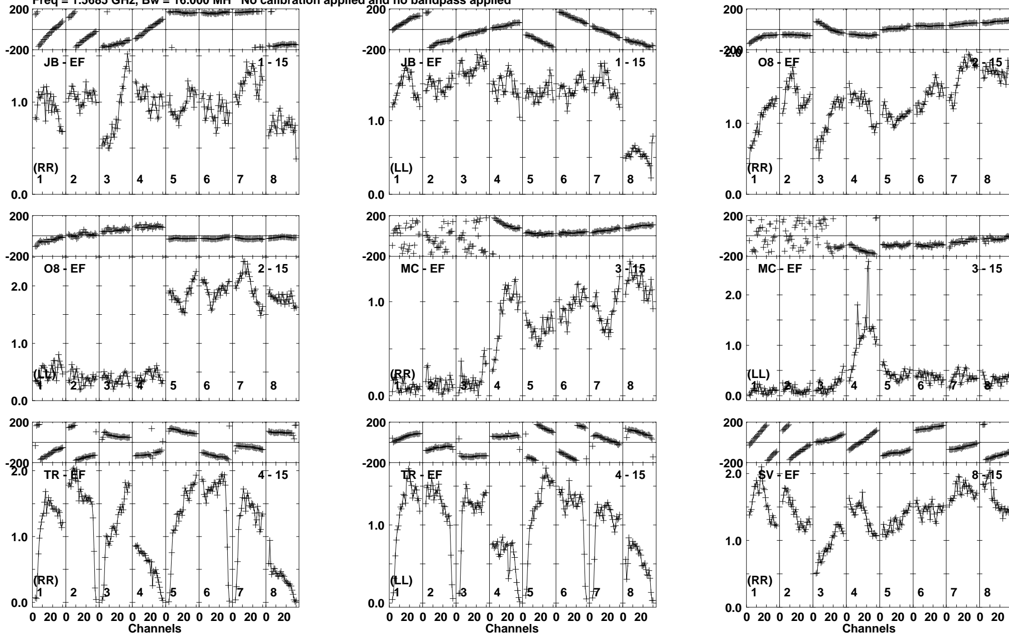
Lower frame: Milli Ampl Jy Top frame: Phas deg Vector averaged cross-power spectrum Baseline: JB (01) - EF (15) Timerange: 00/13:33:31 to 00/13:34:59
