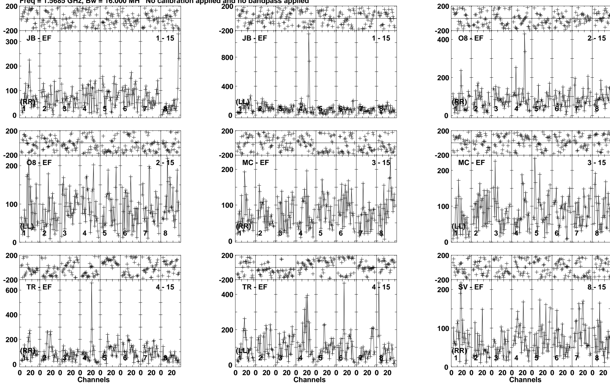
Lower frame: Micro Ampl Jy Top frame: Phas deg Vector averaged cross-power spectrum Baseline: JB (01) - EF (15) Timerange: 00/14:12:01 to 00/14:15:29
