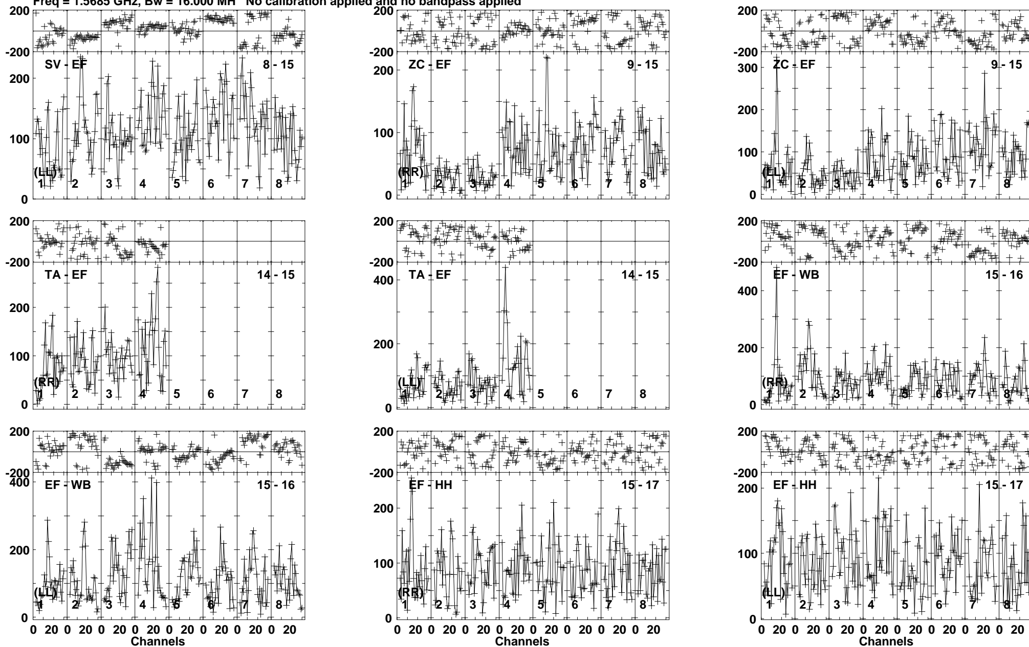
Lower frame: Micro Ampl Jy Top frame: Phas deg Vector averaged cross-power spectrum Baseline: SV (08) - EF (15) Timerange: 00:12:36:03 to 00:12:39:29
