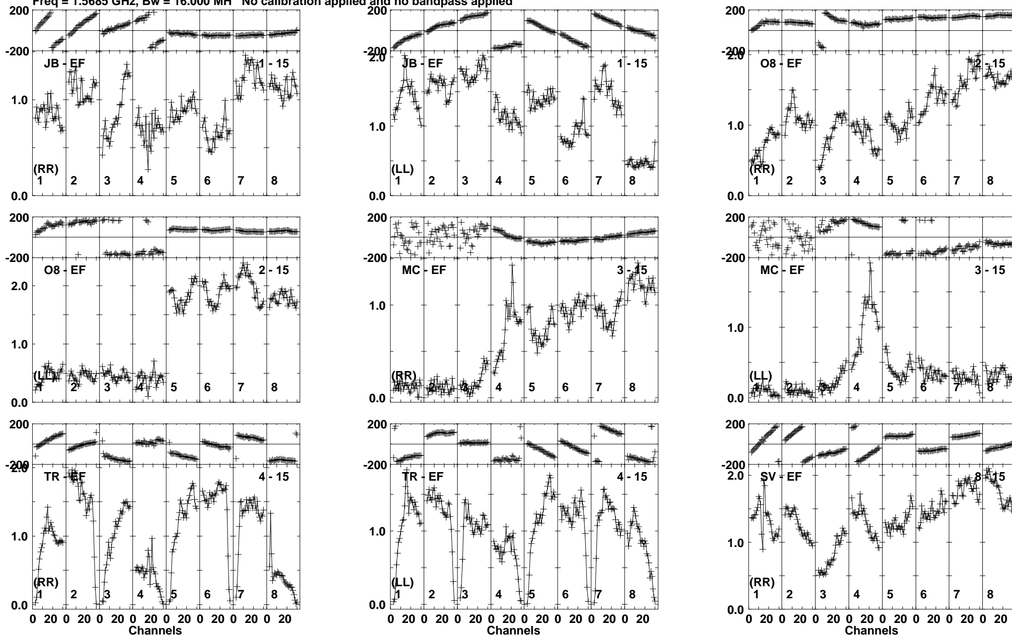
Lower frame: Milli Ampl Jy Top frame: Phas deg Vector averaged cross-power spectrum Baseline: JB (01) - EF (15) Timerange: 00:12:40:11 to 00:12:41:39
