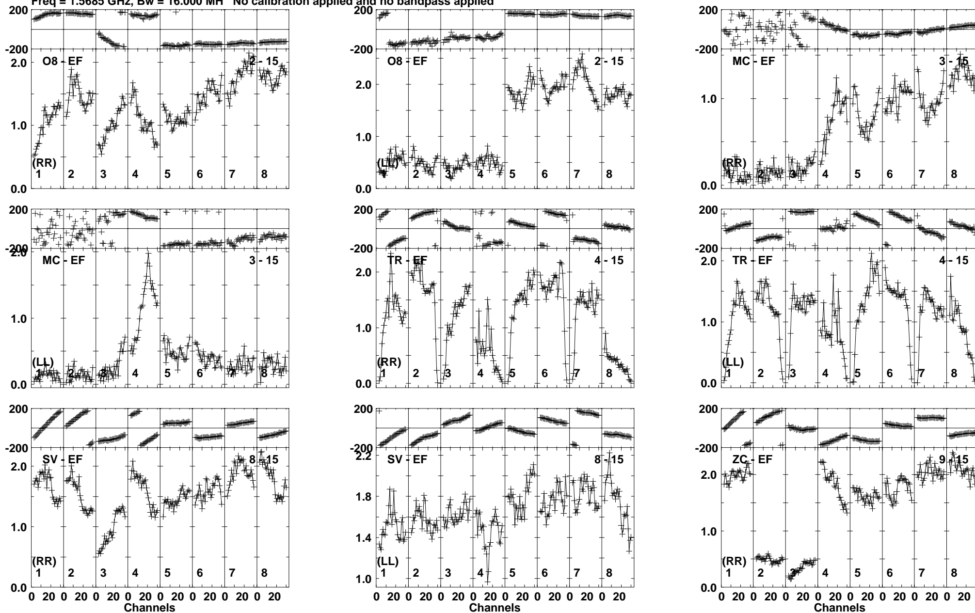
Lower frame: Milli Ampl Jy Top frame: Phas deg Vector averaged cross-power spectrum Baseline: O8 (02) - EF (15) Timerange: 00:12:55:53 to 00:12:57:19
