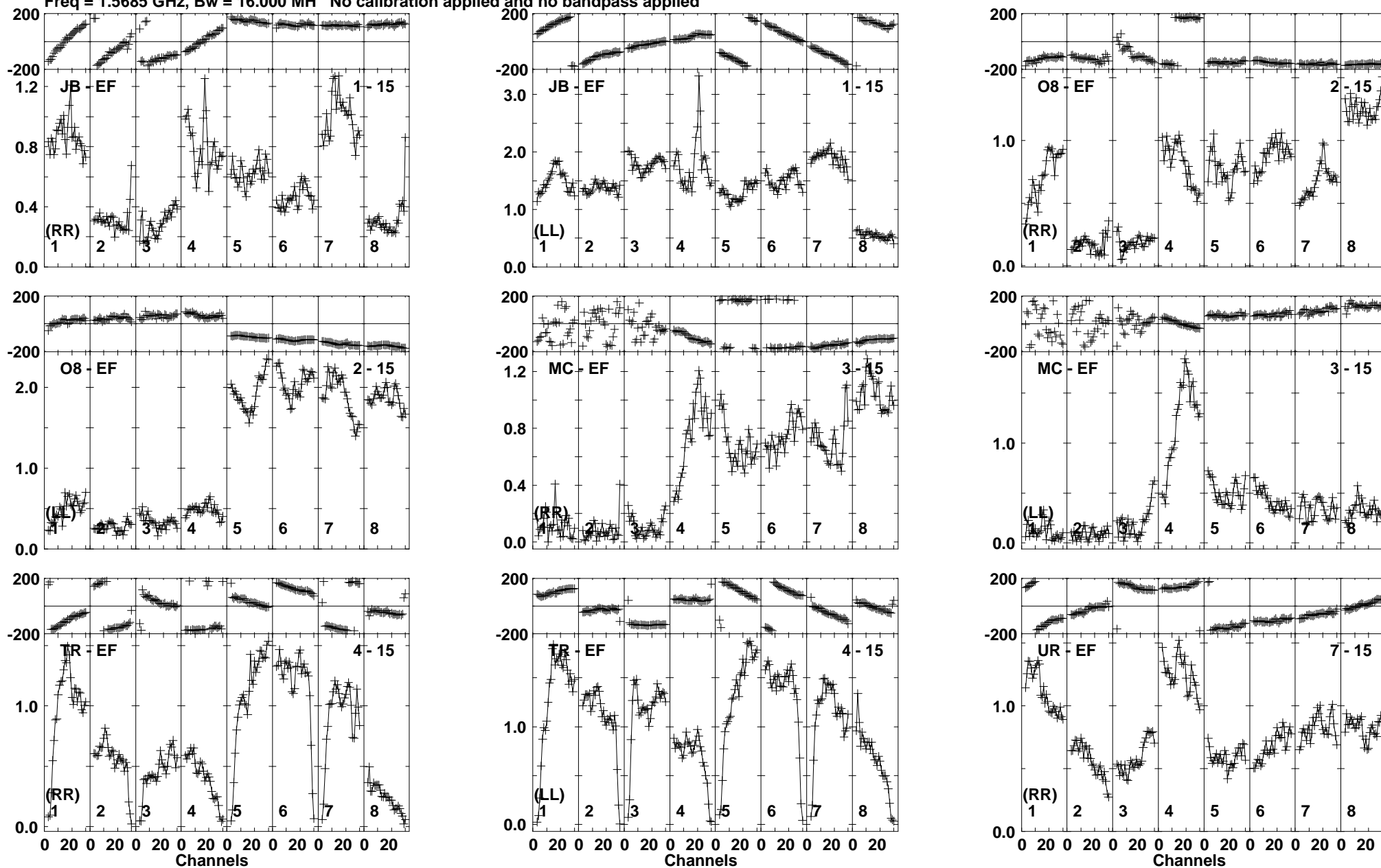
Lower frame: Milli Ampl Jy Top frame: Phas deg Vector averaged cross-power spectrum Baseline: JB (01) - EF (15) Timerange: 00/09:19:31 to 00/09:20:59
