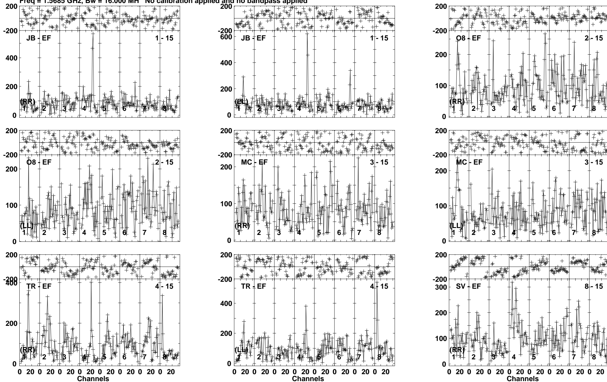
Lower frame: Micro Ampl Jy Top frame: Phas deg Vector averaged cross-power spectrum Baseline: JB (01) - EF (15) Timerange: 00/12:36:03 to 00/12:39:29
