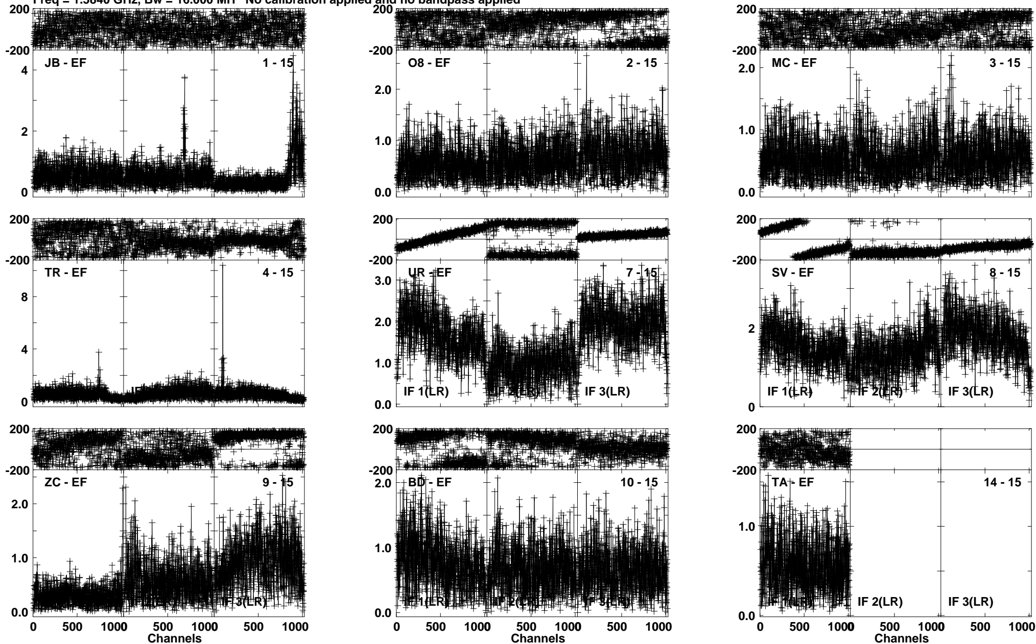
Lower frame: Milli Ampl Jy Top frame: Phas deg Vector averaged cross-power spectrum Baseline: JB (01) - EF (15) Timerange: 00/10/06:03 to 00/10/09:59
