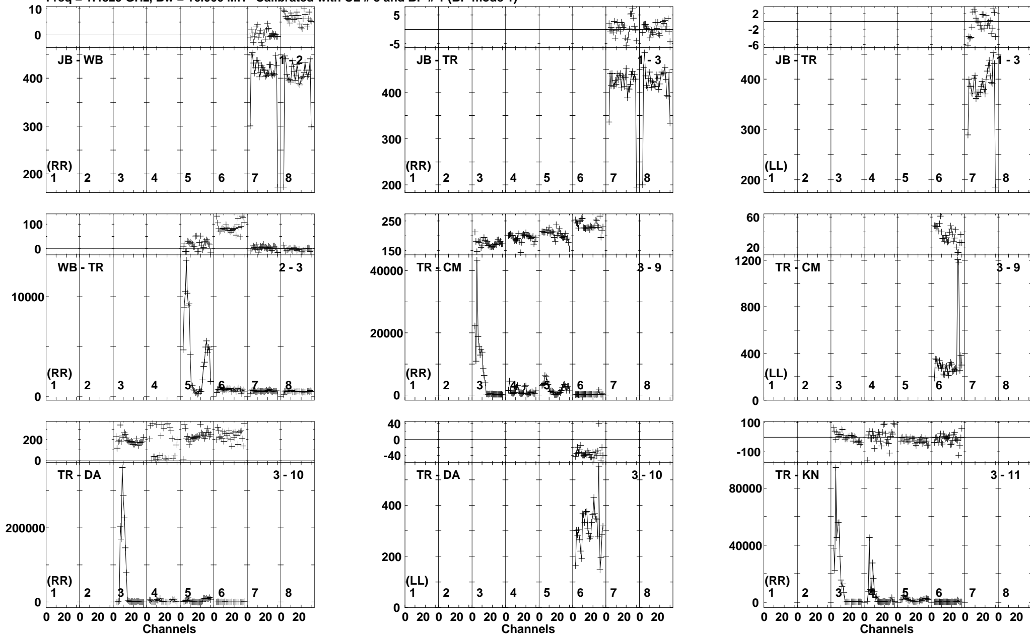
Lower frame: Milli Ampl Jy Top frame: Phas deg Vector averaged cross-power spectrum Baseline: JB (01) - WB (02) Timerange: 00/13:01:11 to 00/13:02:39
