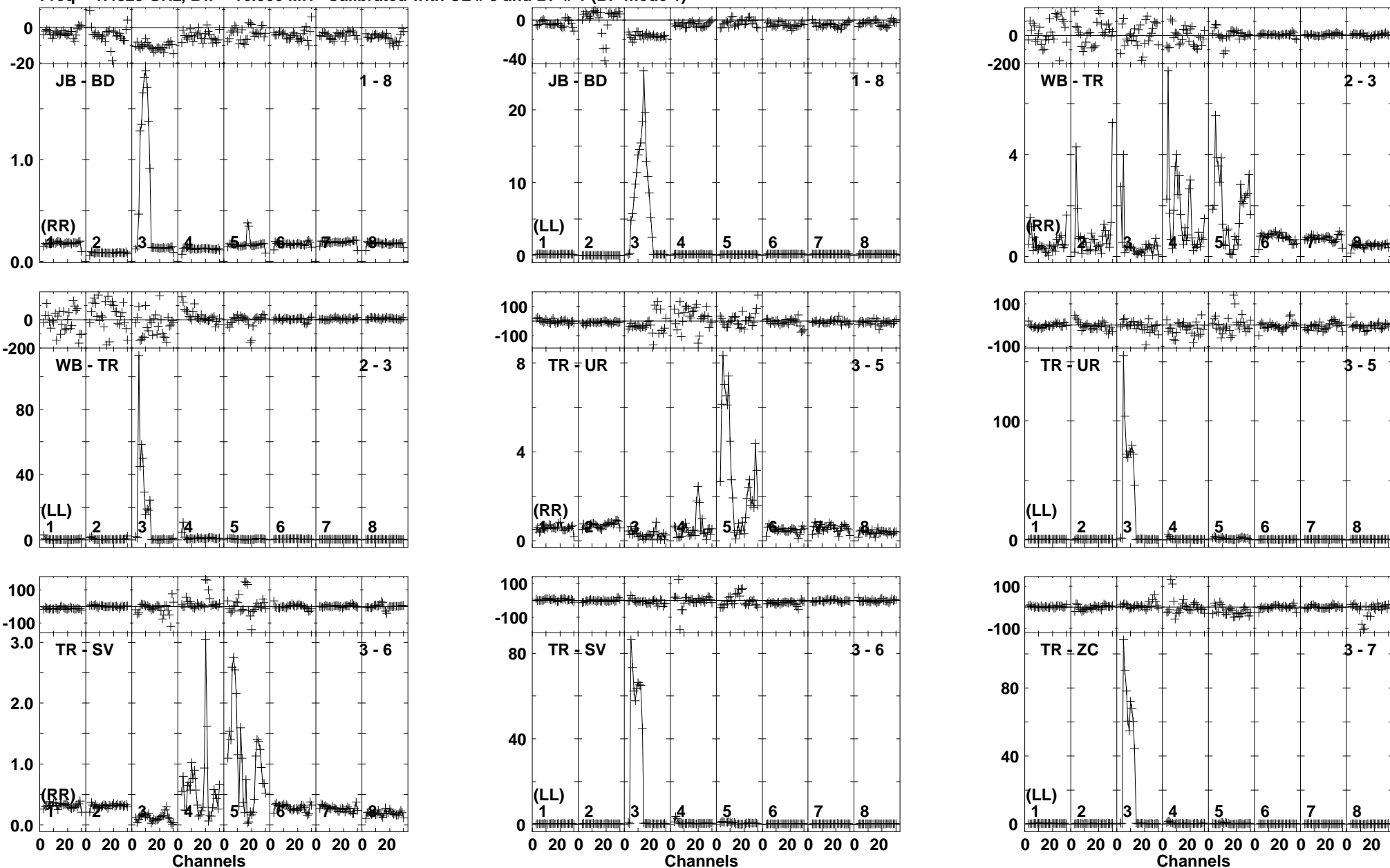
Lower frame: Ampl Jy Top frame: Phas deg Vector averaged cross-power spectrum Baseline: JB (01) - BD (08) Timerange: 00/05:27:26 to 00/05:28:54
