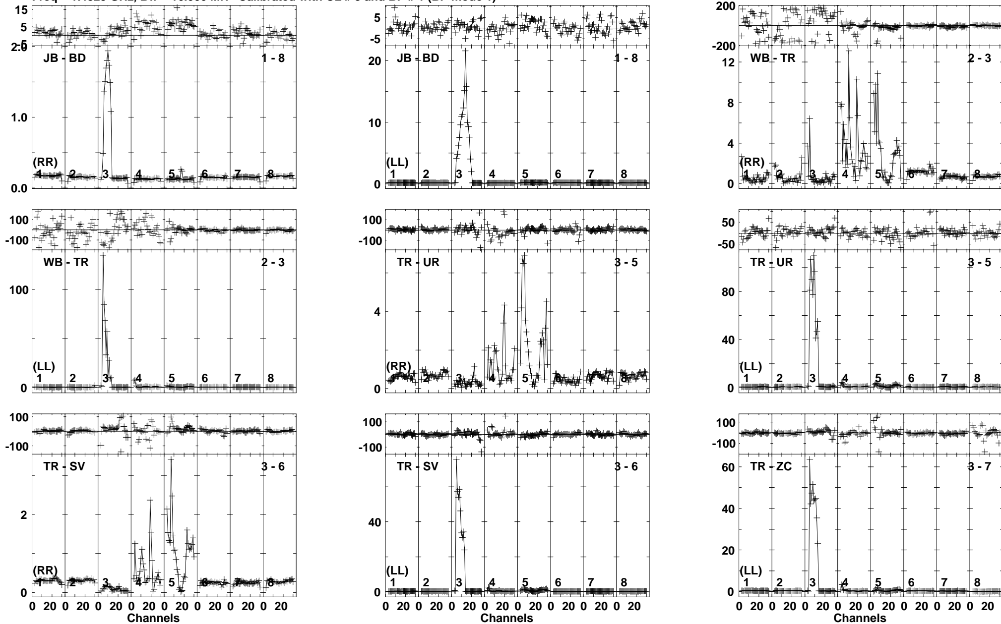
Lower frame: Ampl Jy Top frame: Phas deg Vector averaged cross-power spectrum Baseline: JB (01) - BD (08) Timerange: 00/04:22:51 to 00/04:24:19
