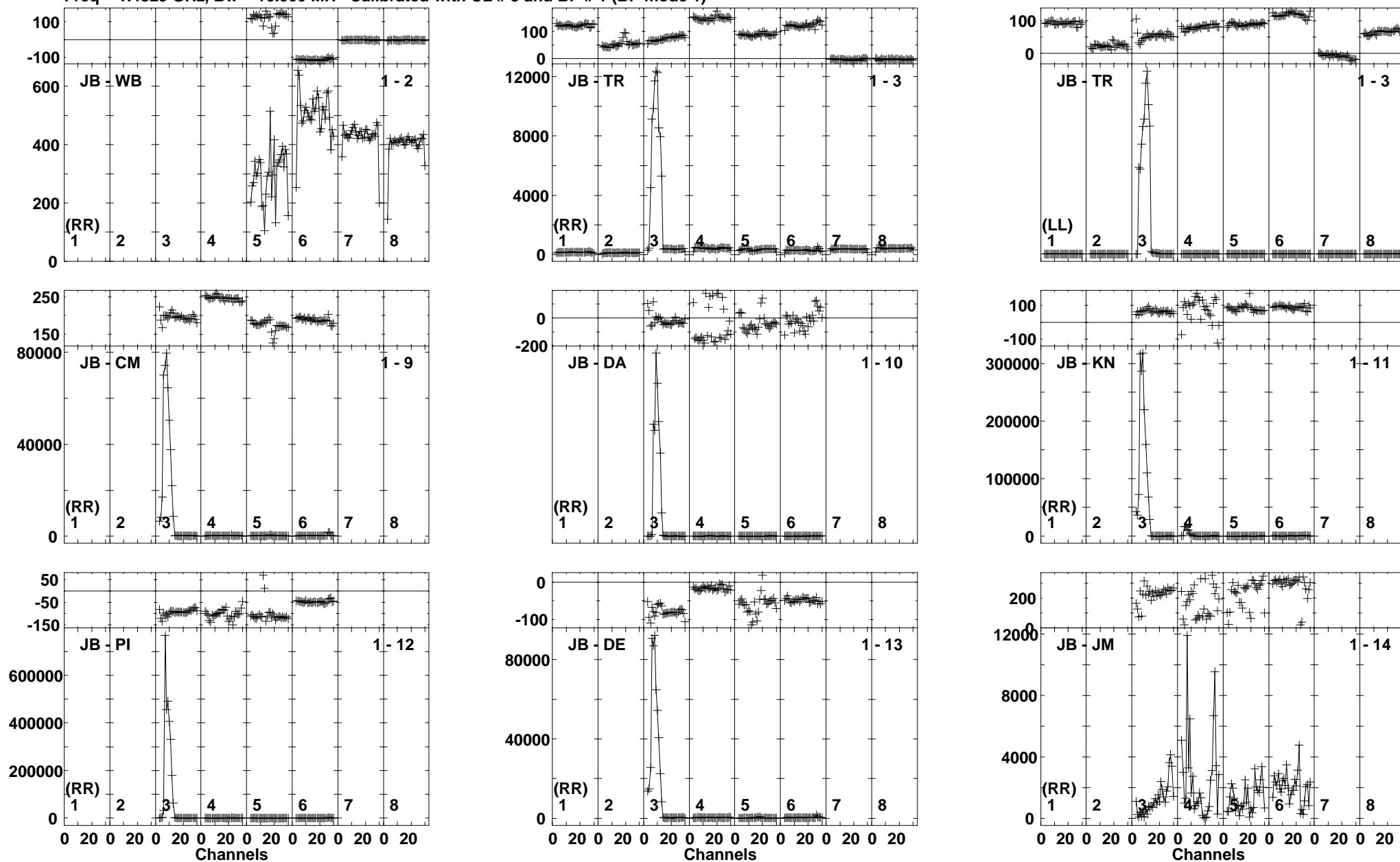
Lower frame: Milli Ampl Jy Top frame: Phas deg Vector averaged cross-power spectrum Baseline: JB (01) - WB (02) Timerange: 00:12:50:31 to 00:12:51:59
