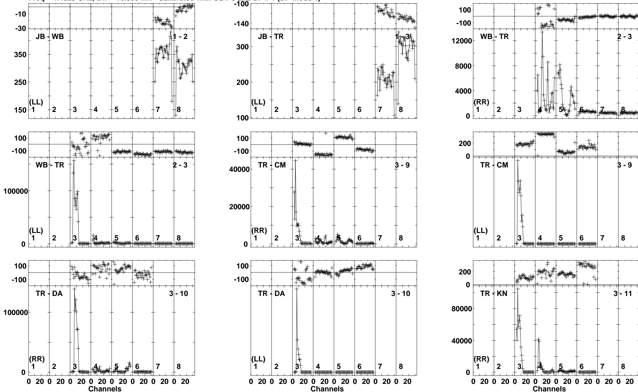
Lower frame: Milli Ampl Jy Top frame: Phas deg Vector averaged cross-power spectrum Baseline: JB (01) - WB (02) Timerange: 00/13:43:51 to 00/13:45:19
