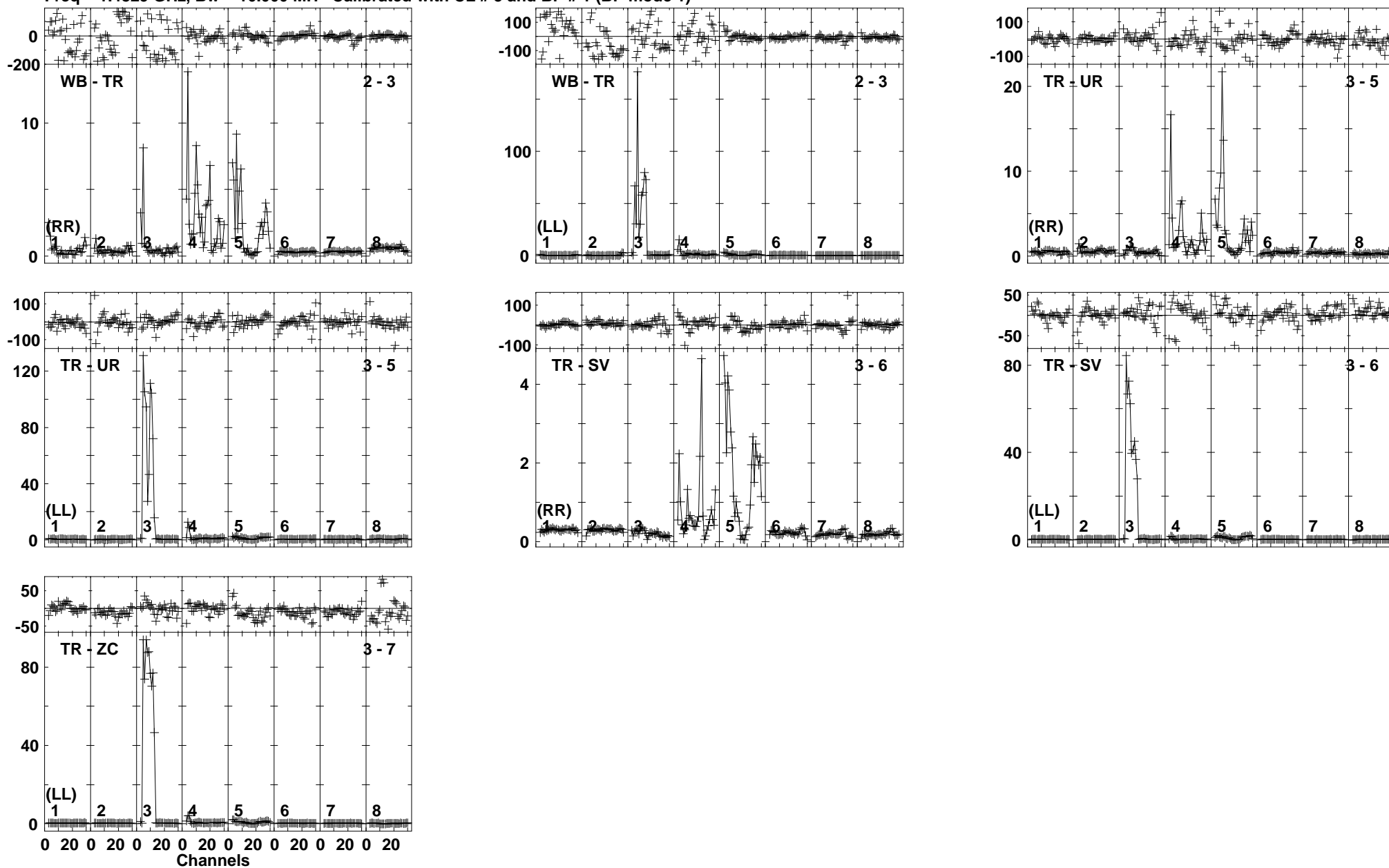
Lower frame: Ampl Jy Top frame: Phas deg Vector averaged cross-power spectrum Baseline: WB (02) - TR (03) Timerange: 00/09:34:26 to 00/09:35:54
