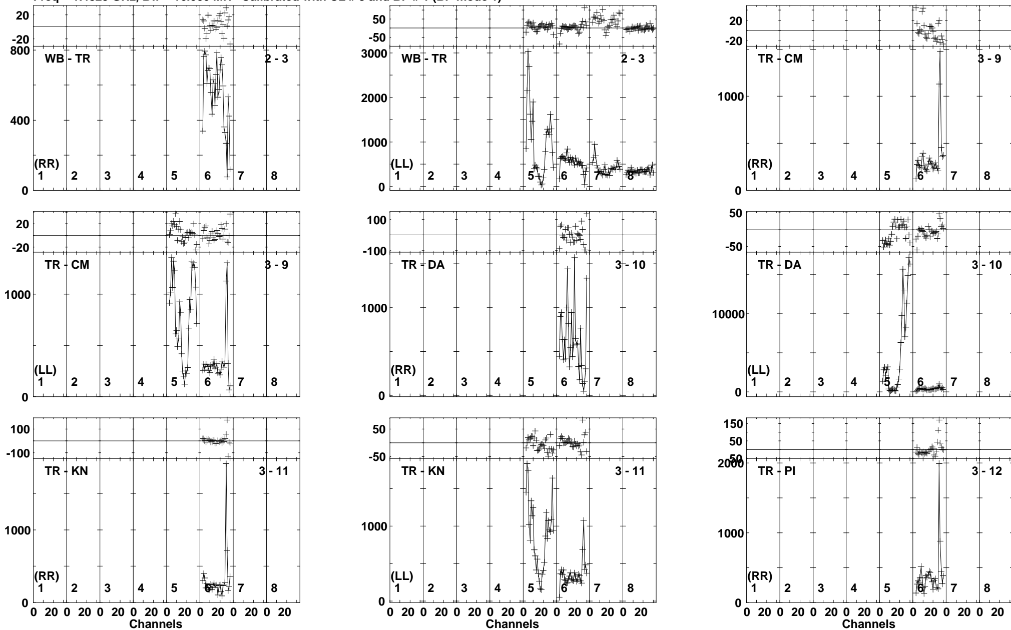
Lower frame: Milli Ampl Jy Top frame: Phas deg Vector averaged cross-power spectrum Baseline: WB (02) - TR (03) Timerange: 00/13:38:11 to 00/13:39:39
