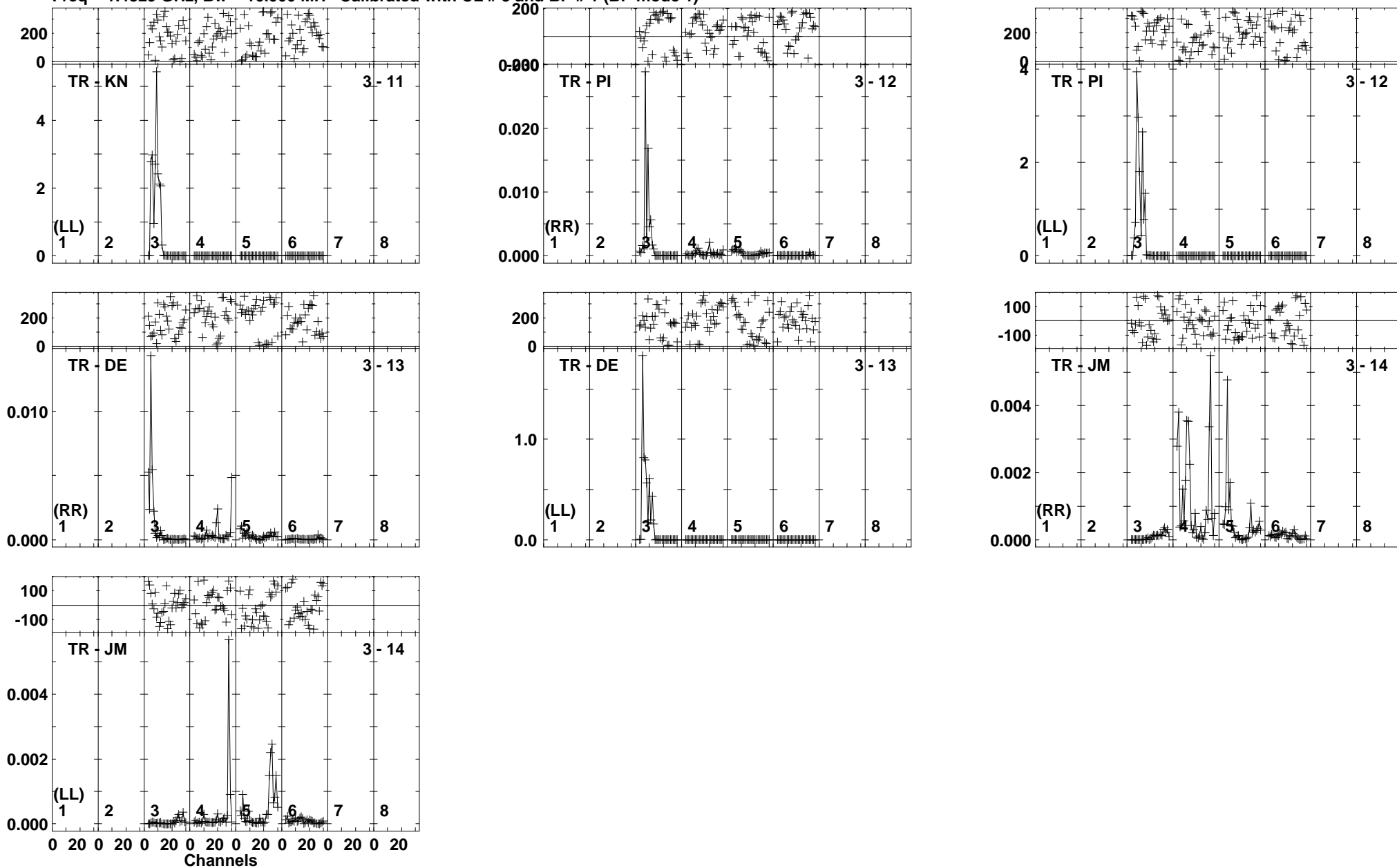
Lower frame: Kilo Ampl Jy Top frame: Phas deg Vector averaged cross-power spectrum Baseline: TR (03) - KN (11) Timerange: 00/13:45:21 to 00/13:48:49
