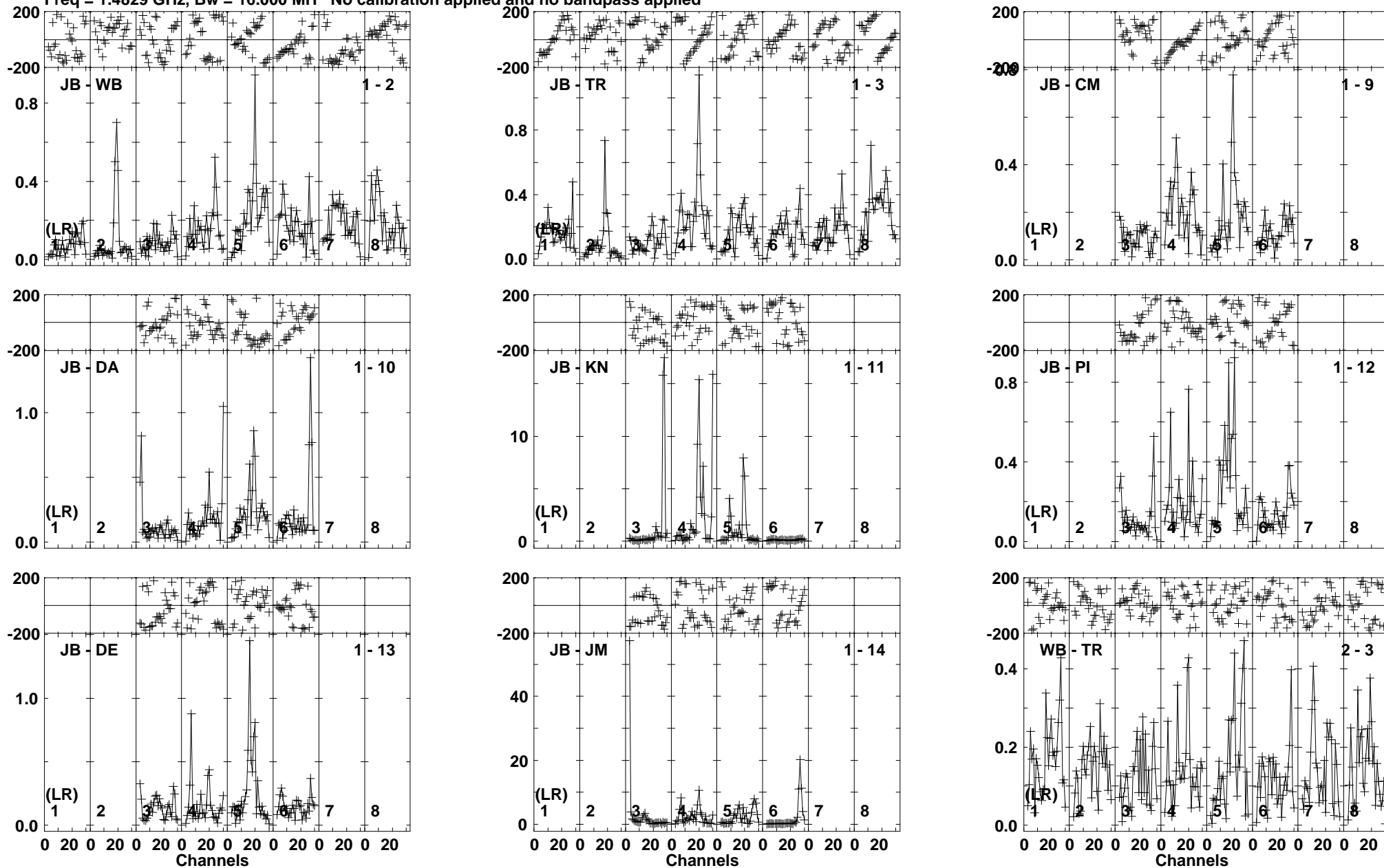
Lower frame: Milli Ampl Jy Top frame: Phas deg Vector averaged cross-power spectrum Baseline: JB (01) - WB (02) Timerange: 00/13:01:11 to 00/13:02:39
