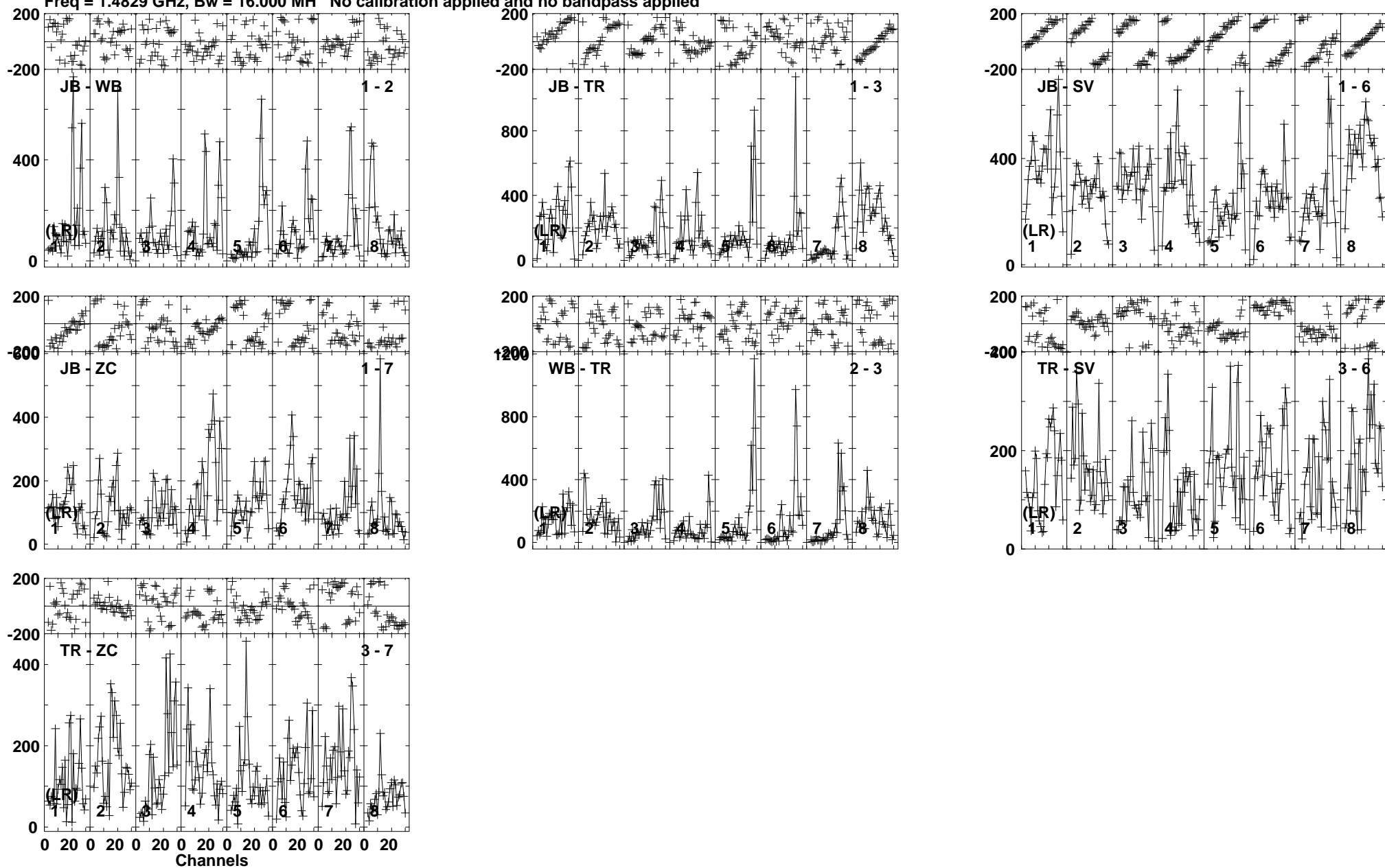
Lower frame: Micro Ampl Jy Top frame: Phas deg Vector averaged cross-power spectrum Baseline: JB (01) - WB (02) Timerange: 00/10:22:46 to 00/10:24:14
