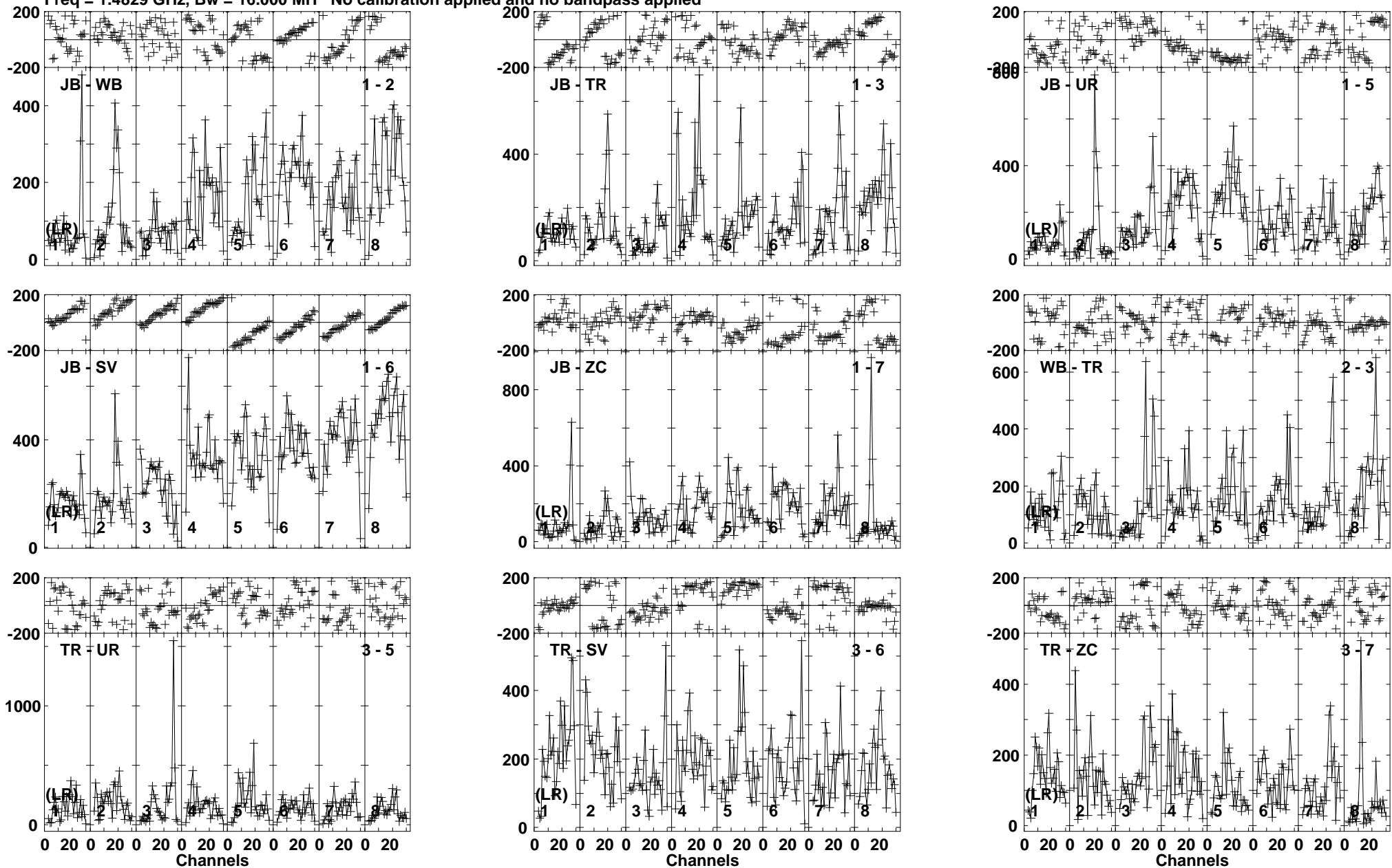
Lower frame: Micro Ampl Jy Top frame: Phas deg Vector averaged cross-power spectrum Baseline: JB (01) - WB (02) Timerange: 00/09:29:26 to 00/09:30:54
