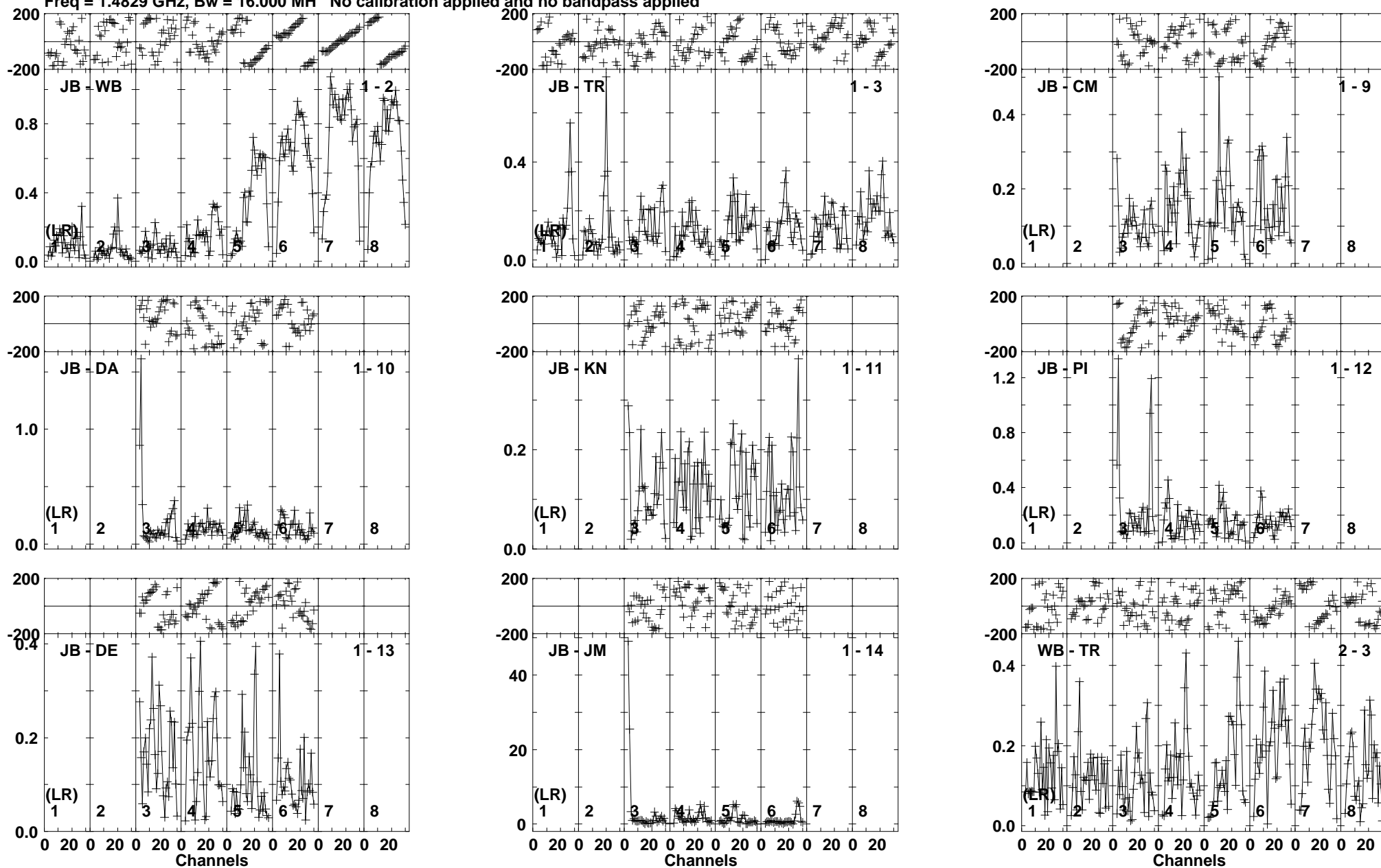
Lower frame: Milli Ampl Jy Top frame: Phas deg Vector averaged cross-power spectrum Baseline: JB (01) - WB (02) Timerange: 00/14:15:51 to 00/14:17:19
