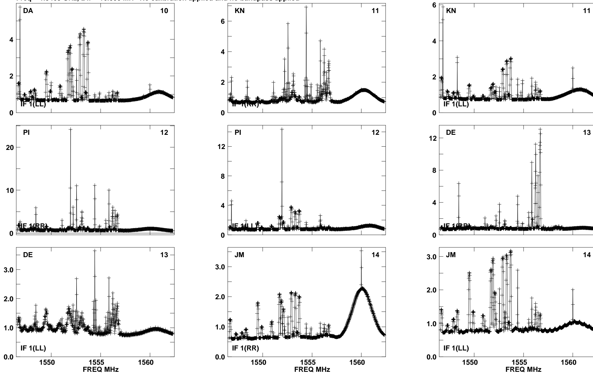
Lower frame: Real Jy Total-power spectrum Antenna: DA (10) Timerange: 00/13:54:31 to 00/13:55:59
