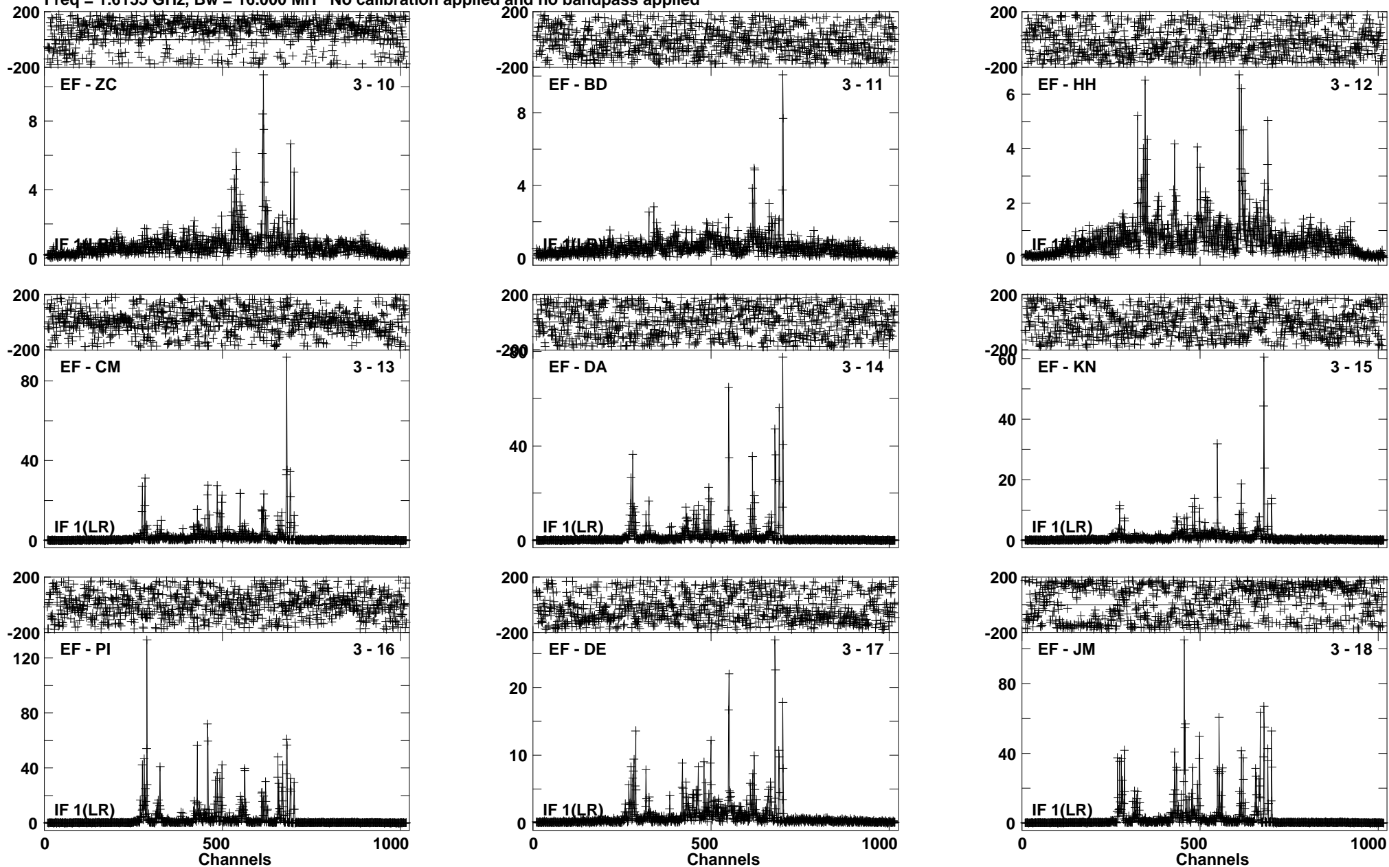
Lower frame: Milli Ampl Jy Top frame: Phas deg Vector averaged cross-power spectrum Baseline: EF (03) - ZC (10) Timerange: 00/11:03:21 to 00/11:04:49
