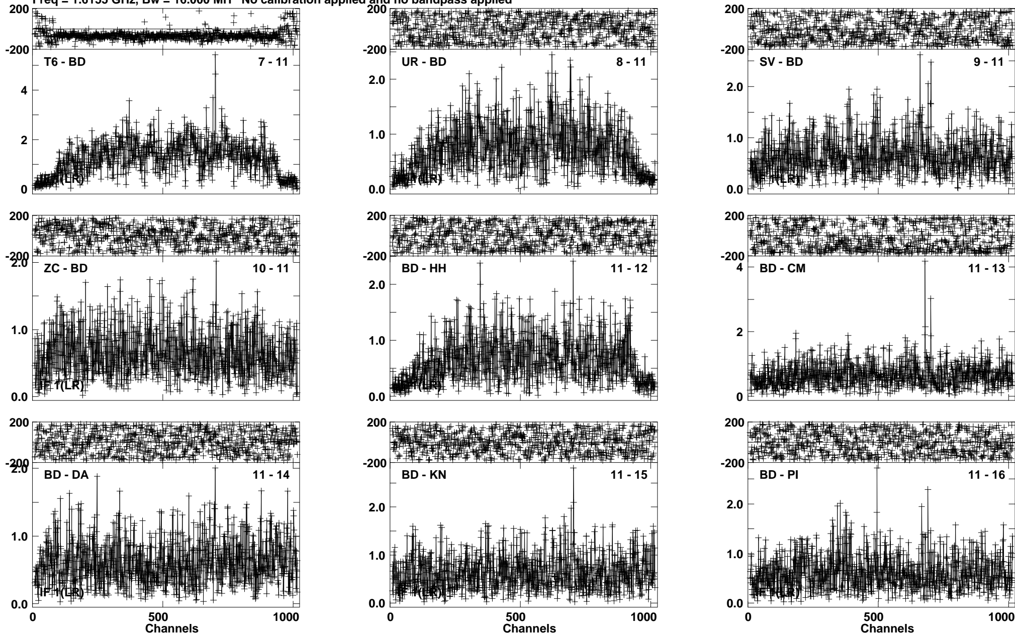
Lower frame: Milli Ampl Jy Top frame: Phas deg Vector averaged cross-power spectrum Baseline: T6 (07) - BD (11) Timerange: 00/09:11:31 to 00/09:12:59
