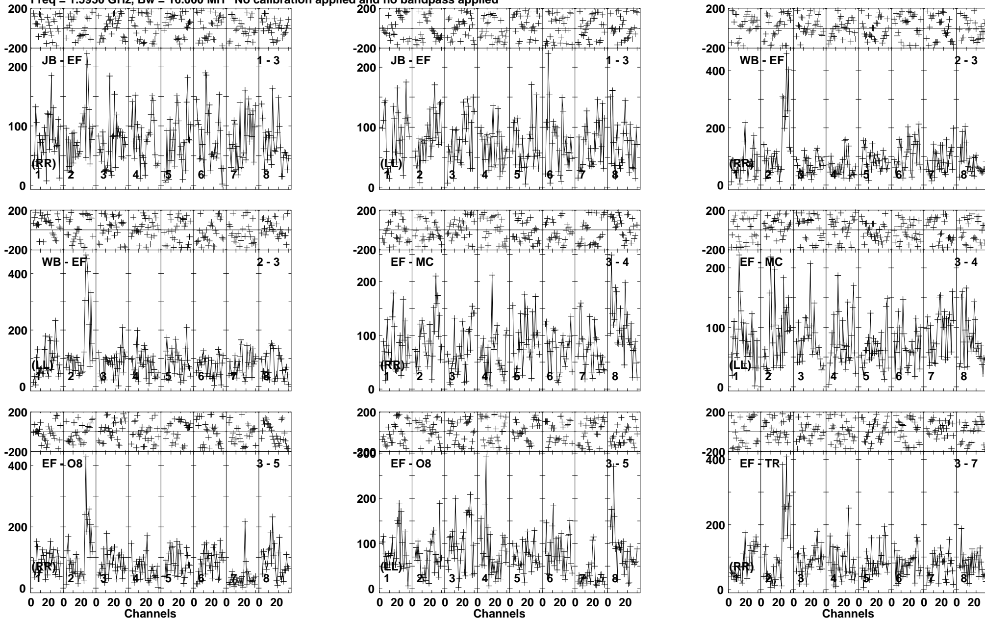
Lower frame: Micro Ampl Jy Top frame: Phas deg Vector averaged cross-power spectrum Baseline: JB (01) - EF (03) Timerange: 00/17:02:57 to 00/17:06:53
