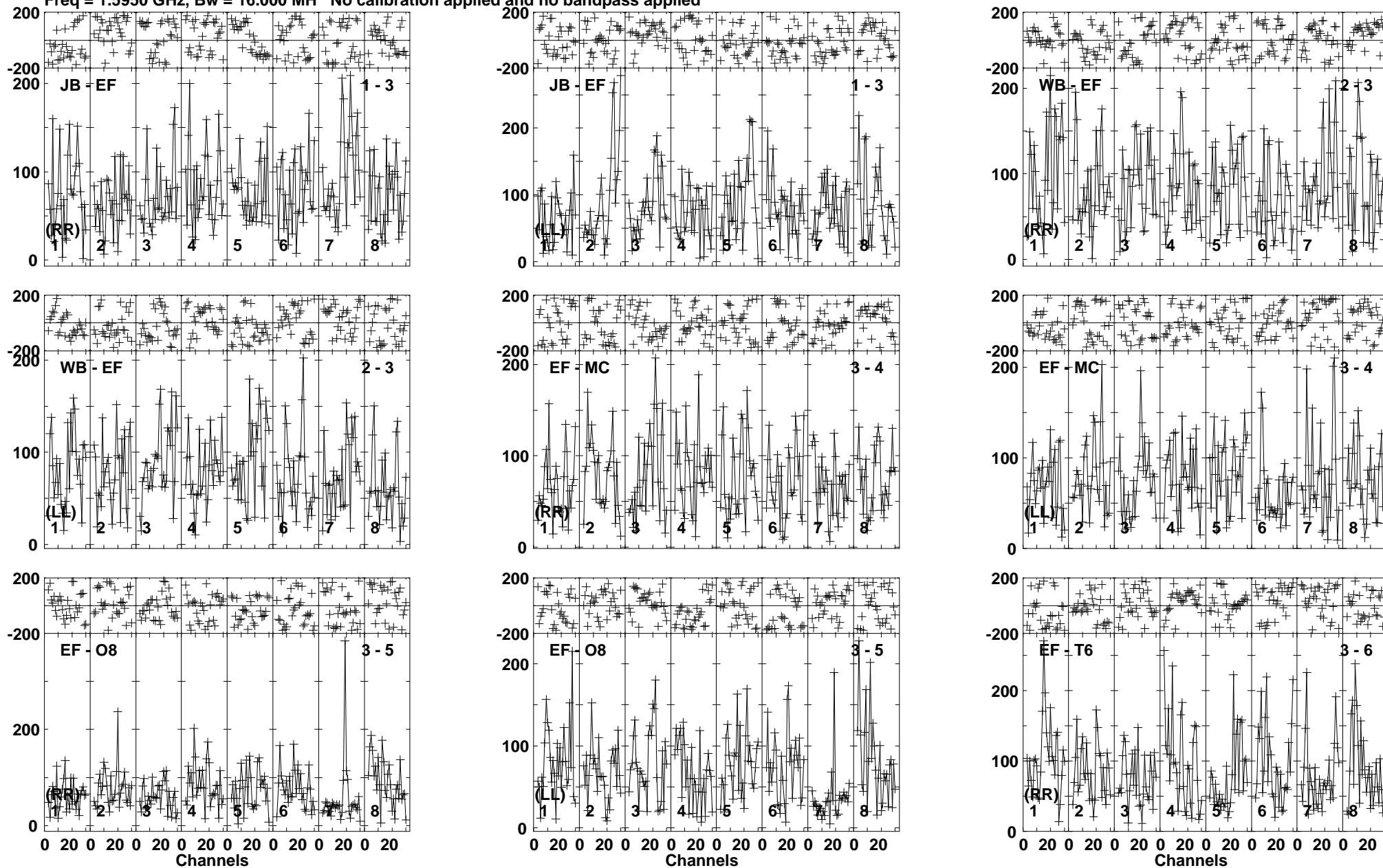
Lower frame: Micro Ampl Jy Top frame: Phas deg Vector averaged cross-power spectrum Baseline: JB (01) - EF (03) Timerange: 01/12:15:47 to 01/12:19:43
