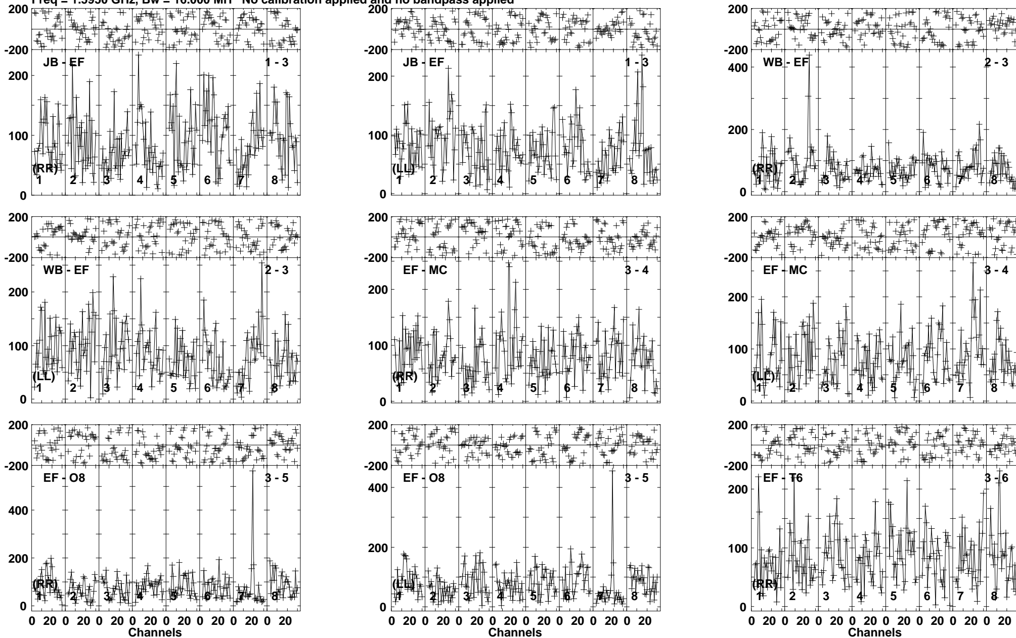
Lower frame: Micro Ampl Jy Top frame: Phas deg Vector averaged cross-power spectrum Baseline: JB (01) - EF (03) Timerange: 01/12:09:01 to 01/12:12:59
