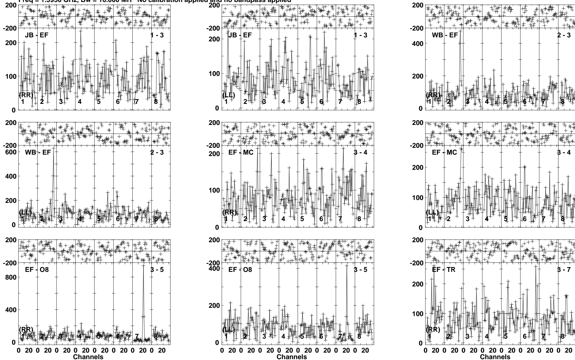
Lower frame: Micro Ampl Jy Top frame: Phas deg Vector averaged cross-power spectrum Baseline: JB (01) - EF (03) Timerange: 00/13:22:01 to 00/13:26:09
