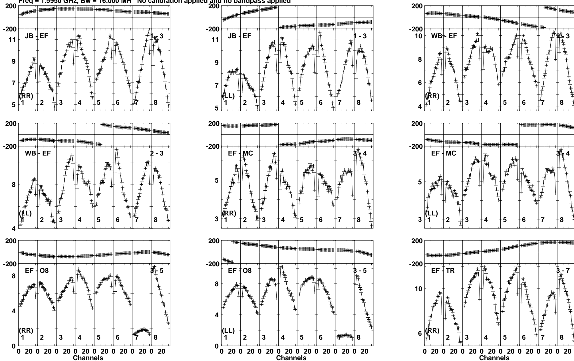
Lower frame: Milli Ampl Jy Top frame: Phas deg Vector averaged cross-power spectrum Baseline: JB (01) - EF (03) Timerange: 00/17:39:11 to 00/17:41:09
