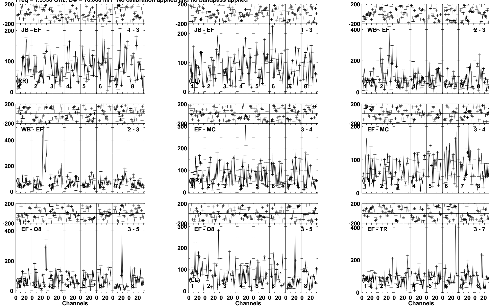
Lower frame: Micro Ampl Jy Top frame: Phas deg Vector averaged cross-power spectrum Baseline: JB (01) - EF (03) Timerange: 00/14:28:47 to 00/14:32:43
