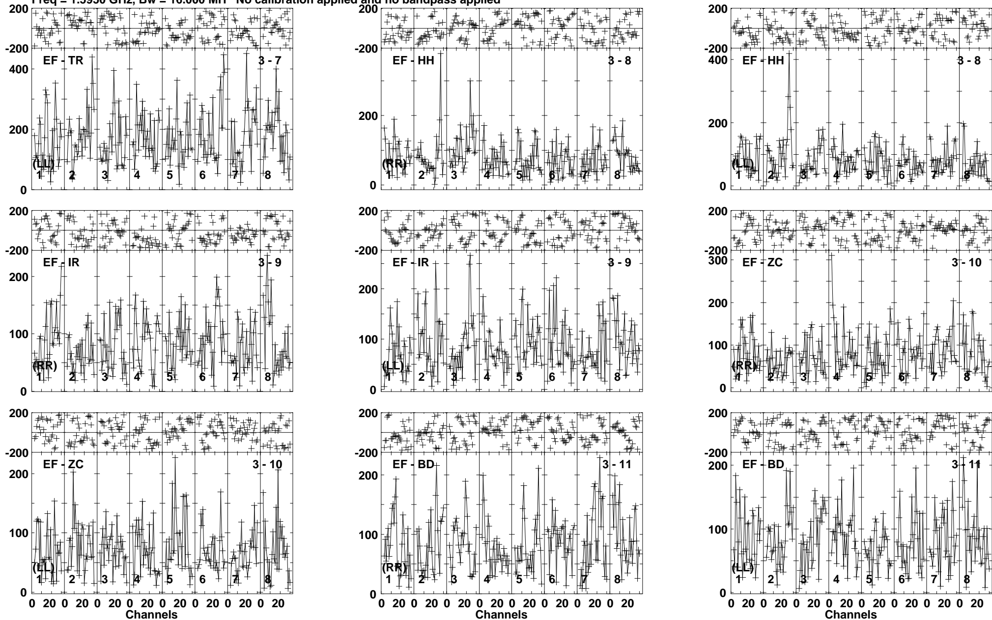
Lower frame: Micro Ampl Jy Top frame: Phas deg Vector averaged cross-power spectrum Baseline: EF (03) - TR (07) Timerange: 00/13:28:11 to 00/13:32:19
