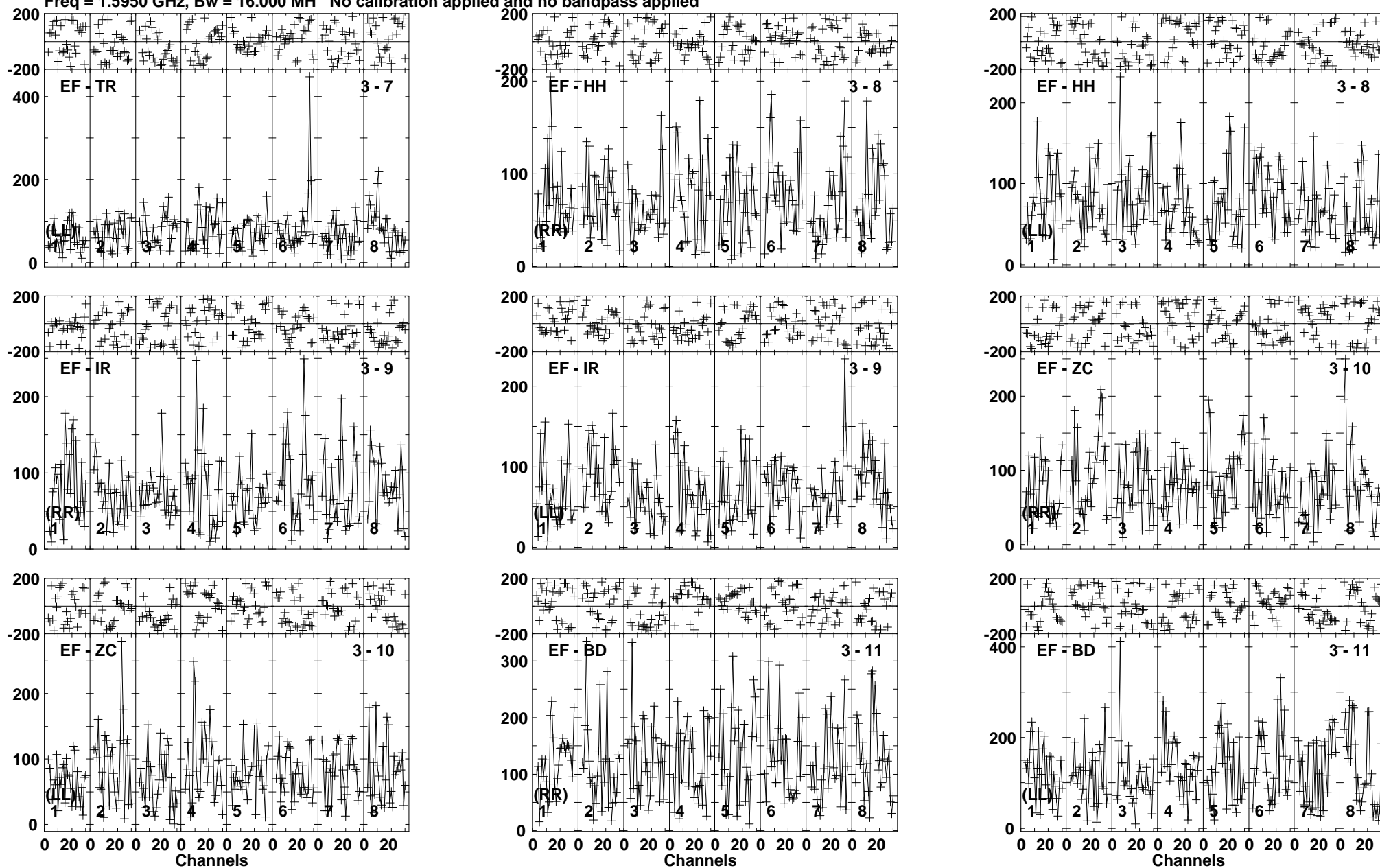
Lower frame: Micro Ampl Jy Top frame: Phas deg Vector averaged cross-power spectrum Baseline: EF (03) - TR (07) Timerange: 00/14:28:47 to 00/14:32:43
