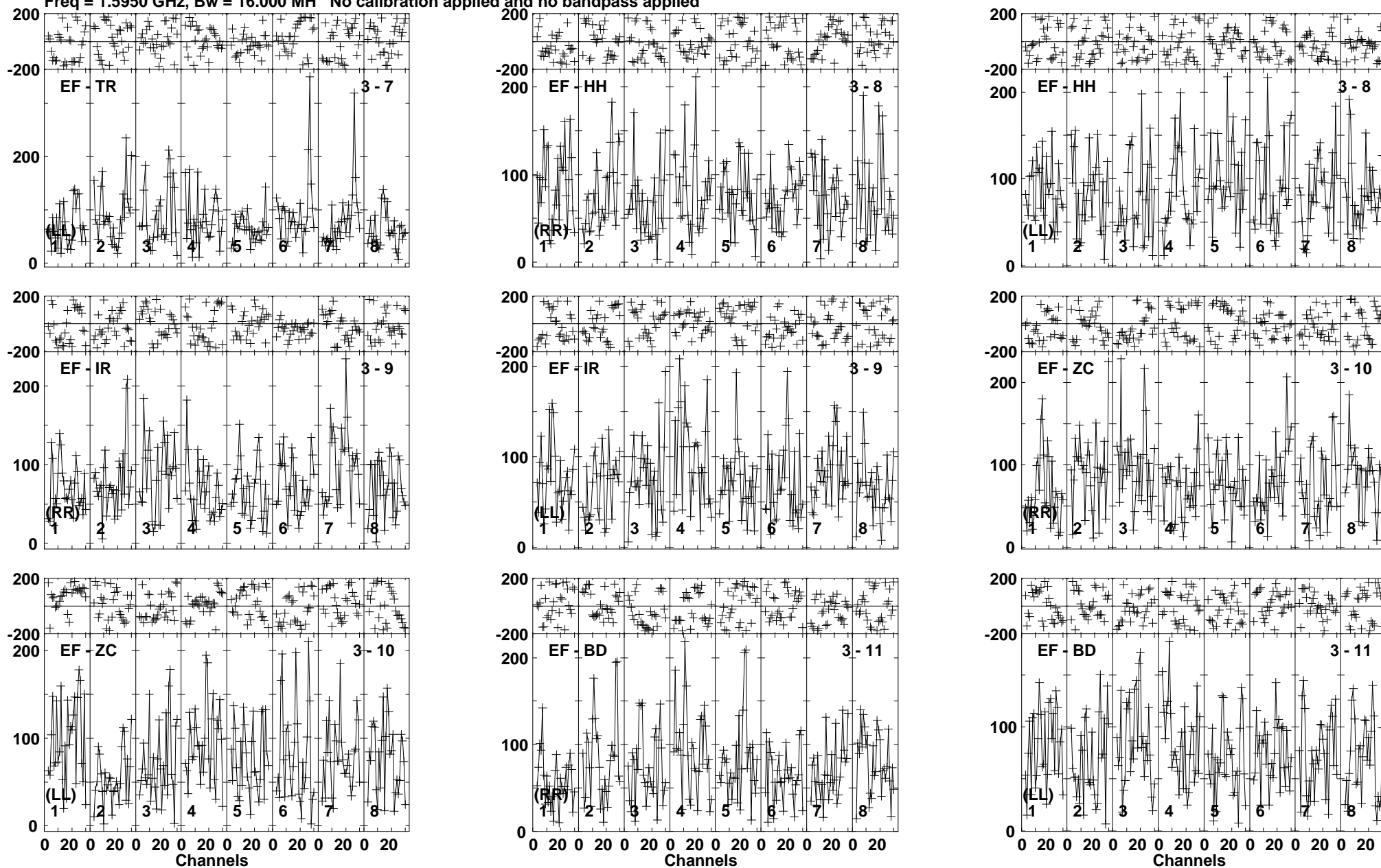
Lower frame: Micro Ampl Jy Top frame: Phas deg Vector averaged cross-power spectrum Baseline: EF (03) - TR (07) Timerange: 00/14:22:47 to 00/14:26:43
