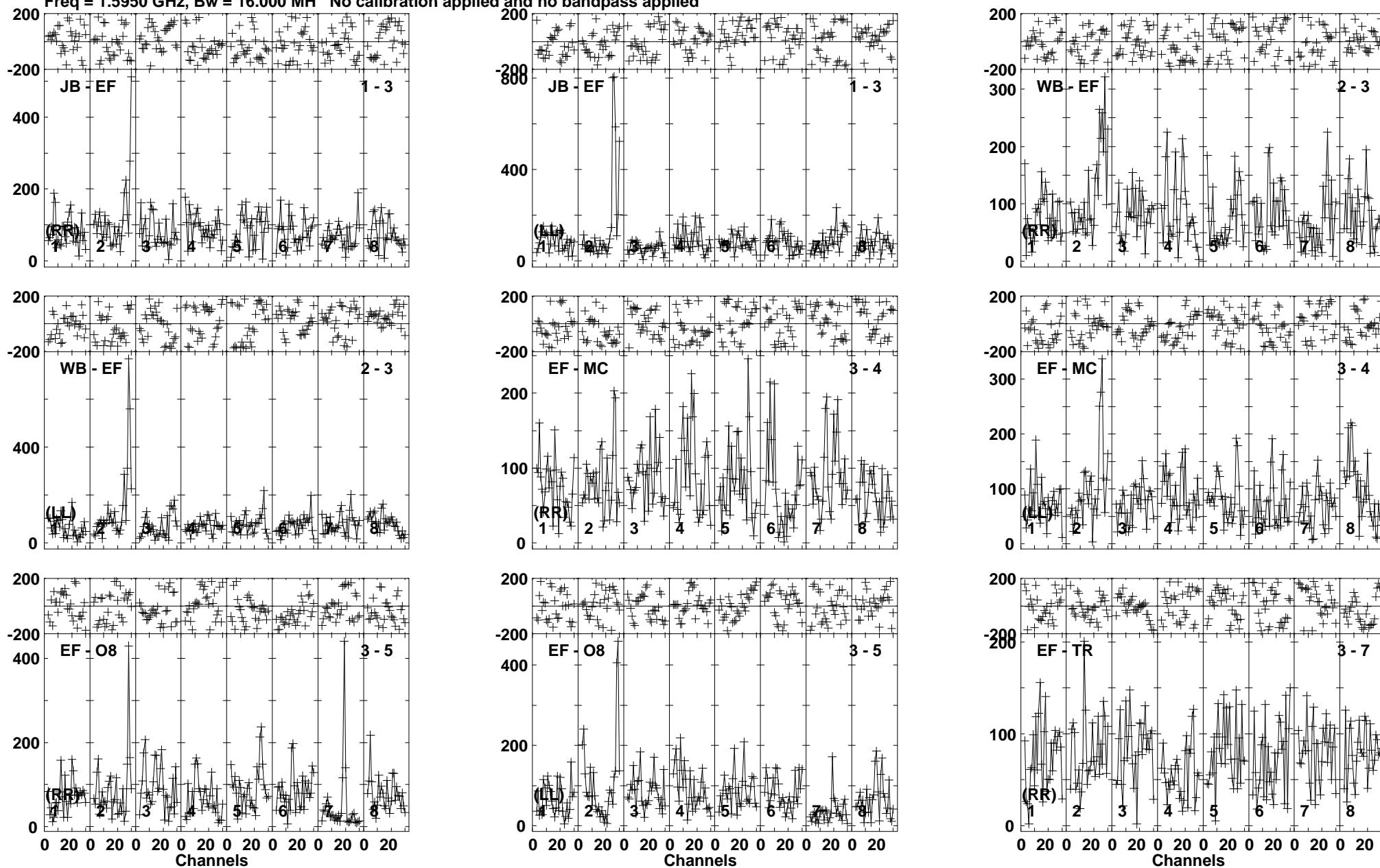
Lower frame: Micro Ampl Jy Top frame: Phas deg Vector averaged cross-power spectrum Baseline: JB (01) - EF (03) Timerange: 00/14:35:27 to 00/14:39:23
