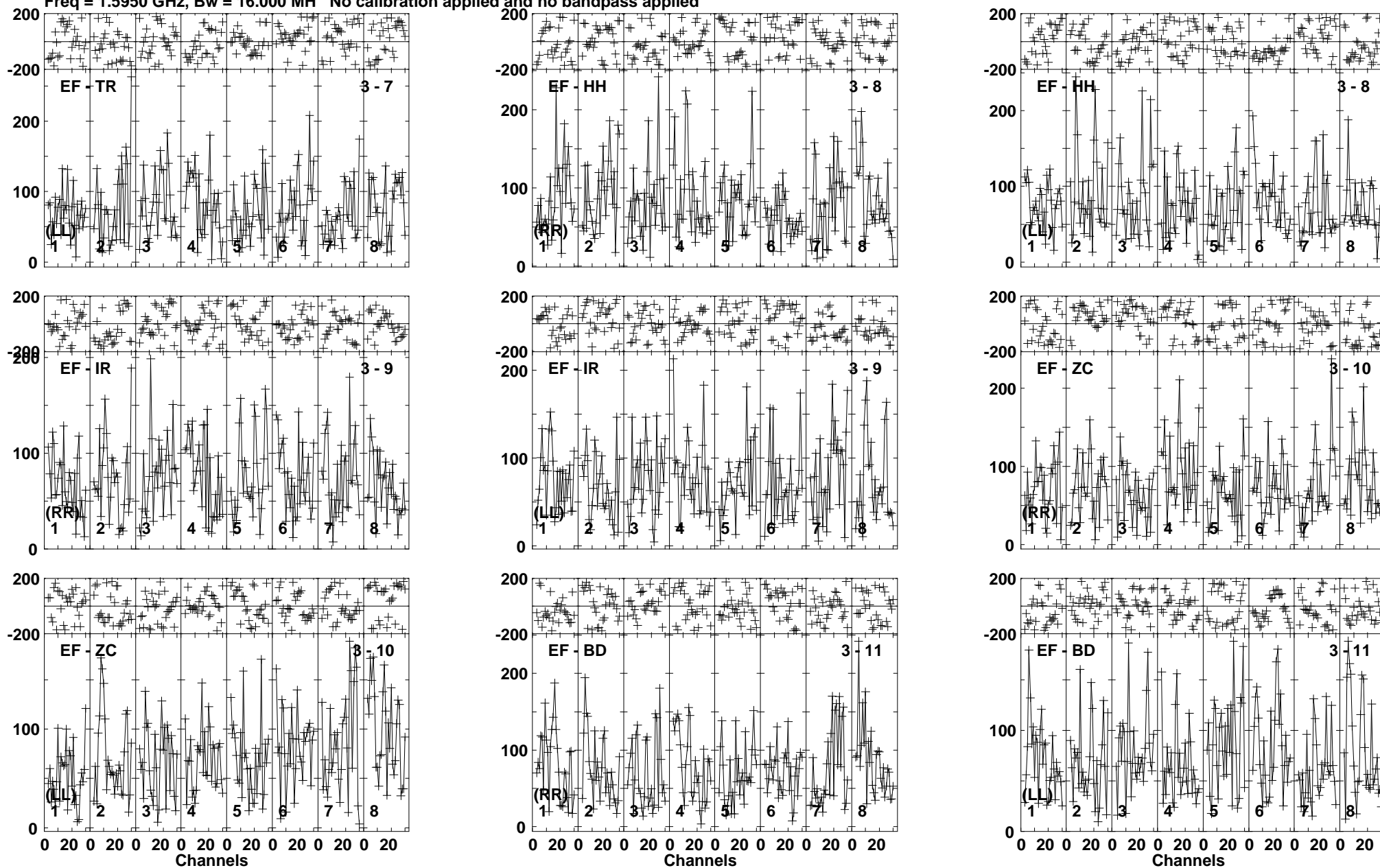
Lower frame: Micro Ampl Jy Top frame: Phas deg Vector averaged cross-power spectrum Baseline: EF (03) - TR (07) Timerange: 00/14:16:07 to 00/14:20:03
