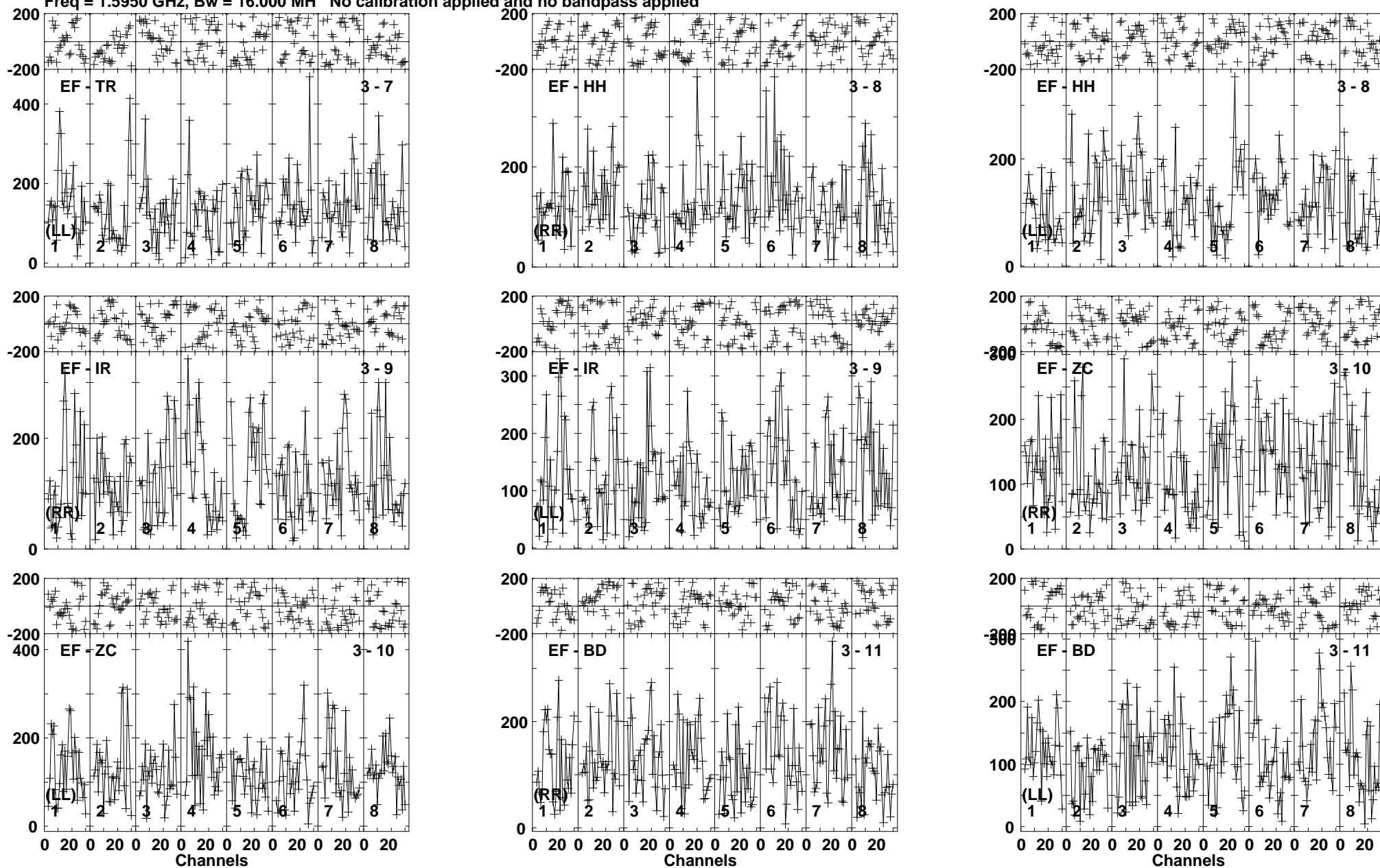
Lower frame: Micro Ampl Jy Top frame: Phas deg Vector averaged cross-power spectrum Baseline: EF (03) - TR (07) Timerange: 00/13:02:01 to 00/13:06:09
