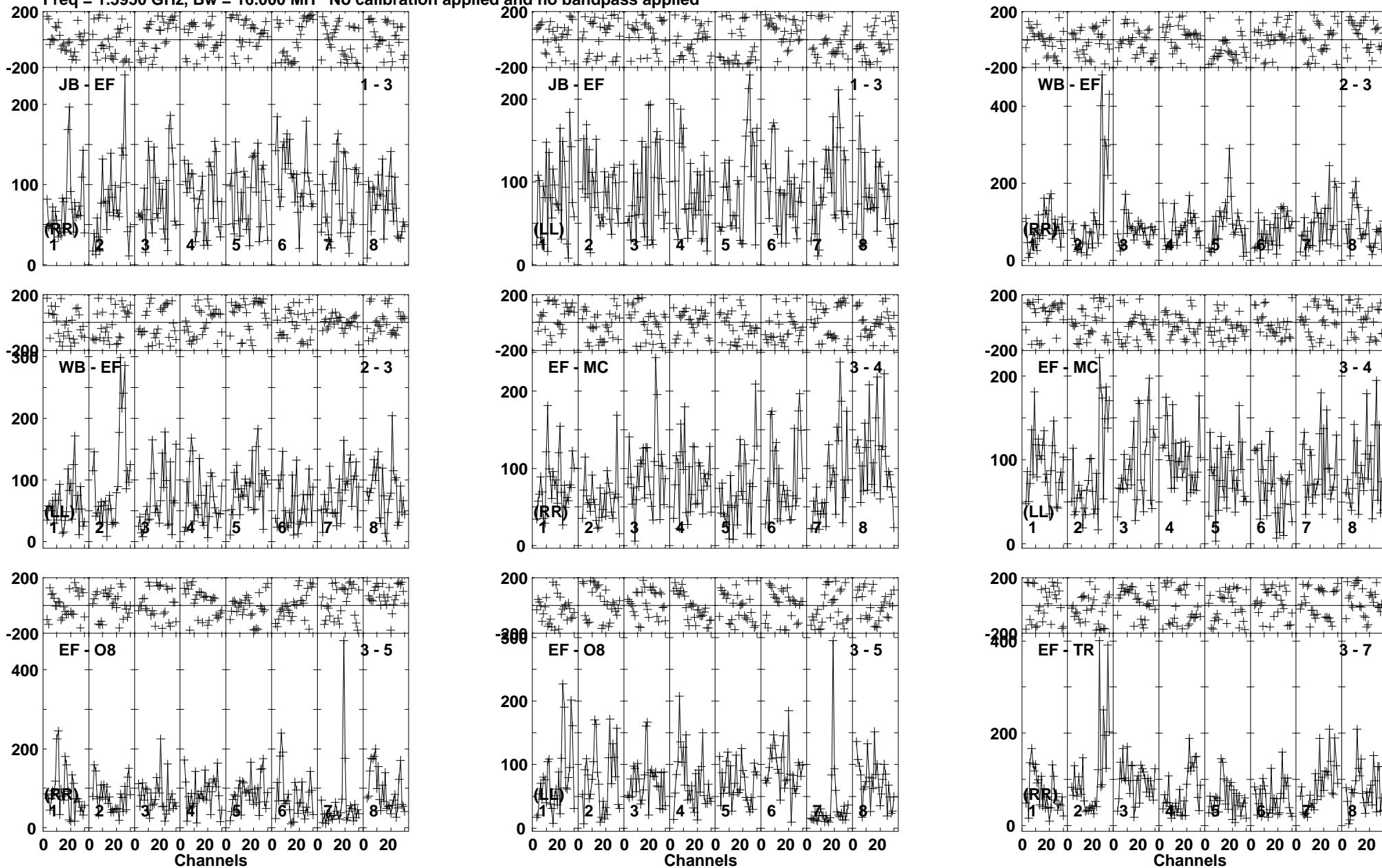
Lower frame: Micro Ampl Jy Top frame: Phas deg Vector averaged cross-power spectrum Baseline: JB (01) - EF (03) Timerange: 00/18:56:57 to 00/19:00:53
