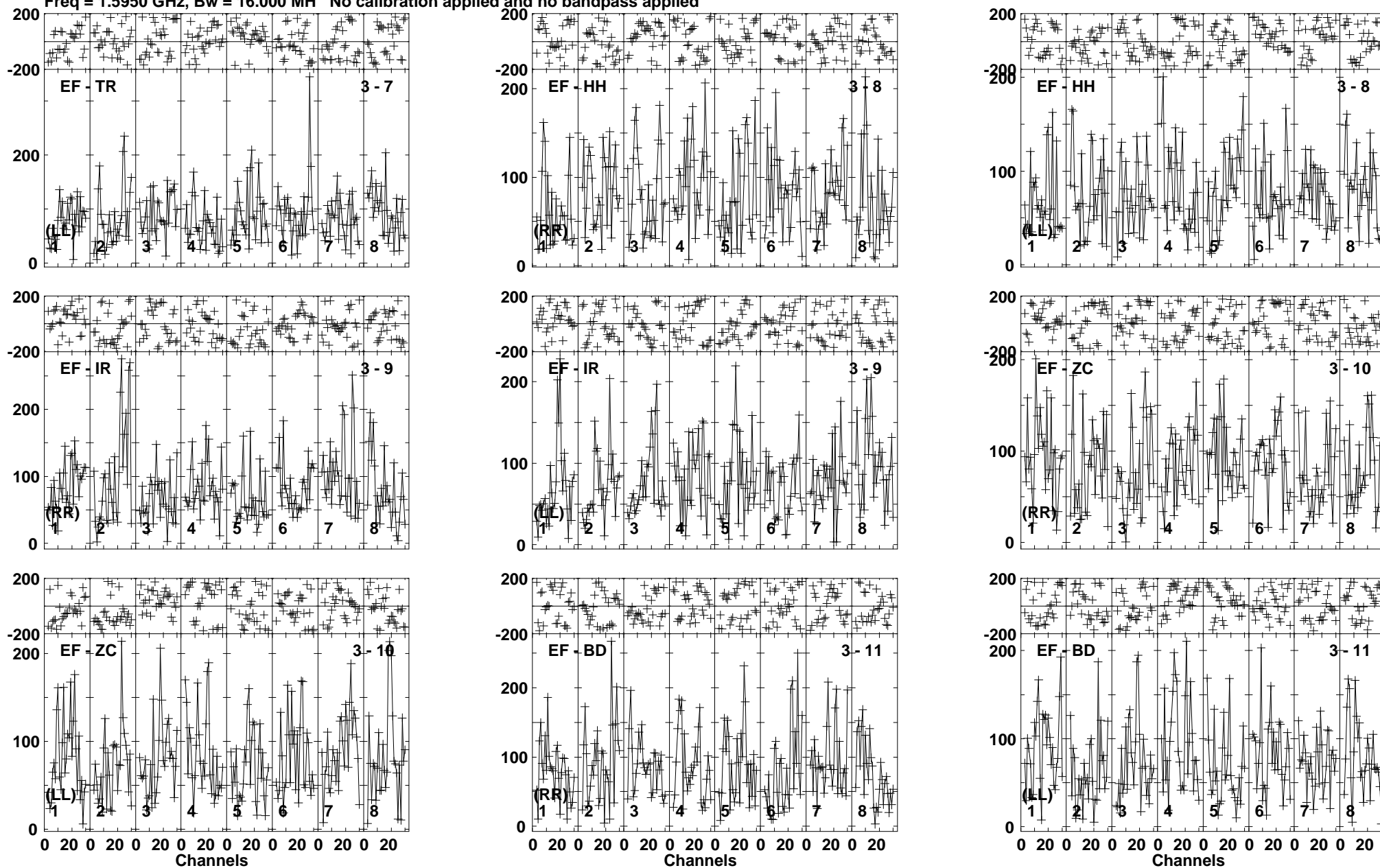
Lower frame: Micro Ampl Jy Top frame: Phas deg Vector averaged cross-power spectrum Baseline: EF (03) - TR (07) Timerange: 00/13:54:21 to 00/13:58:29
