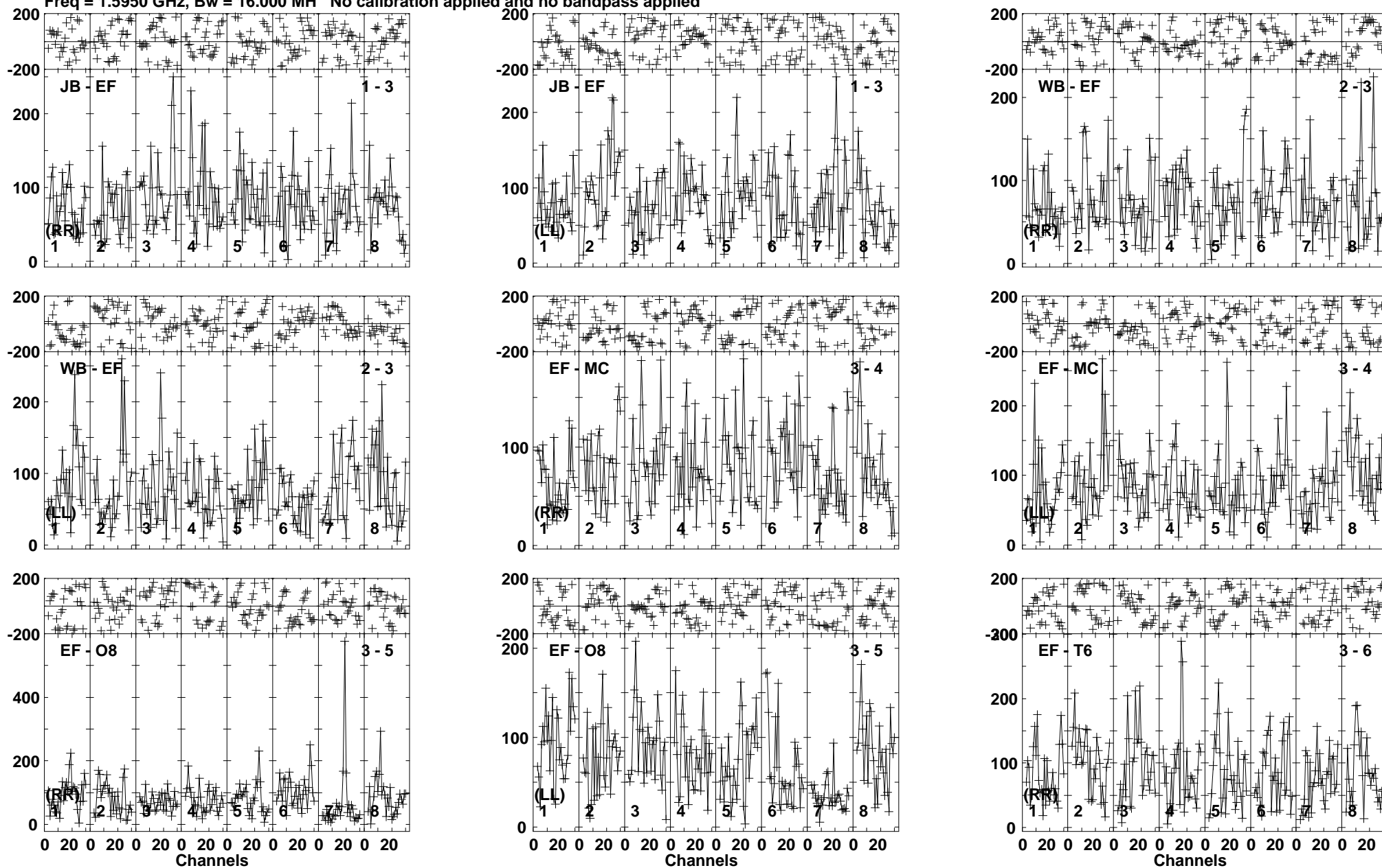
Lower frame: Micro Ampl Jy Top frame: Phas deg Vector averaged cross-power spectrum Baseline: JB (01) - EF (03) Timerange: 01/11:50:17 to 01/11:54:13
