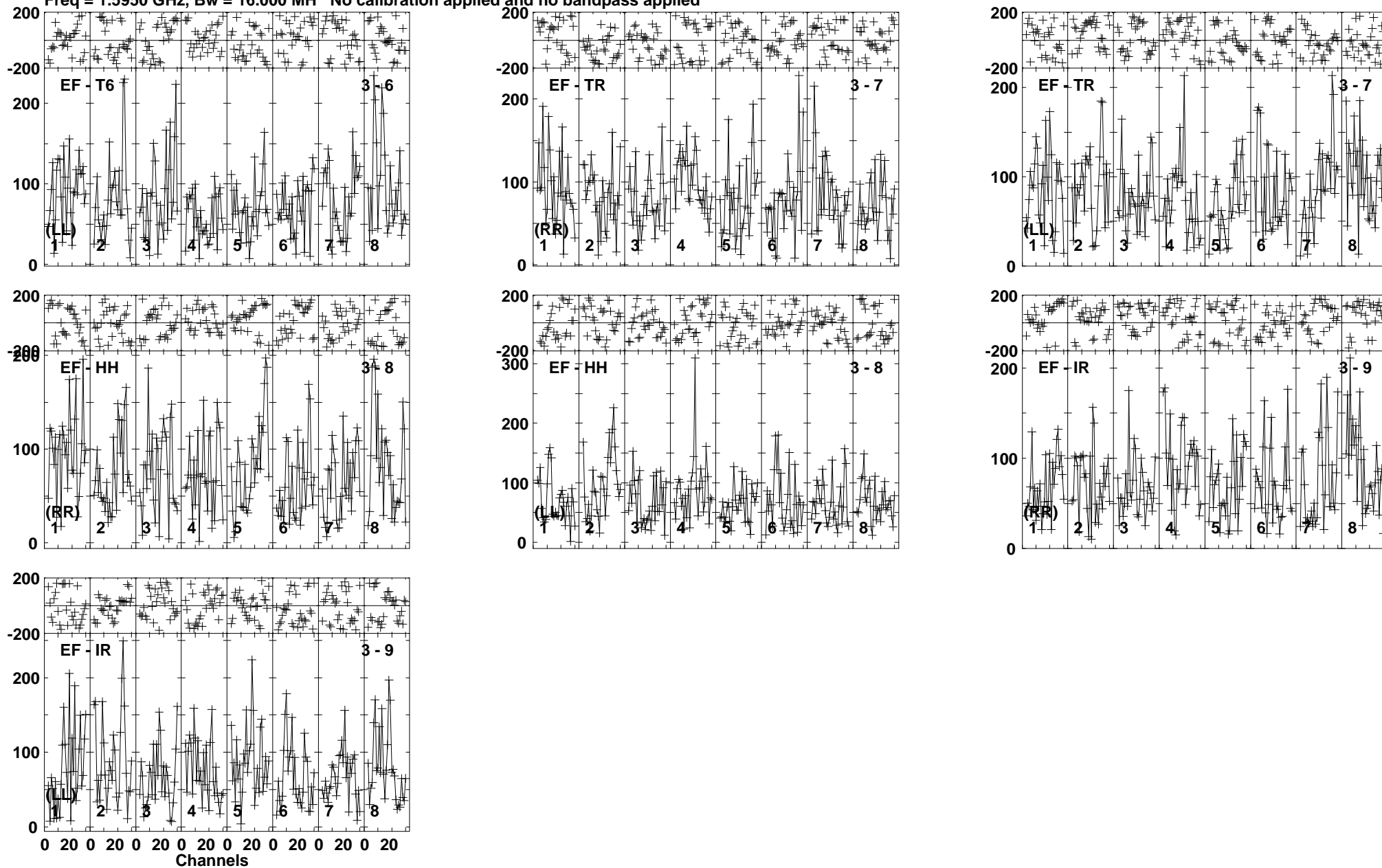
Lower frame: Micro Ampl Jy Top frame: Phas deg Vector averaged cross-power spectrum Baseline: EF (03) - T6 (06) Timerange: 01/10:59:17 to 01/11:03:13
