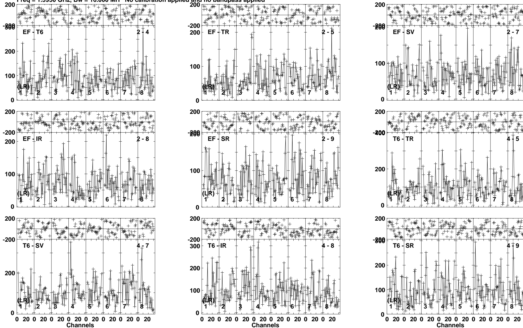
Lower frame: Micro Ampl Jy Top frame: Phas deg Vector averaged cross-power spectrum Baseline: EF (02) - T6 (04) Timerange: 00/15:24:01 to 00/15:27:59
