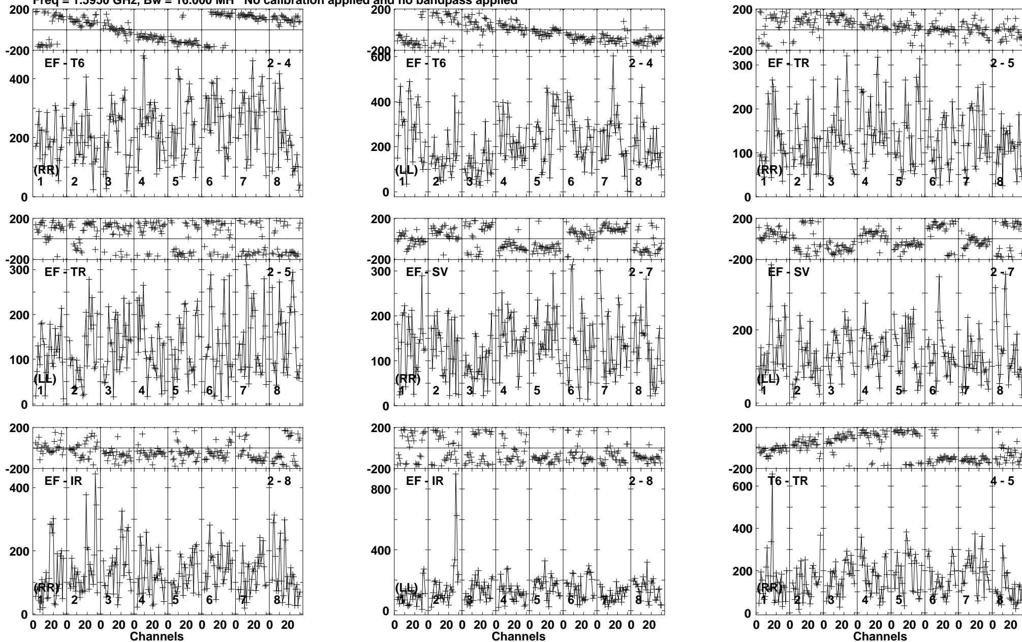
Lower frame: Micro Ampl Jy Top frame: Phas deg Vector averaged cross-power spectrum Baseline: EF (02) - T6 (04) Timerange: 00/13:32:01 to 00/13:33:59
