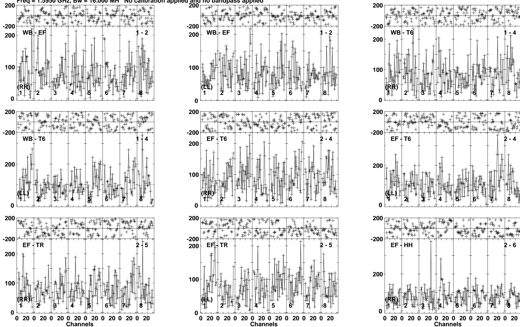
Lower frame: Micro Ampl Jy Top frame: Phas deg Vector averaged cross-power spectrum Baseline: WB (01) - EF (02) Timerange: 00/20:23:41 to 00/20:27:39
