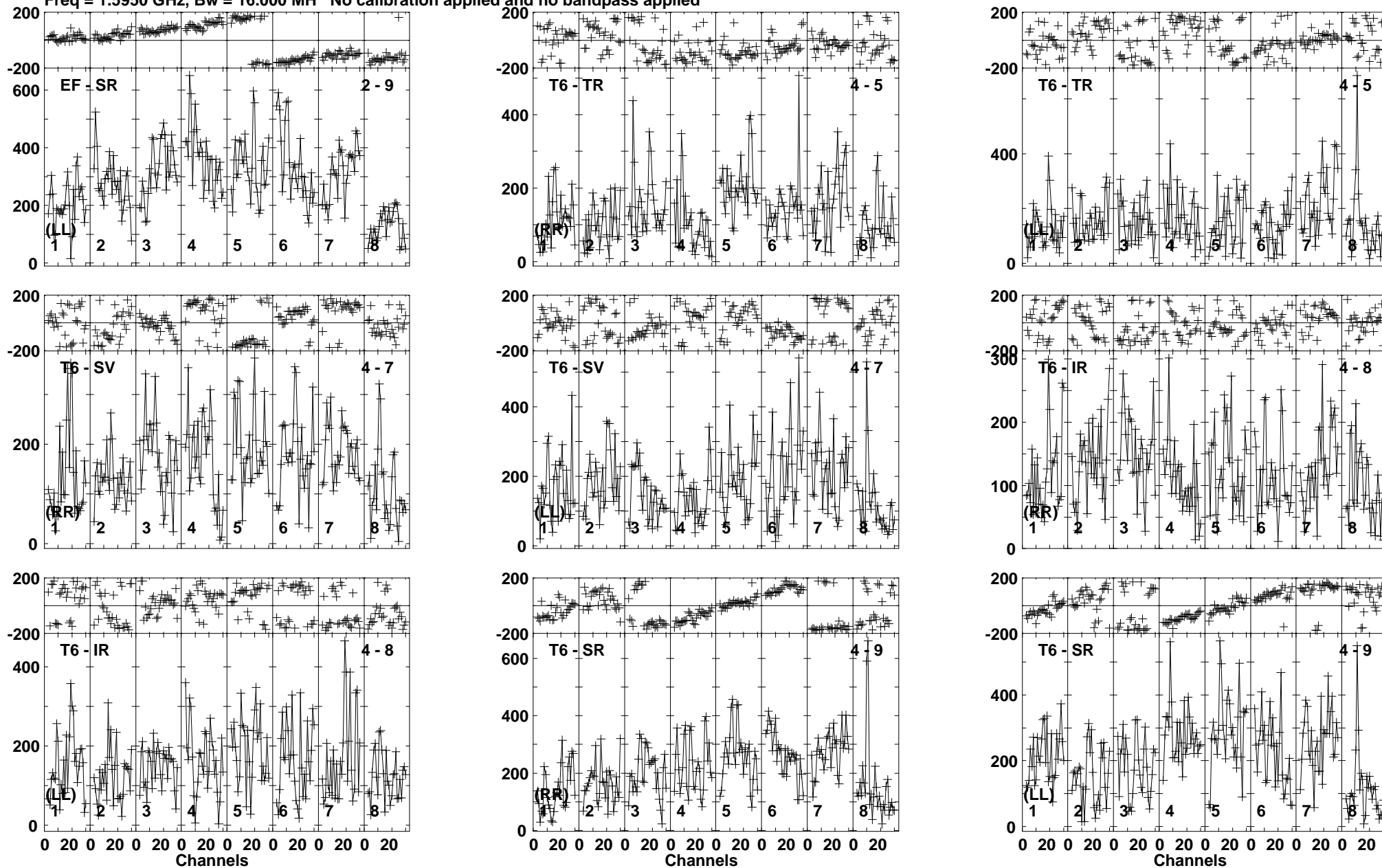
Lower frame: Micro Ampl Jy Top frame: Phas deg Vector averaged cross-power spectrum Baseline: EF (02) - SR (09) Timerange: 00/14:17:01 to 00/14:18:59
