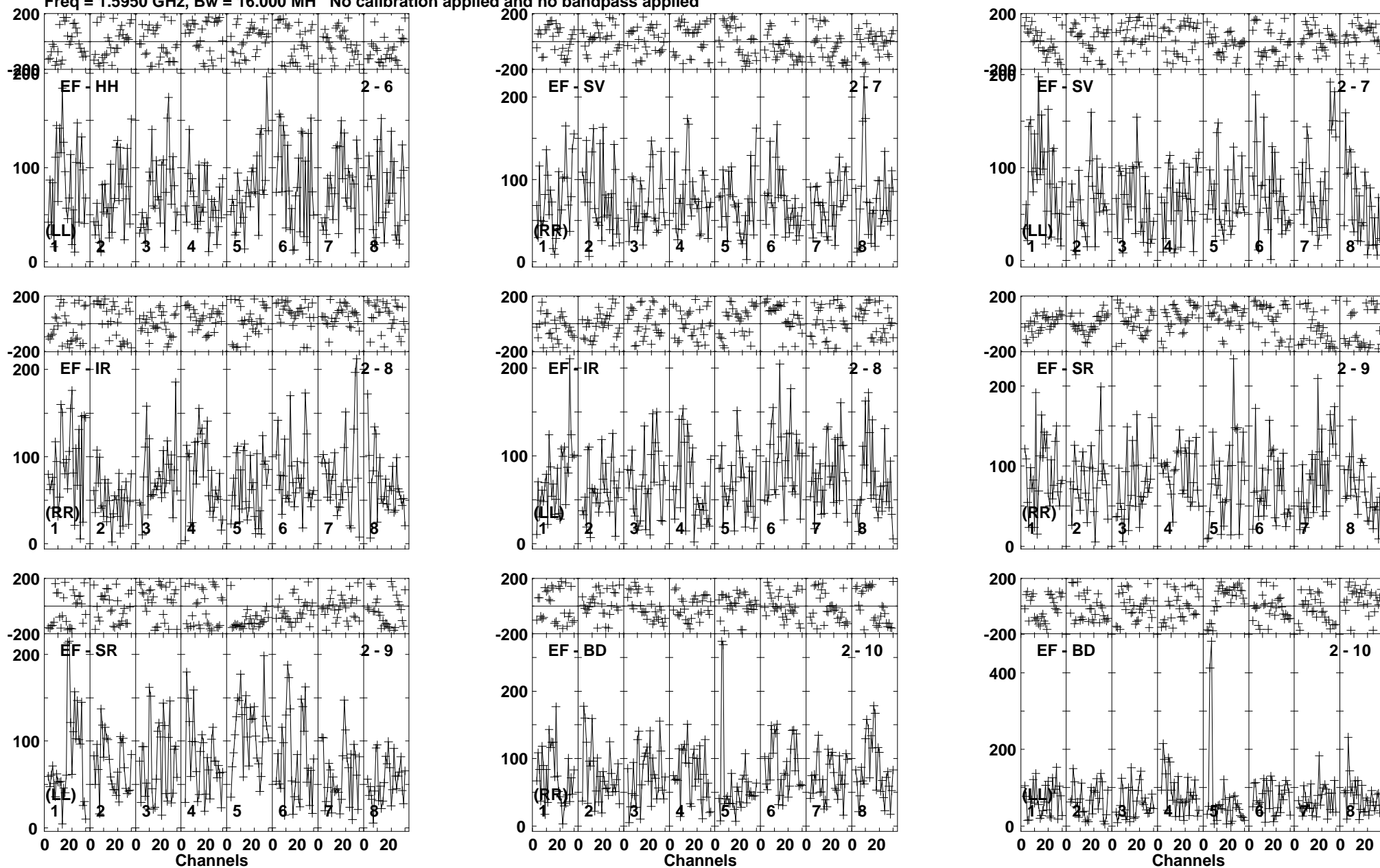
Lower frame: Micro Ampl Jy Top frame: Phas deg Vector averaged cross-power spectrum Baseline: EF (02) - HH (06) Timerange: 00/22:56:51 to 00/23:00:49
