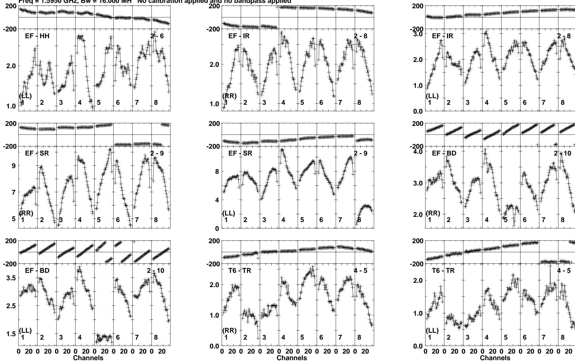
Lower frame: Milli Ampl Jy Top frame: Phas deg Vector averaged cross-power spectrum Baseline: EF (02) - HH (06) Timerange: 00/20:21:41 to 00/20:23:39
