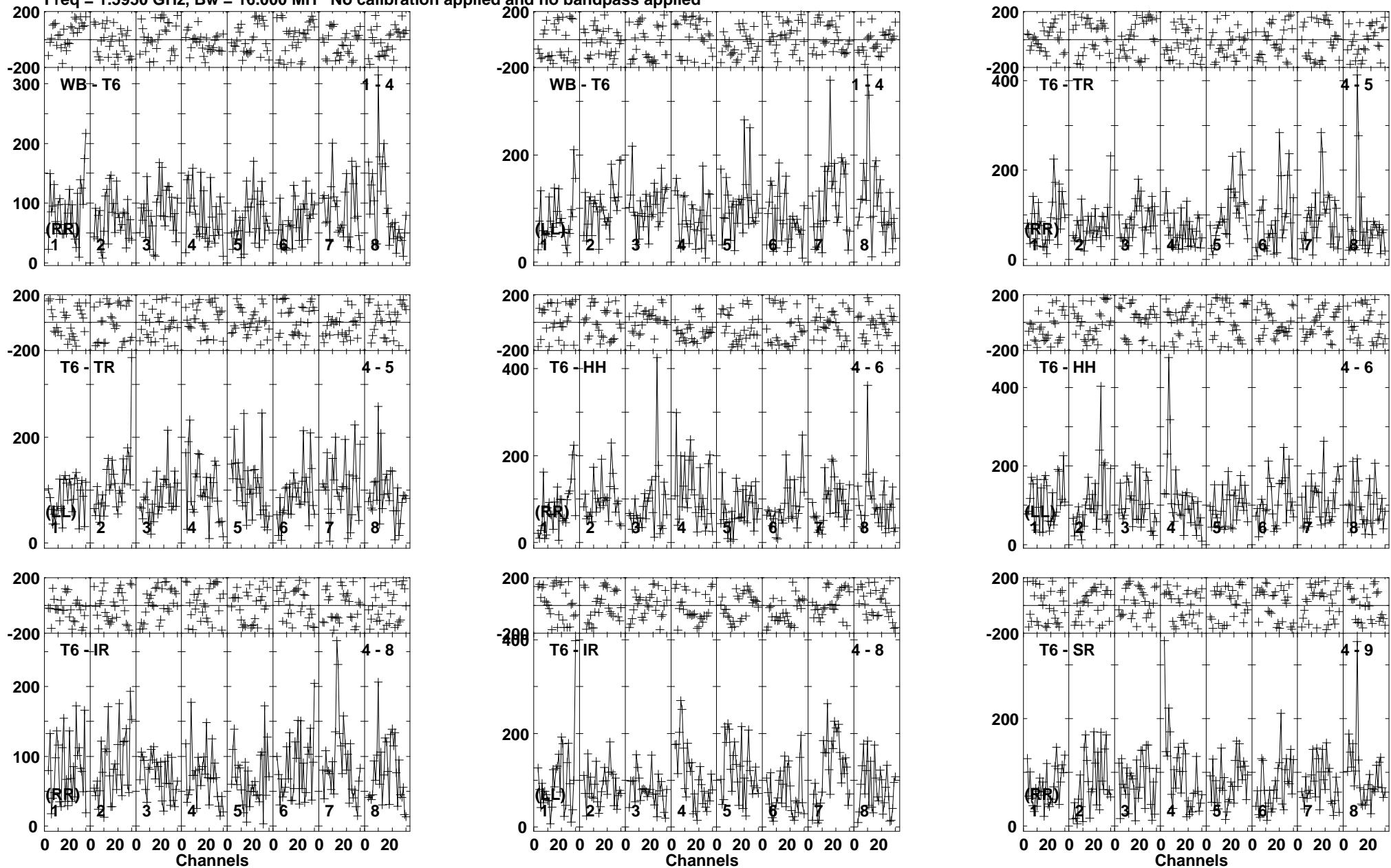
Lower frame: Micro Ampl Jy Top frame: Phas deg Vector averaged cross-power spectrum Baseline: WB (01) - T6 (04) Timerange: 00/18:24:01 to 00/18:27:59
