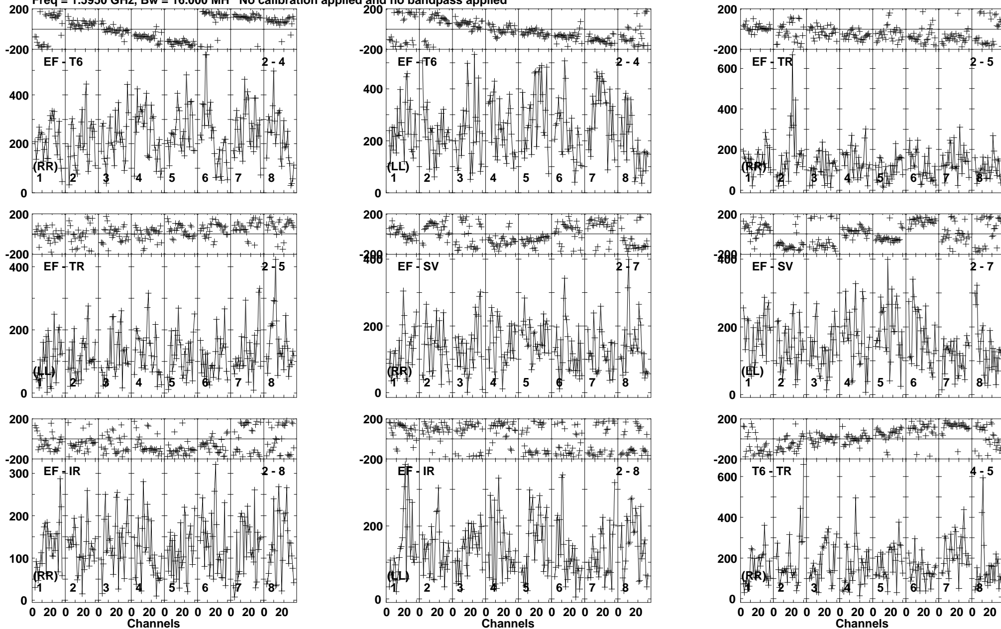
Lower frame: Micro Ampl Jy Top frame: Phas deg Vector averaged cross-power spectrum Baseline: EF (02) - T6 (04) Timerange: 00/13:25:01 to 00/13:26:59
