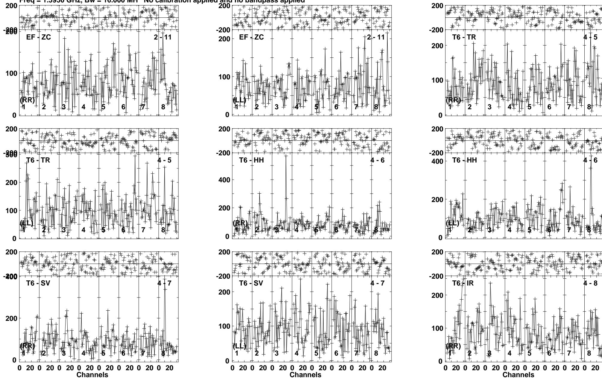
Lower frame: Micro Ampl Jy Top frame: Phas deg Vector averaged cross-power spectrum Baseline: EF (02) - ZC (11) Timerange: 00/22:49:51 to 00/22:53:49
