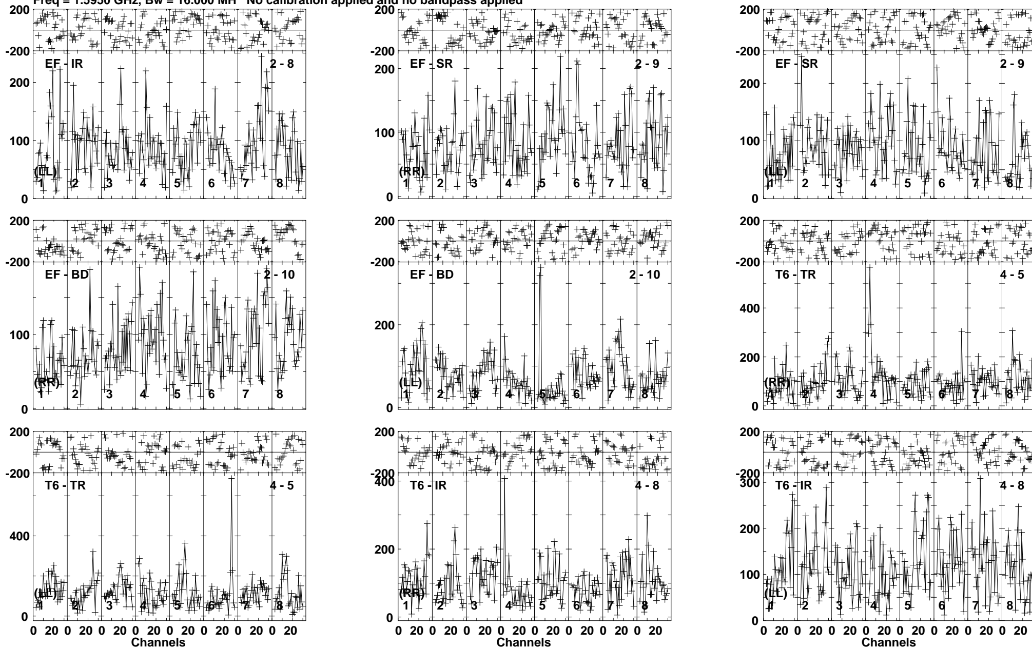
Lower frame: Micro Ampl Jy Top frame: Phas deg Vector averaged cross-power spectrum Baseline: EF (02) - IR (08) Timerange: 00/20:00:01 to 00/20:02:59
