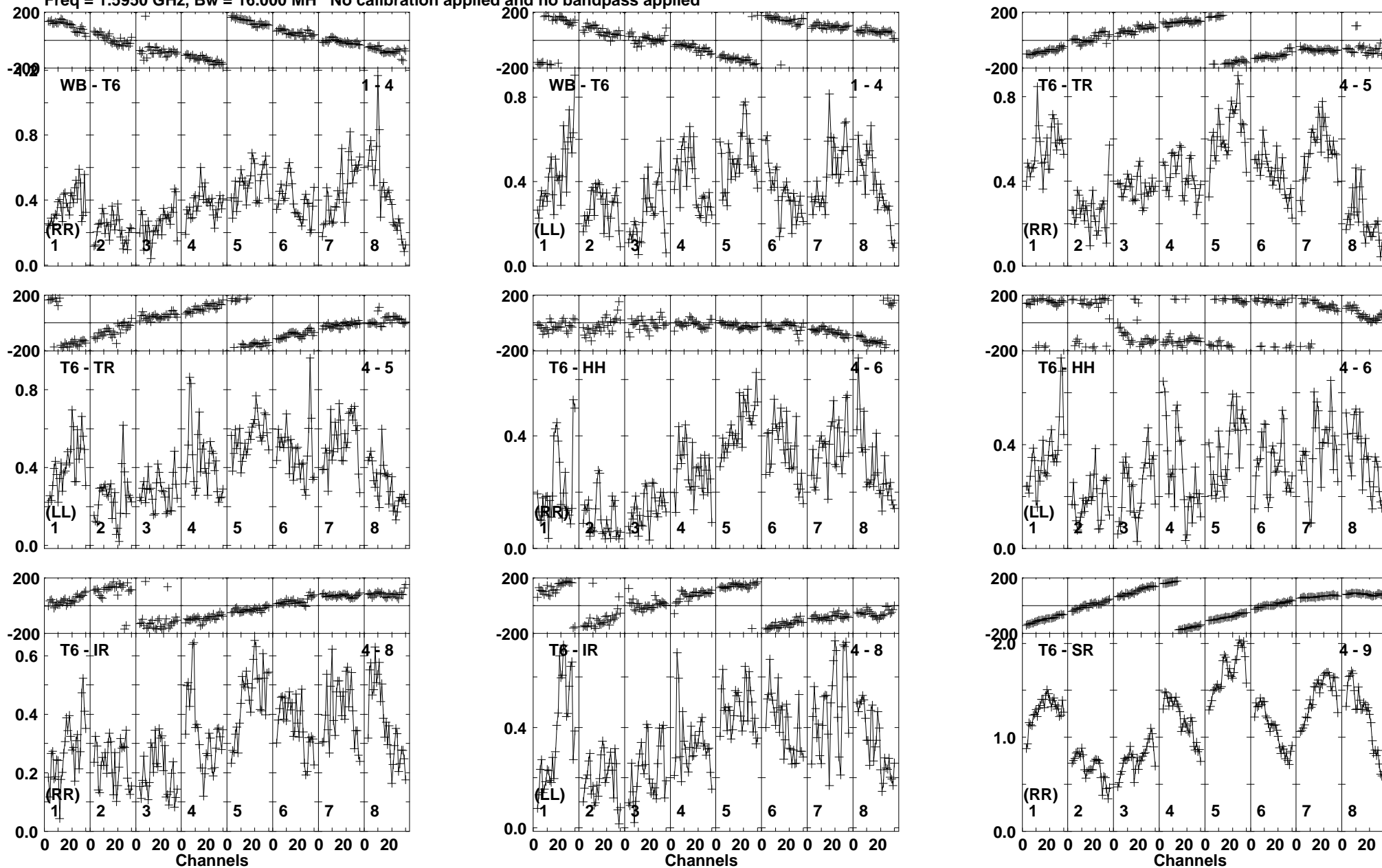
Lower frame: Milli Ampl Jy Top frame: Phas deg Vector averaged cross-power spectrum Baseline: WB (01) - T6 (04) Timerange: 00/18:29:01 to 00/18:30:59
