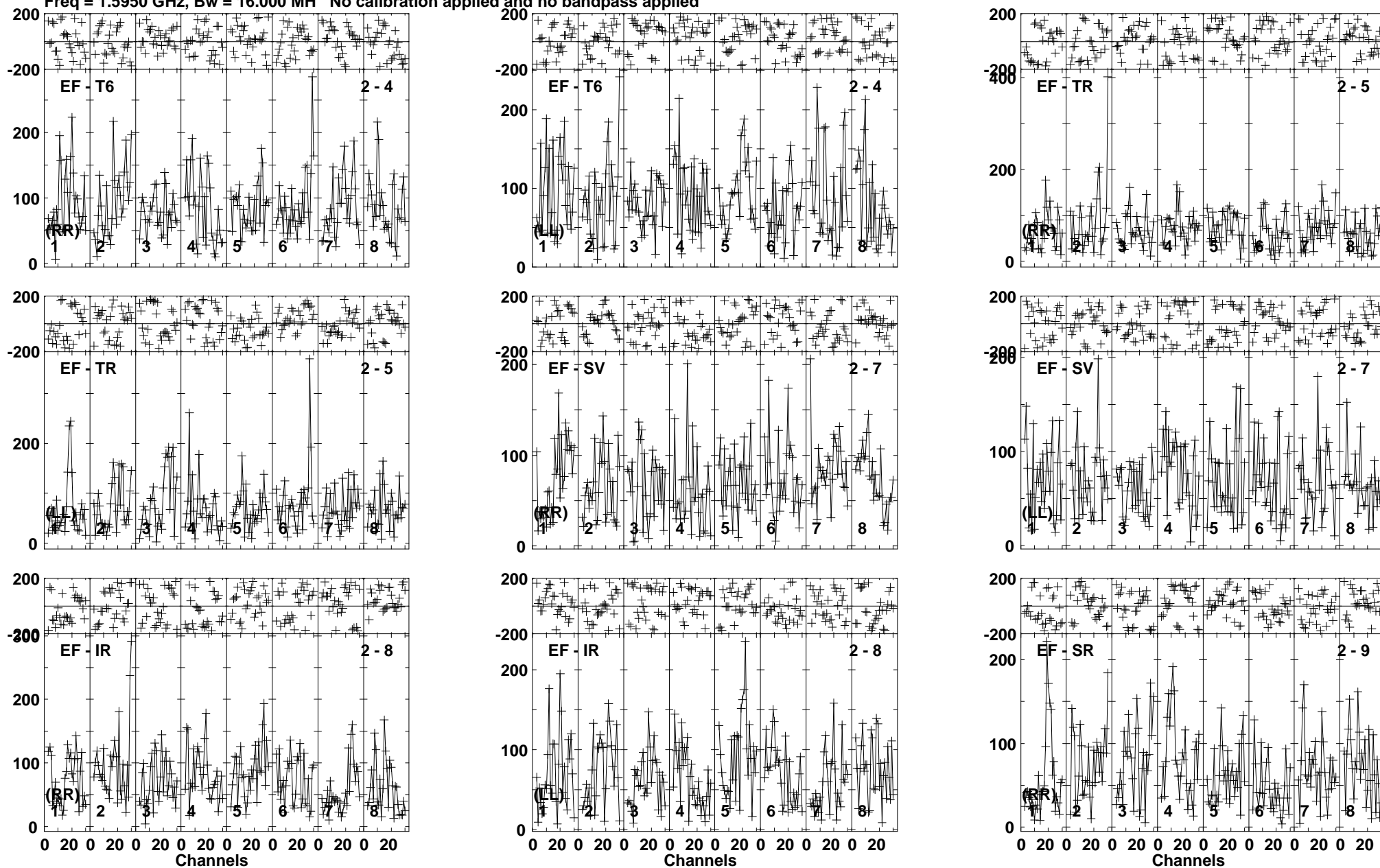
Lower frame: Micro Ampl Jy Top frame: Phas deg Vector averaged cross-power spectrum Baseline: EF (02) - T6 (04) Timerange: 00/14:00:01 to 00/14:03:59
