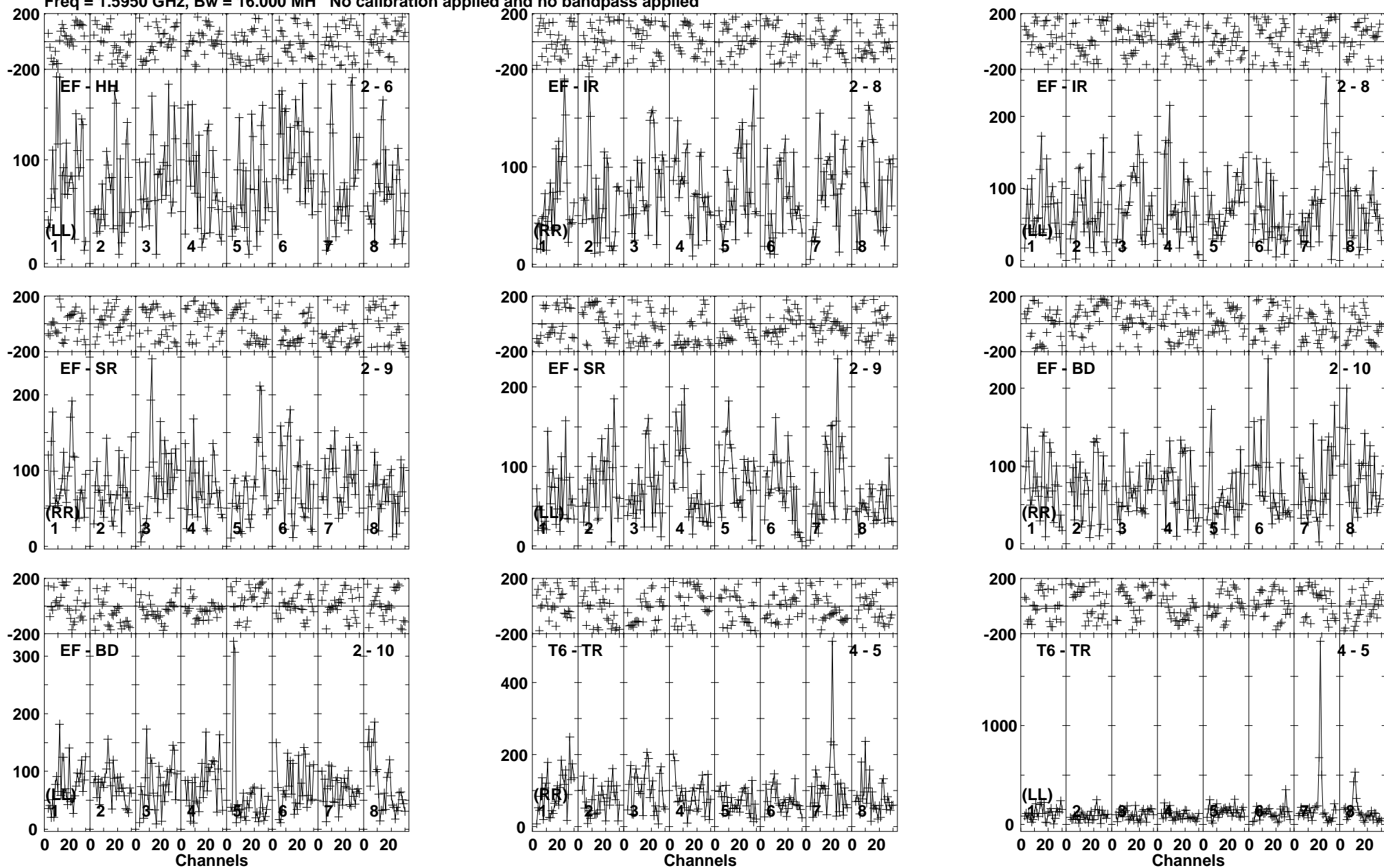
Lower frame: Micro Ampl Jy Top frame: Phas deg Vector averaged cross-power spectrum Baseline: EF (02) - HH (06) Timerange: 00/20:23:41 to 00/20:27:39
