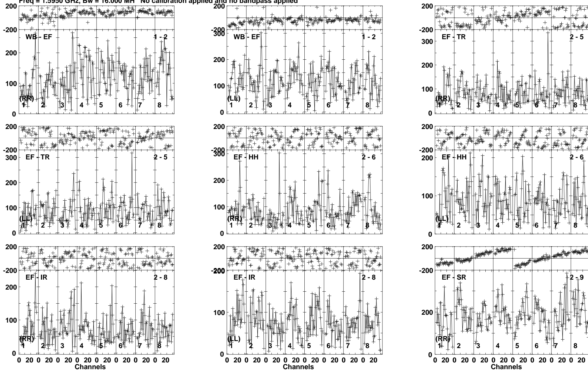
Lower frame: Micro Ampl Jy Top frame: Phas deg Vector averaged cross-power spectrum Baseline: WB (01) - EF (02) Timerange: 00:21:56:11 to 00:22:00:09
