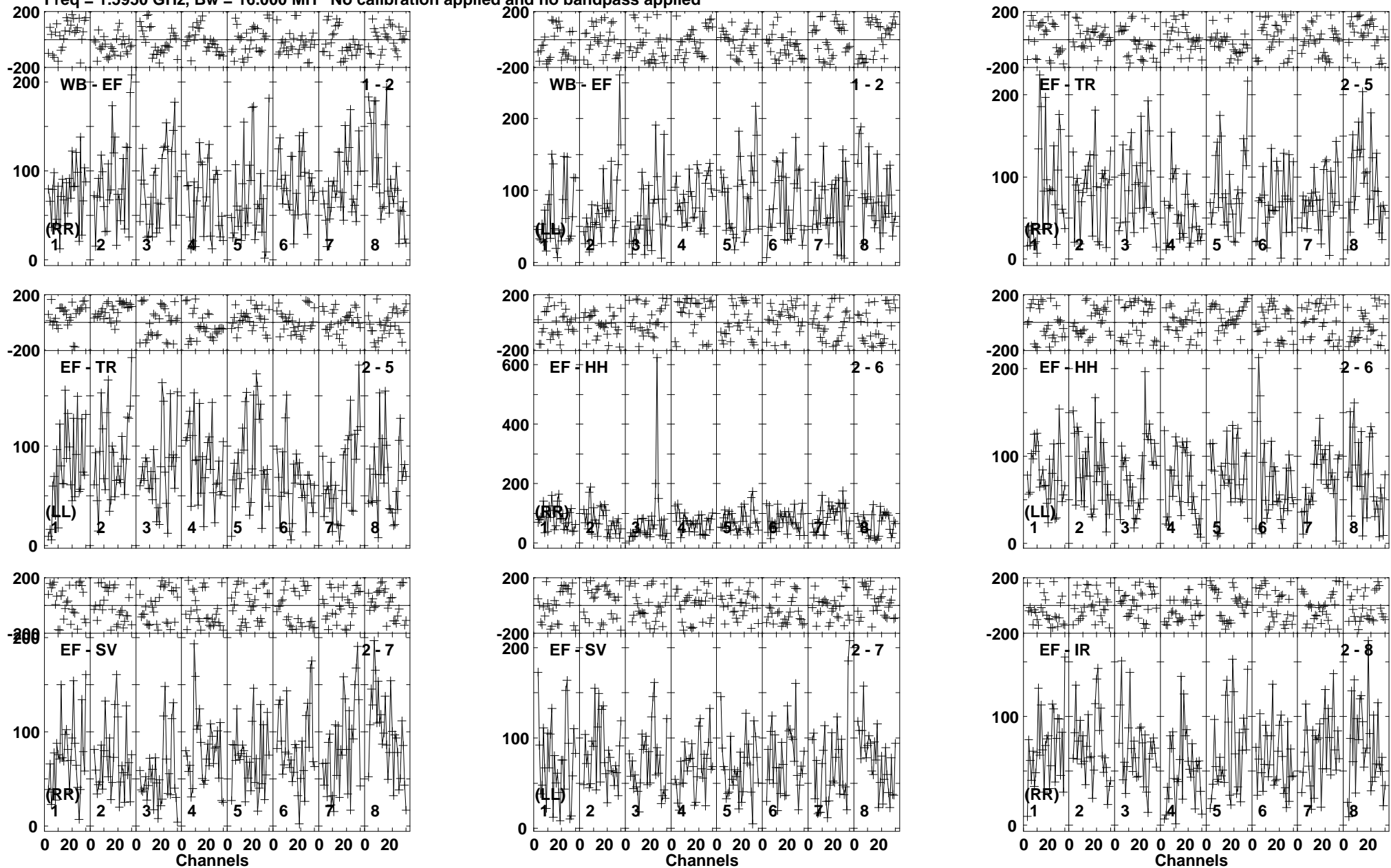
Lower frame: Micro Ampl Jy Top frame: Phas deg Vector averaged cross-power spectrum Baseline: WB (01) - EF (02) Timerange: 00/23:43:51 to 00/23:47:49
