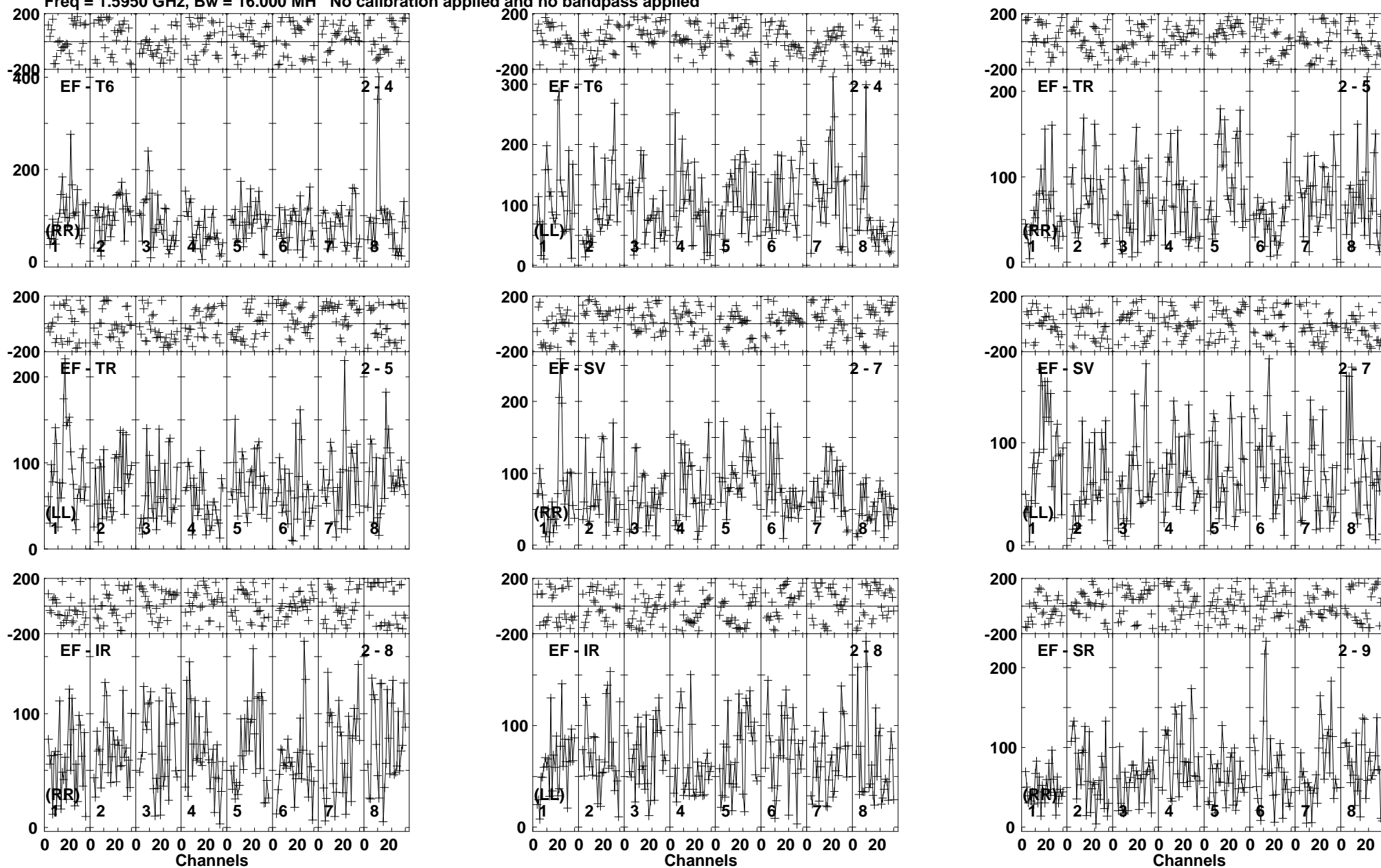
Lower frame: Micro Ampl Jy Top frame: Phas deg Vector averaged cross-power spectrum Baseline: EF (02) - T6 (04) Timerange: 00/14:06:01 to 00/14:09:59
