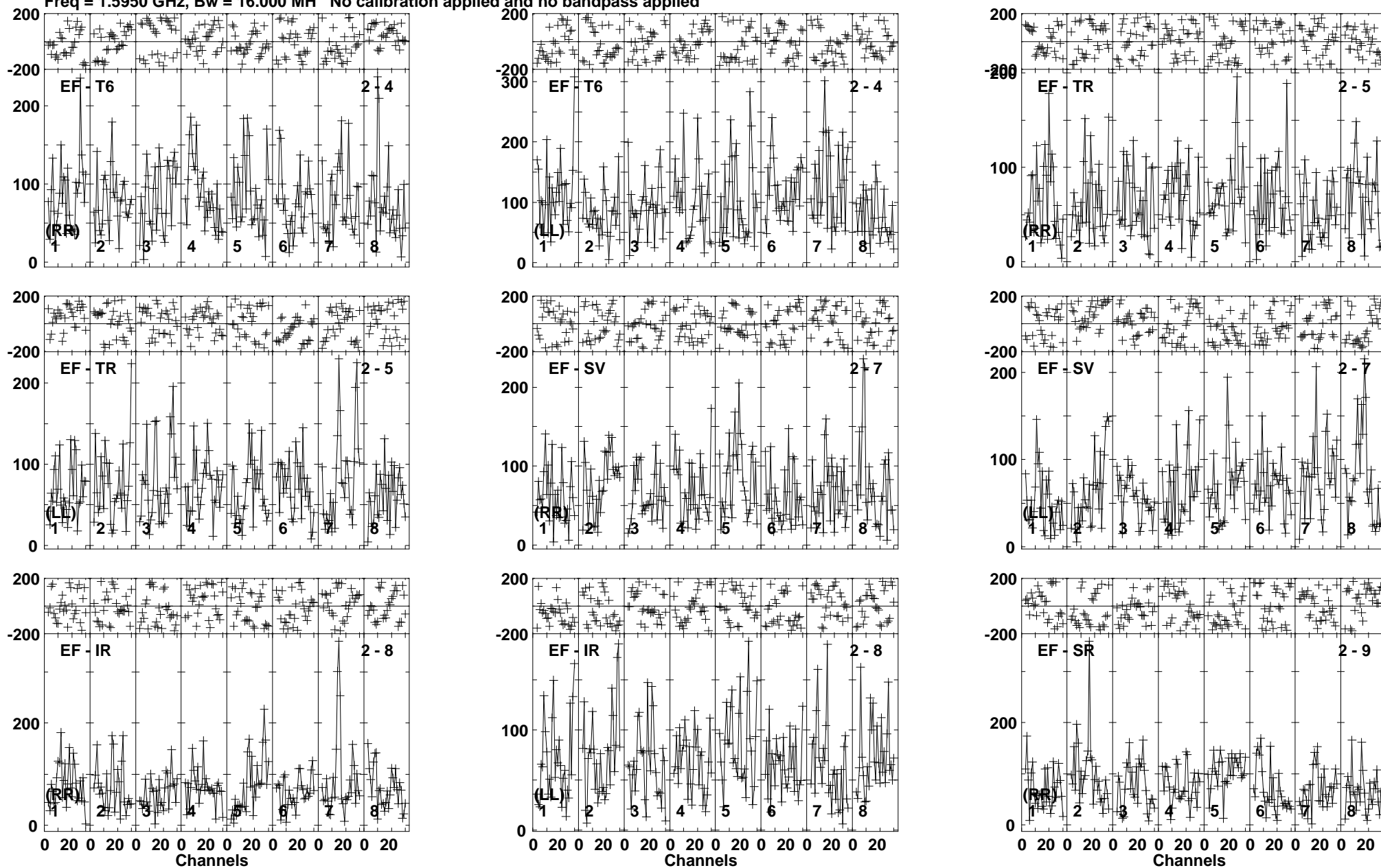
Lower frame: Micro Ampl Jy Top frame: Phas deg Vector averaged cross-power spectrum Baseline: EF (02) - T6 (04) Timerange: 00/14:52:01 to 00/14:55:59
