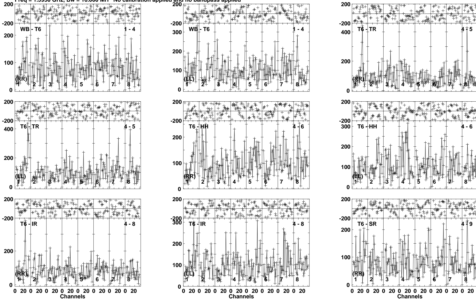
Lower frame: Micro Ampl Jy Top frame: Phas deg Vector averaged cross-power spectrum Baseline: WB (01) - T6 (04) Timerange: 00/15:45:01 to 00/15:48:59
