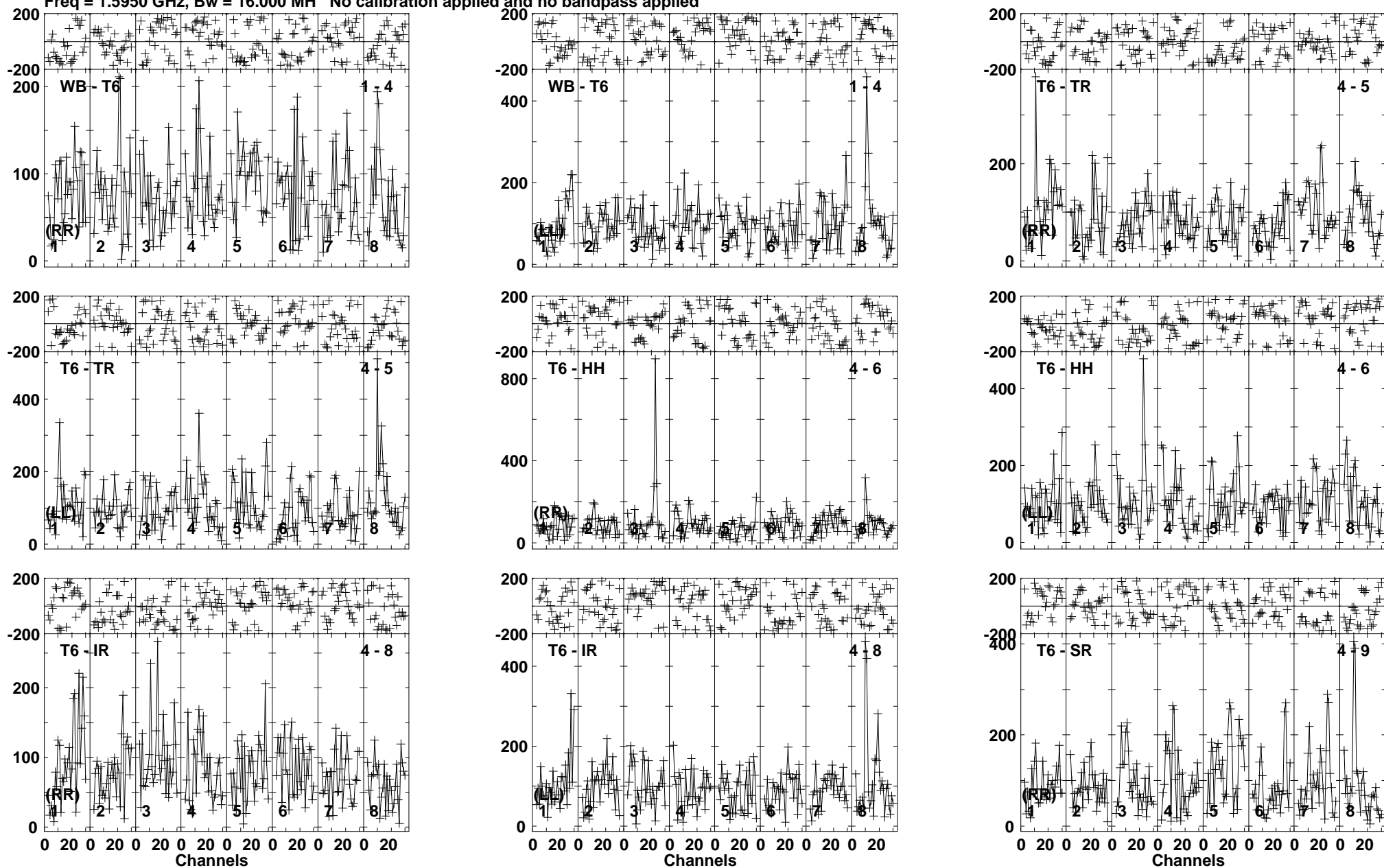
Lower frame: Micro Ampl Jy Top frame: Phas deg Vector averaged cross-power spectrum Baseline: WB (01) - T6 (04) Timerange: 00/16:18:01 to 00/16:21:59
