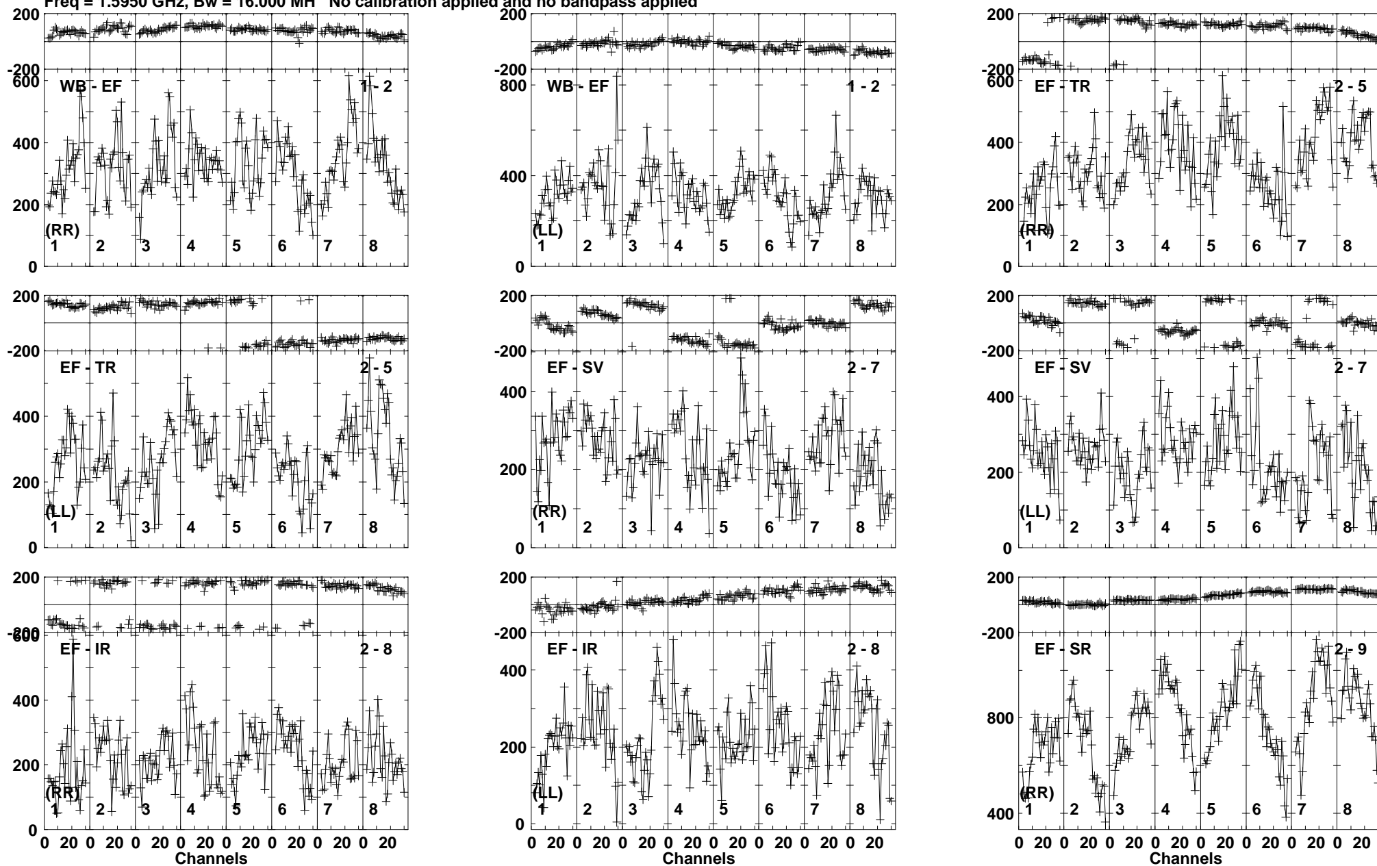
Lower frame: Micro Ampl Jy Top frame: Phas deg Vector averaged cross-power spectrum Baseline: WB (01) - EF (02) Timerange: 00:22:37:11 to 00:22:39:09
