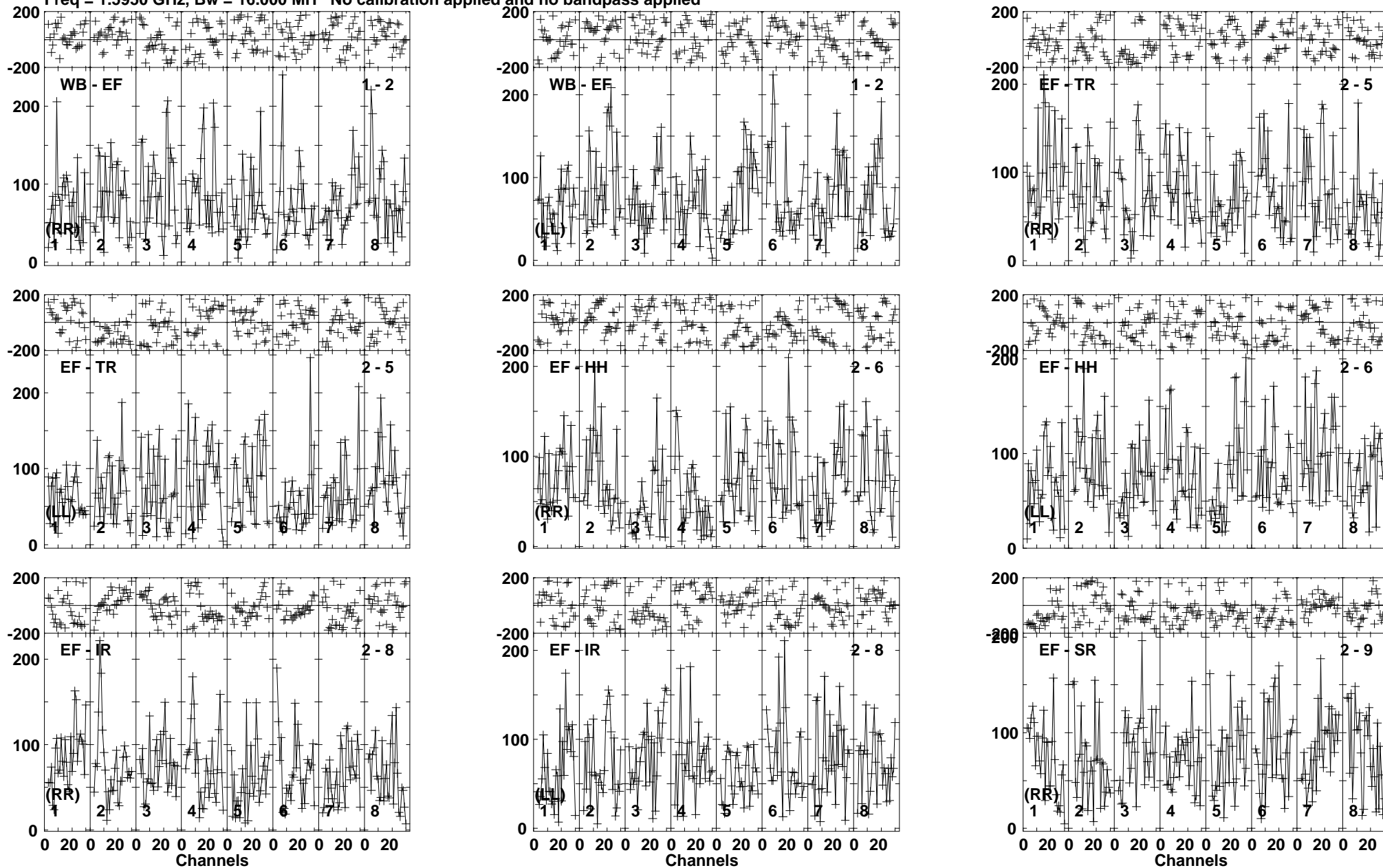
Lower frame: Micro Ampl Jy Top frame: Phas deg Vector averaged cross-power spectrum Baseline: WB (01) - EF (02) Timerange: 00/20:44:41 to 00/20:48:39
