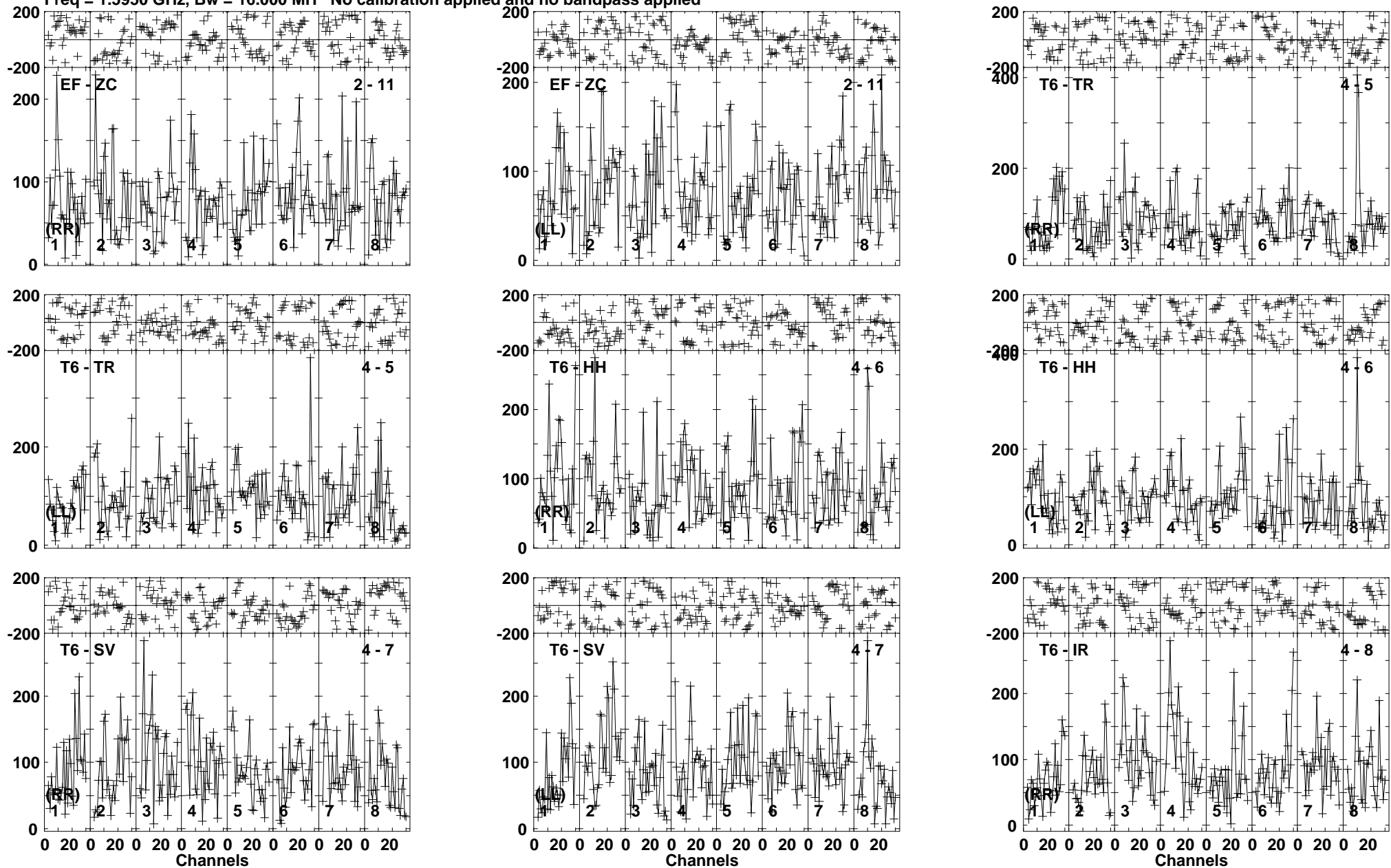
Lower frame: Micro Ampl Jy Top frame: Phas deg Vector averaged cross-power spectrum Baseline: EF (02) - ZC (11) Timerange: 00/23:02:51 to 00/23:06:49
