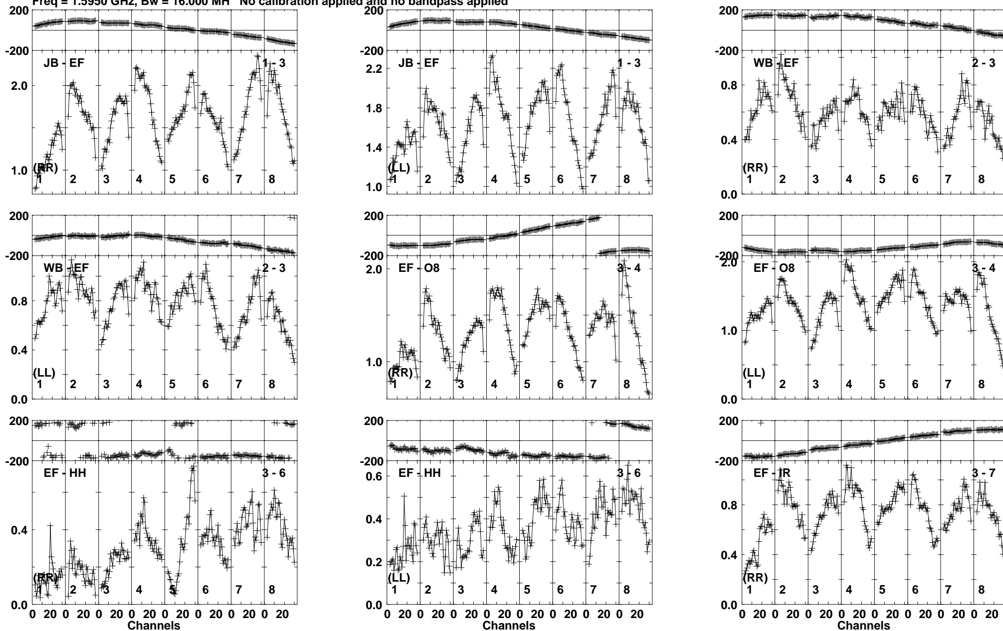
Lower frame: Milli Ampl Jy Top frame: Phas deg Vector averaged cross-power spectrum Baseline: JB (01) - EF (03) Timerange: 00/06:42:00 to 00/06:46:00
