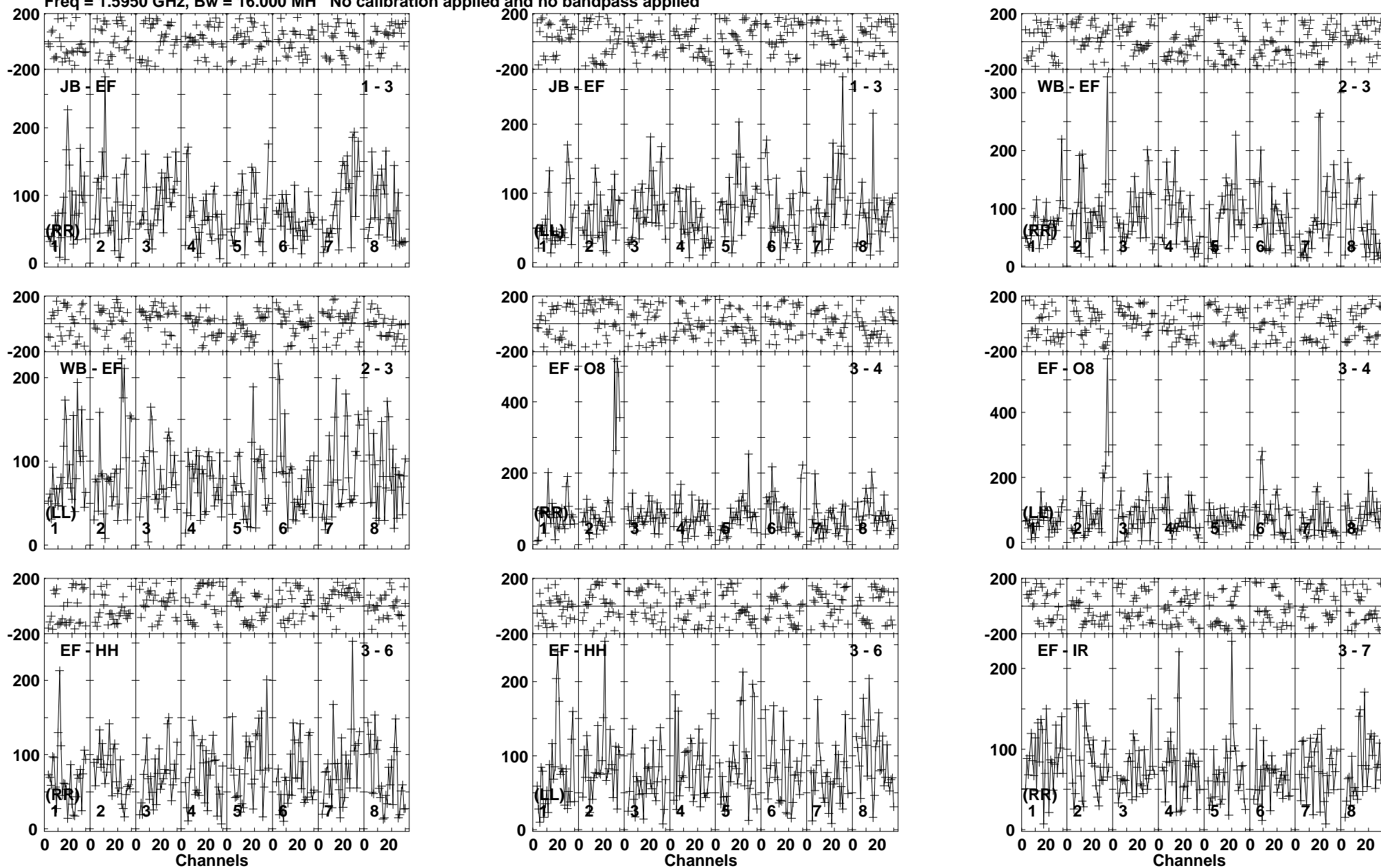
Lower frame: Micro Ampl Jy Top frame: Phas deg Vector averaged cross-power spectrum Baseline: JB (01) - EF (03) Timerange: 00/07:55:00 to 00/07:59:00
