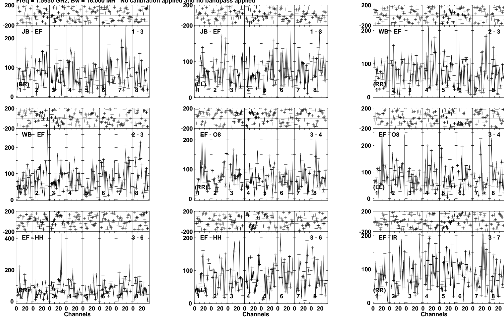
Lower frame: Micro Ampl Jy Top frame: Phas deg Vector averaged cross-power spectrum Baseline: JB (01) - EF (03) Timerange: 00/09:30:31 to 00/09:34:30
