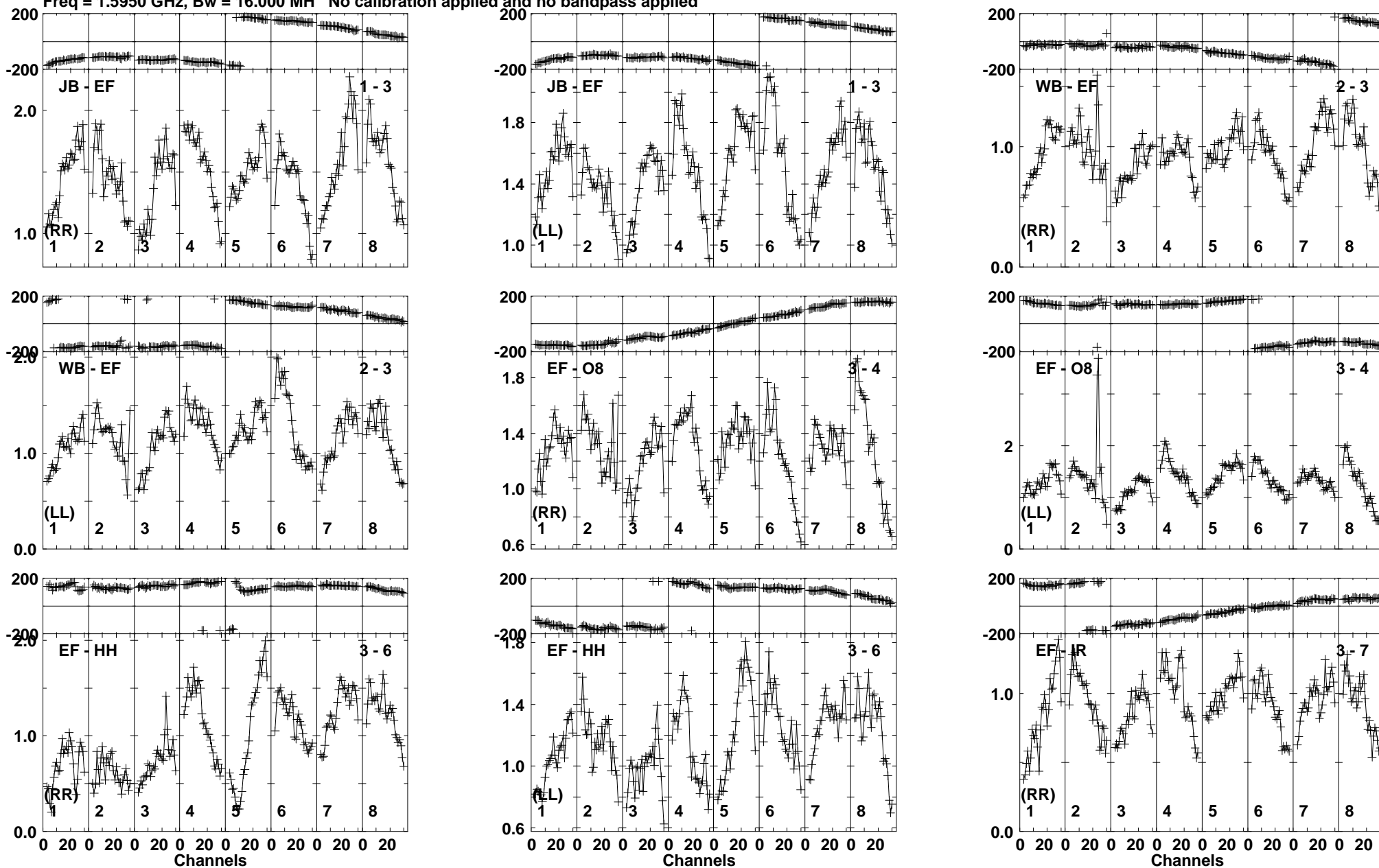
Lower frame: Milli Ampl Jy Top frame: Phas deg Vector averaged cross-power spectrum Baseline: JB (01) - EF (03) Timerange: 00/07:46:30 to 00/07:48:30
