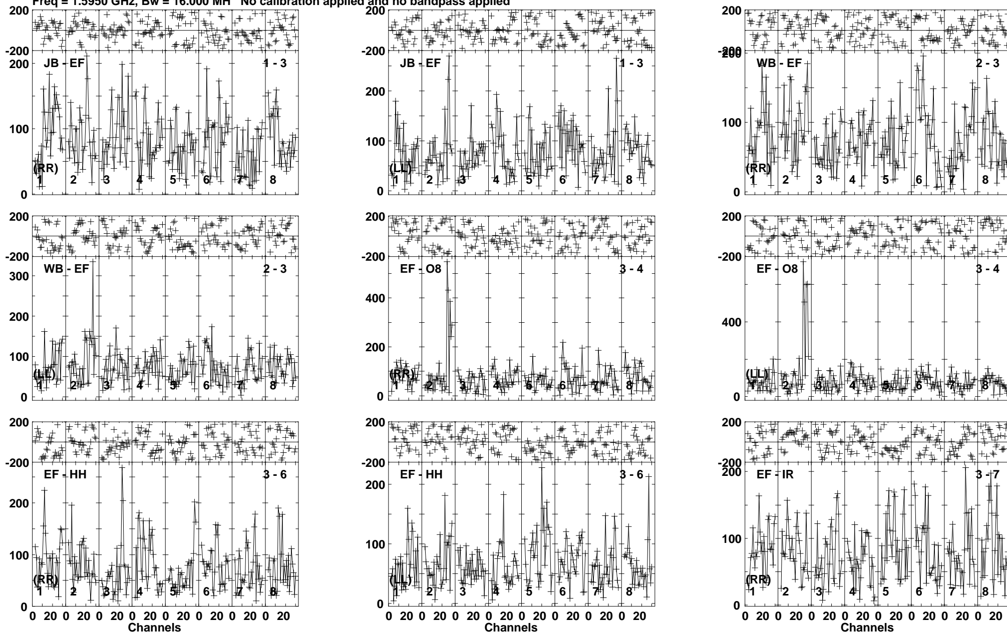
Lower frame: Micro Ampl Jy Top frame: Phas deg Vector averaged cross-power spectrum Baseline: JB (01) - EF (03) Timerange: 00/10/08:01 to 00/10/11:59
