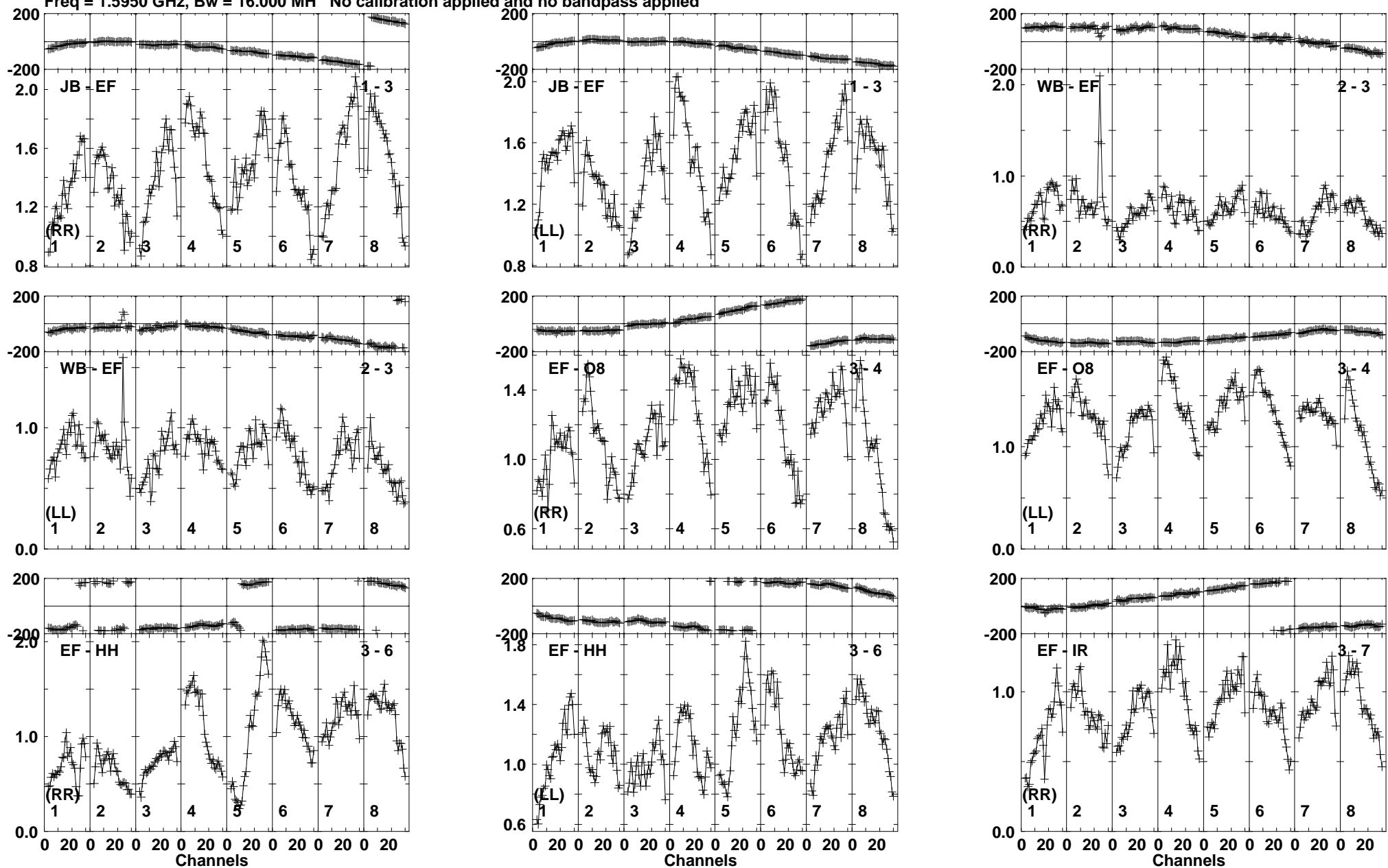
Lower frame: Milli Ampl Jy Top frame: Phas deg Vector averaged cross-power spectrum Baseline: JB (01) - EF (03) Timerange: 00/07:28:00 to 00/07:30:00
