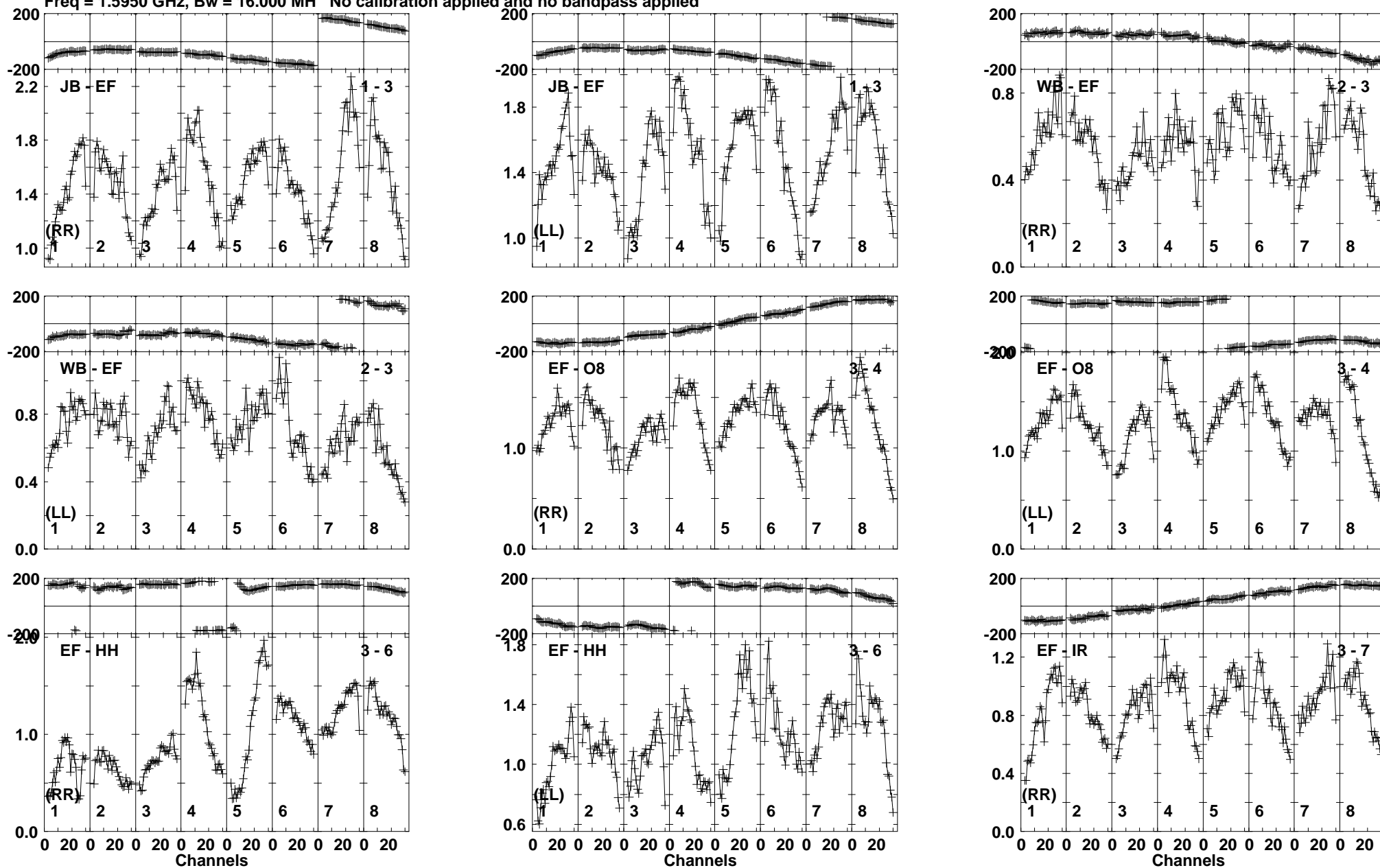
Lower frame: Milli Ampl Jy Top frame: Phas deg Vector averaged cross-power spectrum Baseline: JB (01) - EF (03) Timerange: 00/07:40:31 to 00/07:42:30
