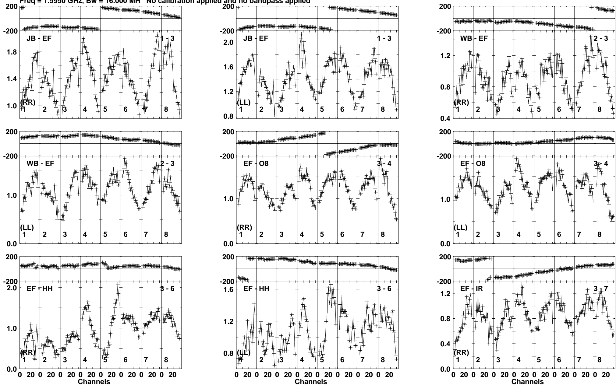
Lower frame: Milli Ampl Jy Top frame: Phas deg Vector averaged cross-power spectrum Baseline: JB (01) - EF (03) Timerange: 00/10:12:01 to 00/10:14:00
