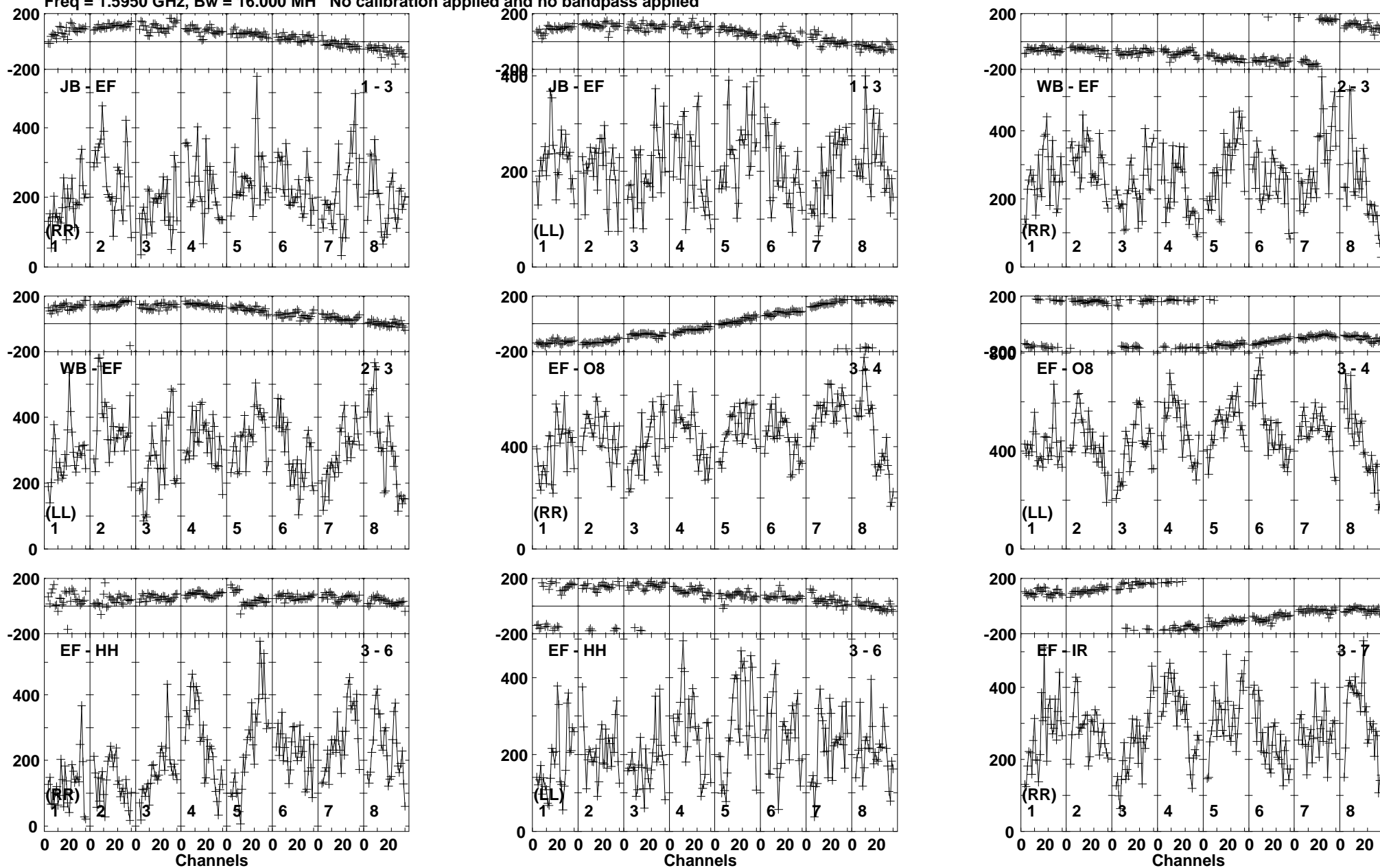
Lower frame: Micro Ampl Jy Top frame: Phas deg Vector averaged cross-power spectrum Baseline: JB (01) - EF (03) Timerange: 00/07:11:30 to 00/07:13:30
