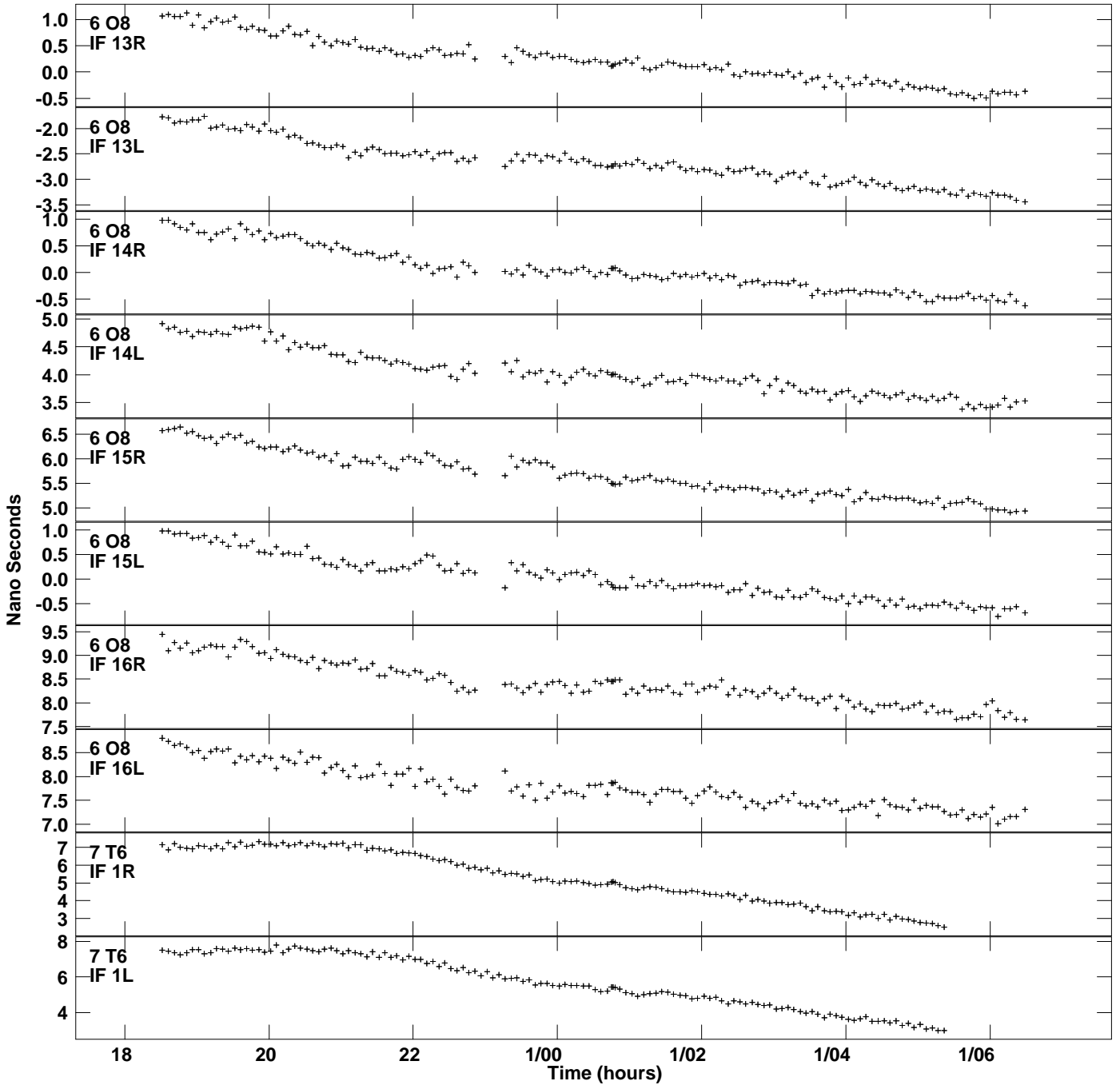
Plot file version 17 created 31-MAR-2023 15:57:13 Delay vs UTC time for EP124A.UVDATA.1 SN 3 Rpol & Lpol IF 1 - 16
