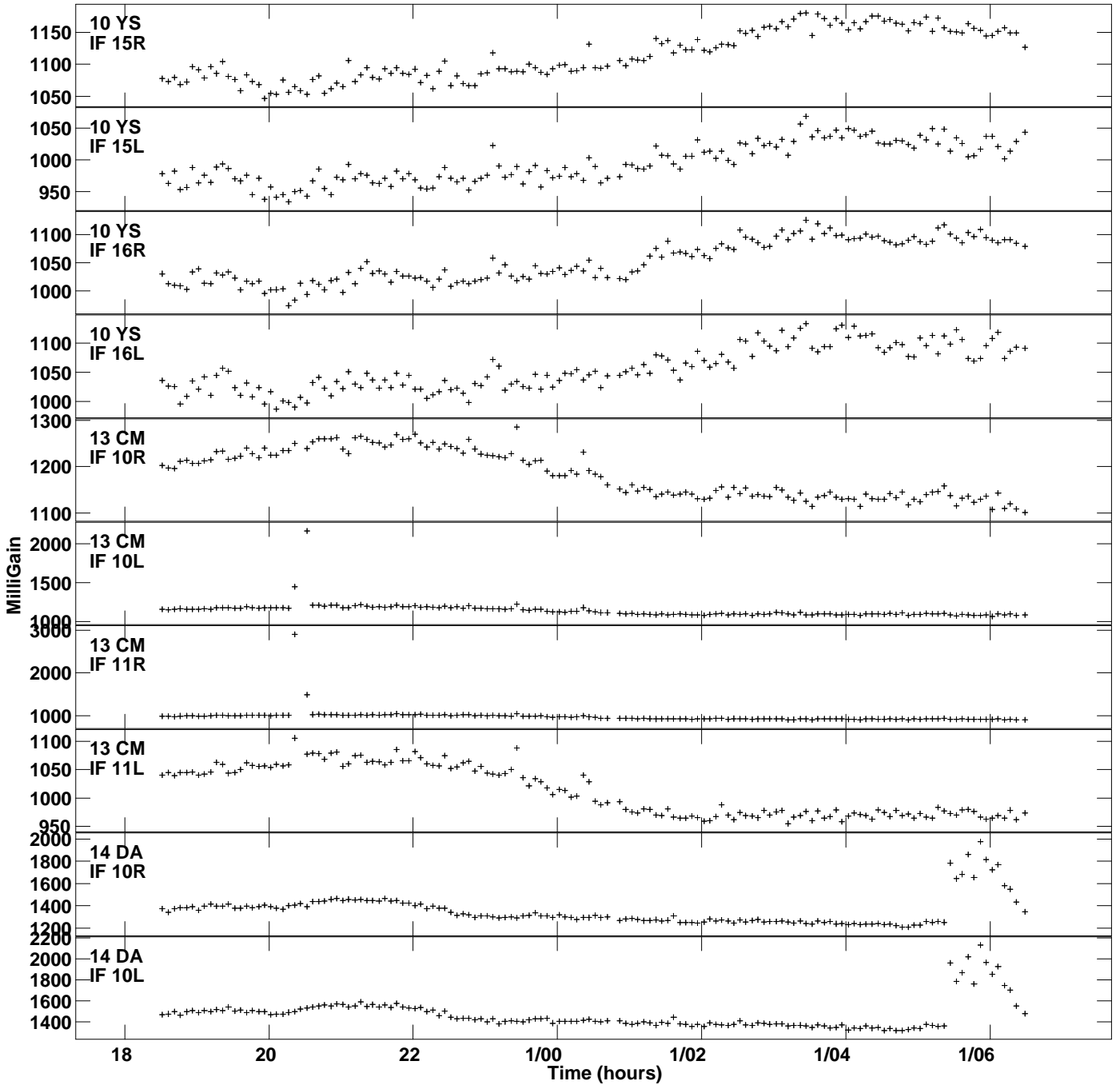
Plot file version 27 created 31-MAR-2023 16:32:32 Gain amp vs UTC time for J1128+5925.MULTI.1 SN 2 Rpol & Lpol IF 1 - 16
