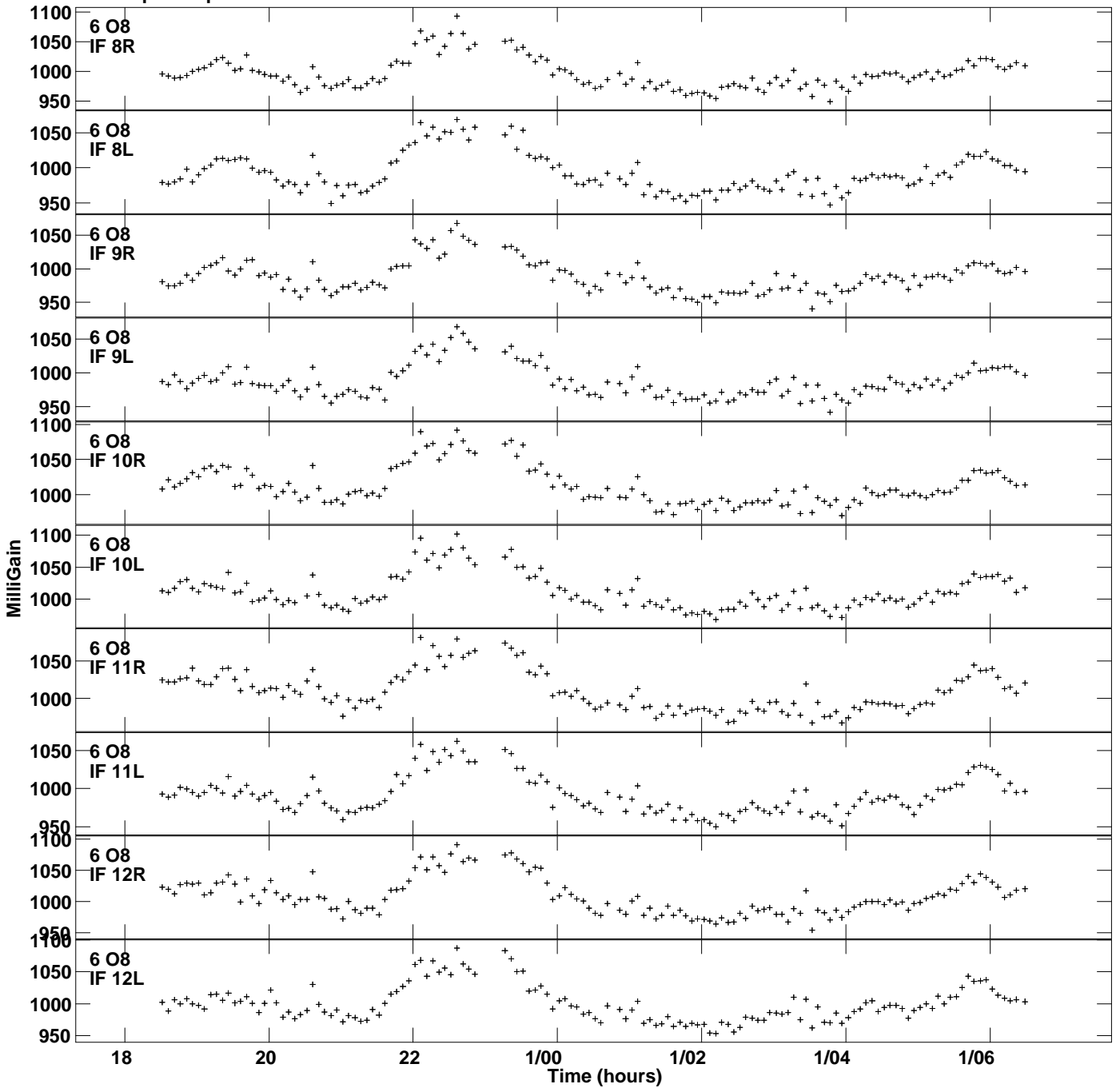
Plot file version 16 created 31-MAR-2023 16:32:32 Gain amp vs UTC time for J1128+5925.MULTI.1 SN 2 Rpol & Lpol IF 1 - 16
