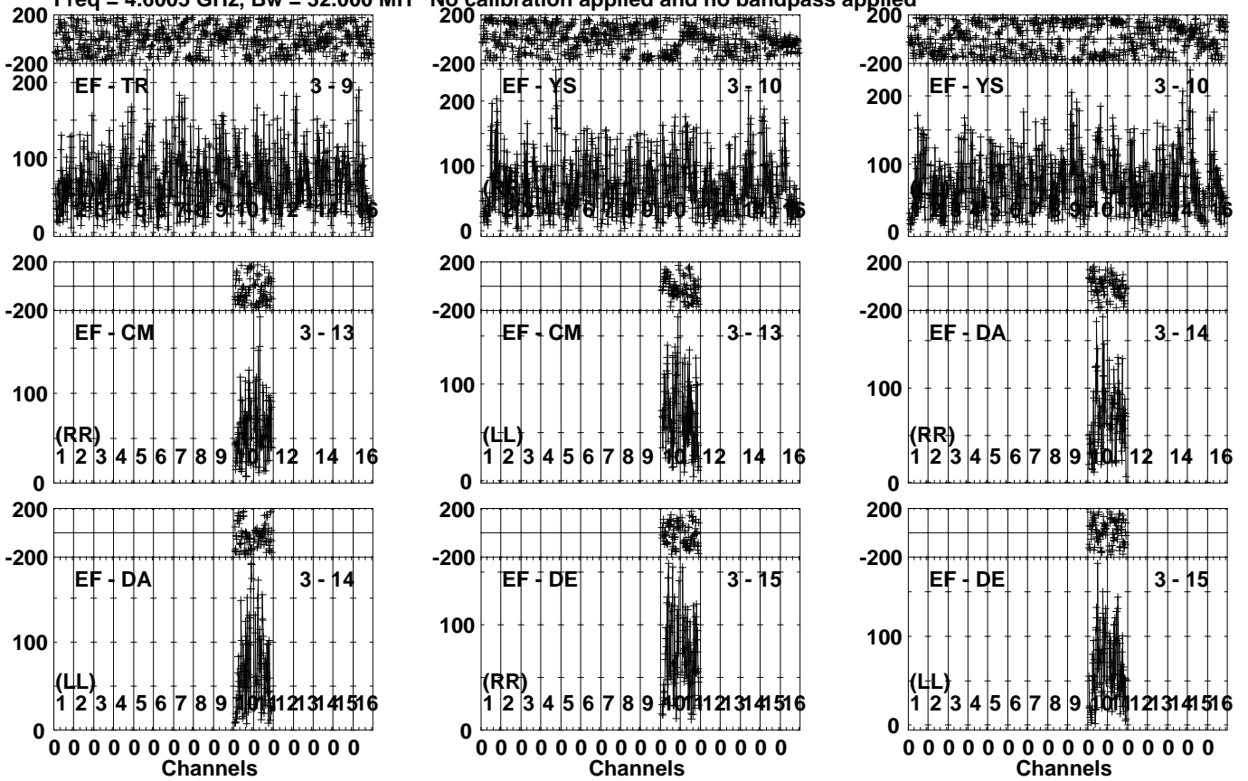
Lower frame: Micro Ampl Jy Top frame: Phas deg Vector averaged cross-power spectrum Several baselines displayed Timerange: 00/19:17:01 to 00/19:20:29
