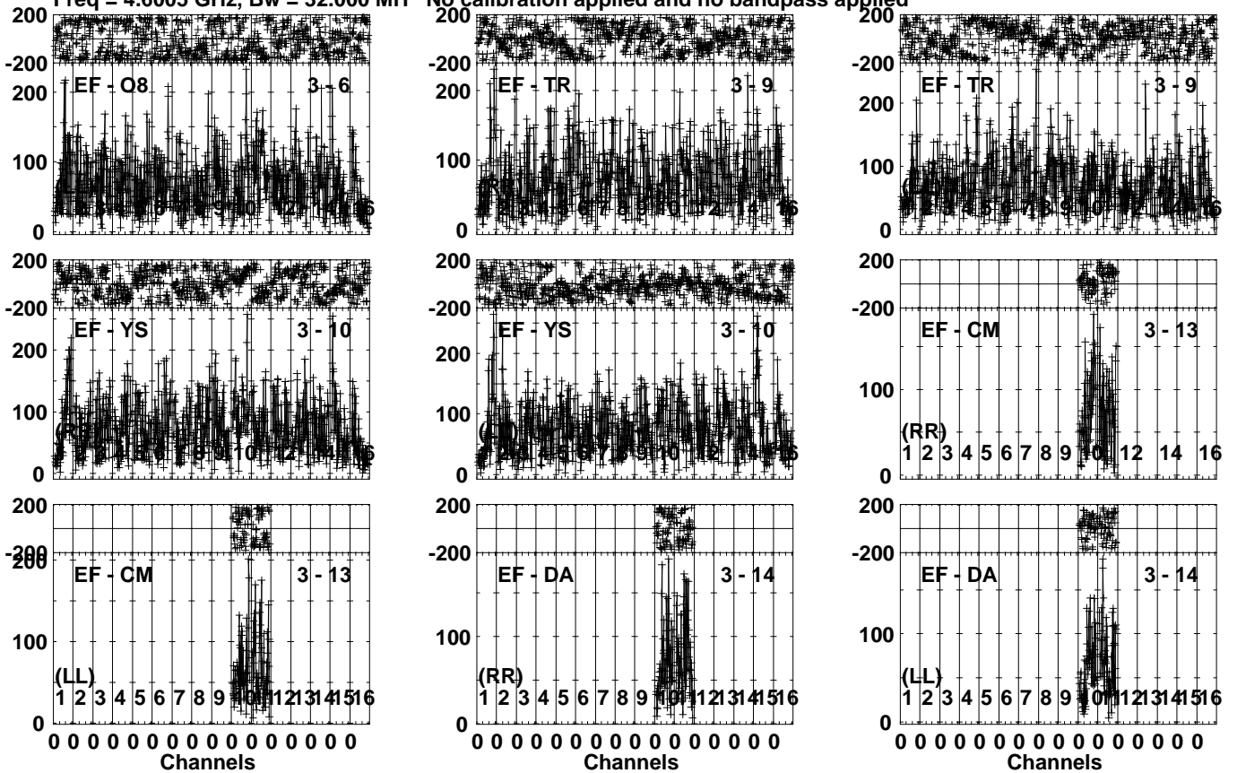
Lower frame: Micro Ampl Jy Top frame: Phas deg Vector averaged cross-power spectrum Several baselines displayed Timerange: 01/05:52:31 to 01/05:55:59
