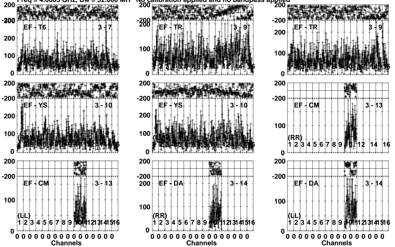
Lower frame: Micro Ampl Jy Top frame: Phas deg Vector averaged cross-power spectrum Several baselines displayed Timerange: 01/02:17:31 to 01/02:20:59
