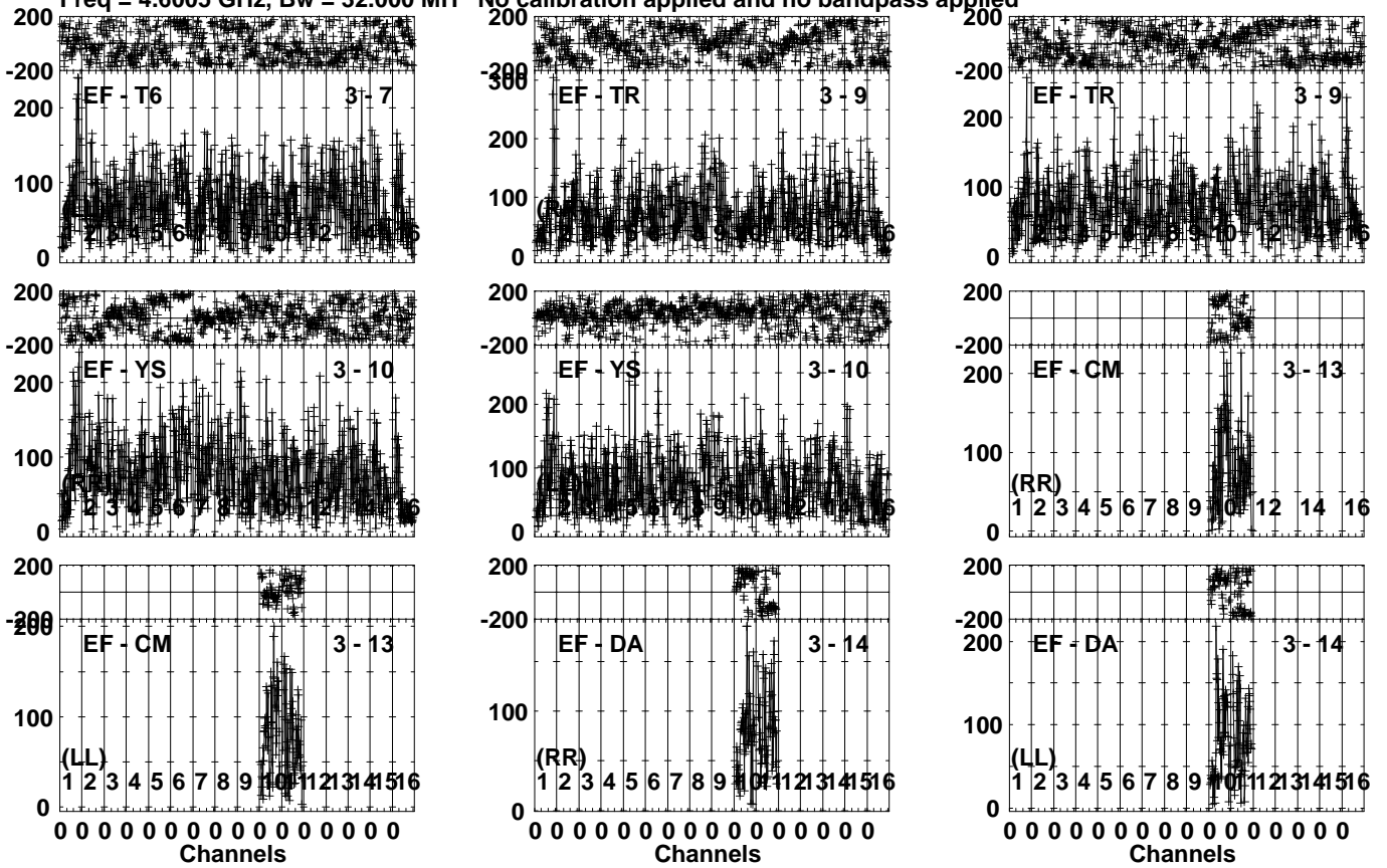
Lower frame: Micro Ampl Jy Top frame: Phas deg Vector averaged cross-power spectrum Several baselines displayed Timerange: 01/02:22:31 to 01/02:25:59
