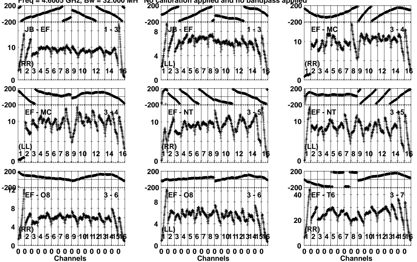
Lower frame: Milli Ampl Jy Top frame: Phas deg Vector averaged cross-power spectrum Several baselines displayed Timerange: 00/22:51:01 to 00/22:51:59
