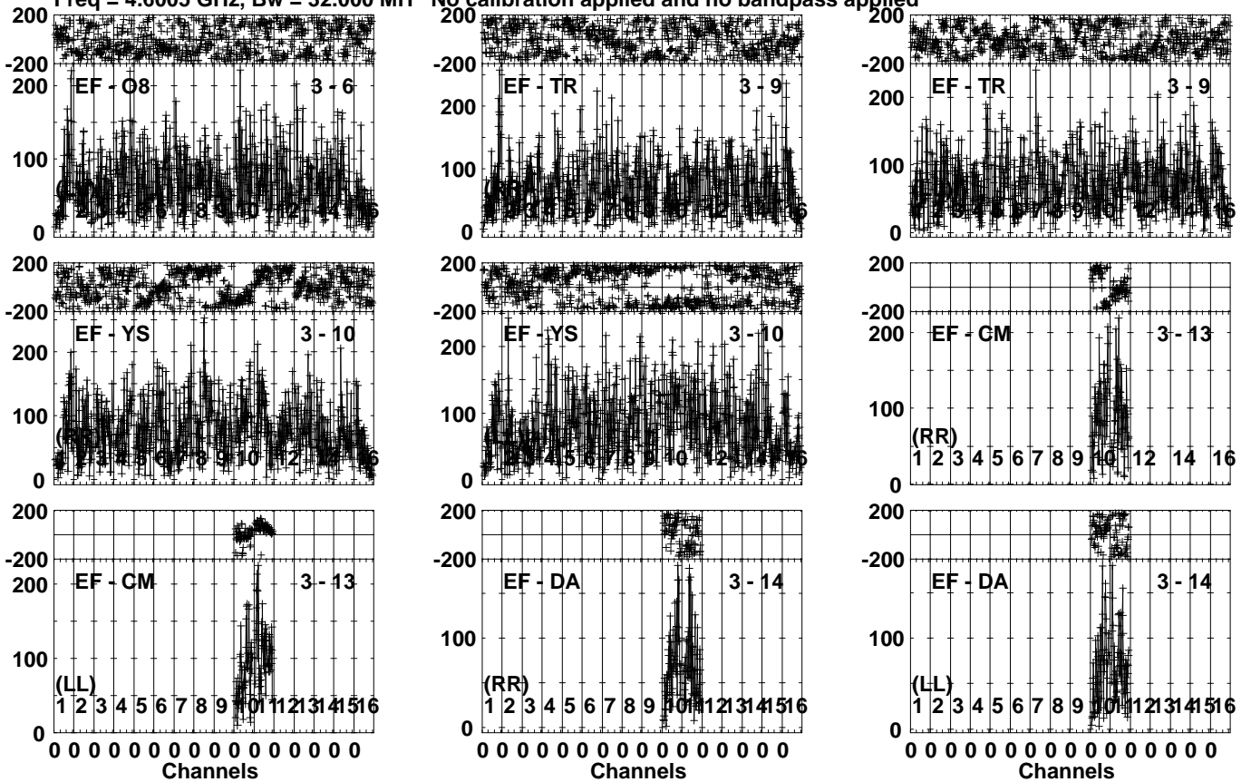
Lower frame: Micro Ampl Jy Top frame: Phas deg Vector averaged cross-power spectrum Several baselines displayed Timerange: 01/05:37:31 to 01/05:40:59
