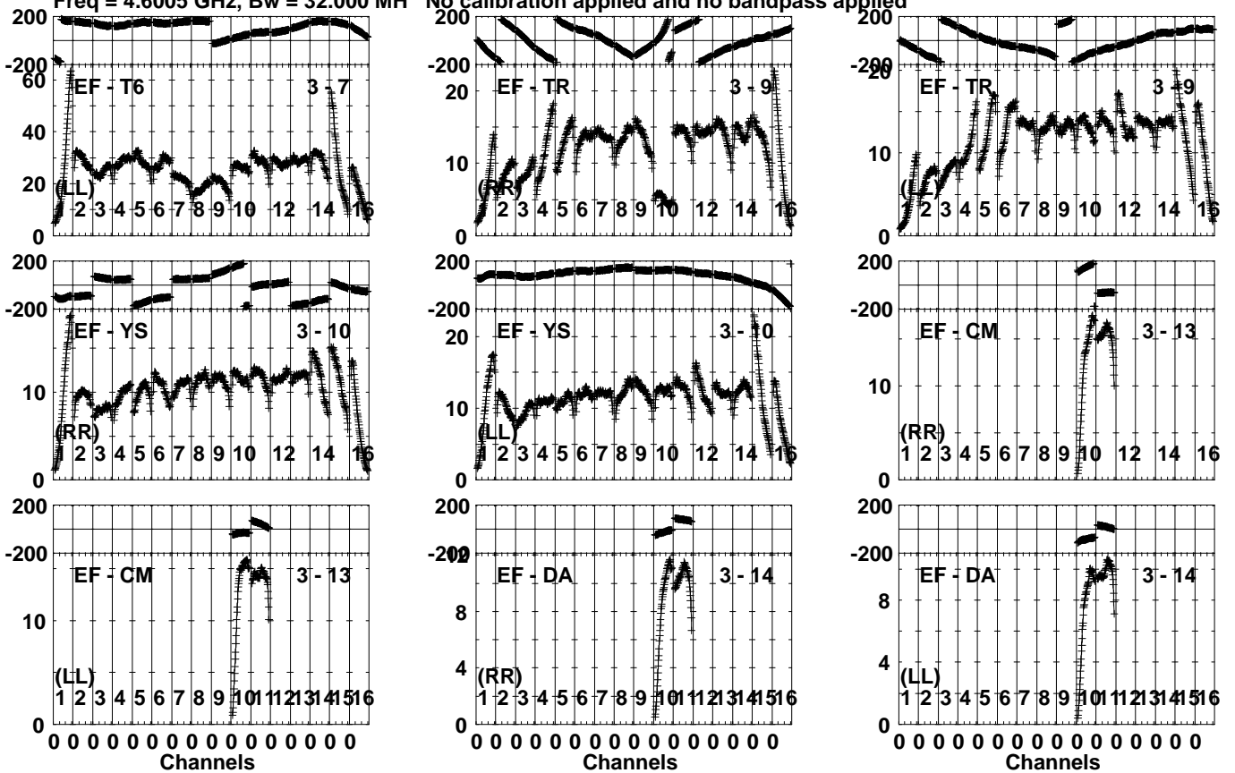
Lower frame: Milli Ampl Jy Top frame: Phas deg Vector averaged cross-power spectrum Several baselines displayed Timerange: 01/01:11:31 to 01/01:12:29
