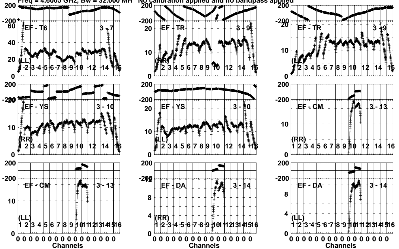
Lower frame: Milli Ampl Jy Top frame: Phas deg Vector averaged cross-power spectrum Several baselines displayed Timerange: 01/01:16:01 to 01/01:17:29
