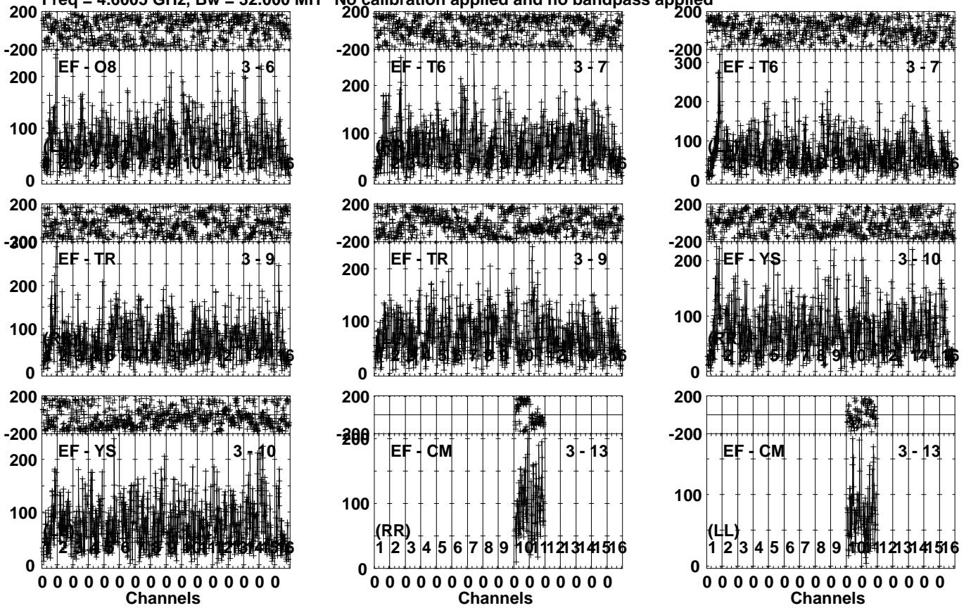
Lower frame: Micro Ampl Jy Top frame: Phas deg Vector averaged cross-power spectrum Several baselines displayed Timerange: 01/03:32:31 to 01/03:35:59
