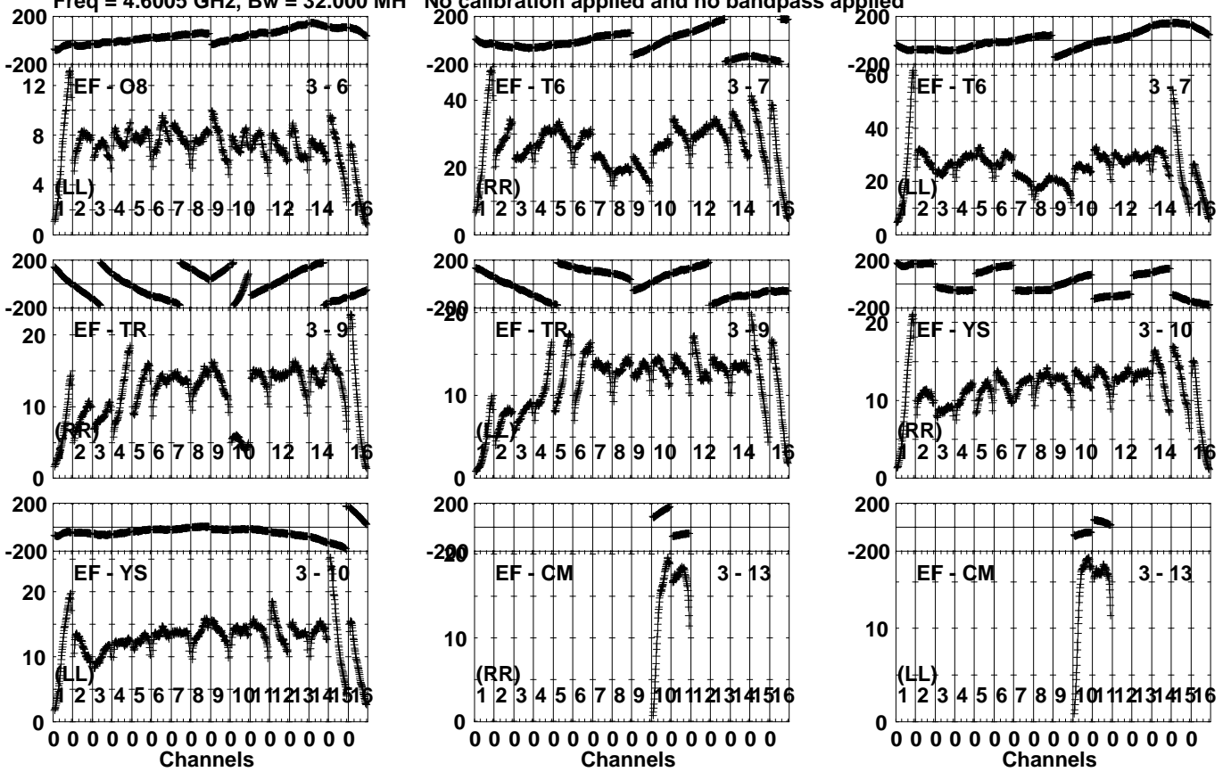
Lower frame: Milli Ampl Jy Top frame: Phas deg Vector averaged cross-power spectrum Several baselines displayed Timerange: 01/04:16:01 to 01/04:17:29
