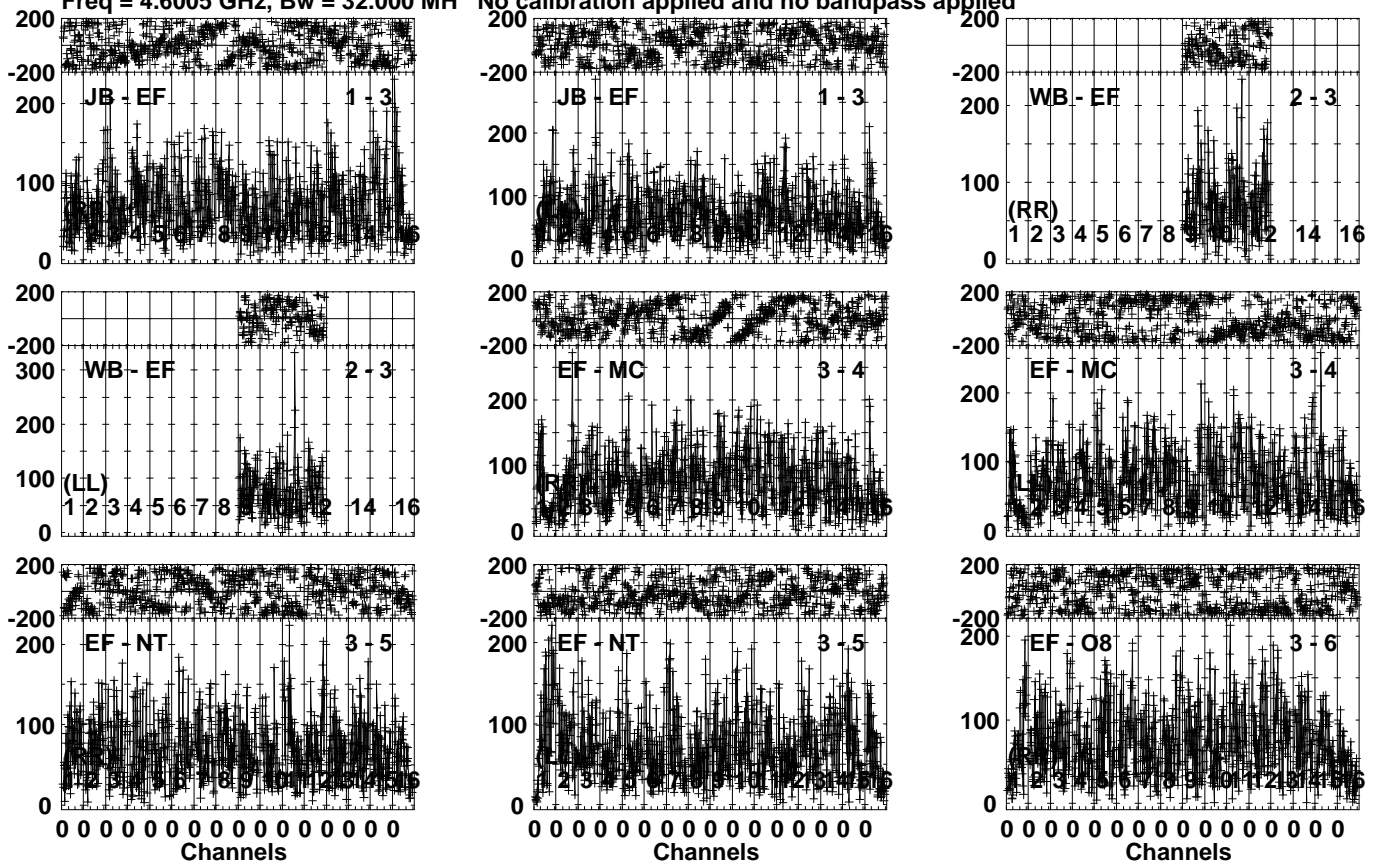
Lower frame: Micro Ampl Jy Top frame: Phas deg Vector averaged cross-power spectrum Several baselines displayed Timerange: 01/03:17:31 to 01/03:20:59
