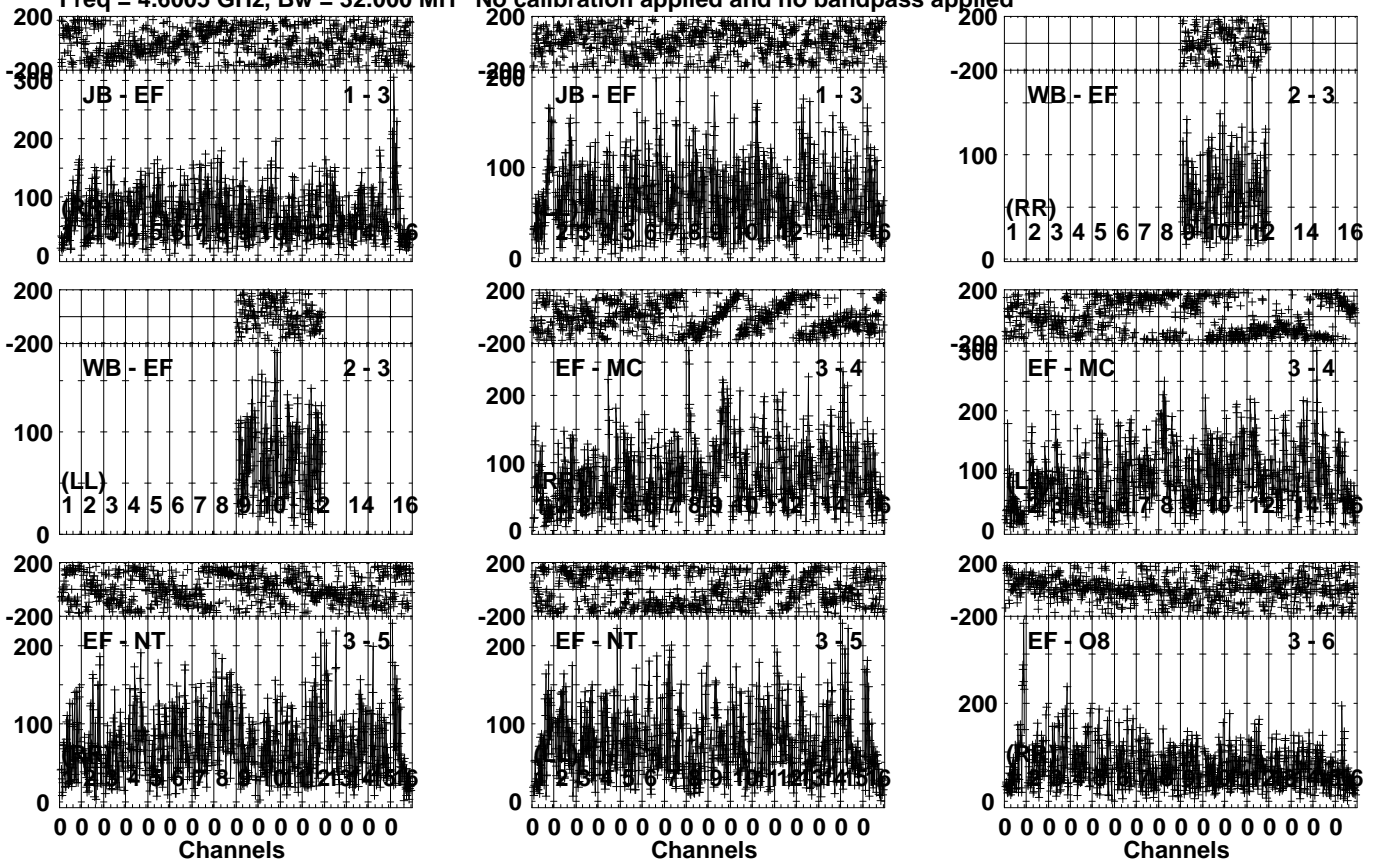
Lower frame: Micro Ampl Jy Top frame: Phas deg Vector averaged cross-power spectrum Several baselines displayed Timerange: 01/05:57:31 to 01/06:00:59
