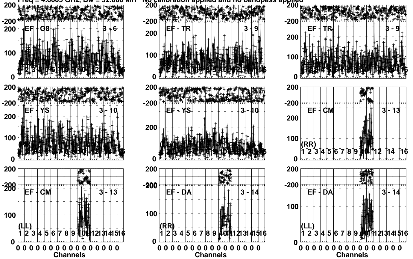
Lower frame: Micro Ampl Jy Top frame: Phas deg Vector averaged cross-power spectrum Several baselines displayed Timerange: 01/05:42:31 to 01/05:45:59
