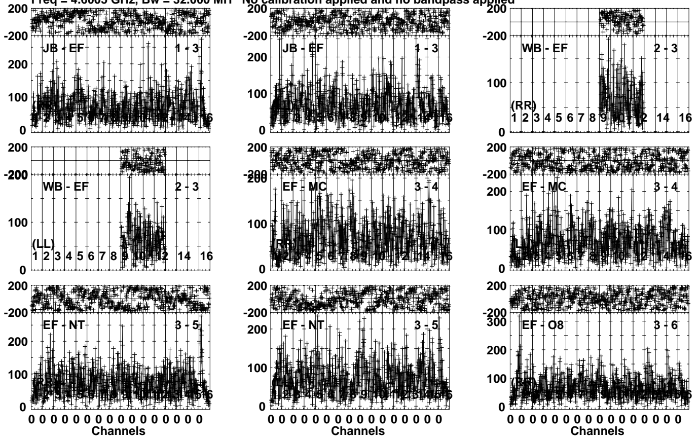
Lower frame: Micro Ampl Jy Top frame: Phas deg Vector averaged cross-power spectrum Several baselines displayed Timerange: 01/04:07:31 to 01/04:10:59
