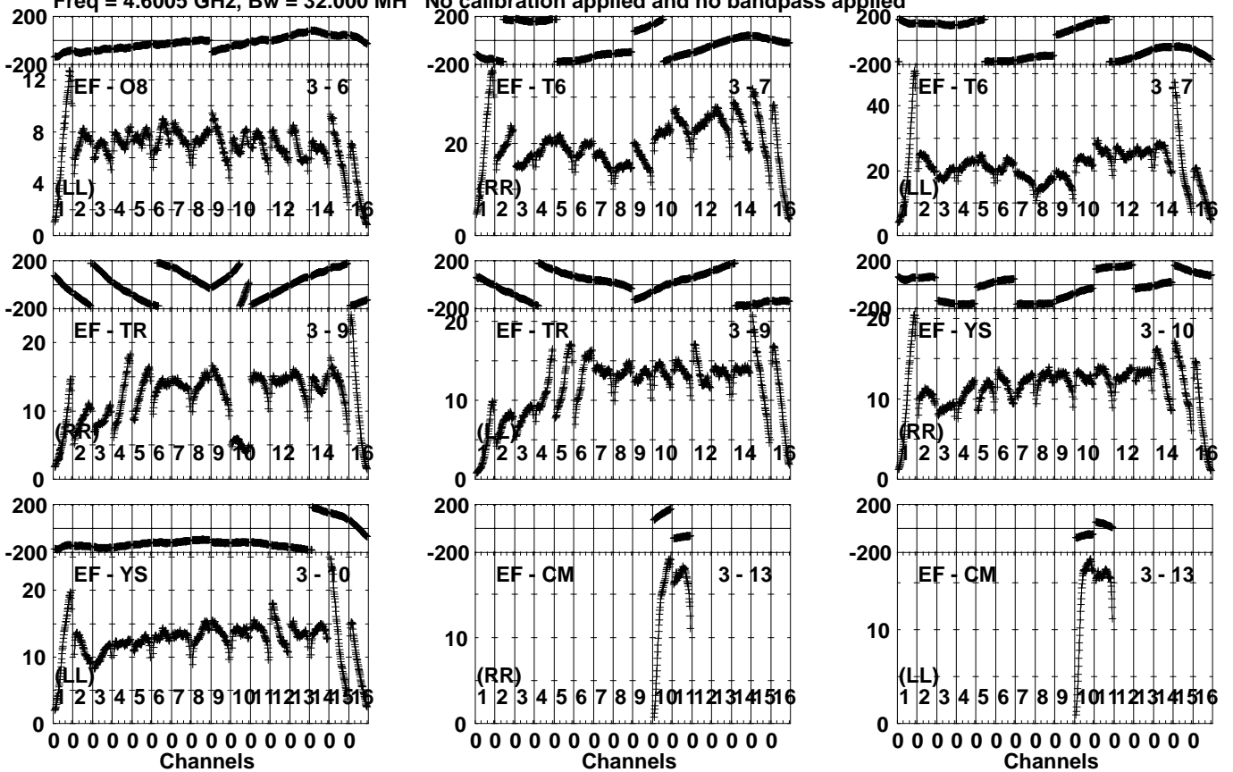
Lower frame: Milli Ampl Jy Top frame: Phas deg Vector averaged cross-power spectrum Several baselines displayed Timerange: 01/03:31:31 to 01/03:32:29
