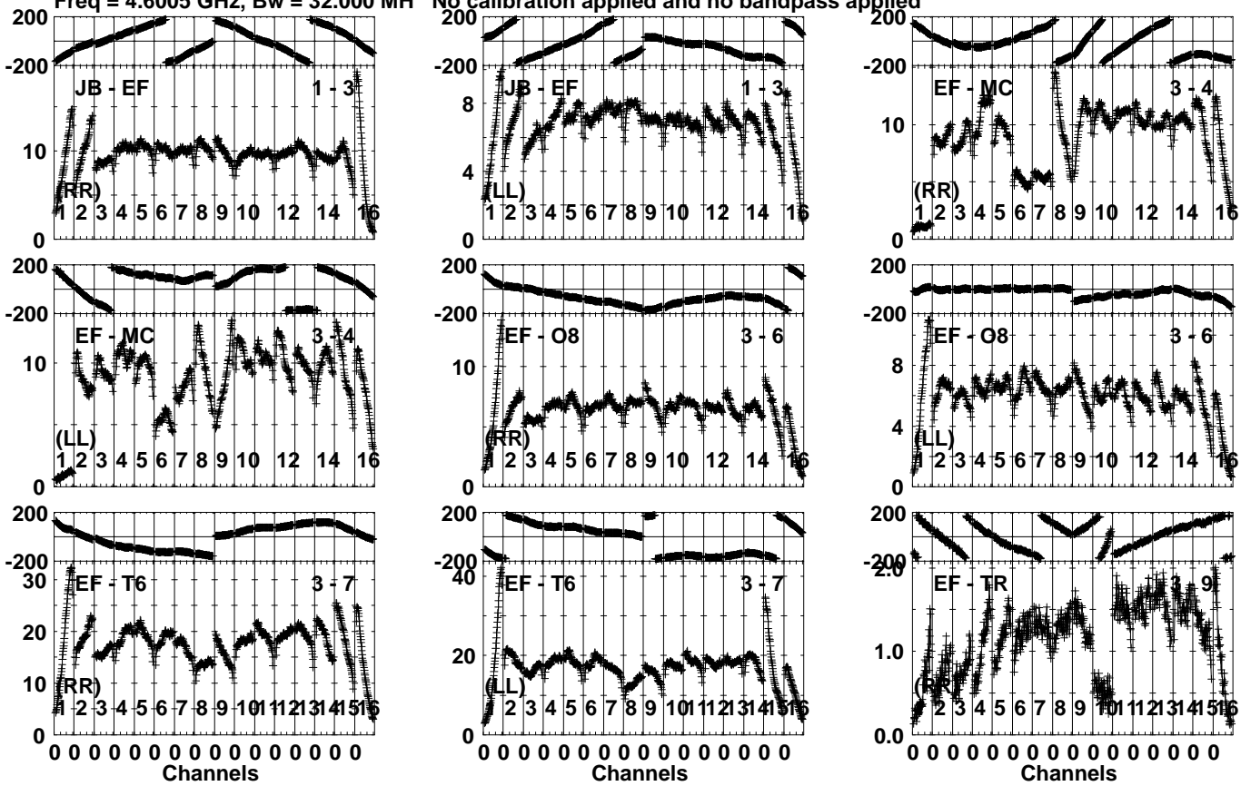
Lower frame: Milli Ampl Jy Top frame: Phas deg Vector averaged cross-power spectrum Several baselines displayed Timerange: 00/18:41:01 to 00/18:41:59
