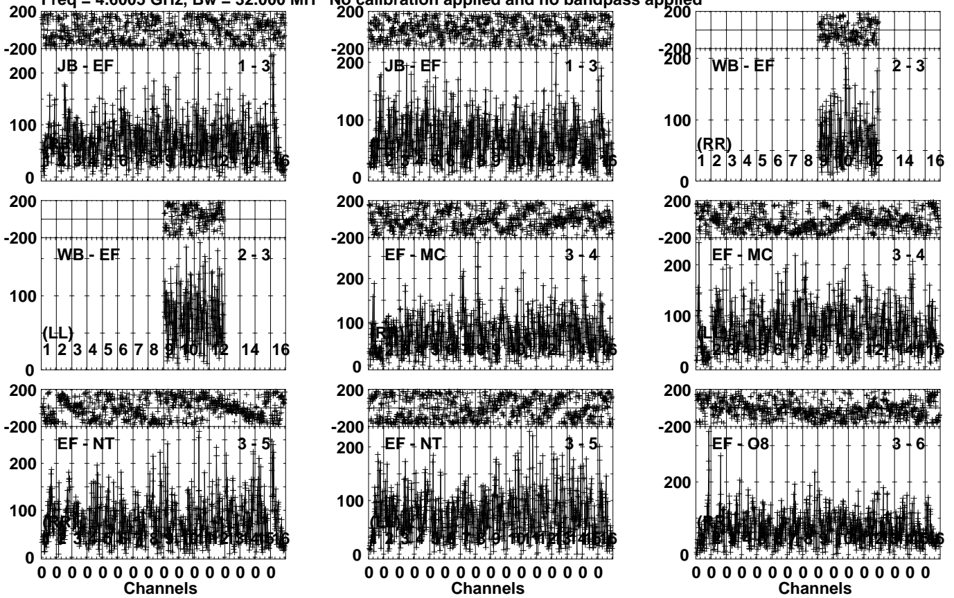
Lower frame: Micro Ampl Jy Top frame: Phas deg Vector averaged cross-power spectrum Several baselines displayed Timerange: 01/05:12:31 to 01/05:15:59
