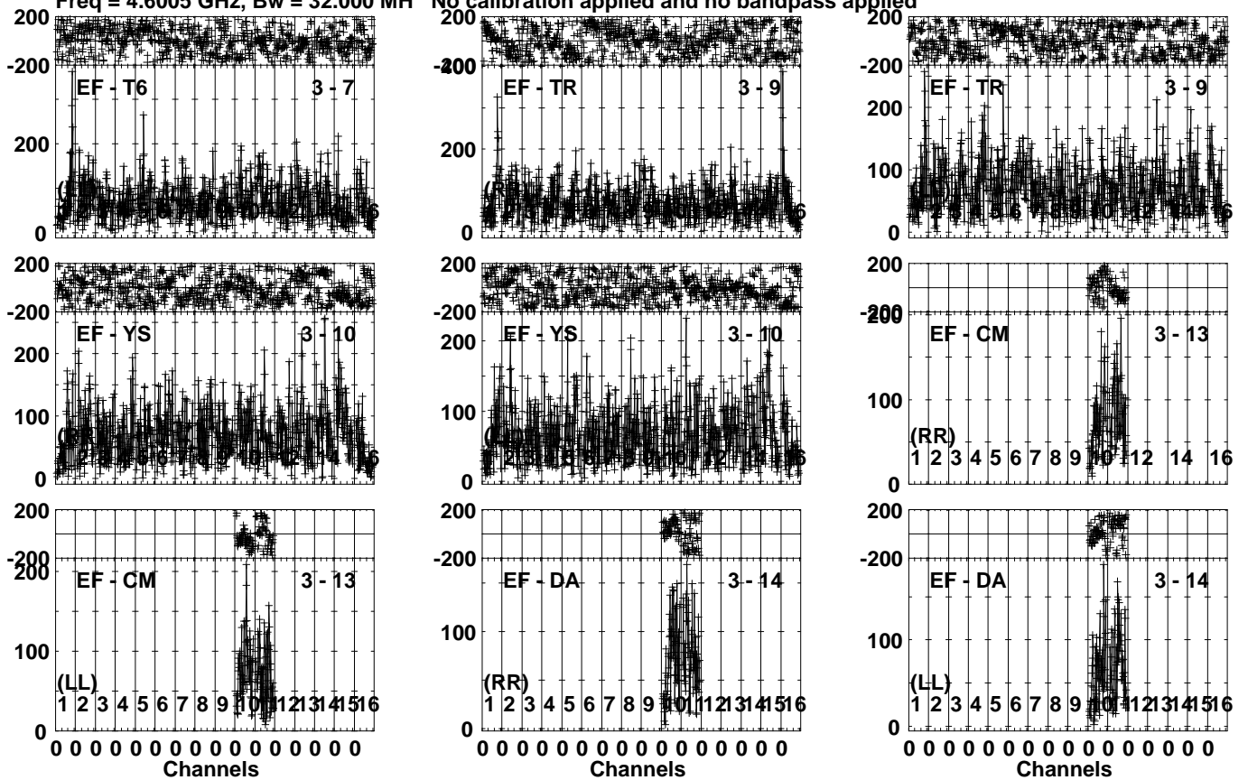
Lower frame: Micro Ampl Jy Top frame: Phas deg Vector averaged cross-power spectrum Several baselines displayed Timerange: 01/01:17:31 to 01/01:20:59
