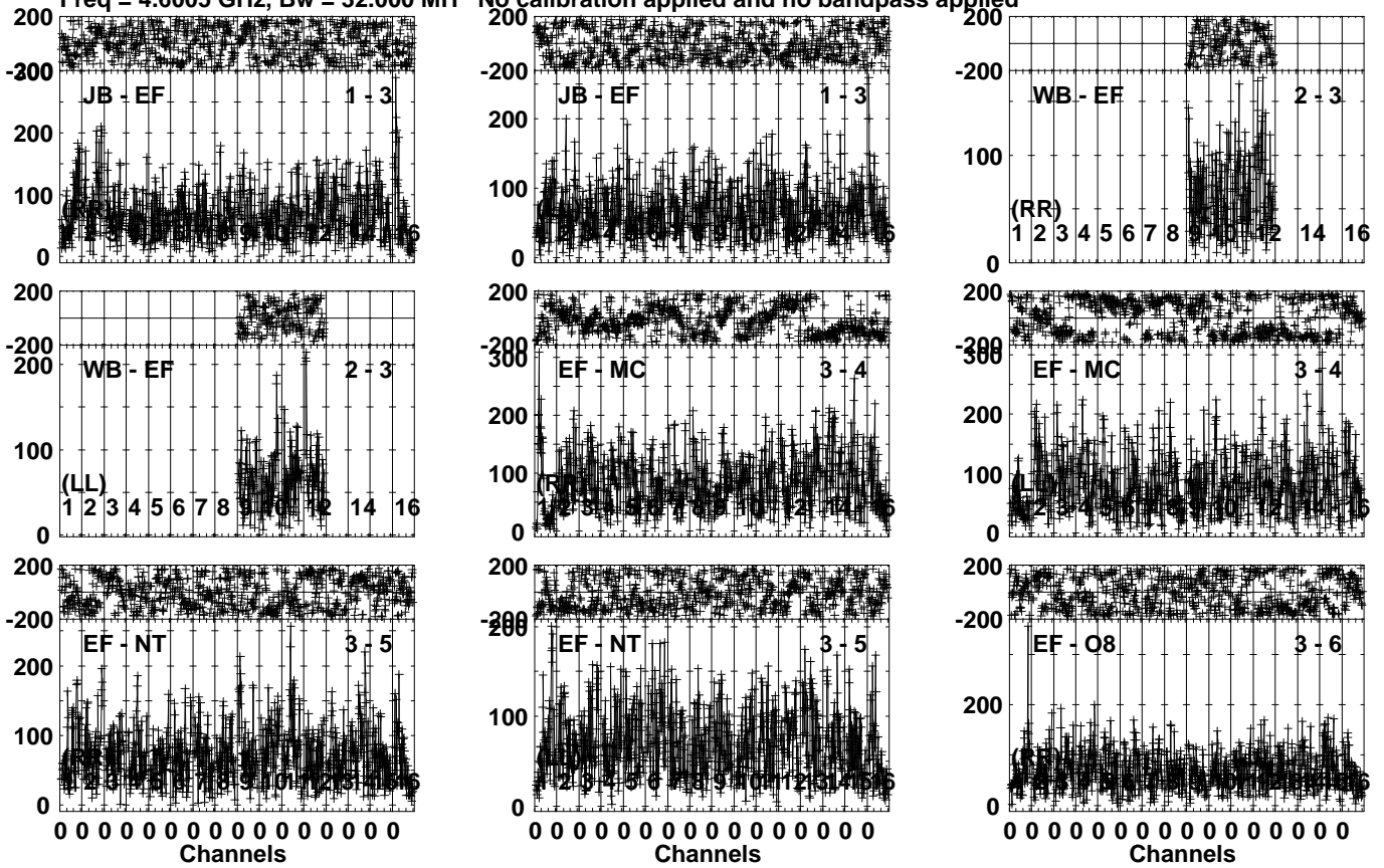
Lower frame: Micro Ampl Jy Top frame: Phas deg Vector averaged cross-power spectrum Several baselines displayed Timerange: 01/03:47:31 to 01/03:50:59
