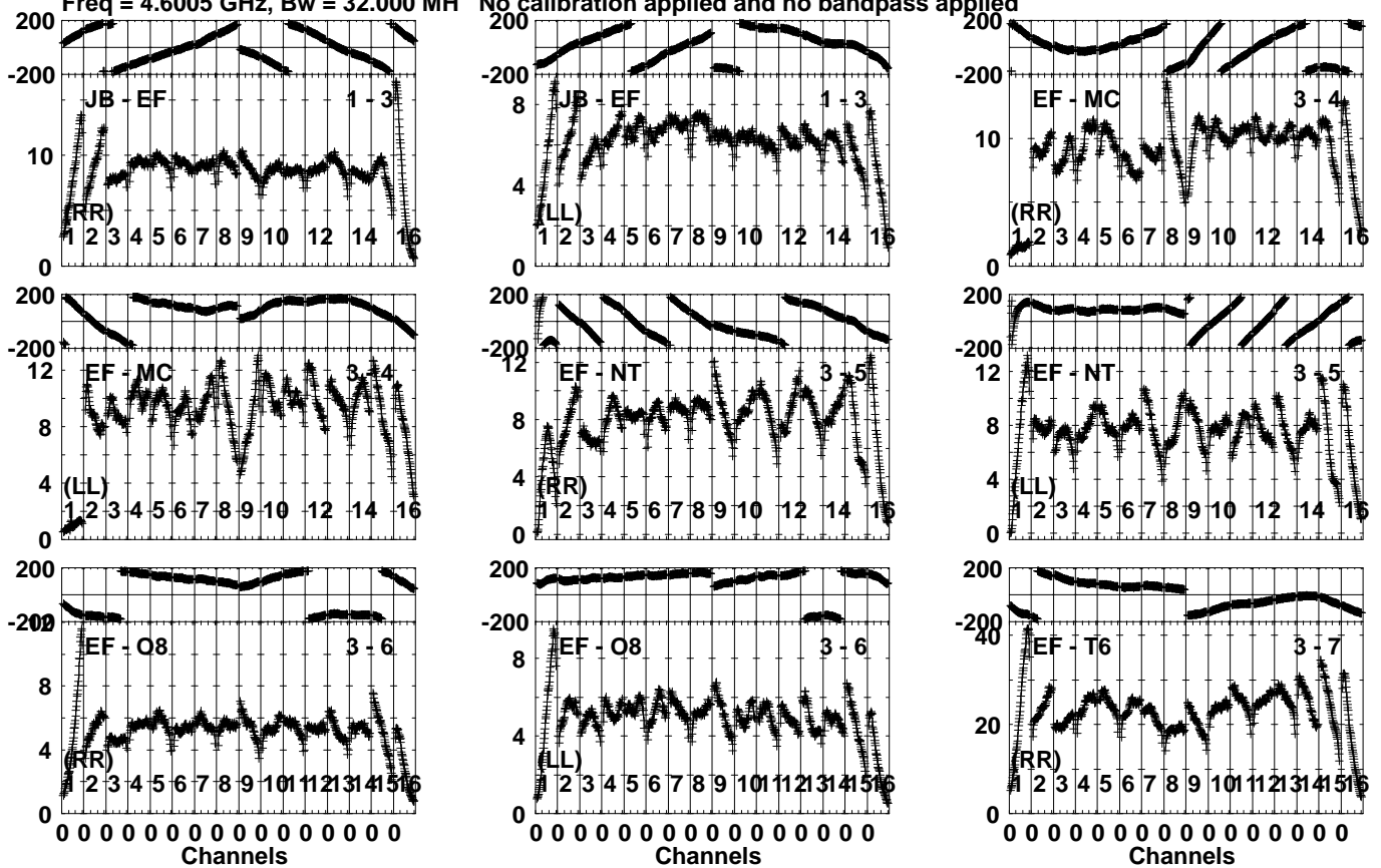
Lower frame: Milli Ampl Jy Top frame: Phas deg Vector averaged cross-power spectrum Several baselines displayed Timerange: 00/22:11:01 to 00/22:11:59
