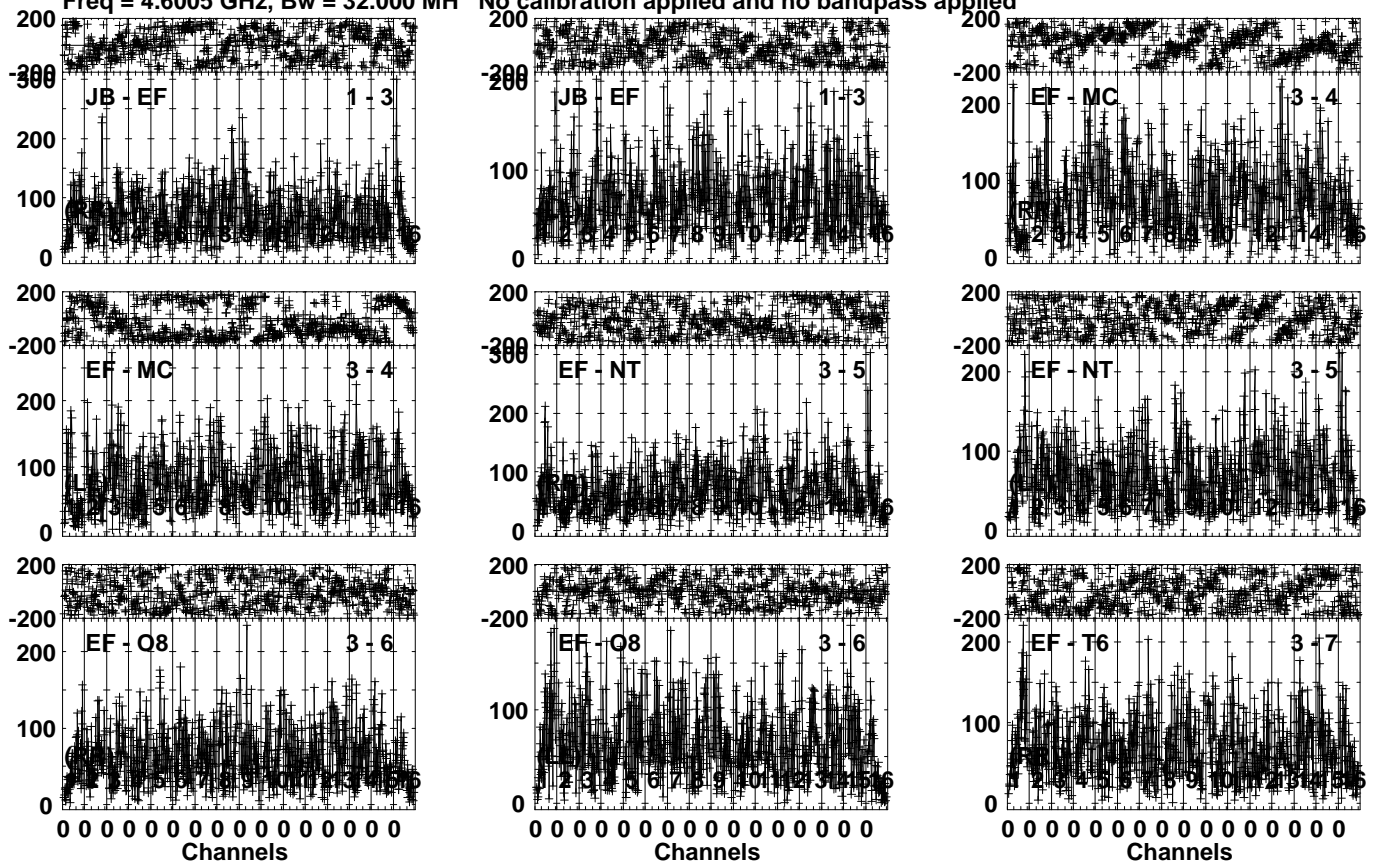
Lower frame: Micro Ampl Jy Top frame: Phas deg Vector averaged cross-power spectrum Several baselines displayed Timerange: 00/23:27:01 to 00/23:30:29
