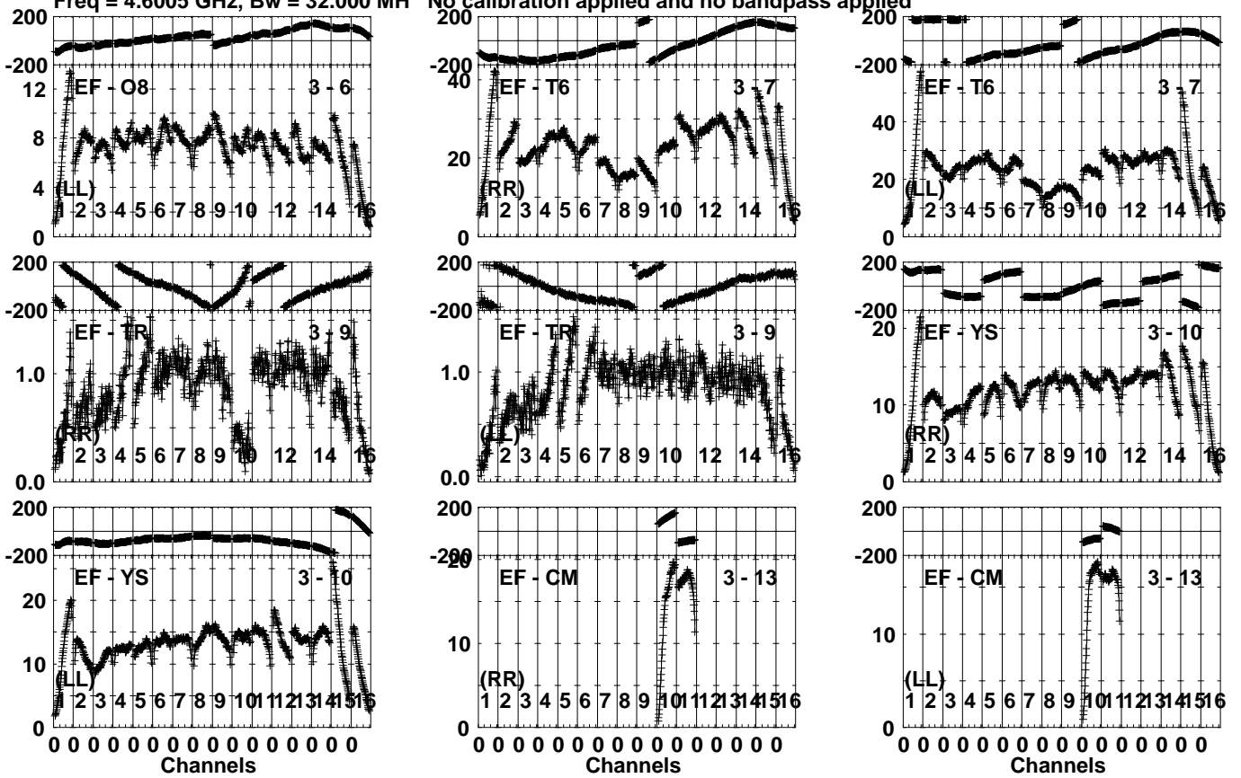
Lower frame: Milli Ampl Jy Top frame: Phas deg Vector averaged cross-power spectrum Several baselines displayed Timerange: 01/04:46:01 to 01/04:47:29
