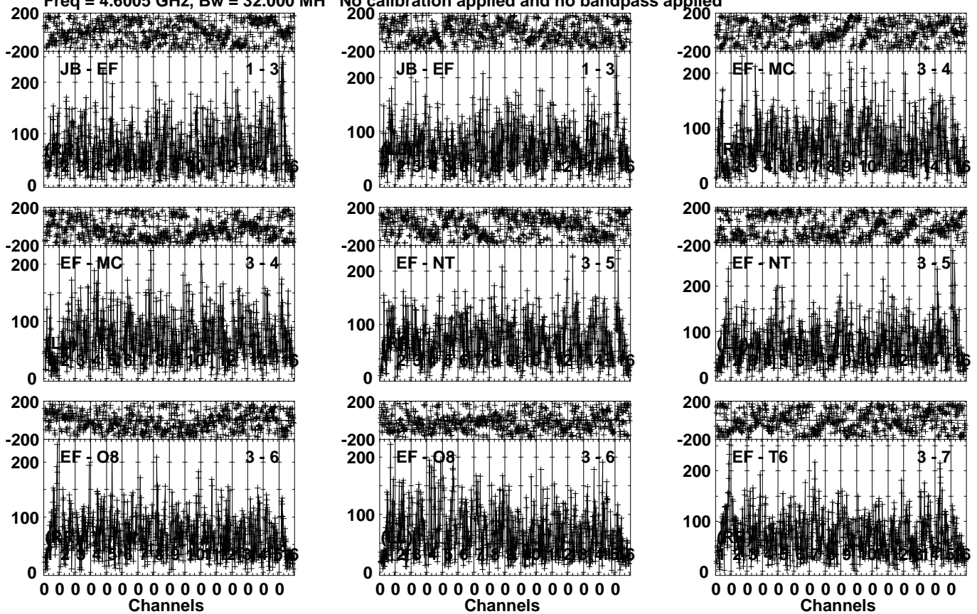
Lower frame: Micro Ampl Jy Top frame: Phas deg Vector averaged cross-power spectrum Several baselines displayed Timerange: 00/22:22:01 to 00/22:25:29
