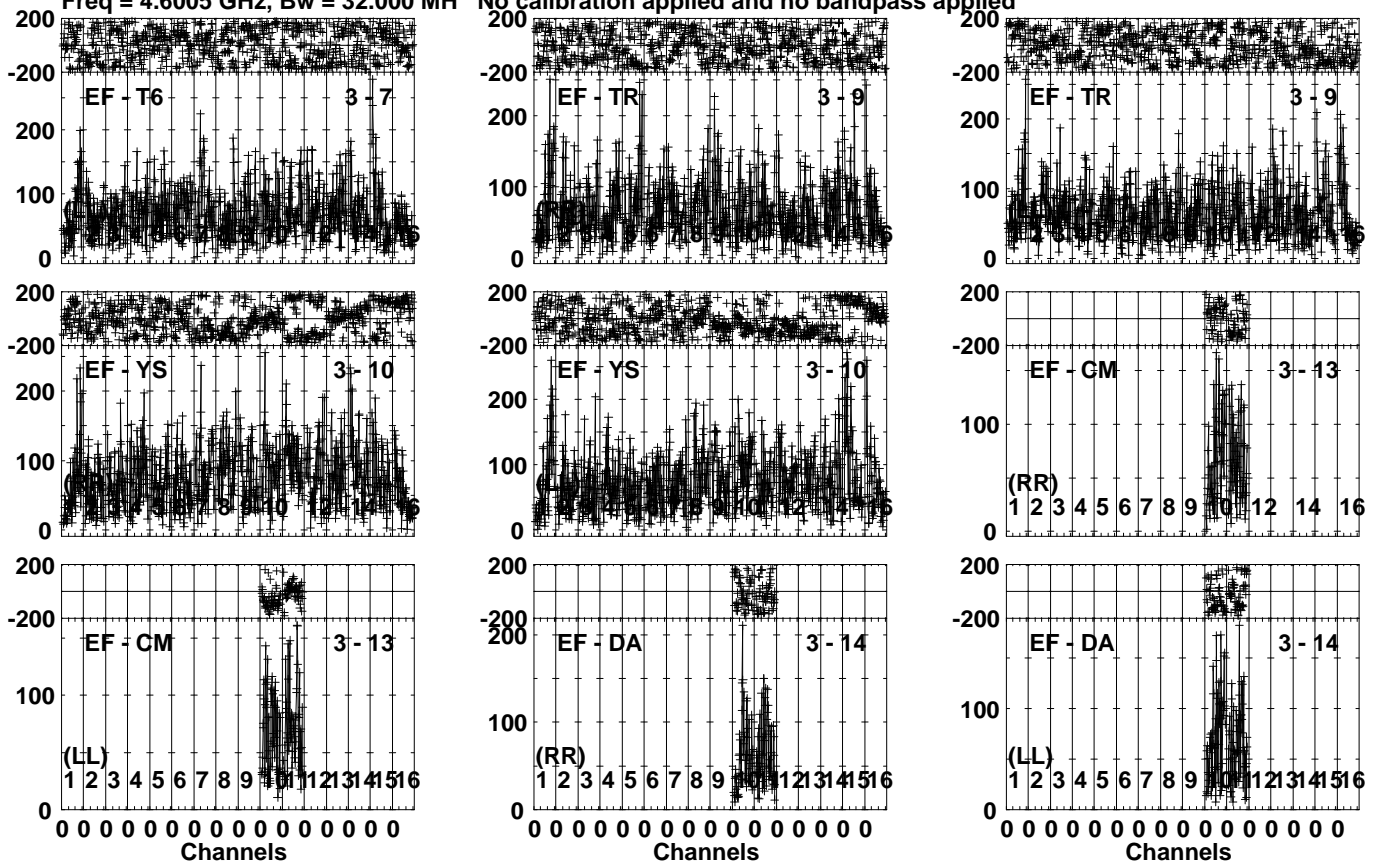
Lower frame: Micro Ampl Jy Top frame: Phas deg Vector averaged cross-power spectrum Several baselines displayed Timerange: 01/02:07:31 to 01/02:10:59
