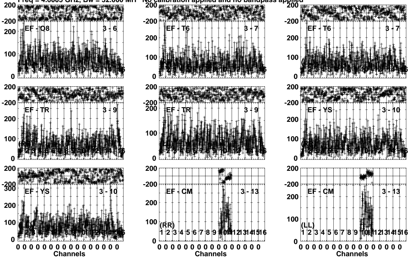
Lower frame: Micro Ampl Jy Top frame: Phas deg Vector averaged cross-power spectrum Several baselines displayed Timerange: 01/05:07:31 to 01/05:10:59
