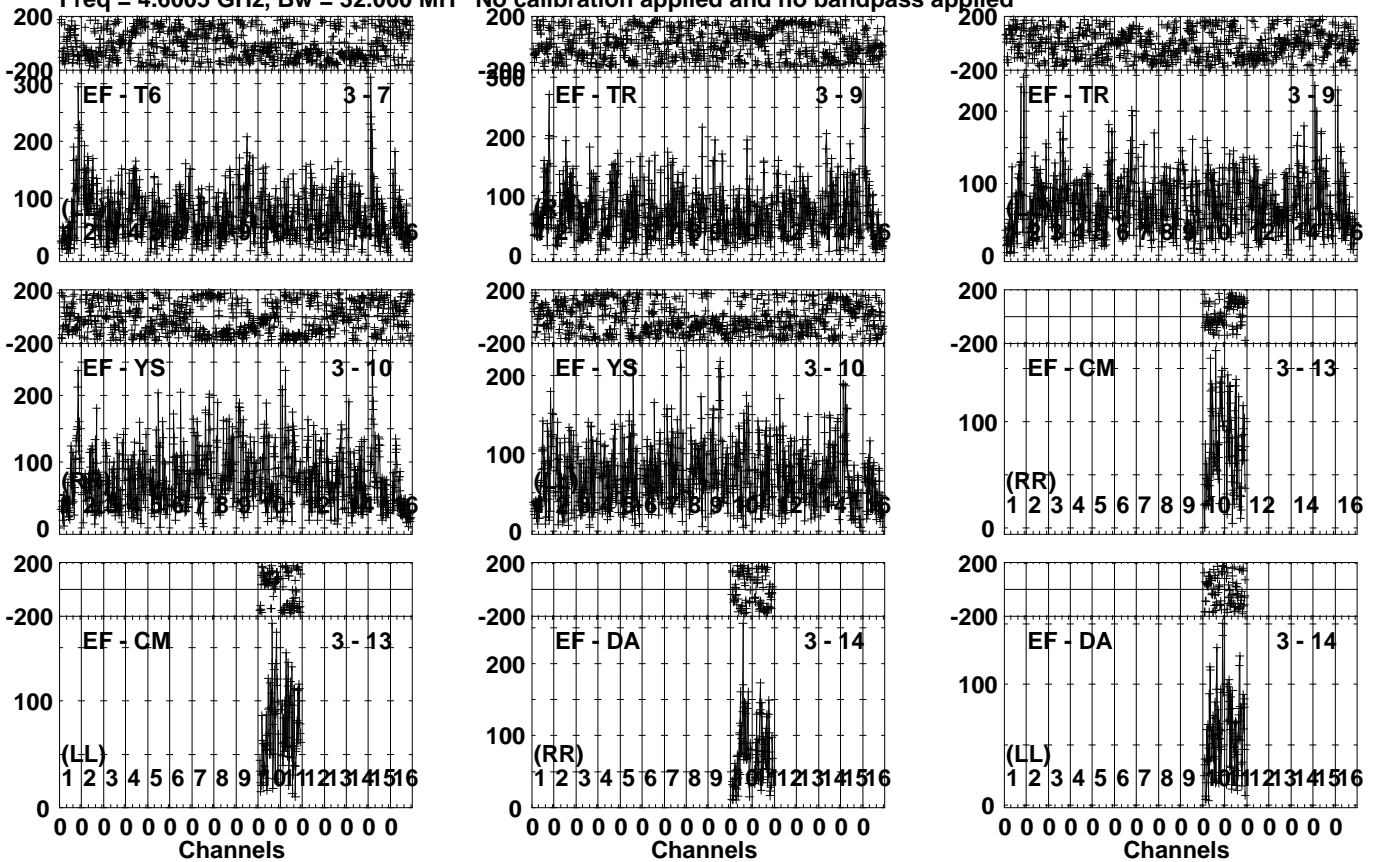
Lower frame: Micro Ampl Jy Top frame: Phas deg Vector averaged cross-power spectrum Several baselines displayed Timerange: 01/02:02:31 to 01/02:05:59
