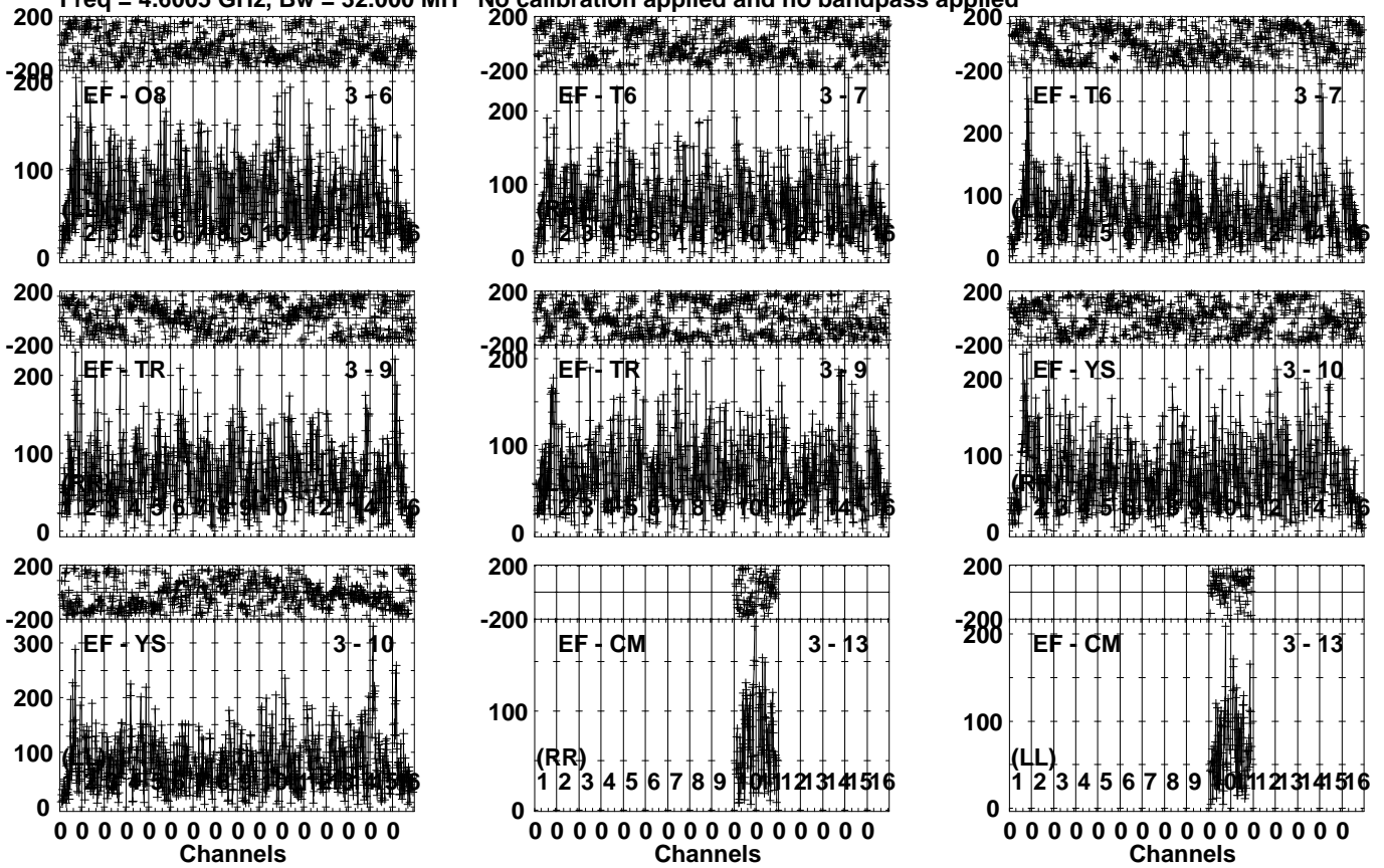
Lower frame: Micro Ampl Jy Top frame: Phas deg Vector averaged cross-power spectrum Several baselines displayed Timerange: 01/04:47:31 to 01/04:50:59
