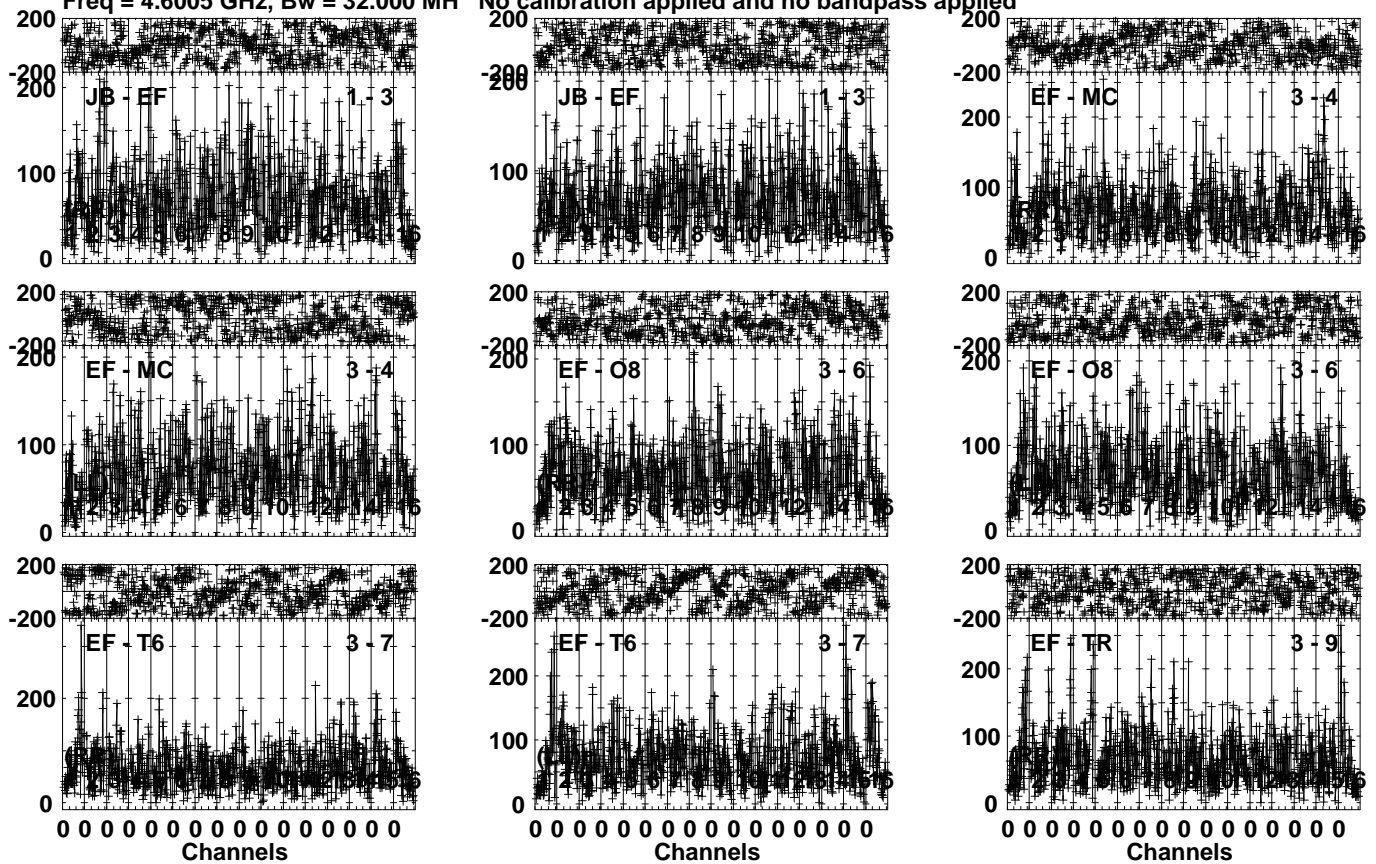
Lower frame: Micro Ampl Jy Top frame: Phas deg Vector averaged cross-power spectrum Several baselines displayed Timerange: 00/20:57:01 to 00/21:00:29
