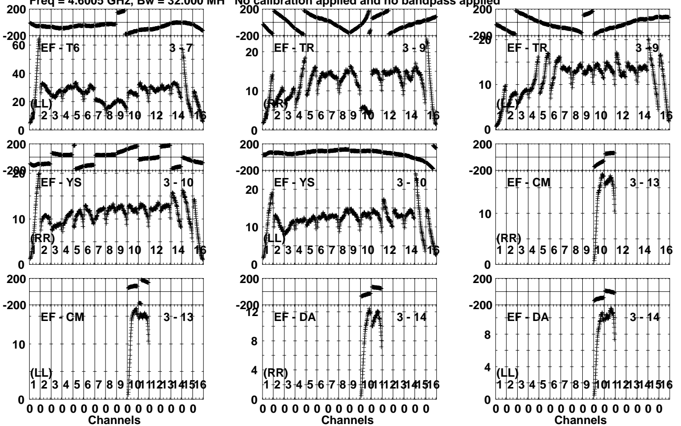
Lower frame: Milli Ampl Jy Top frame: Phas deg Vector averaged cross-power spectrum Several baselines displayed Timerange: 01/02:11:31 to 01/02:12:29
