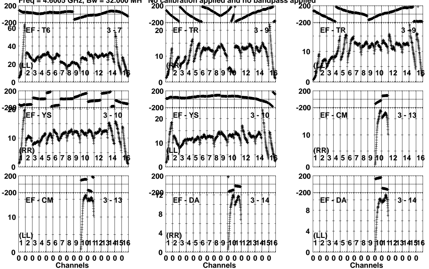
Lower frame: Milli Ampl Jy Top frame: Phas deg Vector averaged cross-power spectrum Several baselines displayed Timerange: 01/01:46:03 to 01/01:47:29
