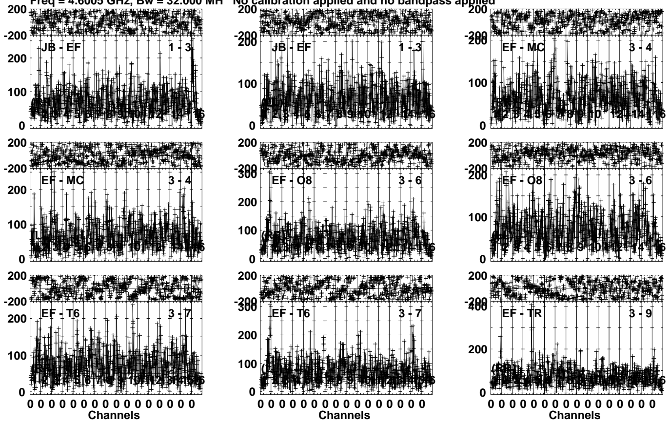
Lower frame: Micro Ampl Jy Top frame: Phas deg Vector averaged cross-power spectrum Several baselines displayed Timerange: 00/19:37:01 to 00/19:40:29
