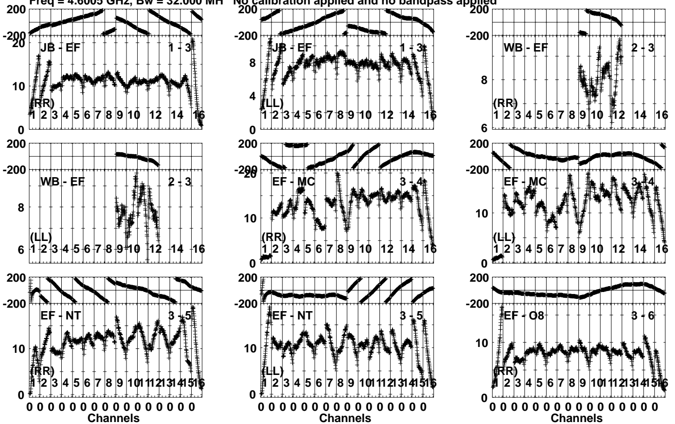
Lower frame: Milli Ampl Jy Top frame: Phas deg Vector averaged cross-power spectrum Several baselines displayed Timerange: 01/06:21:31 to 01/06:22:29
