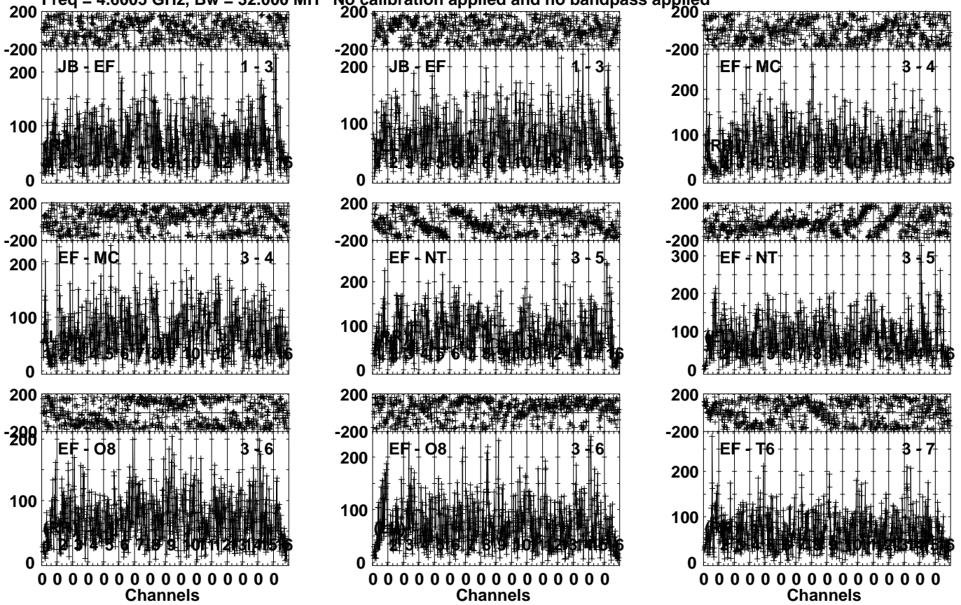
Lower frame: Micro Ampl Jy Top frame: Phas deg Vector averaged cross-power spectrum Several baselines displayed Timerange: 01/02:47:31 to 01/02:50:59
