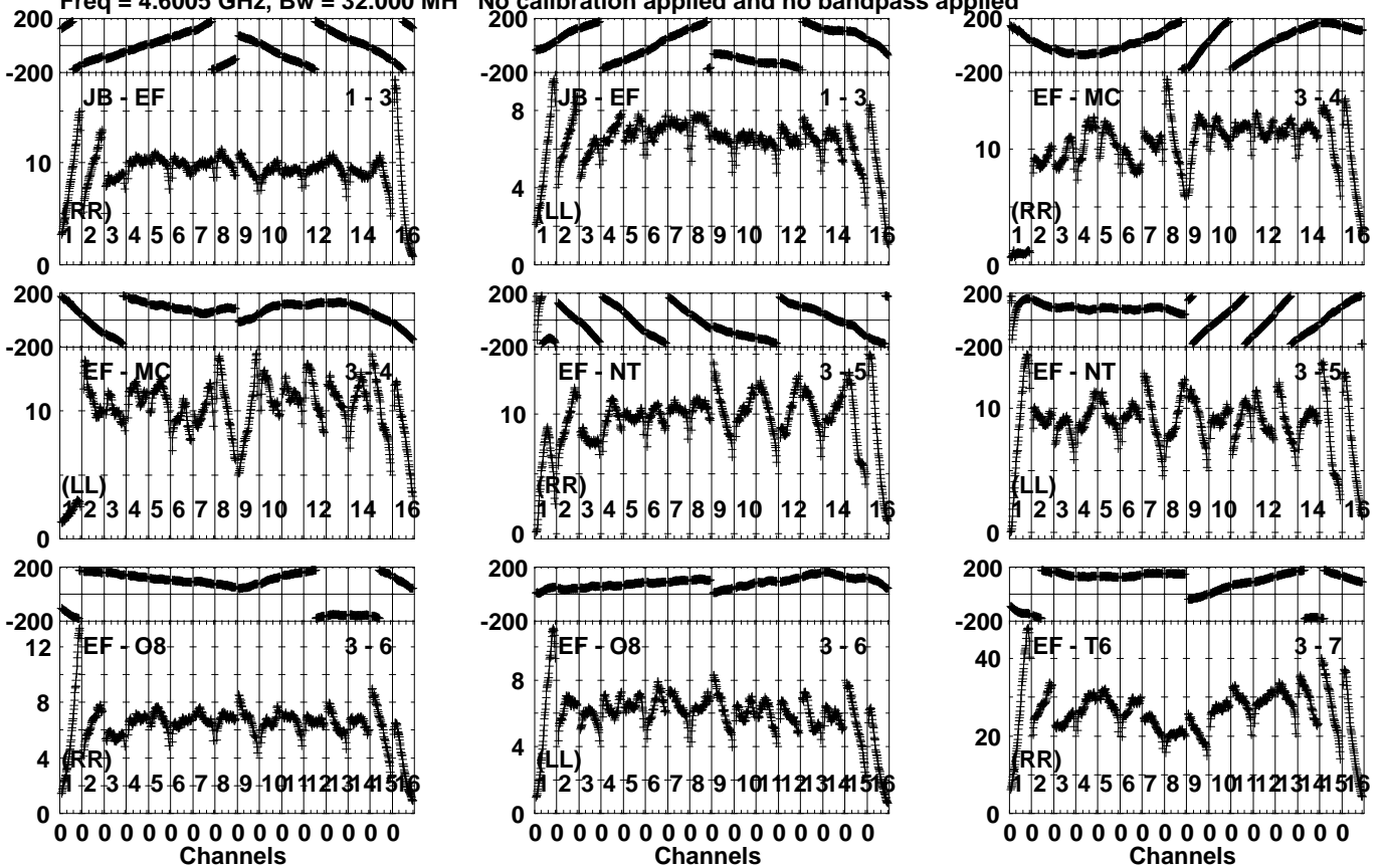
Lower frame: Milli Ampl Jy Top frame: Phas deg Vector averaged cross-power spectrum Several baselines displayed Timerange: 01/00:01:01 to 01/00:01:59
