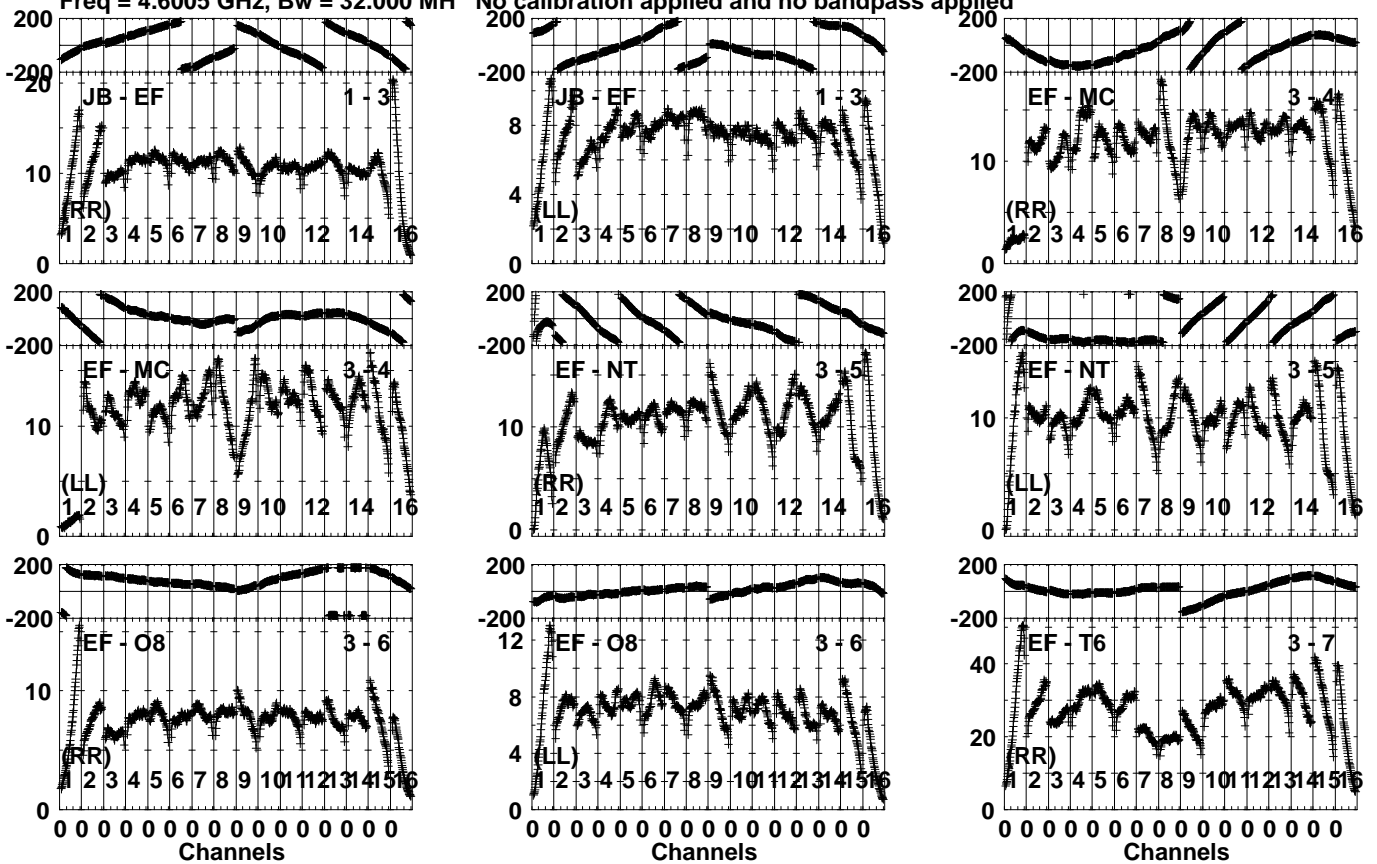
Lower frame: Milli Ampl Jy Top frame: Phas deg Vector averaged cross-power spectrum Several baselines displayed Timerange: 01/02:01:31 to 01/02:02:29
