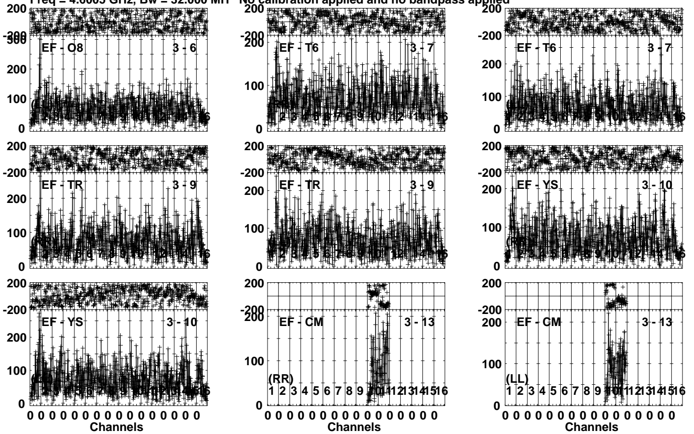
Lower frame: Micro Ampl Jy Top frame: Phas deg Vector averaged cross-power spectrum Several baselines displayed Timerange: 01/04:57:31 to 01/05:00:59
