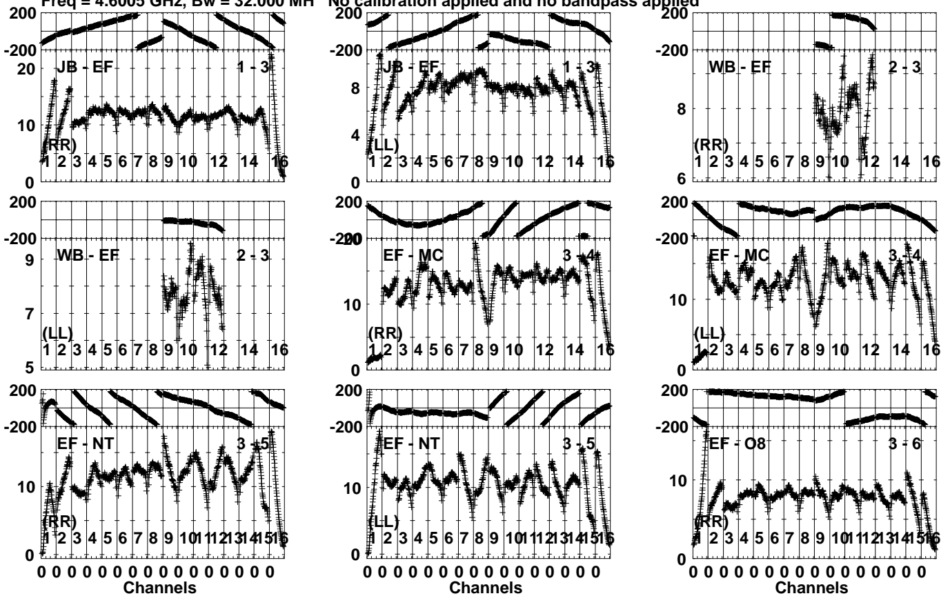
Lower frame: Milli Ampl Jy Top frame: Phas deg Vector averaged cross-power spectrum Several baselines displayed Timerange: 01/04:01:31 to 01/04:02:29
