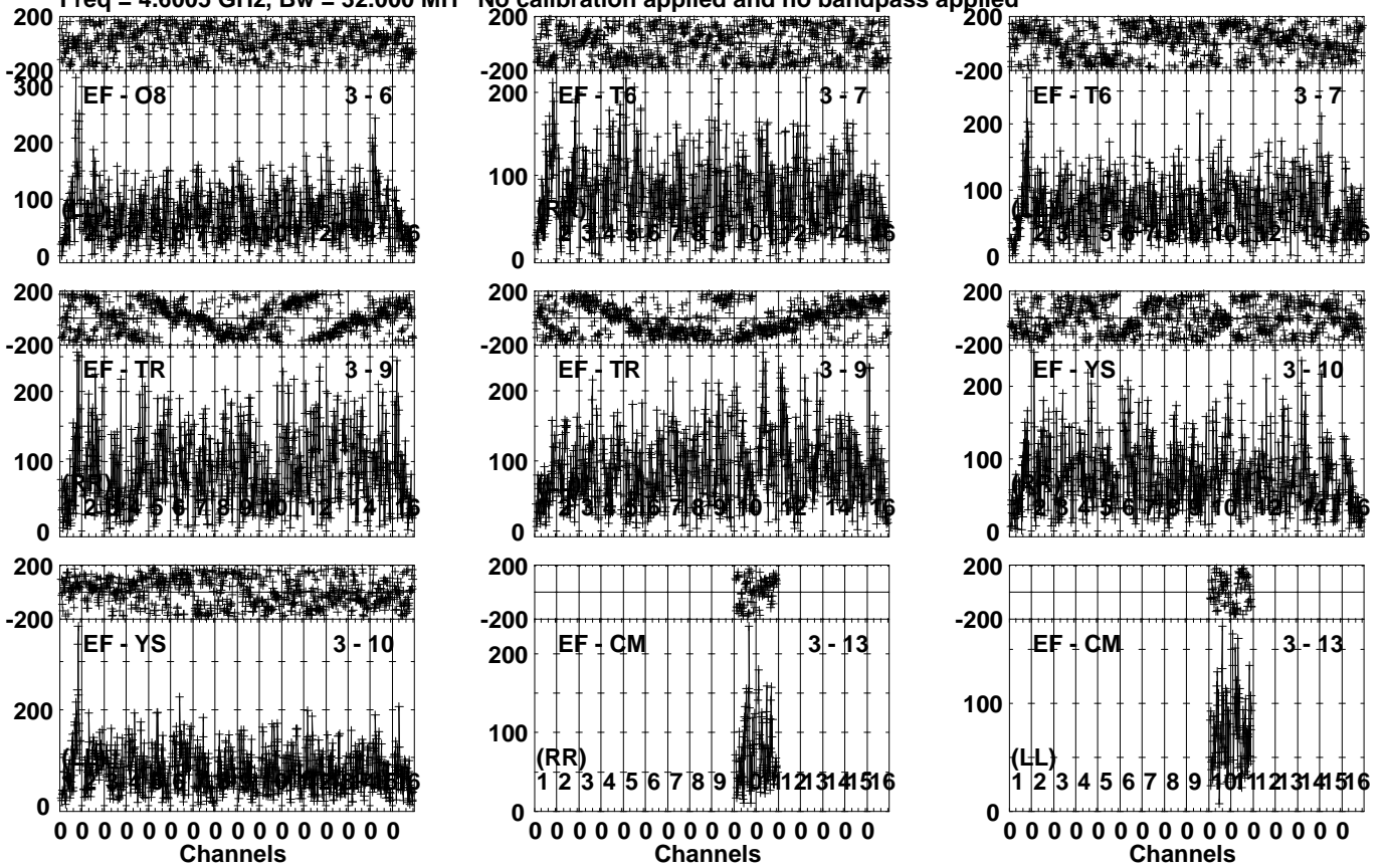
Lower frame: Micro Ampl Jy Top frame: Phas deg Vector averaged cross-power spectrum Several baselines displayed Timerange: 01/03:22:31 to 01/03:25:59
