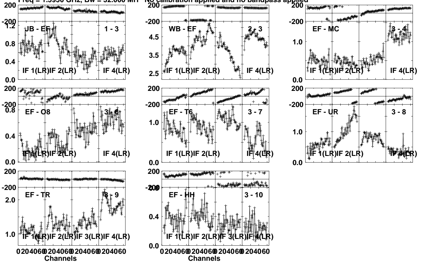
Lower frame: Milli Ampl Jy Top frame: Phas deg Vector averaged cross-power spectrum Several baselines displayed Timerange: 00/02:47:16 to 00/02:48:14
