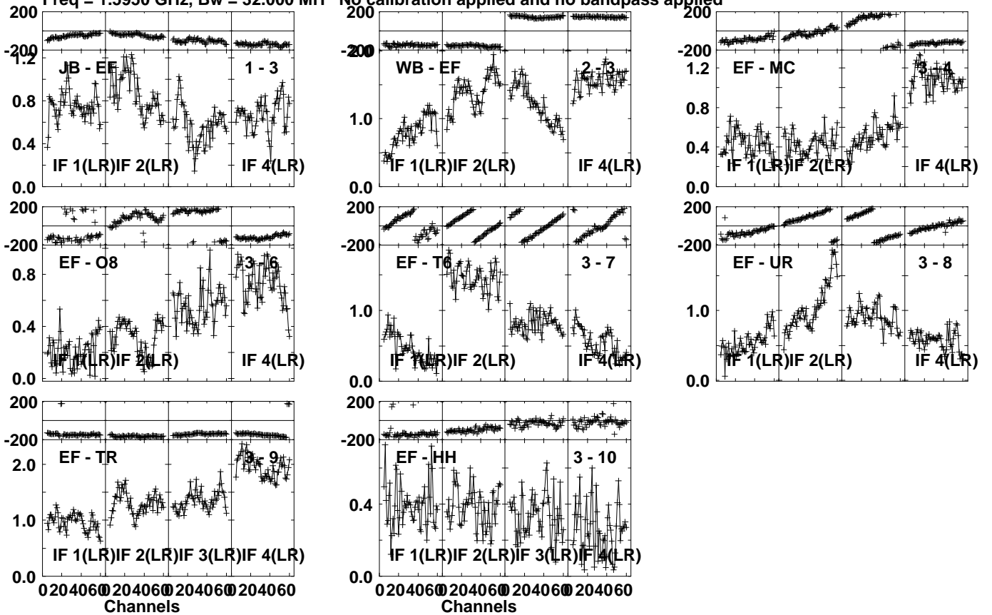
Lower frame: Milli Ampl Jy Top frame: Phas deg Vector averaged cross-power spectrum Several baselines displayed Timerange: 00/03:27:01 to 00/03:28:29
