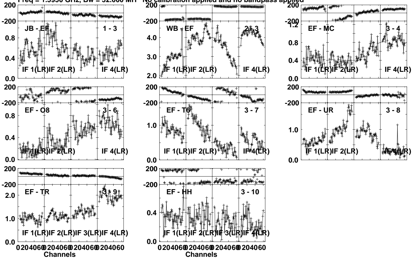
Lower frame: Milli Ampl Jy Top frame: Phas deg Vector averaged cross-power spectrum Several baselines displayed Timerange: 00/01:37:16 to 00/01:38:14
