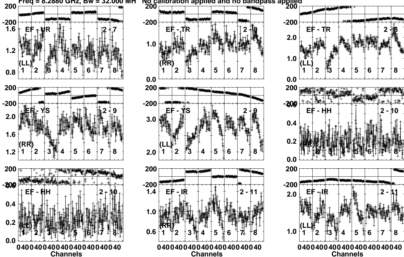
Lower frame: Milli Ampl Jy Top frame: Phas deg Vector averaged cross-power spectrum Several baselines displayed Timerange: 00/22:33:56 to 00/22:34:54
