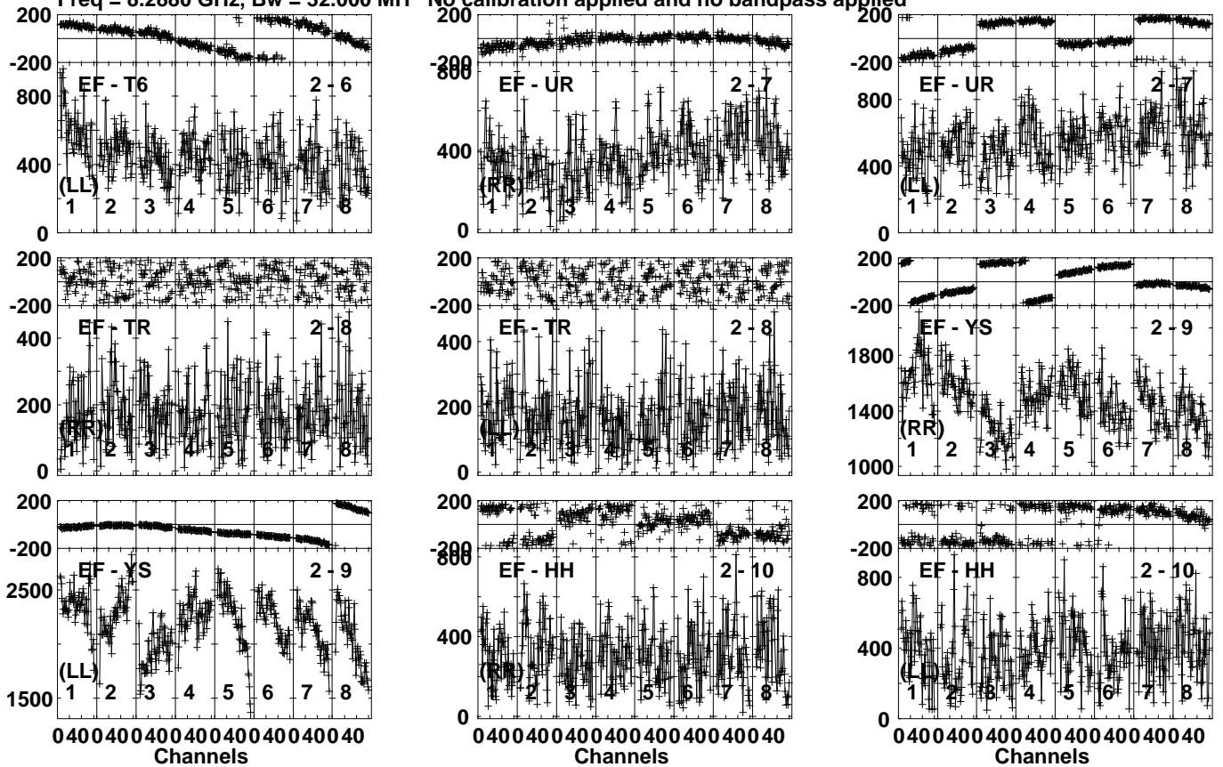
Lower frame: Micro Ampl Jy Top frame: Phas deg Vector averaged cross-power spectrum Several baselines displayed Timerange: 00/18:27:16 to 00/18:28:14
