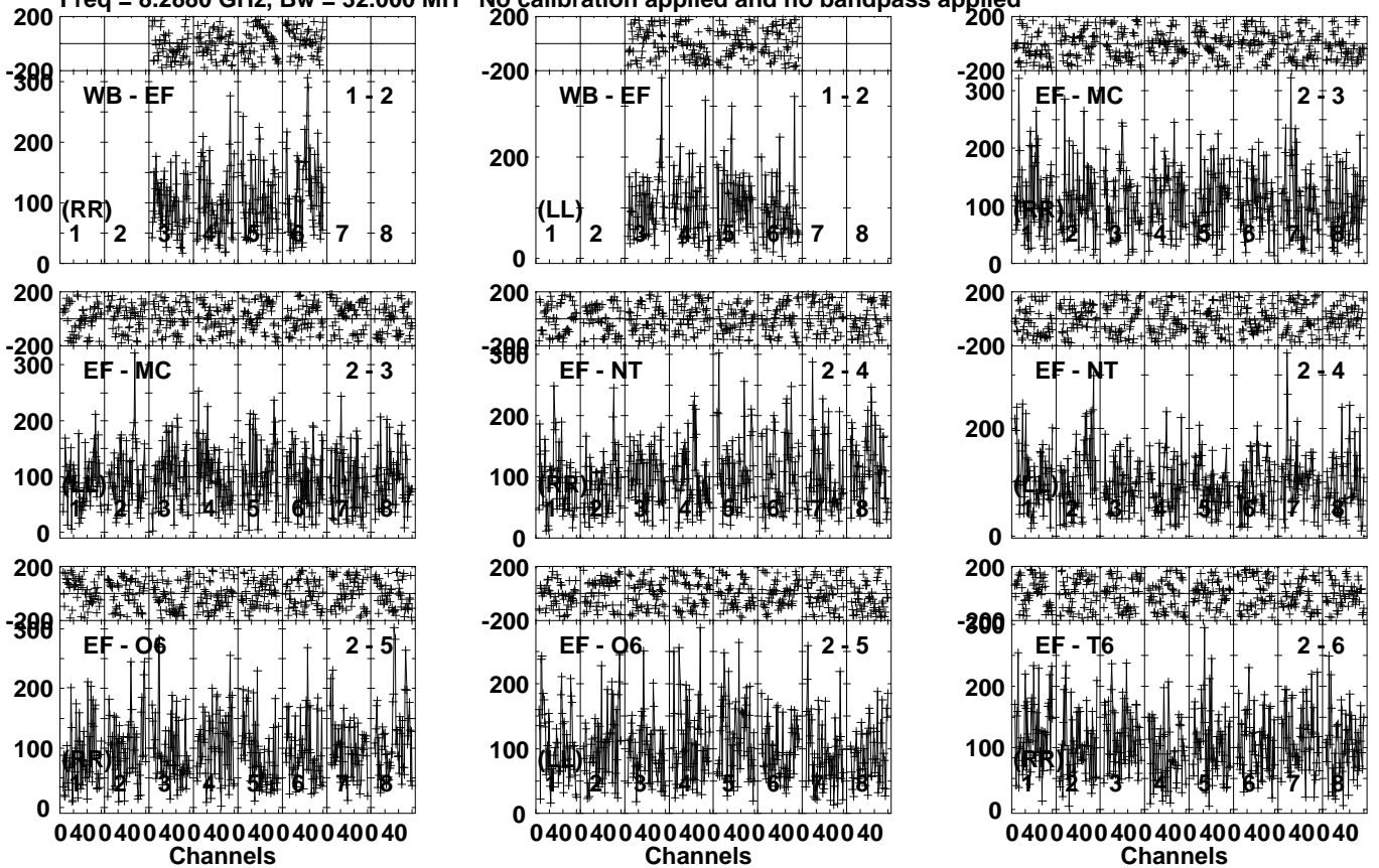
Lower frame: Micro Ampl Jy Top frame: Phas deg Vector averaged cross-power spectrum Several baselines displayed Timerange: 00/17:25:21 to 00/17:27:19
