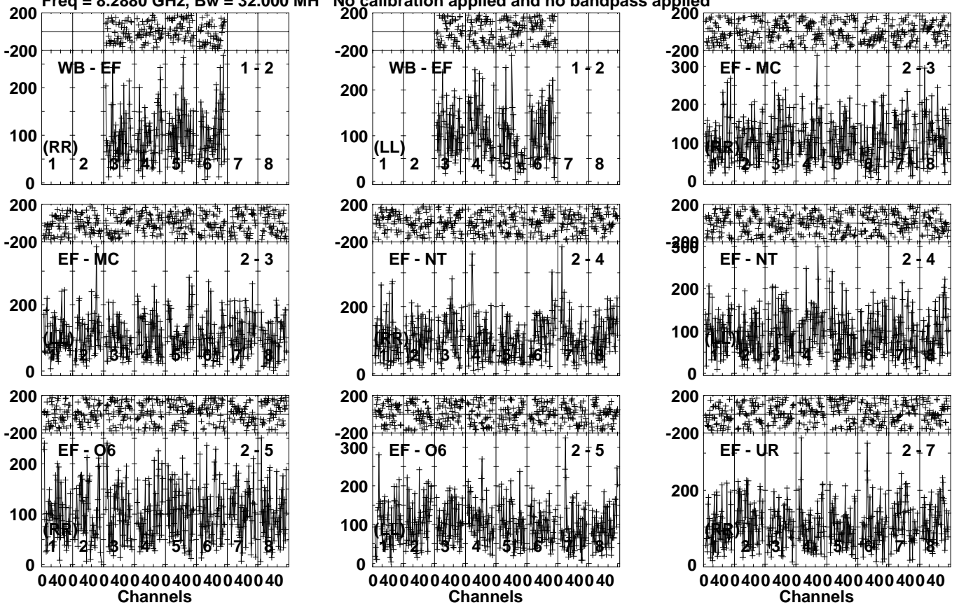
Lower frame: Micro Ampl Jy Top frame: Phas deg Vector averaged cross-power spectrum Several baselines displayed Timerange: 00/22:43:41 to 00/22:45:39
