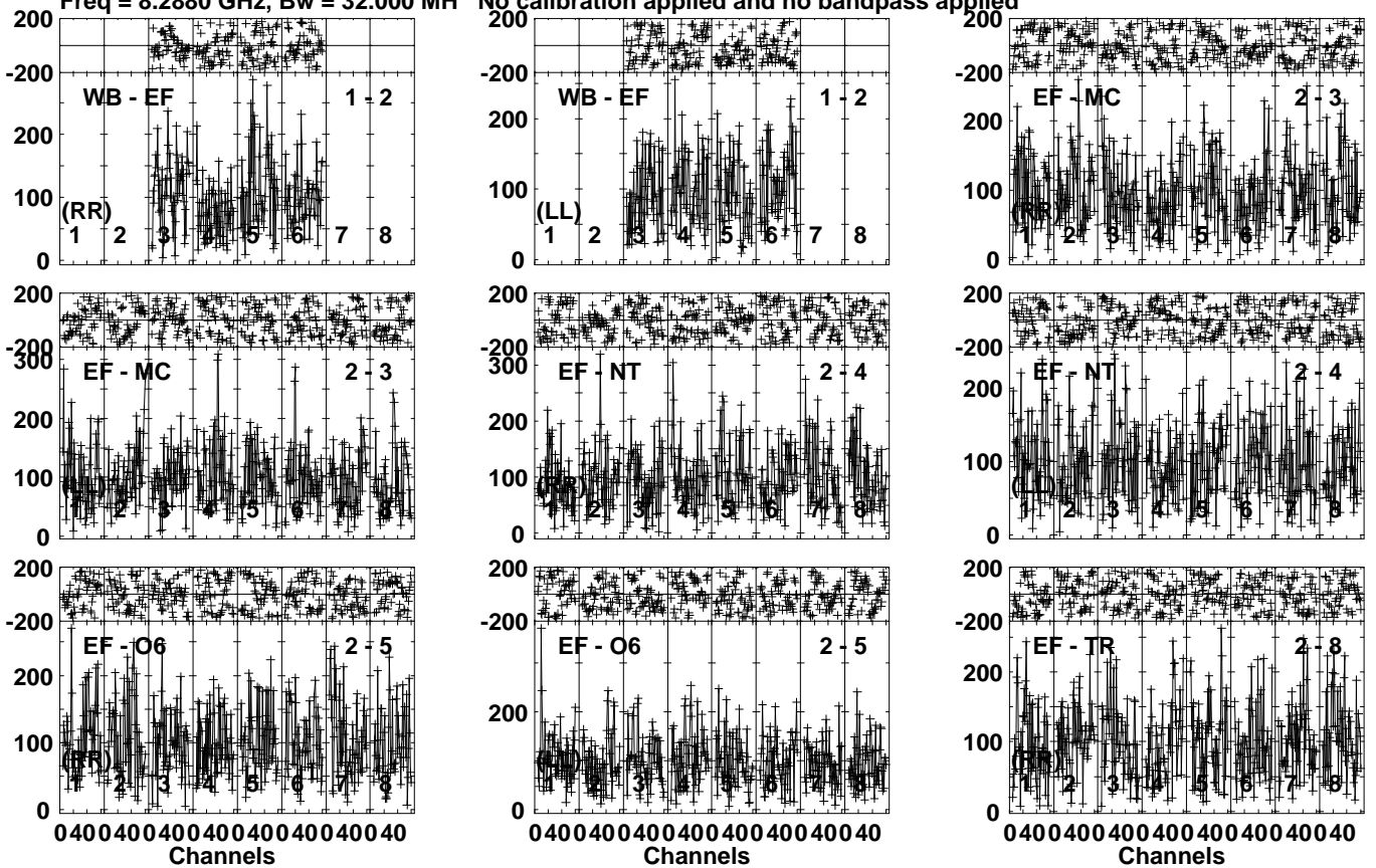
Lower frame: Micro Ampl Jy Top frame: Phas deg Vector averaged cross-power spectrum Several baselines displayed Timerange: 01/01:08:06 to 01/01:10:04
