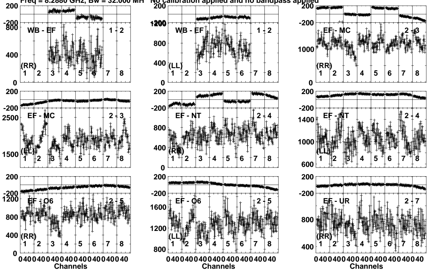
Lower frame: Micro Ampl Jy Top frame: Phas deg Vector averaged cross-power spectrum Several baselines displayed Timerange: 00/22:33:56 to 00/22:34:54
