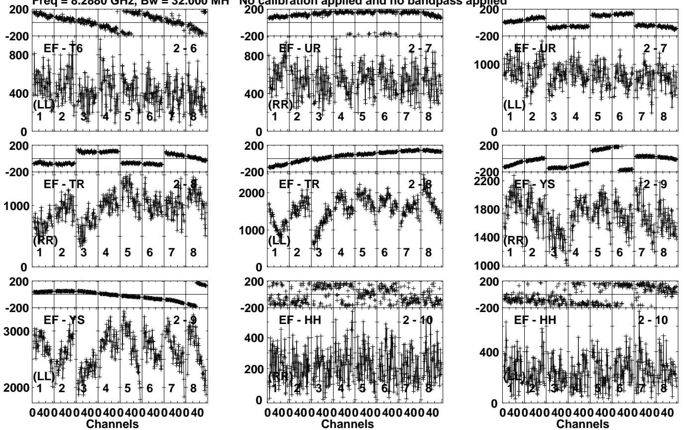
Lower frame: Micro Ampl Jy Top frame: Phas deg Vector averaged cross-power spectrum Several baselines displayed Timerange: 00/19:42:46 to 00/19:43:44
