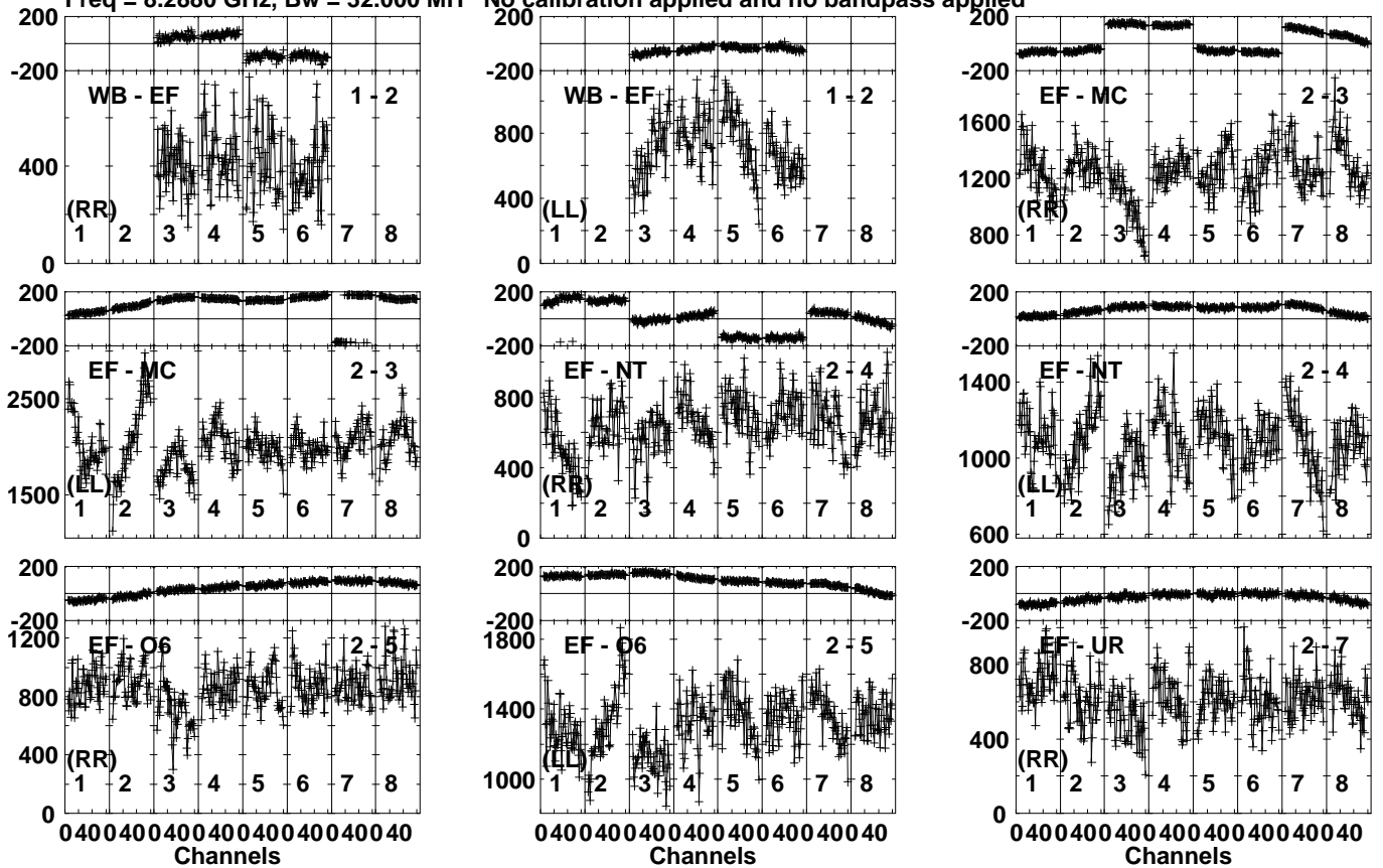
Lower frame: Micro Ampl Jy Top frame: Phas deg Vector averaged cross-power spectrum Several baselines displayed Timerange: 00/20:40:11 to 00/20:41:09
