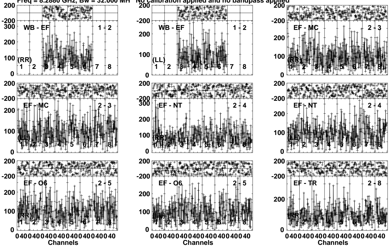
Lower frame: Micro Ampl Jy Top frame: Phas deg Vector averaged cross-power spectrum Several baselines displayed Timerange: 01/00:19:21 to 01/00:21:19
