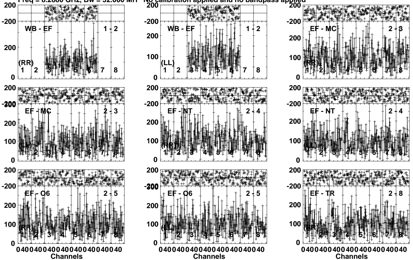
Lower frame: Micro Ampl Jy Top frame: Phas deg Vector averaged cross-power spectrum Several baselines displayed Timerange: 01/00:39:36 to 01/00:41:34
