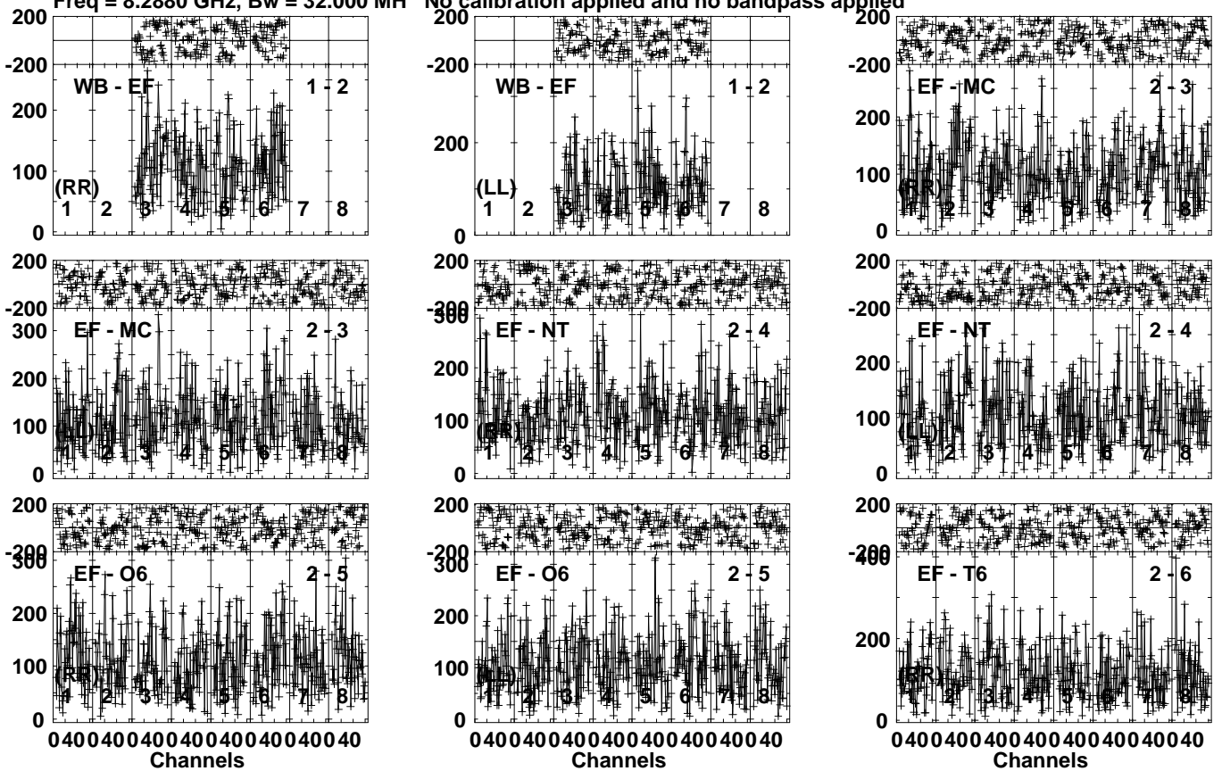
Lower frame: Micro Ampl Jy Top frame: Phas deg Vector averaged cross-power spectrum Several baselines displayed Timerange: 00/16:57:51 to 00/16:59:49
