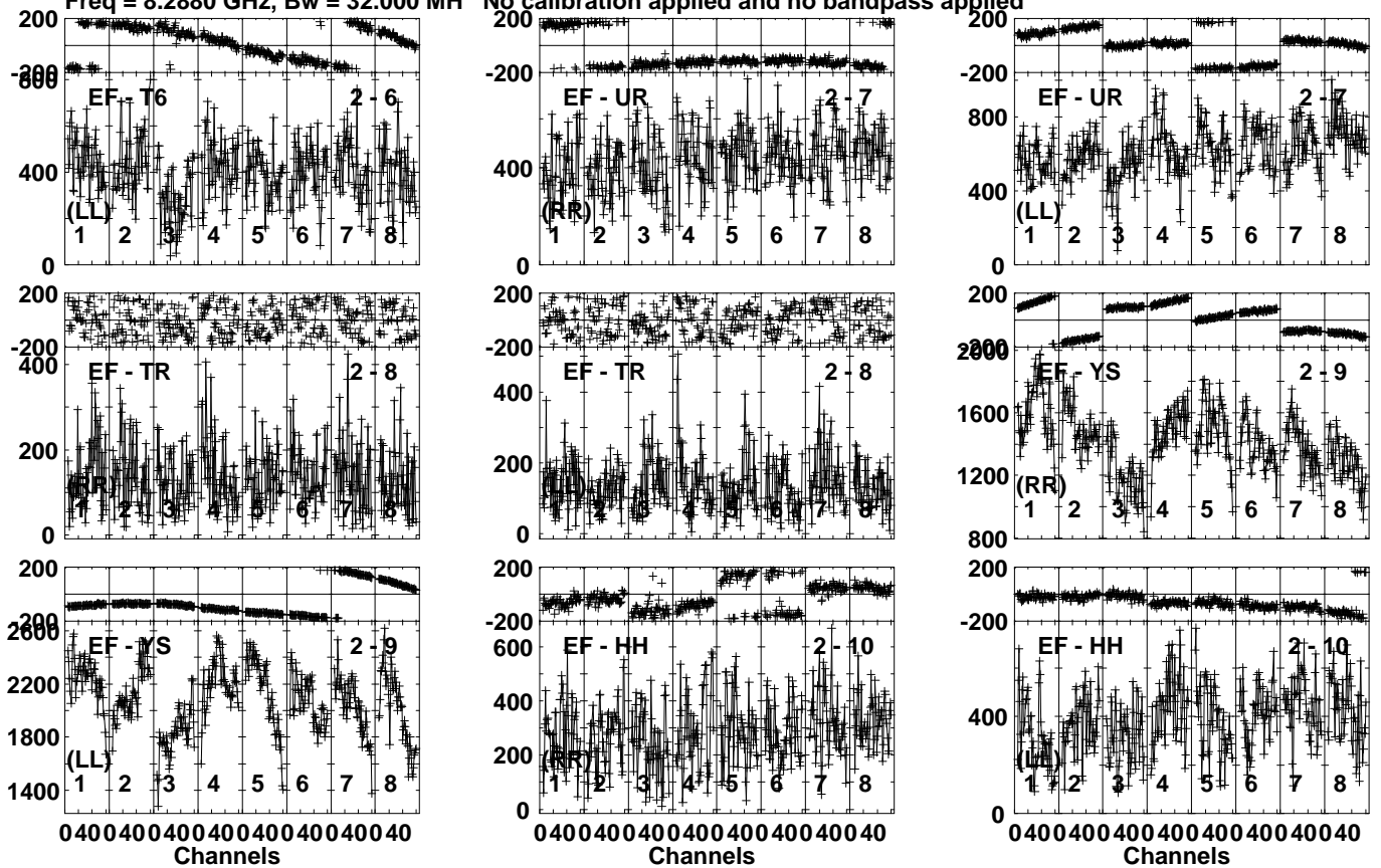
Lower frame: Micro Ampl Jy Top frame: Phas deg Vector averaged cross-power spectrum Several baselines displayed Timerange: 00/18:31:36 to 00/18:32:34
