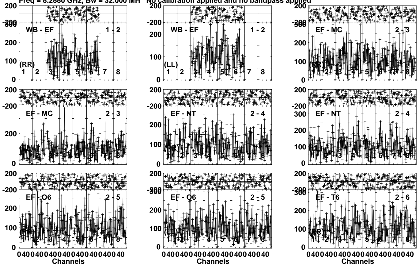
Lower frame: Micro Ampl Jy Top frame: Phas deg Vector averaged cross-power spectrum Several baselines displayed Timerange: 00/18:20:46 to 00/18:22:44
