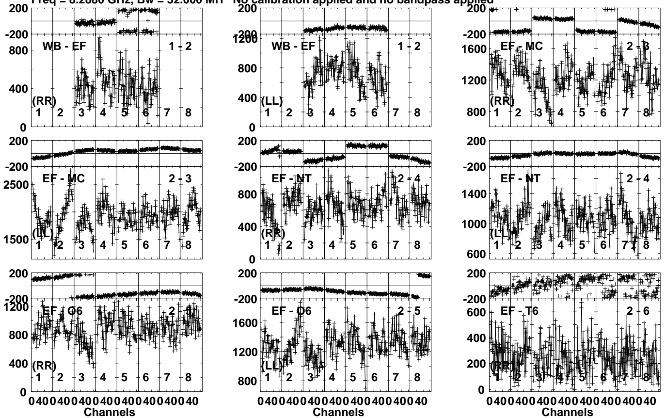
Lower frame: Micro Ampl Jy Top frame: Phas deg Vector averaged cross-power spectrum Several baselines displayed Timerange: 00/20:11:16 to 00/20:12:14
