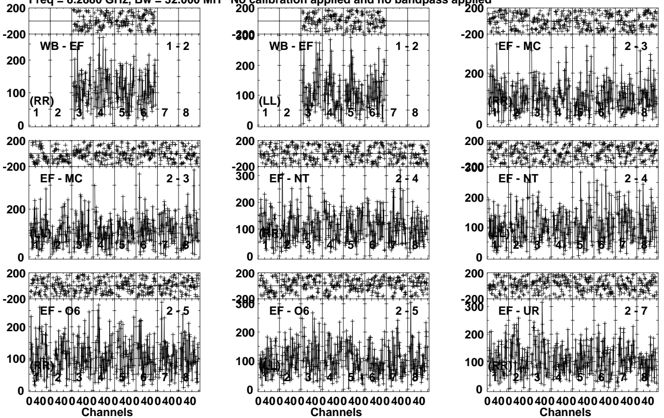
Lower frame: Micro Ampl Jy Top frame: Phas deg Vector averaged cross-power spectrum Several baselines displayed Timerange: 00/21:14:11 to 00/21:16:09
