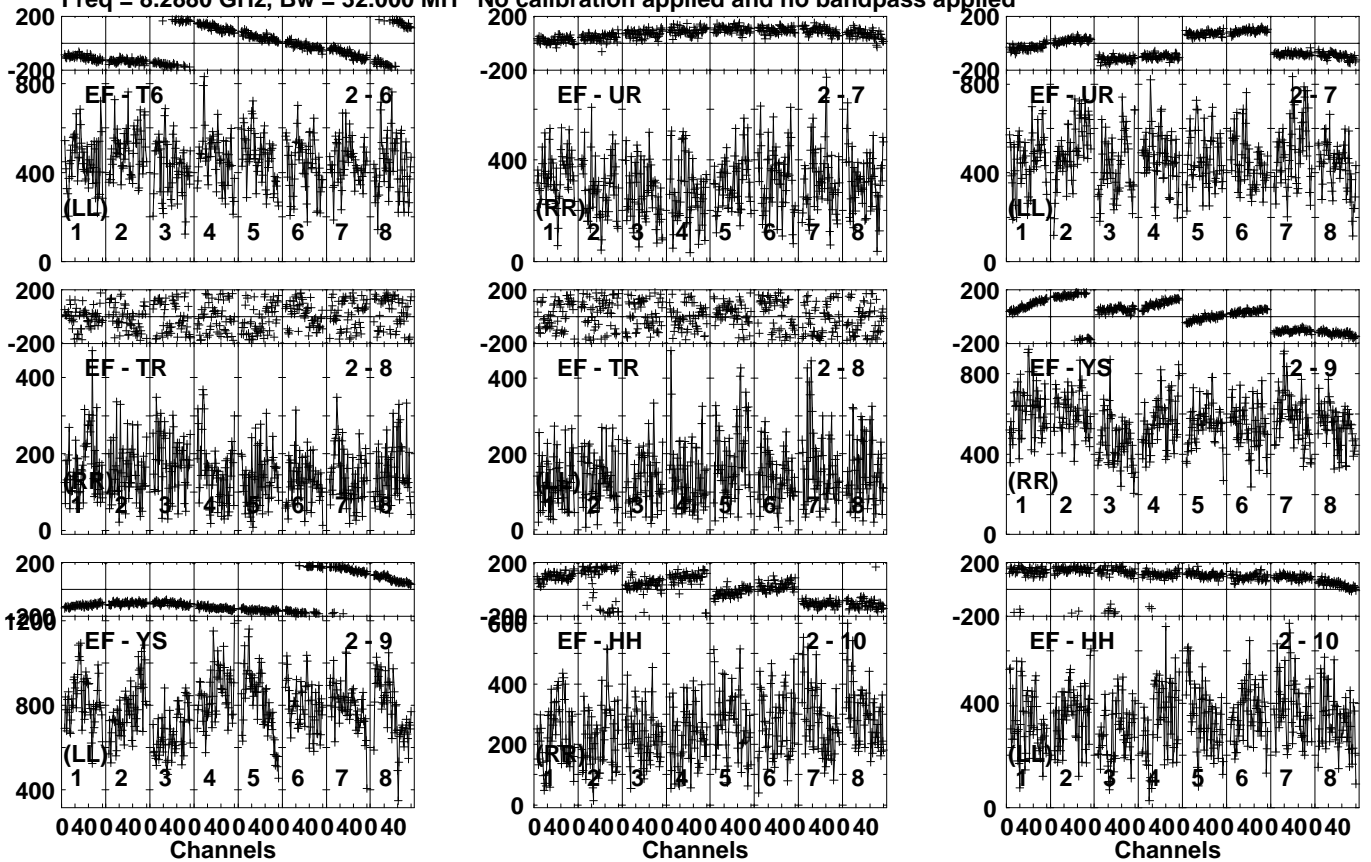
Lower frame: Micro Ampl Jy Top frame: Phas deg Vector averaged cross-power spectrum Several baselines displayed Timerange: 00/17:32:31 to 00/17:33:29
