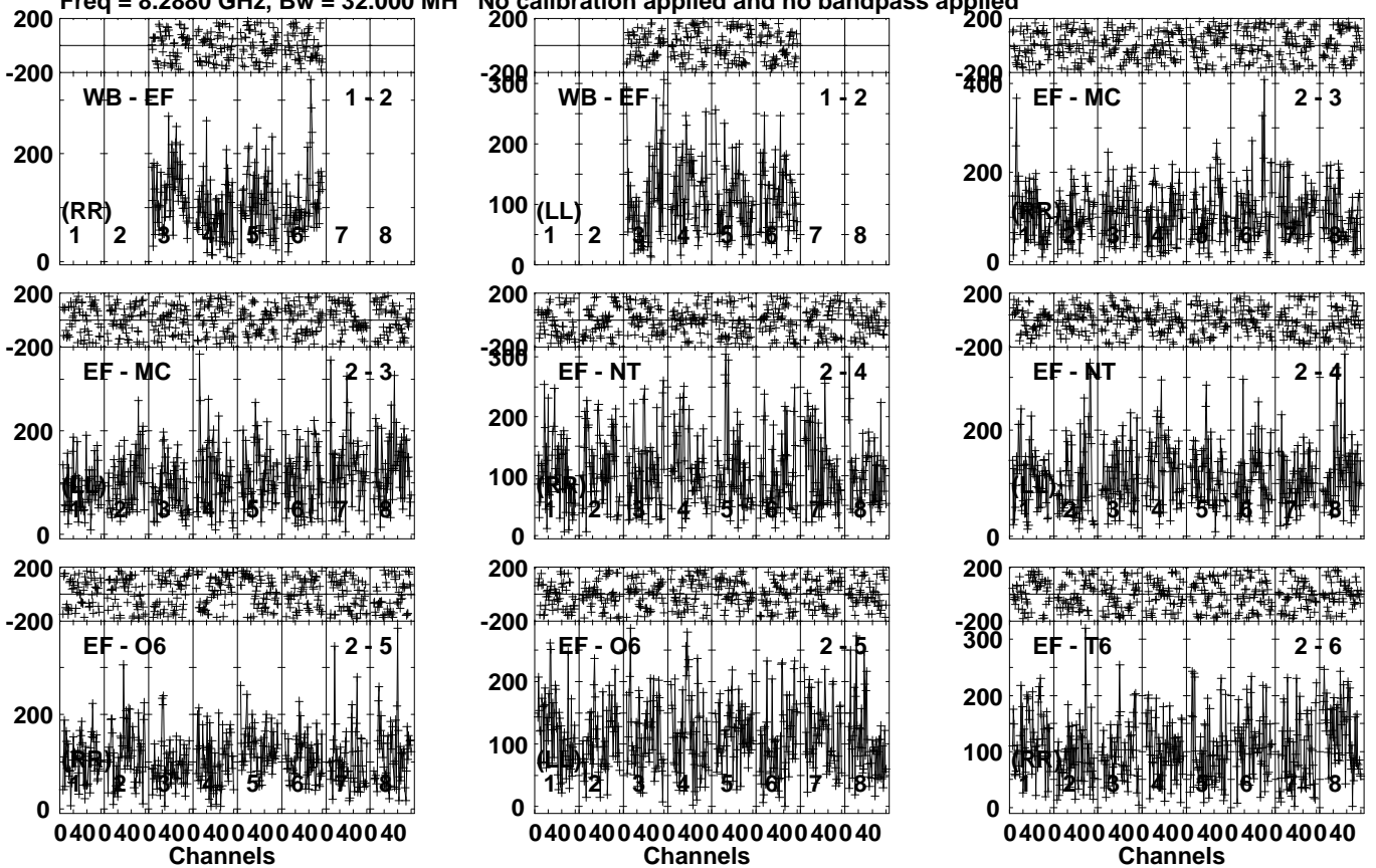
Lower frame: Micro Ampl Jy Top frame: Phas deg Vector averaged cross-power spectrum Several baselines displayed Timerange: 00/20:12:46 to 00/20:14:44
