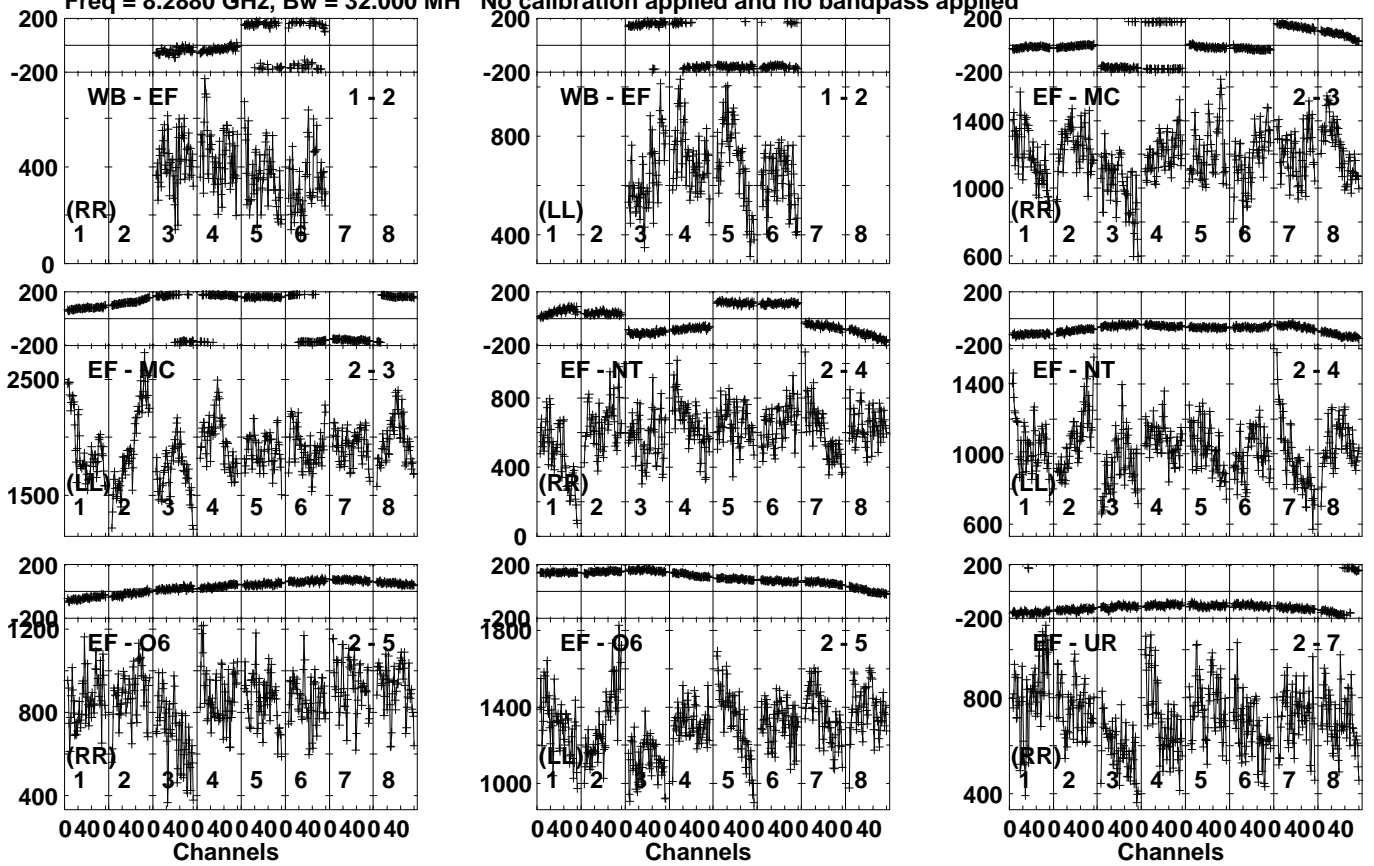
Lower frame: Micro Ampl Jy Top frame: Phas deg Vector averaged cross-power spectrum Several baselines displayed Timerange: 00/22:01:41 to 00/22:02:39
