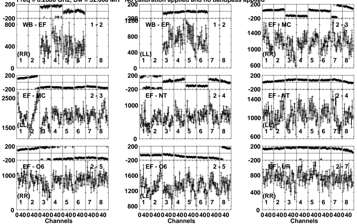
Lower frame: Micro Ampl Jy Top frame: Phas deg Vector averaged cross-power spectrum Several baselines displayed Timerange: 00/22:46:11 to 00/22:47:09
