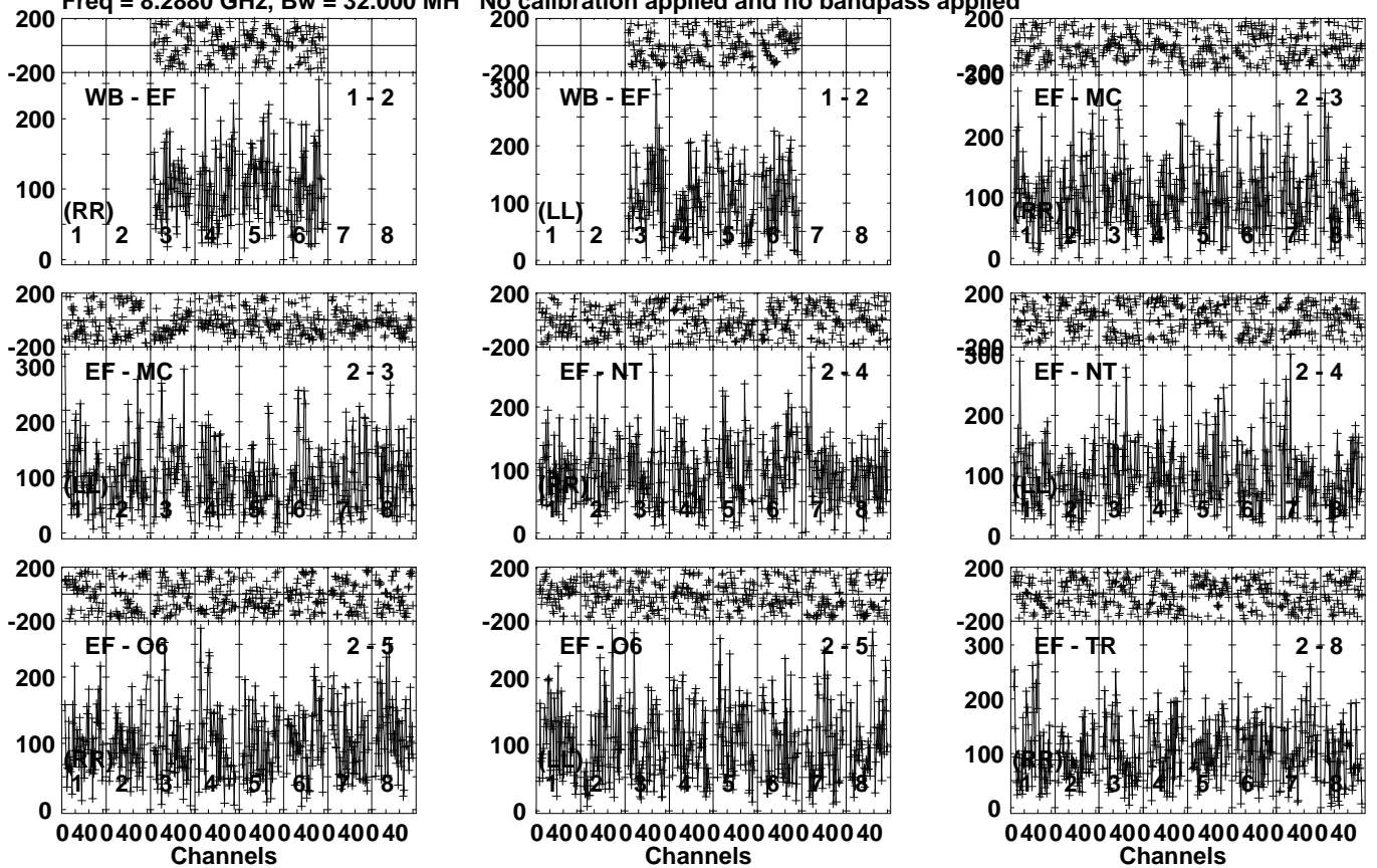
Lower frame: Micro Ampl Jy Top frame: Phas deg Vector averaged cross-power spectrum Several baselines displayed Timerange: 00/23:50:36 to 00/23:52:34
