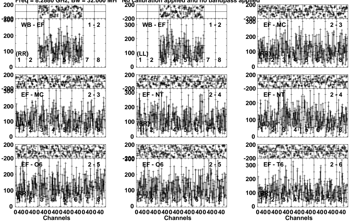
Lower frame: Micro Ampl Jy Top frame: Phas deg Vector averaged cross-power spectrum Several baselines displayed Timerange: 00/17:46:26 to 00/17:48:24
