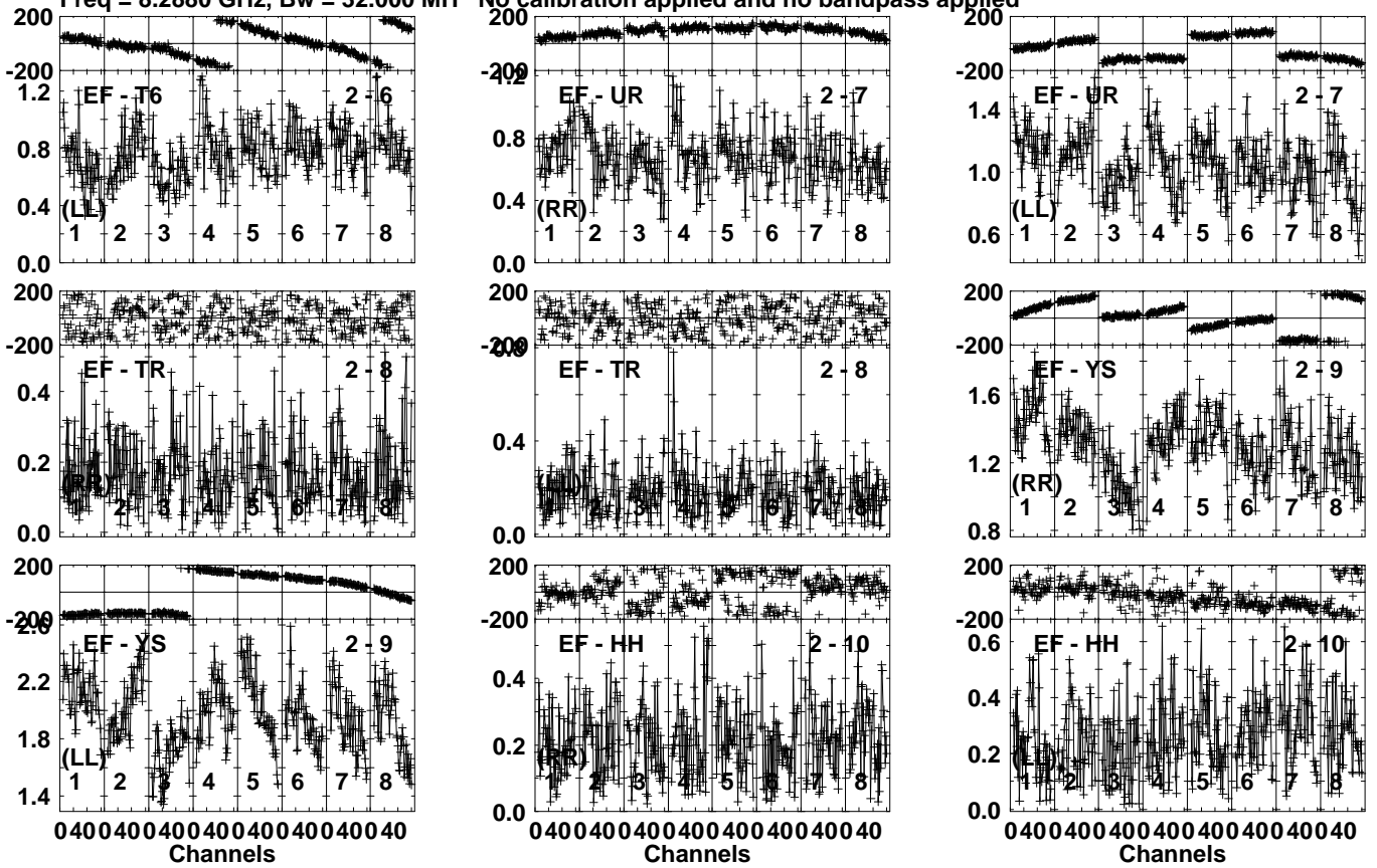
Lower frame: Milli Ampl Jy Top frame: Phas deg Vector averaged cross-power spectrum Several baselines displayed Timerange: 00/19:12:36 to 00/19:13:34
