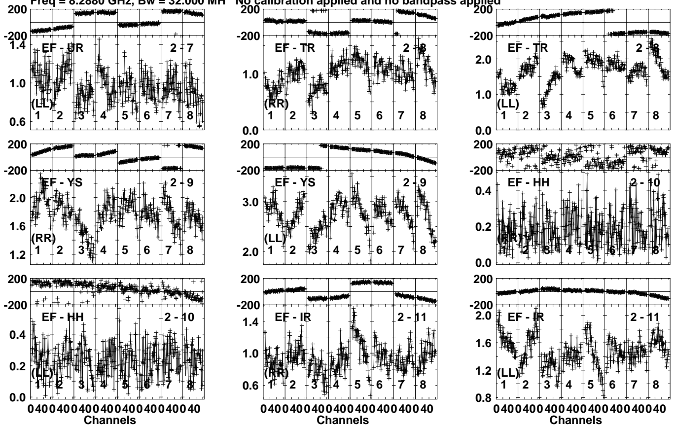
Lower frame: Milli Ampl Jy Top frame: Phas deg Vector averaged cross-power spectrum Several baselines displayed Timerange: 00/20:40:11 to 00/20:41:09
