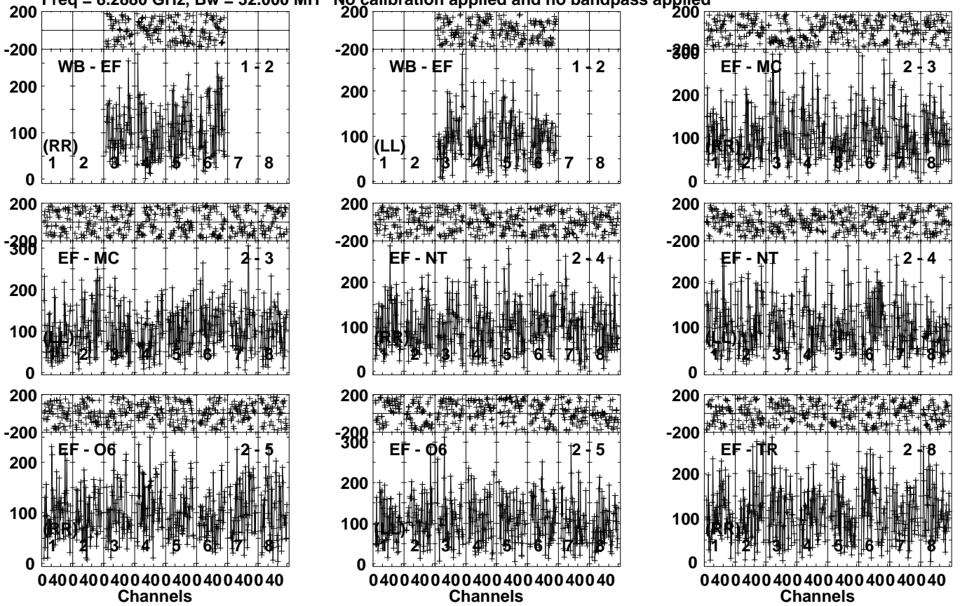
Lower frame: Micro Ampl Jy Top frame: Phas deg Vector averaged cross-power spectrum Several baselines displayed Timerange: 00/23:26:06 to 00/23:28:04
