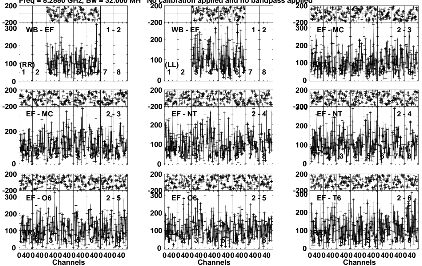
Lower frame: Micro Ampl Jy Top frame: Phas deg Vector averaged cross-power spectrum Several baselines displayed Timerange: 00/19:48:36 to 00/19:50:34
