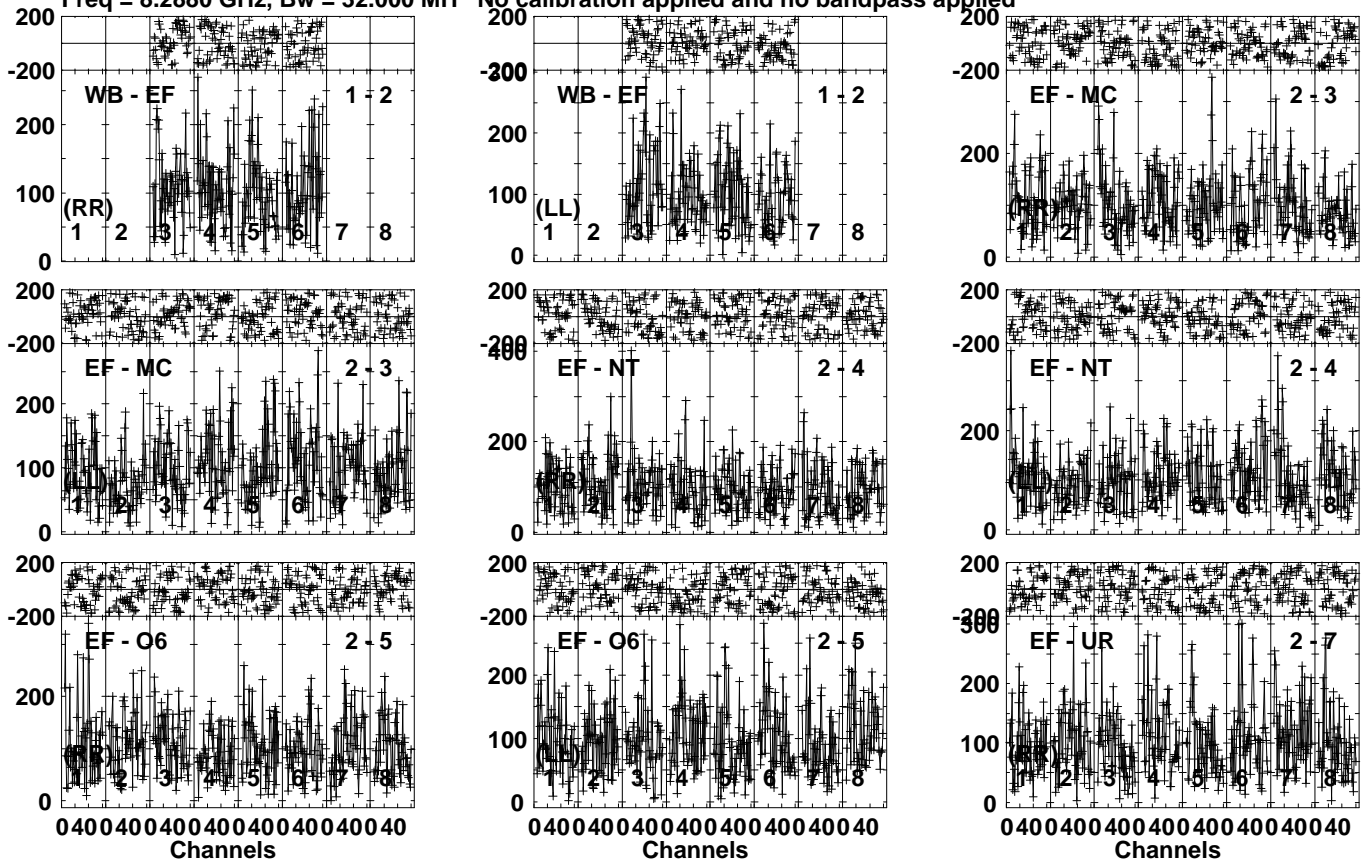
Lower frame: Micro Ampl Jy Top frame: Phas deg Vector averaged cross-power spectrum Several baselines displayed Timerange: 00/22:51:56 to 00/22:53:54
