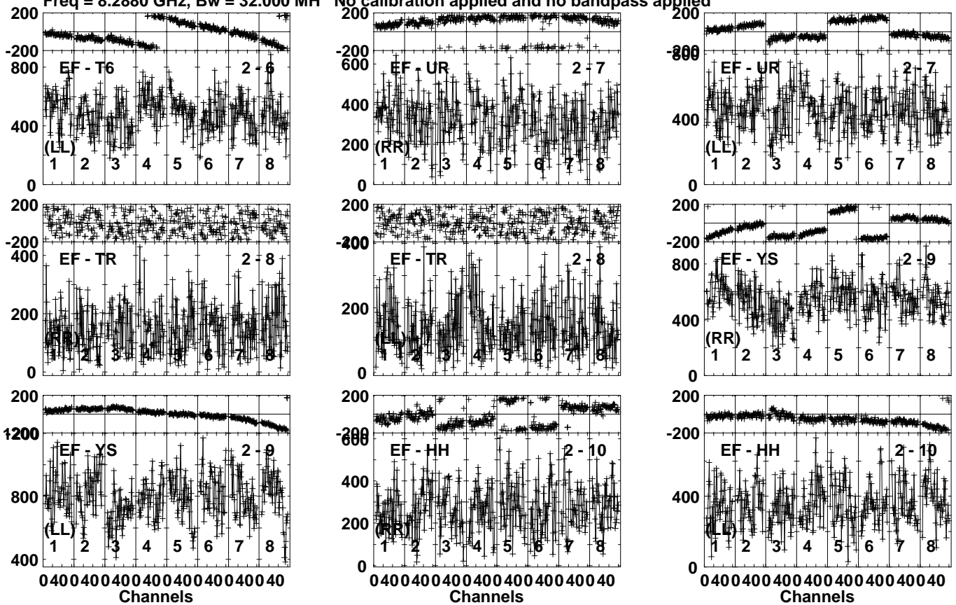
Lower frame: Micro Ampl Jy Top frame: Phas deg Vector averaged cross-power spectrum Several baselines displayed Timerange: 00/17:44:56 to 00/17:45:54
