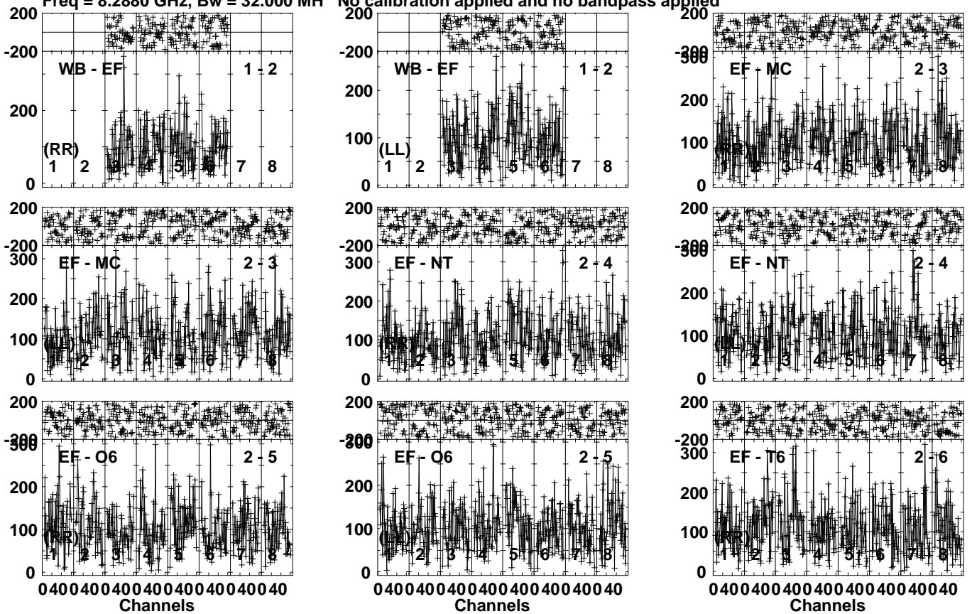
Lower frame: Micro Ampl Jy Top frame: Phas deg Vector averaged cross-power spectrum Several baselines displayed Timerange: 00/19:05:46 to 00/19:07:44
