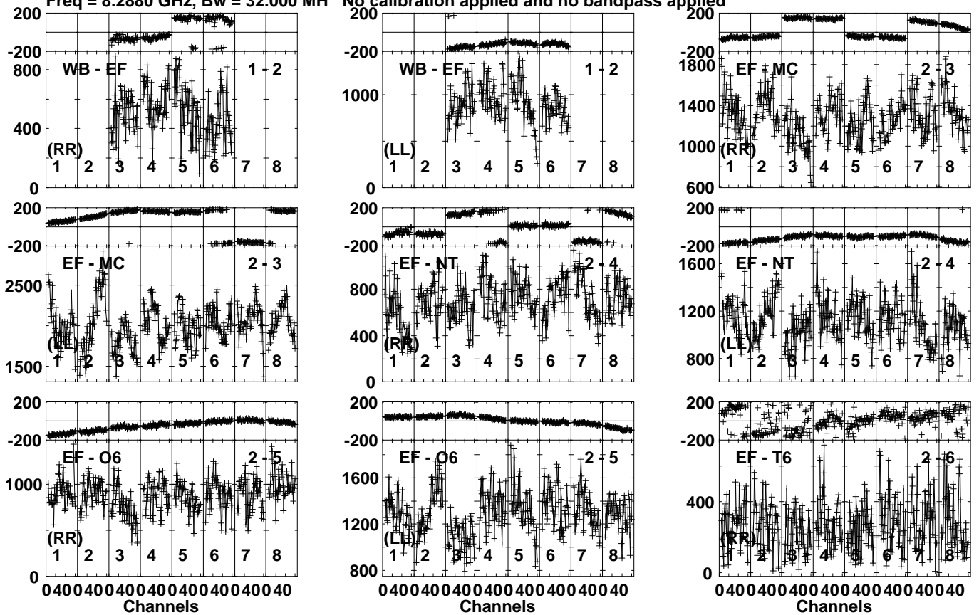
Lower frame: Micro Ampl Jy Top frame: Phas deg Vector averaged cross-power spectrum Several baselines displayed Timerange: 00/19:38:46 to 00/19:39:44
