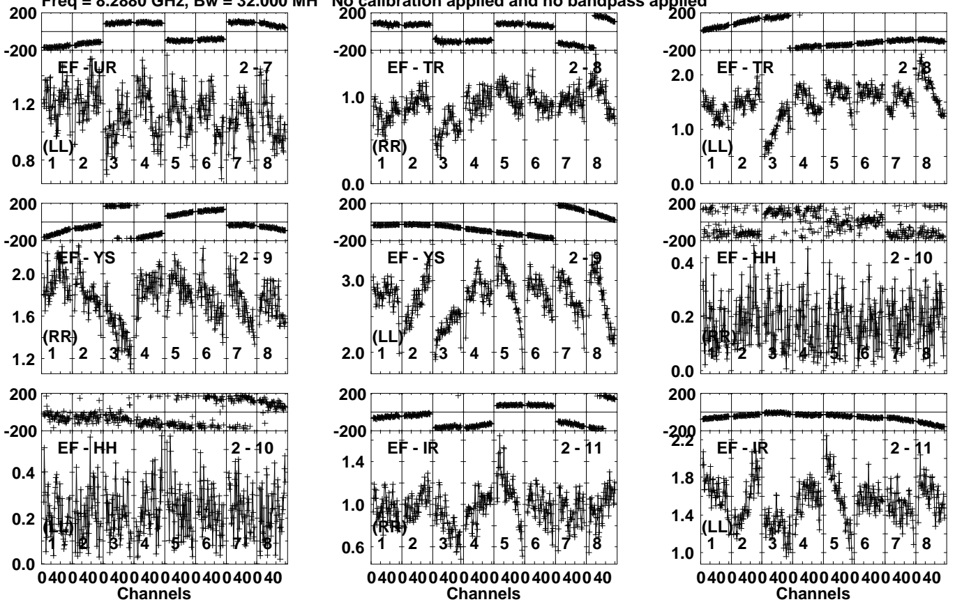
Lower frame: Milli Ampl Jy Top frame: Phas deg Vector averaged cross-power spectrum Several baselines displayed Timerange: 00/22:01:41 to 00/22:02:39
