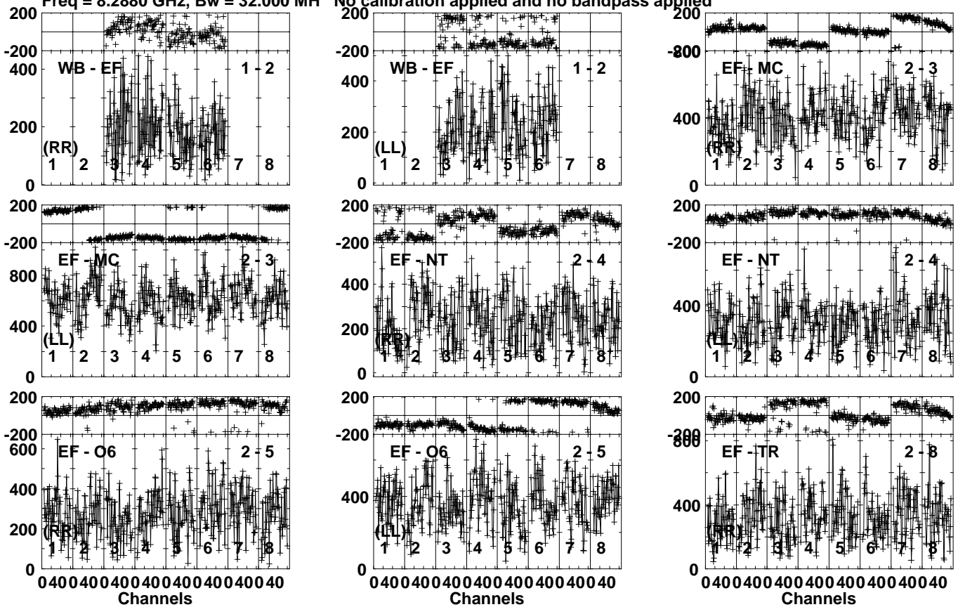
Lower frame: Micro Ampl Jy Top frame: Phas deg Vector averaged cross-power spectrum Several baselines displayed Timerange: 01/02:09:11 to 01/02:10:09
