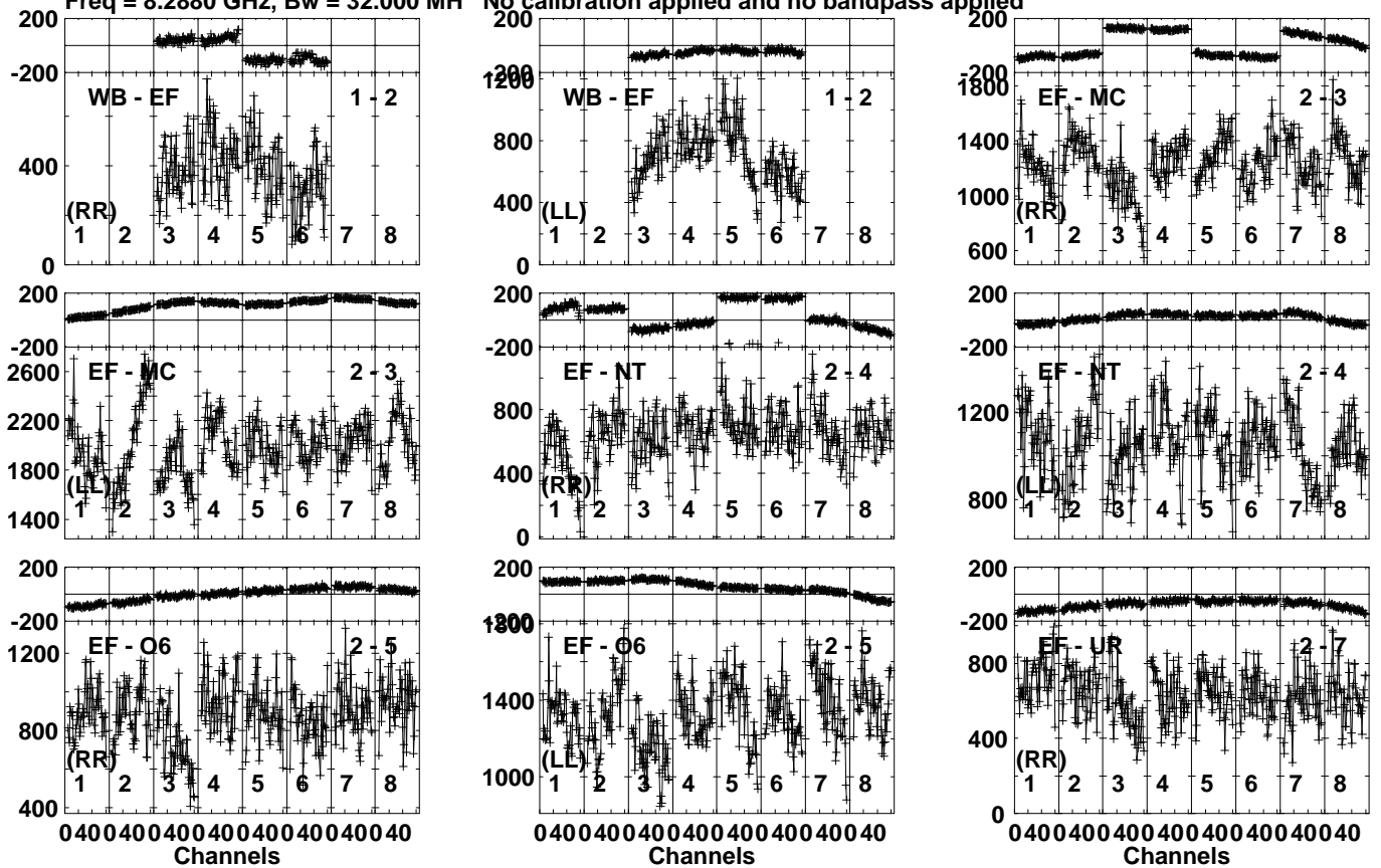
Lower frame: Micro Ampl Jy Top frame: Phas deg Vector averaged cross-power spectrum Several baselines displayed Timerange: 00/20:44:11 to 00/20:45:09
