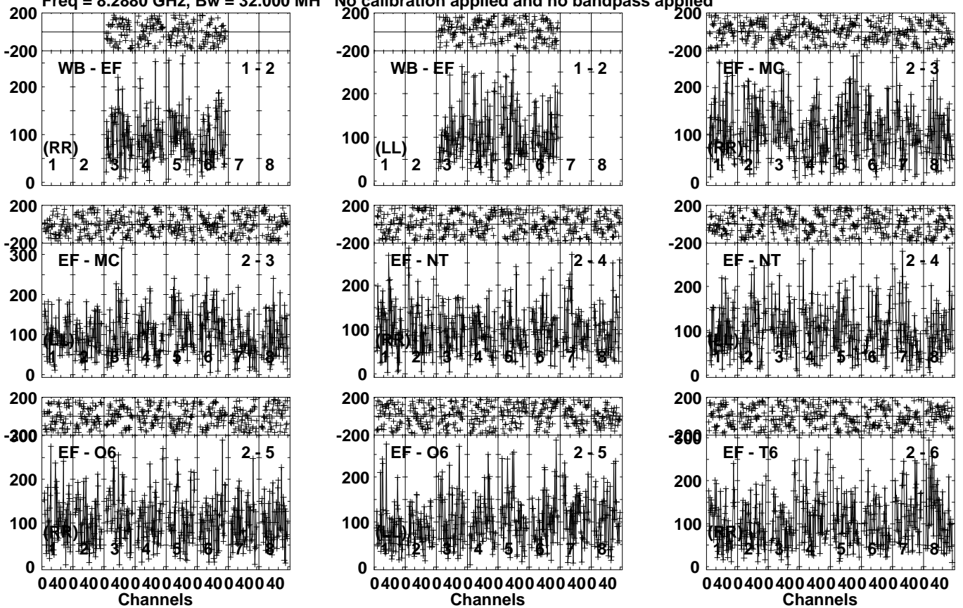
Lower frame: Micro Ampl Jy Top frame: Phas deg Vector averaged cross-power spectrum Several baselines displayed Timerange: 00/20:16:46 to 00/20:18:44
