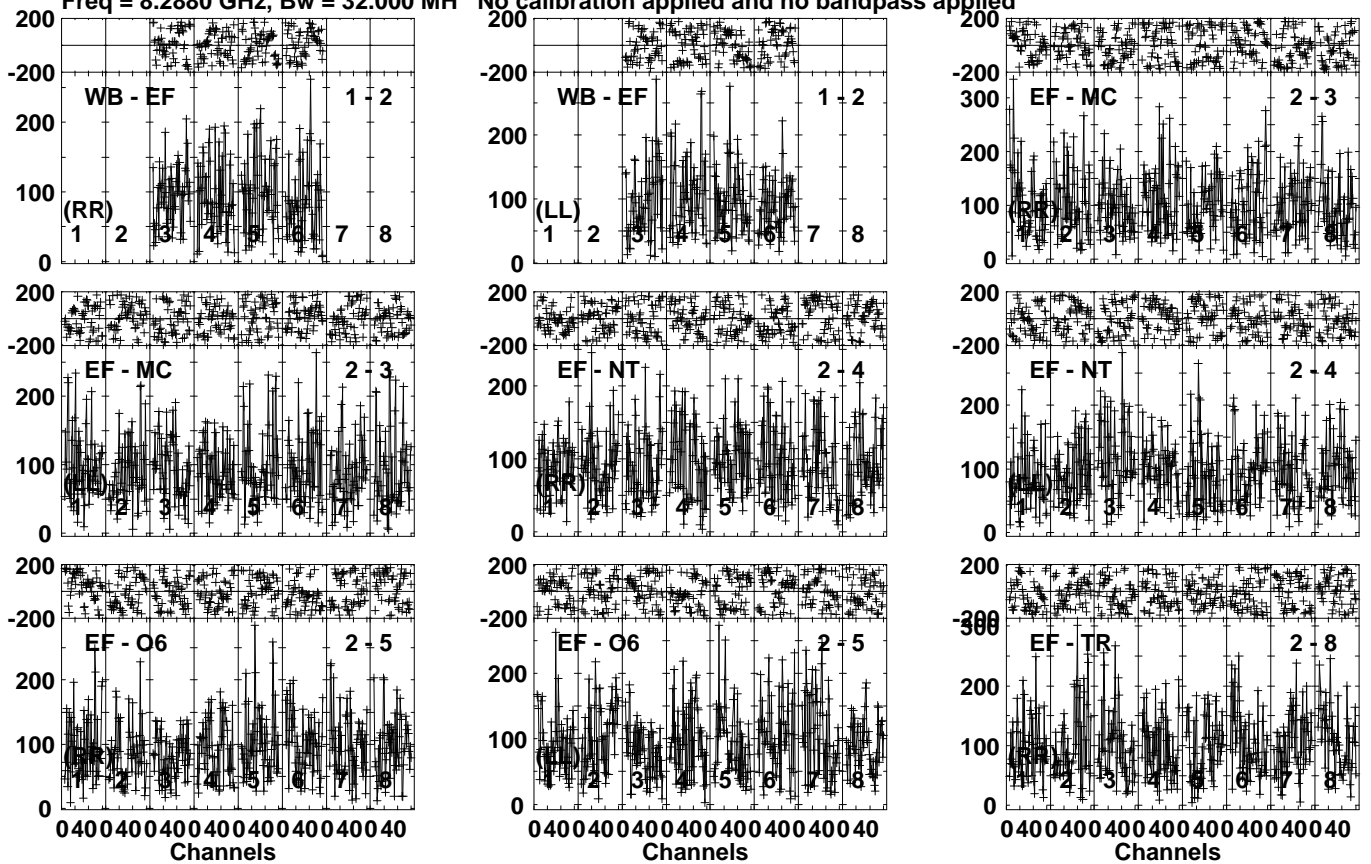
Lower frame: Micro Ampl Jy Top frame: Phas deg Vector averaged cross-power spectrum Several baselines displayed Timerange: 01/00:15:06 to 01/00:17:04
