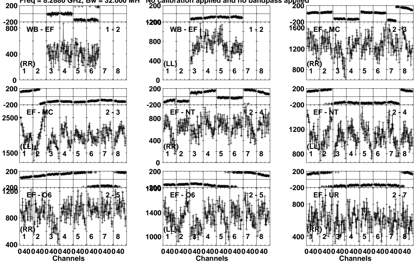
Lower frame: Micro Ampl Jy Top frame: Phas deg Vector averaged cross-power spectrum Several baselines displayed Timerange: 00/20:27:36 to 00/20:28:34
