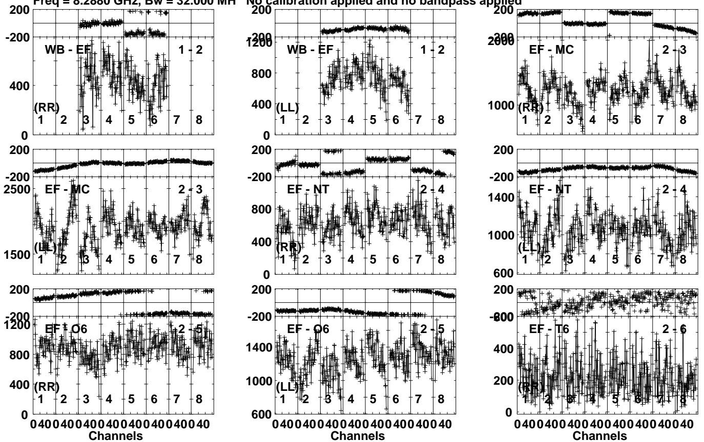
Lower frame: Micro Ampl Jy Top frame: Phas deg Vector averaged cross-power spectrum Several baselines displayed Timerange: 00/20:15:16 to 00/20:16:14
