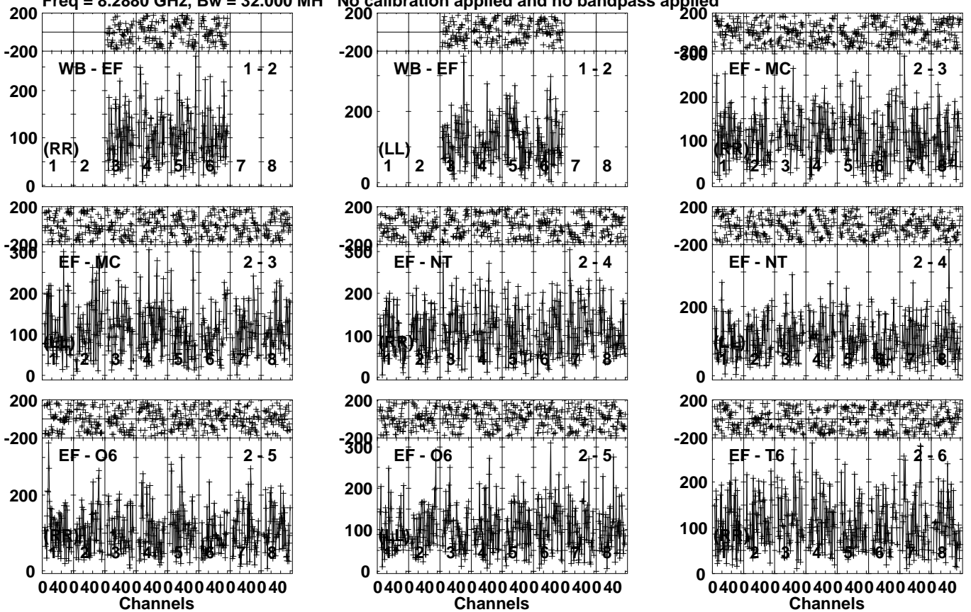
Lower frame: Micro Ampl Jy Top frame: Phas deg Vector averaged cross-power spectrum Several baselines displayed Timerange: 00/19:10:06 to 00/19:12:04
