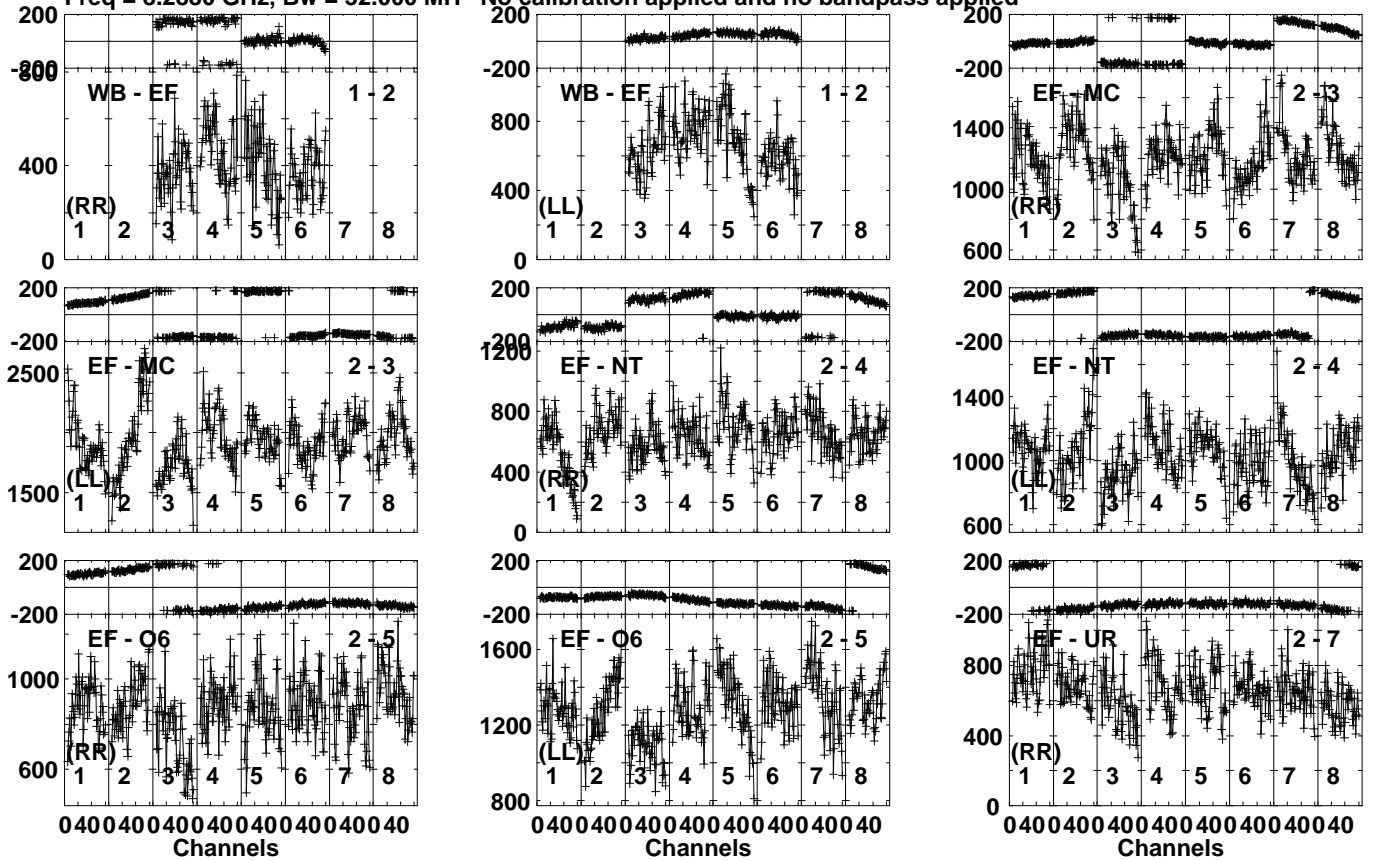
Lower frame: Micro Ampl Jy Top frame: Phas deg Vector averaged cross-power spectrum Several baselines displayed Timerange: 00/21:08:41 to 00/21:09:39
