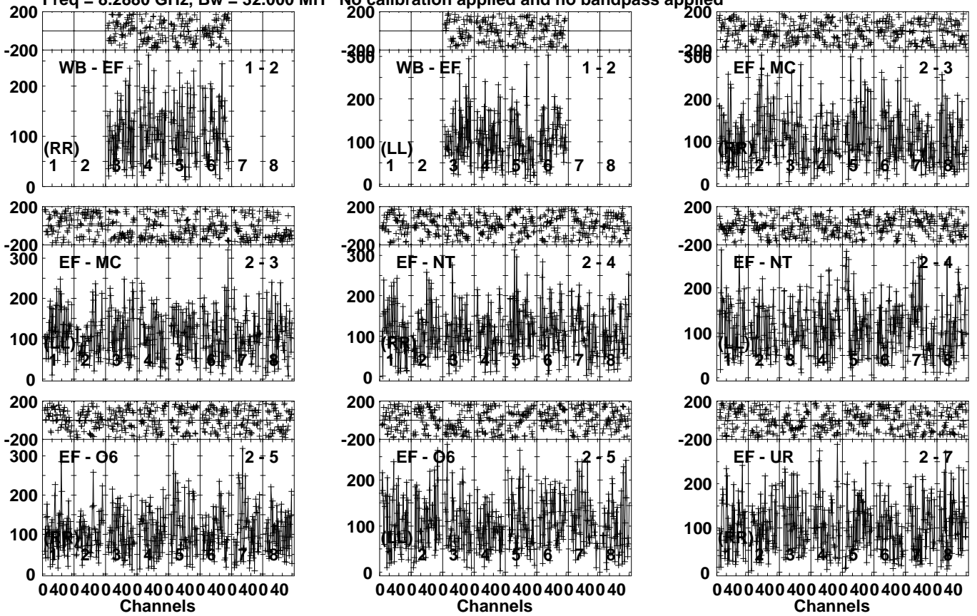
Lower frame: Micro Ampl Jy Top frame: Phas deg Vector averaged cross-power spectrum Several baselines displayed Timerange: 00/21:22:26 to 00/21:24:24
