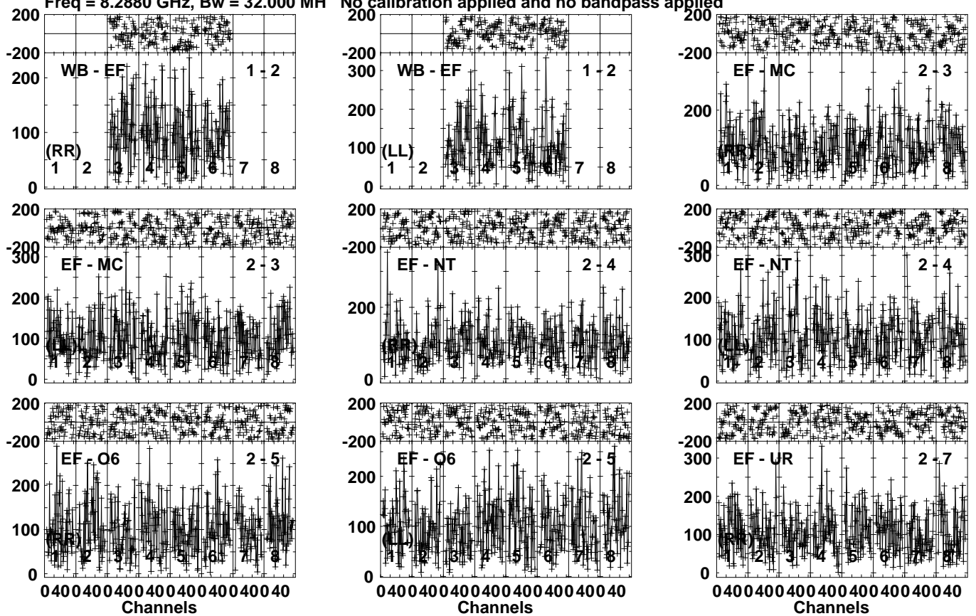
Lower frame: Micro Ampl Jy Top frame: Phas deg Vector averaged cross-power spectrum Several baselines displayed Timerange: 00/20:37:26 to 00/20:39:24
