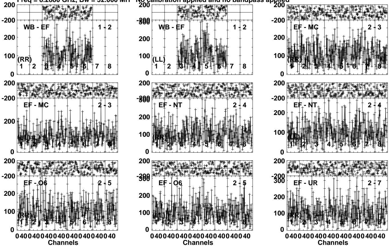
Lower frame: Micro Ampl Jy Top frame: Phas deg Vector averaged cross-power spectrum Several baselines displayed Timerange: 00/22:07:11 to 00/22:09:09
