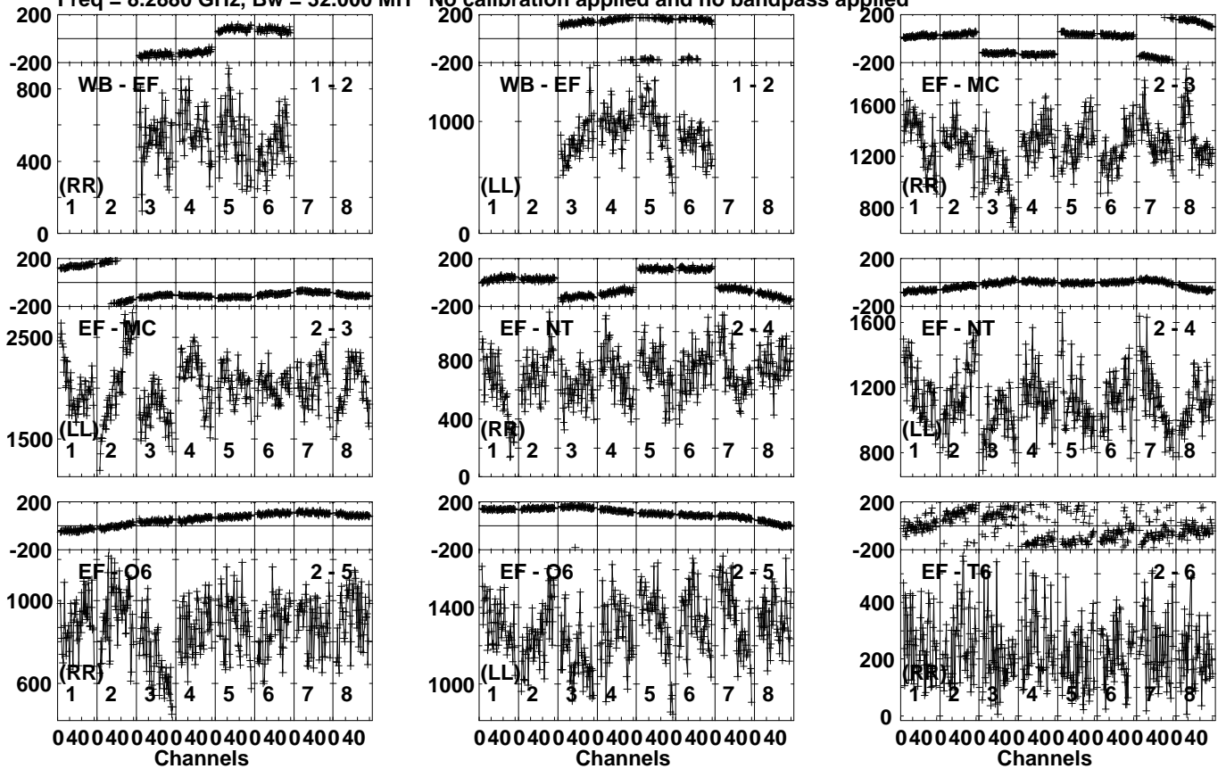
Lower frame: Micro Ampl Jy Top frame: Phas deg Vector averaged cross-power spectrum Several baselines displayed Timerange: 00/19:34:46 to 00/19:35:44
