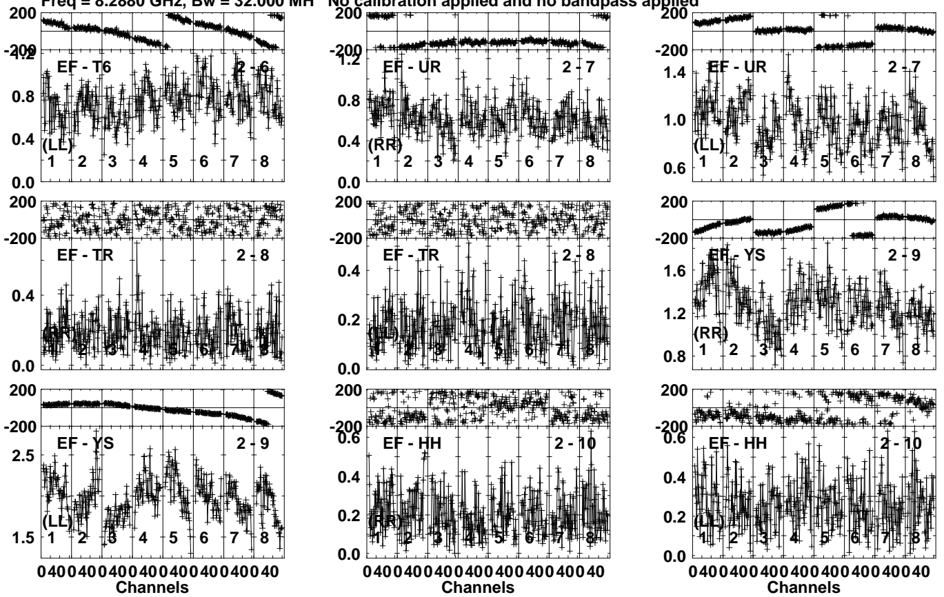
Lower frame: Milli Ampl Jy Top frame: Phas deg Vector averaged cross-power spectrum Several baselines displayed Timerange: 00/19:24:56 to 00/19:25:54
