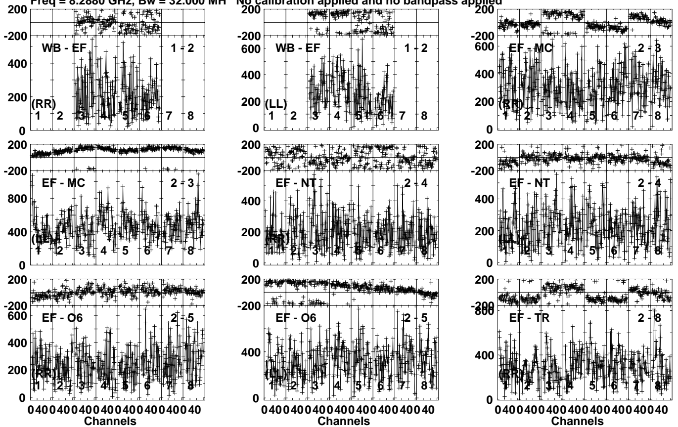
Lower frame: Micro Ampl Jy Top frame: Phas deg Vector averaged cross-power spectrum Several baselines displayed Timerange: 01/02:04:06 to 01/02:05:04
