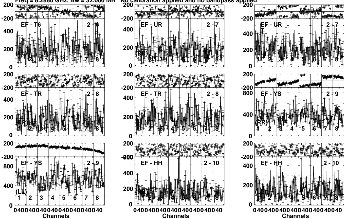
Lower frame: Micro Ampl Jy Top frame: Phas deg Vector averaged cross-power spectrum Several baselines displayed Timerange: 00/17:00:21 to 00/17:01:19
