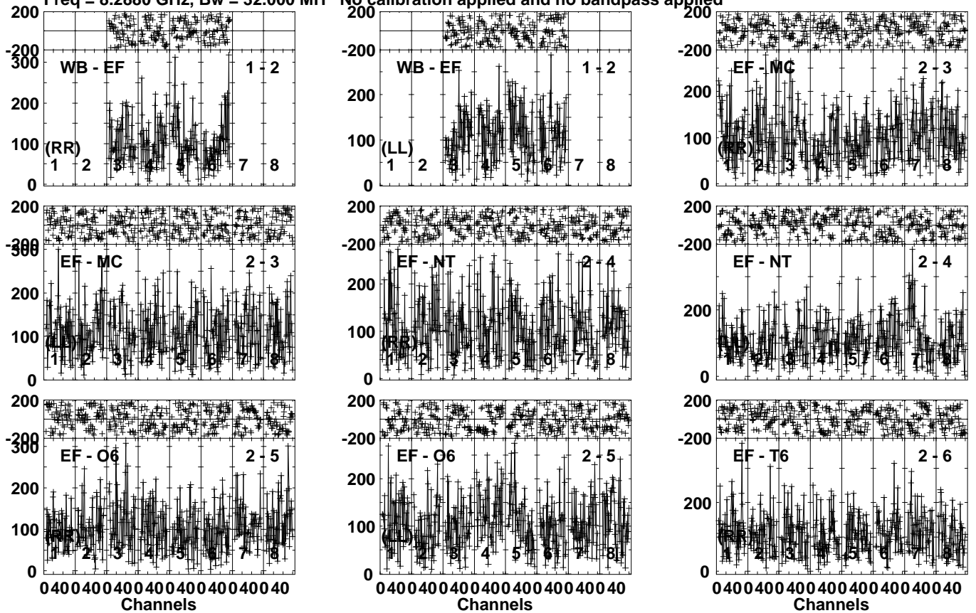
Lower frame: Micro Ampl Jy Top frame: Phas deg Vector averaged cross-power spectrum Several baselines displayed Timerange: 00/19:22:26 to 00/19:24:24
