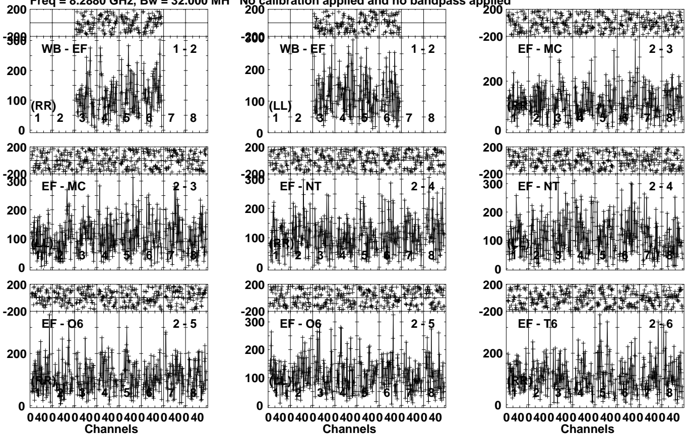
Lower frame: Micro Ampl Jy Top frame: Phas deg Vector averaged cross-power spectrum Several baselines displayed Timerange: 00/17:58:41 to 00/18:00:39
