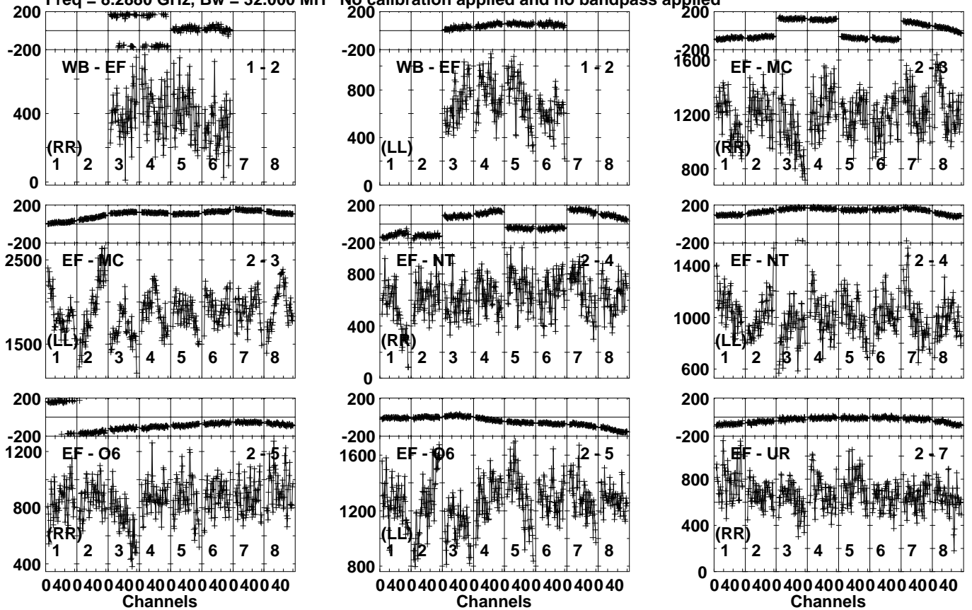
Lower frame: Micro Ampl Jy Top frame: Phas deg Vector averaged cross-power spectrum Several baselines displayed Timerange: 00/21:24:56 to 00/21:25:54
