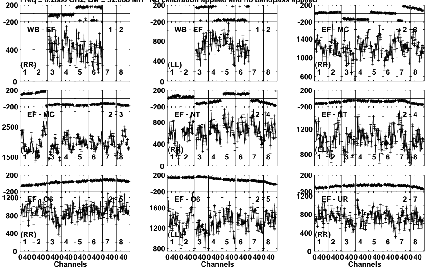
Lower frame: Micro Ampl Jy Top frame: Phas deg Vector averaged cross-power spectrum Several baselines displayed Timerange: 00/21:57:26 to 00/21:58:24
