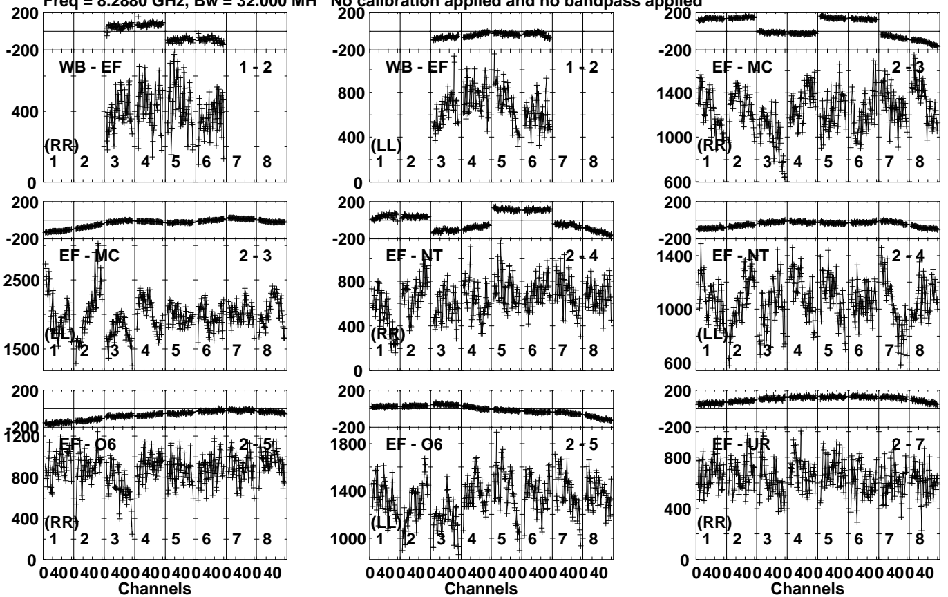
Lower frame: Micro Ampl Jy Top frame: Phas deg Vector averaged cross-power spectrum Several baselines displayed Timerange: 00/20:56:26 to 00/20:57:24
