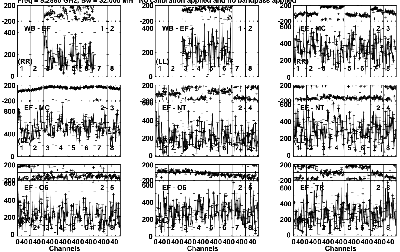
Lower frame: Micro Ampl Jy Top frame: Phas deg Vector averaged cross-power spectrum Several baselines displayed Timerange: 01/01:51:46 to 01/01:52:44
