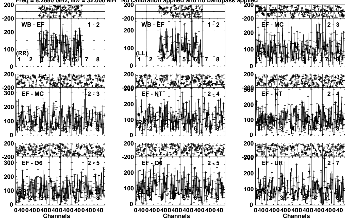
Lower frame: Micro Ampl Jy Top frame: Phas deg Vector averaged cross-power spectrum Several baselines displayed Timerange: 00/21:42:41 to 00/21:44:39
