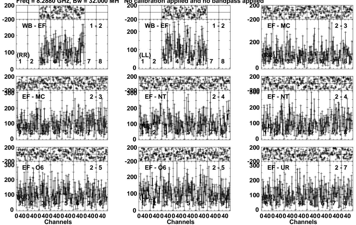
Lower frame: Micro Ampl Jy Top frame: Phas deg Vector averaged cross-power spectrum Several baselines displayed Timerange: 00/21:50:56 to 00/21:52:54
