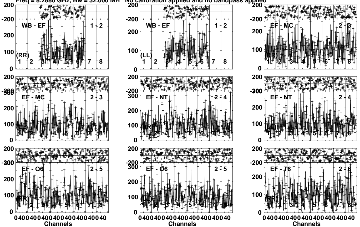
Lower frame: Micro Ampl Jy Top frame: Phas deg Vector averaged cross-power spectrum Several baselines displayed Timerange: 00/18:53:26 to 00/18:55:24
