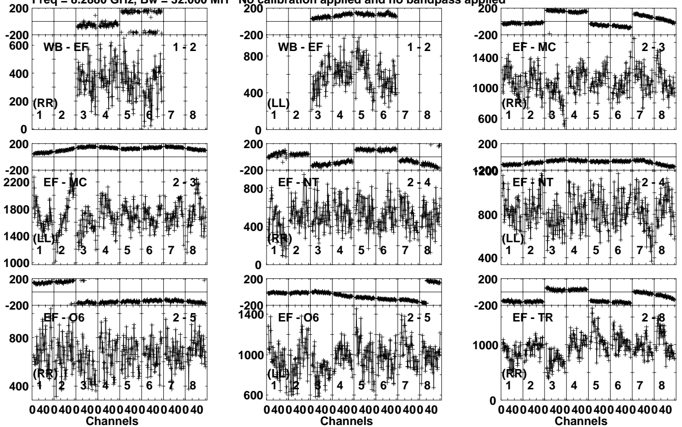
Lower frame: Micro Ampl Jy Top frame: Phas deg Vector averaged cross-power spectrum Several baselines displayed Timerange: 01/01:53:16 to 01/01:54:14
