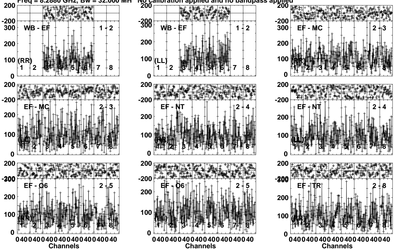
Lower frame: Micro Ampl Jy Top frame: Phas deg Vector averaged cross-power spectrum Several baselines displayed Timerange: 00/23:46:36 to 00/23:48:34
