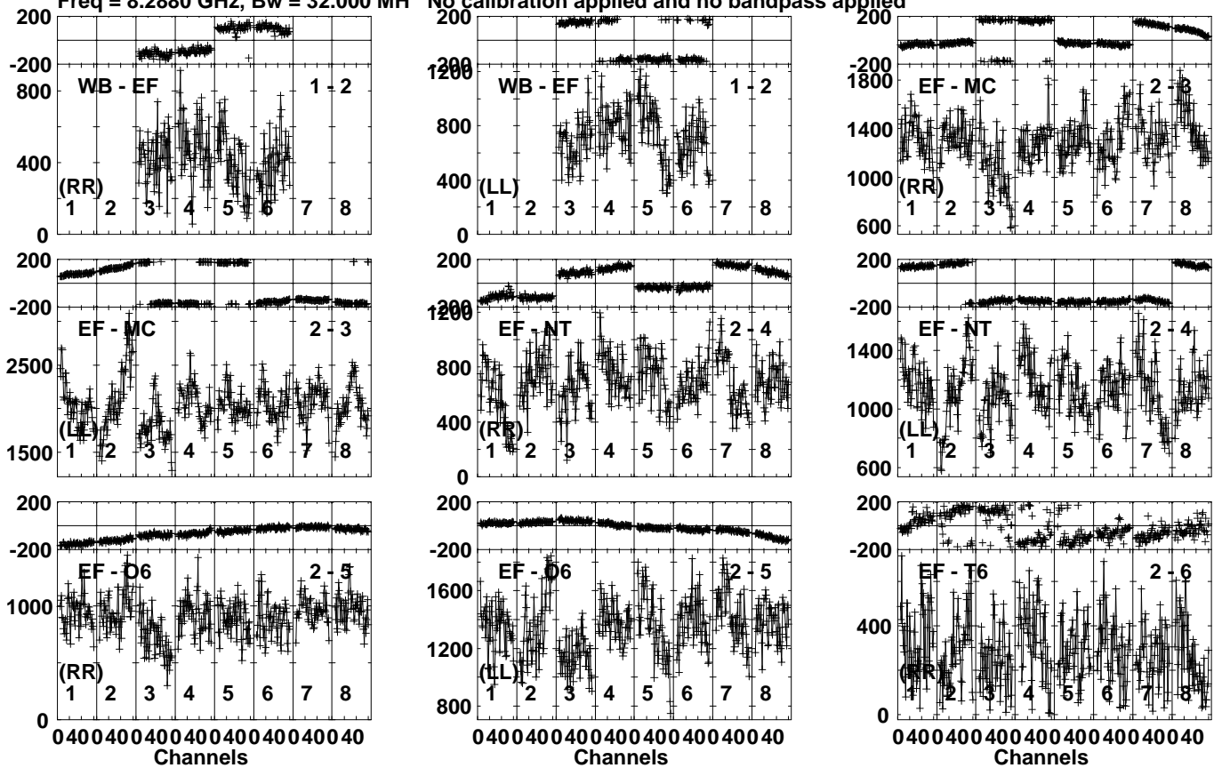
Lower frame: Micro Ampl Jy Top frame: Phas deg Vector averaged cross-power spectrum Several baselines displayed Timerange: 00/19:51:06 to 00/19:52:04
