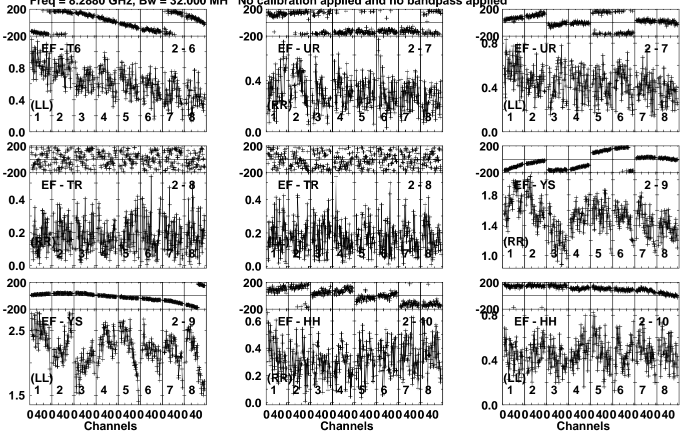
Lower frame: Milli Ampl Jy Top frame: Phas deg Vector averaged cross-power spectrum Several baselines displayed Timerange: 00/18:14:56 to 00/18:15:54
