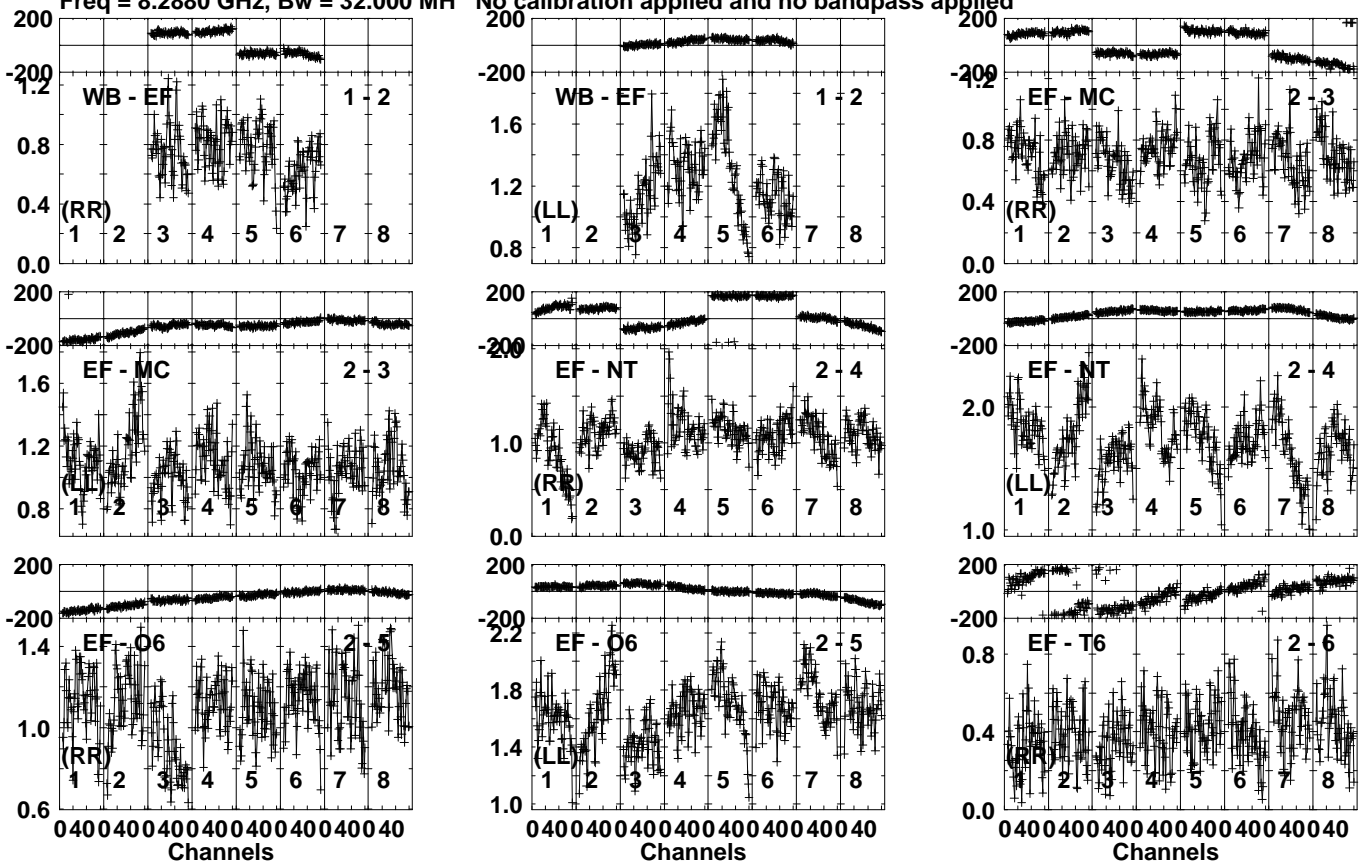
Lower frame: Milli Ampl Jy Top frame: Phas deg Vector averaged cross-power spectrum Several baselines displayed Timerange: 00/19:04:16 to 00/19:05:14
