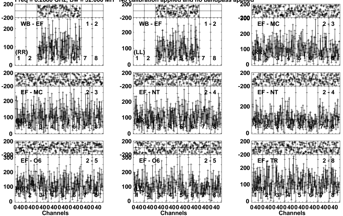
Lower frame: Micro Ampl Jy Top frame: Phas deg Vector averaged cross-power spectrum Several baselines displayed Timerange: 00/23:22:06 to 00/23:24:04
