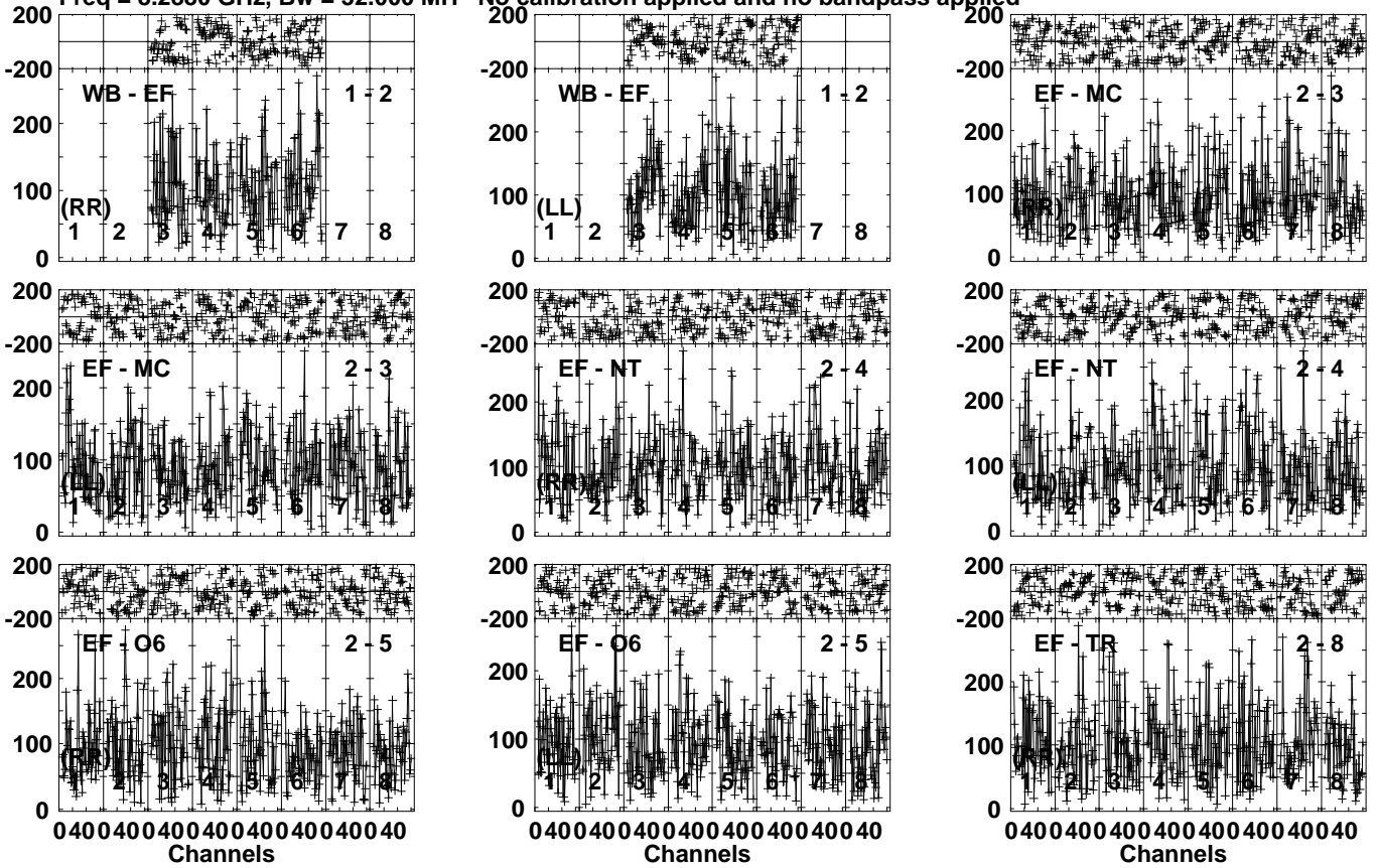
Lower frame: Micro Ampl Jy Top frame: Phas deg Vector averaged cross-power spectrum Several baselines displayed Timerange: 01/01:04:06 to 01/01:06:04
