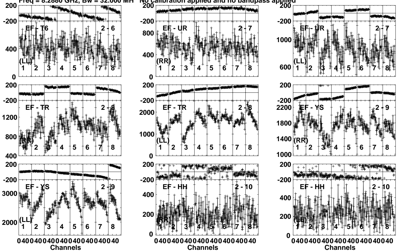
Lower frame: Micro Ampl Jy Top frame: Phas deg Vector averaged cross-power spectrum Several baselines displayed Timerange: 00/19:47:06 to 00/19:48:04
