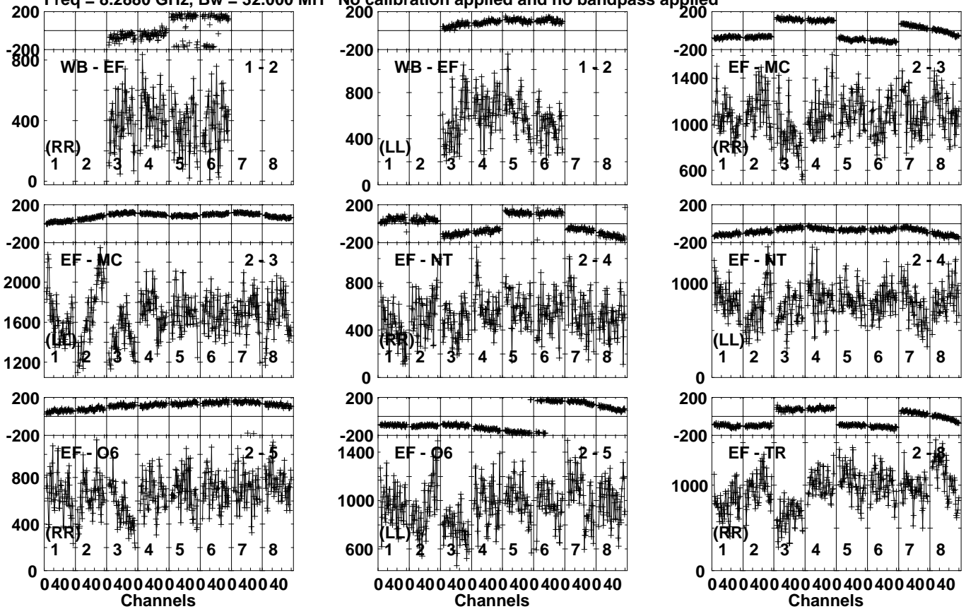
Lower frame: Micro Ampl Jy Top frame: Phas deg Vector averaged cross-power spectrum Several baselines displayed Timerange: 01/01:59:36 to 01/02:00:34
