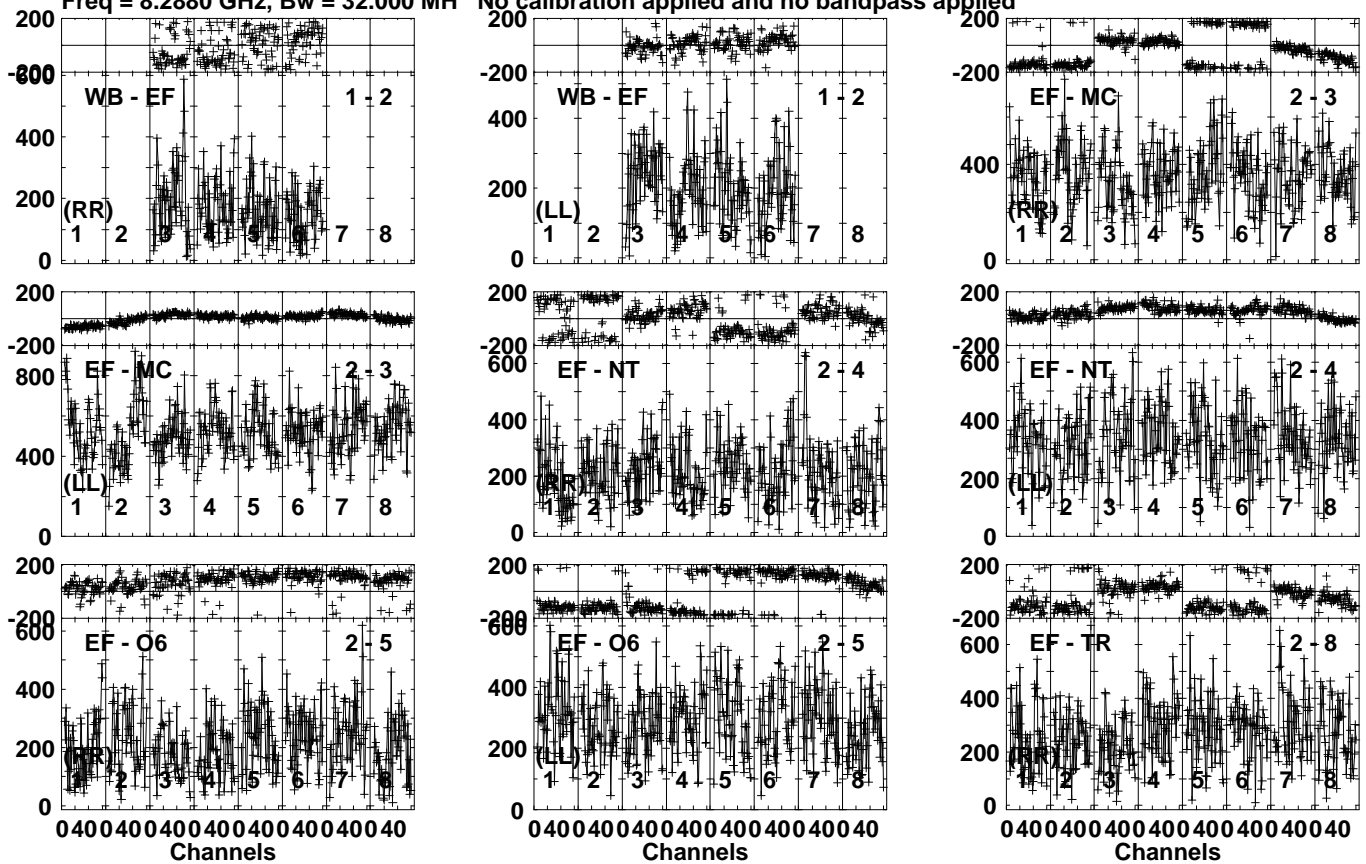
Lower frame: Micro Ampl Jy Top frame: Phas deg Vector averaged cross-power spectrum Several baselines displayed Timerange: 01/01:28:36 to 01/01:29:34
