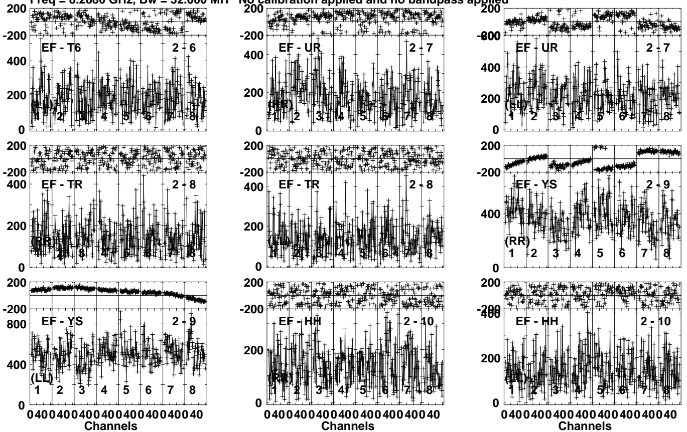
Lower frame: Micro Ampl Jy Top frame: Phas deg Vector averaged cross-power spectrum Several baselines displayed Timerange: 00/16:56:21 to 00/16:57:19
