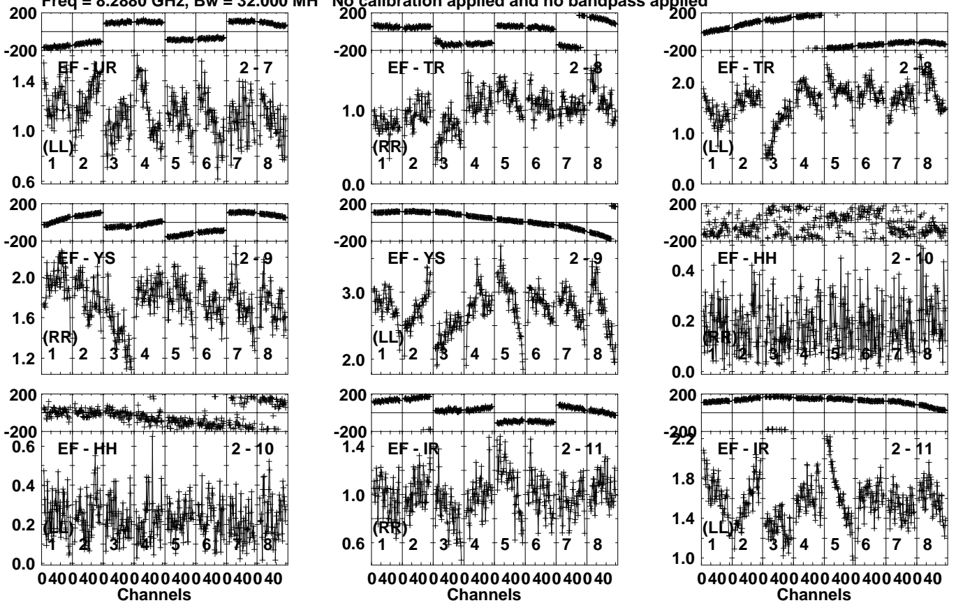
Lower frame: Milli Ampl Jy Top frame: Phas deg Vector averaged cross-power spectrum Several baselines displayed Timerange: 00/21:45:11 to 00/21:46:09
