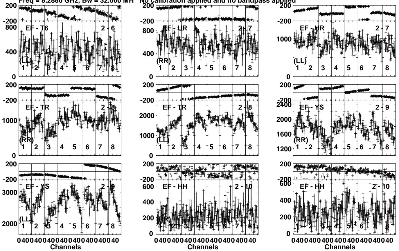
Lower frame: Micro Ampl Jy Top frame: Phas deg Vector averaged cross-power spectrum Several baselines displayed Timerange: 00/20:03:26 to 00/20:04:24
