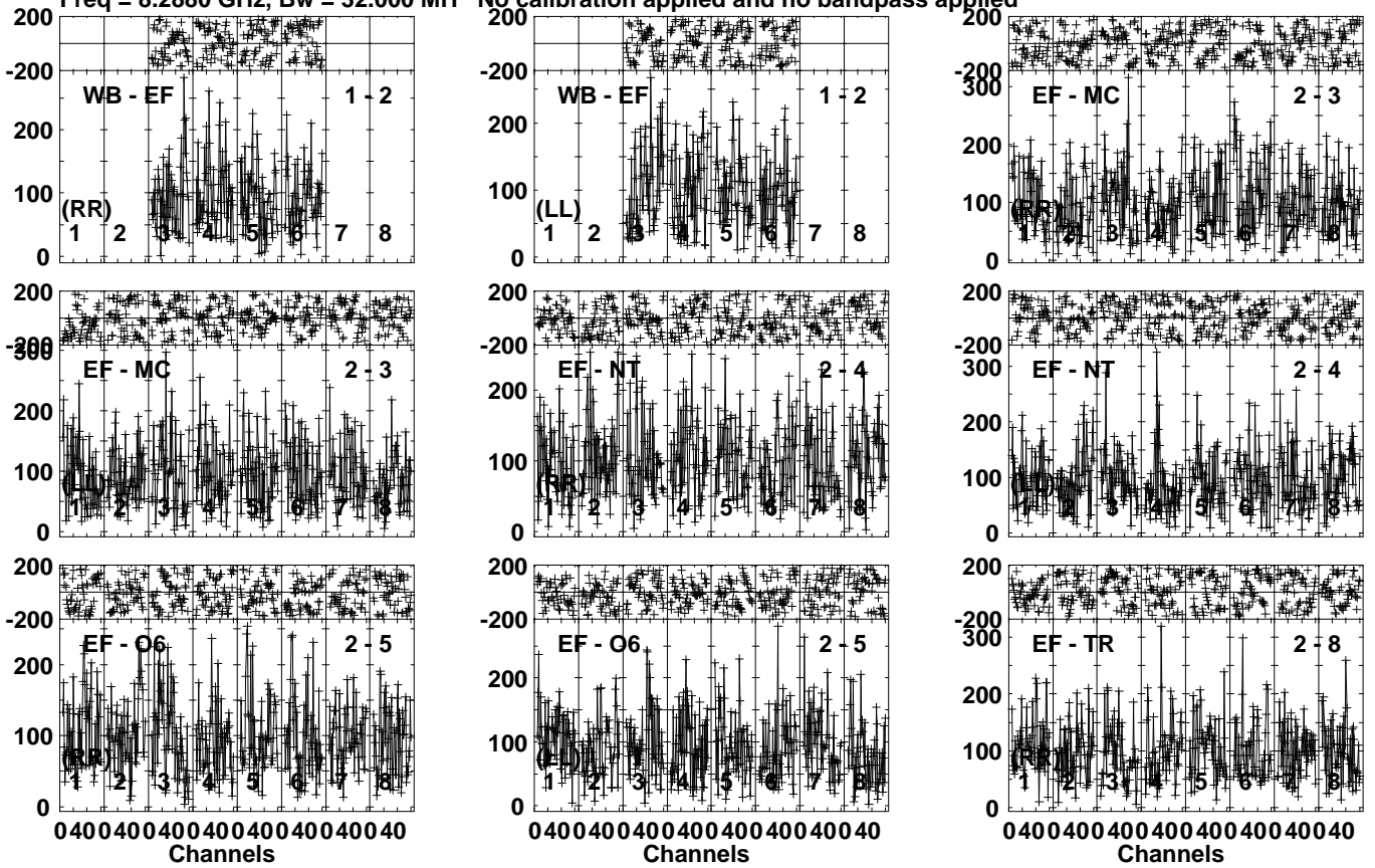
Lower frame: Micro Ampl Jy Top frame: Phas deg Vector averaged cross-power spectrum Several baselines displayed Timerange: 00/23:05:51 to 00/23:07:49
