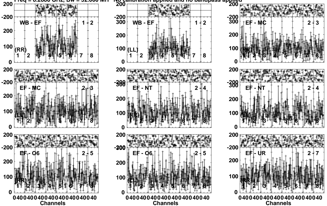
Lower frame: Micro Ampl Jy Top frame: Phas deg Vector averaged cross-power spectrum Several baselines displayed Timerange: 00/22:19:11 to 00/22:21:09
