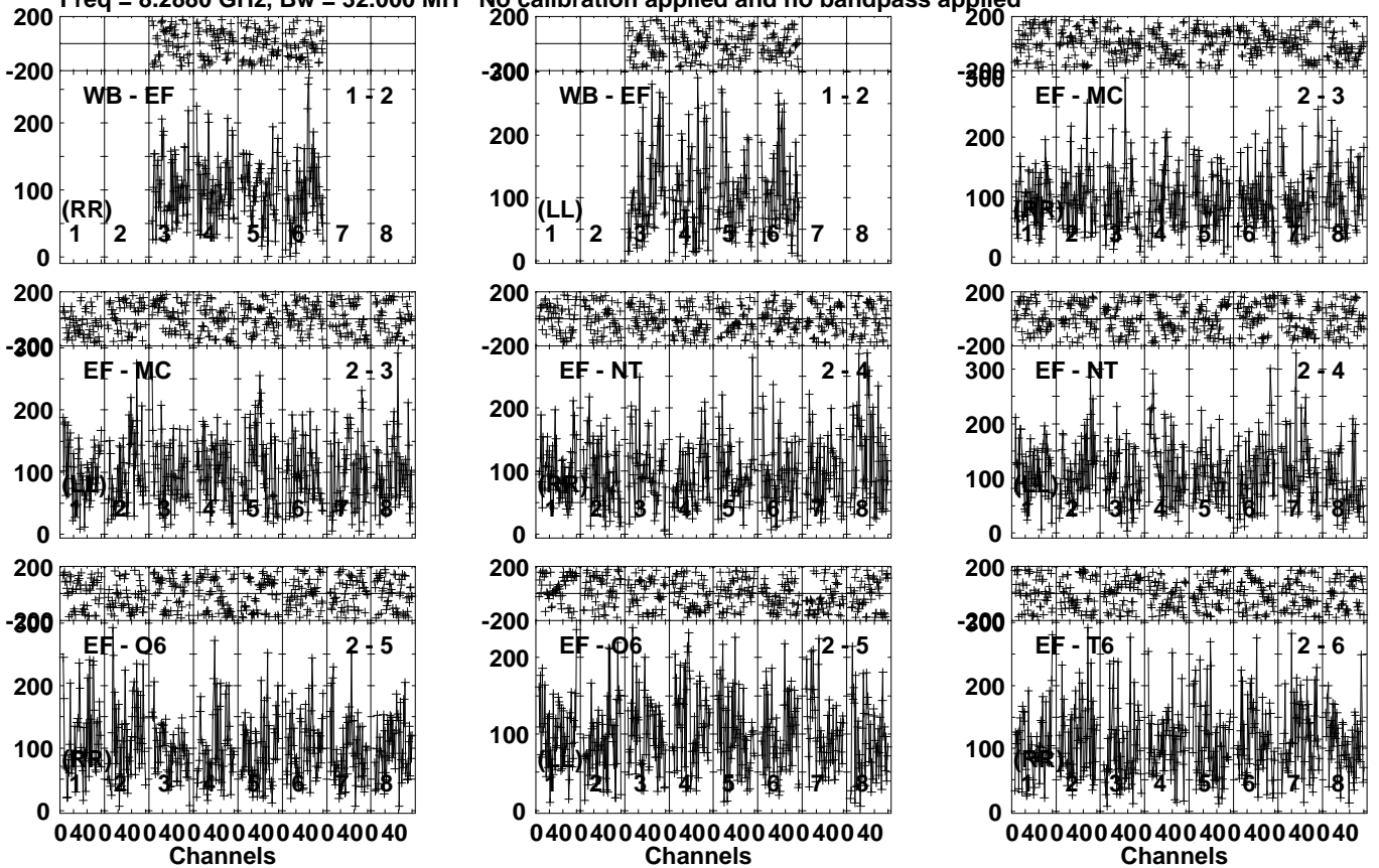
Lower frame: Micro Ampl Jy Top frame: Phas deg Vector averaged cross-power spectrum Several baselines displayed Timerange: 00/17:29:41 to 00/17:31:39
