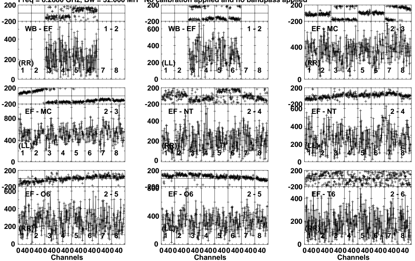
Lower frame: Micro Ampl Jy Top frame: Phas deg Vector averaged cross-power spectrum Several baselines displayed Timerange: 00/16:52:06 to 00/16:53:04
