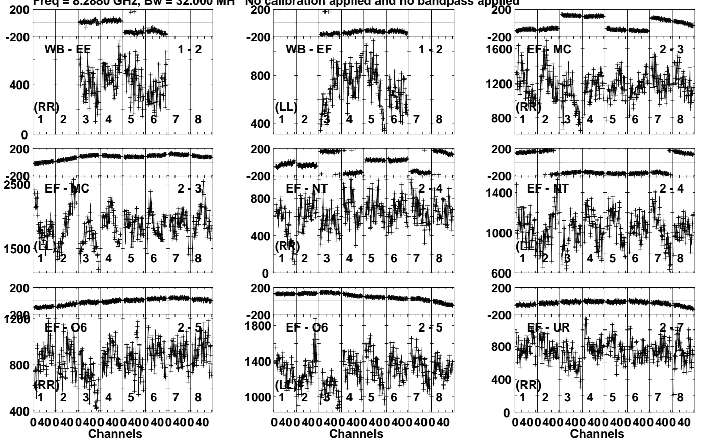
Lower frame: Micro Ampl Jy Top frame: Phas deg Vector averaged cross-power spectrum Several baselines displayed Timerange: 00/22:25:56 to 00/22:26:54
