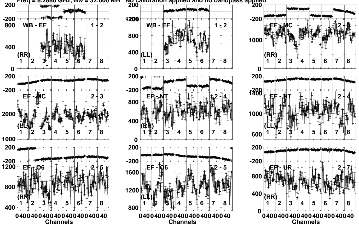
Lower frame: Micro Ampl Jy Top frame: Phas deg Vector averaged cross-power spectrum Several baselines displayed Timerange: 00/21:37:11 to 00/21:38:09
