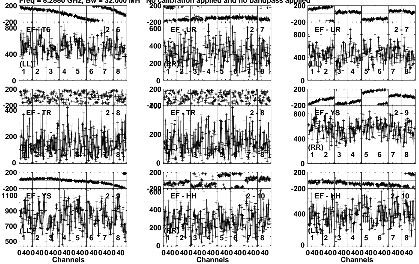
Lower frame: Micro Ampl Jy Top frame: Phas deg Vector averaged cross-power spectrum Several baselines displayed Timerange: 00/17:57:11 to 00/17:58:09
