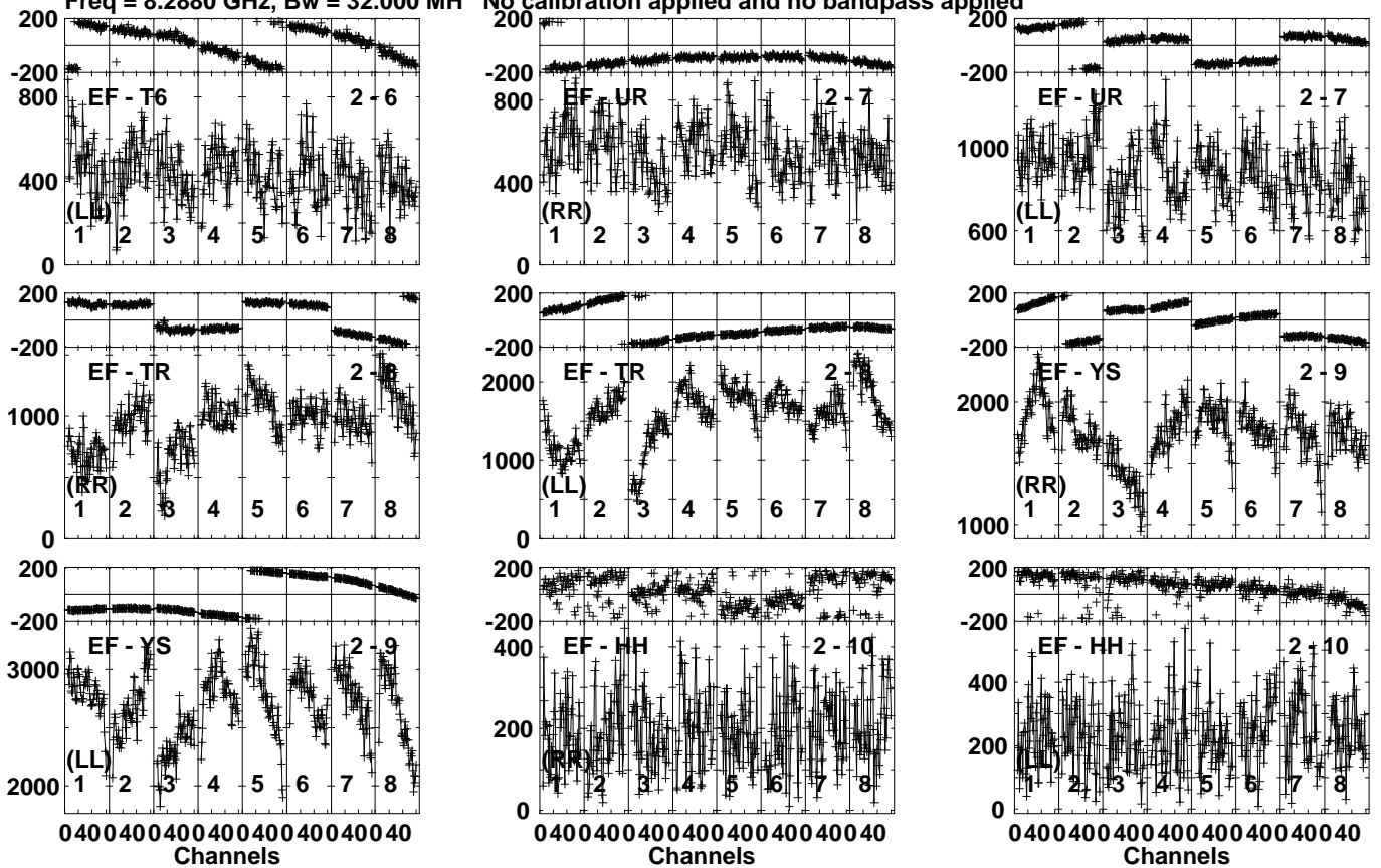
Lower frame: Micro Ampl Jy Top frame: Phas deg Vector averaged cross-power spectrum Several baselines displayed Timerange: 00/19:59:26 to 00/20:00:24
