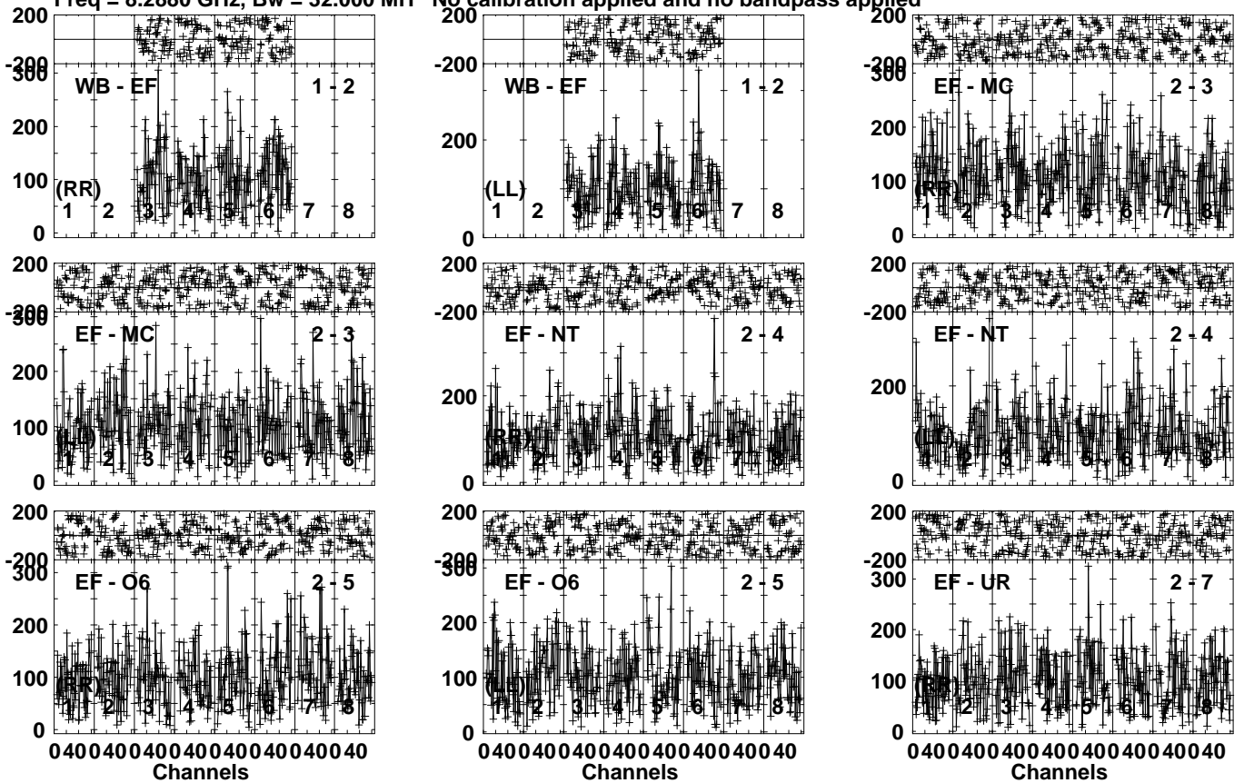
Lower frame: Micro Ampl Jy Top frame: Phas deg Vector averaged cross-power spectrum Several baselines displayed Timerange: 00/21:38:41 to 00/21:40:39
