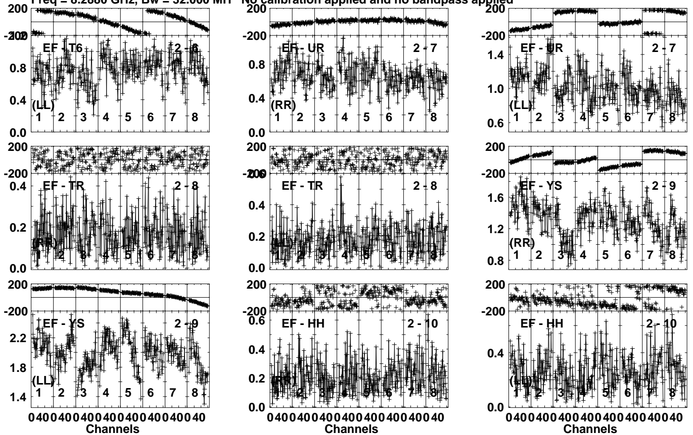
Lower frame: Milli Ampl Jy Top frame: Phas deg Vector averaged cross-power spectrum Several baselines displayed Timerange: 00/19:16:36 to 00/19:17:34
