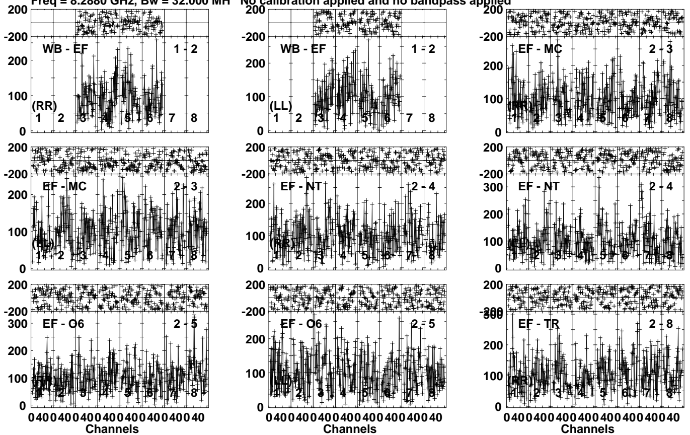
Lower frame: Micro Ampl Jy Top frame: Phas deg Vector averaged cross-power spectrum Several baselines displayed Timerange: 00/23:58:51 to 01/00:00:49
